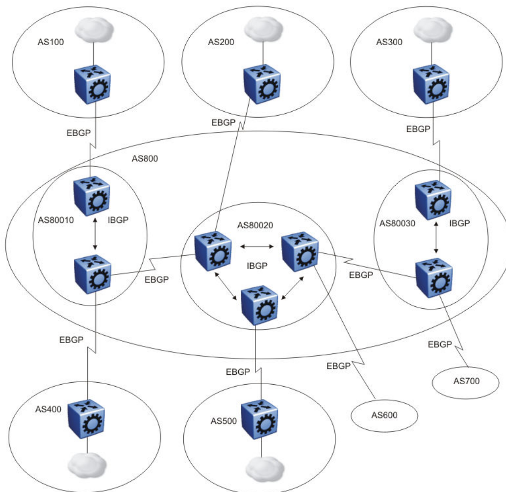
Figure 28: Confederations
