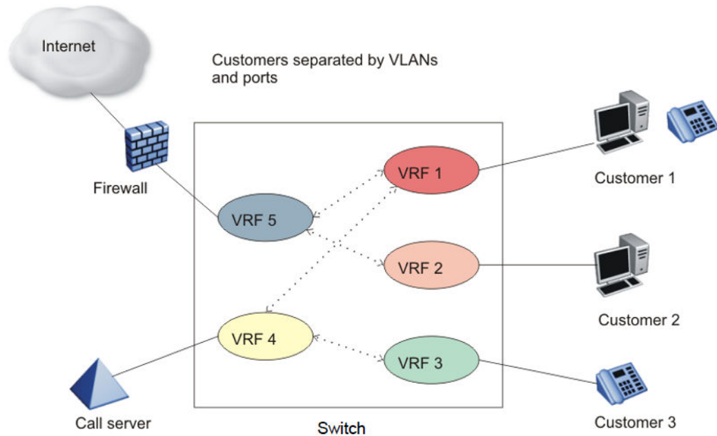
Figure 253: Inter-VRF forwarding
