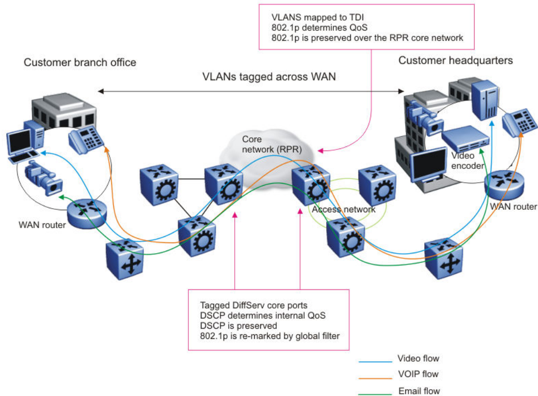
Figure 206: RPR QoS internetworking
