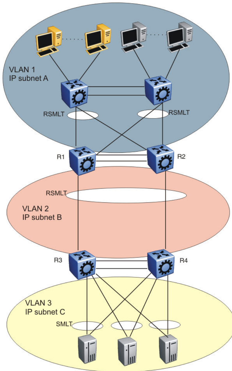
Figure 220: SMLT and RSMLT in Layer 3 environments
