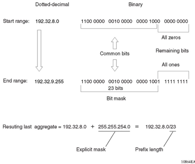
Figure 26: Last aggregate and prefix length
