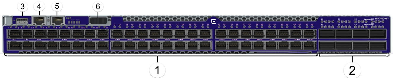
Figure 263: VSP 7400-48Y
