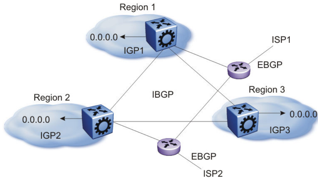
Figure 40: Multiple regions separated by iBGP
