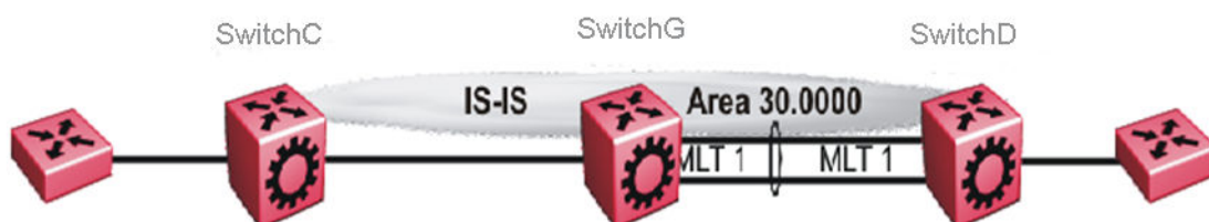
Figure 67: IS-IS SPBM global
