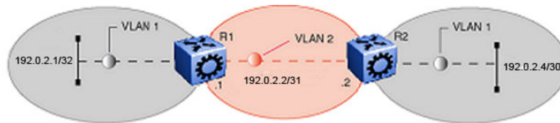
Figure 157: IP routing between VLANs
