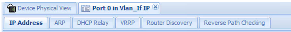
Figure 16: Menu bar
