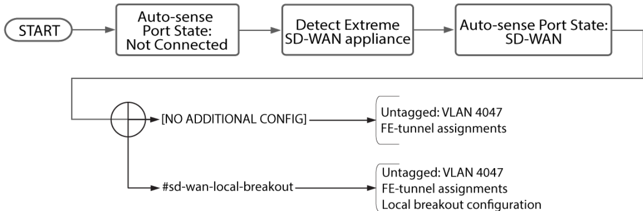
Figure 12: Auto-sense SD-WAN
