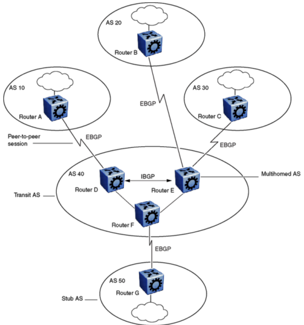
Figure 22: BGP networks
