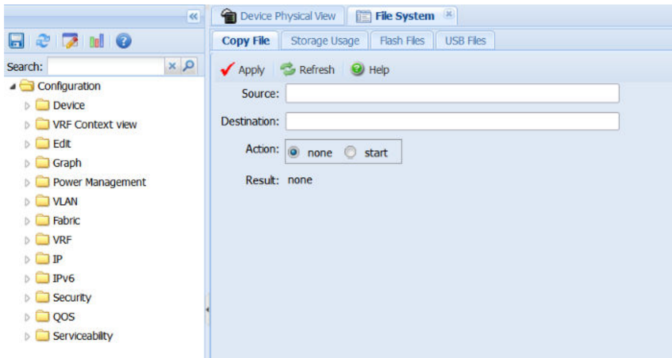
Figure 15: EDM window
