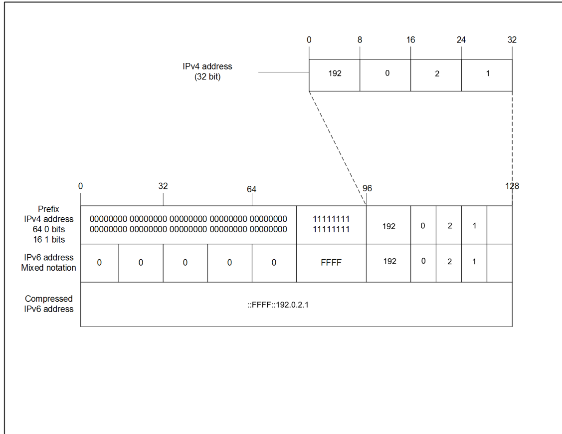
Figure 43: IPv4-mapped IPv6 address components
