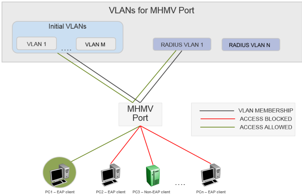
Figure 61: MHHM - authenticated client
