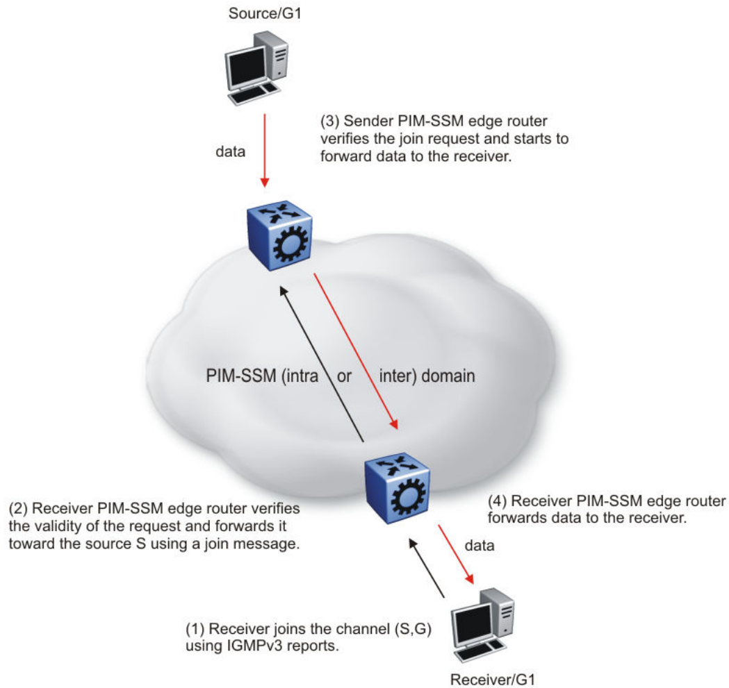
Figure 133: PIM-SSM architecture
