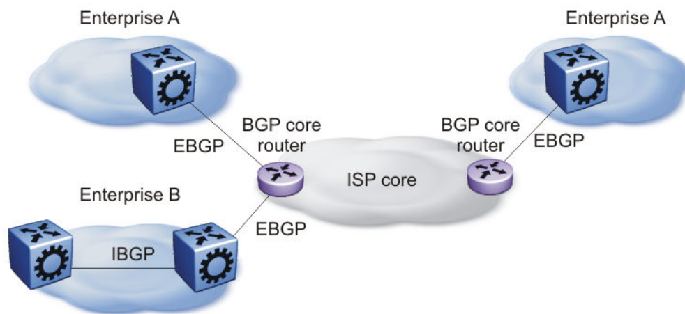
Figure 39: BGP and edge aggregation
