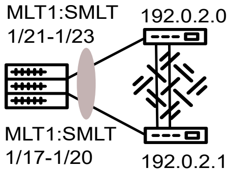
Figure 84: FA configuration in dual-homed SMLT
