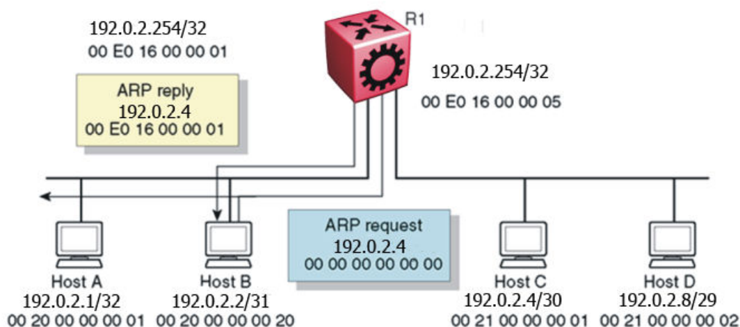
Figure 19: Proxy ARP operation
