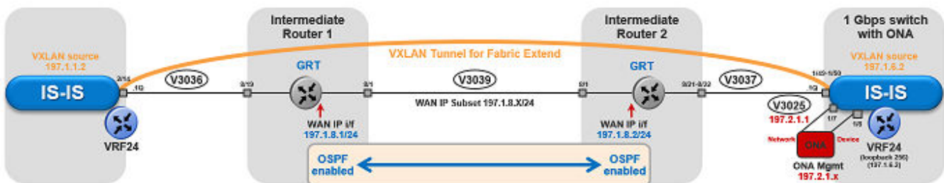
Figure 77: IP (VRF) traffic flow component view
