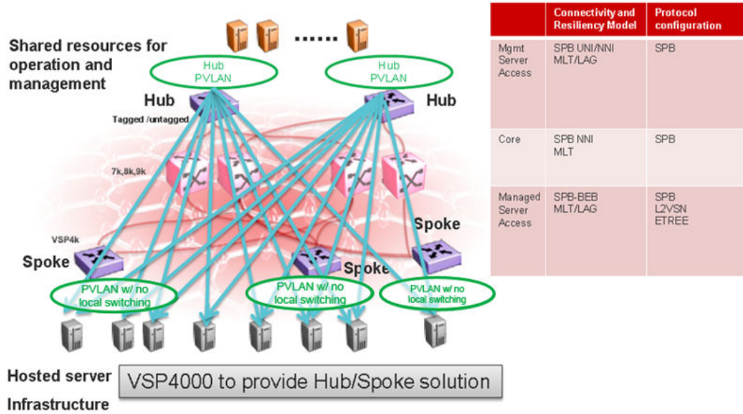
Figure 122: Data center hosting private VLAN
