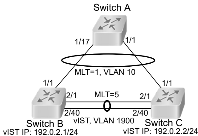
Figure 199: Network topology for traffic flow example
