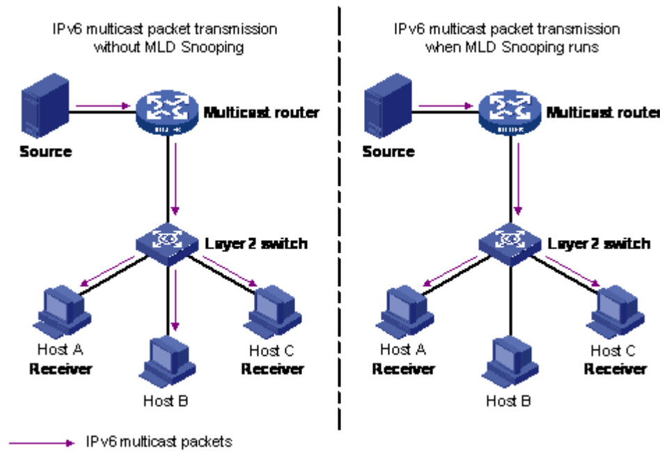
Figure 155: IPv6 multicast packet transmission when MLD snooping is enabled and not enabled
