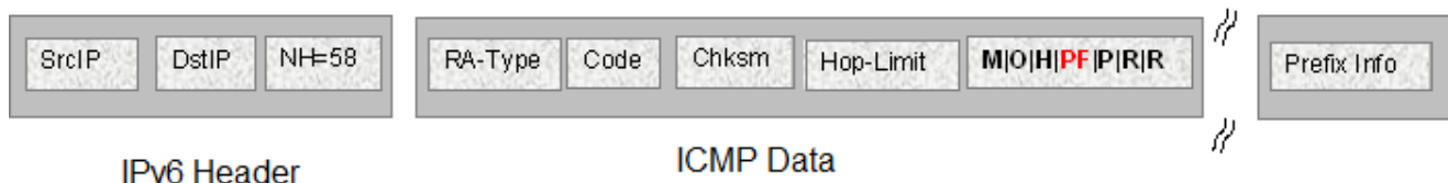
Figure 191: IPv6 ICMP RA data packet outline for router preference validation
