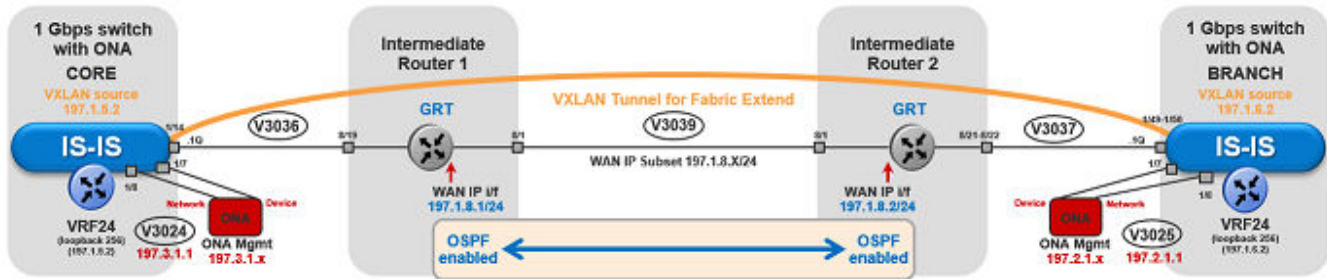
Figure 82: Fabric Extend traffic flow component view
