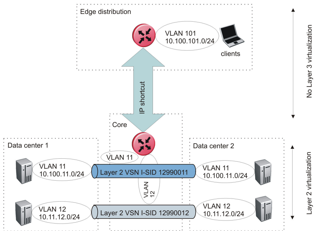
Figure 114: IP shortcut scenario to move traffic between data centers
