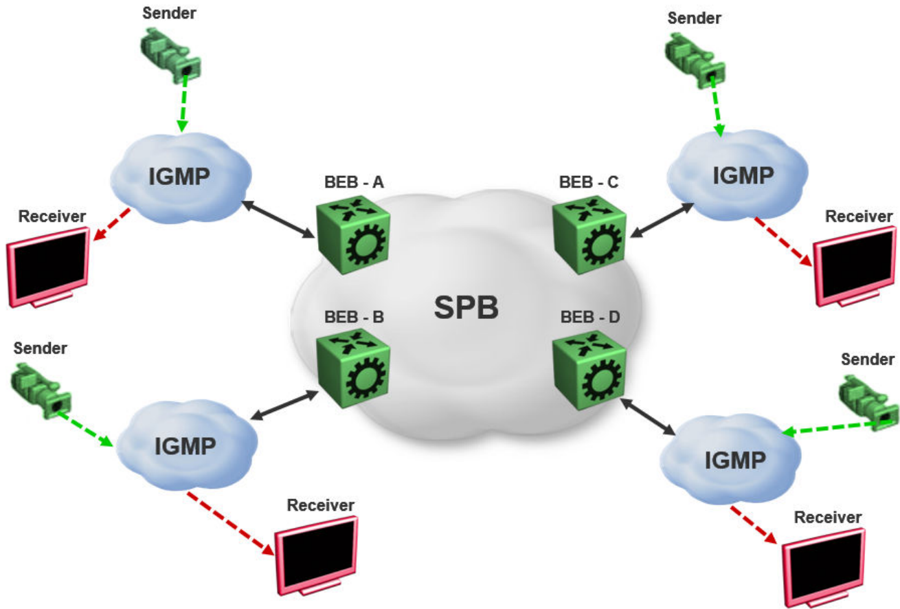
Figure 241: IP Multicast over Fabric Connect streams
