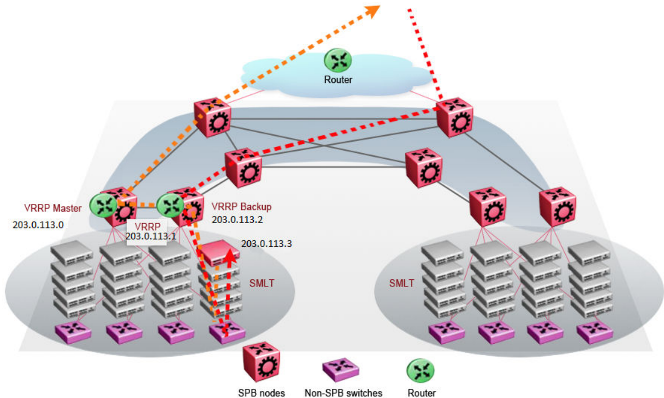
Figure 117: Traditional routing before moving VMs
