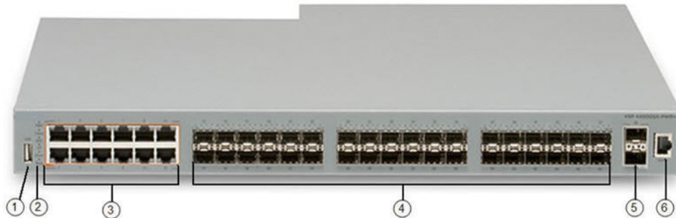
Figure 280: VSP 4450GSX-DC
