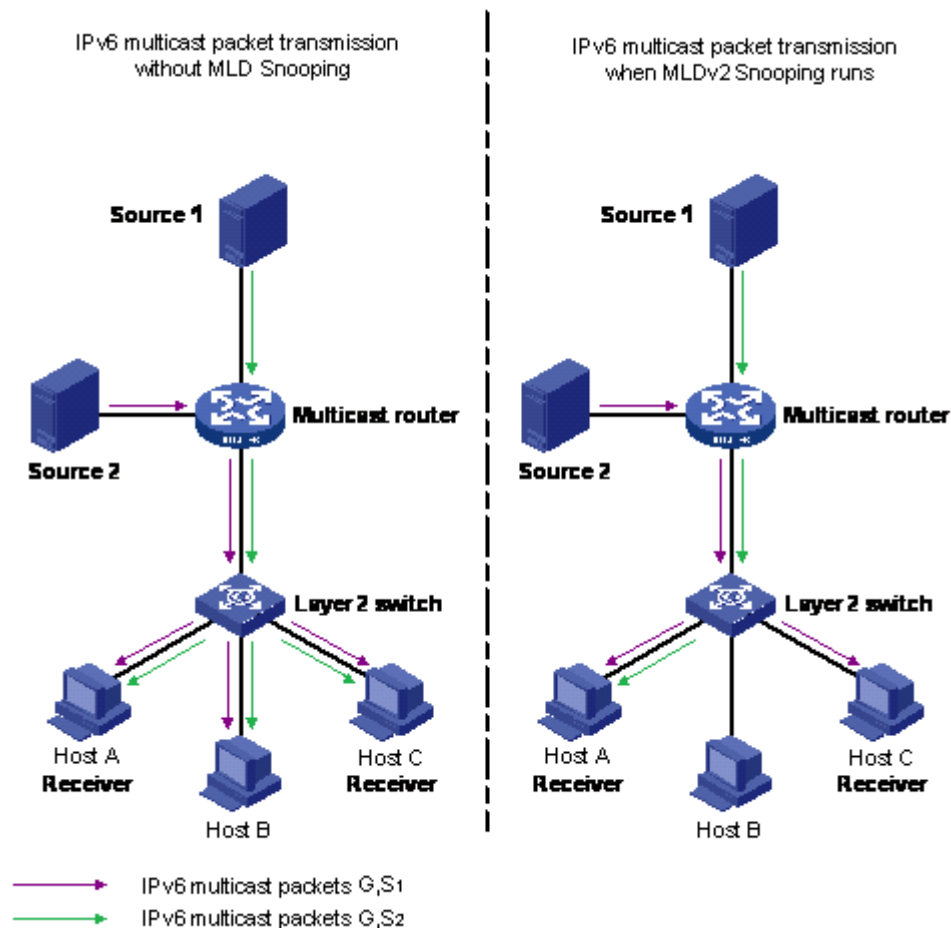
Figure 156: IPv6 multicast packet transmission when MLD v2 snooping is enabled and not enabled
