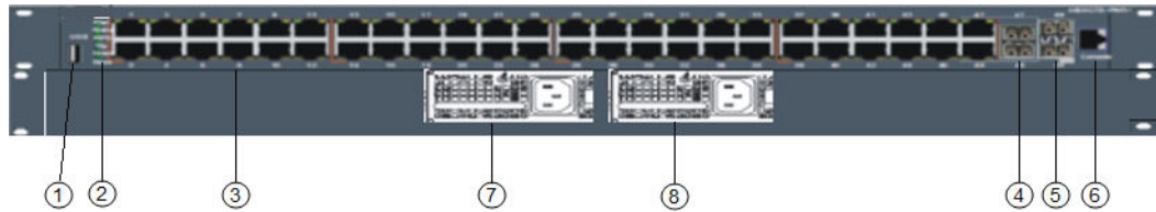
Figure 279: VSP 4450GTX-HT-PWR+
