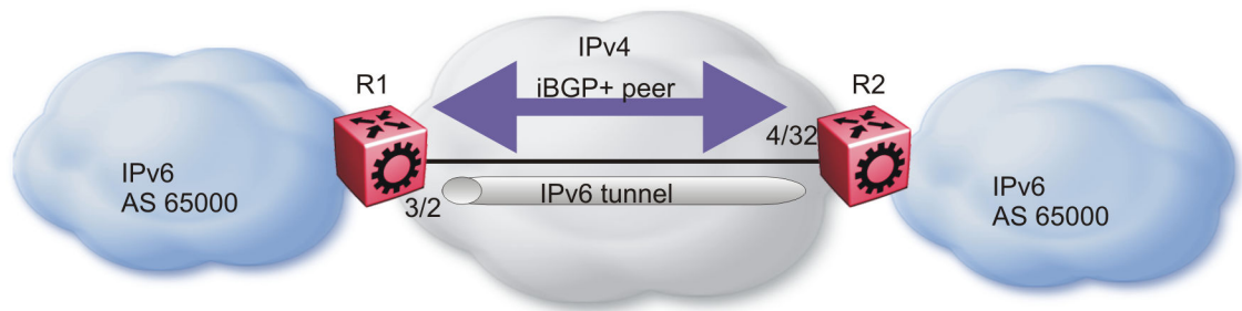
Figure 43: iBGP+ peers on CLIP interfaces with IPv6 tunneling
