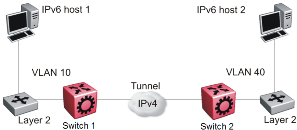
Figure 180: Tunnel configuration between router ports
