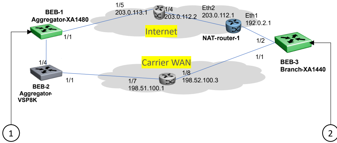
Figure 165: IPsec NAT-T with NAT router on one side
