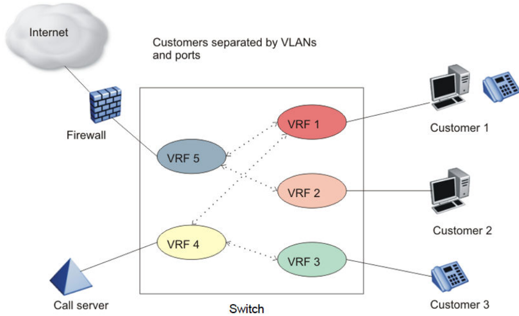
Figure 268: Inter-VRF forwarding
