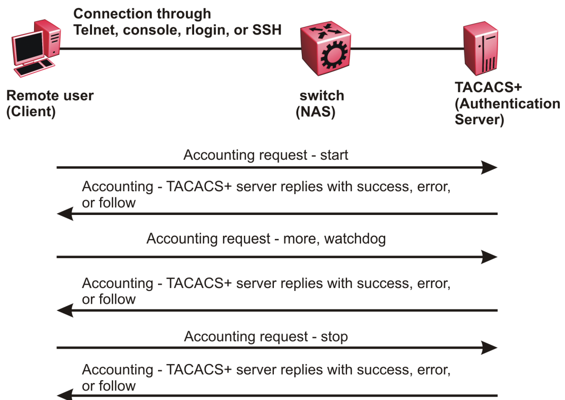
Figure 253: Accounting process
