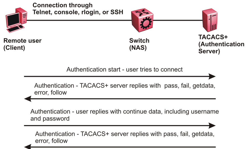
Figure 251: Authentication process
