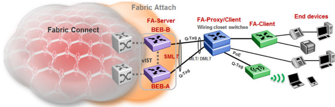
Figure 89: FA in a dual-homed SMLT deployment
