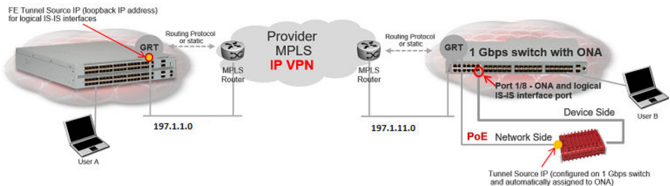
Figure 74: IP using GRT traffic flow
