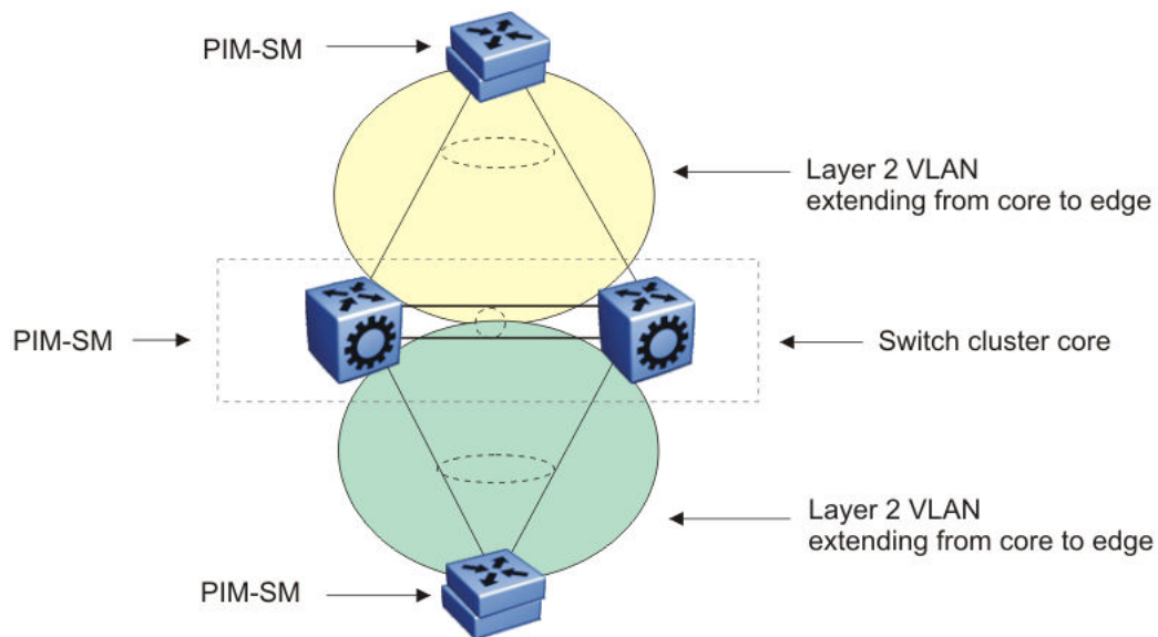
Figure 150: Multicast SMLT triangle
