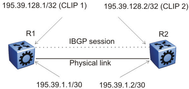
Figure 170: Routers with iBGP connections
