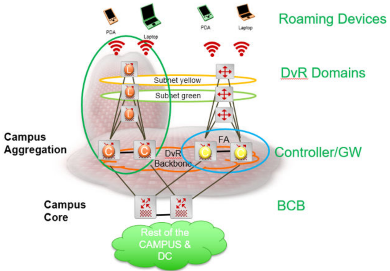
Figure 53: Wireless roaming in Campus
