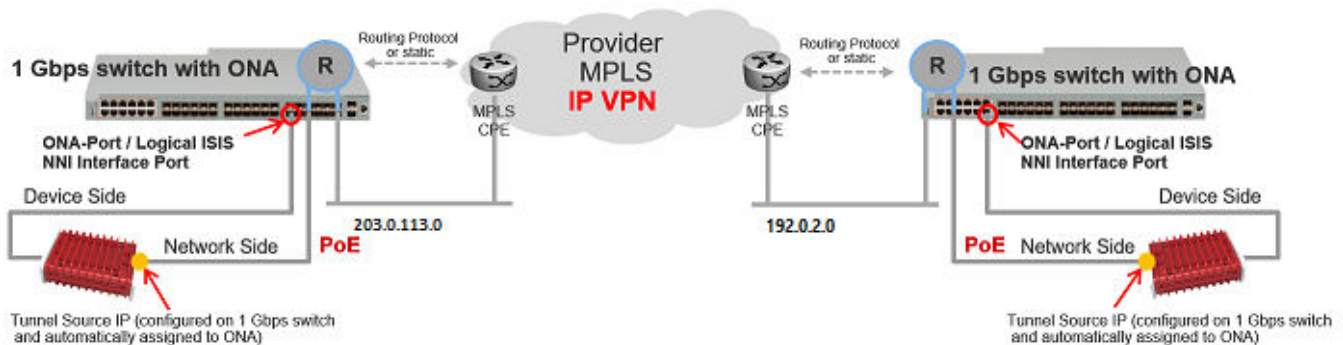
Figure 81: Fabric Extend traffic flow
