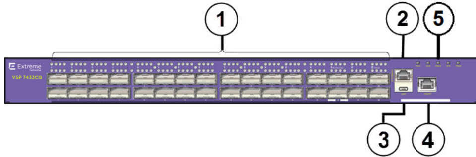
Figure 281: VSP 7432CQ
