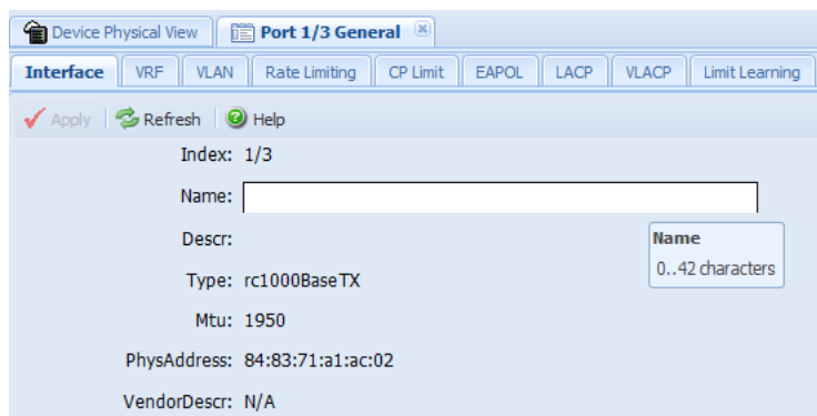
Figure 16: Content pane
