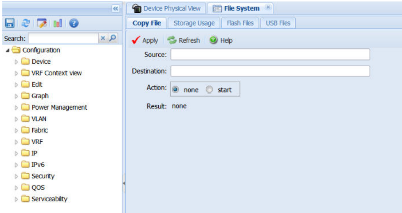
Figure 13: EDM window
