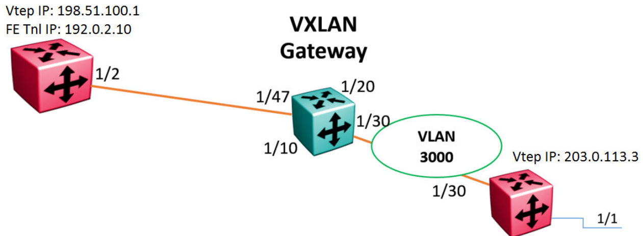
Figure 277: VXLAN Gateway configuration example
