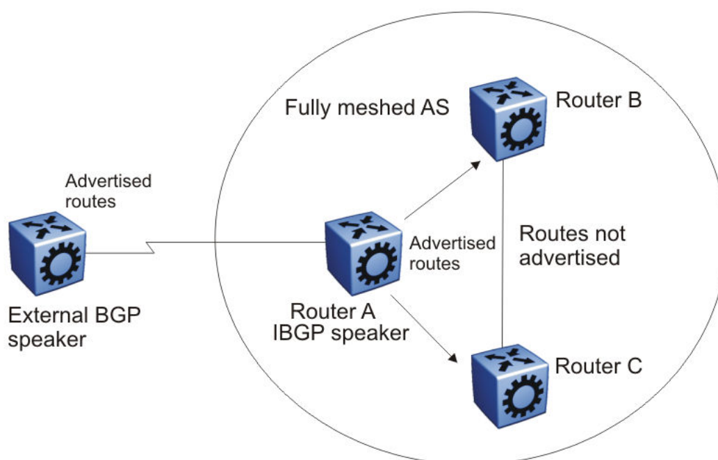
Figure 27: Fully meshed AS with iBGP speakers
