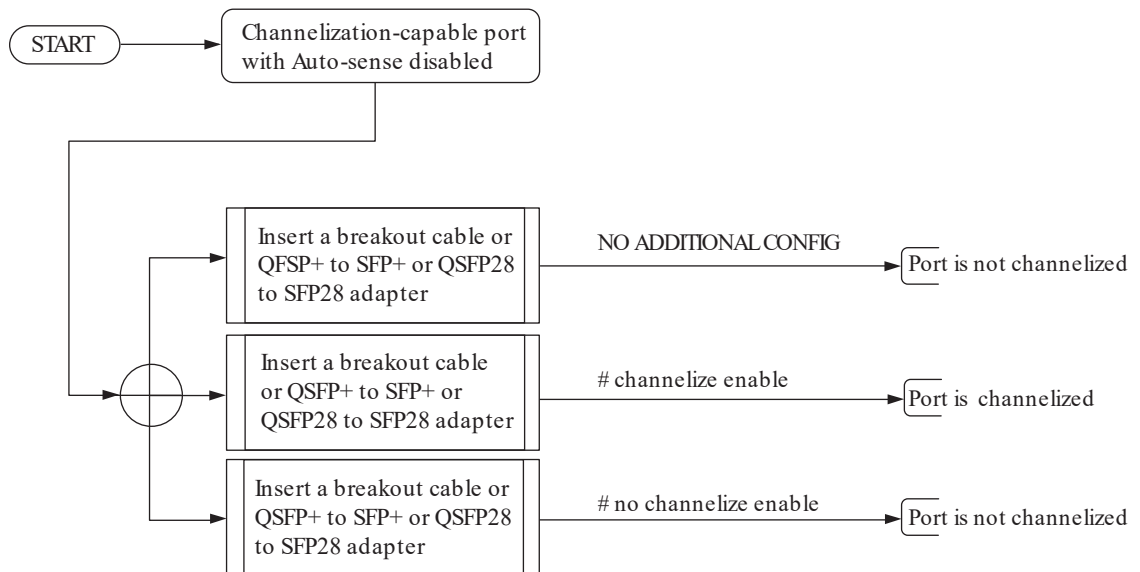
Figure 10: Automatic Channelization with Auto-sense disabled
