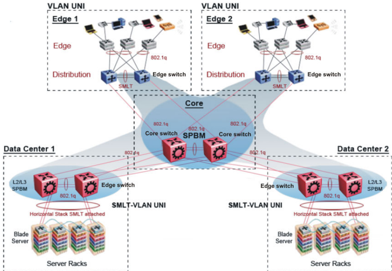
Figure 113: SPBM campus without SMLT
