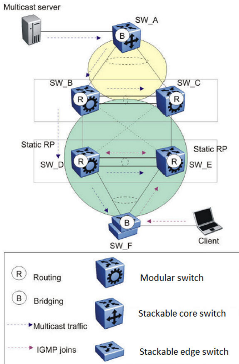
Figure 148: Multicast behavior in SMLT environment
