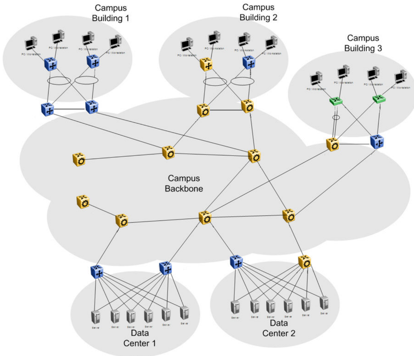
Figure 127: SPBM IP shortcuts in a campus
