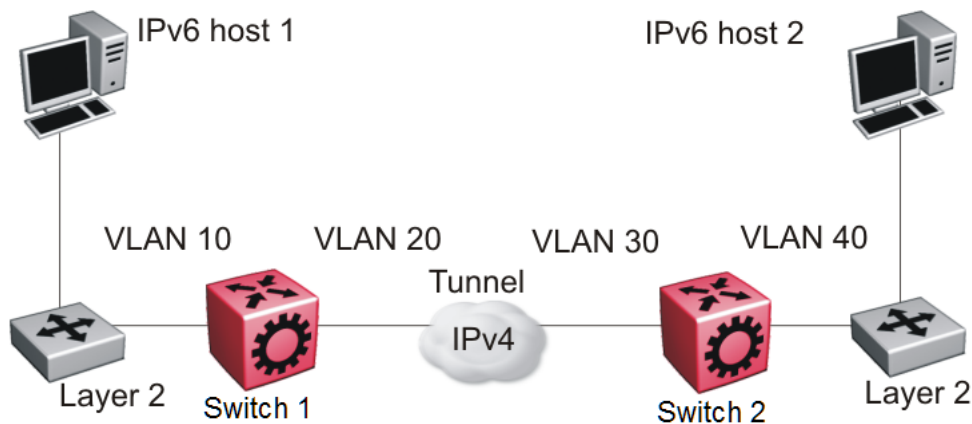
Figure 181: Tunnel configuration between VLANs
