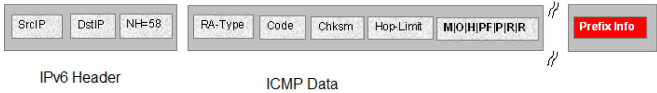
Figure 187: IPv6 ICMP RA Data Packet Outline
