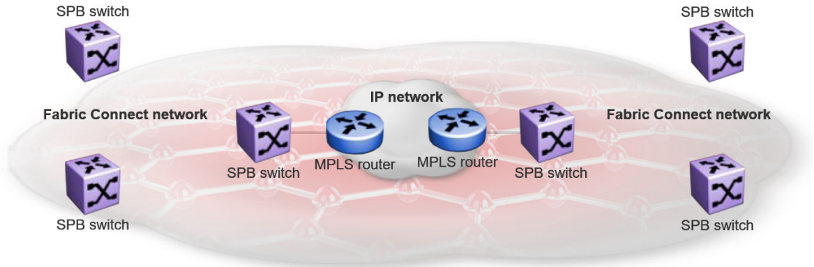
Figure 72: Fabric Extend over IPsec Deployment Option
