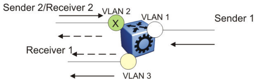
Figure 142: Data flow using deny-both policy
