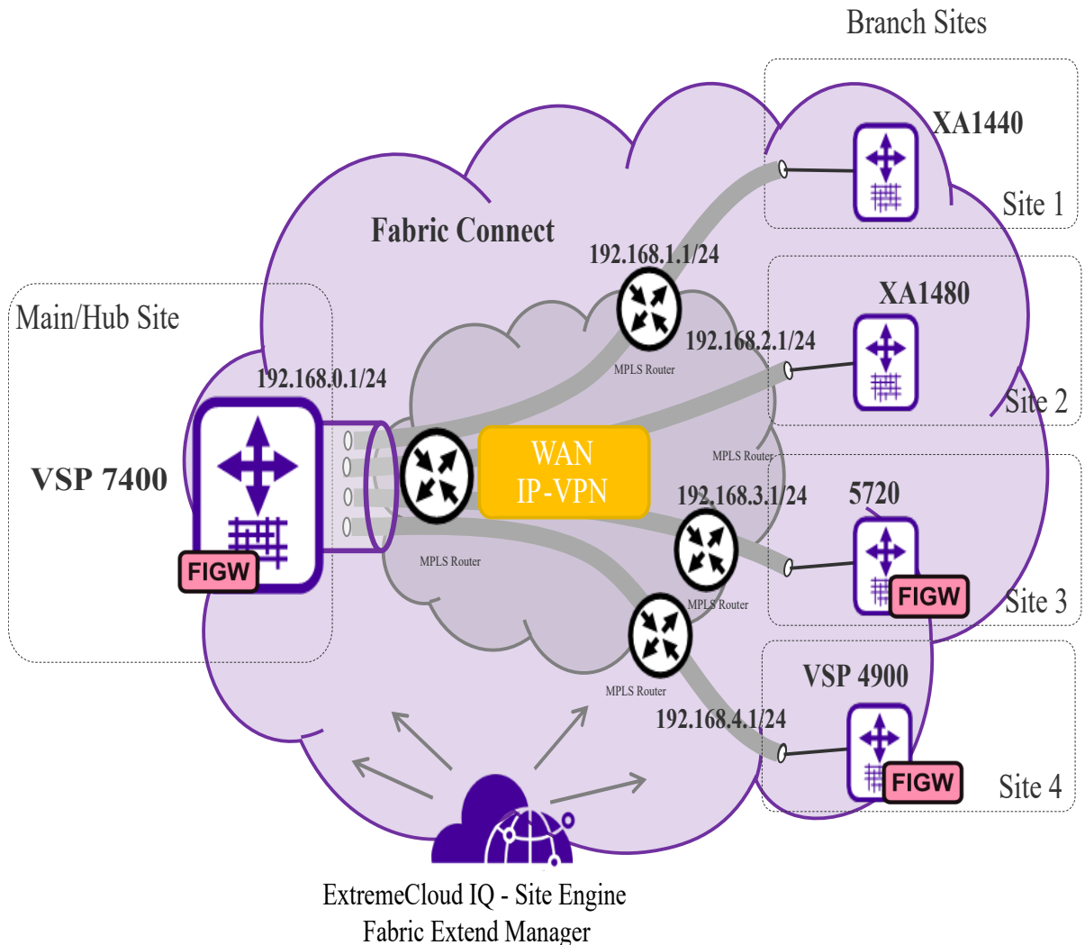
Figure 68: Fabric Extend IP VPN Deployment Option
