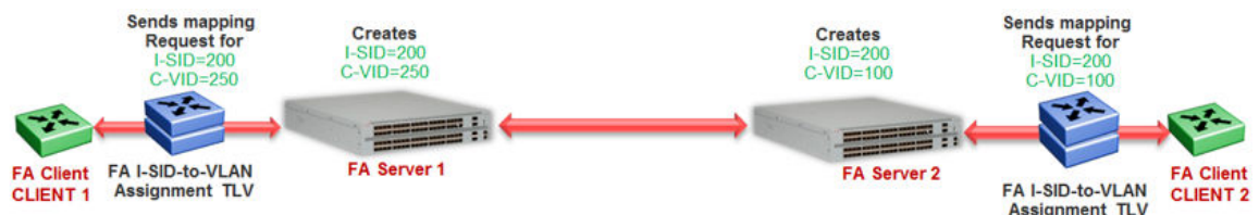
Figure 86: Learning of I-SID-to-VLAN mappings
