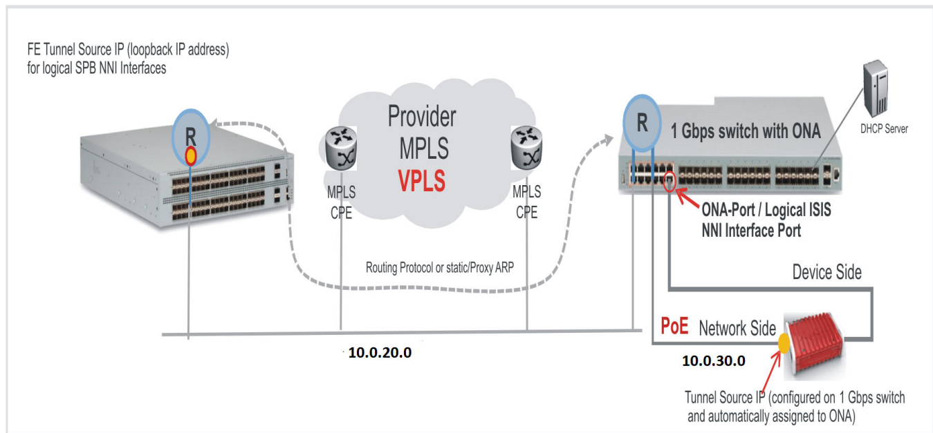
Figure 78: FE over VPLS traffic flow
