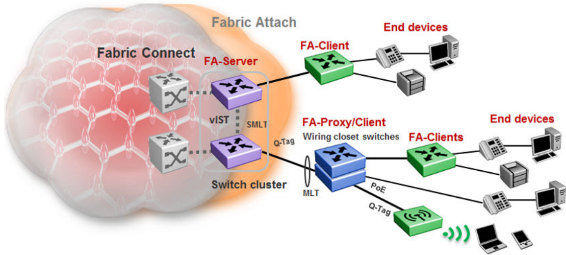
Figure 90: Fabric Attach in a single-homed SMLT deployment
