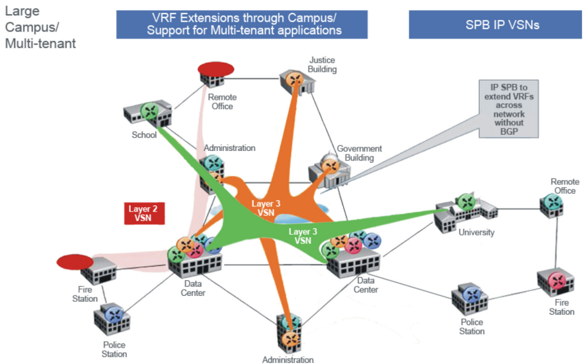
Figure 57: Multi-tenant SPBM metro network
