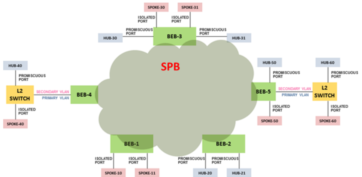
Figure 60: Sample E-Tree configuration
