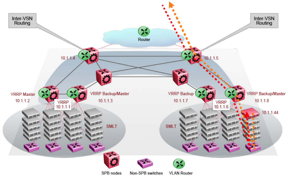
Figure 120: Optimized routing after moving VMs
