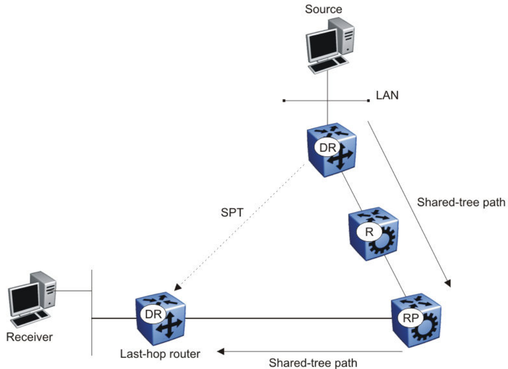
Figure 143: Shared tree and shortest-path tree
