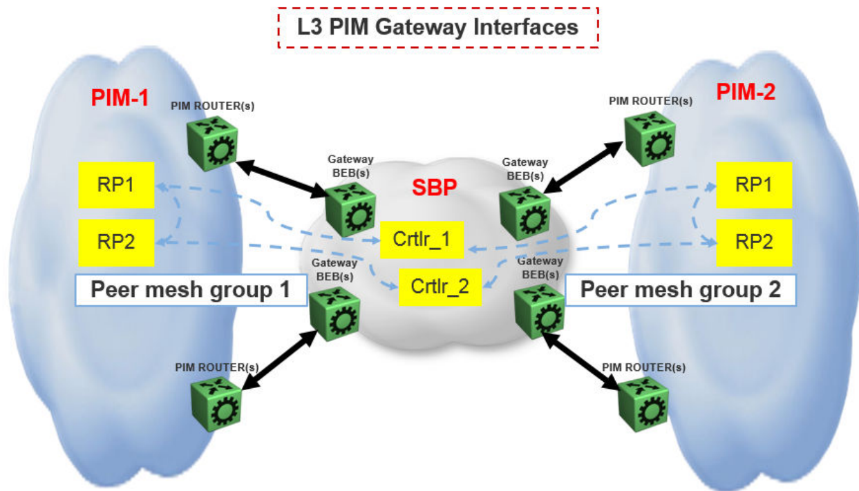
Figure 248: Multi domain configuration
