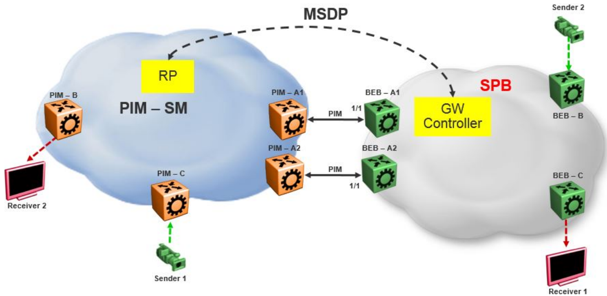
Figure 245: SPB-PIM Gateway base case configuration
