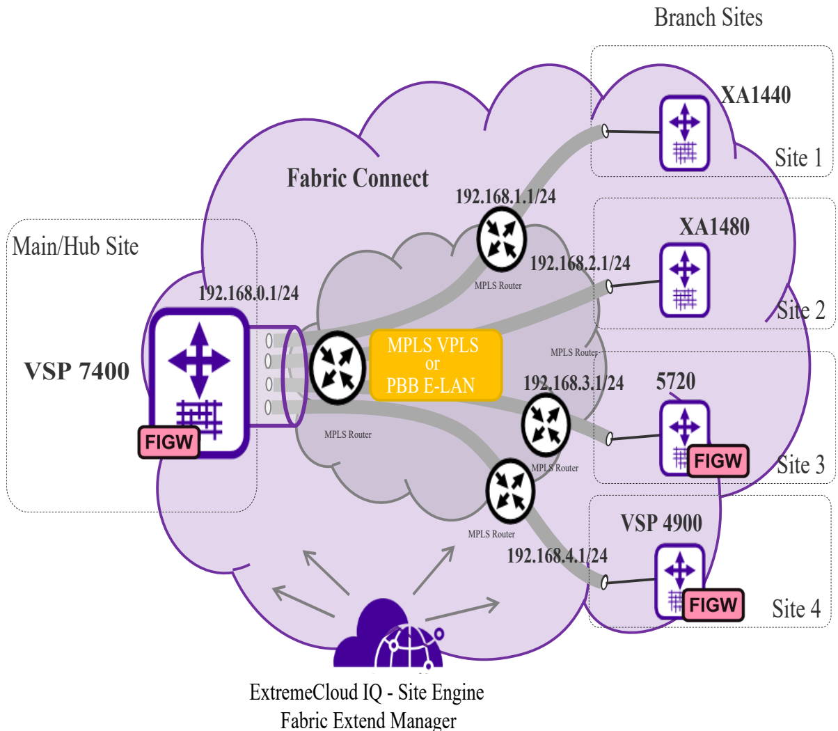
Figure 69: Fabric Extend VPLS Deployment Option
