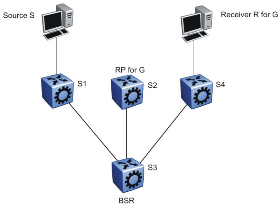
Figure 144: PIM-SM simplified example
