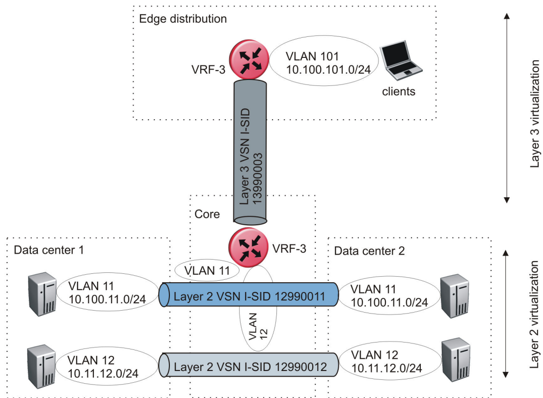
Figure 115: VRF scenario to move traffic between data centers
