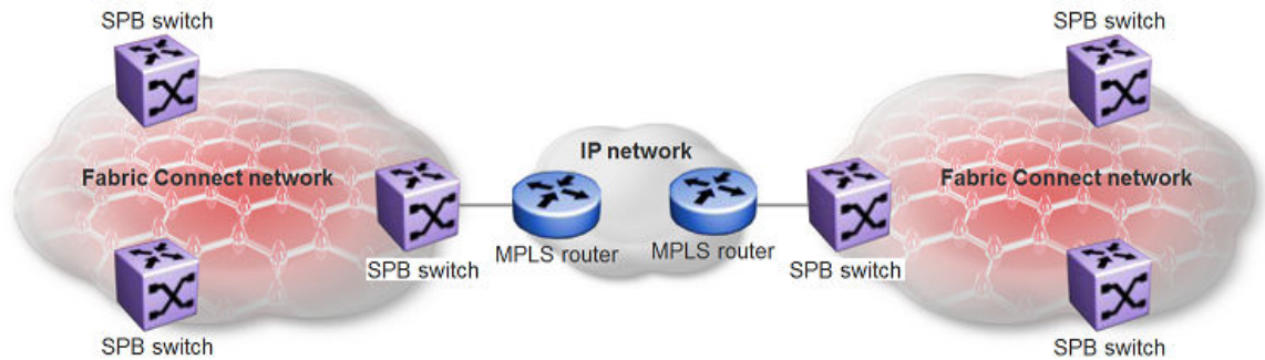
Figure 64: Fabric Connect networks connected by an IP network
