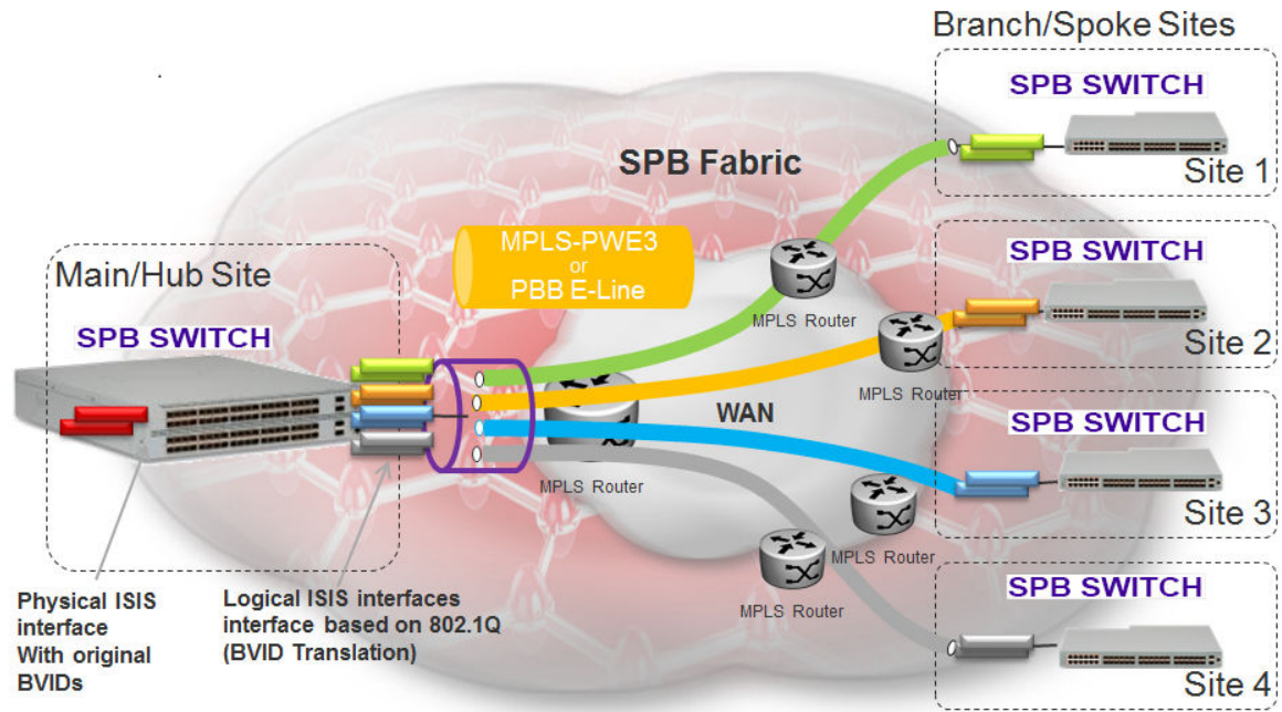
Figure 71: Fabric Extend Pseudowire Deployment Option
