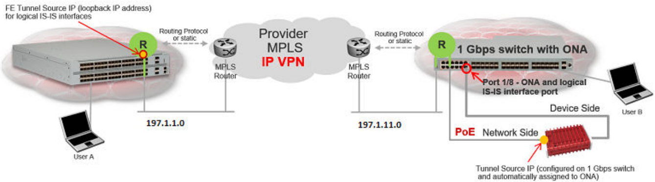
Figure 76: IP using VRF traffic flow
