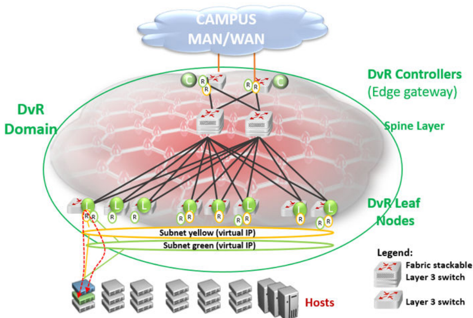
Figure 48: SPB Fabric network with central Layer 3 Controller and distributed Layer 3 datapath at the edges
