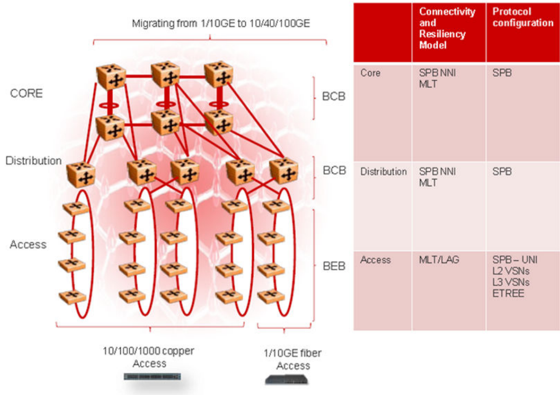
Figure 125: Metro ring access solution
