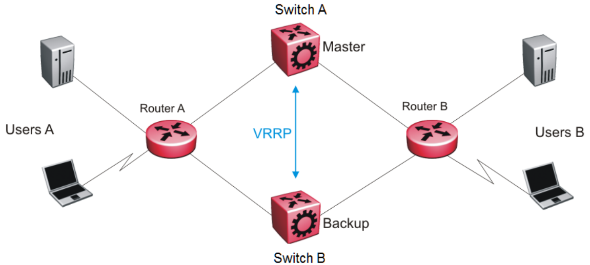
Figure 273: VRRP network topology
