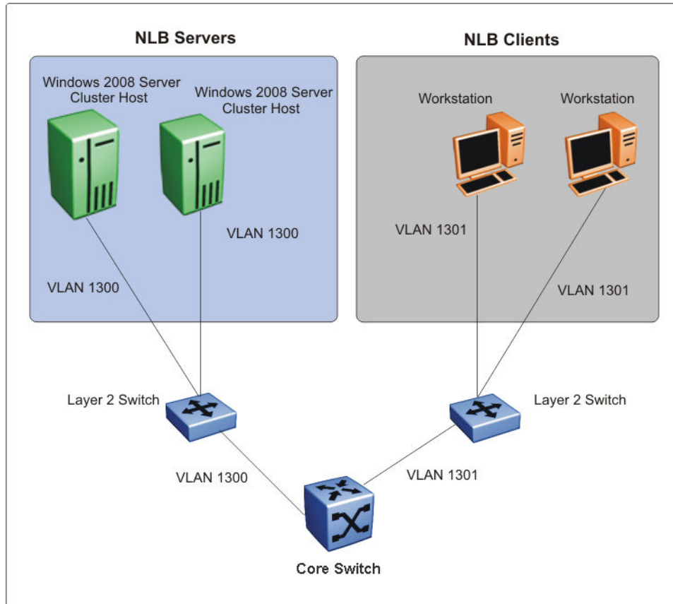
Figure 264: Supported NLB topology—example 1
