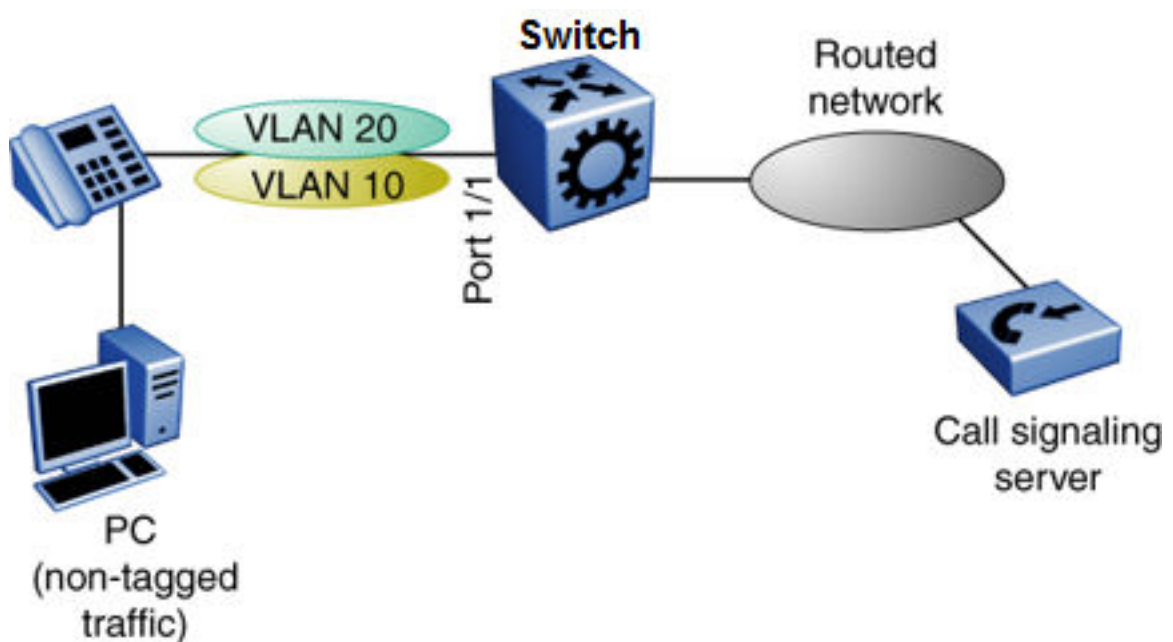
Figure 263: Network with IP phone and PC
