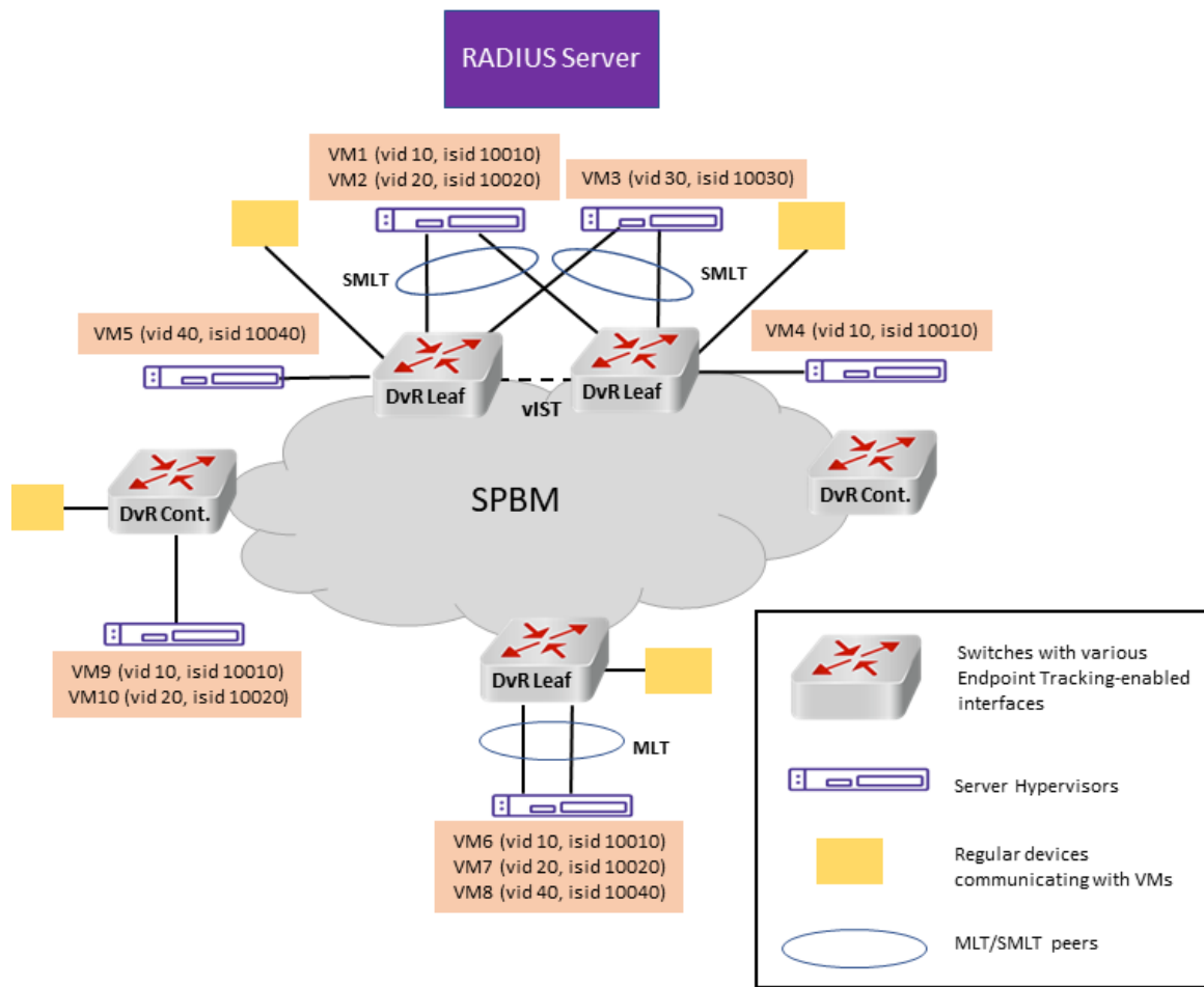
Figure 95: DvR Topology Example
