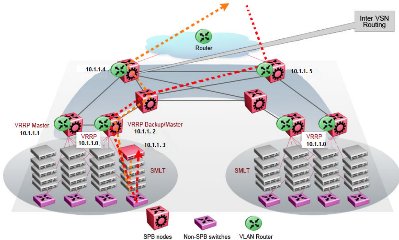
Figure 119: Optimized routing before moving VMs
