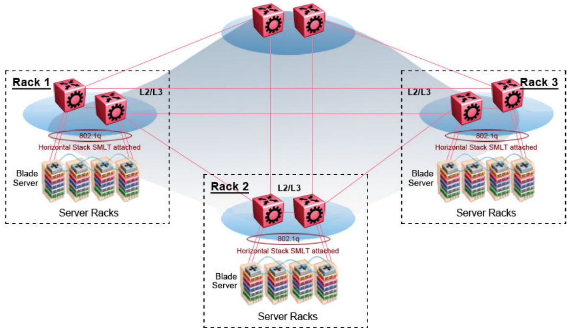
Figure 58: SPBM ring topology with shared data centers
