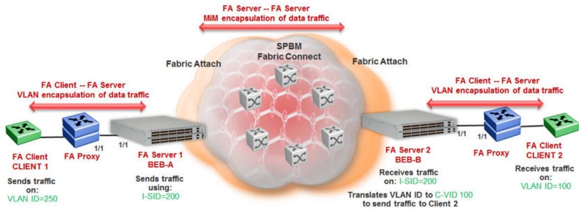
Figure 87: Data encapsulation — VLAN encapsulation and MiM encapsulation
