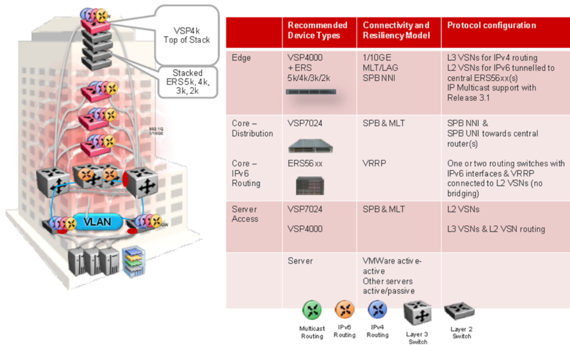
Figure 121: Small core — multi-tenant
