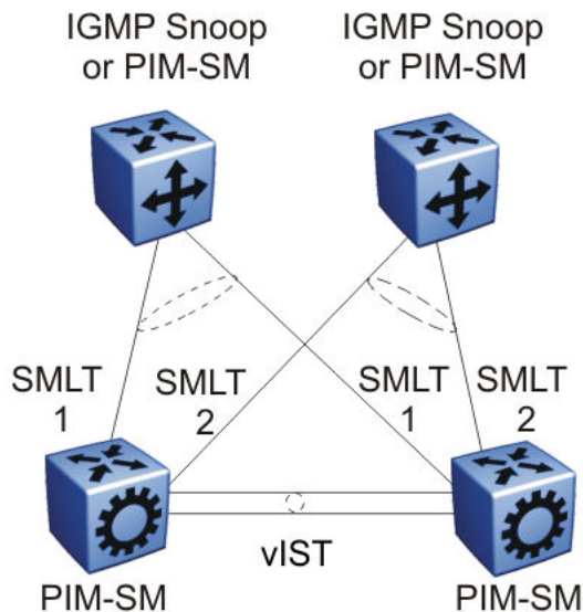
Figure 149: Multicast routing using PIM-SM
