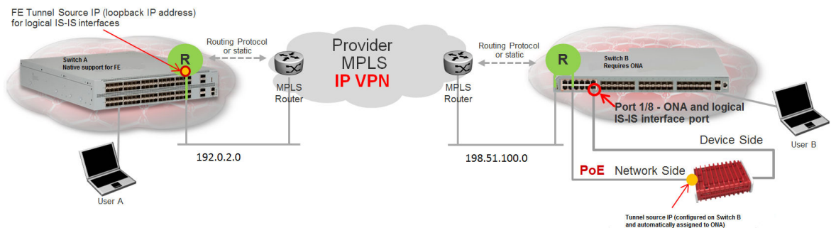
Figure 67: Fabric Extend traffic flow
