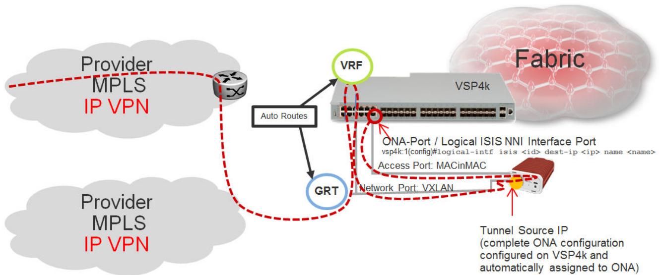
Figure 73: Autorouting between GRT and VRF
