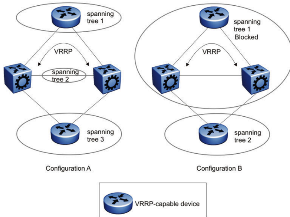
Figure 272: VRRP and STG configurations
