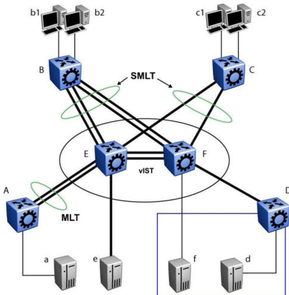
Figure 198: SMLT aggregation switches and operations
