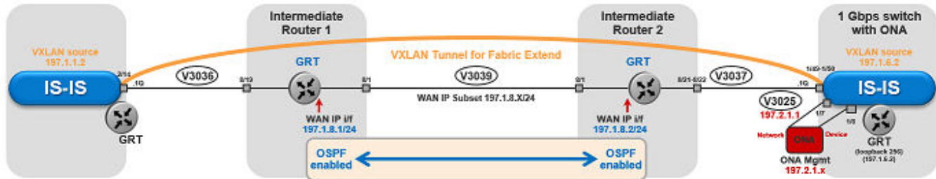
Figure 75: IP (GRT) traffic flow component view
