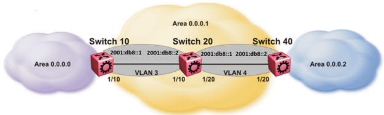
Figure 167: OSPFv3 virtual link with IPsec configuration
