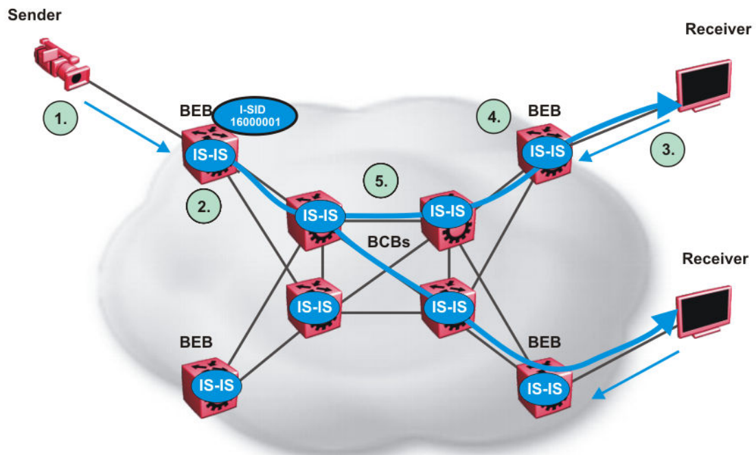
Figure 157: IP Multicast over Fabric Connect streams
