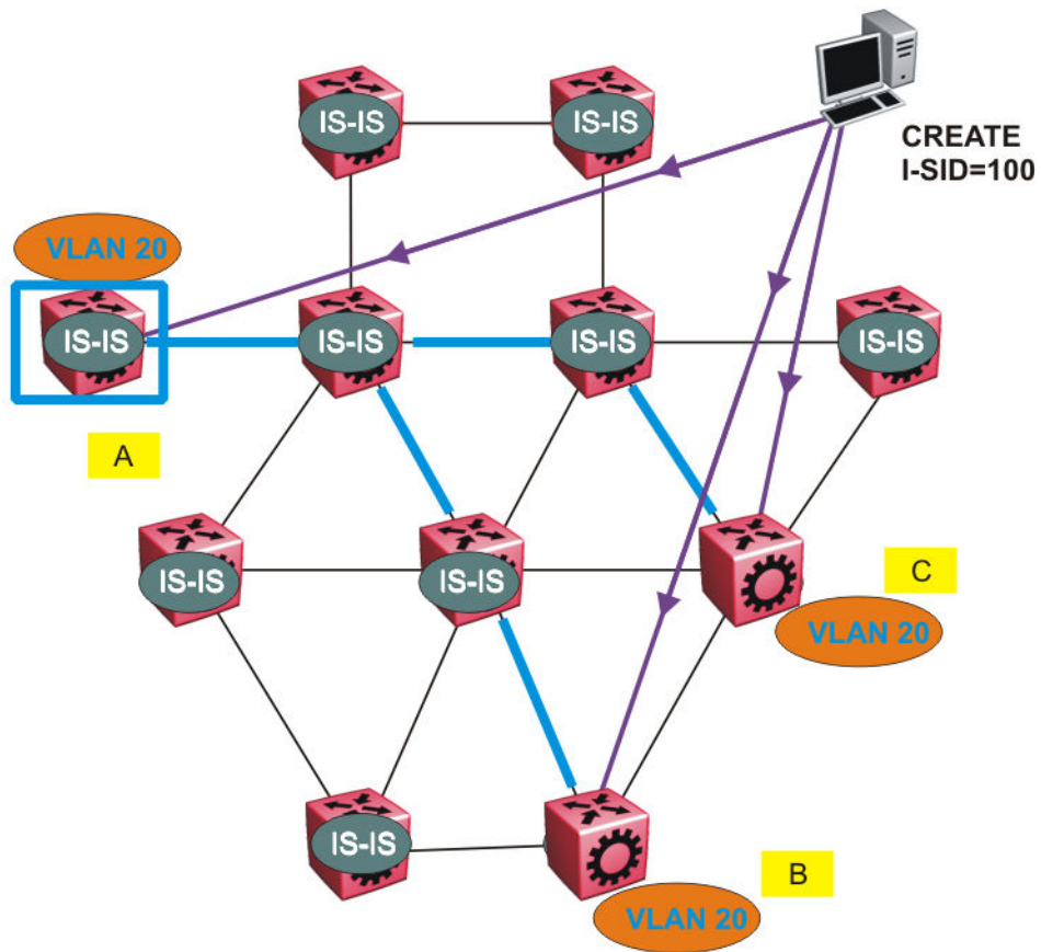
Figure 104: Shortest path tree for source node A
