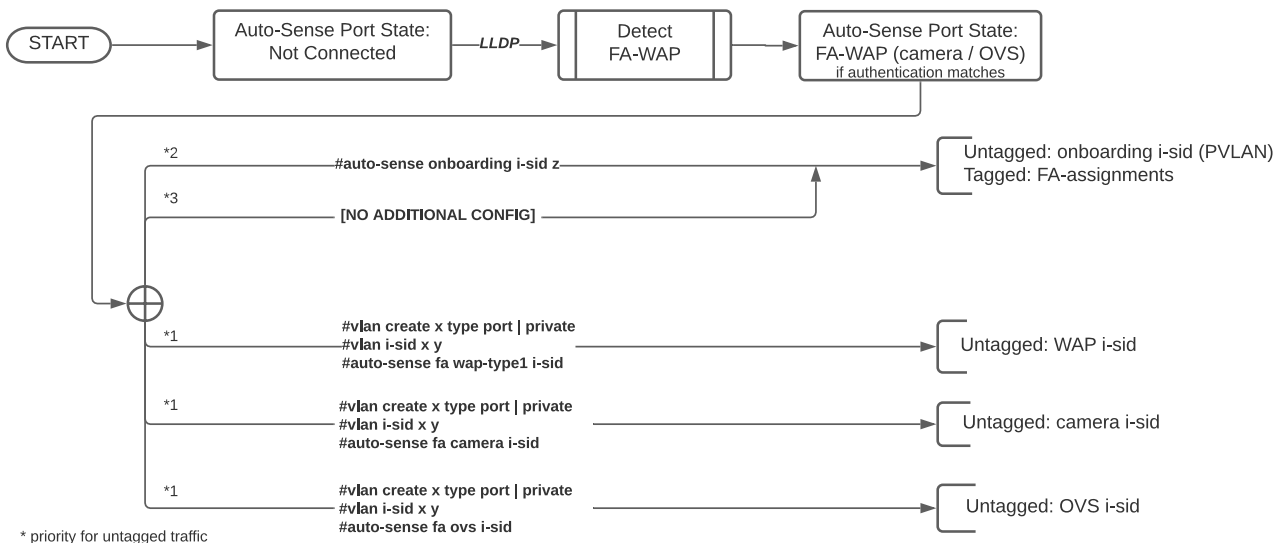
Figure 7: Auto-sense FA WAP / camera / OVS without NAC
