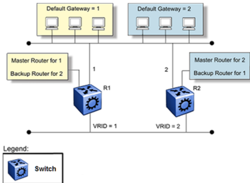
Figure 270: Virtual Router Redundancy Protocol configuration
