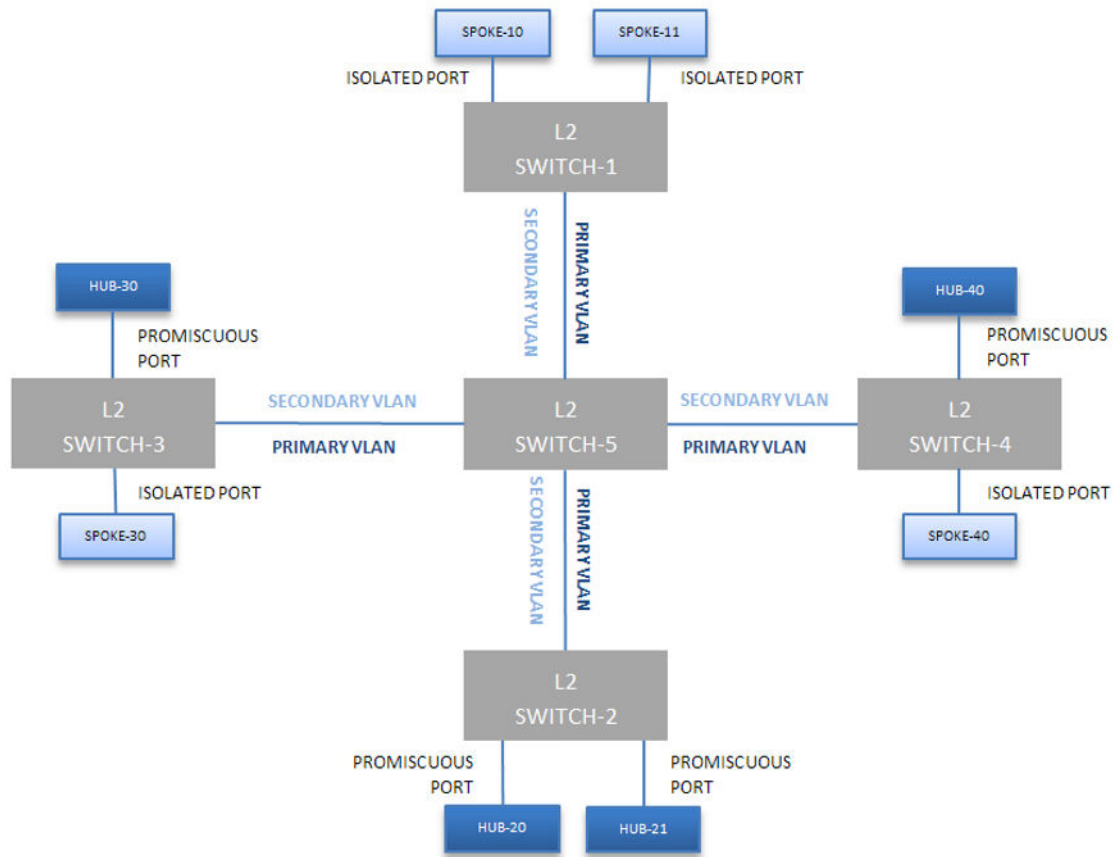
Figure 261: Private VLAN Topology
