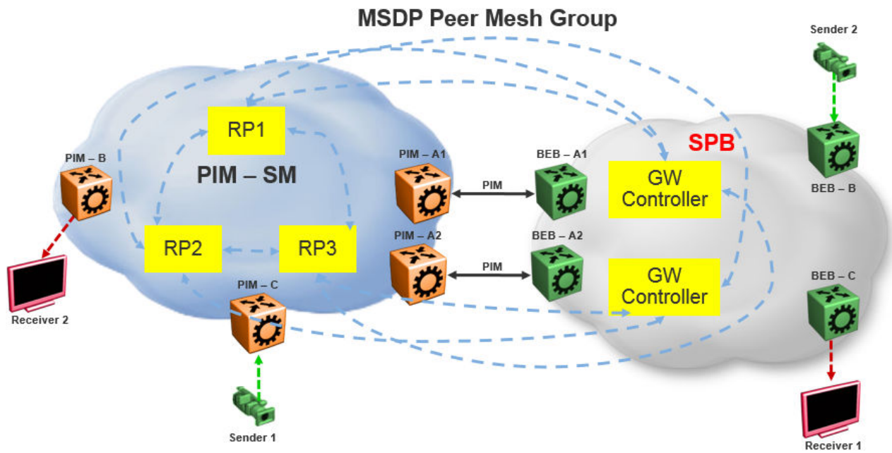
Figure 247: Peer Mesh Group
