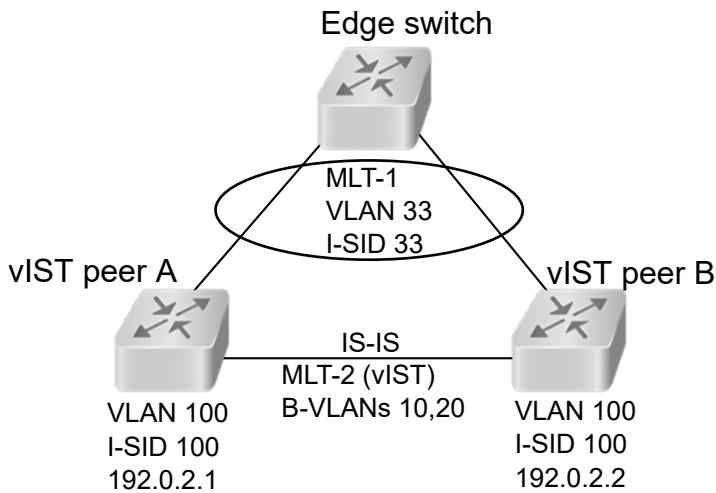
Figure 200: SMLT with vIST configuration example
