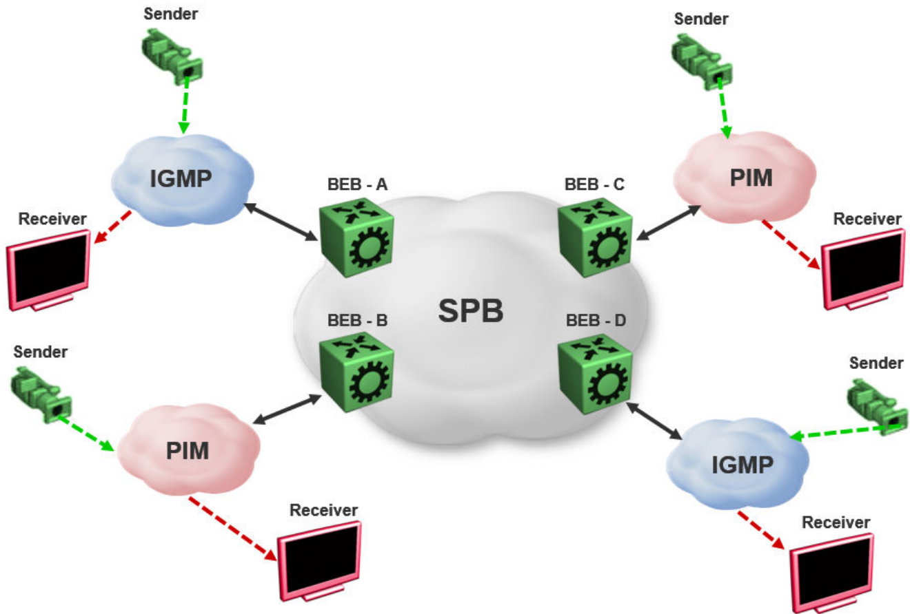
Figure 242: IP Multicast over Fabric Connect Streams
