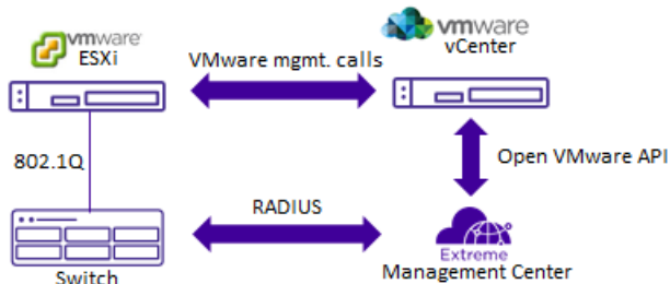
Figure 94: ExtremeCloud IQ - Site Engine Endpoint Tracking Interaction Example
