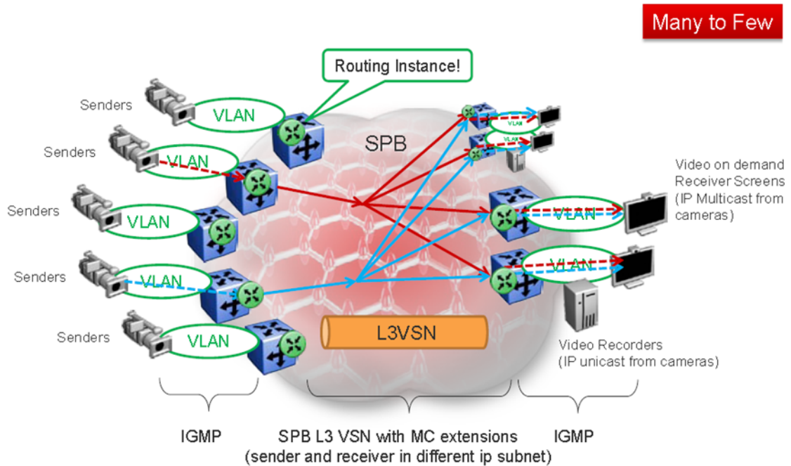
Figure 124: Deployment scenario — Routed video surveillance and IP camera deployment for transportation, airports, and government
