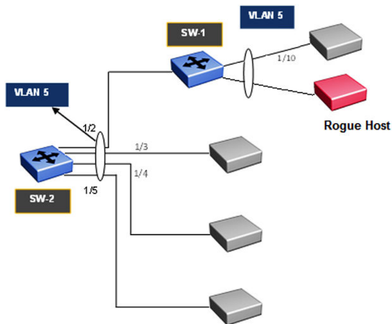
Figure 182: First Hop Security topology
