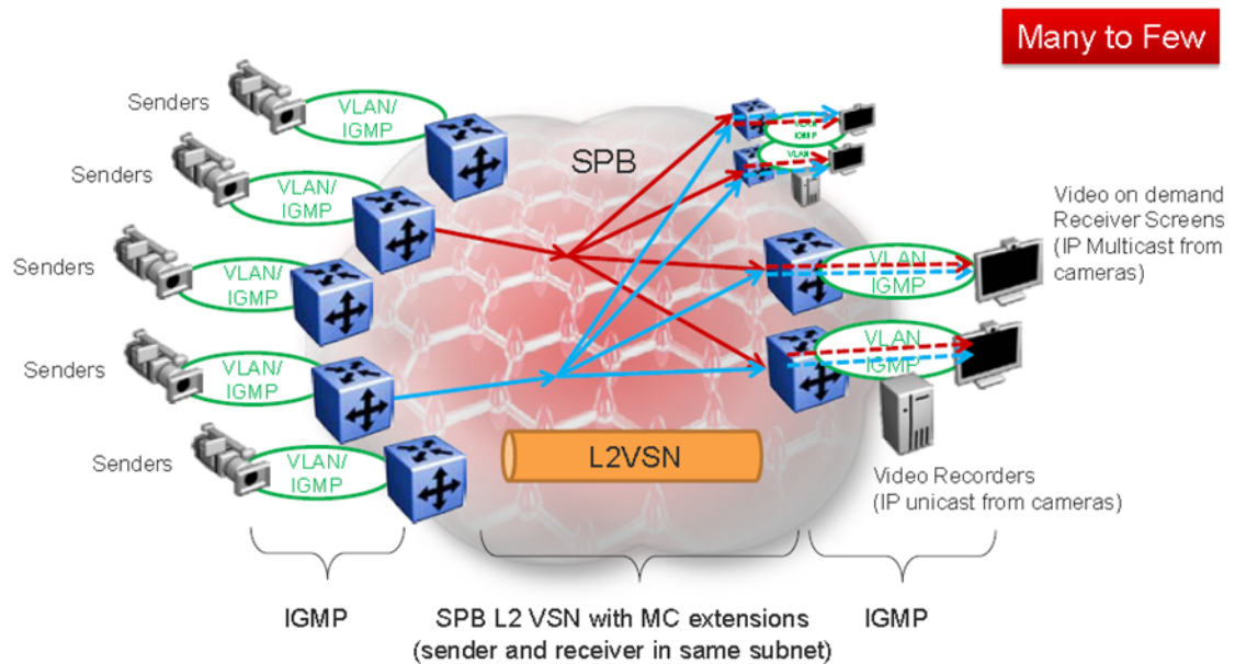
Figure 123: Deployment scenario — bridged video surveillance and IP camera deployment for transportation, airports, and government
