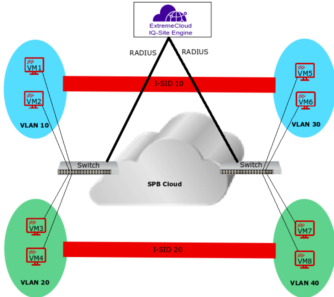
Figure 93: Endpoint Tracking Example
