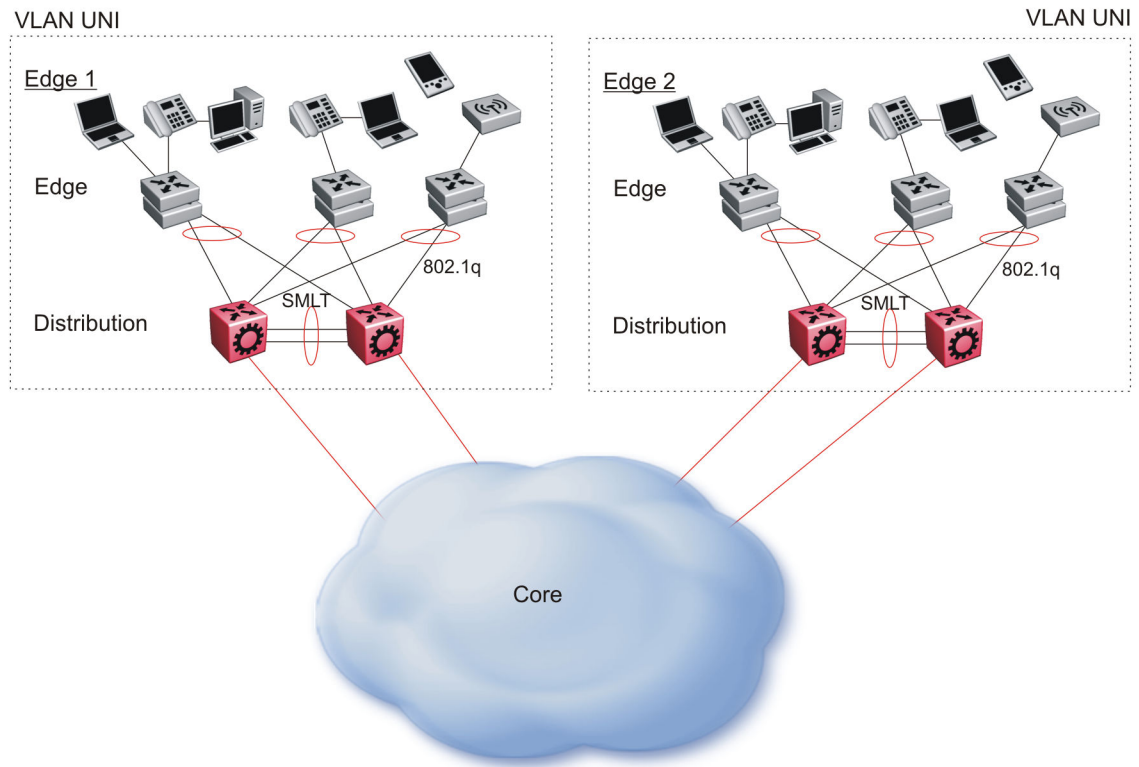
Figure 112: Access to the SPBM Core
