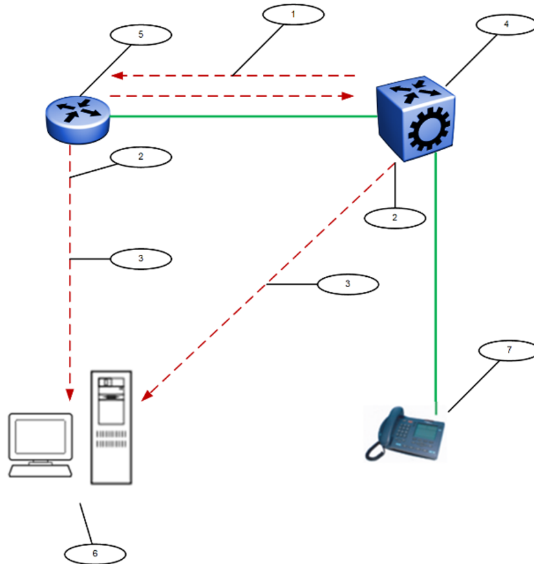
Figure 194: LLDP in a LAN
