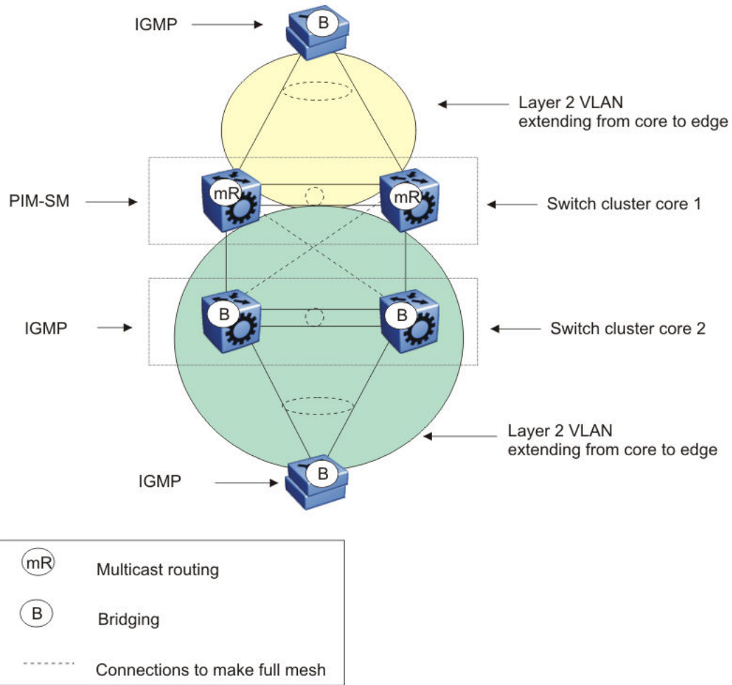
Figure 151: Multicast SMLT square 1
