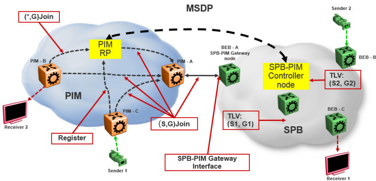
Figure 244: SPB-PIM GW components
