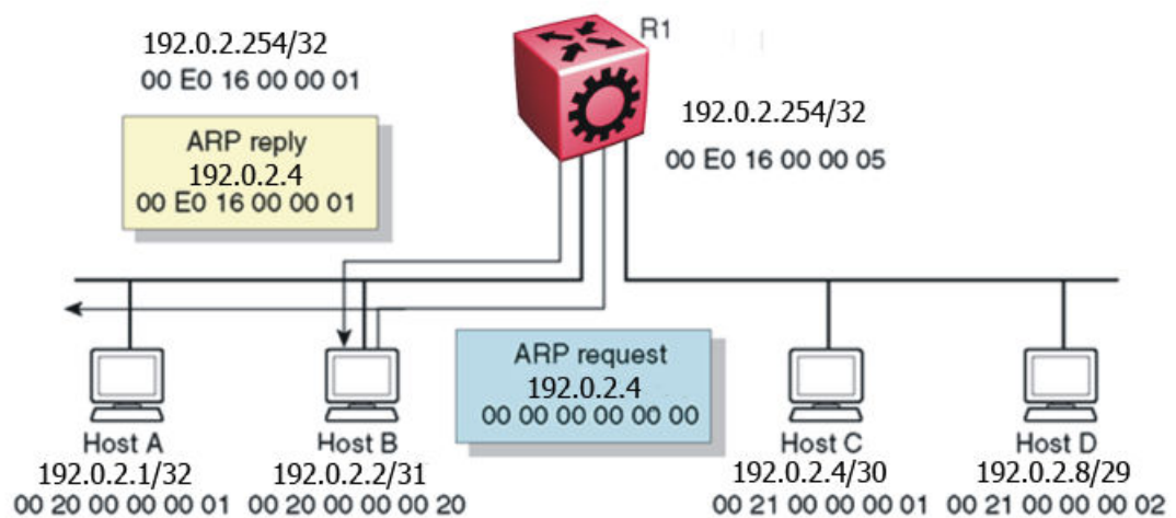
Figure 17: Proxy ARP operation
