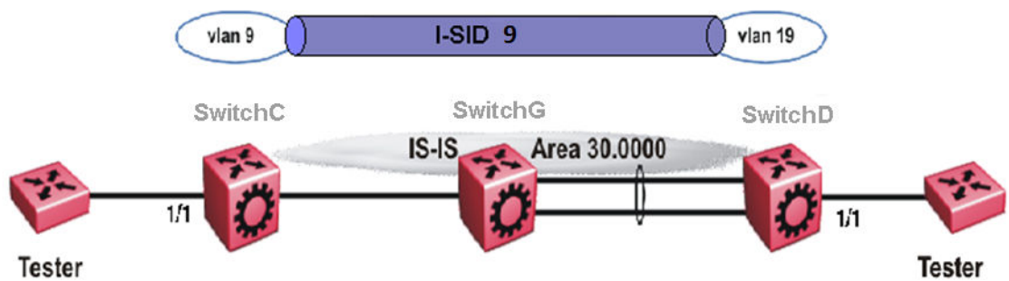
Figure 108: Layer 2 VSN with different VLAN IDs
