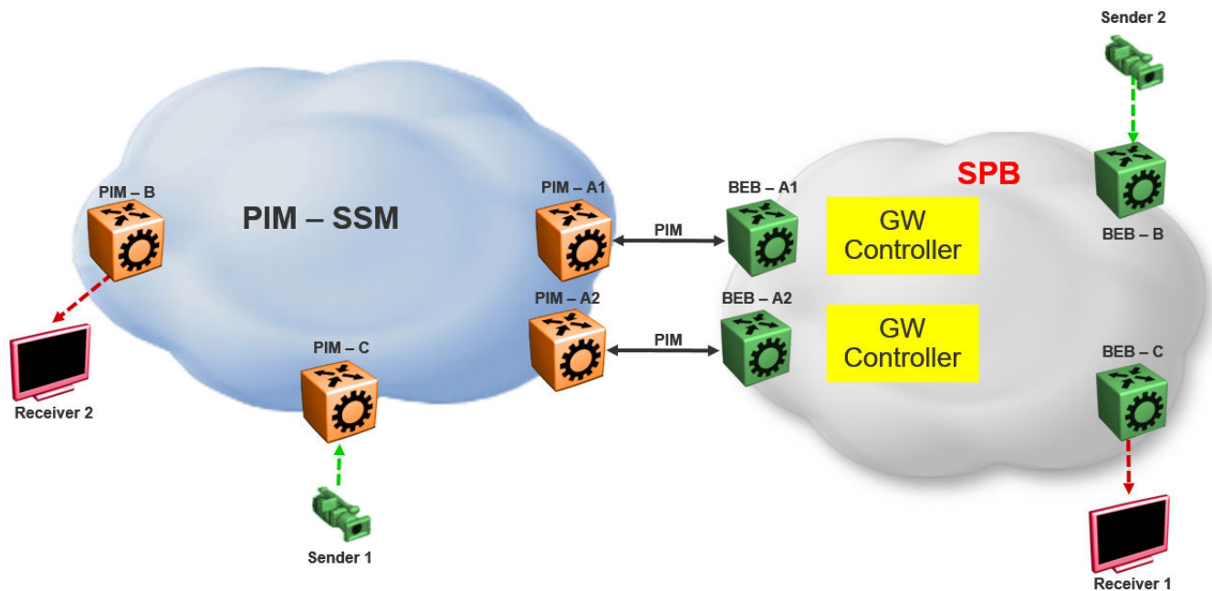
Figure 246: Static configuration of SSM groups in Controllers
