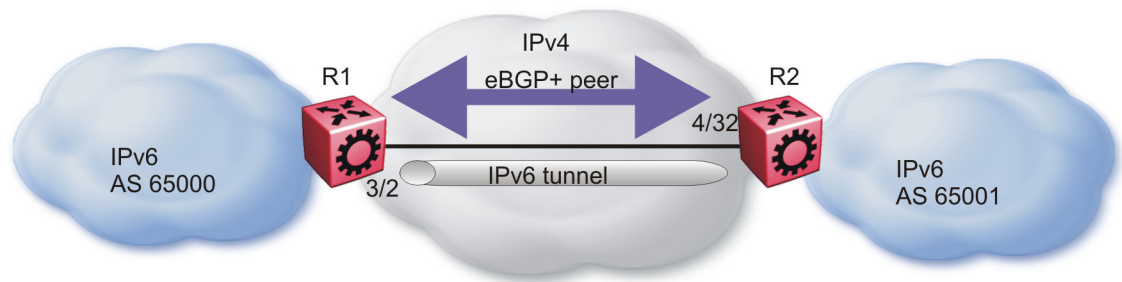
Figure 42: eBGP+ peers with IPv6 tunneling
