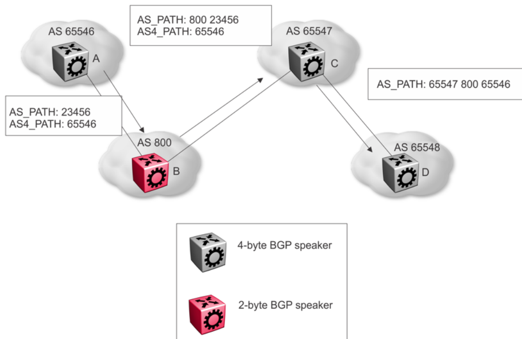
Figure 21: 2-byte and 4-byte Mixed Environment
