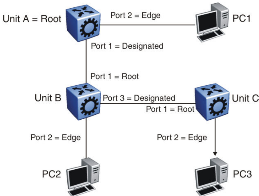
Figure 240: RSTP negotiation process
