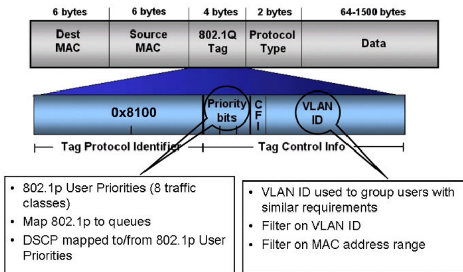
Figure 262: VLAN tag insertion
