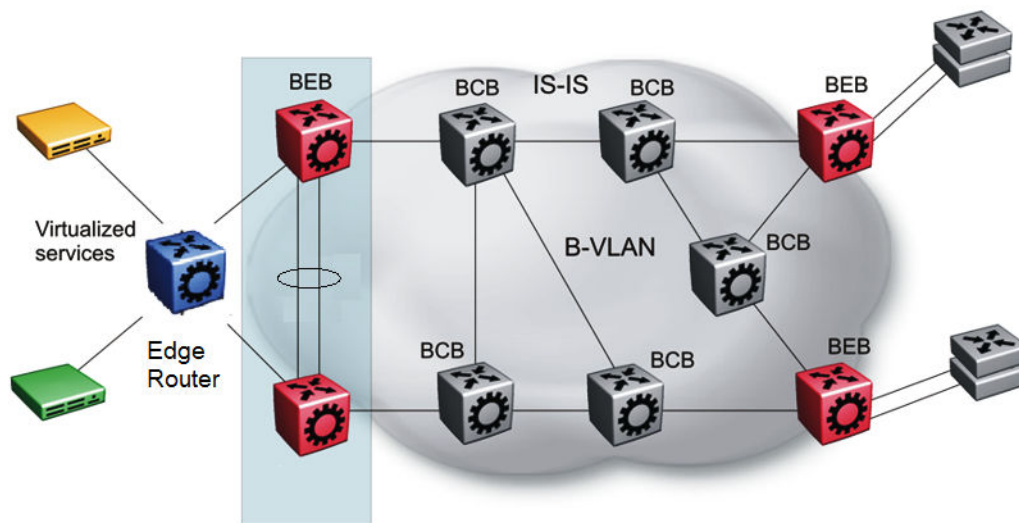
Figure 111: SPBM basic architecture
