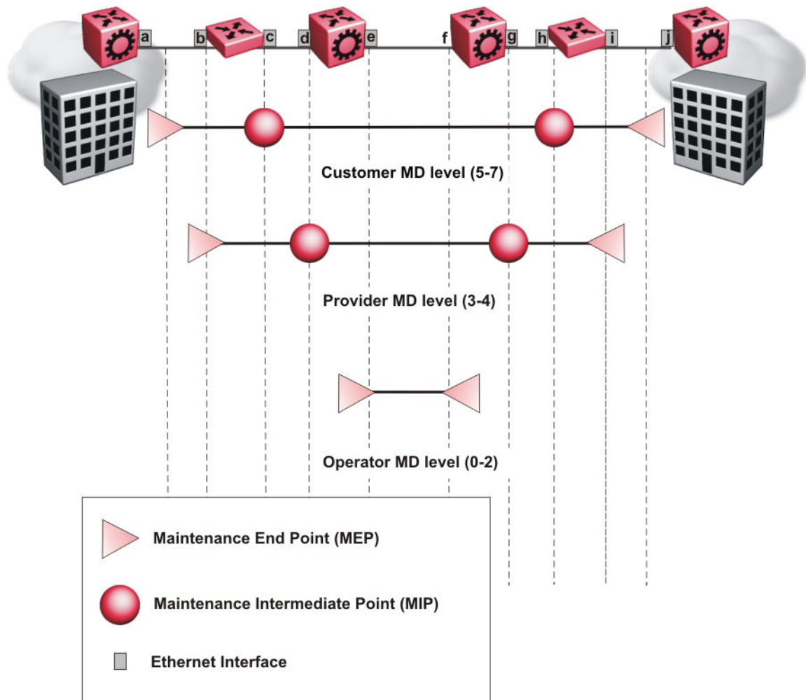
Figure 257: MD level assignment
