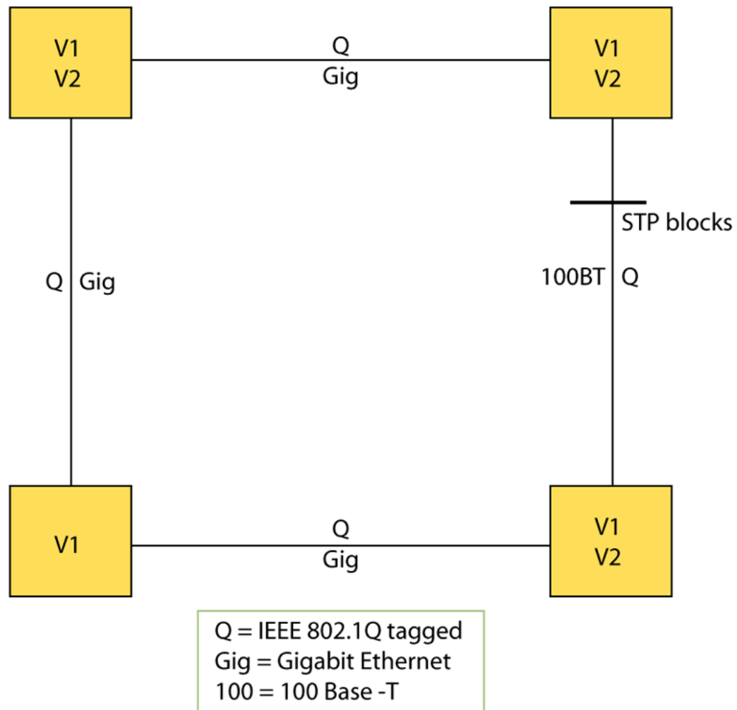
Figure 266: VLAN isolation
