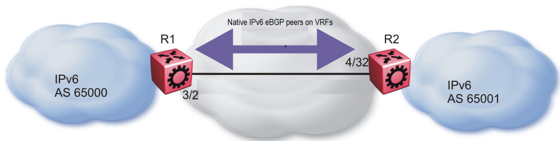
Figure 44: Native IPv6 eBGP peers on VRFs
