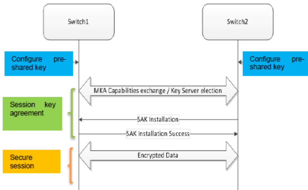
Figure 196: Switch to switch MACsec deployment scenario
