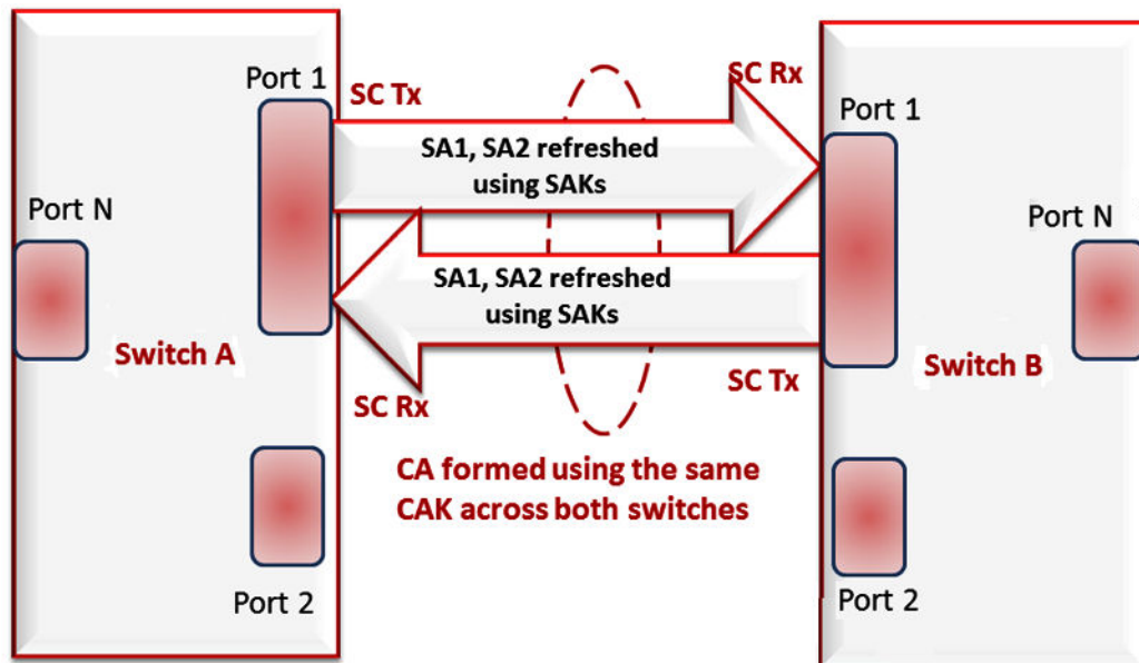
Figure 195: MACsec relationship
