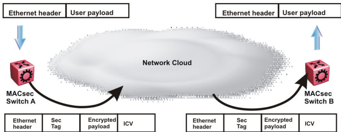
Figure 197: MACsec operation
