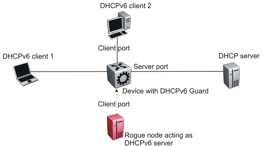
Figure 183: DHCPv6 Topology 1
