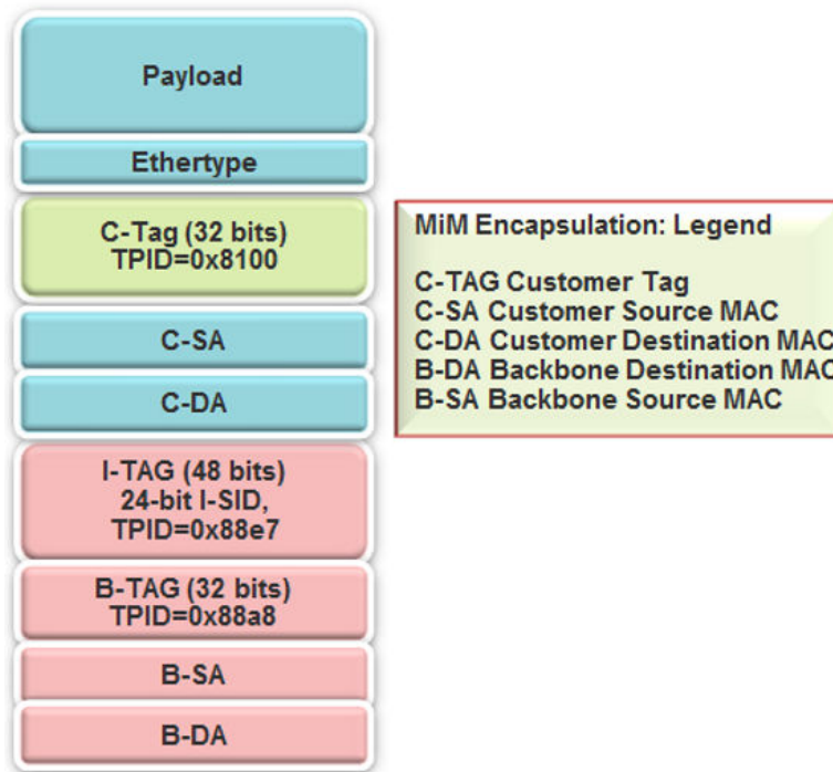
Figure 88: MiM encapsulation
