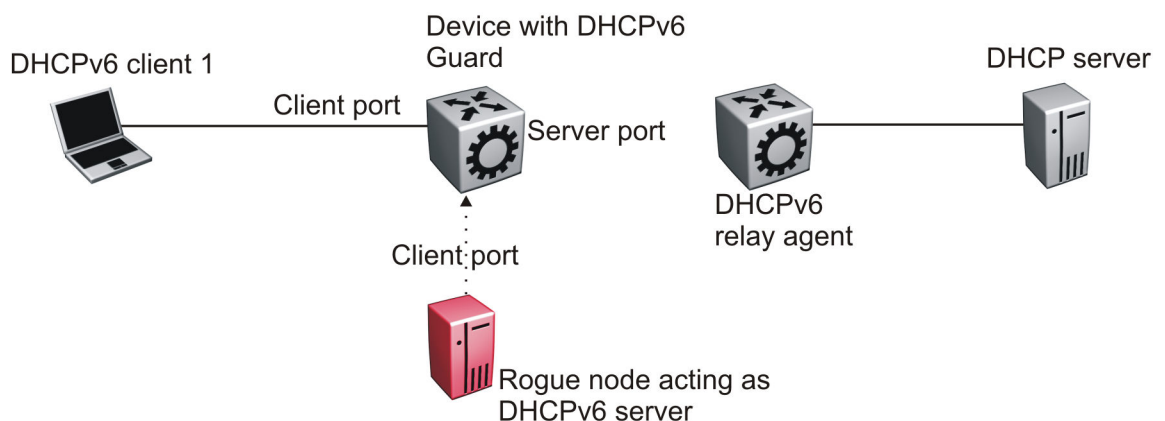
Figure 183: DHCPv6 Topology 1
