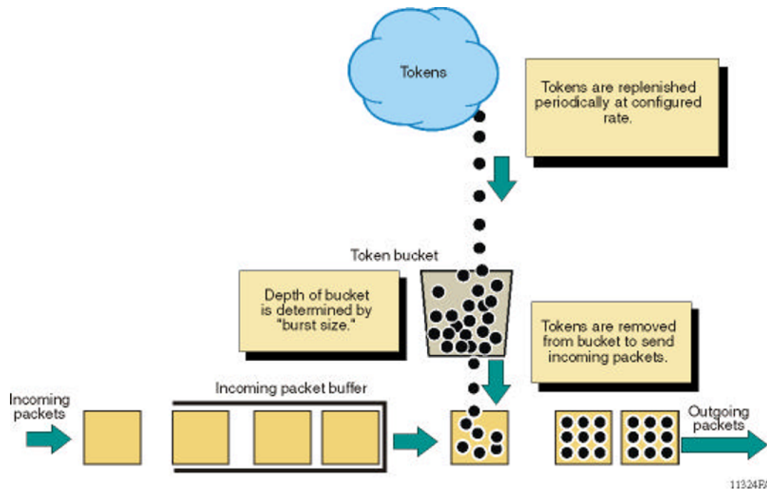
Figure 218: Token flow
