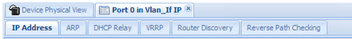
Figure 14: Menu bar
