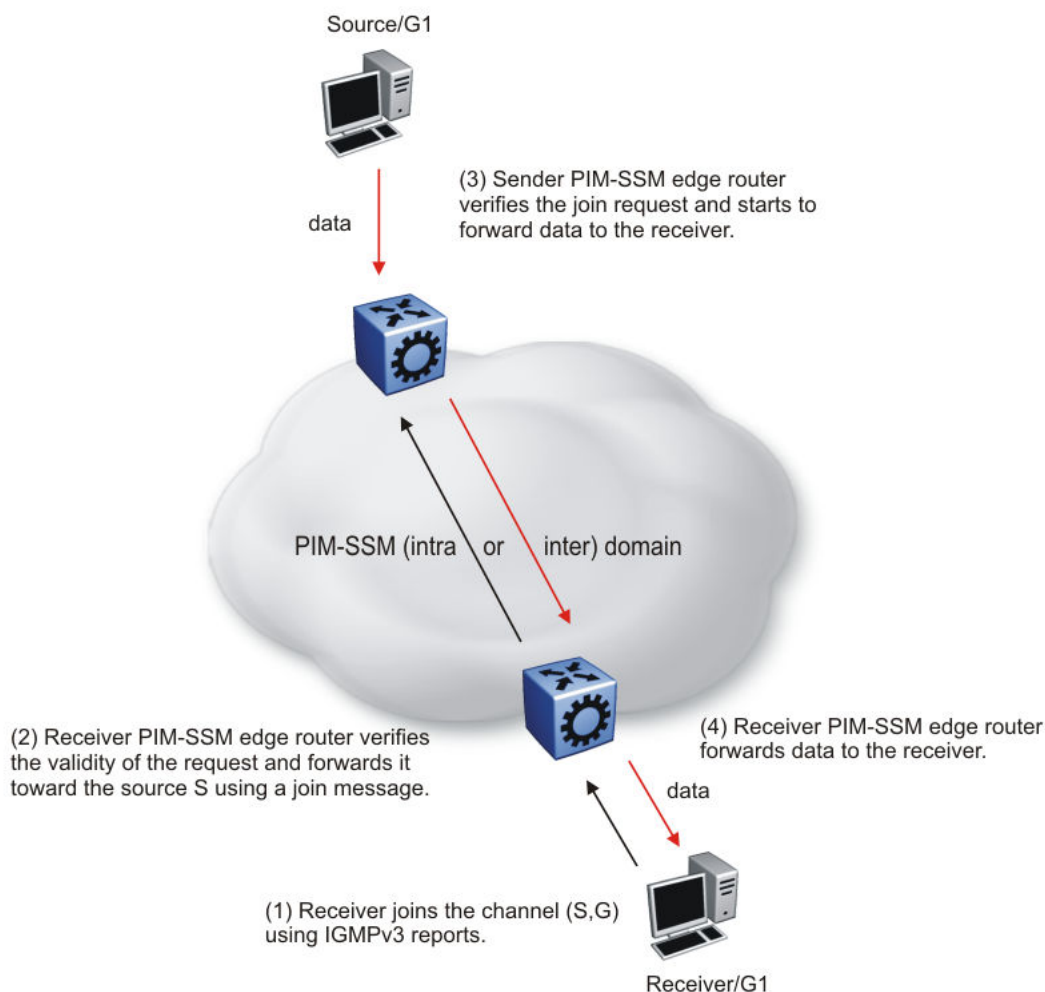
Figure 145: PIM-SSM architecture
