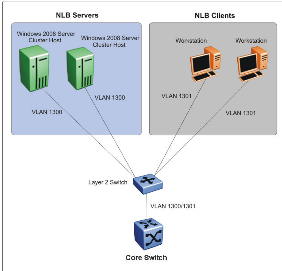
Figure 265: Supported NLB topology—example 2
