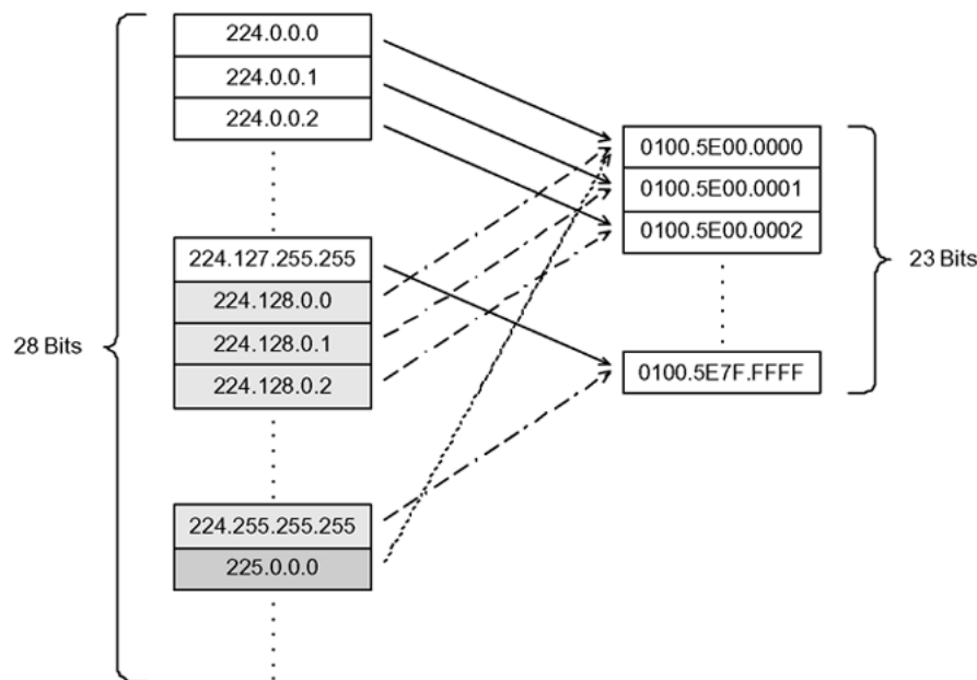
Figure 147: Multicast IP address to MAC address mapping
