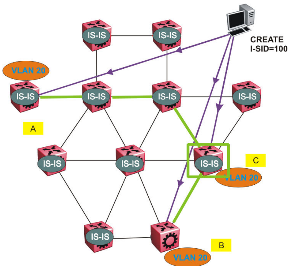
Figure 106: Shortest path tree for source node C
