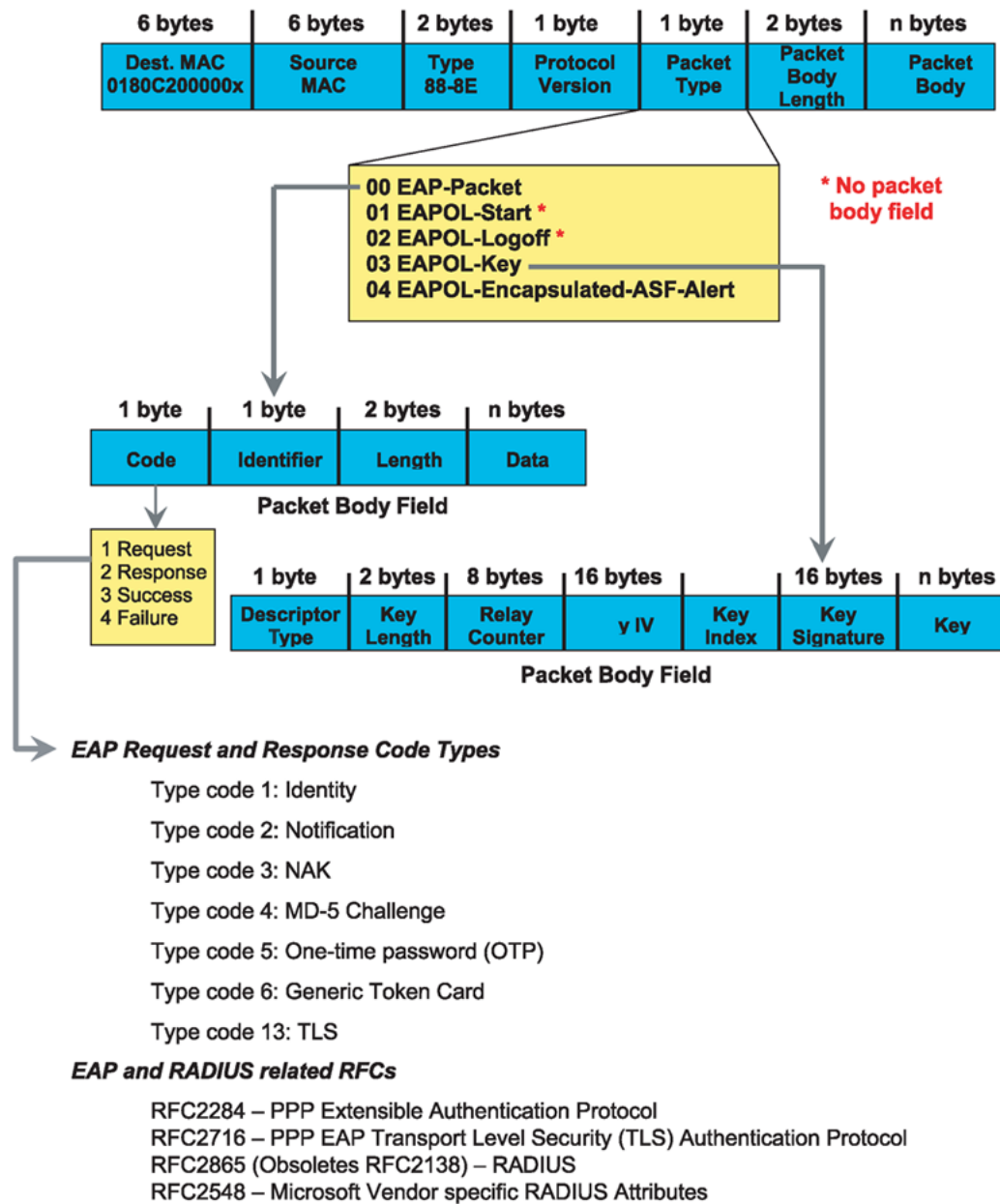
Figure 55: 802.1x Ethernet frame
