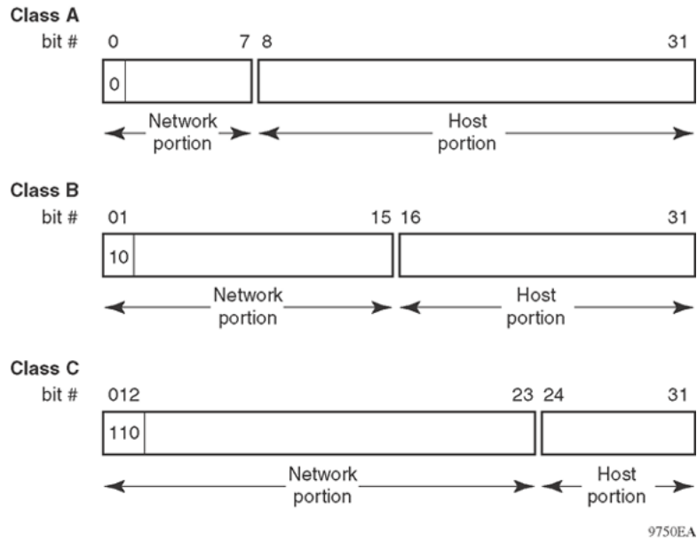
Figure 168: Network and host boundaries in IP address classes
