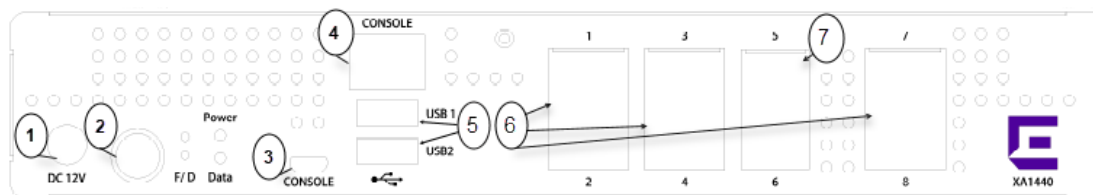
Figure 285: XA1400 Series switches rear panel
