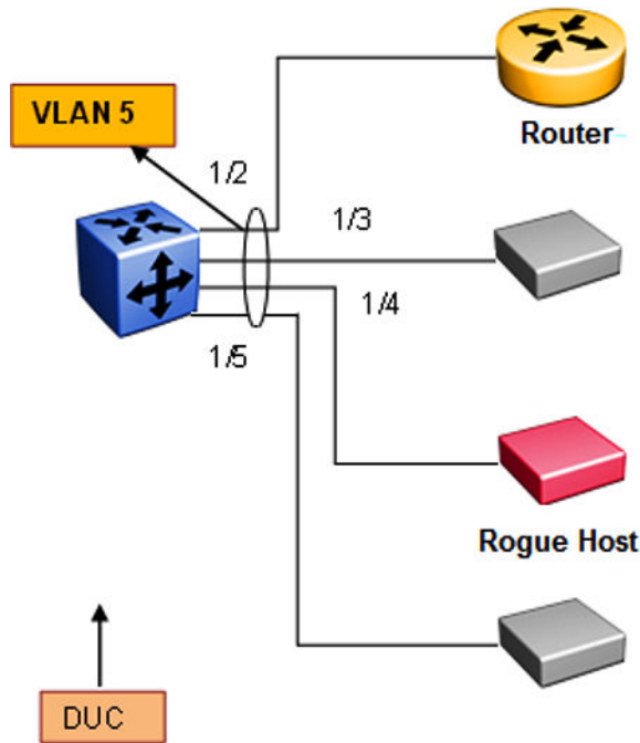
Figure 185: RA Guard Topology1
