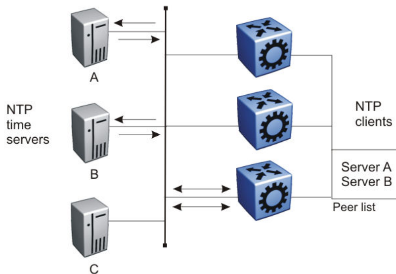
Figure 207: NTP Time Servers Operating in Unicast Client Mode
