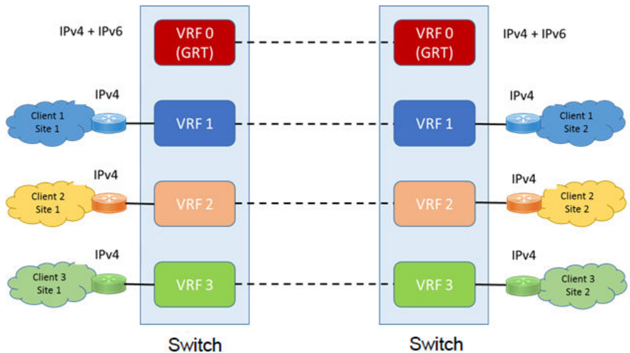
Figure 267: Multiple virtual routers in one system
