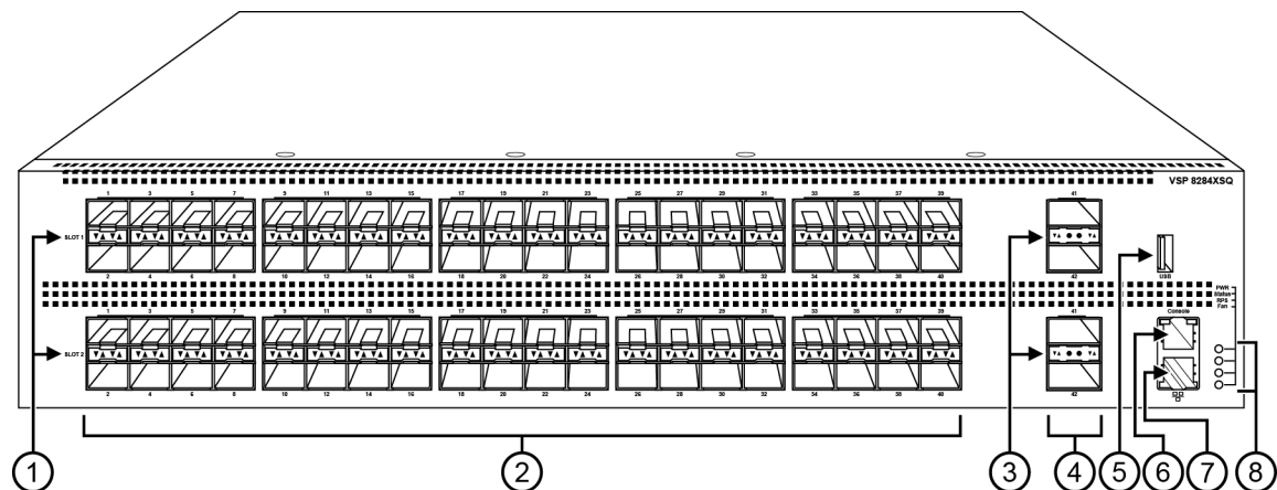
Figure 283: VSP 8284XSQ front view
