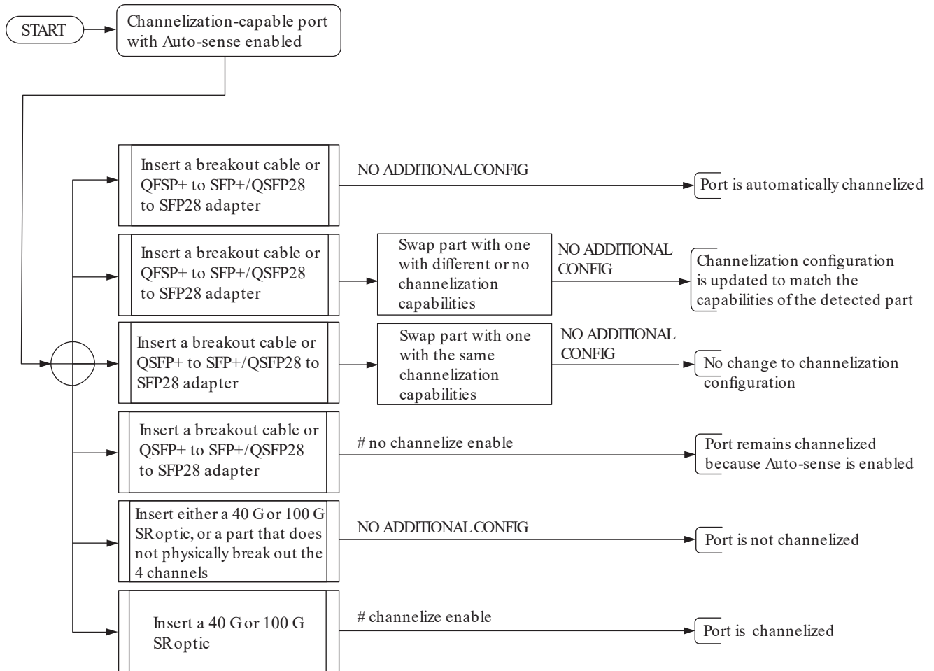
Figure 9: Automatic Channelization with Auto-sense enabled
