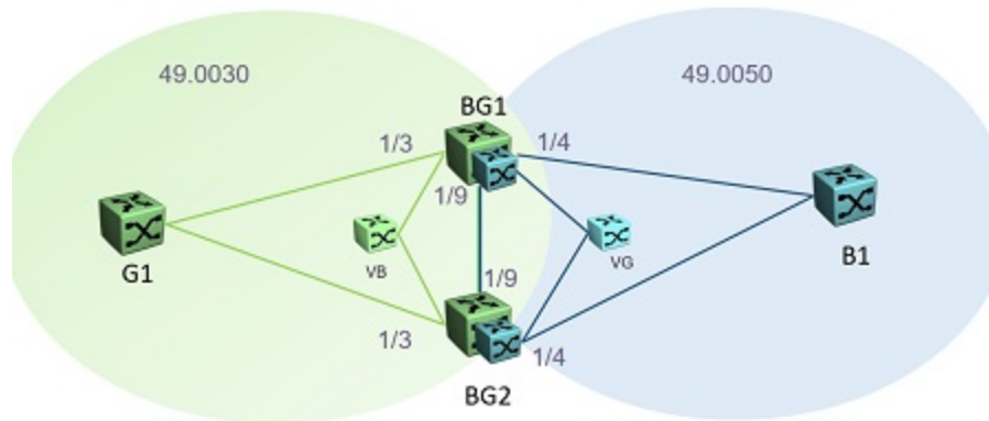
Figure 99: Multi-area SPB network example
