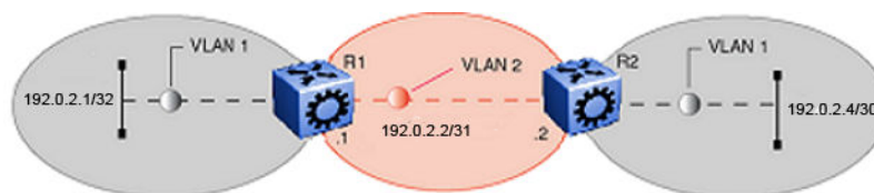
Figure 171: IP routing between VLANs
