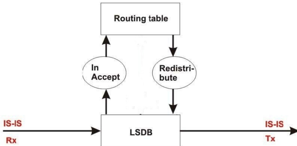
Figure 15: Route filtering for the IS-IS routing protocol
