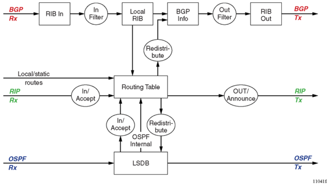
Figure 14: Route filtering for BGP, RIP, and OSPF routing protocols
