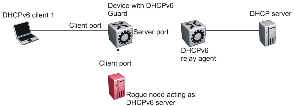
Figure 172: DHCPv6 Topology 1
