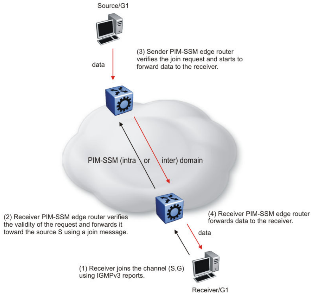
Figure 134: PIM-SSM architecture
