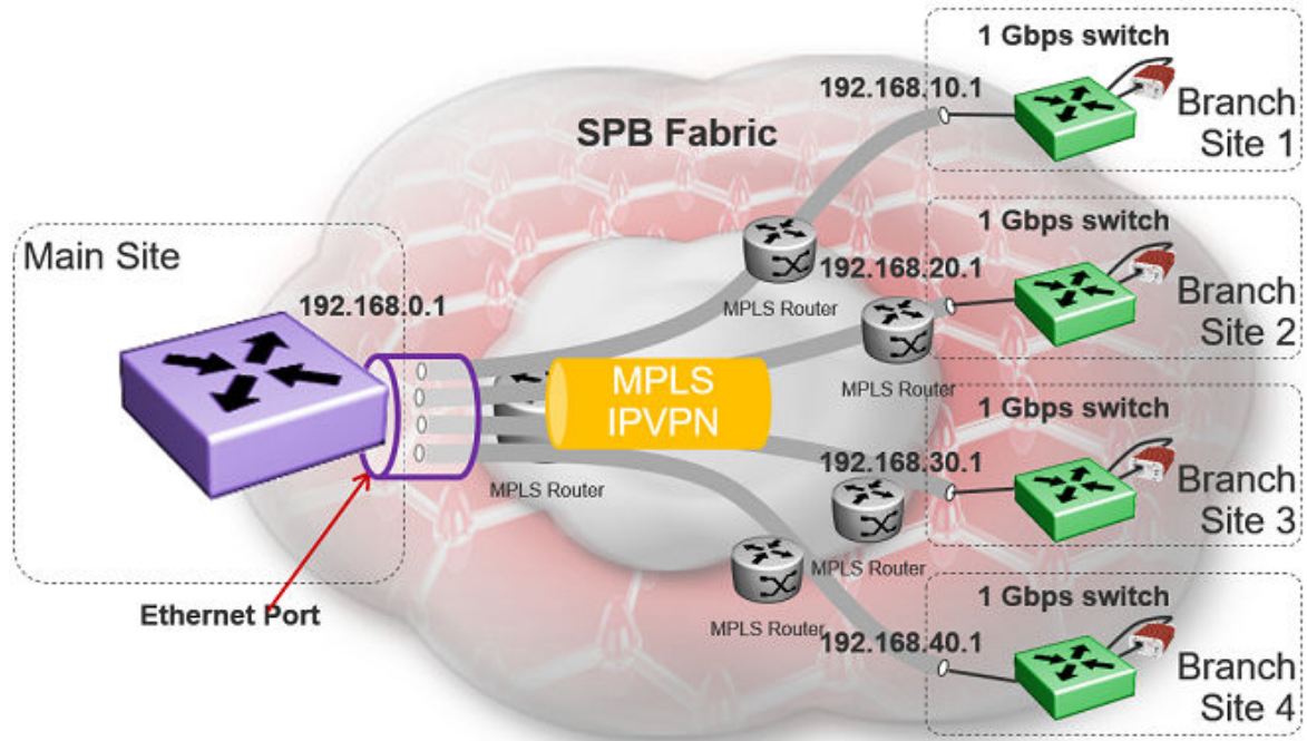
Figure 57: Fabric Extend IP VPN Deployment Option
