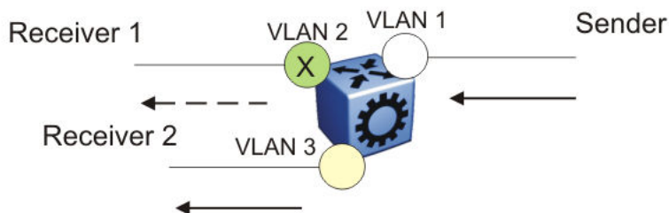
Figure 130: Data flow using deny-rx policy
