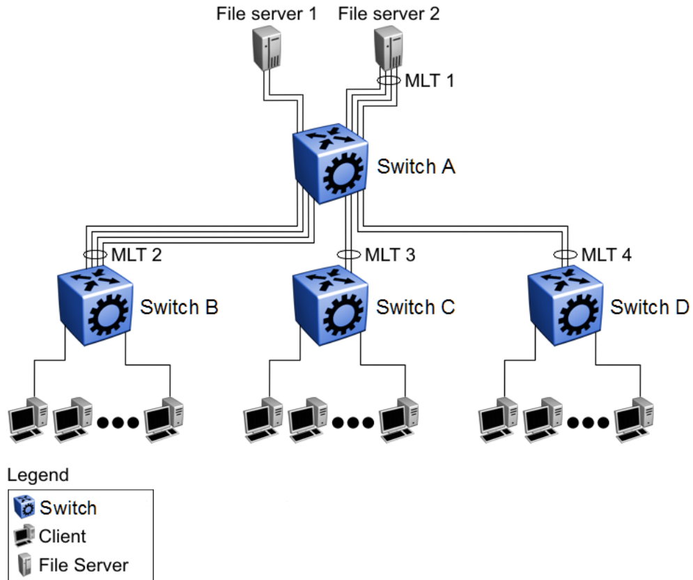
Figure 194: Client/server multilink trunk configuration
