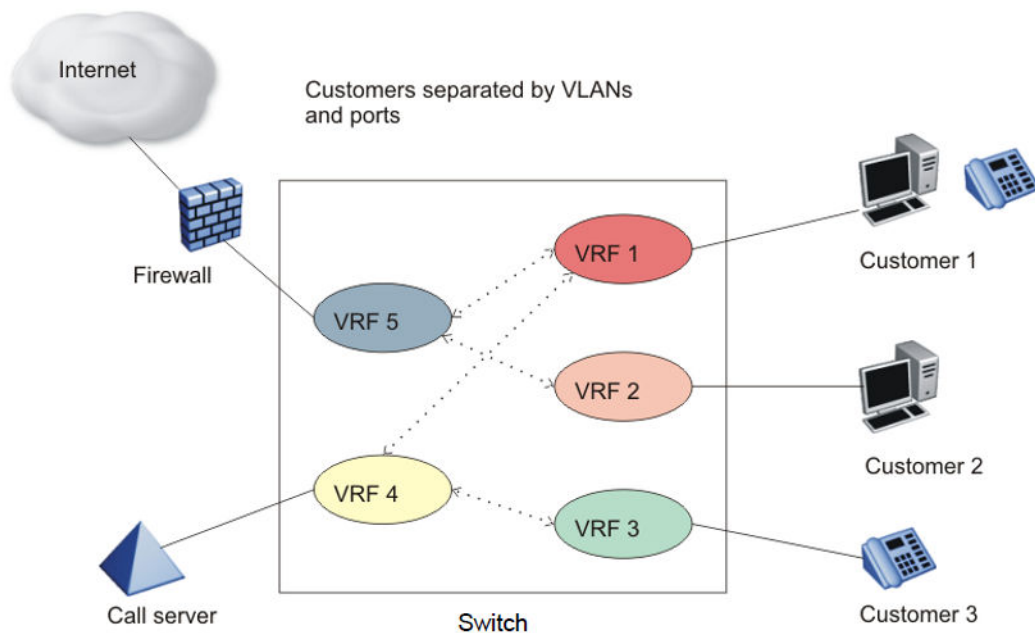
Figure 259: Inter-VRF forwarding
