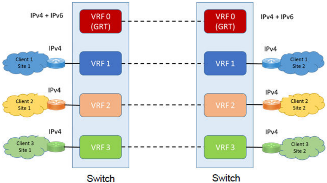
Figure 258: Multiple virtual routers in one system
