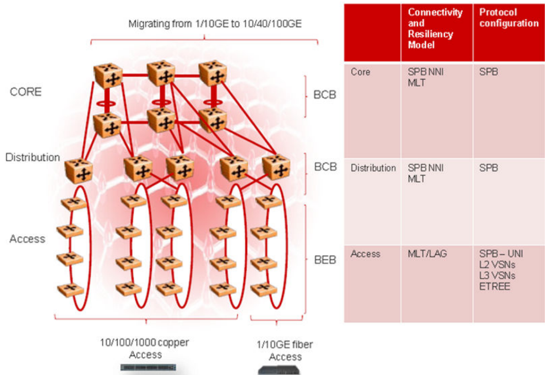
Figure 114: Metro ring access solution
