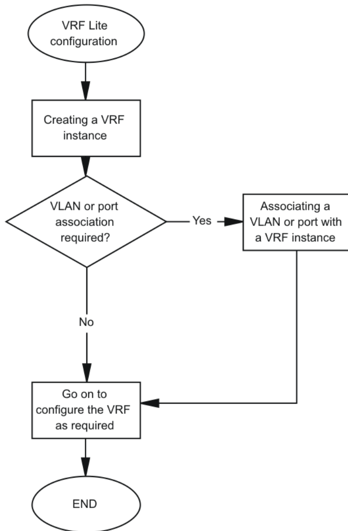
Figure 260: VRF Lite configuration procedures
