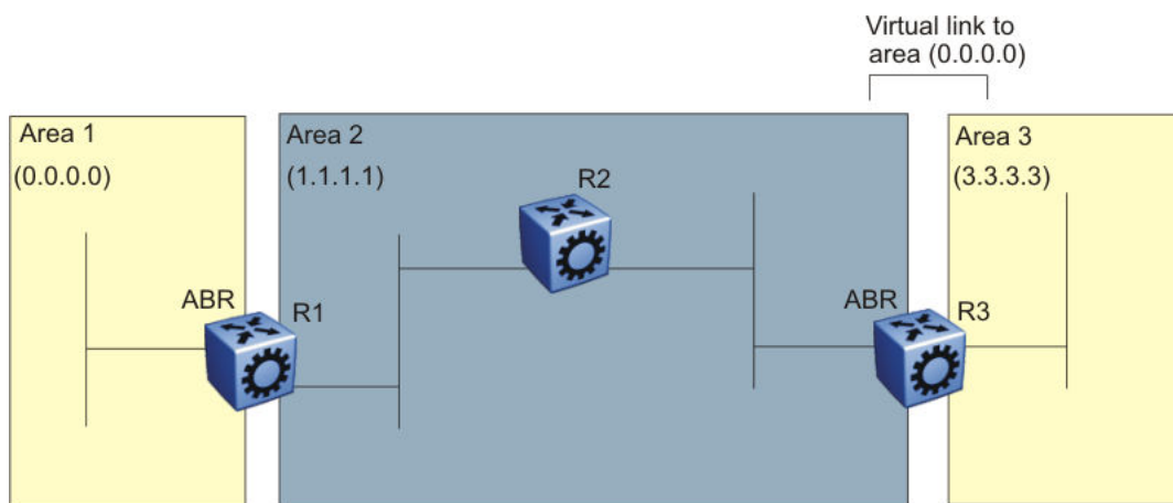
Figure 202: Virtual link between ABRs through a transit area
