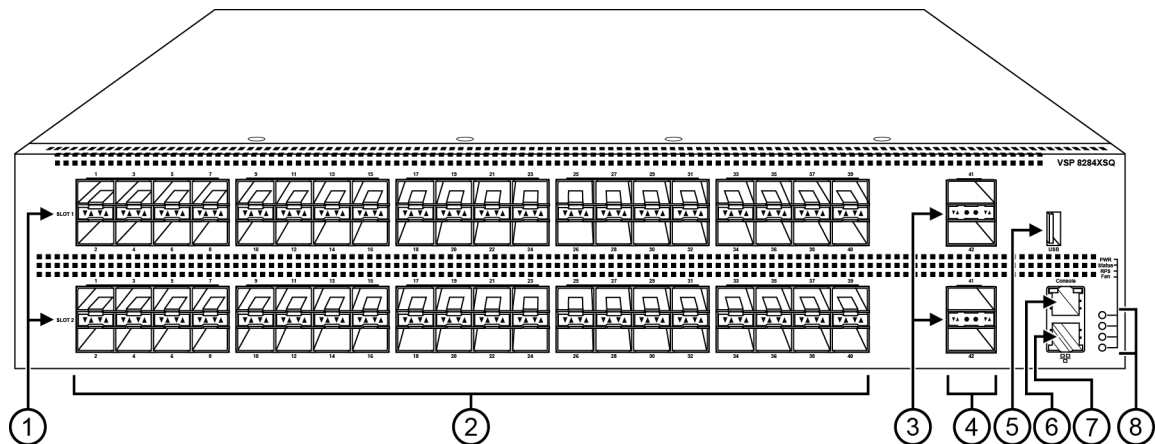
Figure 282: VSP 8284XSQ front view
