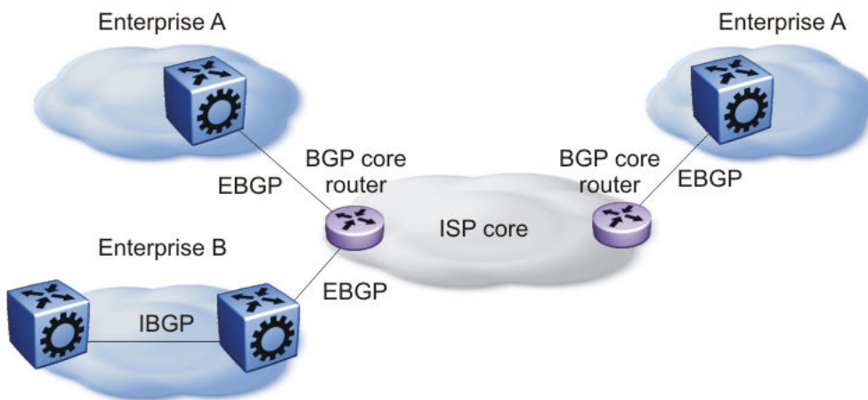
Figure 27: BGP and Edge Aggregation
