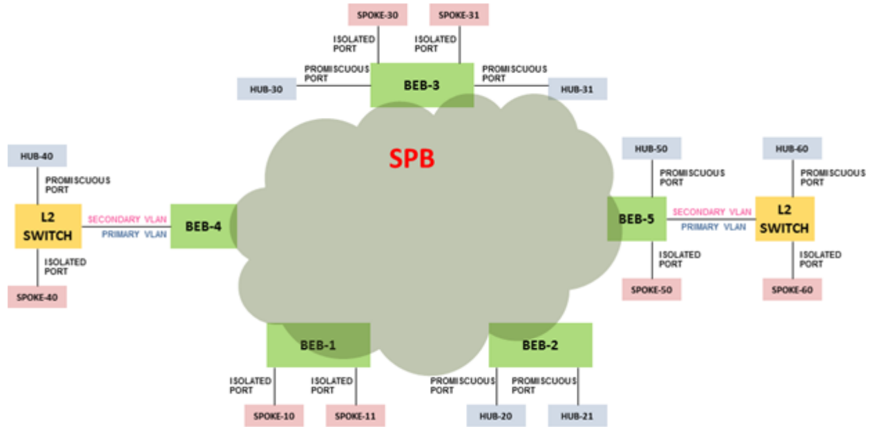
Figure 52: Sample E-Tree configuration
