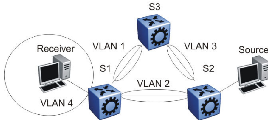
Figure 135: IP multicast sources and receivers on interconnected VLANs
