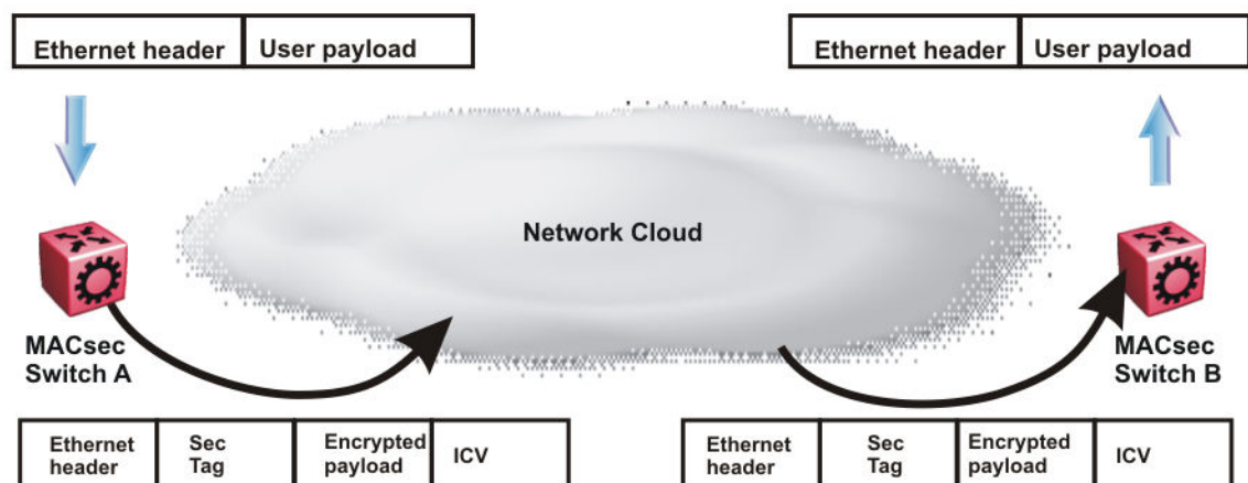
Figure 186: MACsec operation
