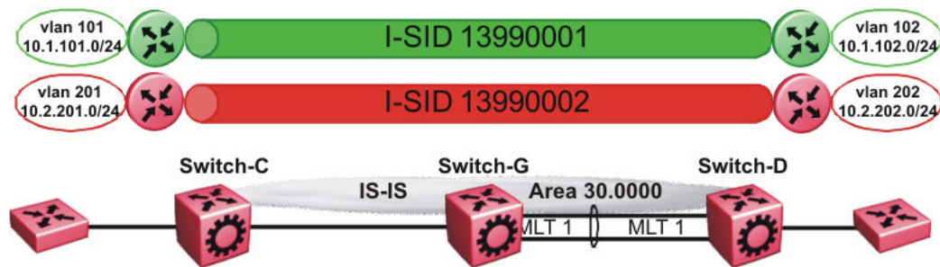
Figure 124: Layer 3 VSN
