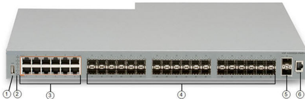
Figure 279: VSP 4450GSX-DC
