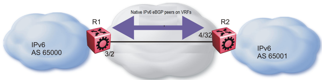
Figure 34: Native IPv6 eBGP peers on VRFs
