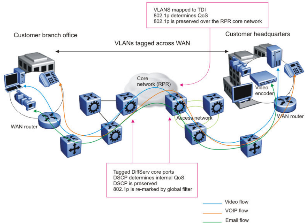
Figure 211: RPR QoS internetworking
