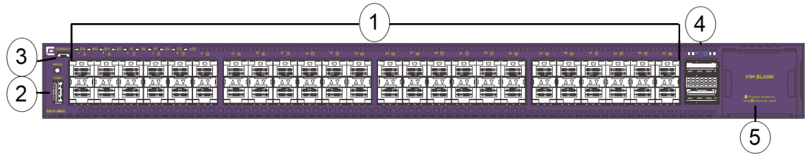
Figure 276: 5520-48SE
