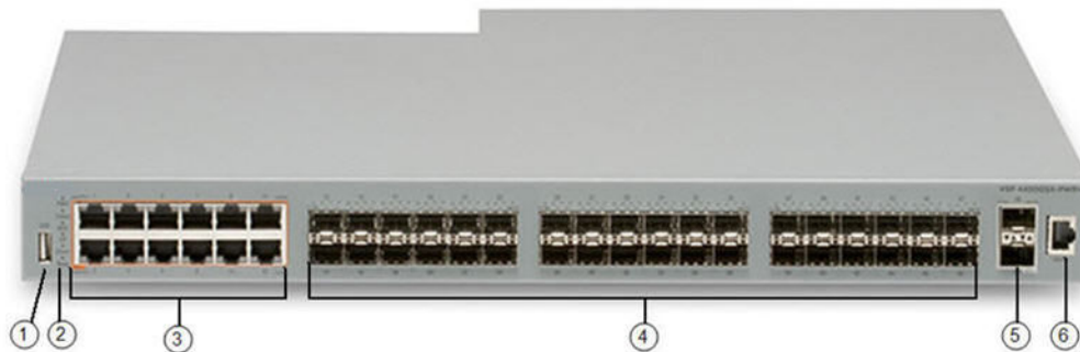
Figure 277: VSP 4450GSX-PWR+
