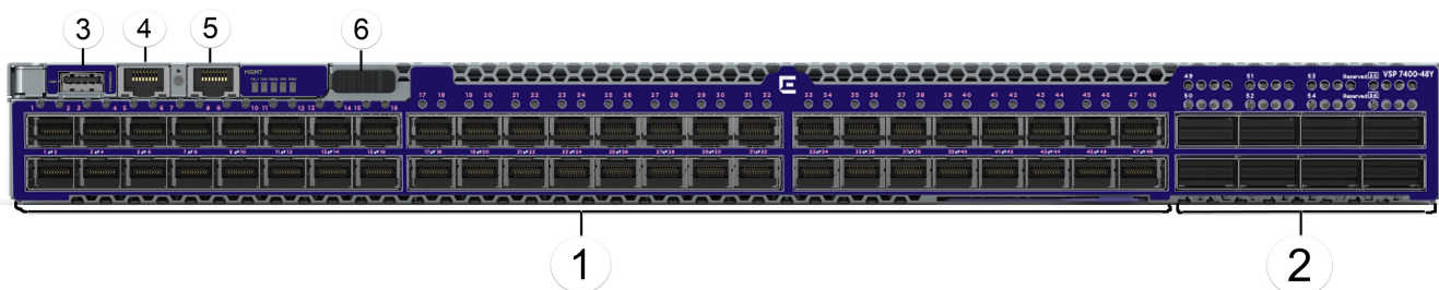
Figure 281: VSP 7400-48Y
