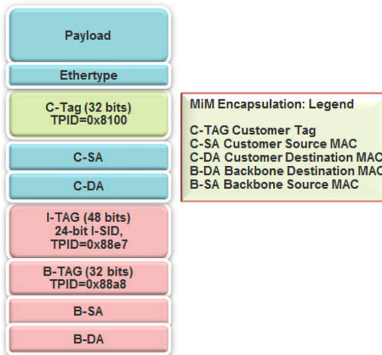
Figure 68: MiM encapsulation
