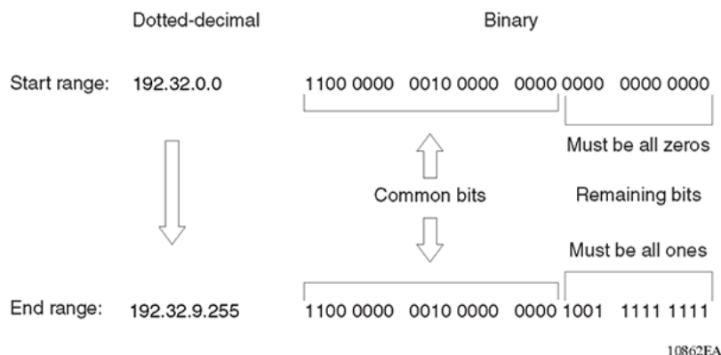
Figure 12: Binary notation conversion
