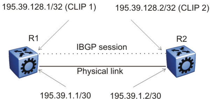
Figure 159: Routers with iBGP connections
