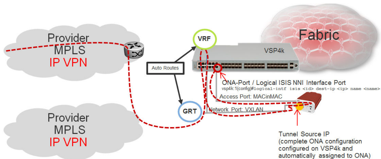
Figure 62: Autorouting between GRT and VRF
