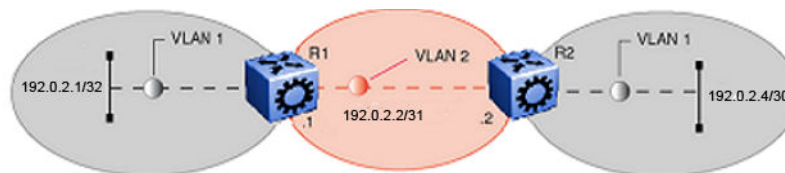
Figure 160: IP routing between VLANs
