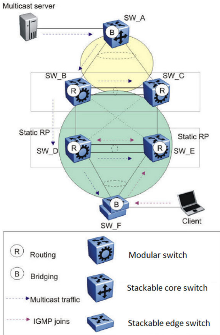
Figure 137: Multicast behavior in SMLT environment
