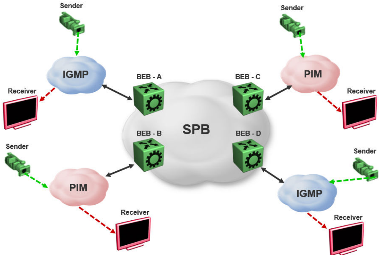
Figure 233: IP Multicast over Fabric Connect Streams
