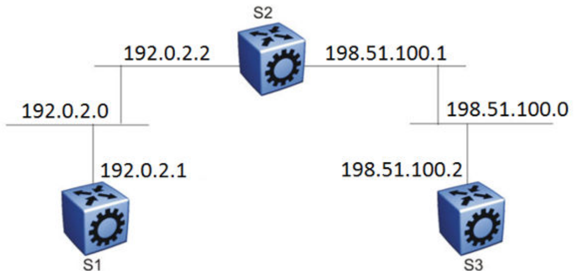
Figure 205: Example 2: OSPF on two subnets in one area
