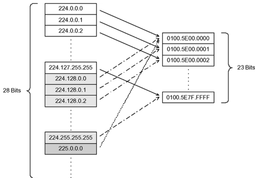
Figure 136: Multicast IP address to MAC address mapping
