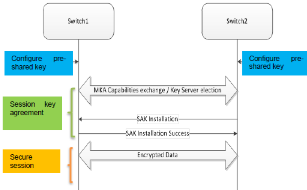
Figure 185: Switch to switch MACsec deployment scenario
