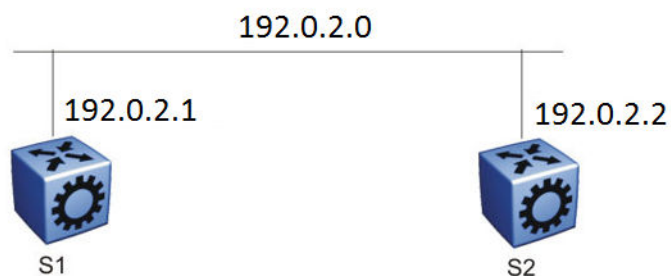
Figure 204: Example 1: OSPF on one subnet in one area
