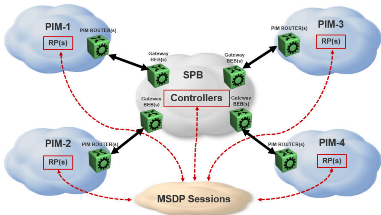
Figure 234: Multicast over Fabric Connect with SPB-PIM GW
