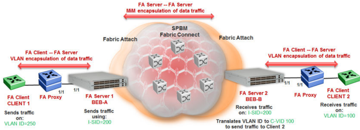
Figure 67: Data encapsulation – VLAN encapsulation and MiM encapsulation
