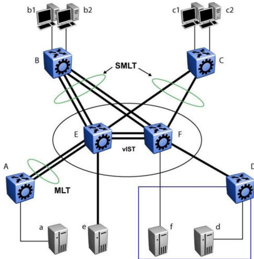
Figure 187: SMLT aggregation switches and operations
