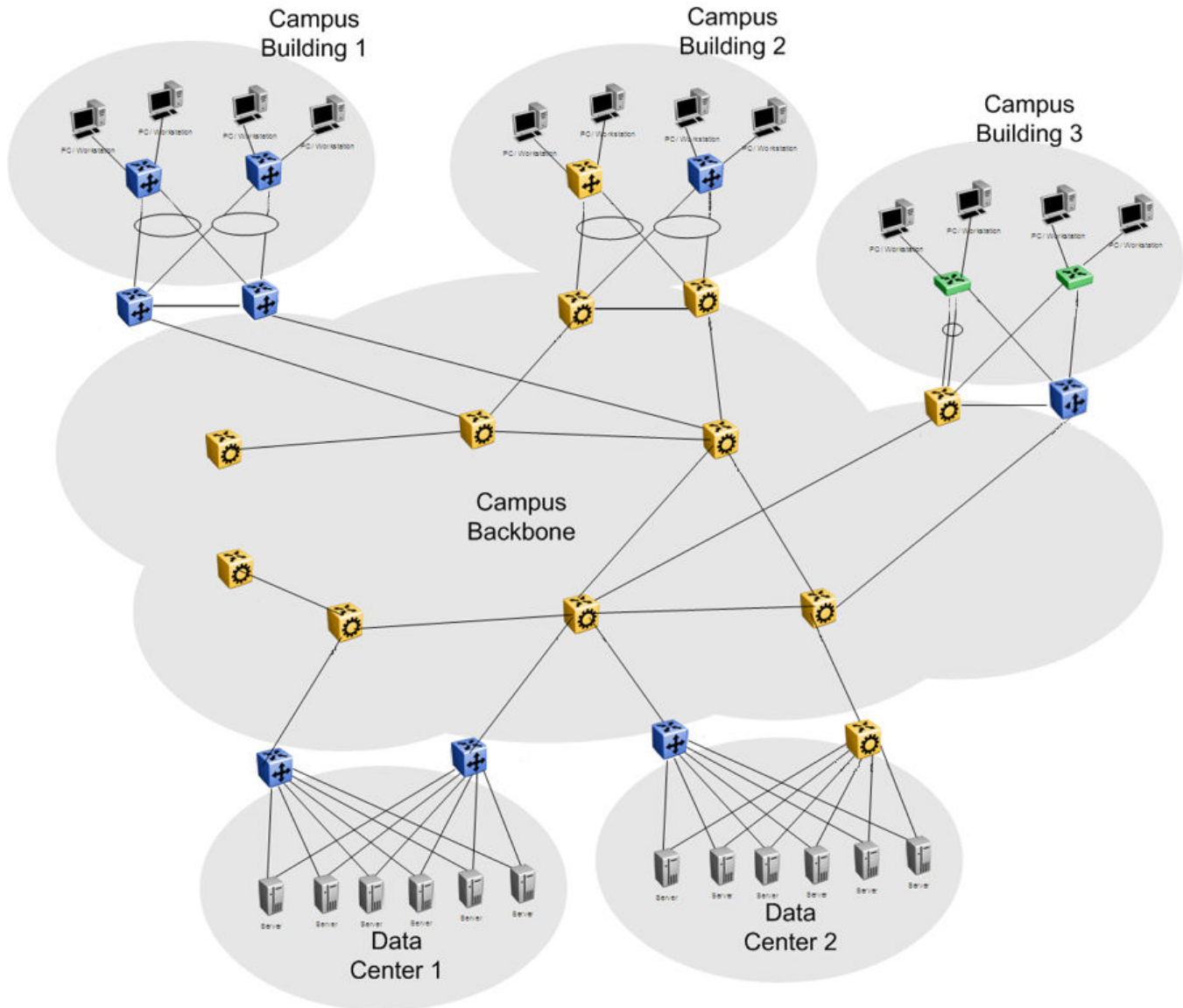
Figure 116: SPBM IP shortcuts in a campus
