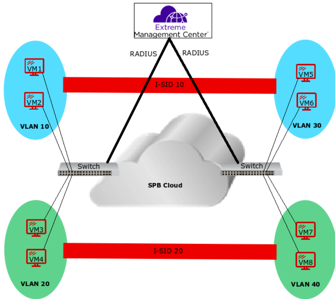
Figure 71: Endpoint Tracking Example
