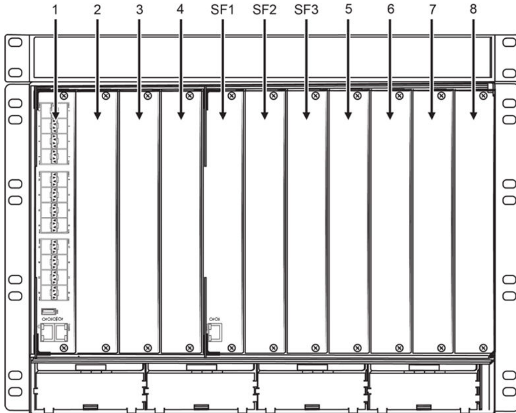
Figure 284: VSP 8608 front view
