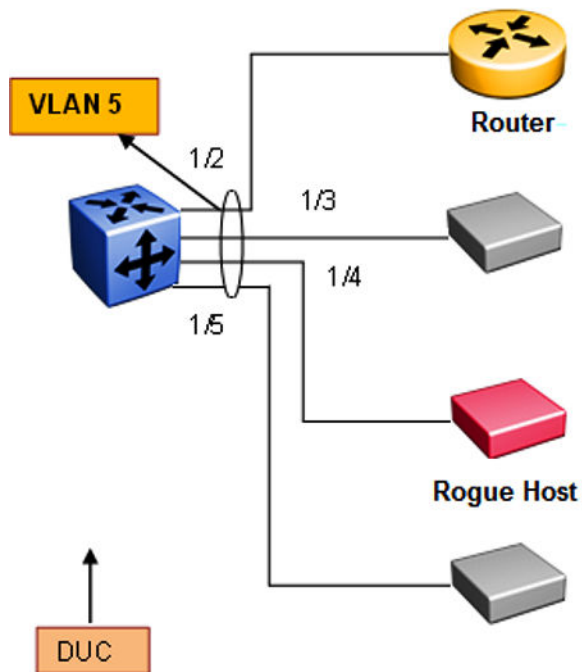
Figure 174: RA Guard Topology1
