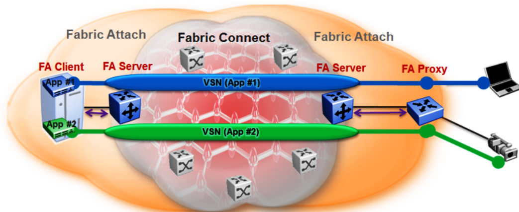
Figure 63: Fabric Attach Server connecting client or proxy devices to the Fabric network
