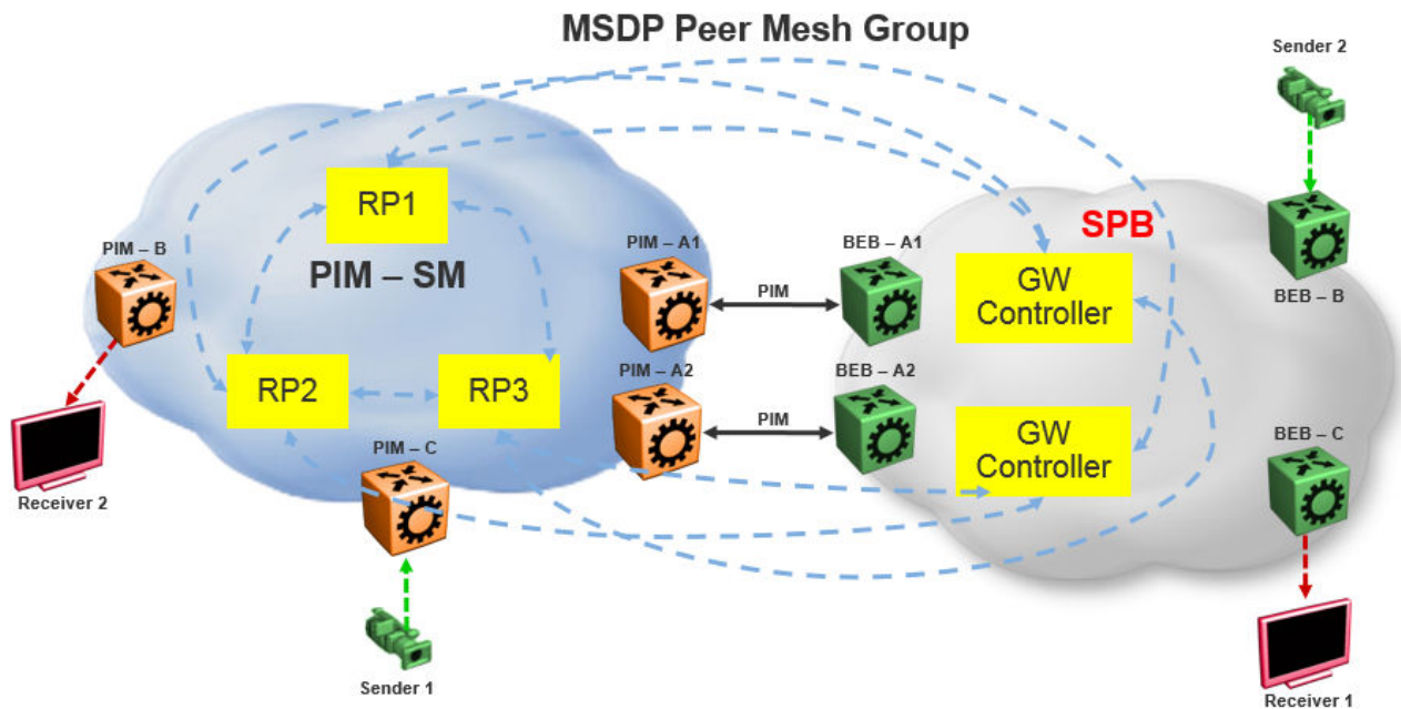
Figure 238: Peer Mesh Group
