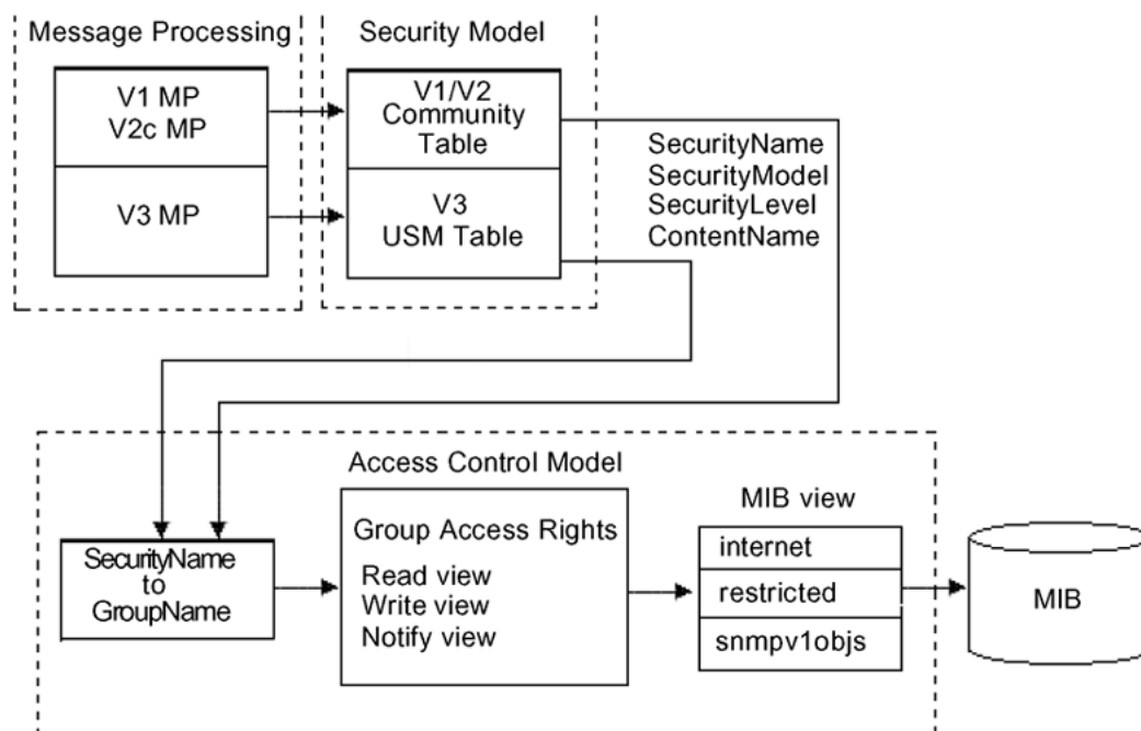
Figure 228: USM association with VACM
