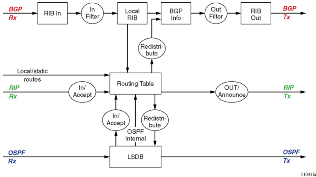
Figure 219: Route filtering for BGP, RIP, and OSPF routing protocols
