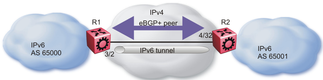
Figure 32: eBGP+ peers with IPv6 tunneling
