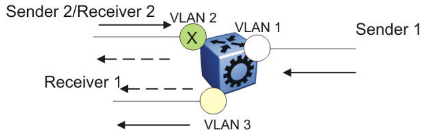
Figure 131: Data flow using deny-both policy
