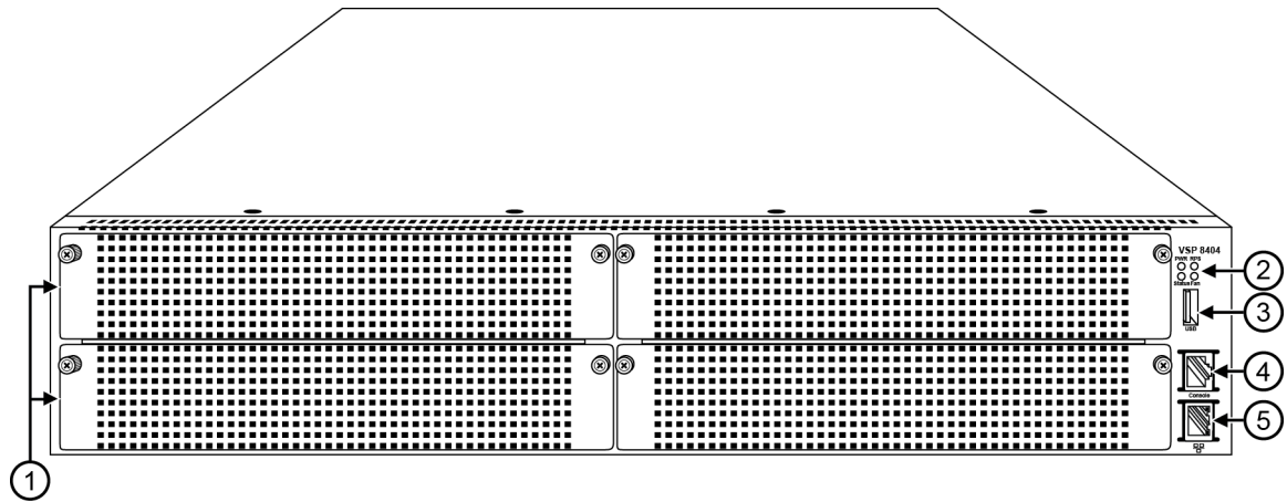
Figure 283: VSP 8404 front view
