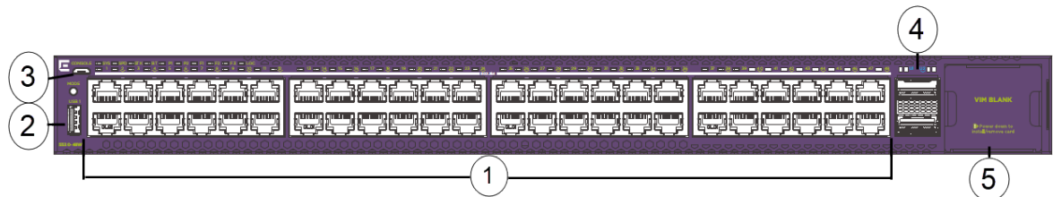
Figure 273: 5520-48W
