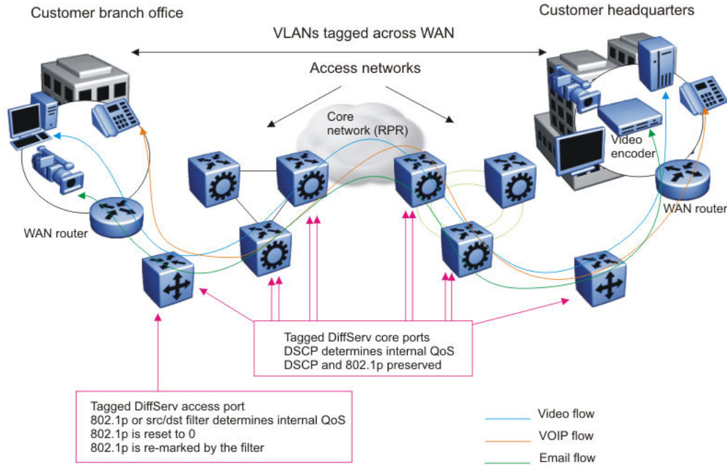
Figure 212: Trusted routed traffic
