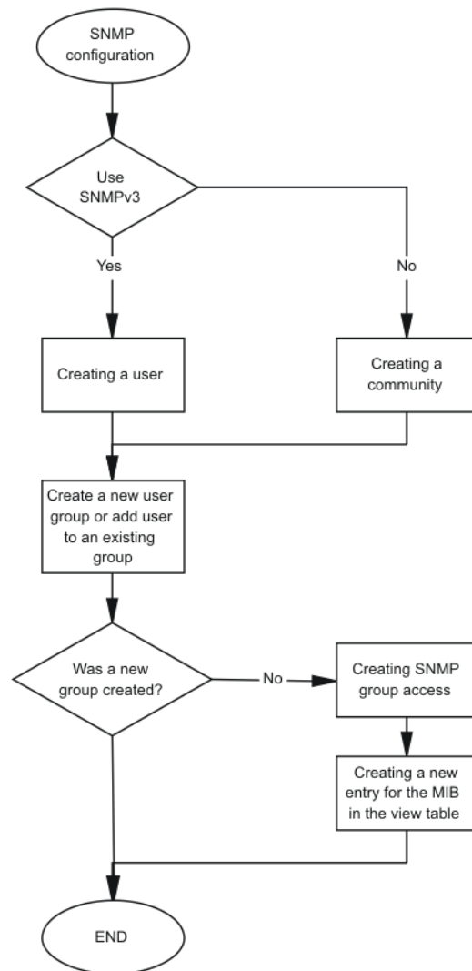
Figure 230: SNMP configuration using Enterprise Device Manager procedures
