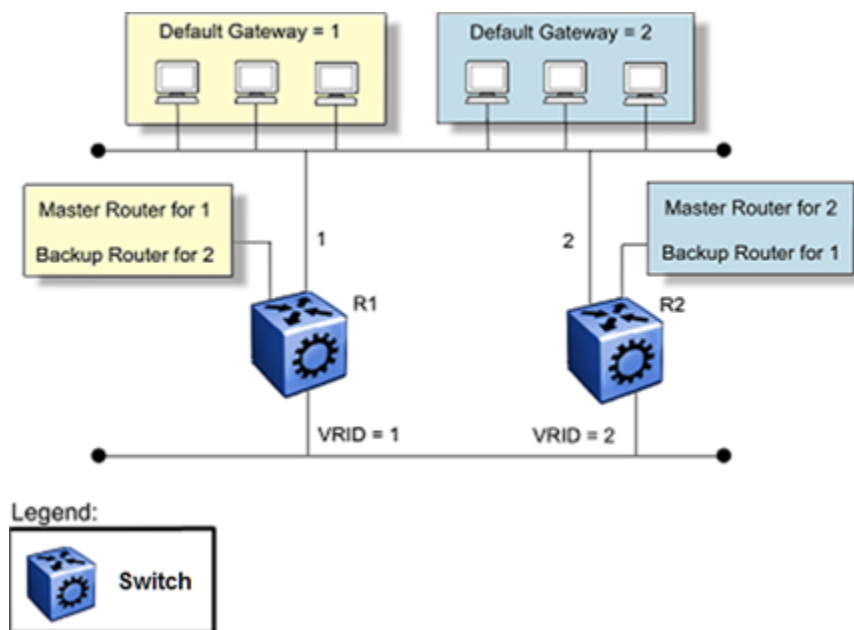
Figure 261: Virtual Router Redundancy Protocol configuration
