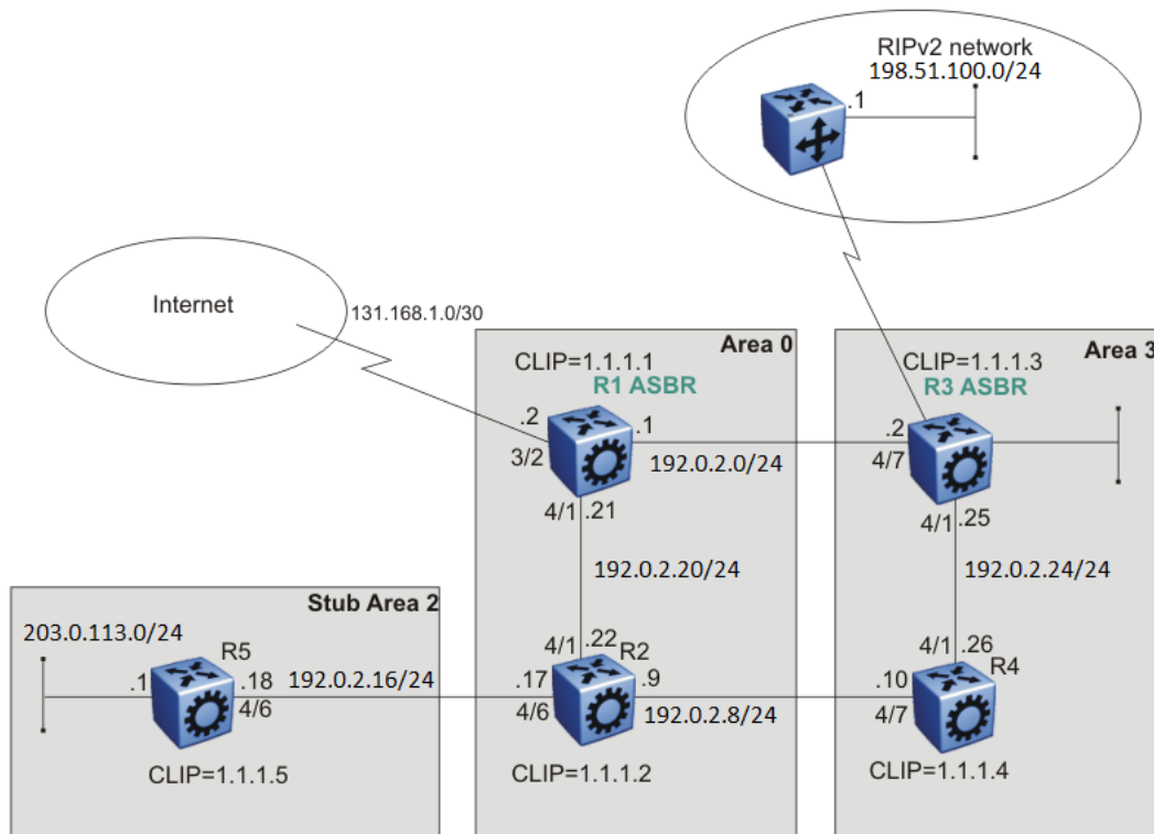
Figure 199: Multiarea configuration example
