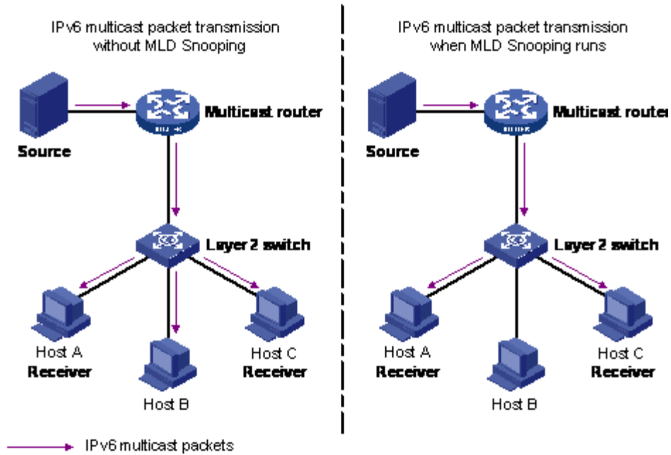
Figure 144: IPv6 multicast packet transmission when MLD snooping is enabled and not enabled
