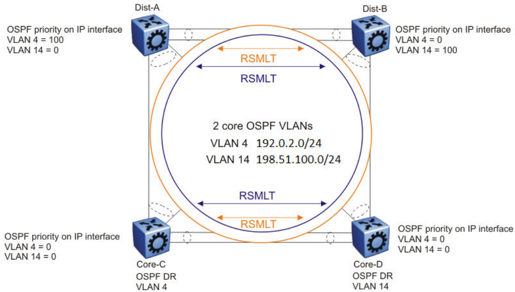
Figure 203: RSMLT with dual core VLANs
