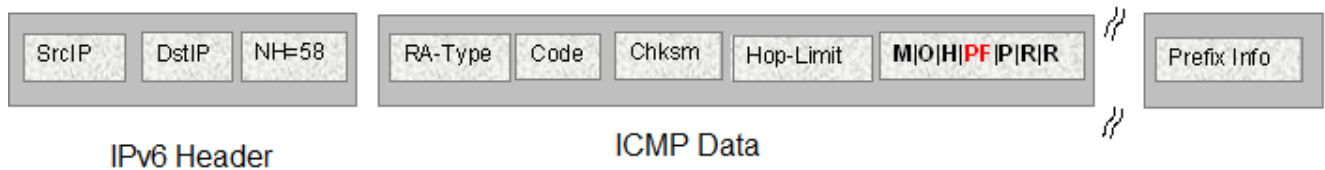
Figure 180: IPv6 ICMP RA data packet outline for router preference validation
