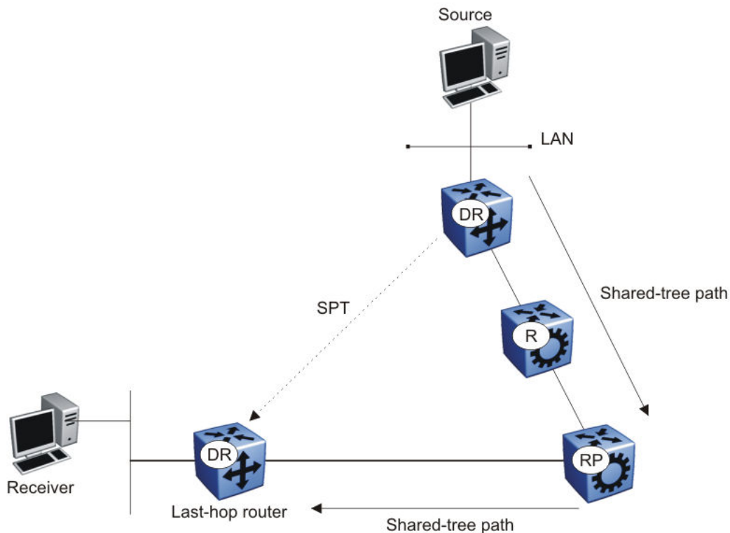
Figure 132: Shared tree and shortest-path tree
