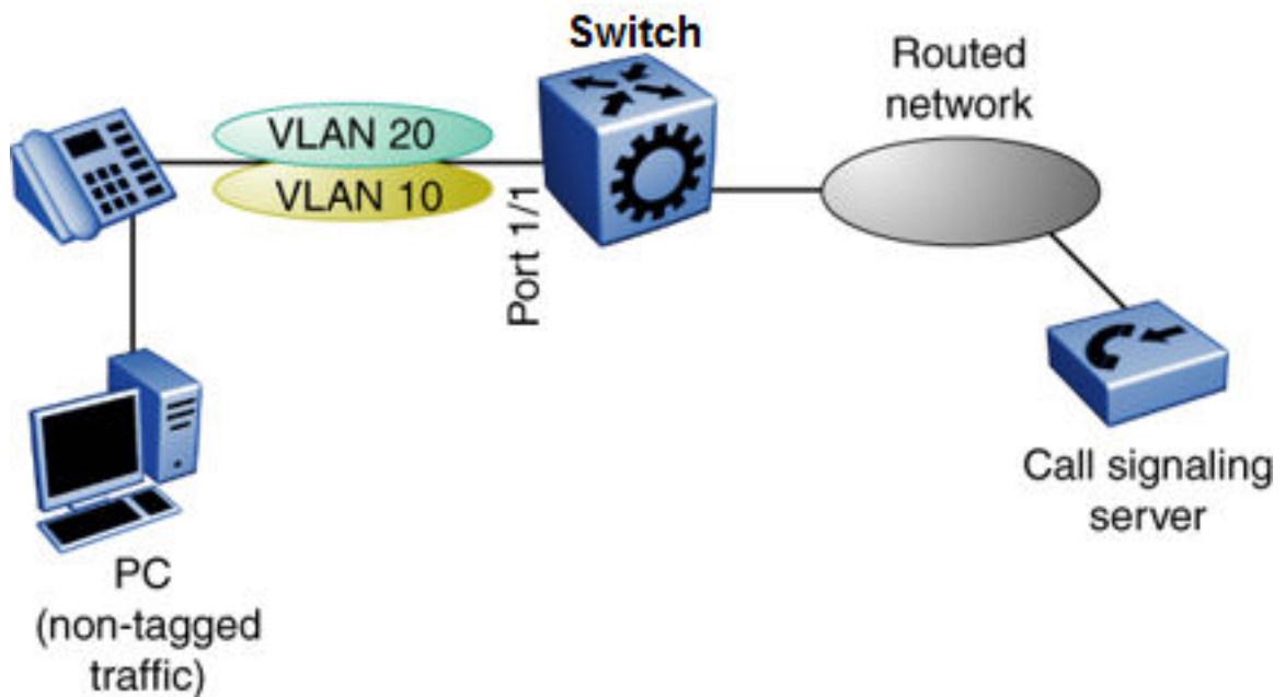
Figure 254: Network with IP phone and PC
