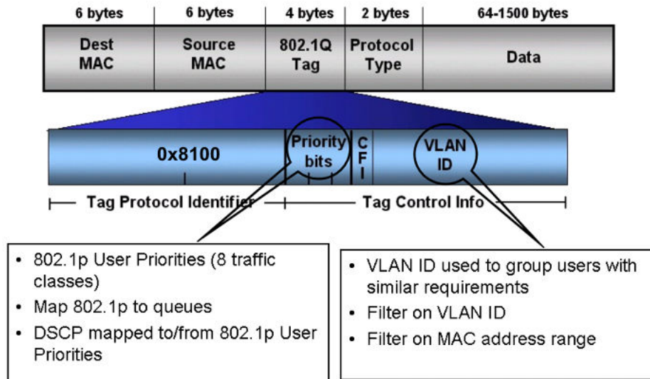
Figure 253: VLAN tag insertion
