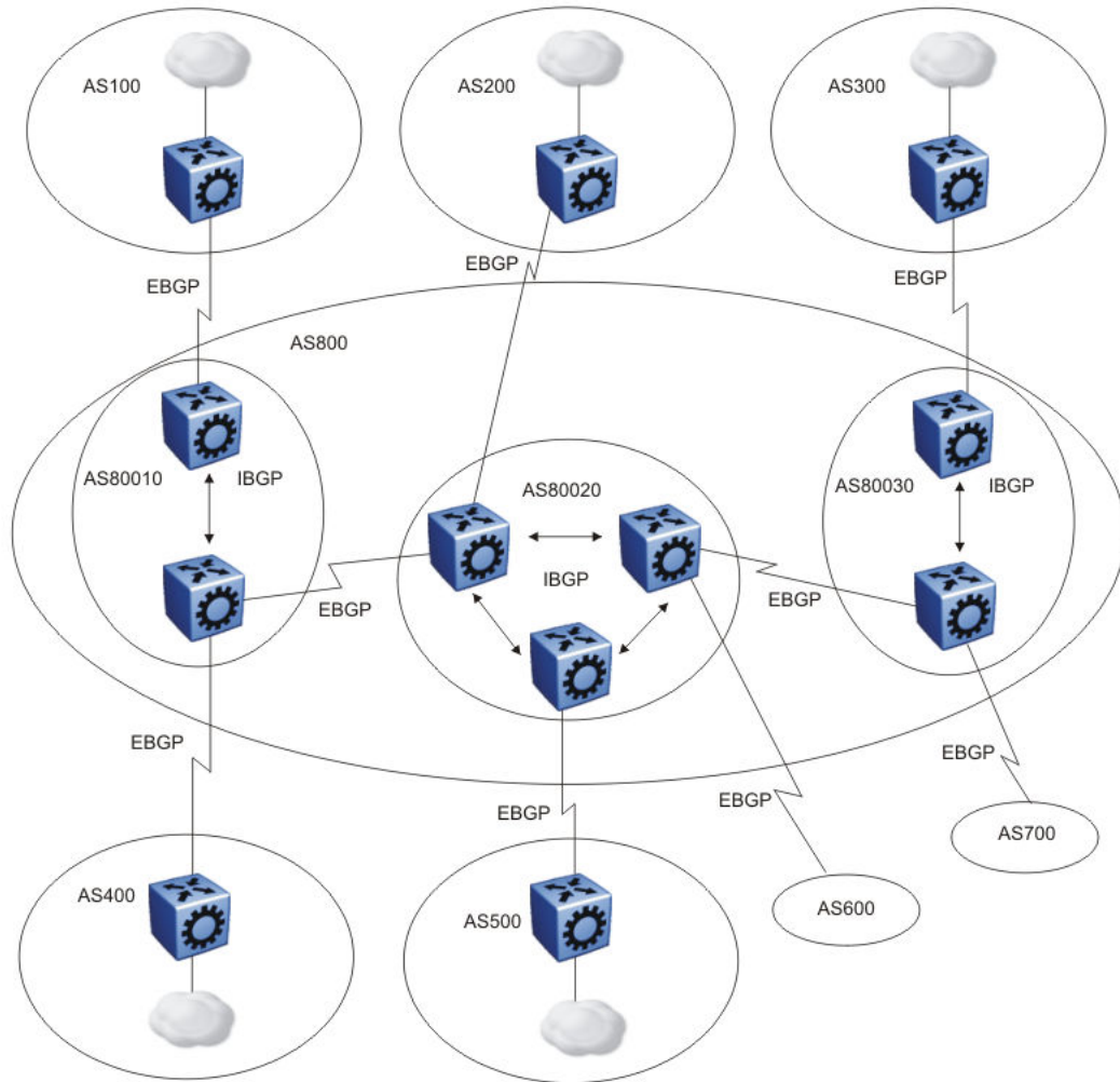
Figure 16: Confederations
