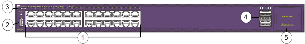
Figure 270: 5520-24T
