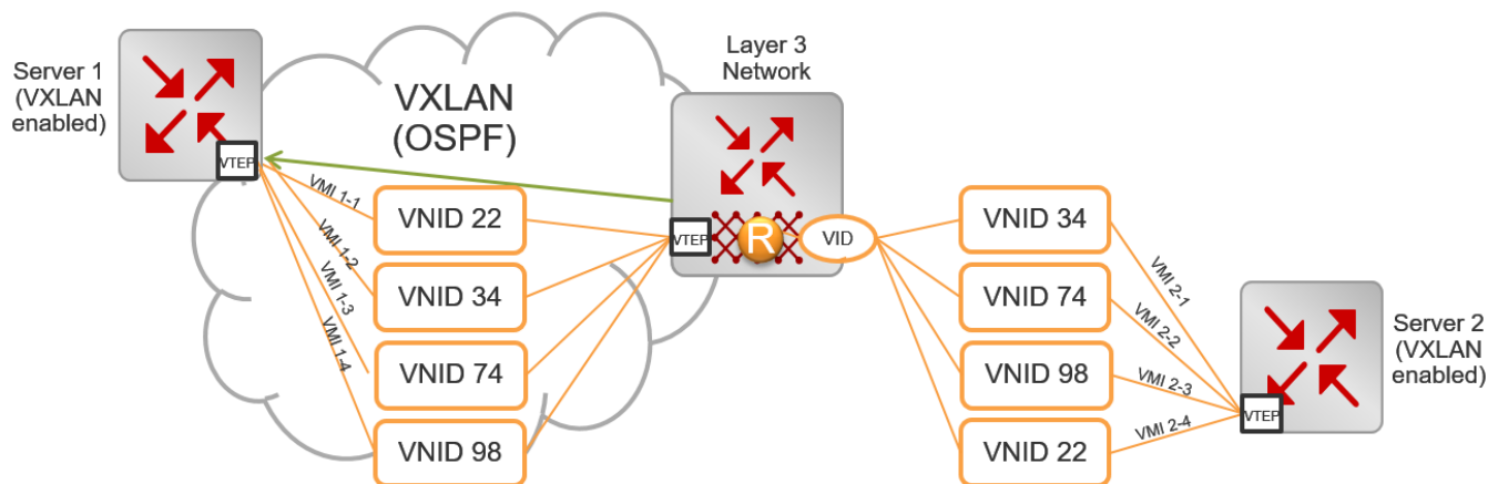
Figure 267: VXLAN-to-VXLAN deployment
