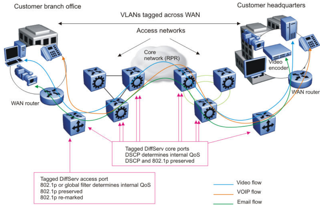
Figure 210: Trusted bridged traffic
