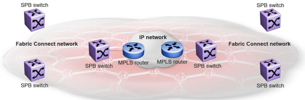
Figure 61: Fabric Extend over IPsec Deployment Option
