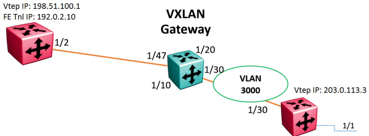
Figure 269: VXLAN Gateway configuration example
