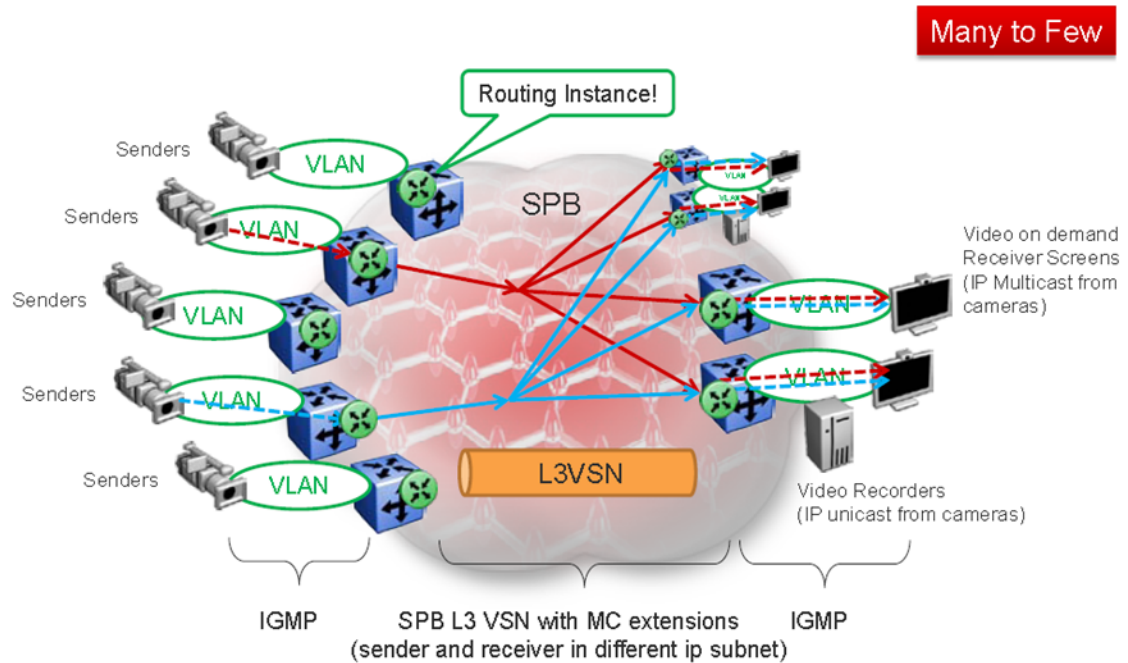
Figure 113: Deployment scenario — Routed video surveillance and IP camera deployment for transportation, airports, and government
