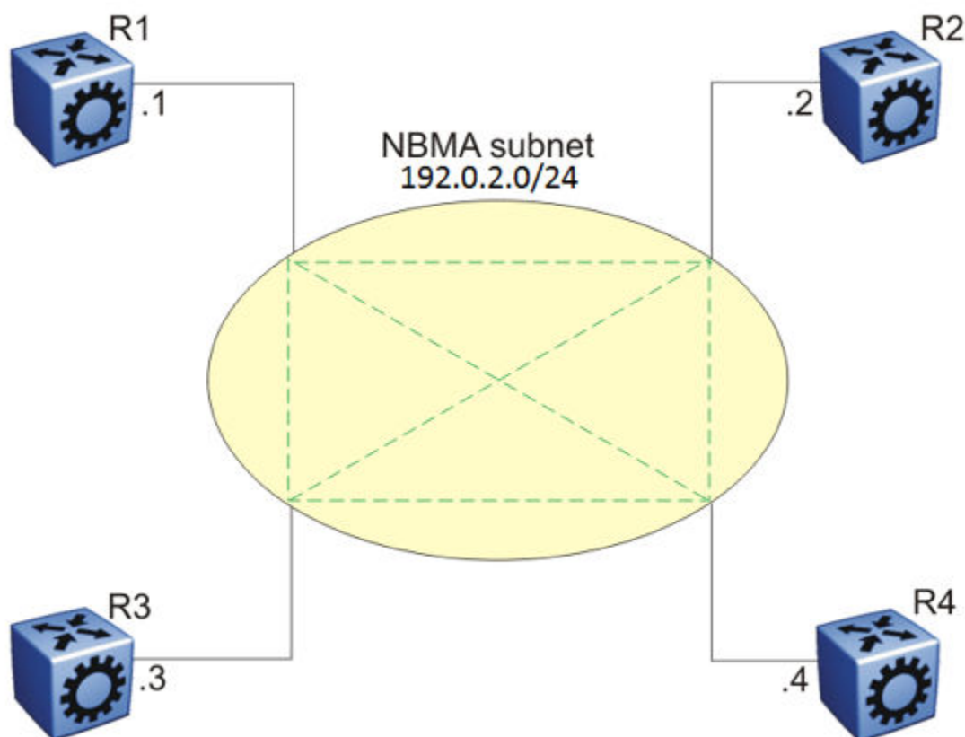
Figure 200: NBMA Subnet
