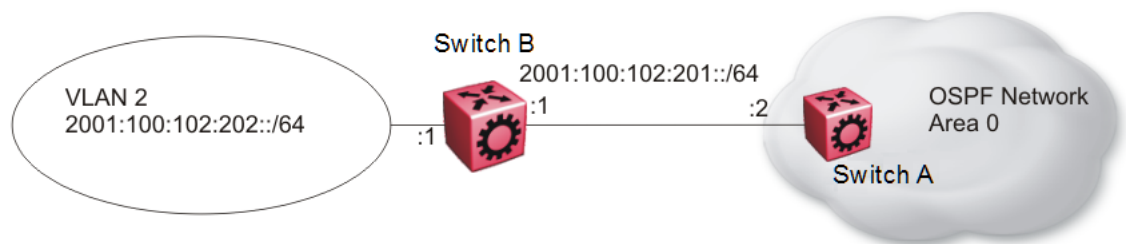
Figure 207: OSPFv3 configuration
