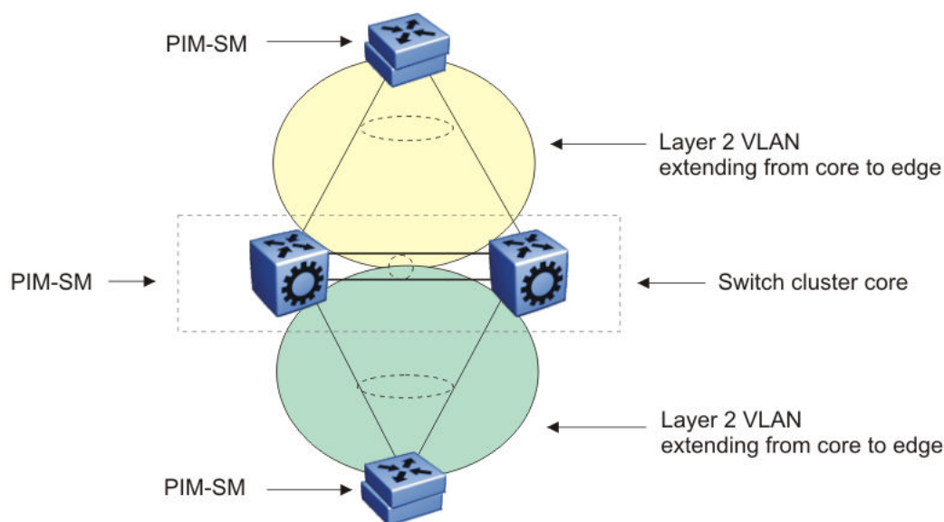
Figure 139: Multicast SMLT triangle
