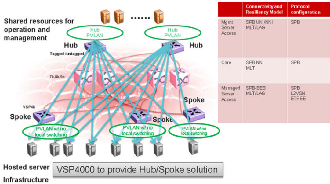
Figure 111: Data center hosting private VLAN
