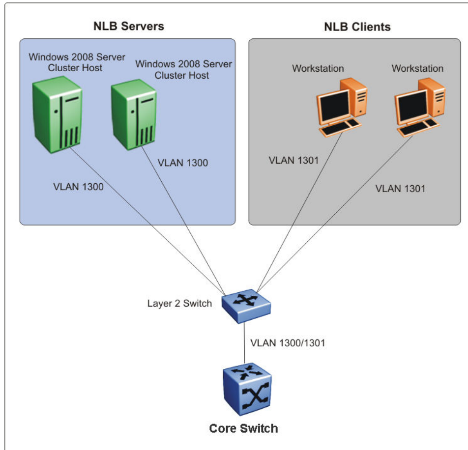
Figure 256: Supported NLB topology-example 2
