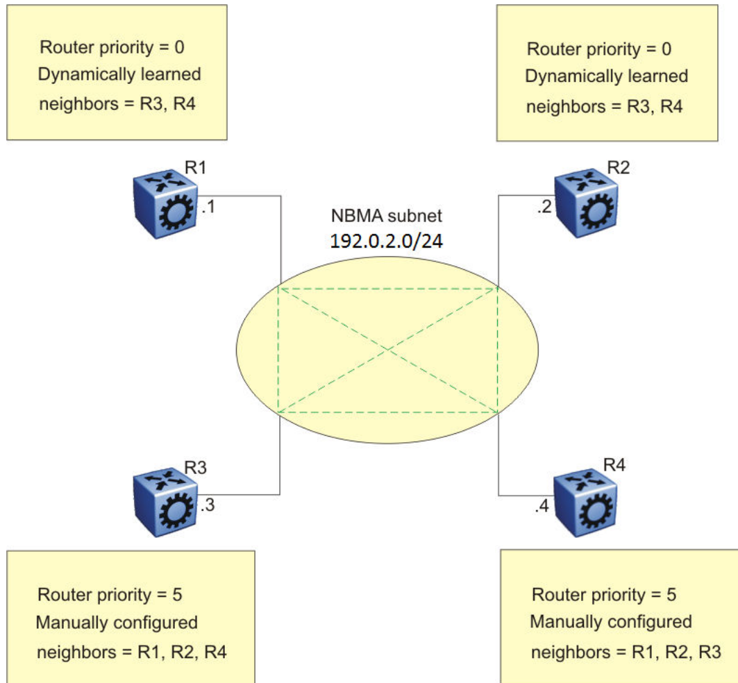
Figure 201: NBMA Subnet Configuration Example
