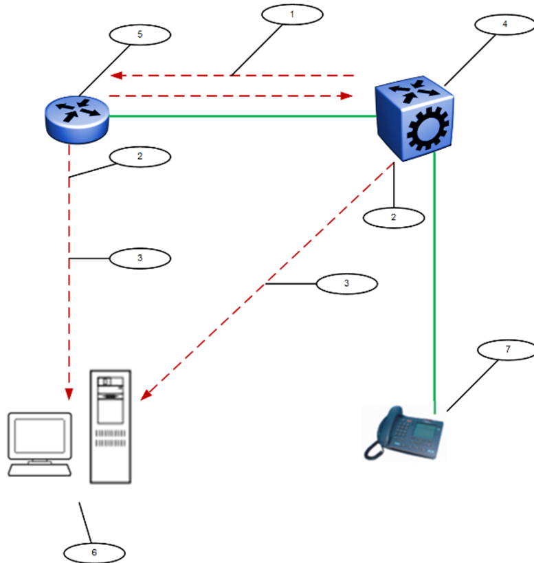
Figure 183: LLDP in a LAN
