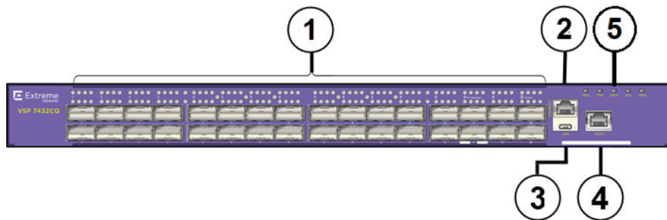
Figure 280: VSP 7432CQ
