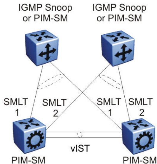
Figure 138: Multicast routing using PIM-SM
