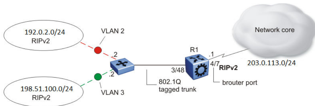
Figure 215: Configuration example-RIPv2 only
