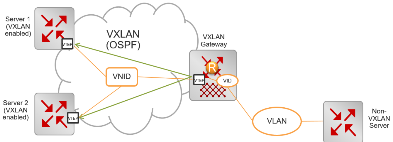
Figure 266: VXLAN-to-VLAN deployment
