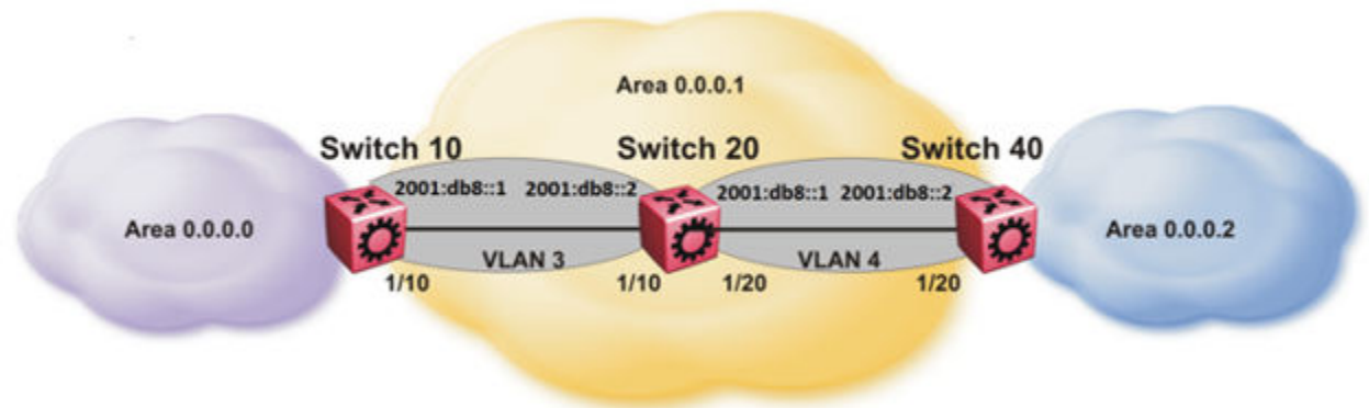
Figure 156: OSPFv3 virtual link with IPsec configuration
