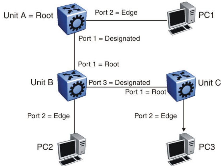
Figure 231: RSTP negotiation process
