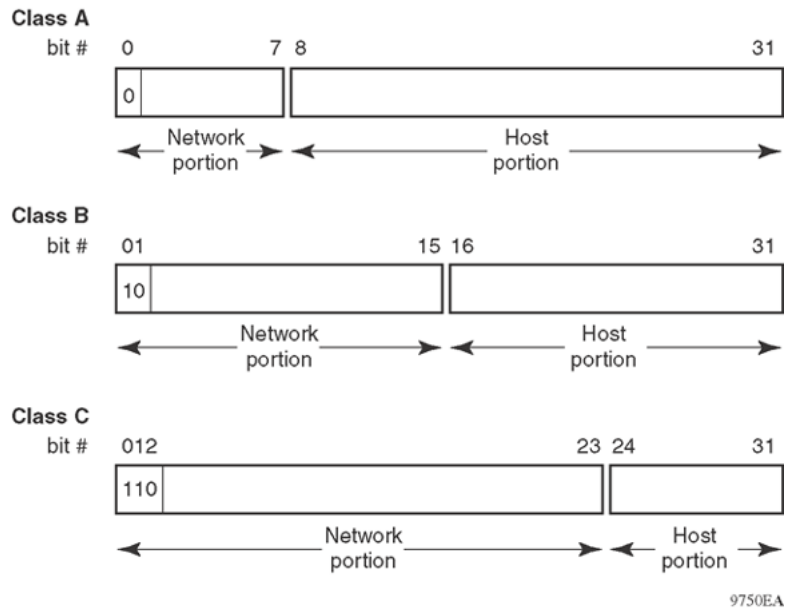
Figure 157: Network and host boundaries in IP address classes
