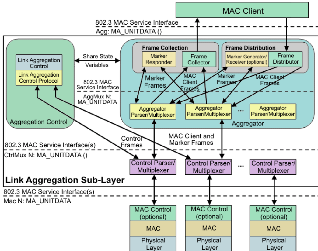
Figure 182: Link aggregation sublayer (according to IEEE 802.3ad)
