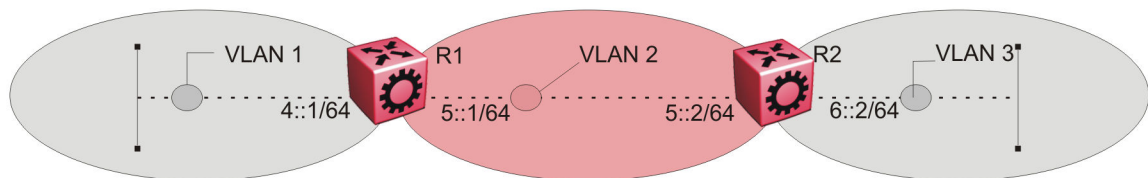
Figure 168: IPv6 routing between VLANs
