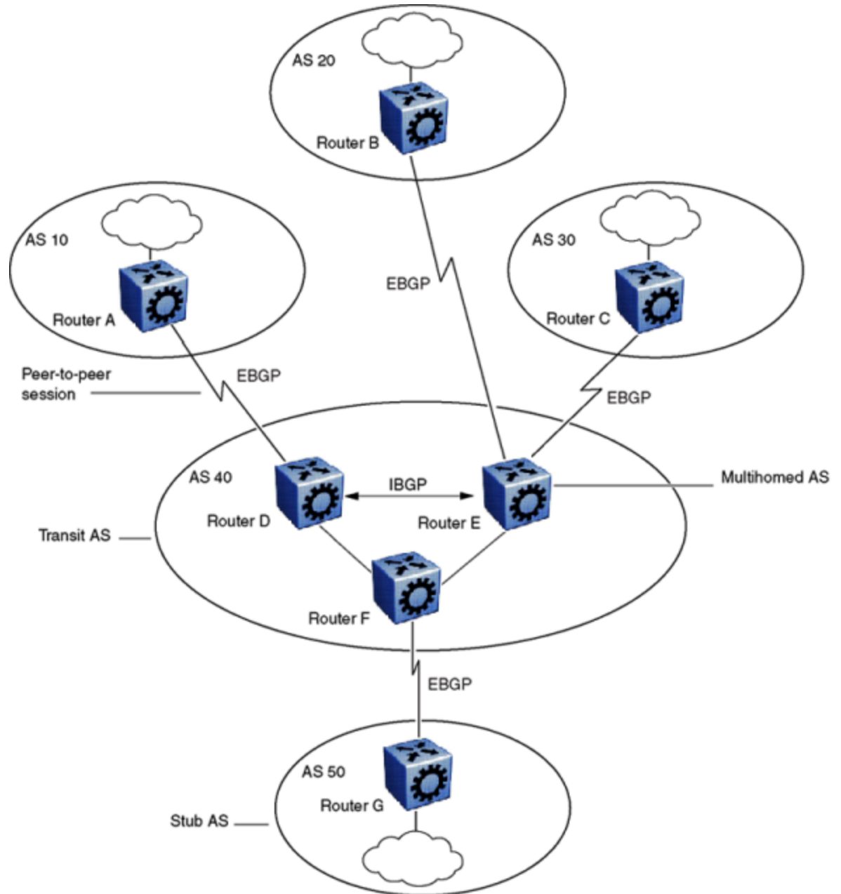
Figure 10: BGP networks
