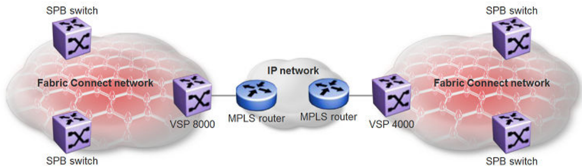
Figure 53: Fabric Connect networks connected by an IP network
