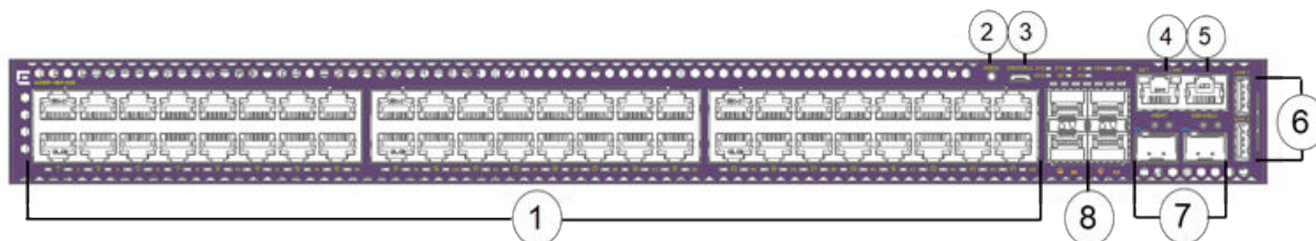
Figure 279: 5420F-48P-4XE Front Panel
