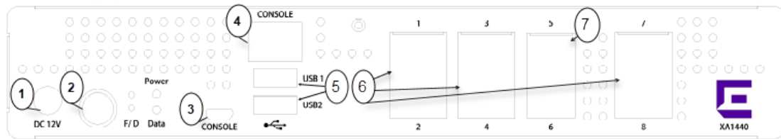
Figure 302: XA1400 Series switches rear panel
