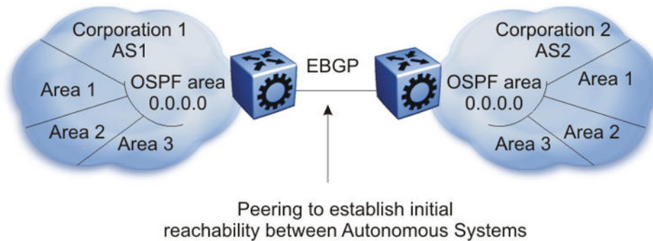
Figure 26: Routing Domain Interconnection with BGP
