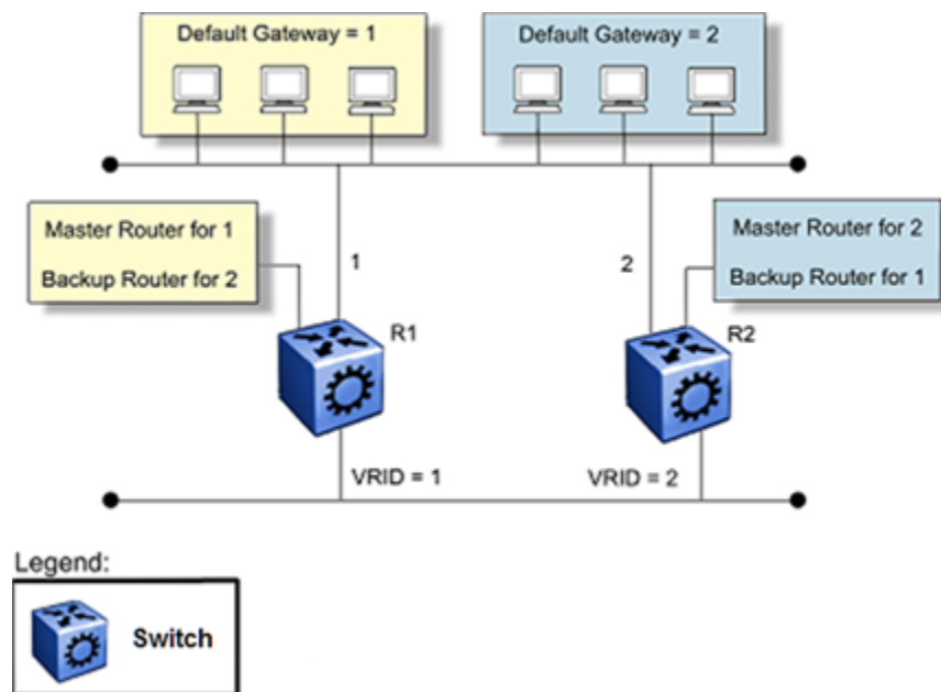
Figure 264: Virtual Router Redundancy Protocol configuration
