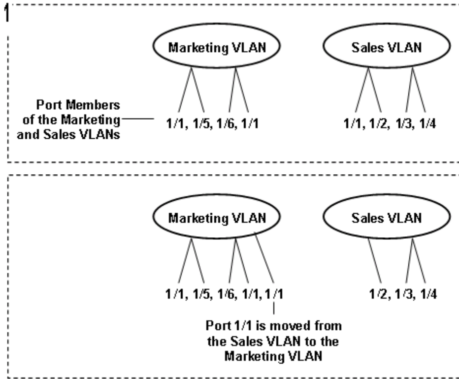
Figure 254: Port-based VLAN
