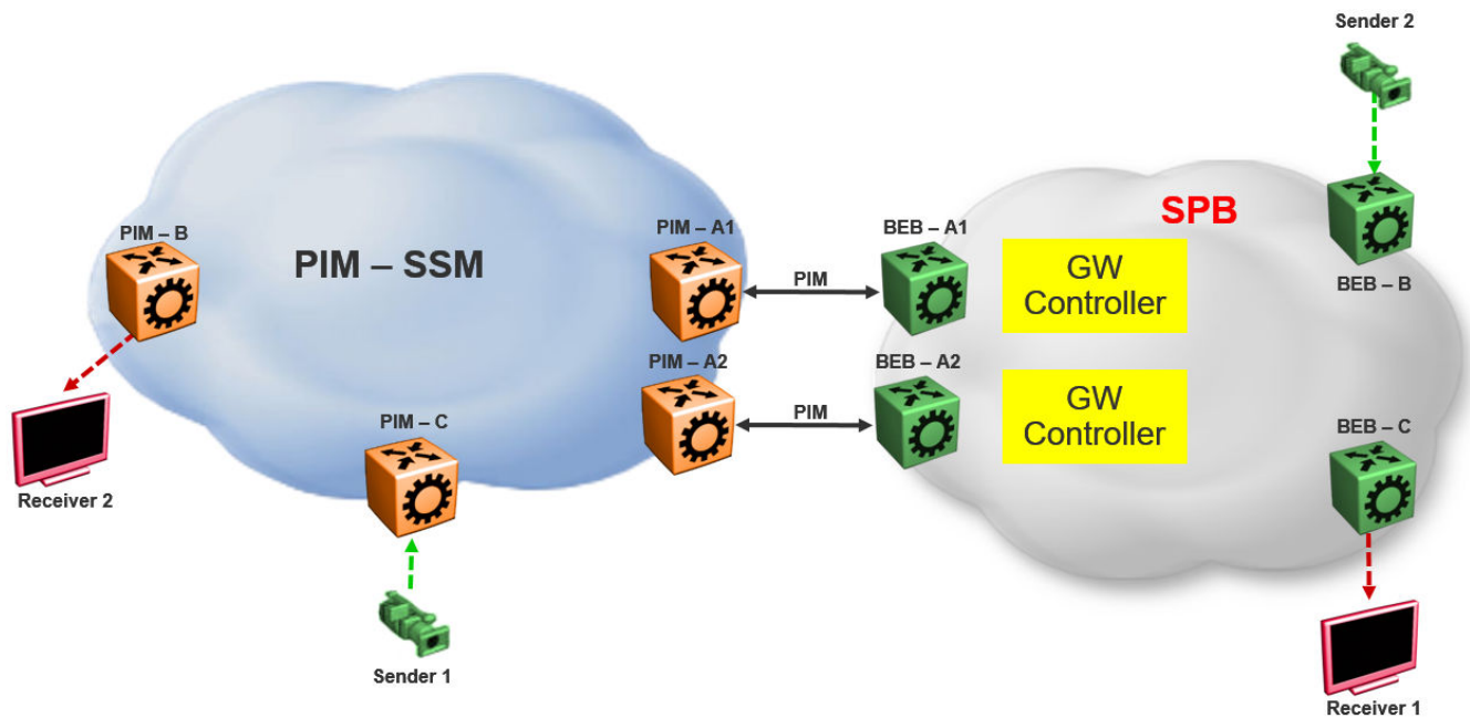
Figure 240: Static configuration of SSM groups in Controllers
