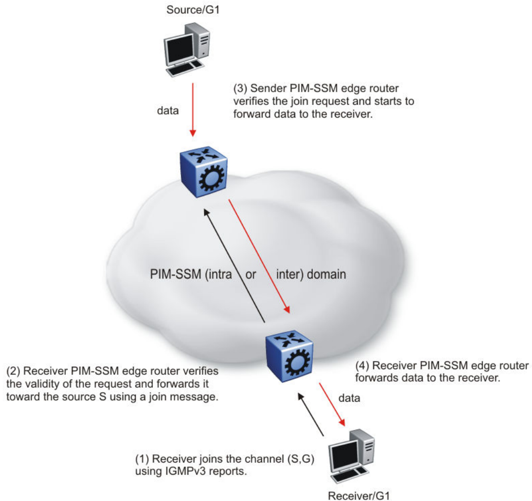
Figure 135: PIM-SSM architecture
