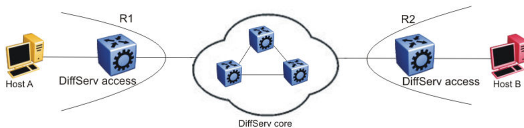
Figure 209: DiffServ network core and edge devices
