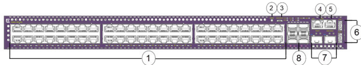
Figure 285: 5420M-48T-4YE Front Panel
