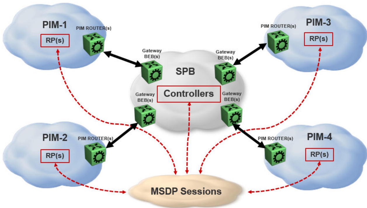
Figure 237: Multicast over Fabric Connect with SPB-PIM GW
