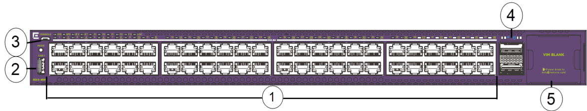
Figure 290: 5520-48W
