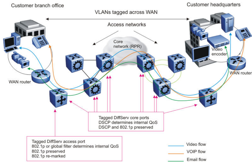
Figure 211: Trusted bridged traffic
