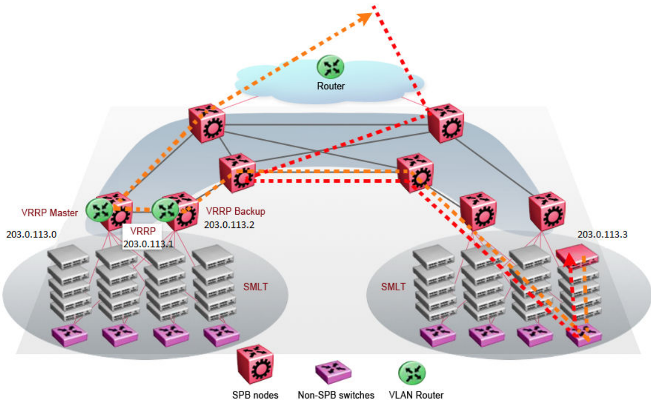
Figure 108: Traditional routing after moving VMs
