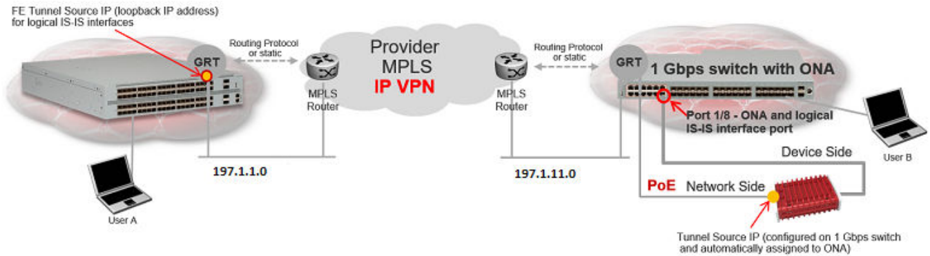
Figure 78: IP using GRT traffic flow
