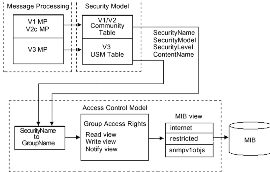
Figure 231: USM association with VACM
