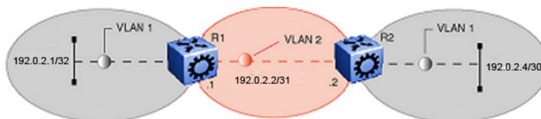
Figure 161: IP routing between VLANs
