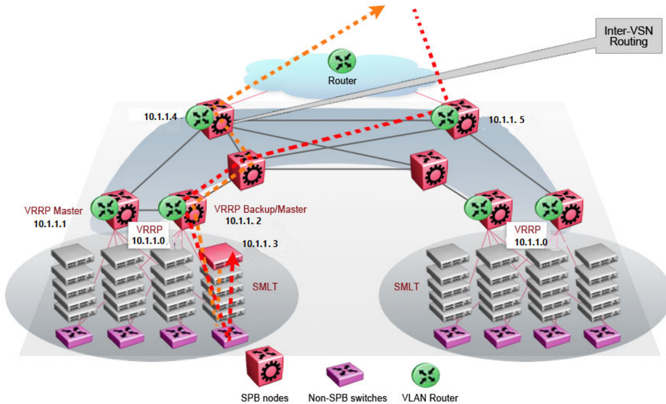
Figure 109: Optimized routing before moving VMs
