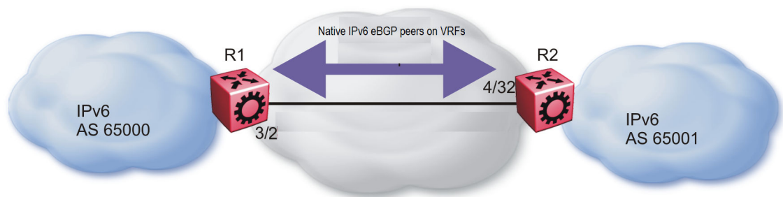
Figure 34: Native IPv6 eBGP peers on VRFs
