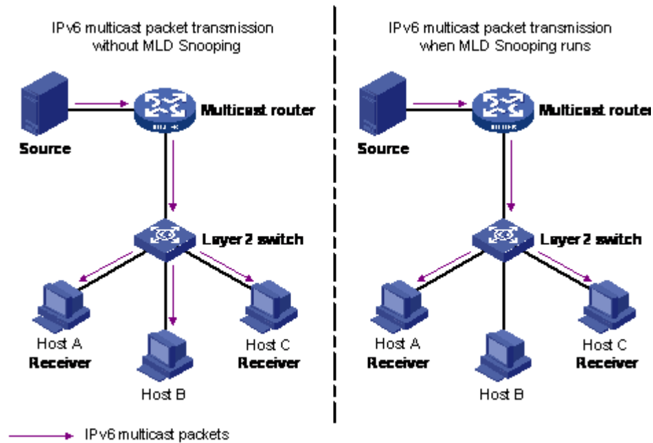
Figure 145: IPv6 multicast packet transmission when MLD snooping is enabled and not enabled
