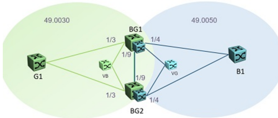
Figure 89: Multi-area SPB network example
