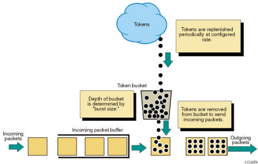
Figure 210: Token flow
