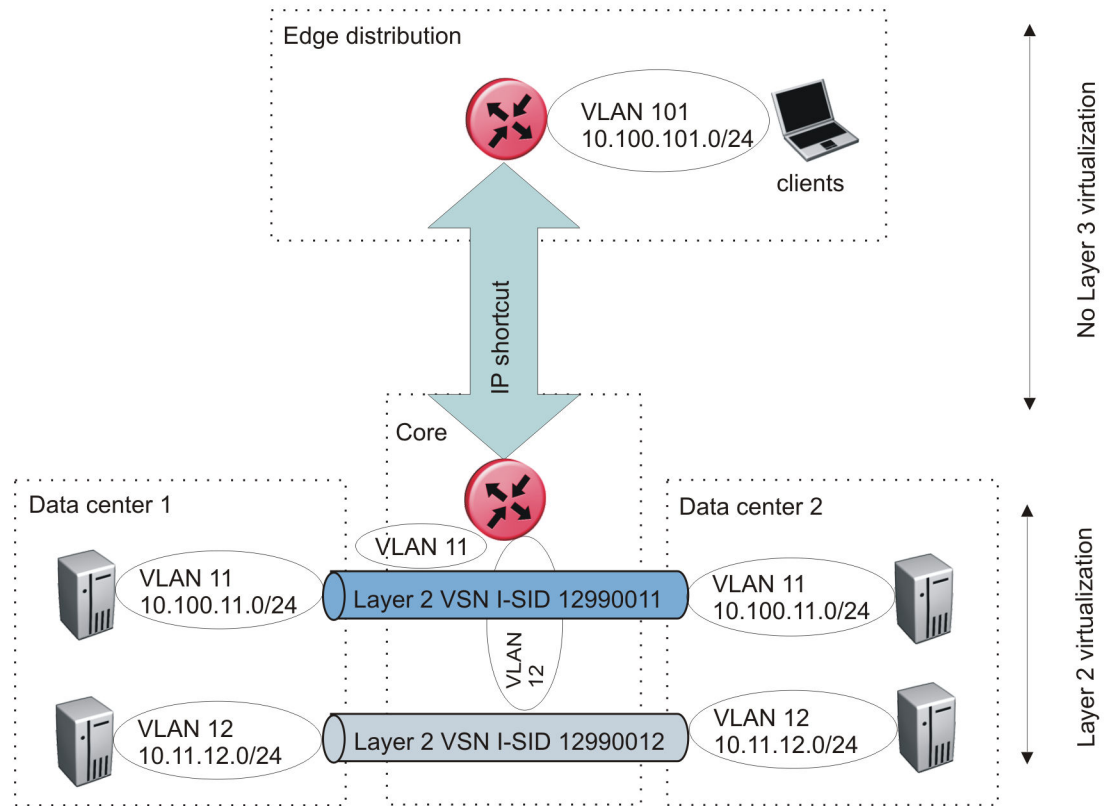
Figure 104: IP shortcut scenario to move traffic between data centers
