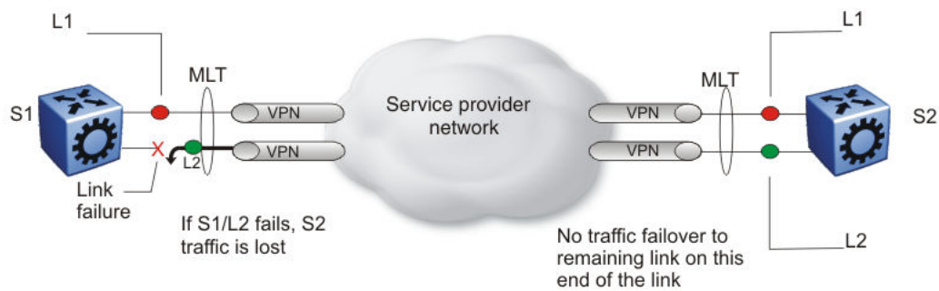
Figure 253: Problem description (2 of 2)
