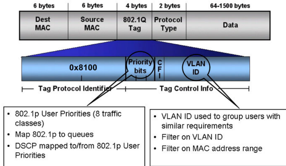
Figure 256: VLAN tag insertion
