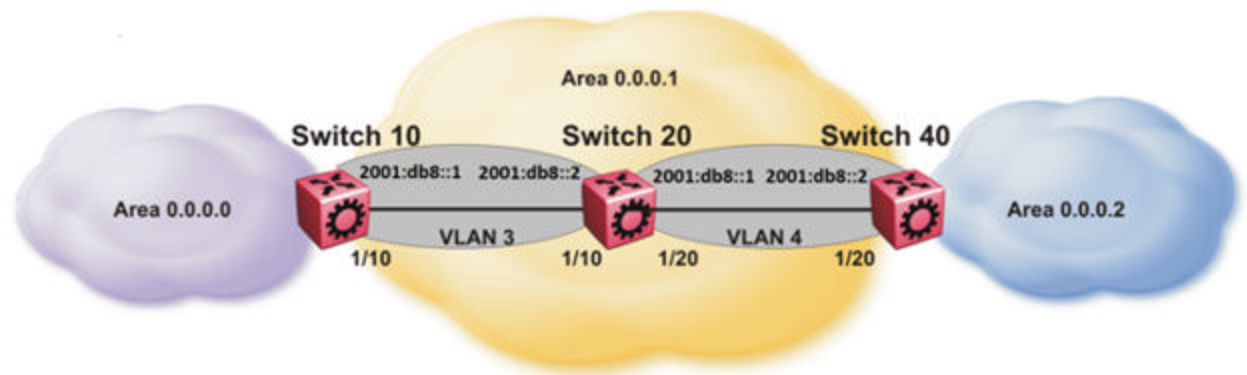
Figure 157: OSPFv3 virtual link with IPsec configuration
