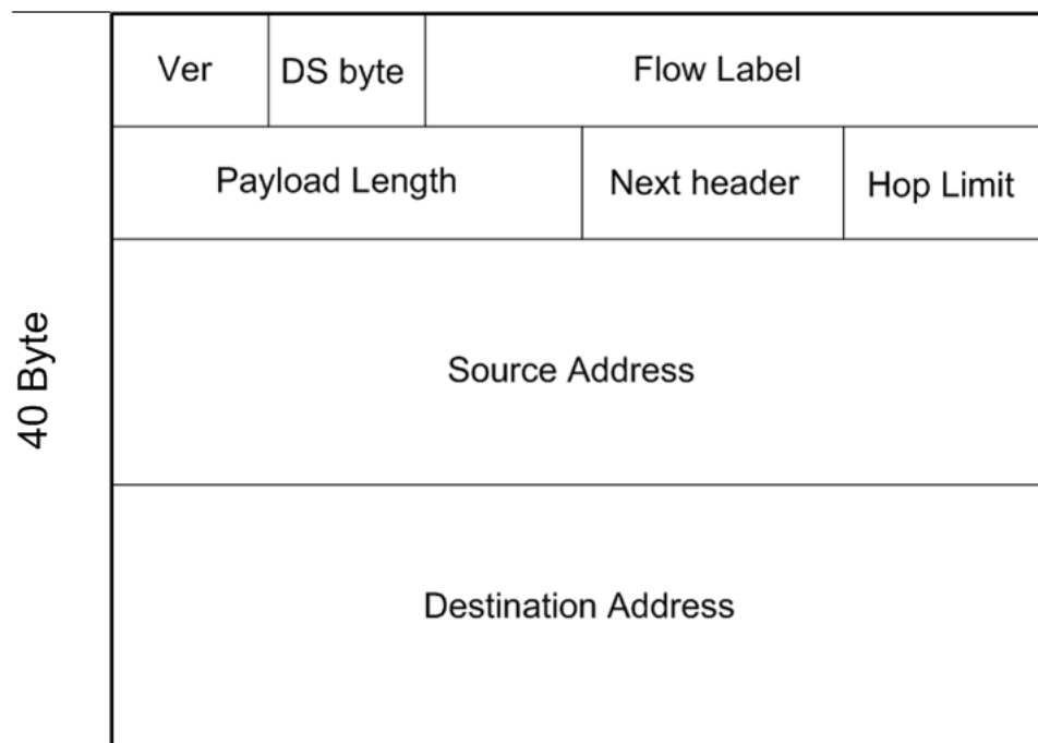
Figure 163: IPv6 header
