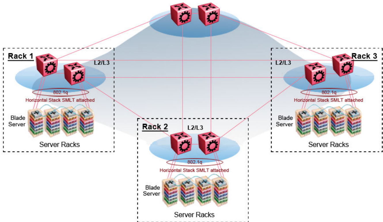
Figure 106: SPBM data center—full mesh
