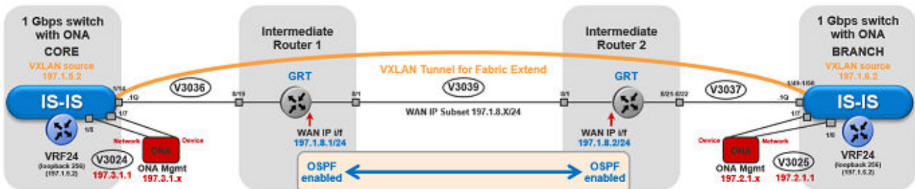
Figure 86: Fabric Extend traffic flow component view
