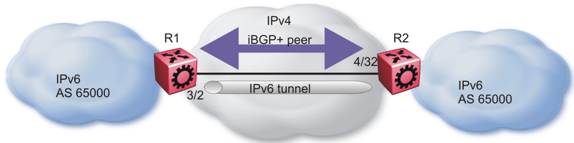
Figure 33: iBGP+ peers on CLIP interfaces with IPv6 tunneling
