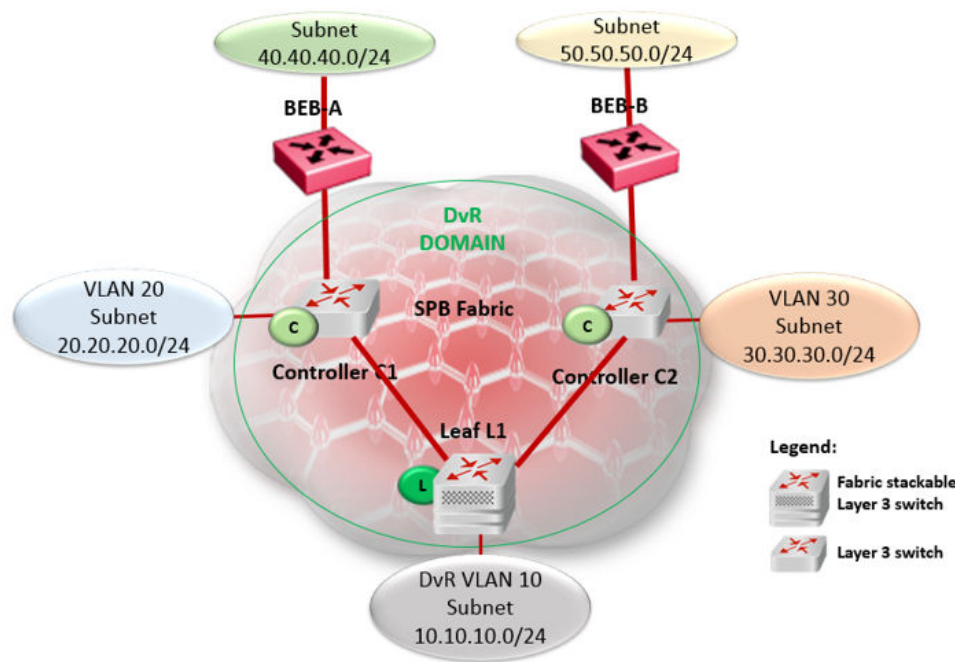
Figure 40: Redistribution of IPv4 local and static routes
