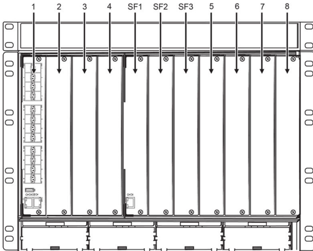
Figure 301: VSP 8608 front view
