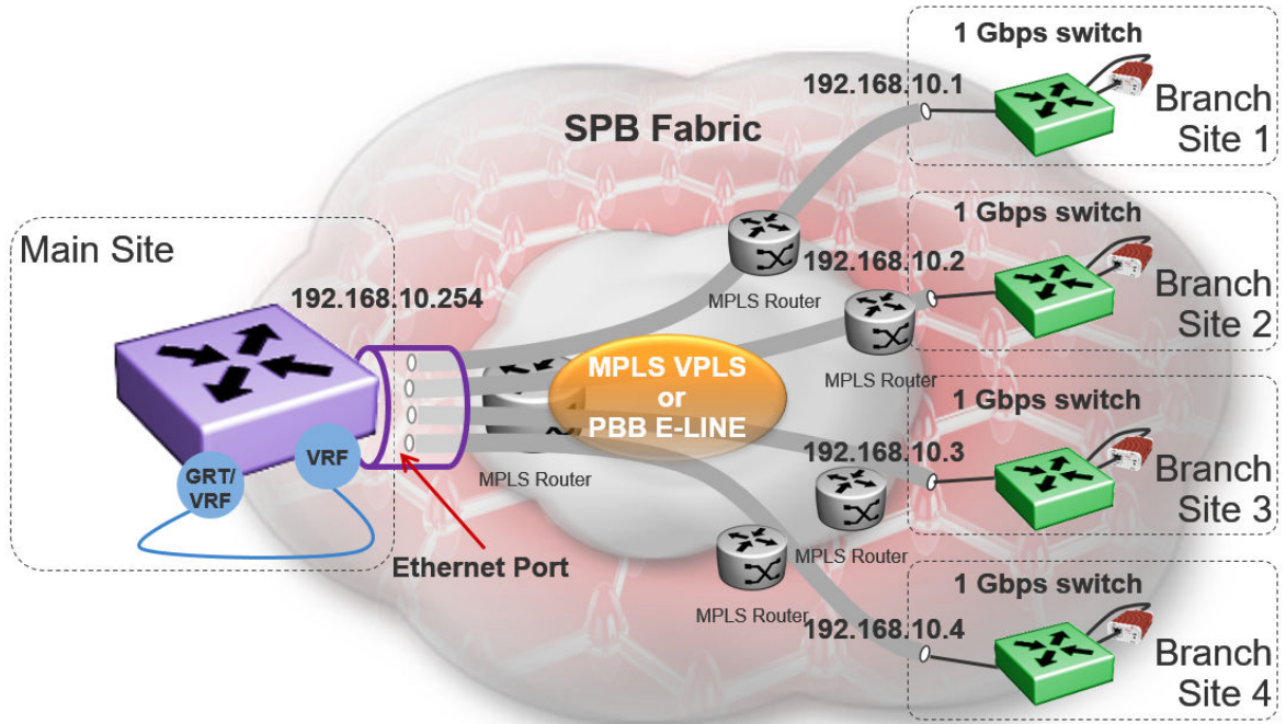
Figure 56: Fabric Extend VPLS Deployment Option
