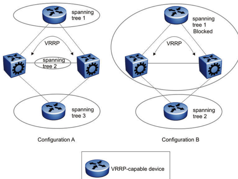
Figure 267: VRRP and STG configurations
