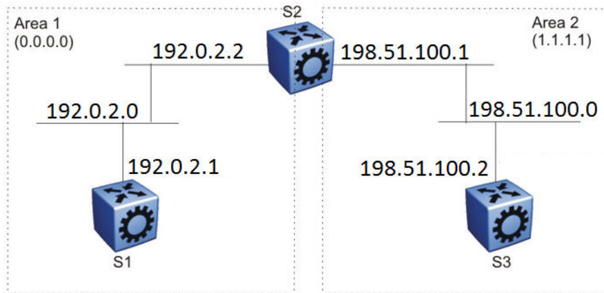
Figure 207: Example 3: OSPF on two subnets in two areas
