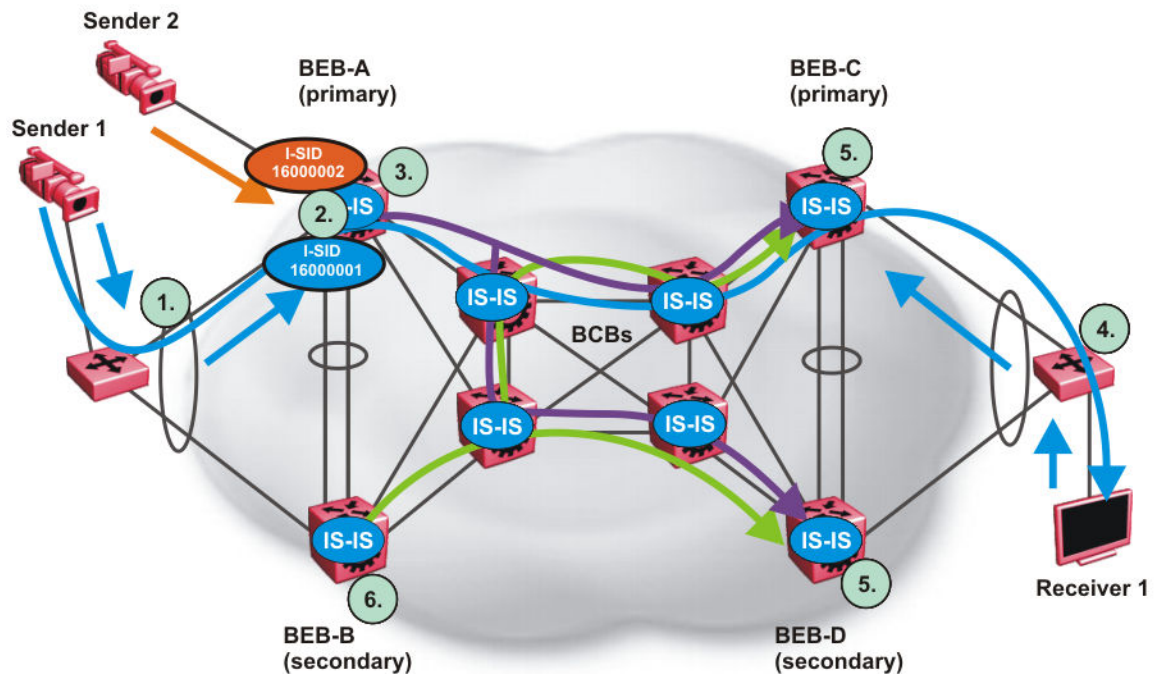
Figure 148: IP Multicast over Fabric Connect streams in an SMLT configuration
