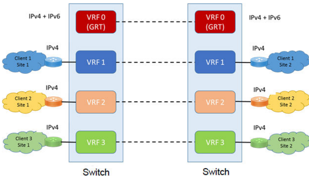
Figure 261: Multiple virtual routers in one system
