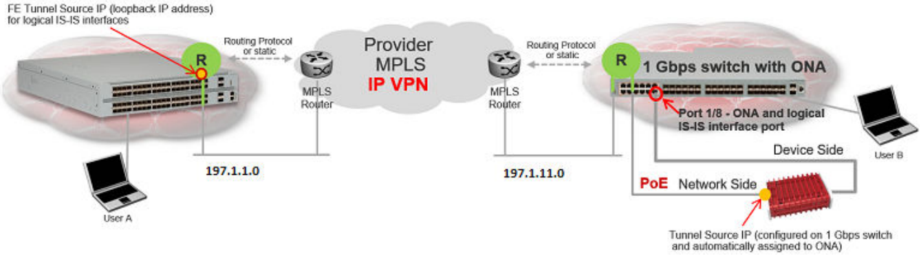
Figure 80: IP using VRF traffic flow
