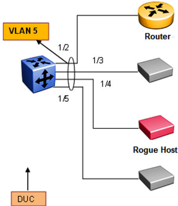
Figure 175: RA Guard Topology1
