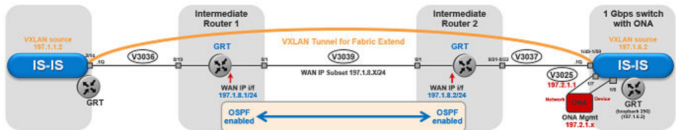
Figure 79: IP (GRT) traffic flow component view
