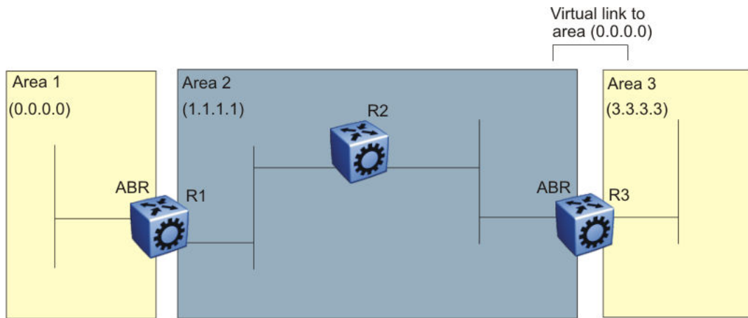
Figure 203: Virtual link between ABRs through a transit area
