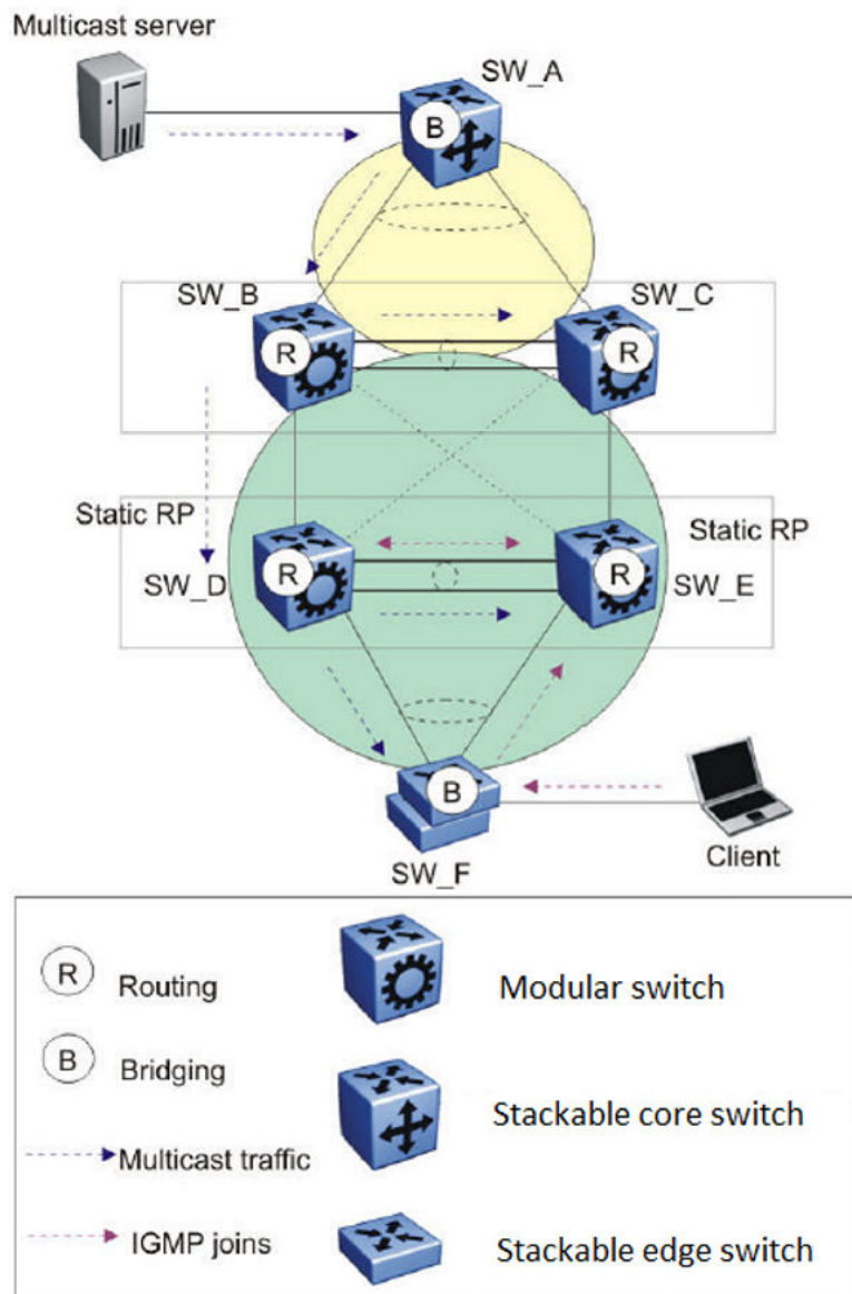
Figure 138: Multicast behavior in SMLT environment
