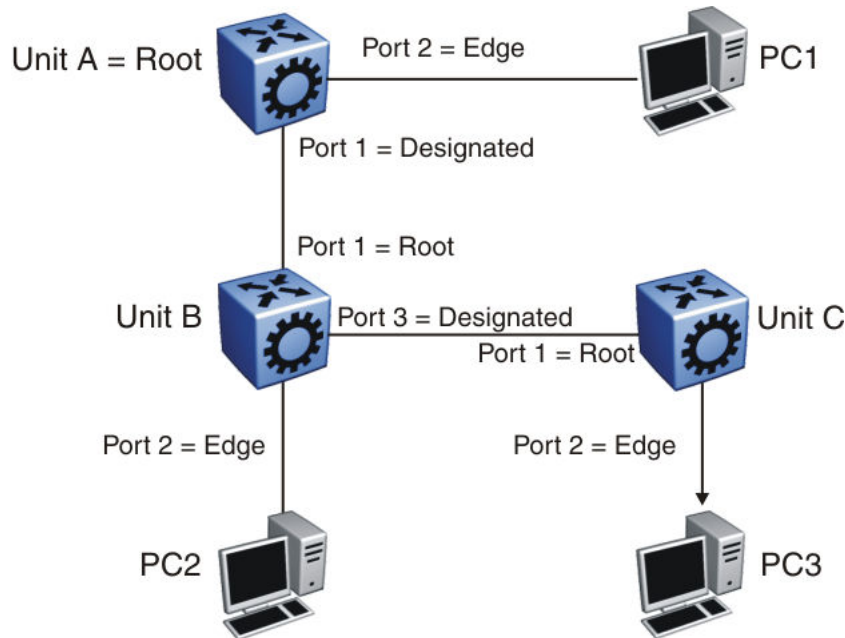
Figure 234: RSTP negotiation process
