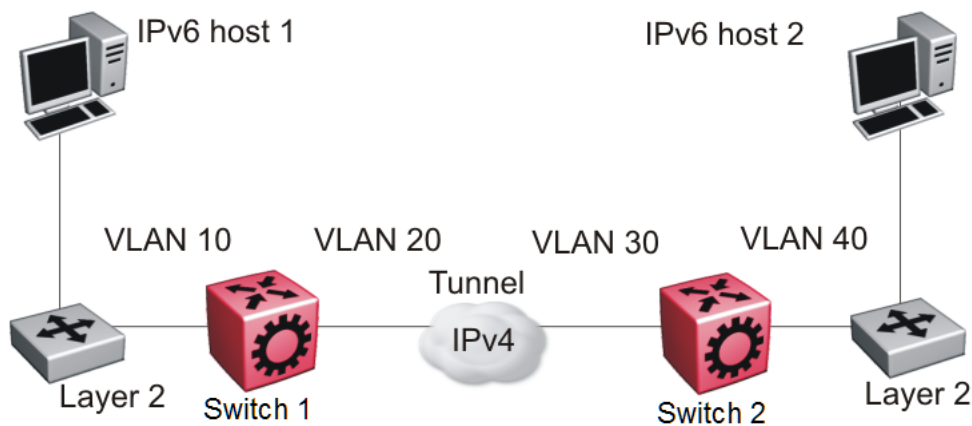
Figure 171: Tunnel configuration between VLANs
