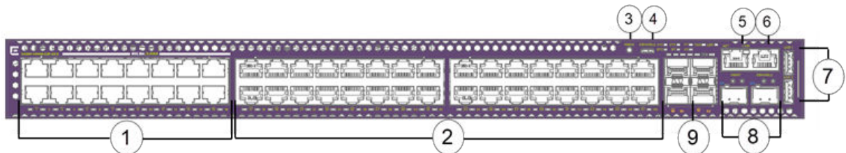
Figure 277: 5420F-16MW-32P-4XE Front Panel
