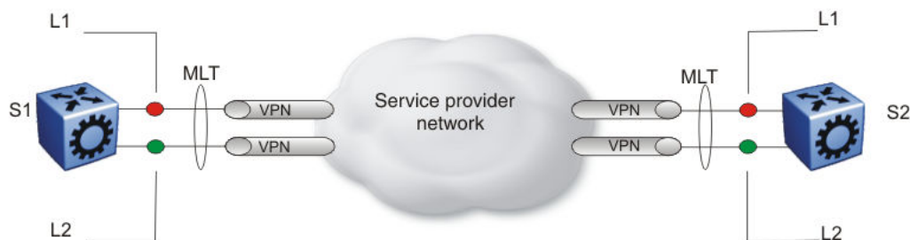
Figure 252: Problem description (1 of 2)
