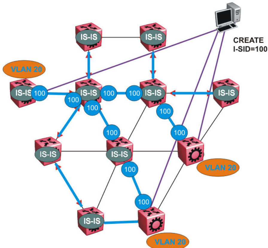
Figure 93: SPBM BMAC and I-SID population
