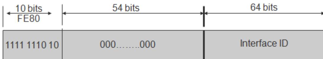
Figure 167: Unicast Link-local address
