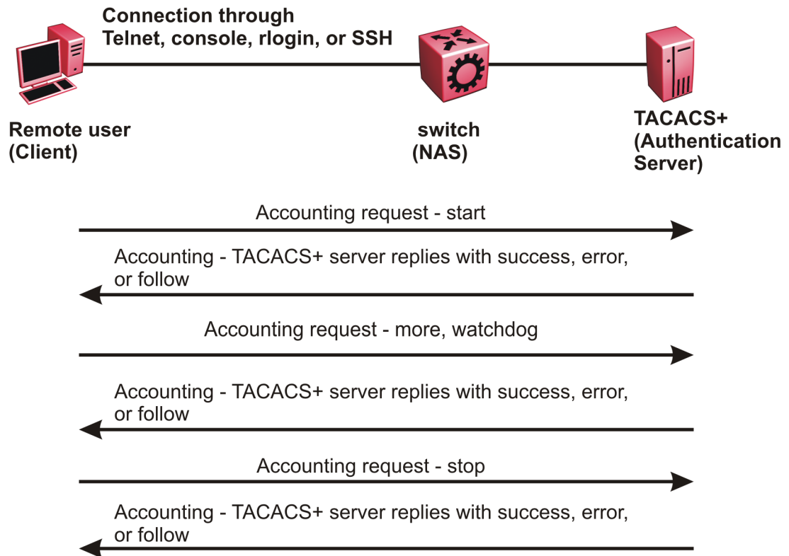
Figure 247: Accounting process
