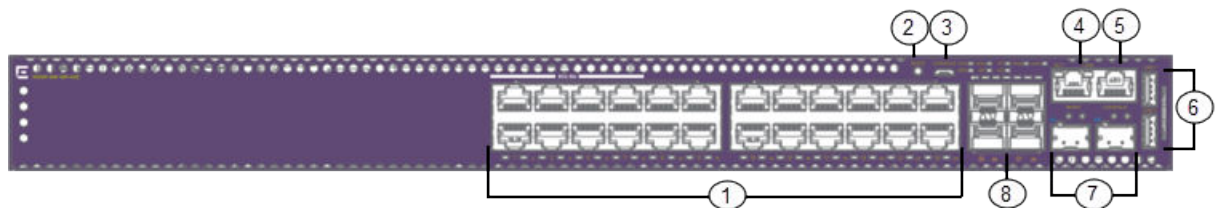
Figure 273: 5420F-8W-16P-4XE Front Panel
