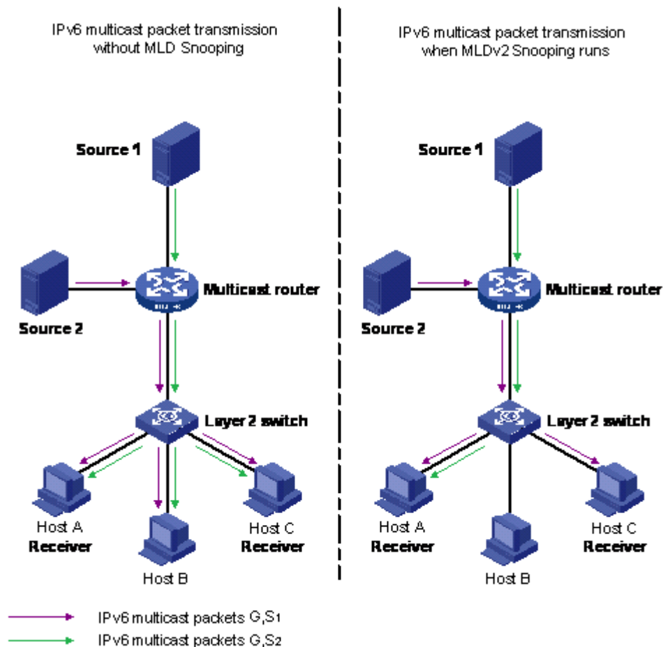
Figure 146: IPv6 multicast packet transmission when MLD v2 snooping is enabled and not enabled
