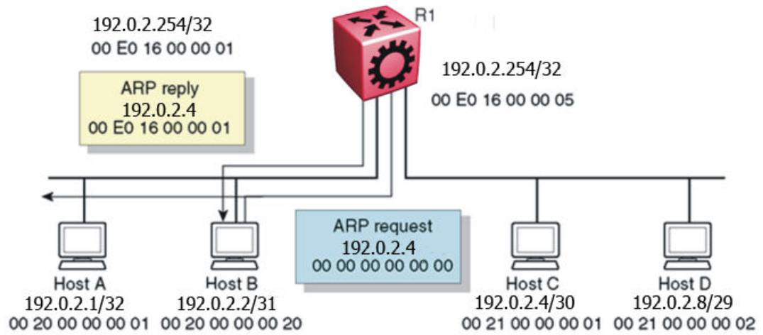
Figure 7: Proxy ARP operation
