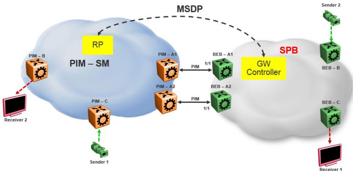
Figure 239: SPB-PIM Gateway base case configuration
