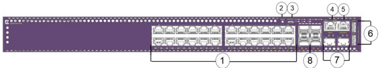
Figure 276: 5420F-24T-4XE Front Panel
