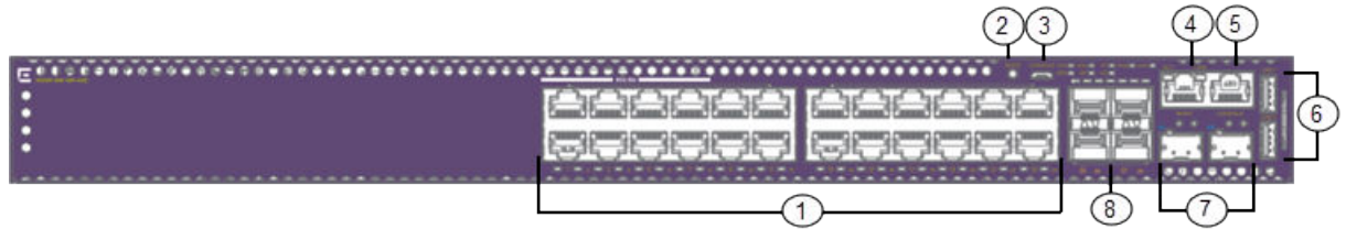
Figure 275: 5420F-24S-4XE Front Panel
