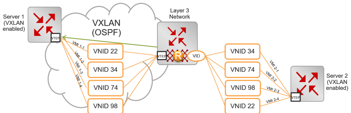
Figure 270: VXLAN-to-VXLAN deployment
