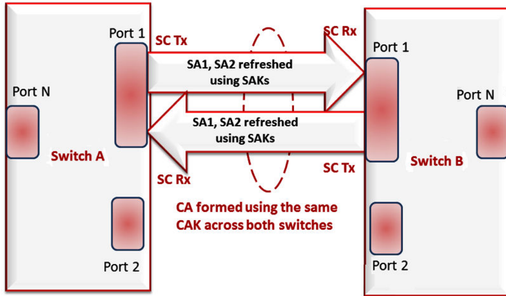
Figure 185: MACsec relationship
