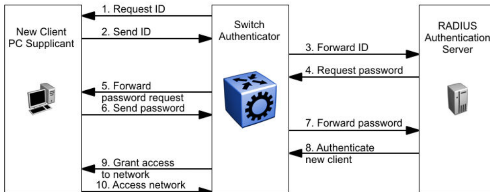
Figure 44: EAP configuration example
