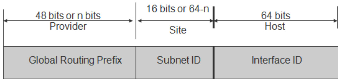
Figure 166: Unicast global address parts
