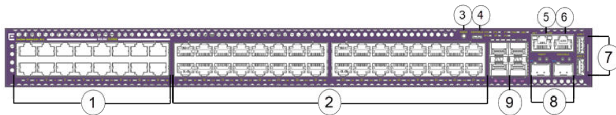
Figure 284: 5420M-16MW-32P-4YE Front Panel
