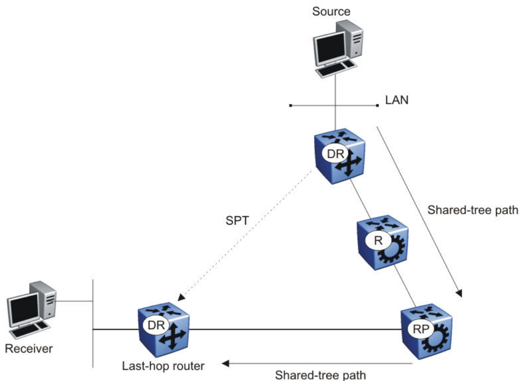
Figure 133: Shared tree and shortest-path tree
