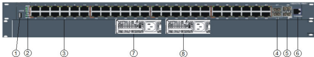
Figure 295: VSP 4450GTX-HT-PWR+
