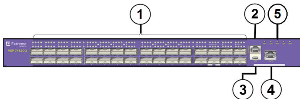
Figure 297: VSP 7432CQ
