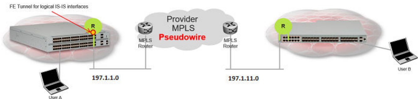
Figure 83: FE over Pseudowire traffic flow
