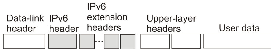
Figure 164: IPv6 header with extension headers
