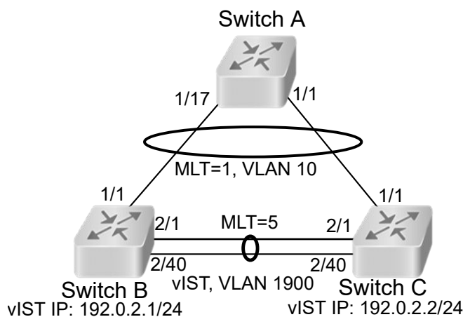
Figure 189: Network topology for traffic flow example
