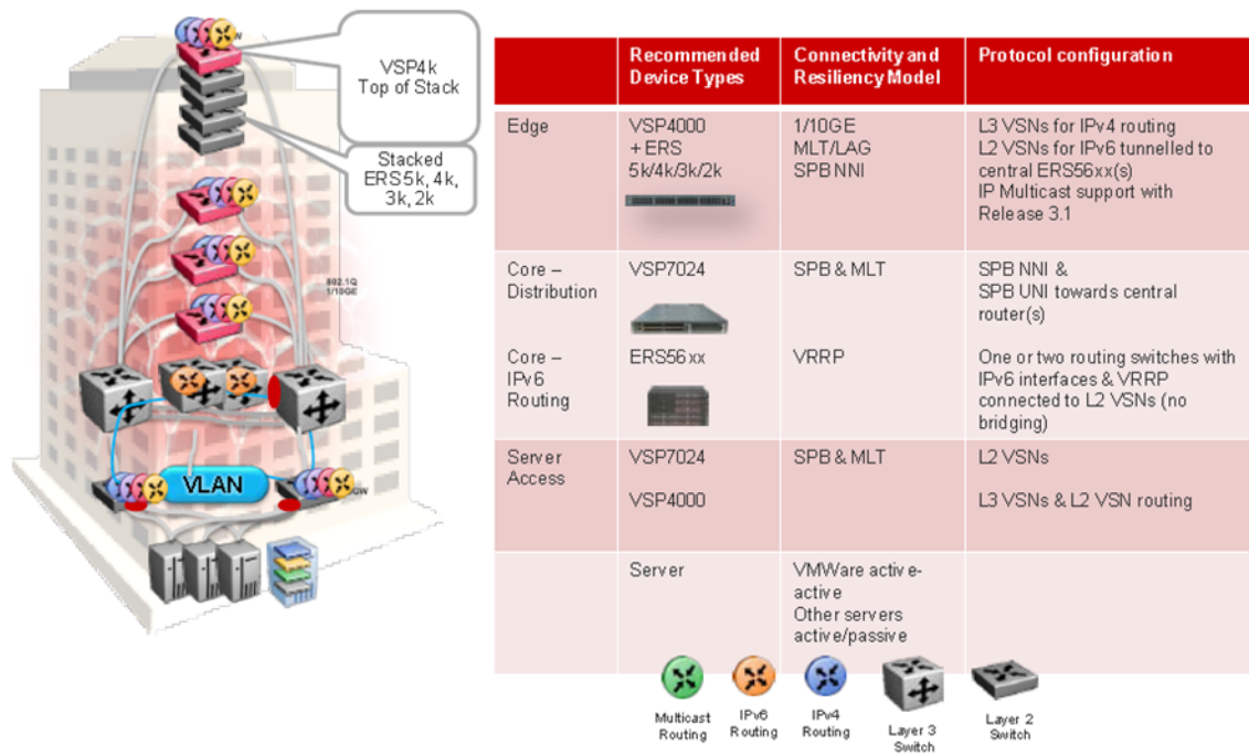
Figure 111: Small core – multi-tenant
