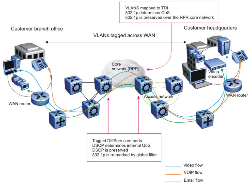
Figure 212: RPR QoS internetworking
