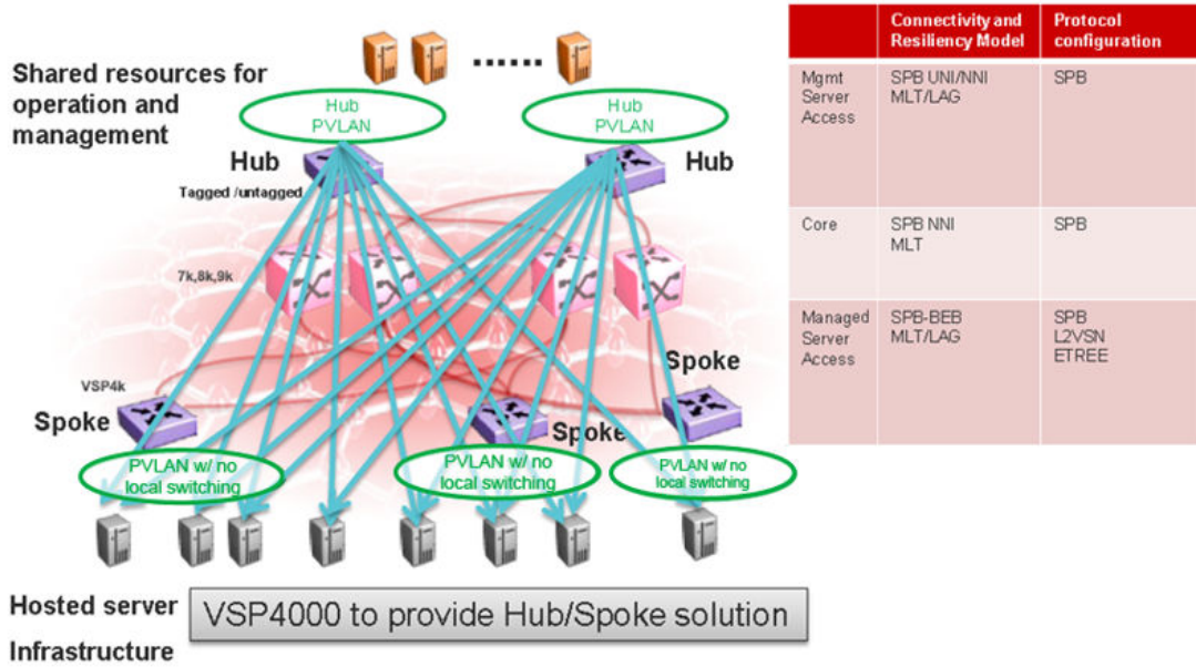
Figure 112: Data center hosting private VLAN
