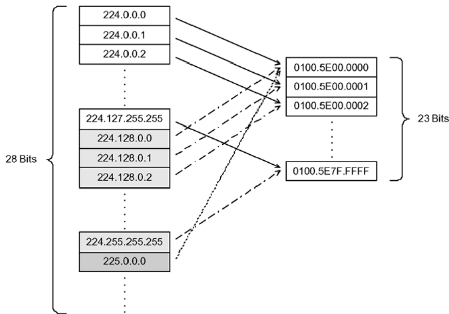
Figure 137: Multicast IP address to MAC address mapping
