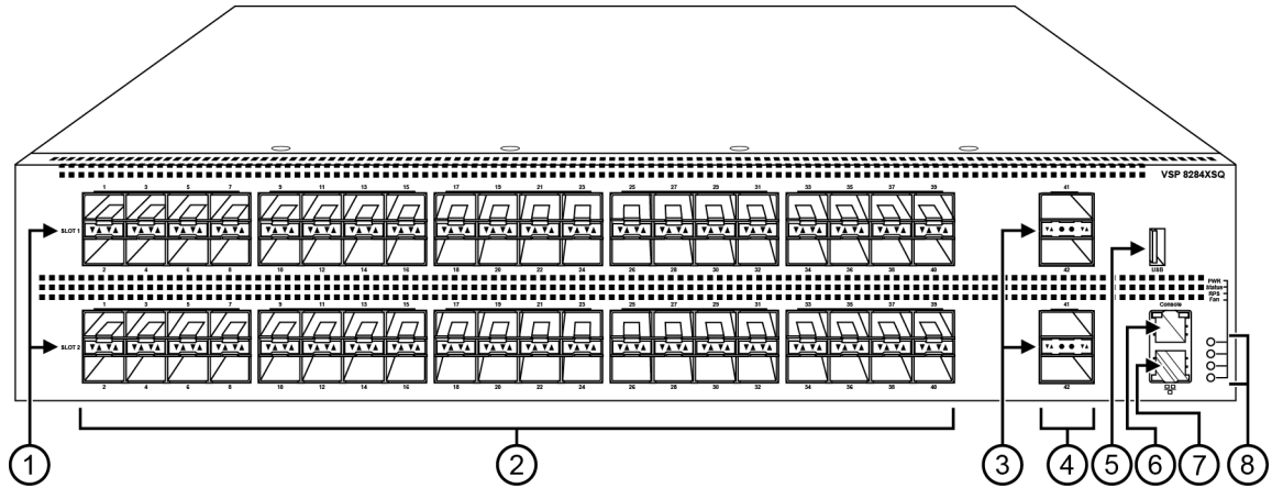
Figure 299: VSP 8284XSQ front view
