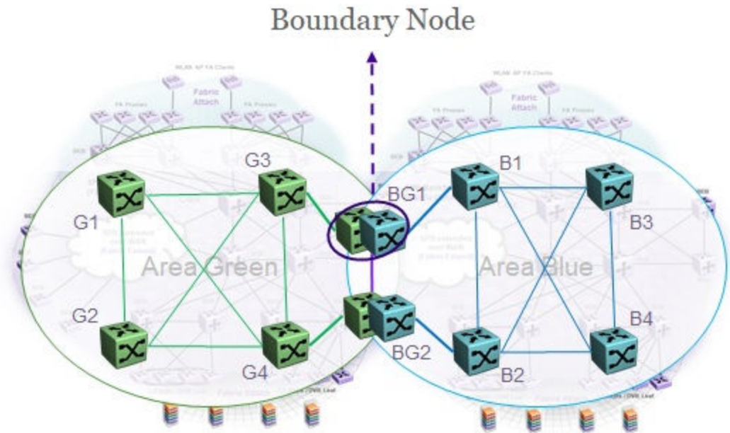
Figure 73: Boundary nodes in the Multi-area SPB network
