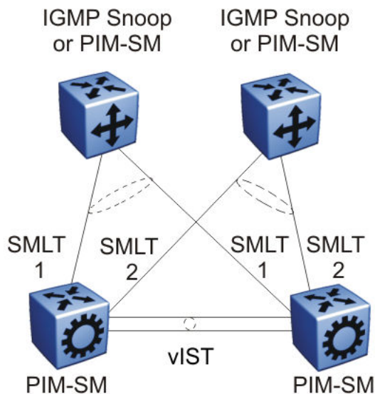
Figure 139: Multicast routing using PIM-SM
