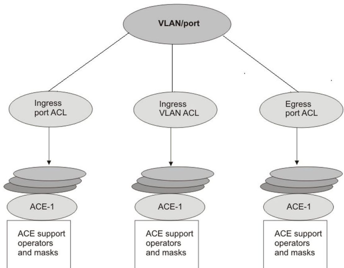
Figure 250: ACE and ACL relationships
