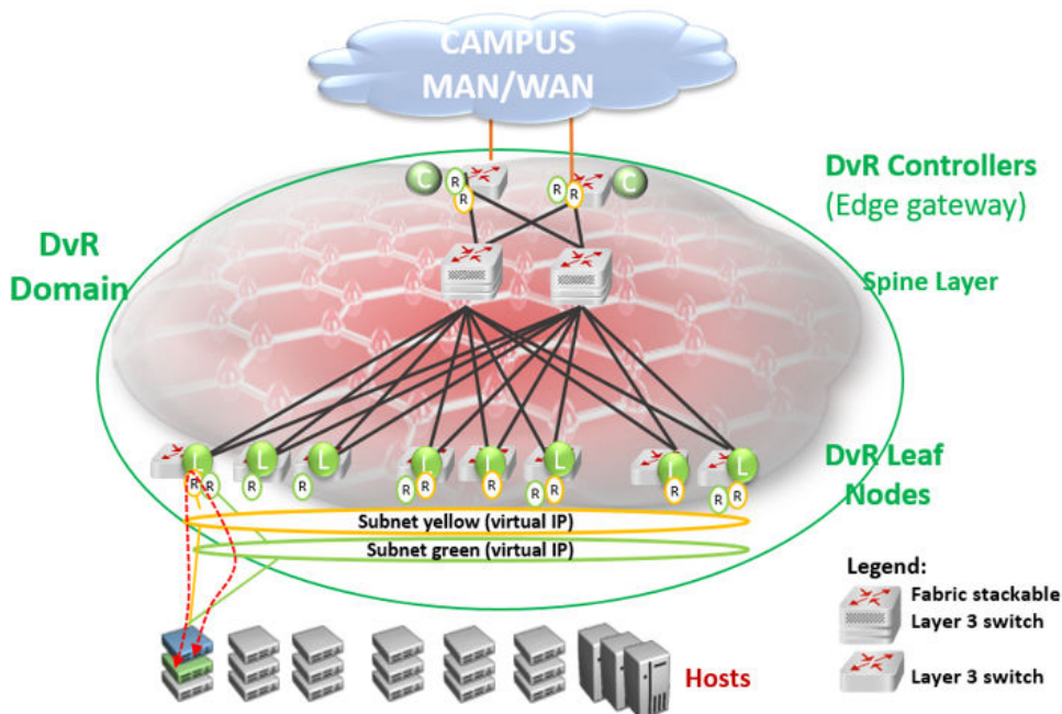
Figure 38: SPB Fabric network with central Layer 3 Controller and distributed Layer 3 datapath at the edges
