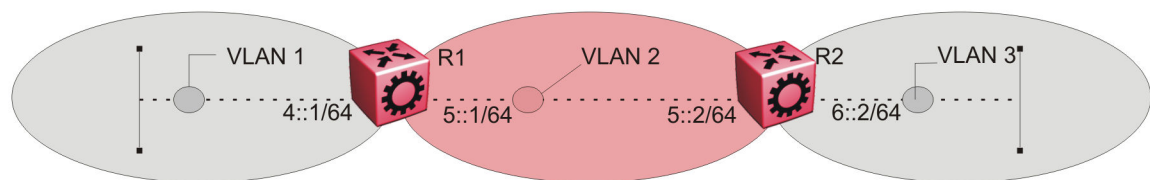
Figure 169: IPv6 routing between VLANs
