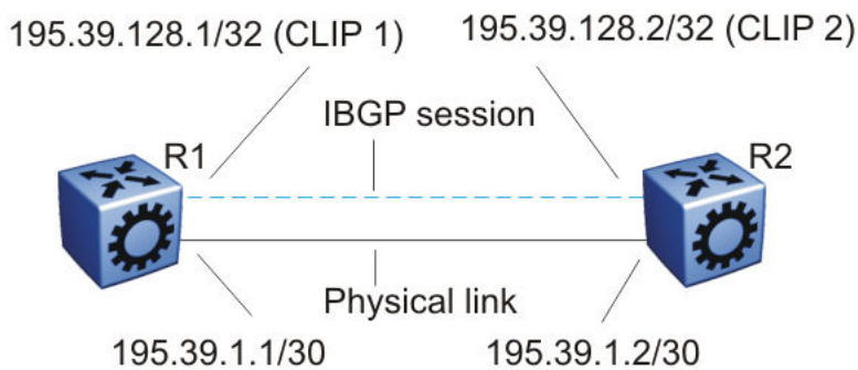
Figure 24: Routers with iBGP connections
