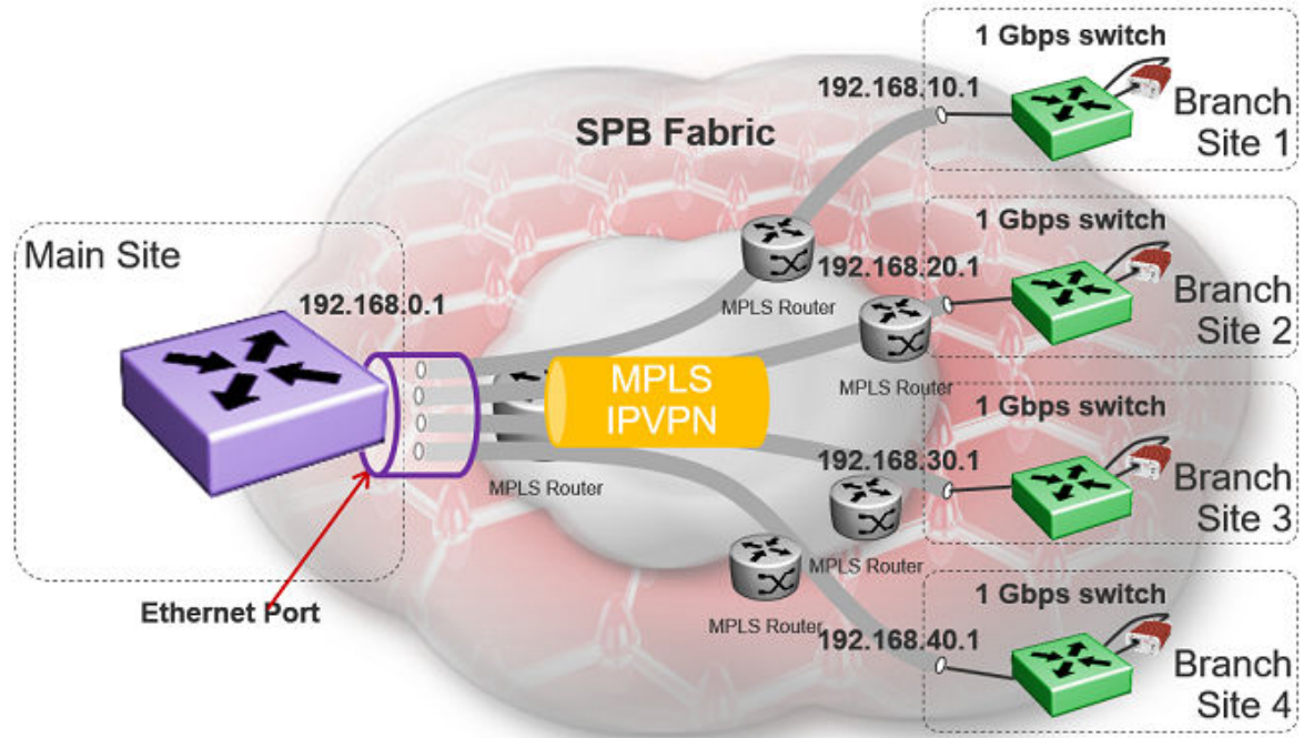
Figure 55: Fabric Extend IP VPN Deployment Option
