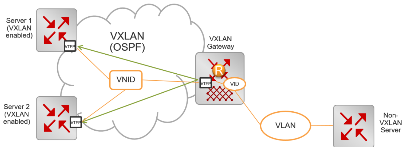
Figure 269: VXLAN-to-VLAN deployment
