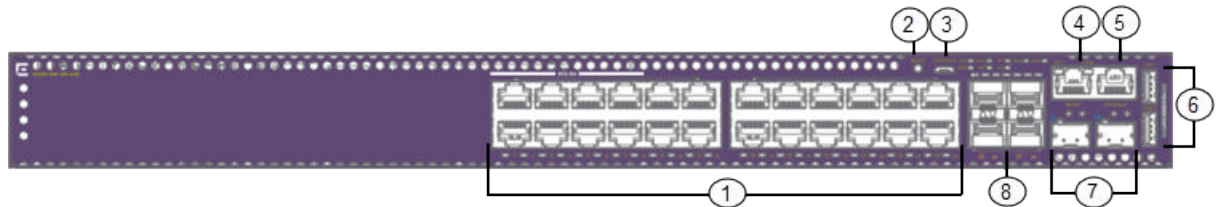
Figure 274: 5420F-24P-4XE Front Panel
