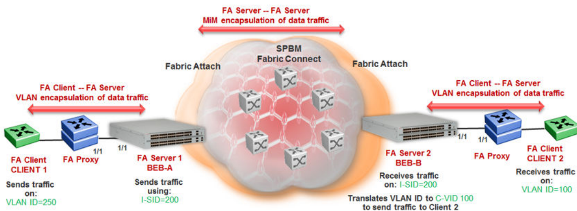
Figure 65: Data encapsulation – VLAN encapsulation and MiM encapsulation
