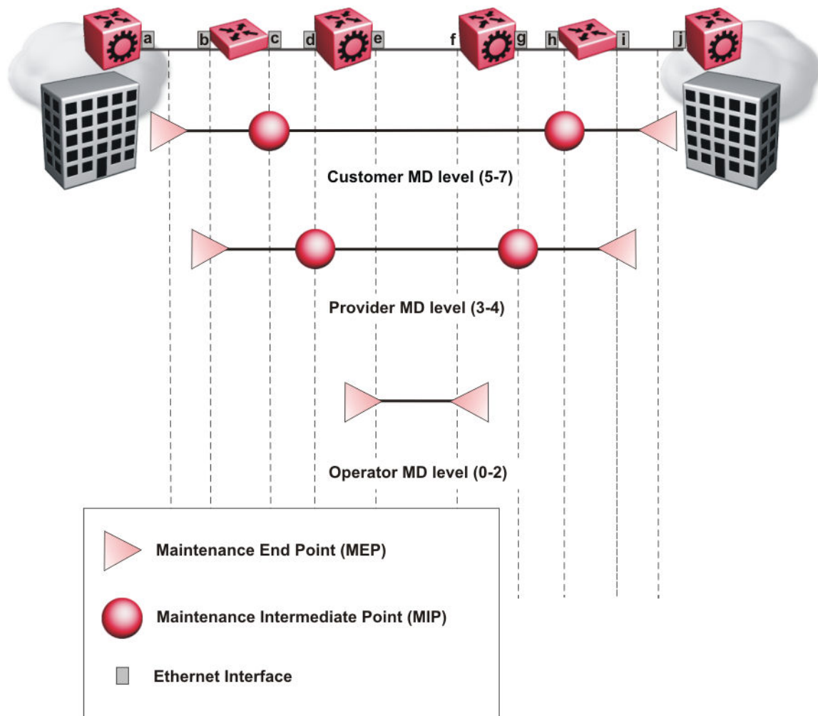
Figure 251: MD level assignment
