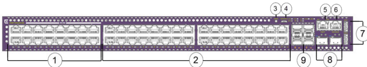
Figure 278: 5420F-16W-32P-4XE Front Panel
