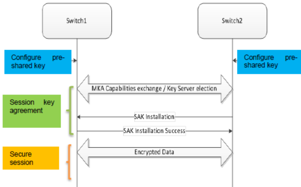
Figure 186: Switch to switch MACsec deployment scenario
