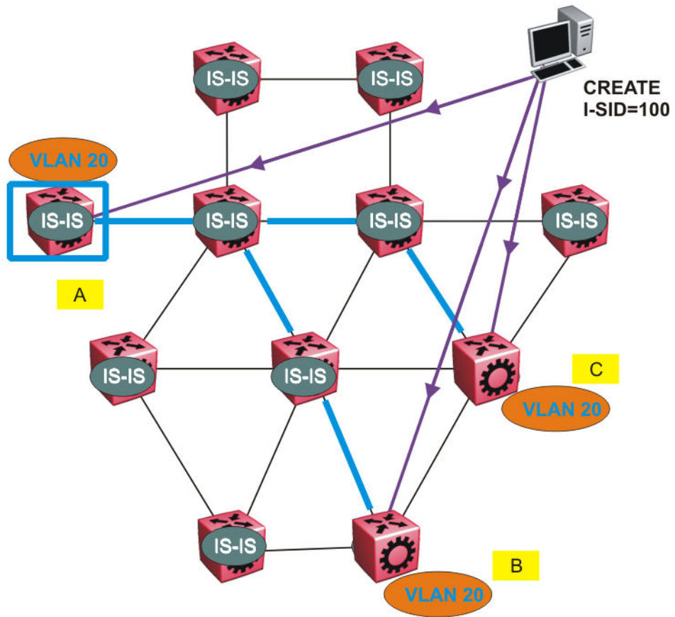
Figure 94: Shortest path tree for source node A
