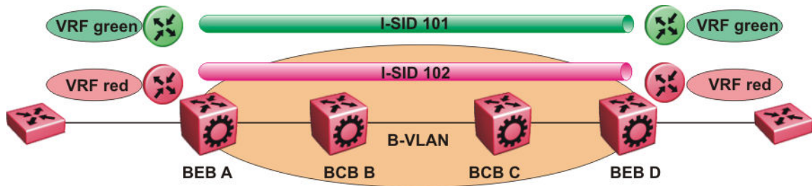
Figure 123: SPBM Layer 3 VSN
