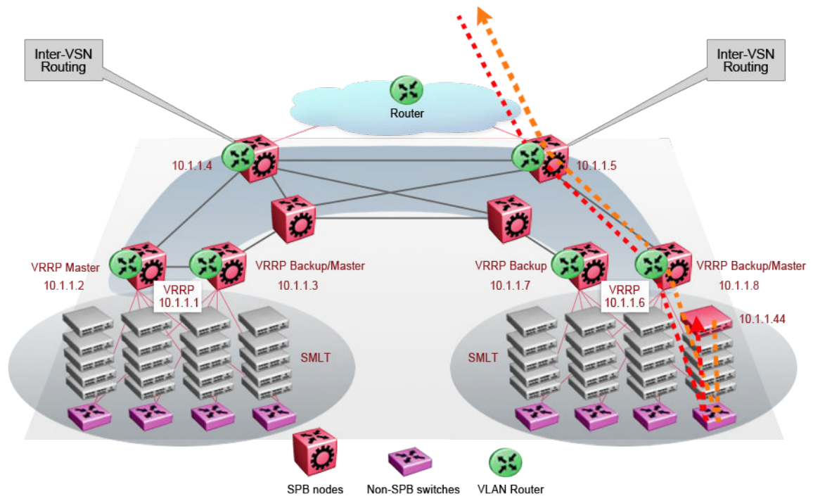
Figure 110: Optimized routing after moving VMs
