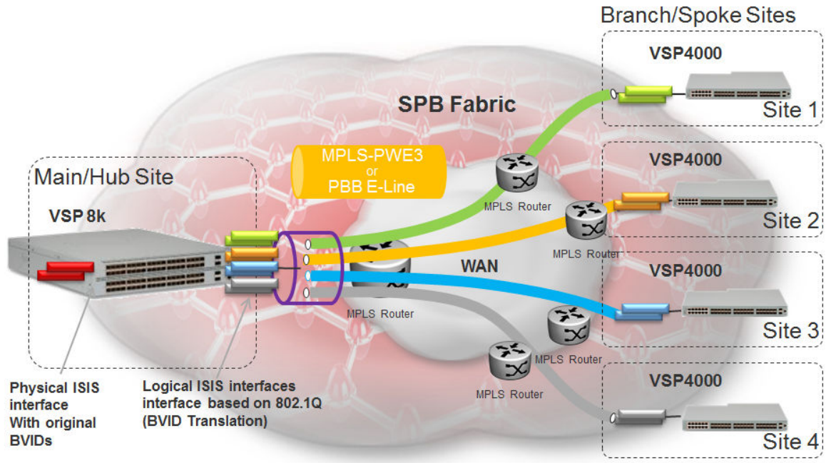
Figure 58: Fabric Extend Pseudowire Deployment Option
