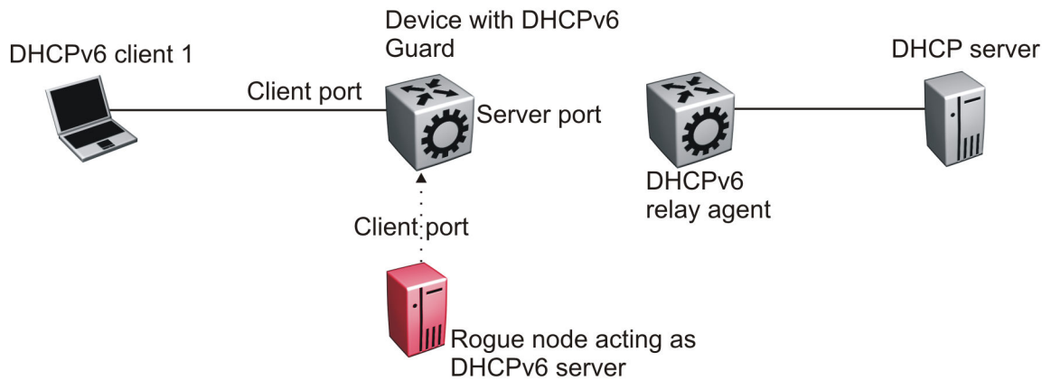
Figure 173: DHCPv6 Topology 1
