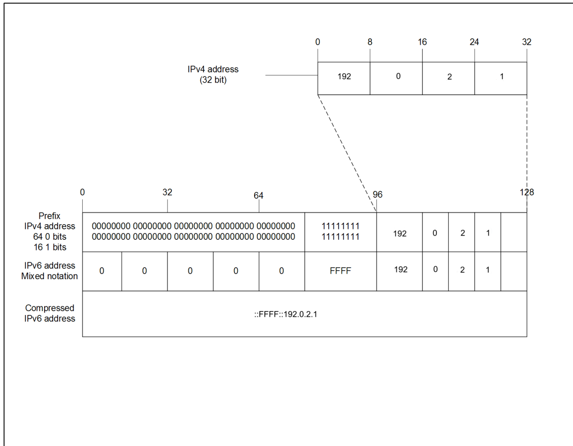
Figure 31: IPv4-mapped IPv6 address components
