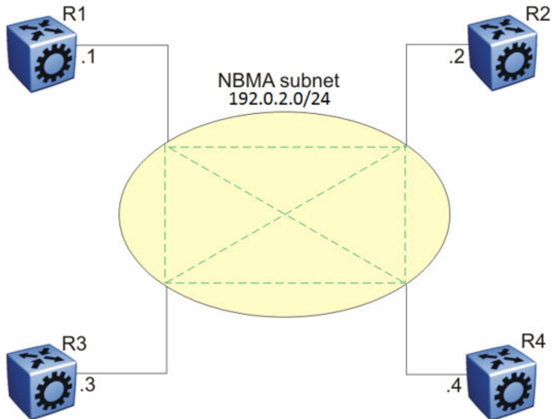
Figure 201: NBMA Subnet
