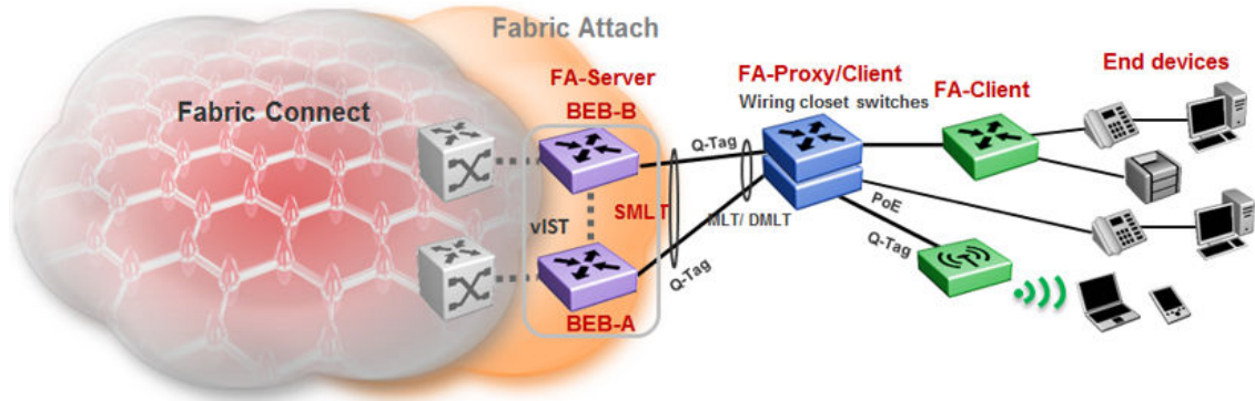
Figure 67: FA in a dual-homed SMLT deployment
