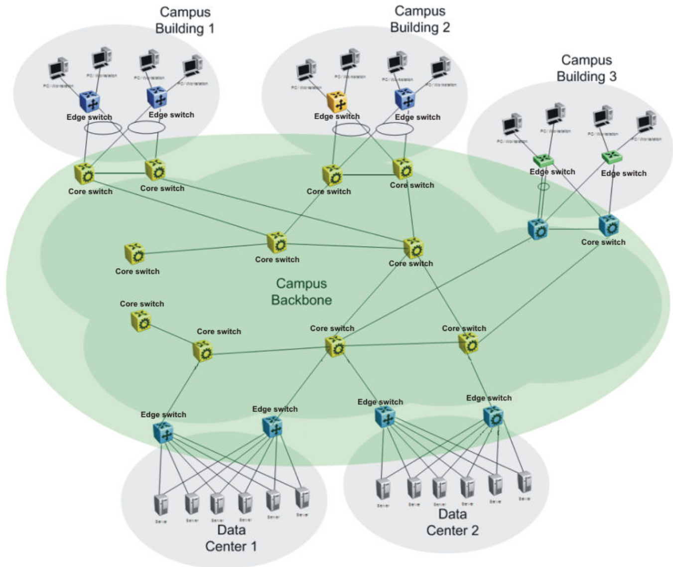
Figure 90: SPBM L2 VSN in a campus
