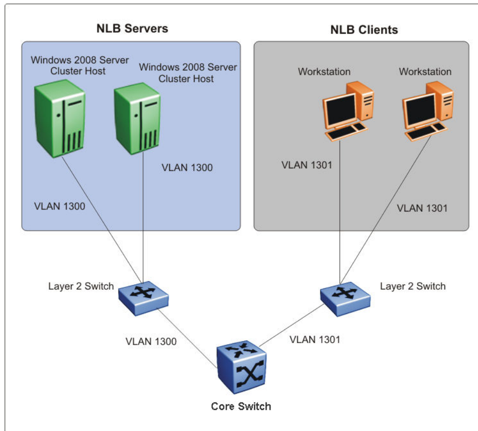
Figure 258: Supported NLB topology-example 1
