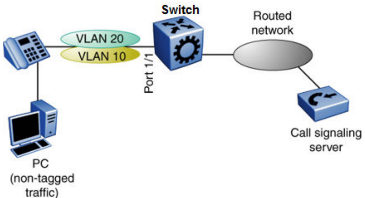
Figure 257: Network with IP phone and PC
