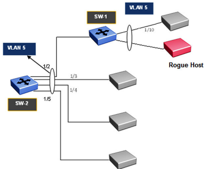
Figure 172: First Hop Security topology
