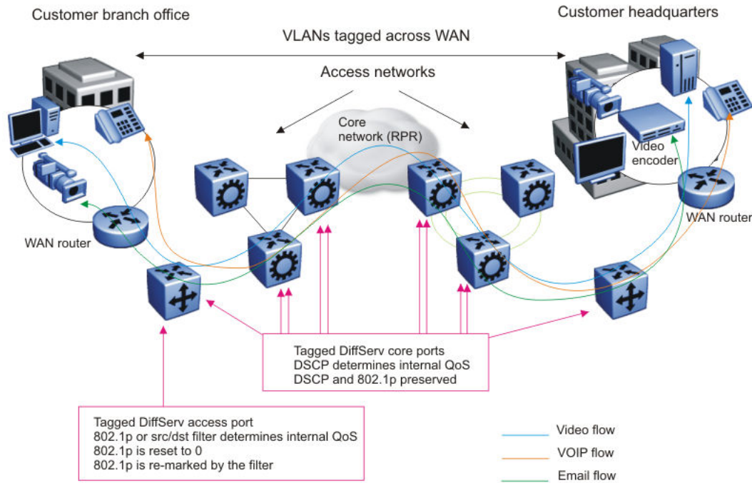
Figure 213: Trusted routed traffic
