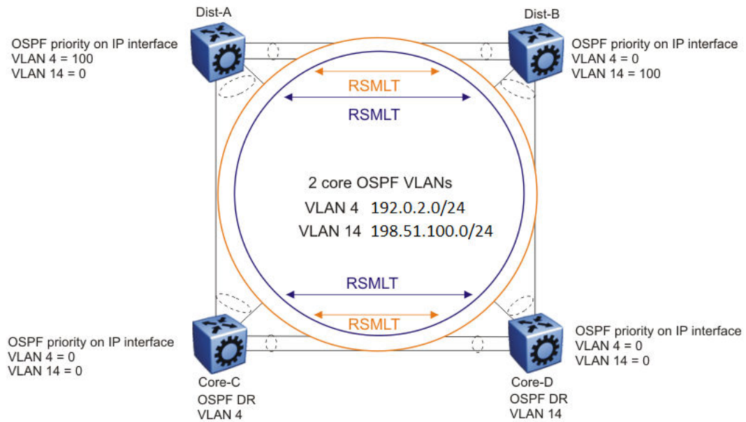
Figure 204: RSMLT with dual core VLANs
