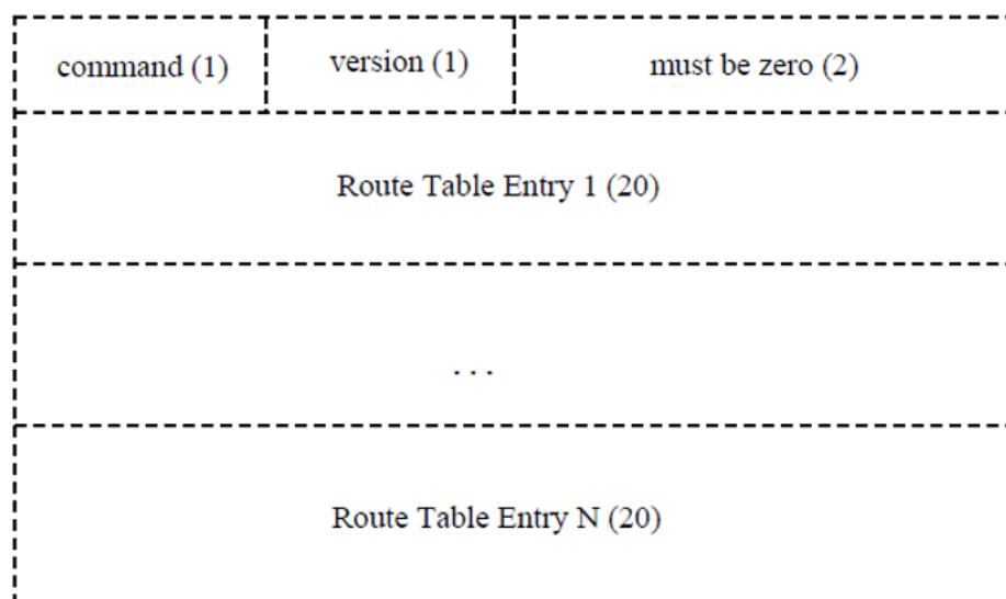
Figure 217: RIPng packet format
