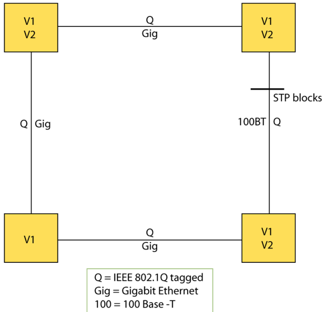
Figure 260: VLAN isolation
