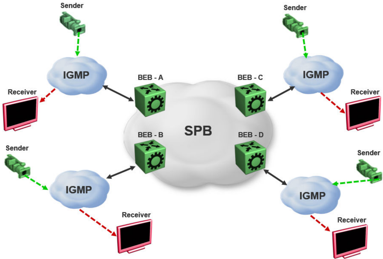
Figure 235: IP Multicast over Fabric Connect streams
