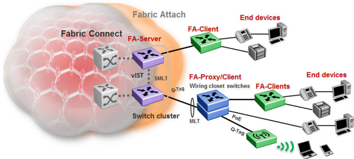
Figure 68: Fabric Attach in a single-homed SMLT deployment
