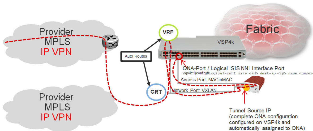
Figure 60: Autorouting between GRT and VRF
