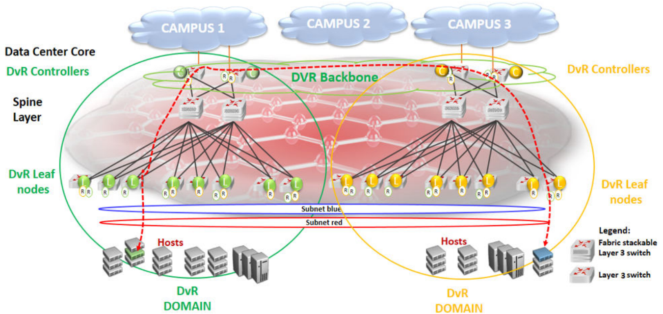
Figure 39: Shortest path routing between servers in different data centers
