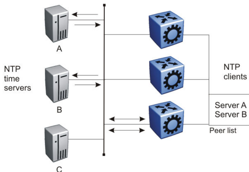
Figure 197: NTP Time Servers Operating in Unicast Client Mode
