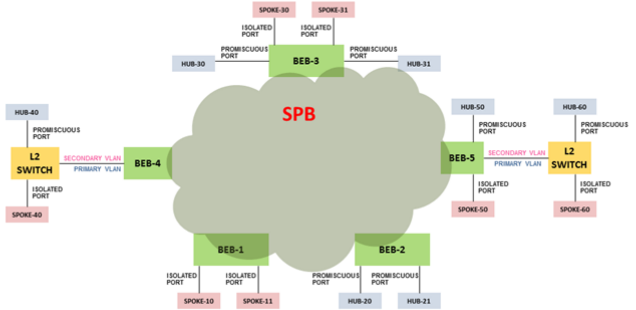
Figure 50: Sample E-Tree configuration
