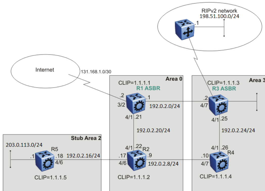
Figure 200: Multiarea configuration example
