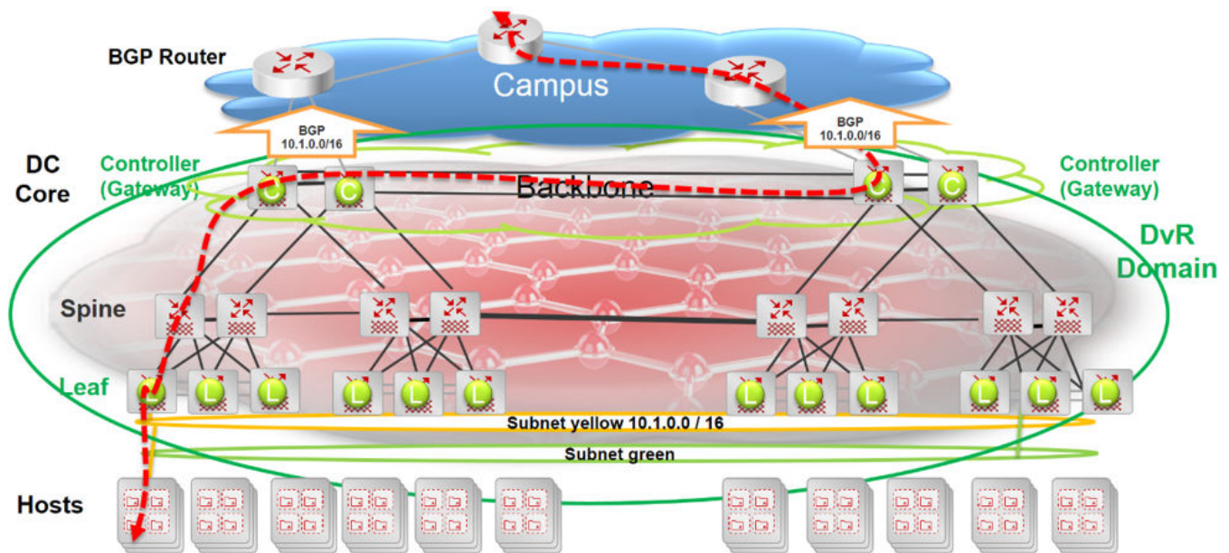
Figure 41: Inefficient traffic flow
