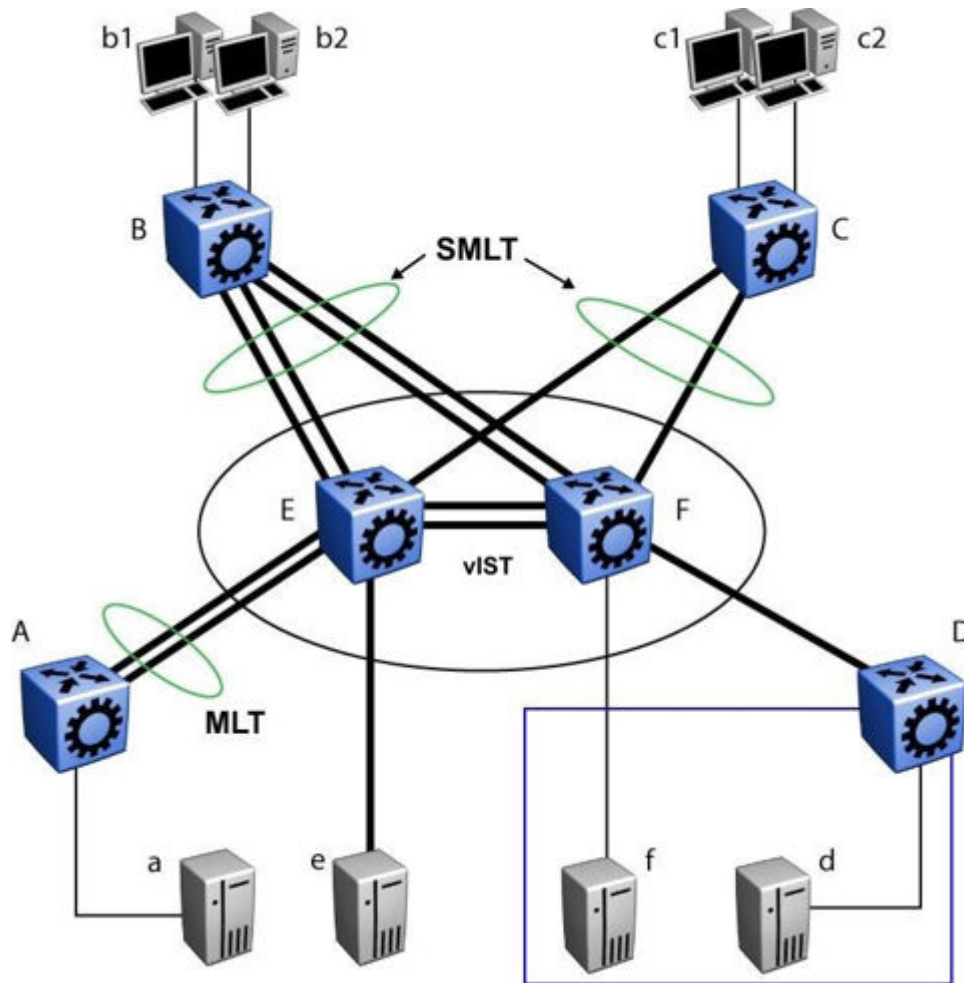
Figure 188: SMLT aggregation switches and operations
