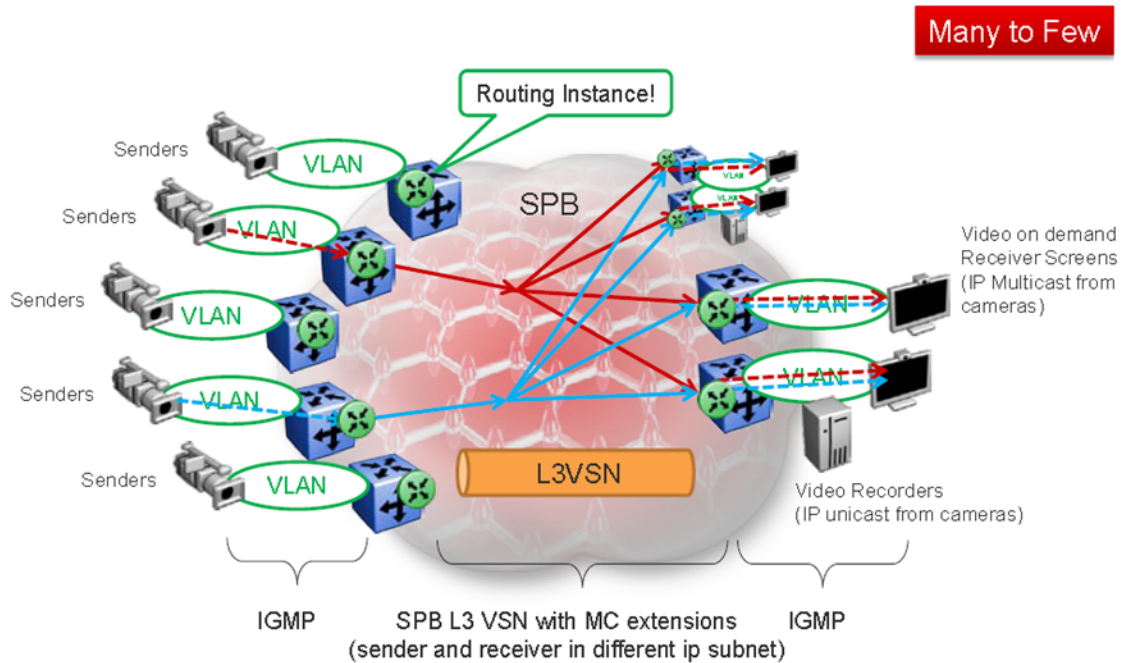
Figure 114: Deployment scenario — Routed video surveillance and IP camera deployment for transportation, airports, and government
