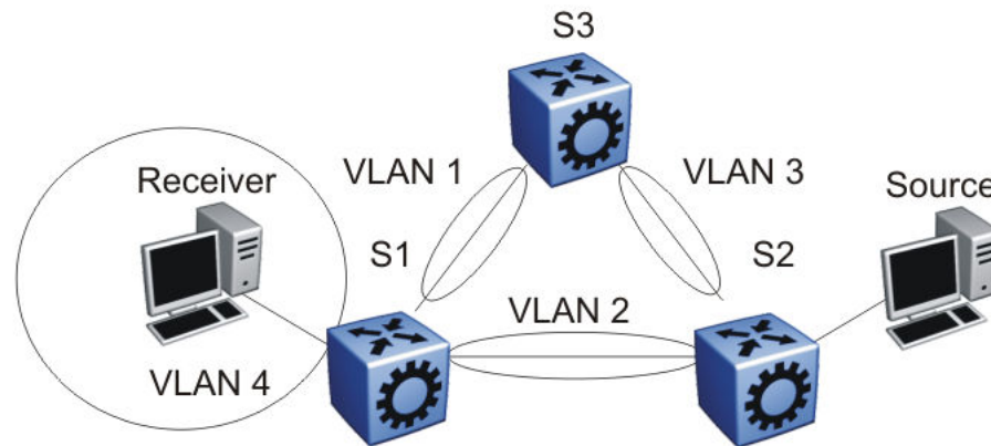
Figure 136: IP multicast sources and receivers on interconnected VLANs
