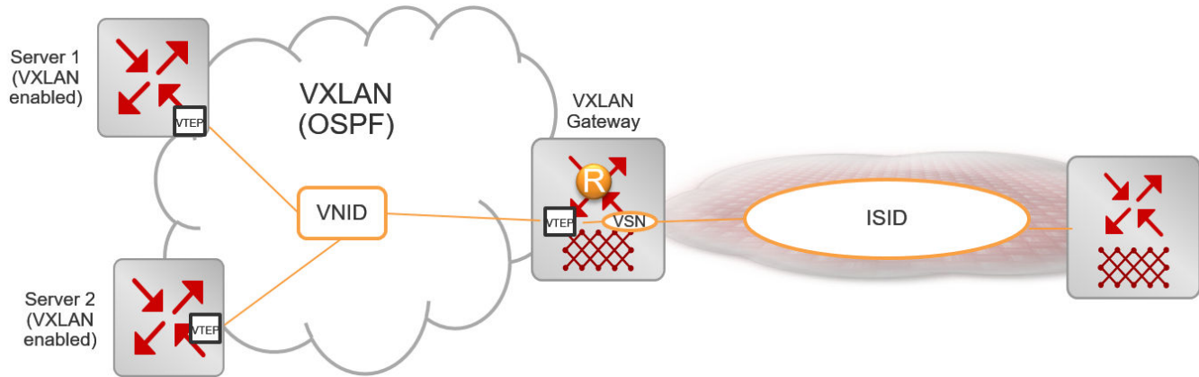
Figure 271: VXLAN-to-SPB deployment
