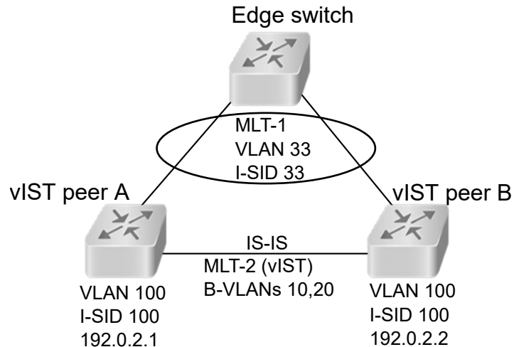
Figure 190: SMLT with vIST configuration example
