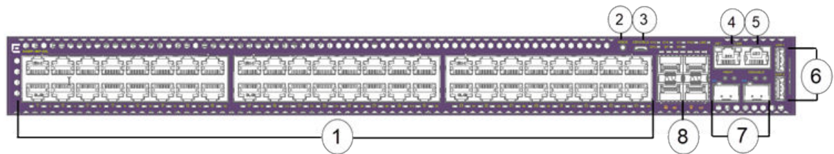
Figure 280: 5420F-48P-4XL Front Panel
