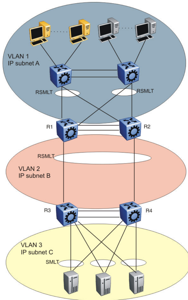
Figure 226: SMLT and RSMLT in Layer 3 environments
