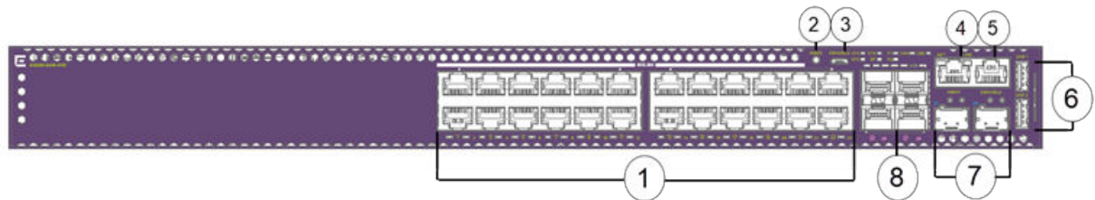
Figure 283: 5420M-24W-4YE Front Panel
