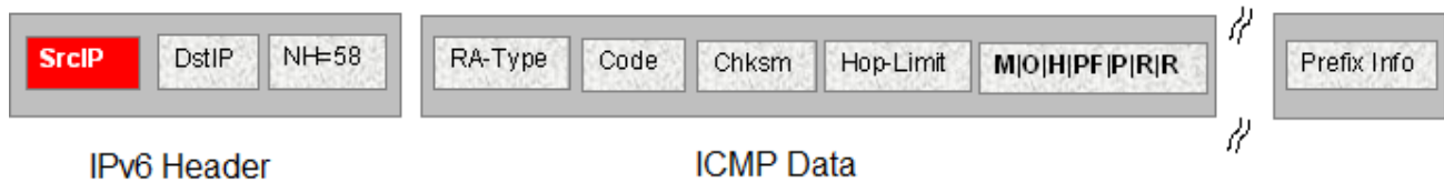
Figure 176: IPv6 ICMP RA Data Packet Online
