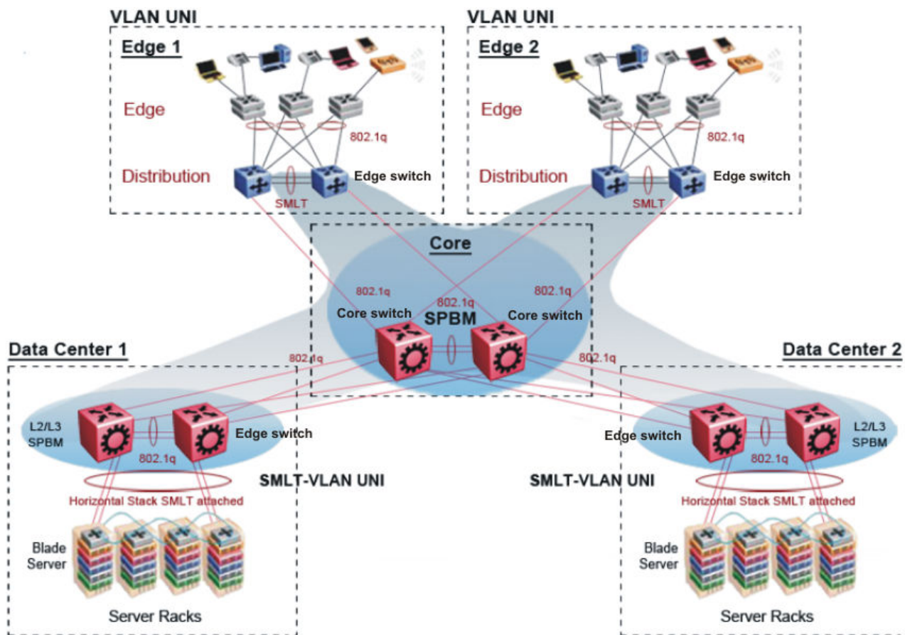
Figure 103: SPBM campus without SMLT
