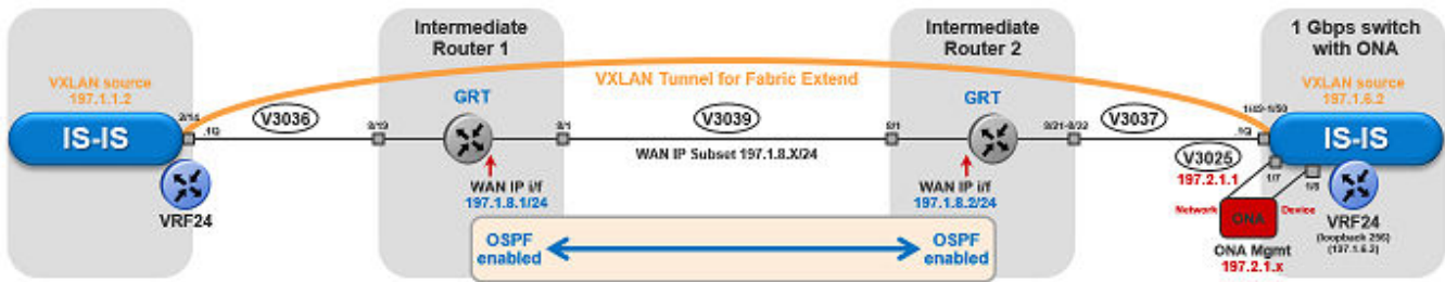
Figure 81: IP (VRF) traffic flow component view
