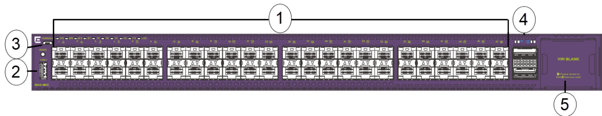
Figure 293: 5520-48SE
