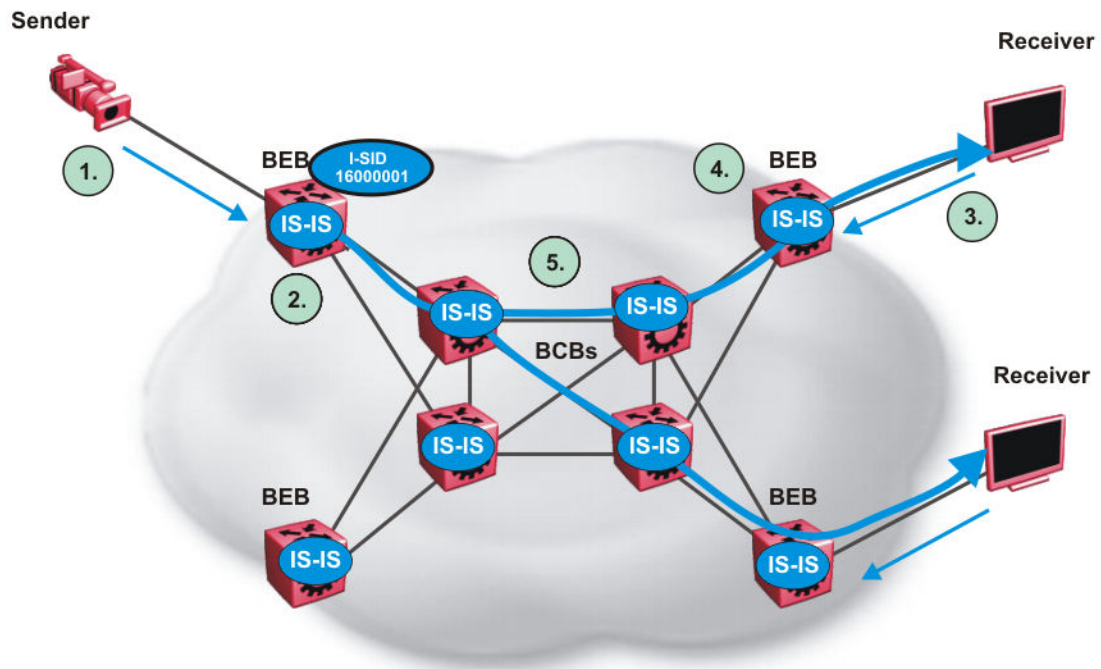
Figure 147: IP Multicast over Fabric Connect streams
