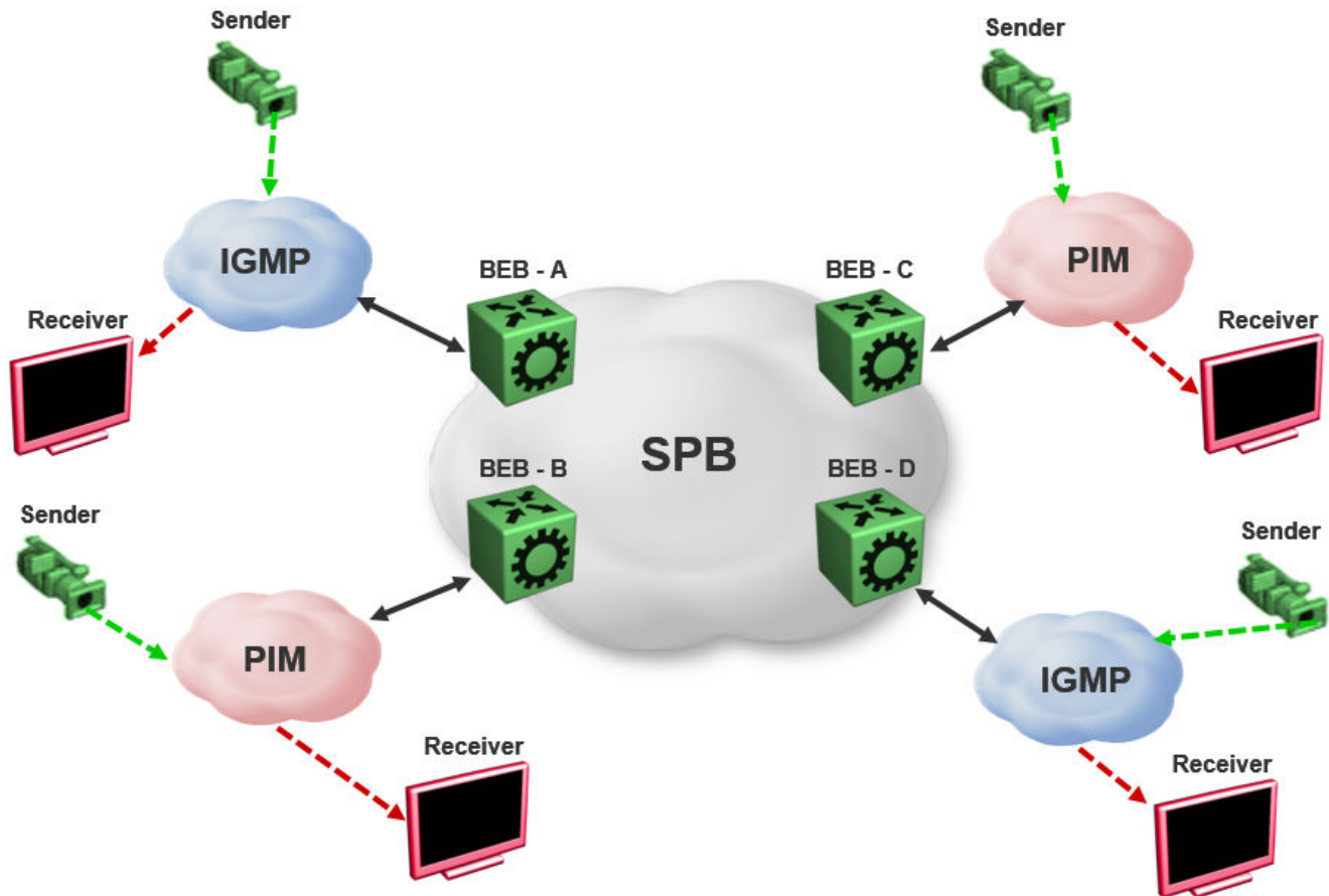
Figure 236: IP Multicast over Fabric Connect Streams
