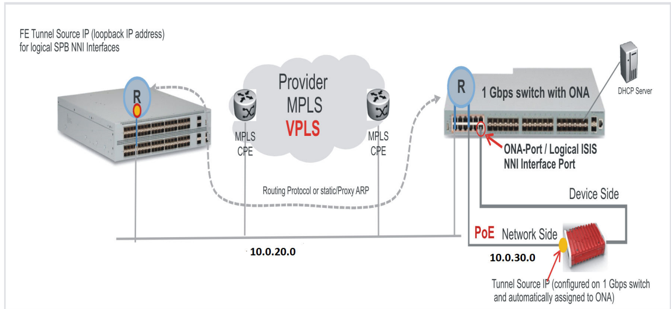
Figure 82: FE over VPLS traffic flow
