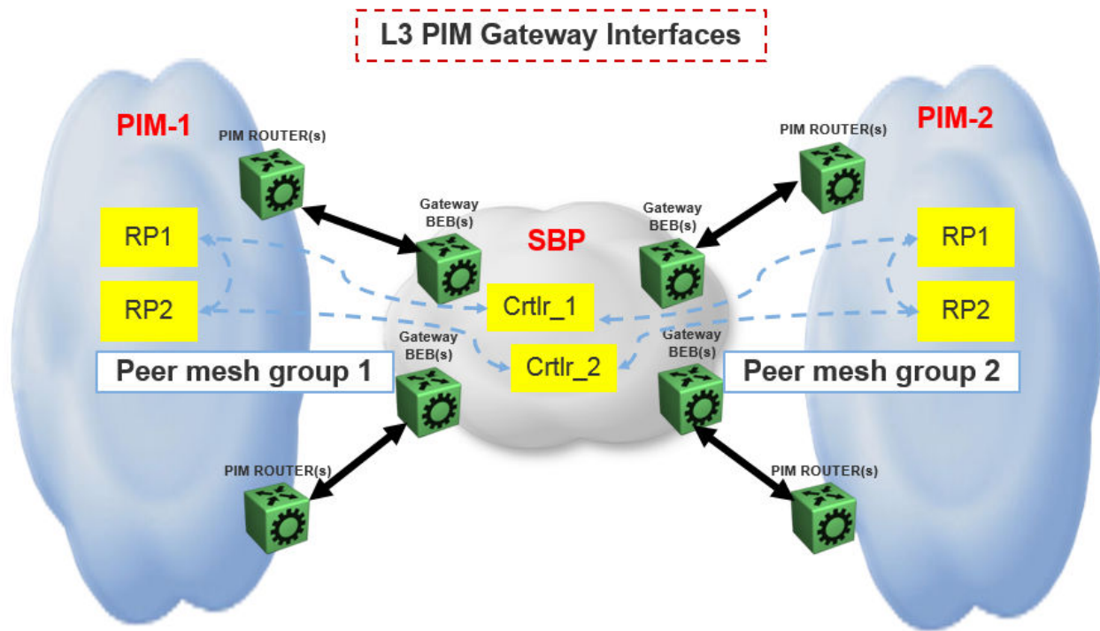
Figure 242: Multi domain configuration
