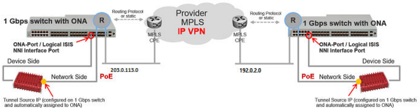
Figure 85: Fabric Extend traffic flow
