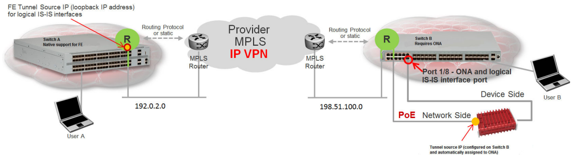
Figure 54: Fabric Extend traffic flow
