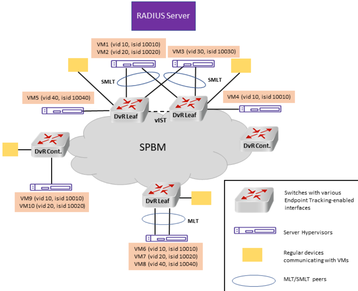
Figure 71: DvR Topology Example
