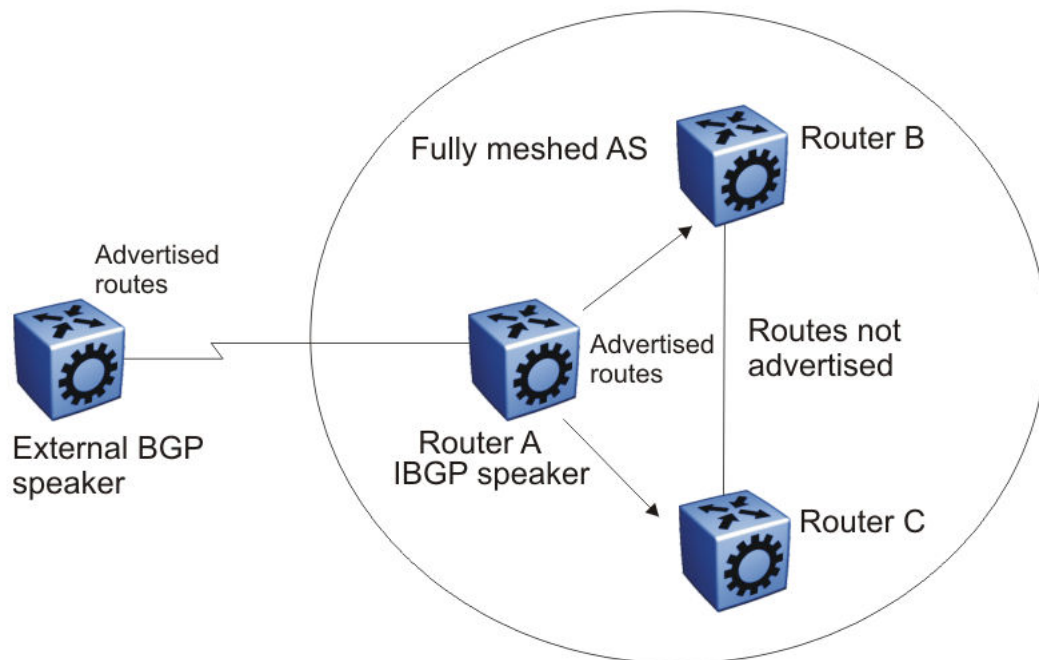
Figure 17: Fully meshed AS with iBGP speakers
