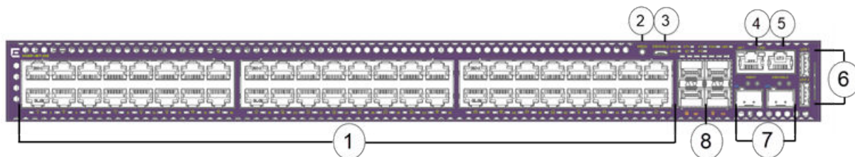
Figure 281: 5420F-48T-4XE Front Panel
