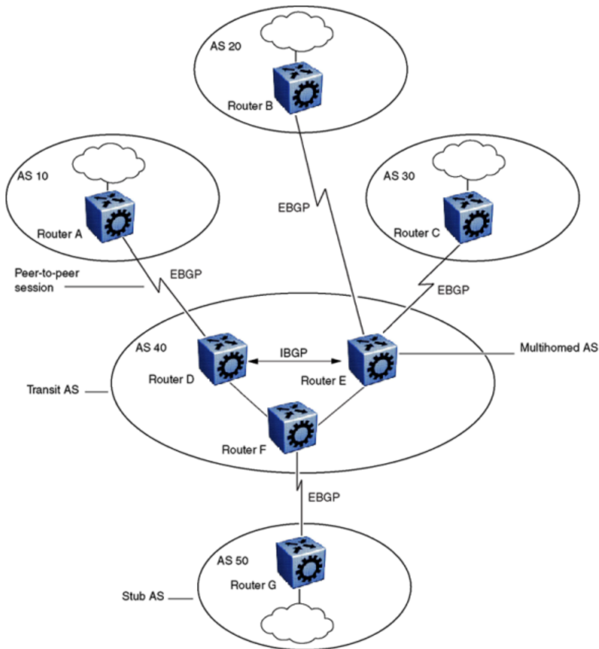
Figure 10: BGP networks
