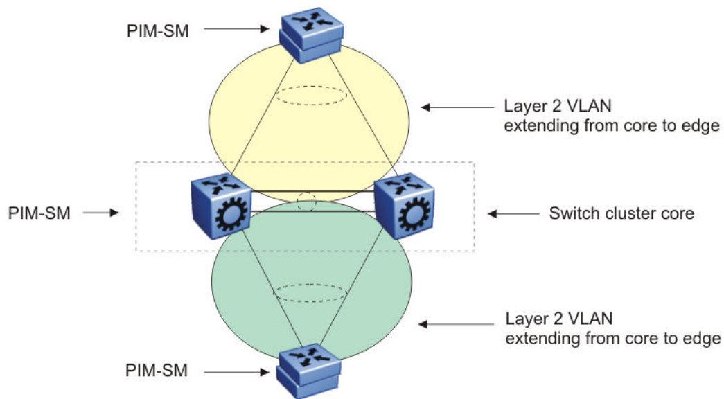
Figure 140: Multicast SMLT triangle
