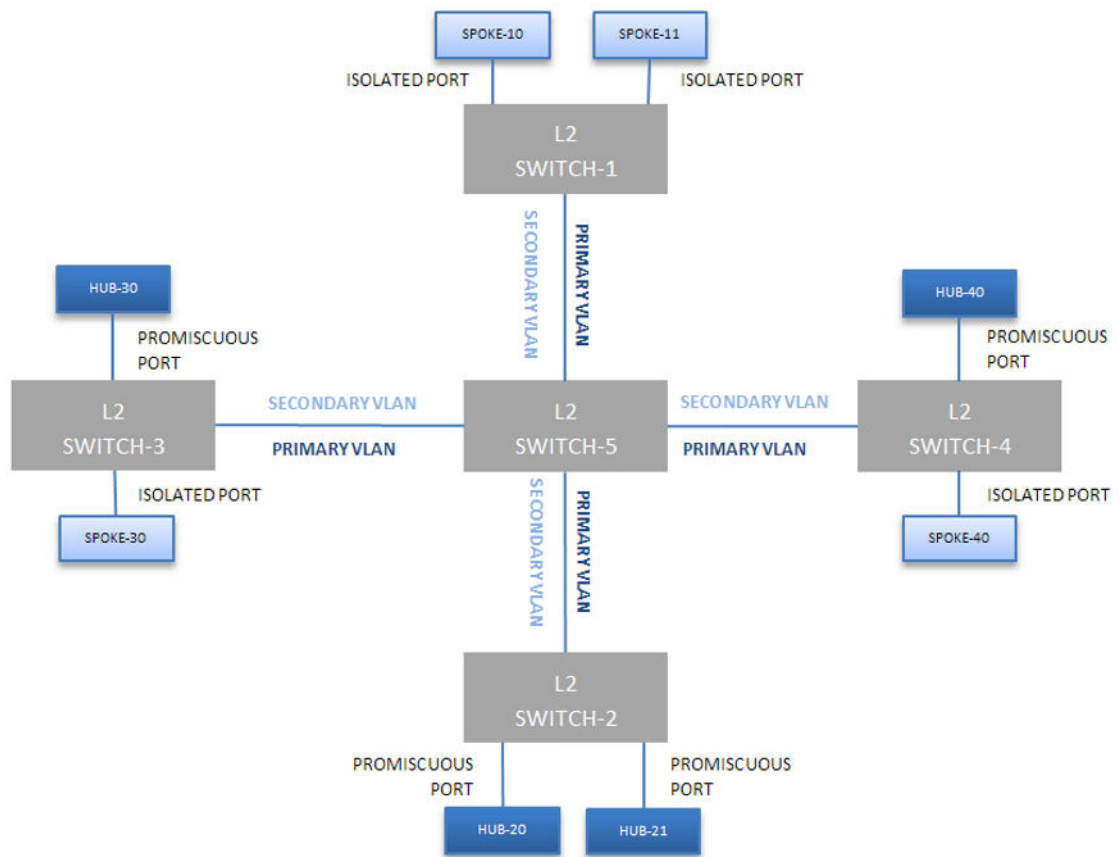
Figure 255: Private VLAN Topology
