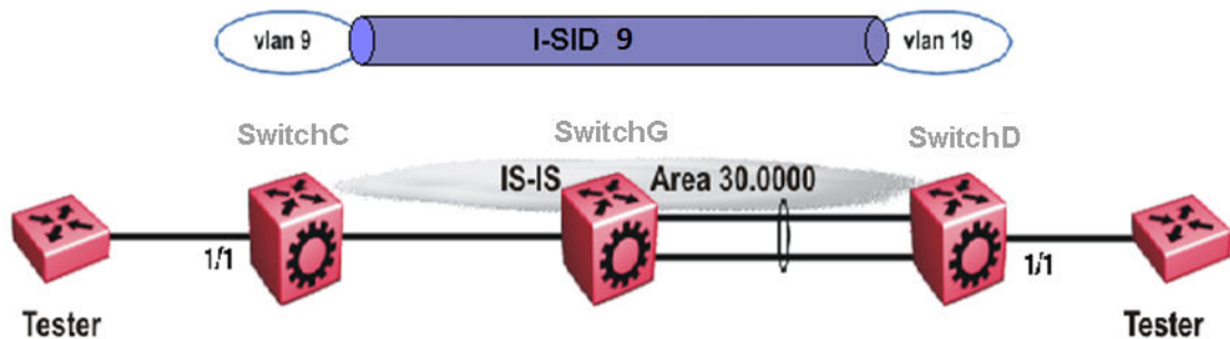
Figure 98: Layer 2 VSN with different VLAN IDs
