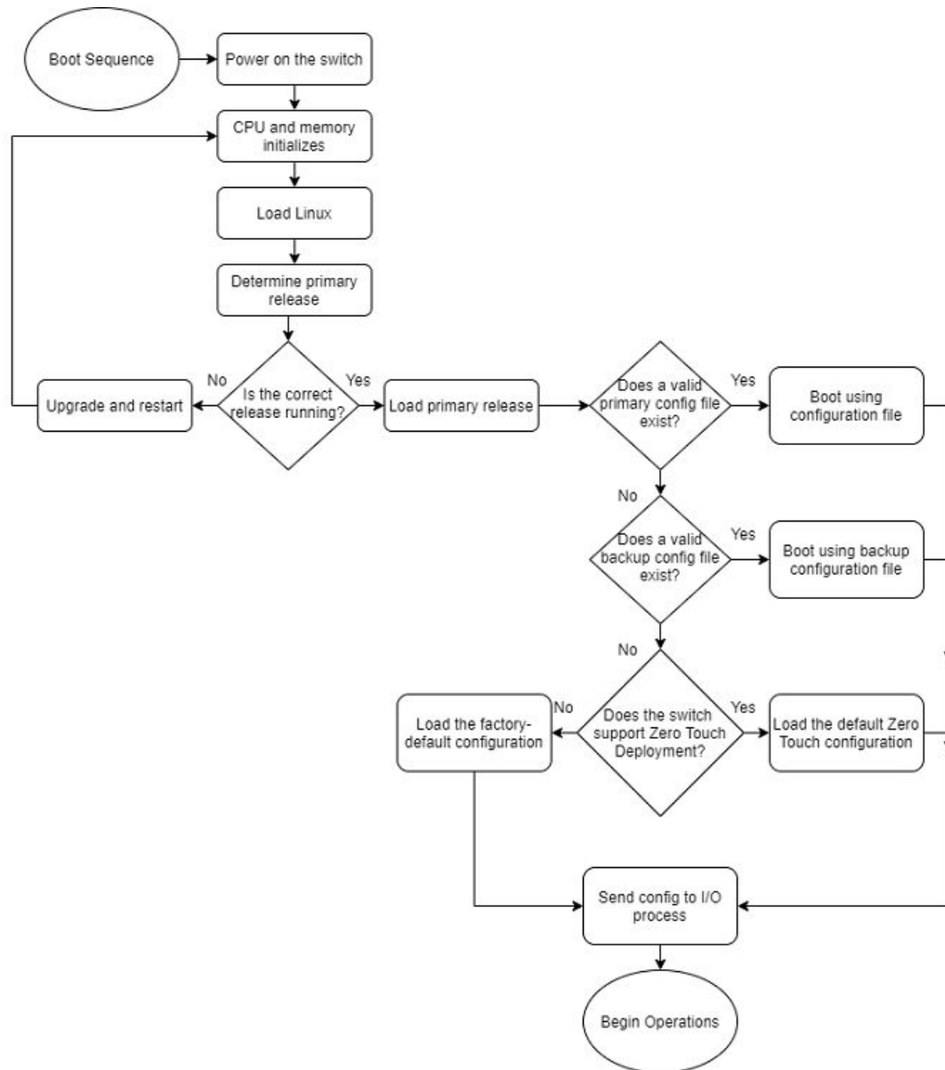
Figure 1: Boot Sequence
