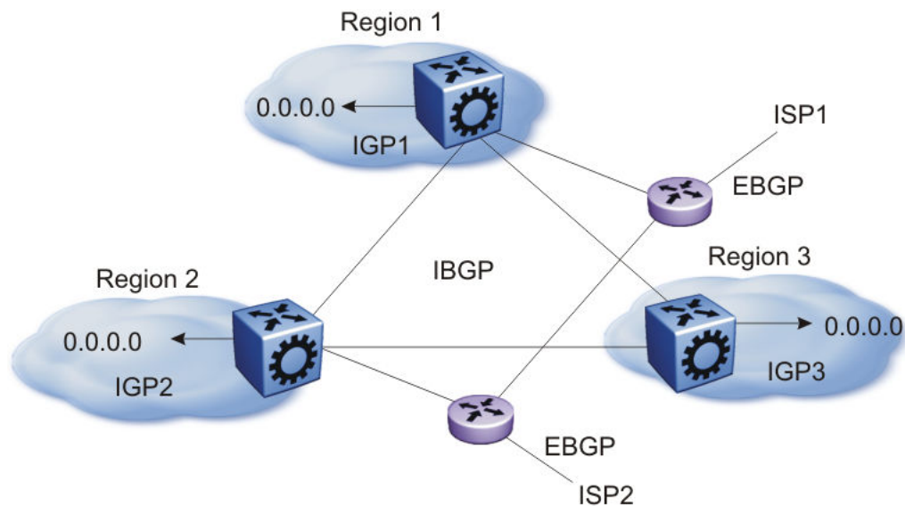
Figure 28: Multiple Regions Separated by iBGP
