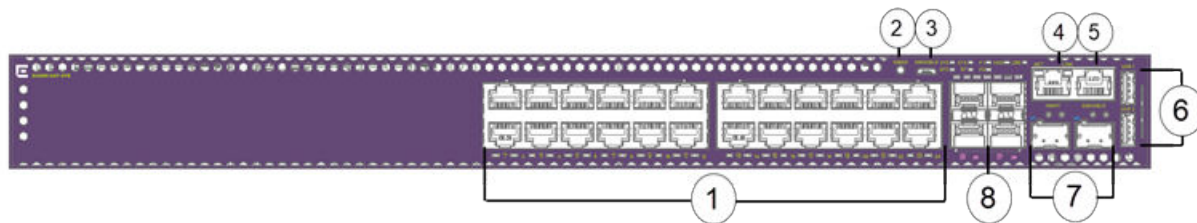
Figure 282: 5420M-24T-4YE Front Panel
