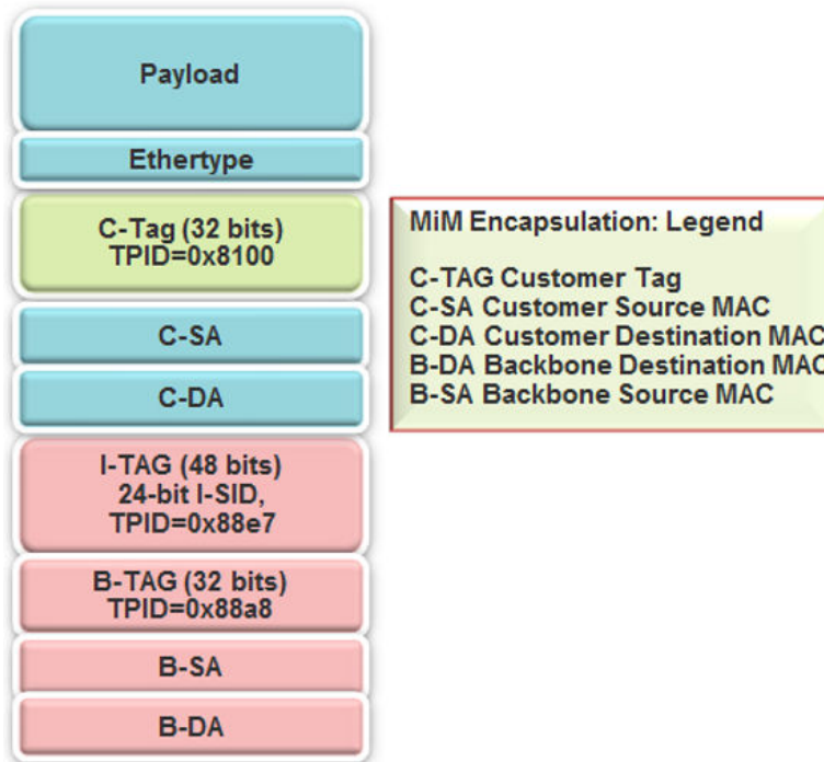
Figure 66: MiM encapsulation
