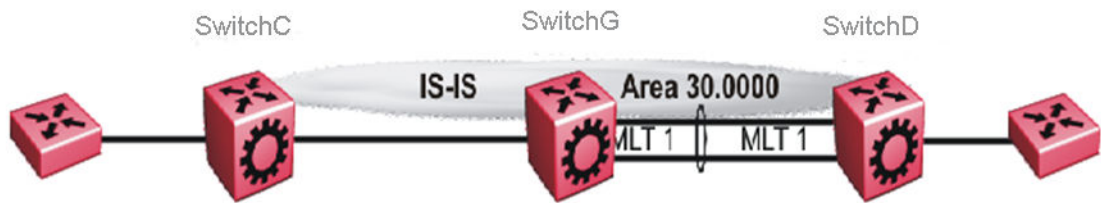
Figure 84: IS-IS SPBM global
