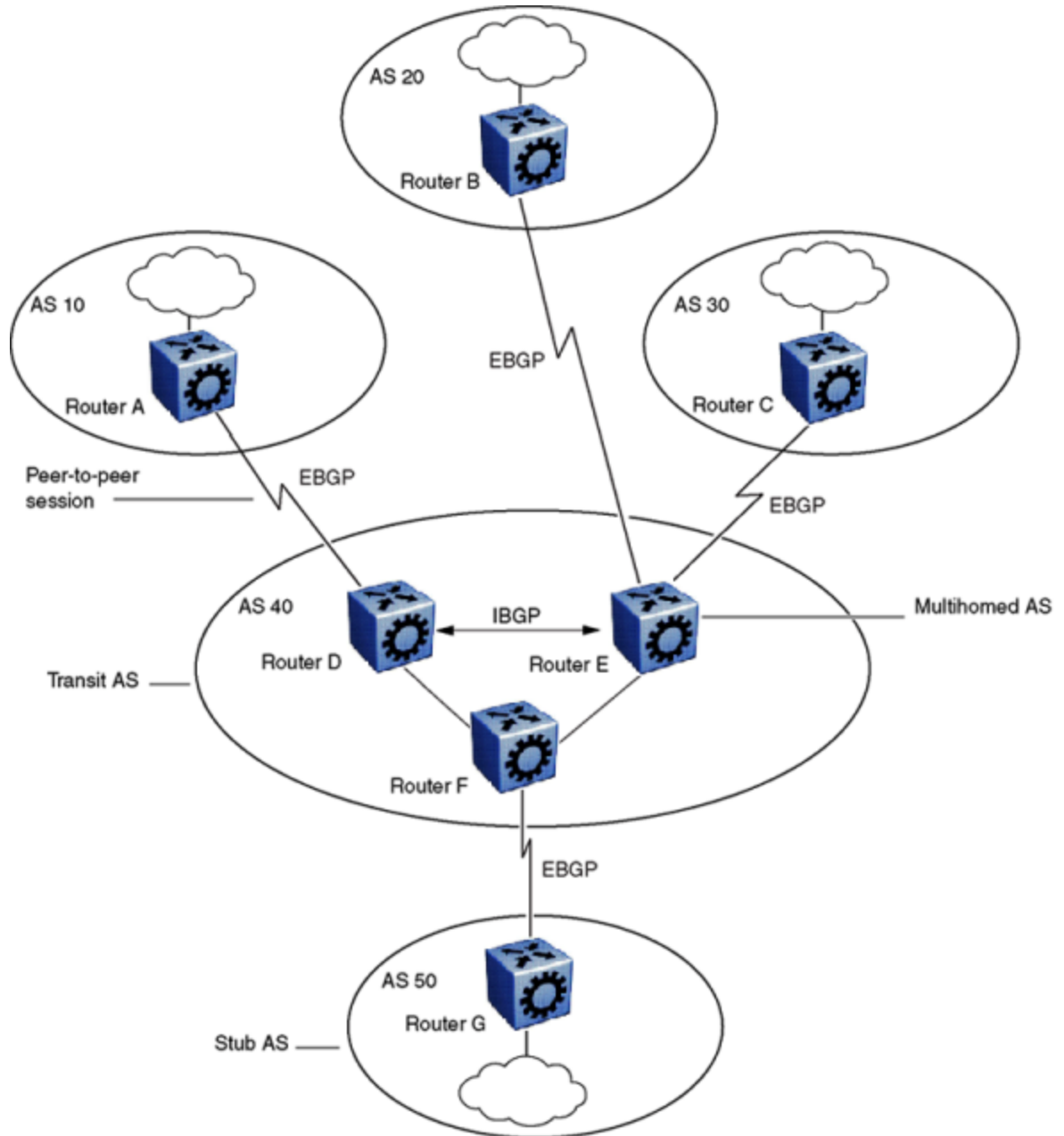
Figure 18: BGP networks
