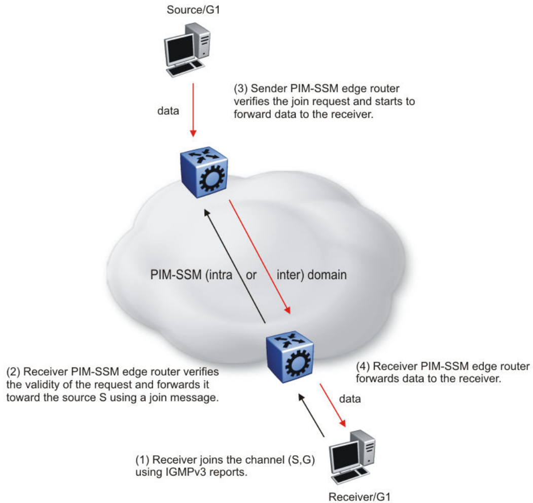
Figure 143: PIM-SSM architecture
