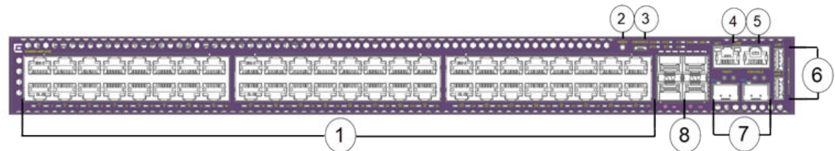
Figure 293: 5420M-48T-4YE Front Panel
