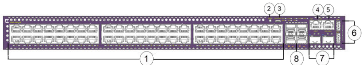
Figure 287: 5420F-48P-4XE Front Panel
