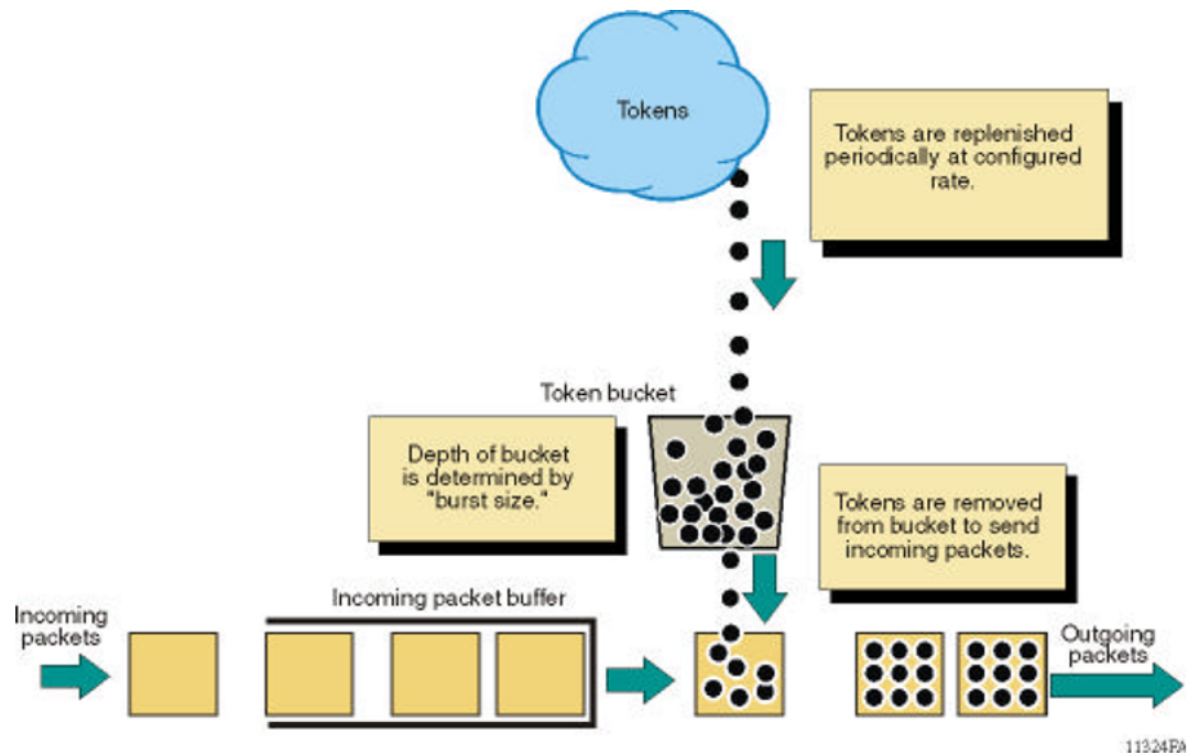
Figure 218: Token flow
