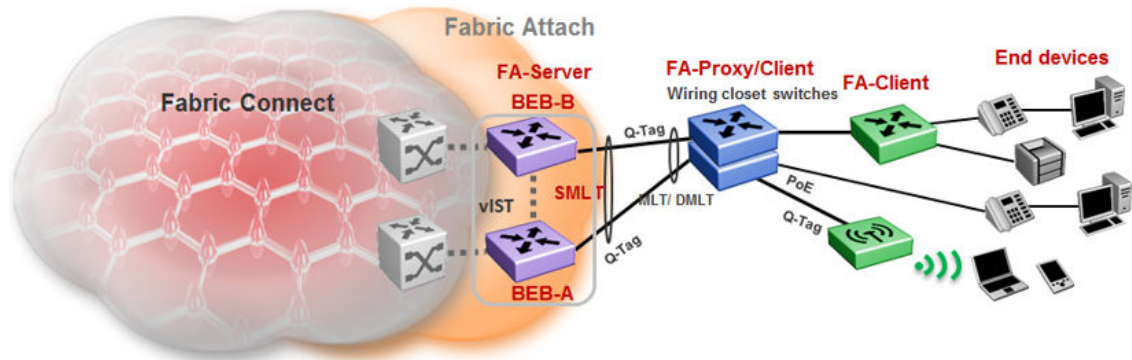
Figure 75: FA in a dual-homed SMLT deployment
