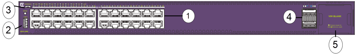
Figure 296: 5520-24W
