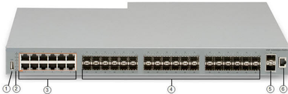
Figure 302: VSP 4450GSX-PWR+
