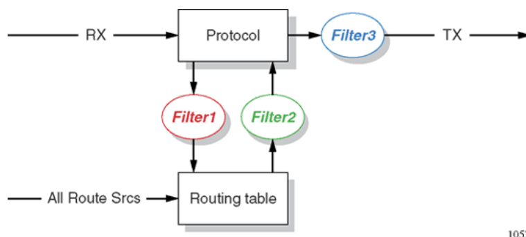
Figure 232: Route filtering stages
