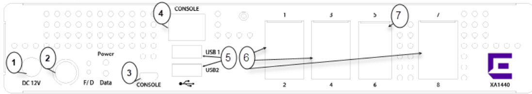
Figure 310: XA1400 Series switches rear panel
