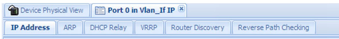
Figure 12: Menu bar
