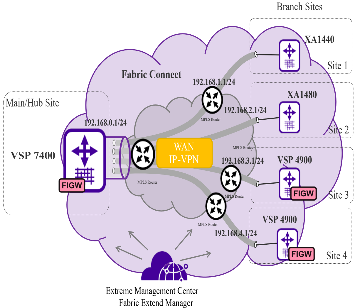
Figure 63: Fabric Extend IP VPN Deployment Option
