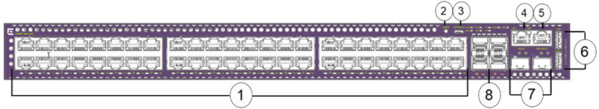
Figure 288: 5420F-48P-4XL Front Panel
