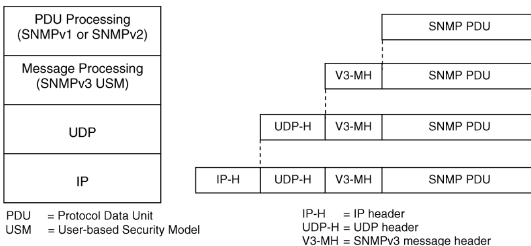
Figure 238: SNMPv3 USM
