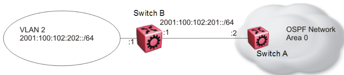
Figure 216: OSPFv3 configuration
