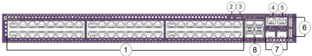
Figure 289: 5420F-48T-4XE Front Panel
