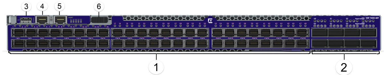
Figure 285: VSP 7400-48Y
