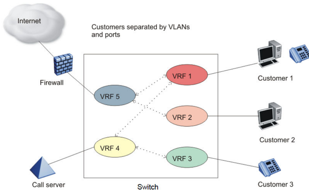
Figure 270: Inter-VRF forwarding
