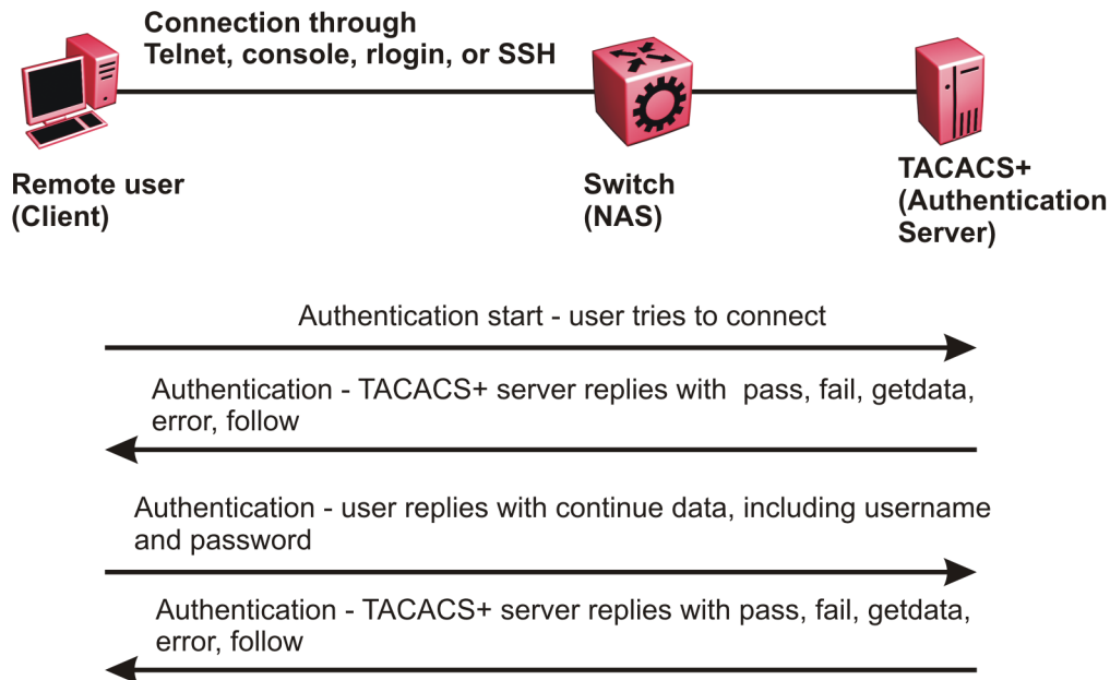
Figure 253: Authentication process
