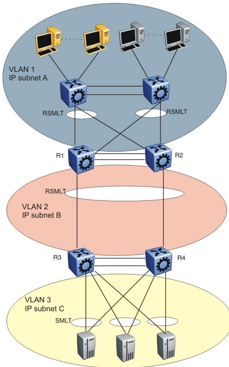
Figure 234: SMLT and RSMLT in Layer 3 environments
