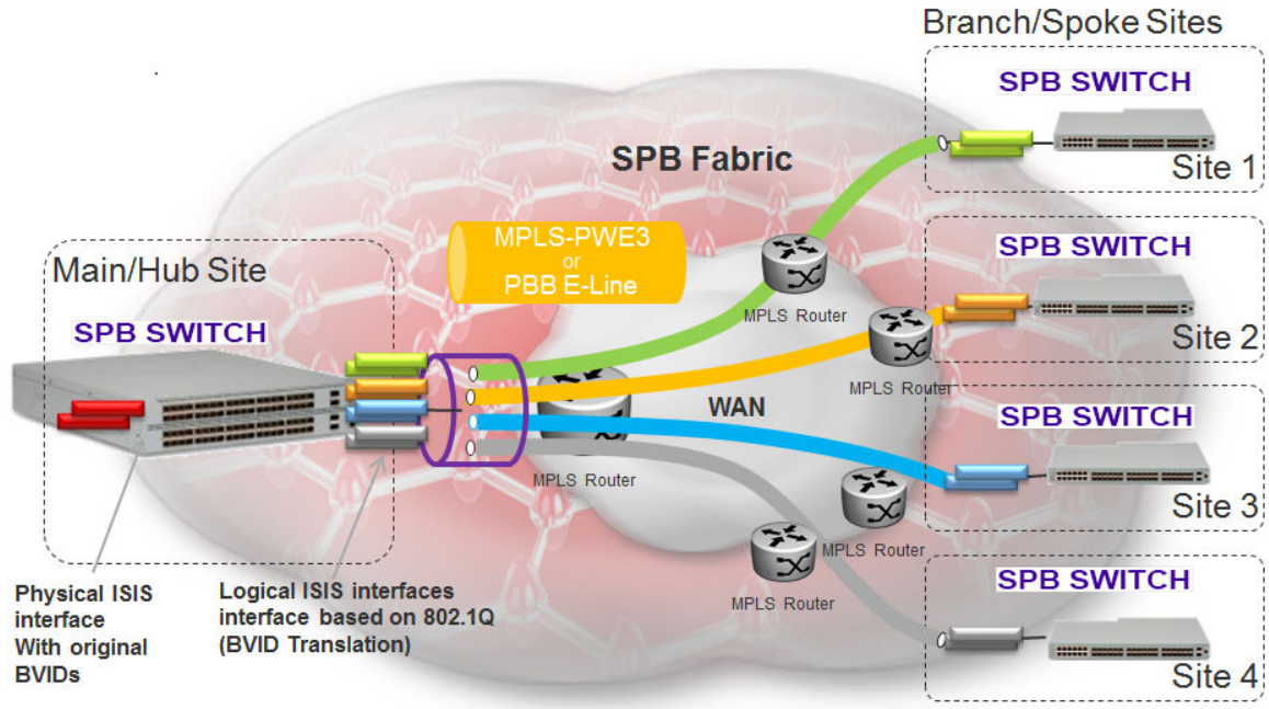
Figure 66: Fabric Extend Pseudowire Deployment Option
