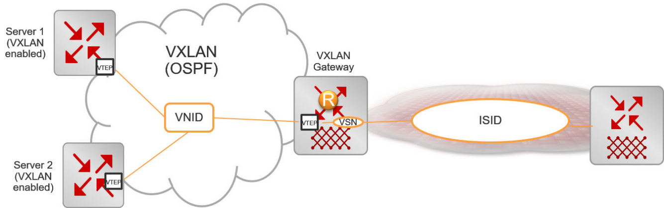
Figure 279: VXLAN-to-SPB deployment
