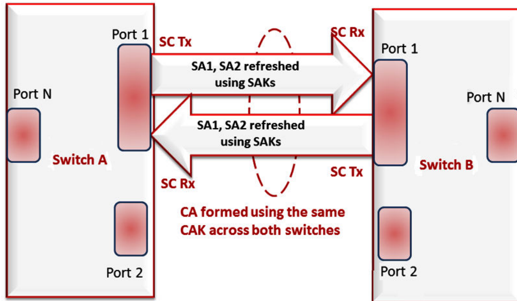
Figure 193: MACsec relationship
