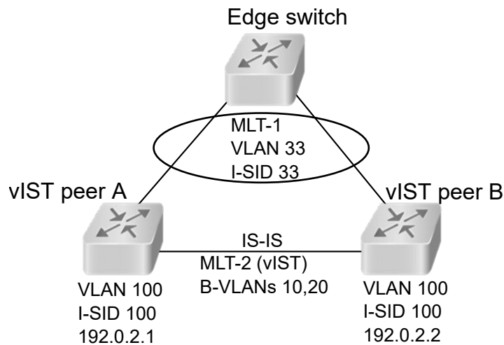
Figure 198: SMLT with vIST configuration example
