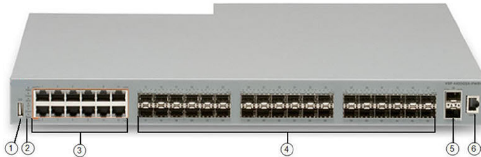
Figure 283: VSP 4450GSX-DC
