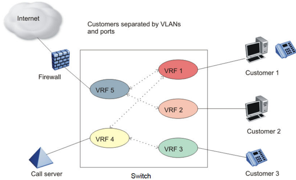
Figure 270: Inter-VRF forwarding
