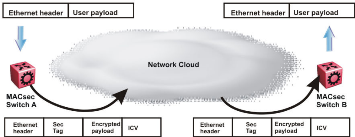
Figure 195: MACsec operation
