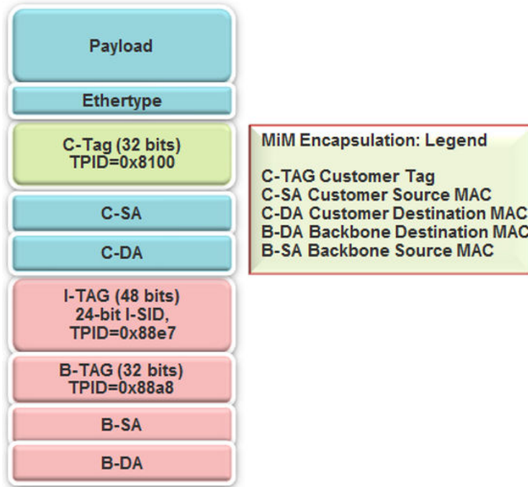
Figure 74: MiM encapsulation
