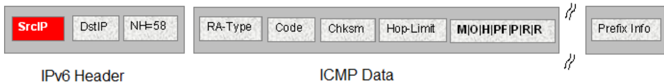
Figure 184: IPv6 ICMP RA Data Packet Online
