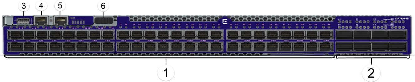
Figure 285: VSP 7400-48Y
