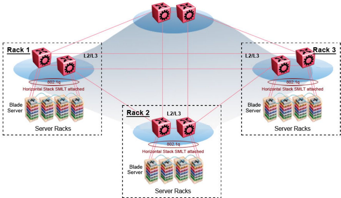
Figure 105: SPBM data center—full mesh
