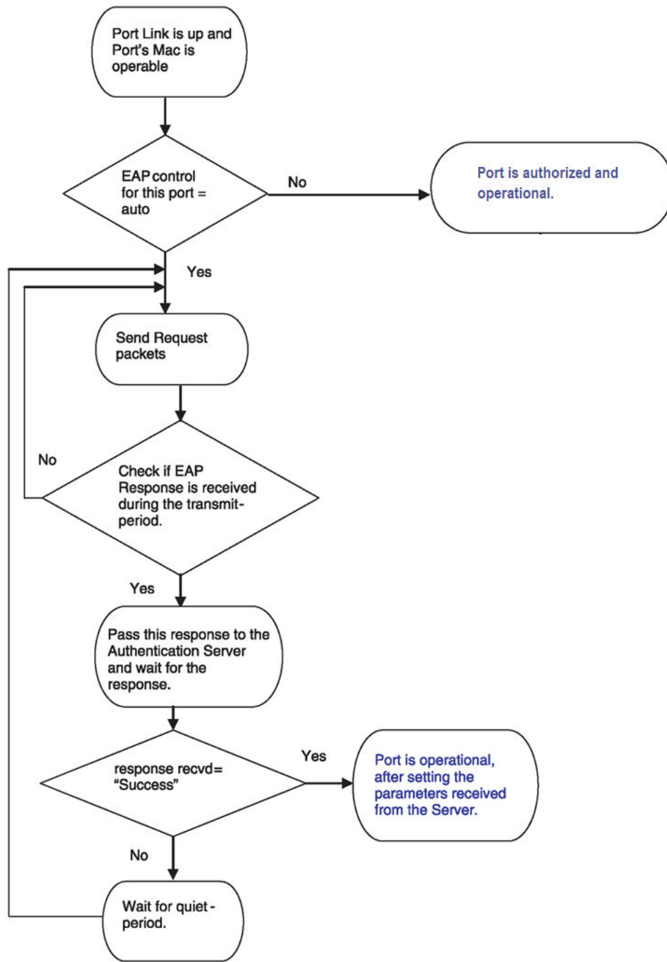
Figure 58: EAP flow diagram
