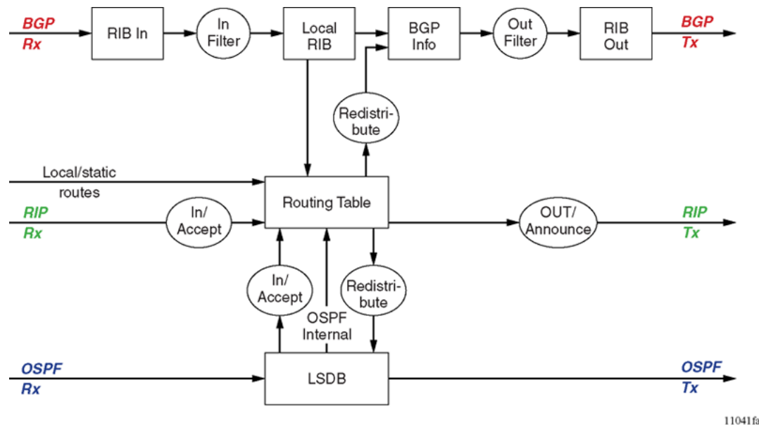
Figure 212: Route filtering for BGP, RIP, and OSPF routing protocols
