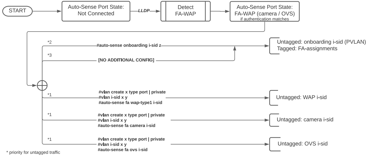
Figure 8: Auto-sense FA WAP / camera / OVS without NAC
