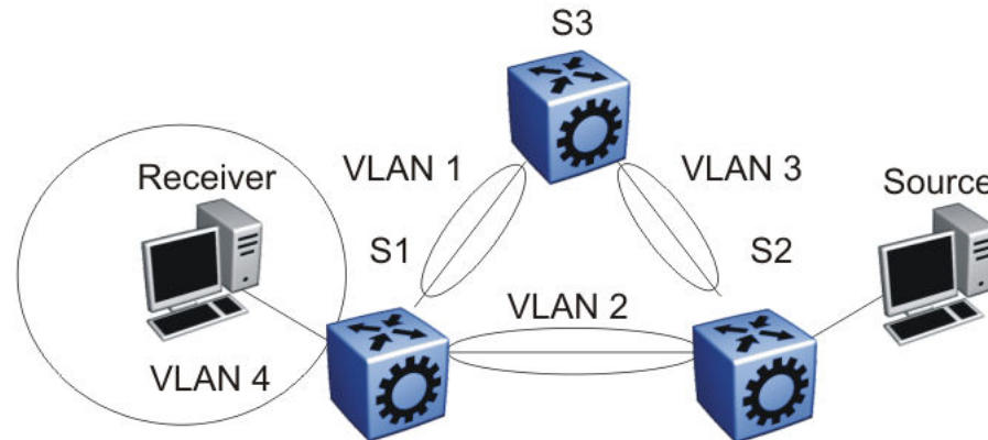
Figure 130: IP multicast sources and receivers on interconnected VLANs
