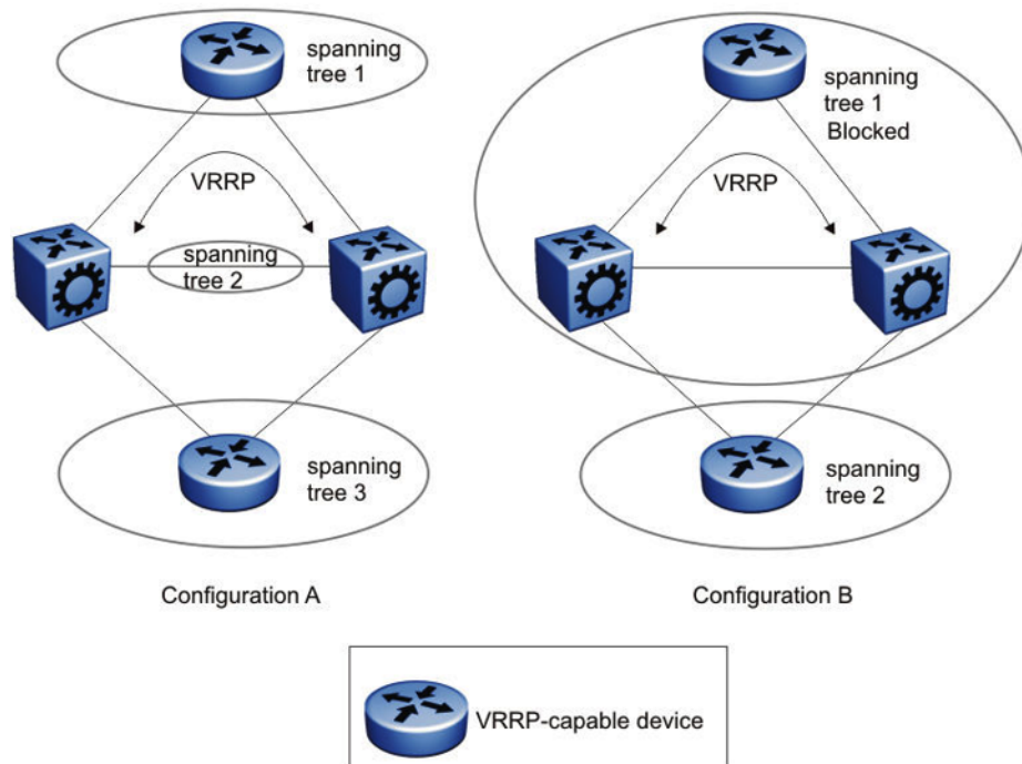
Figure 252: VRRP and STG configurations
