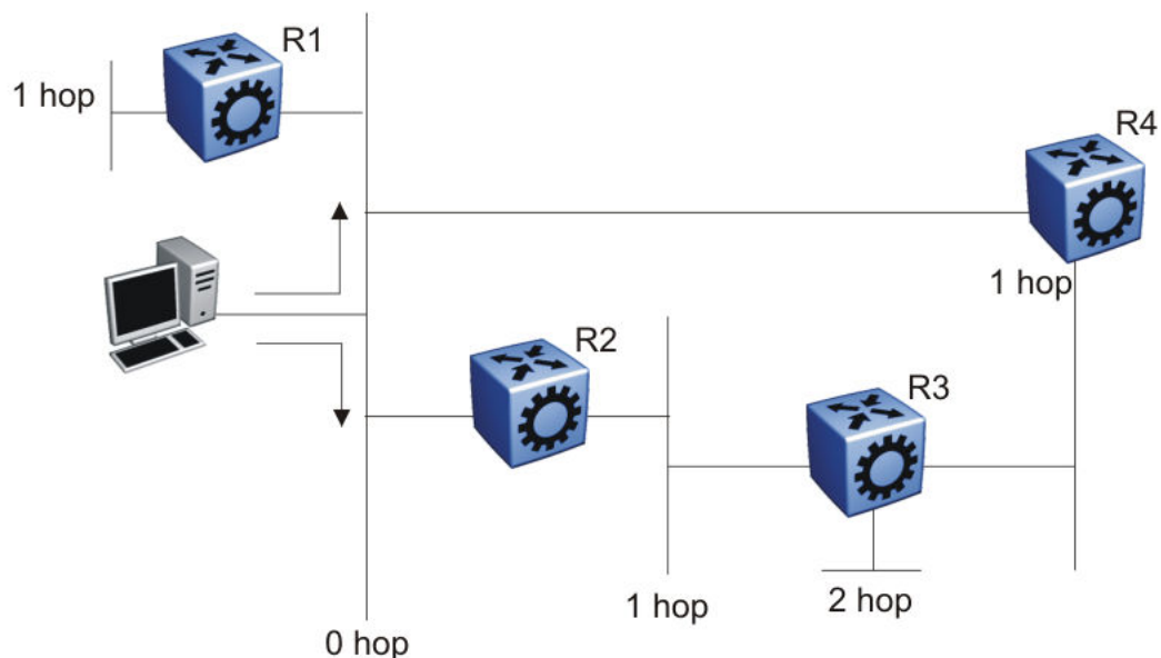
Figure 206: Hop count or metric in RIP
