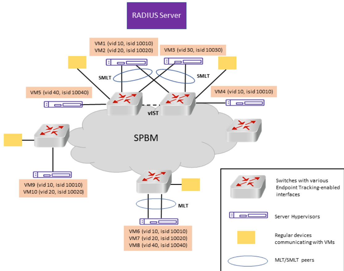
Figure 85: SPBM Cloud Example
