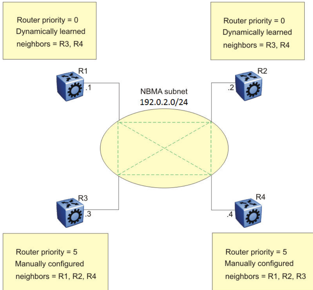
Figure 192: NBMA Subnet Configuration Example
