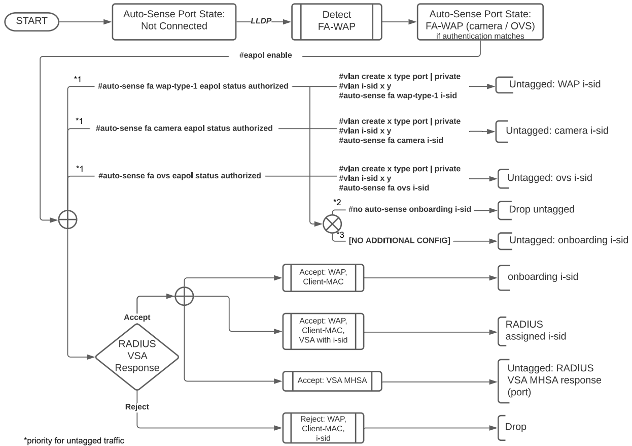
Figure 9: Auto-sense FA WAP / camera / OVS with NAC
