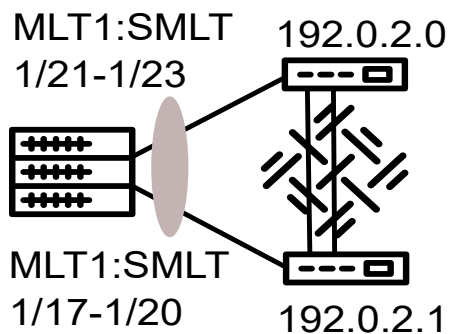
Figure 80: FA configuration in dual-homed SMLT
