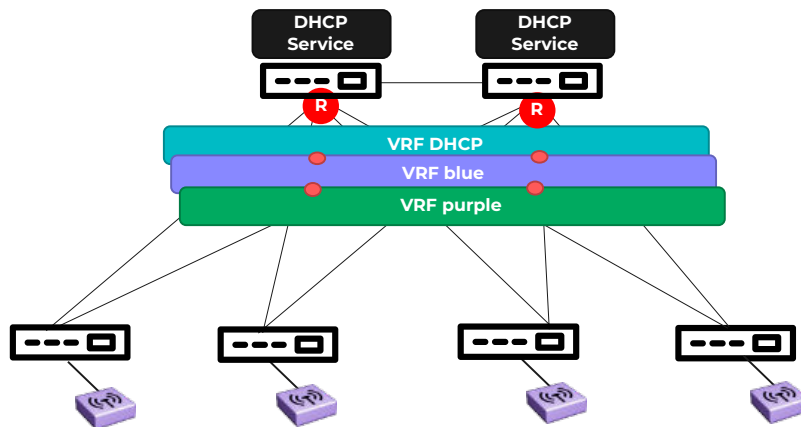
Figure 47: DHCP Server with Multiple VRF - Small Campus Network
