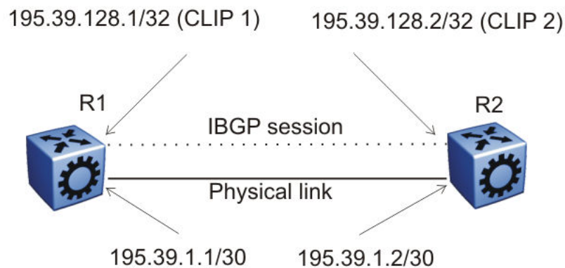
Figure 152: Routers with iBGP connections
