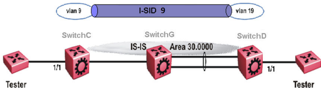
Figure 97: Layer 2 VSN with different VLAN IDs
