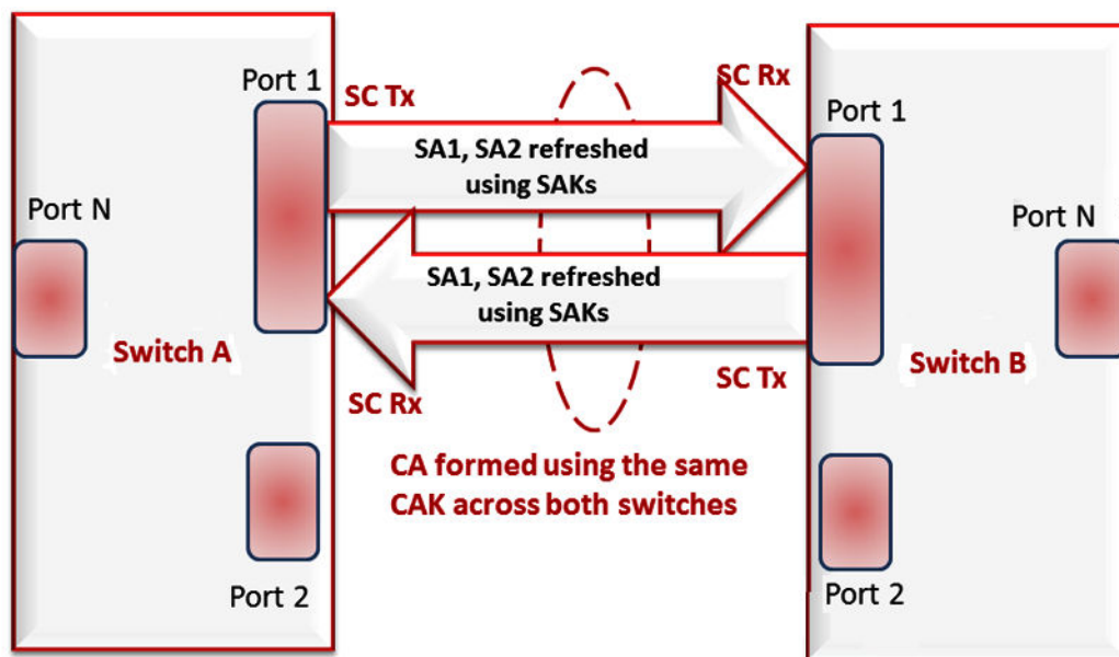
Figure 177: MACsec relationship
