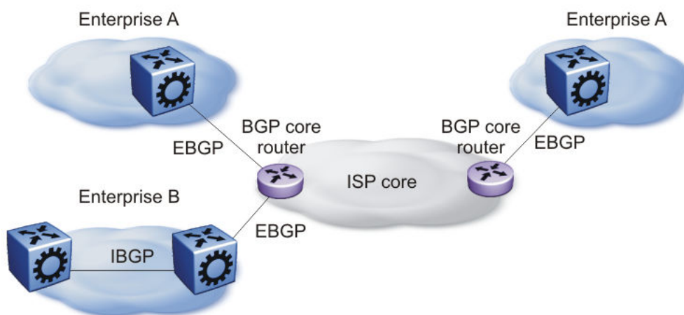
Figure 38: BGP and Edge Aggregation
