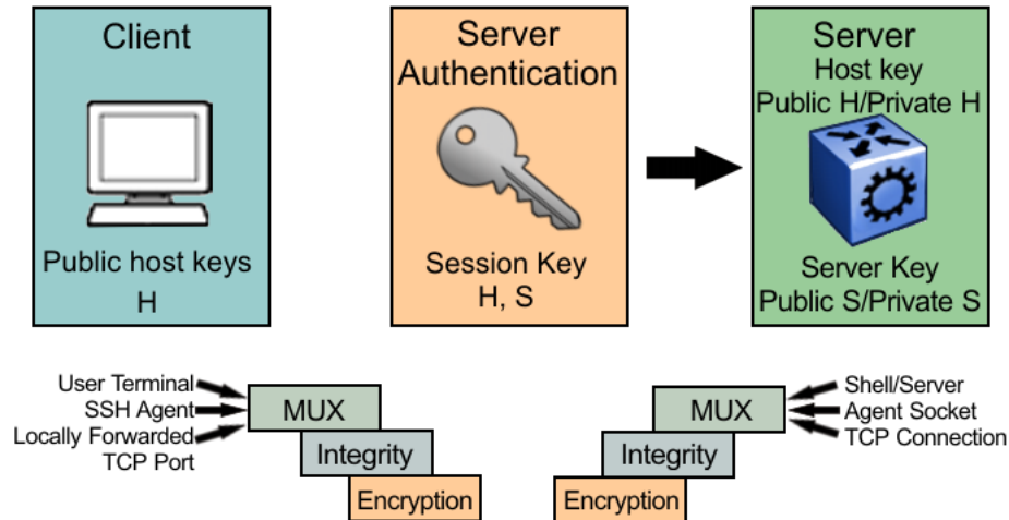
Figure 217: Overview of the SSHv2 protocol
