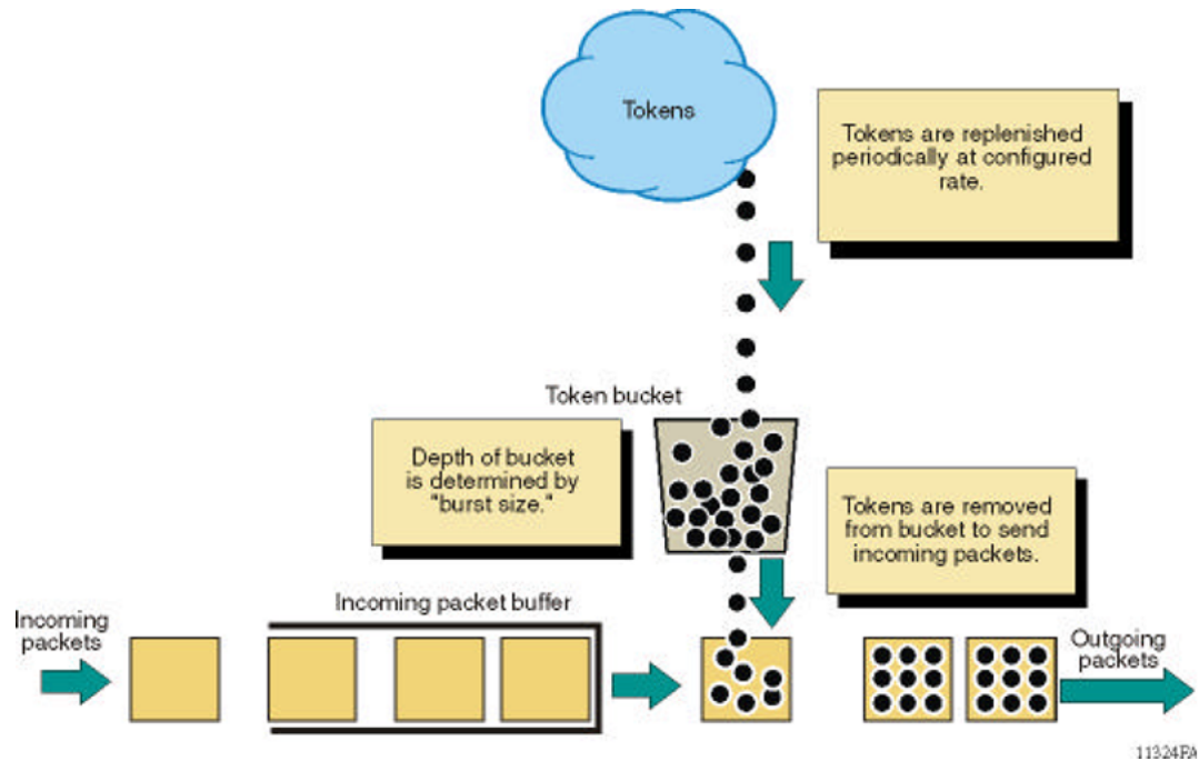
Figure 200: Token flow
