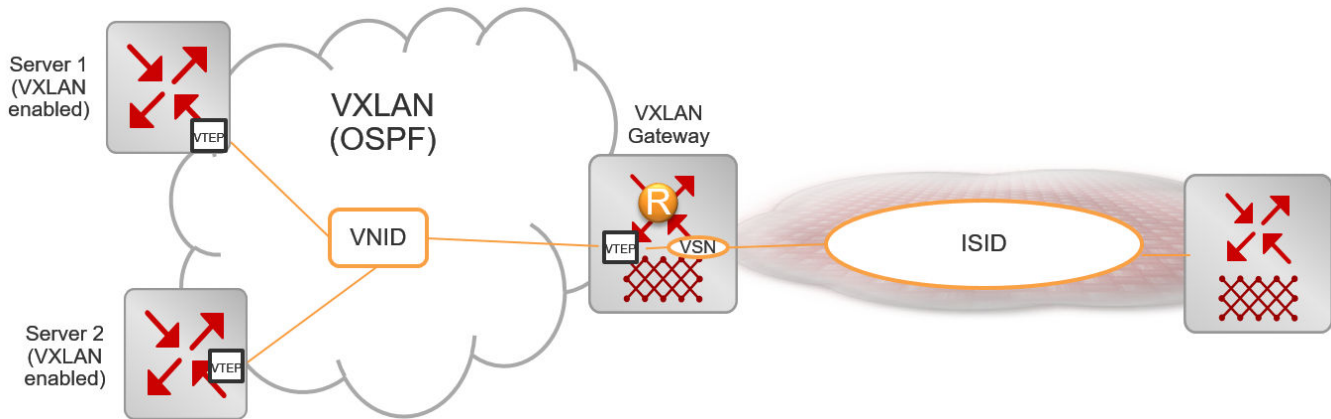
Figure 256: VXLAN-to-SPB deployment
