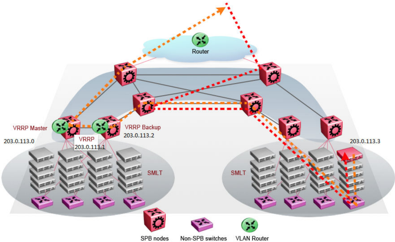
Figure 107: Traditional routing after moving VMs
