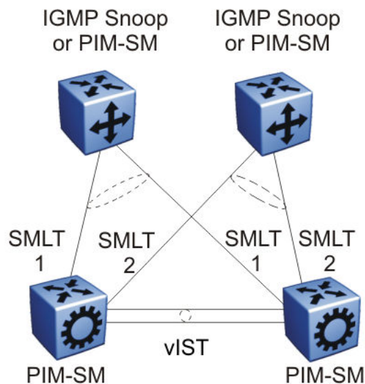
Figure 133: Multicast routing using PIM-SM
