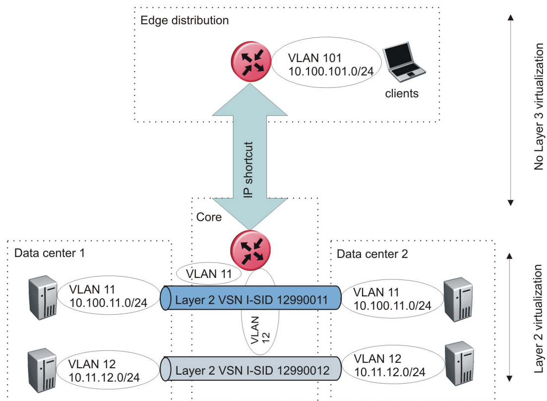
Figure 103: IP shortcut scenario to move traffic between data centers
