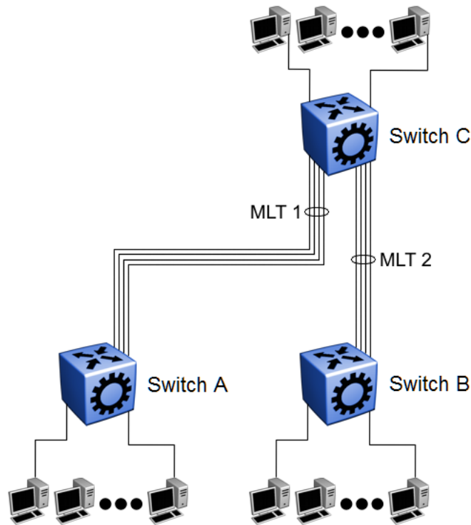
Figure 185: Switch-to-switch multilink trunks configuration
