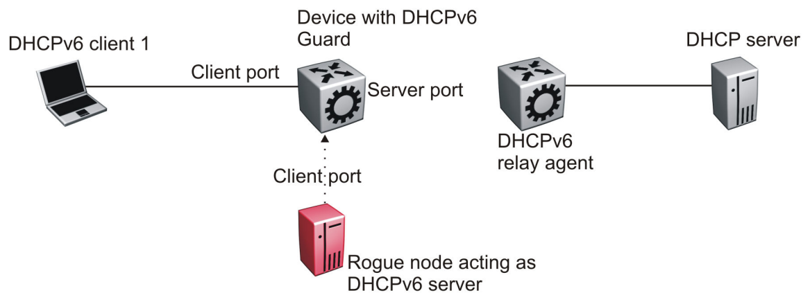
Figure 166: DHCPv6 Topology 2
