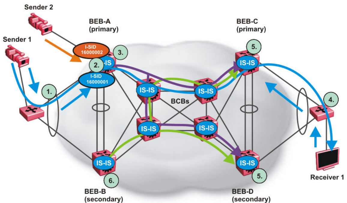
Figure 142: IP Multicast over Fabric Connect streams in an SMLT configuration
