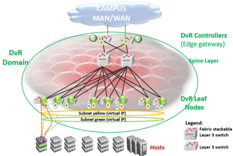
Figure 50: SPB Fabric network with central Layer 3 Controller and distributed Layer 3 datapath at the edges
