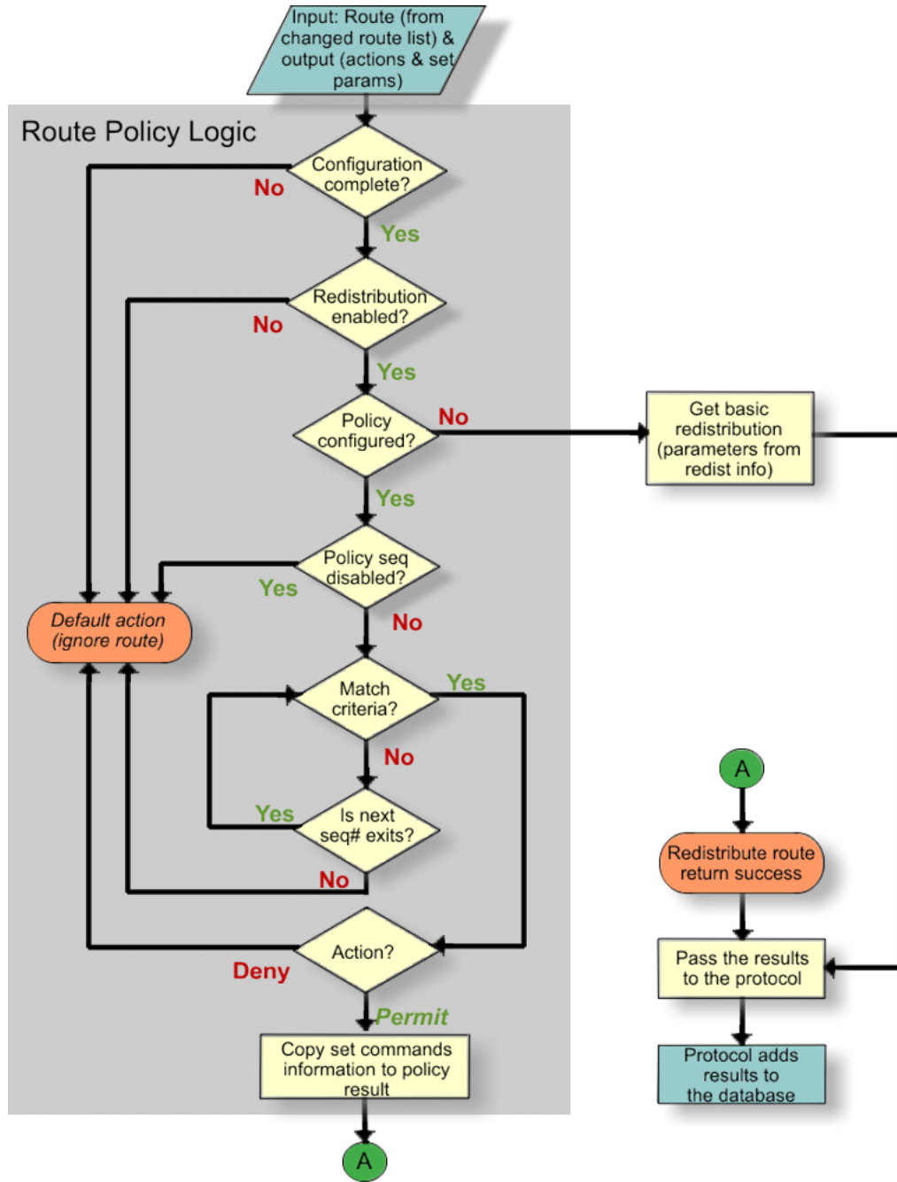
Figure 215: Route filtering logic
