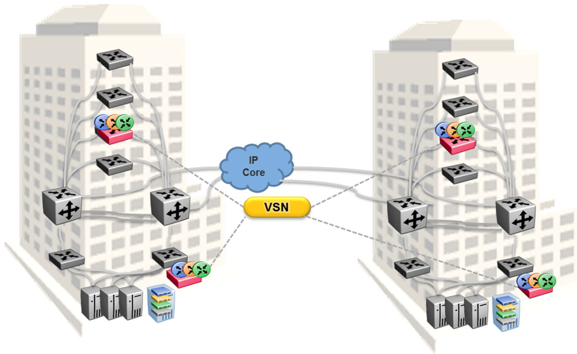
Figure 71: Fabric Extend Full Mesh Campus Deployment Option
