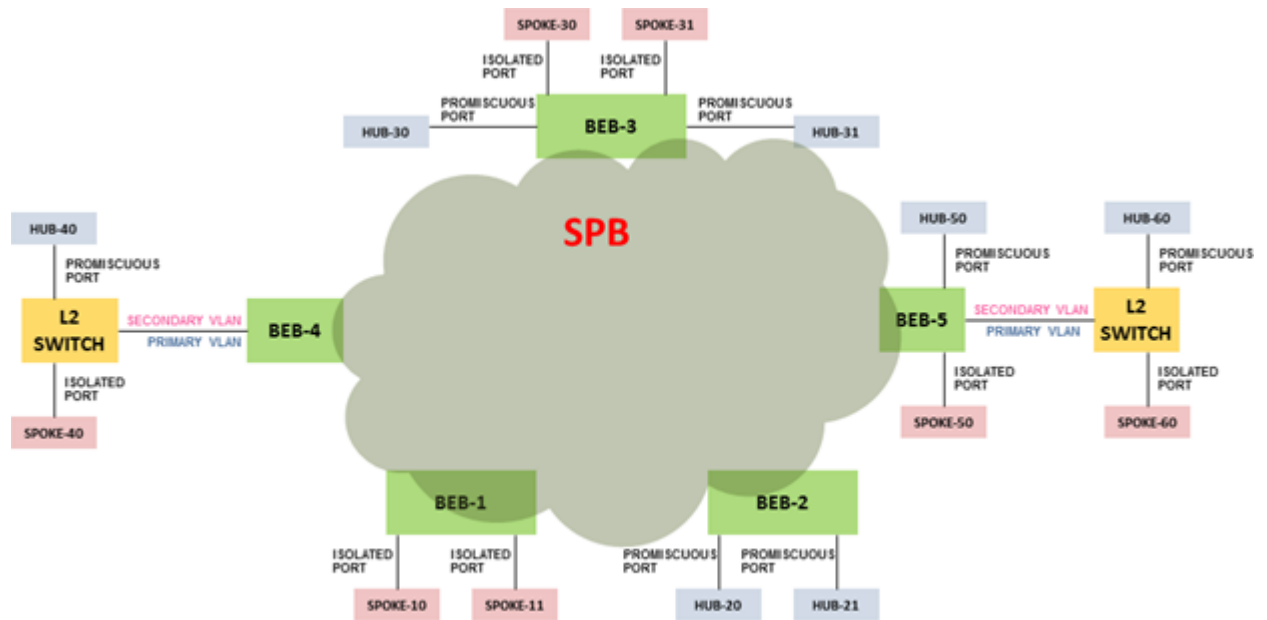
Figure 62: Sample E-Tree configuration
