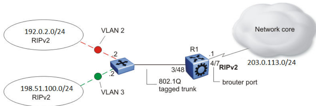
Figure 208: Configuration example-RIPv2 only
