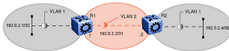
Figure 153: IP routing between VLANs
