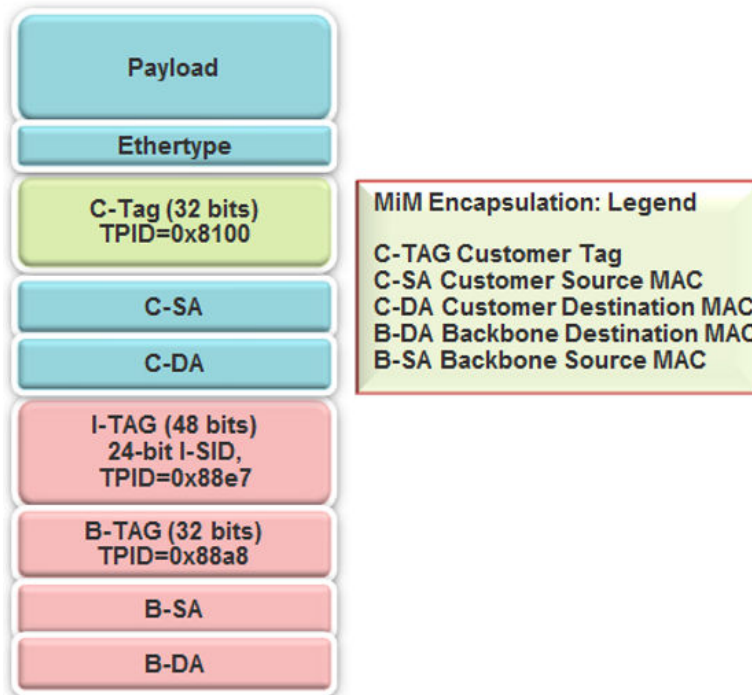
Figure 77: MiM encapsulation
