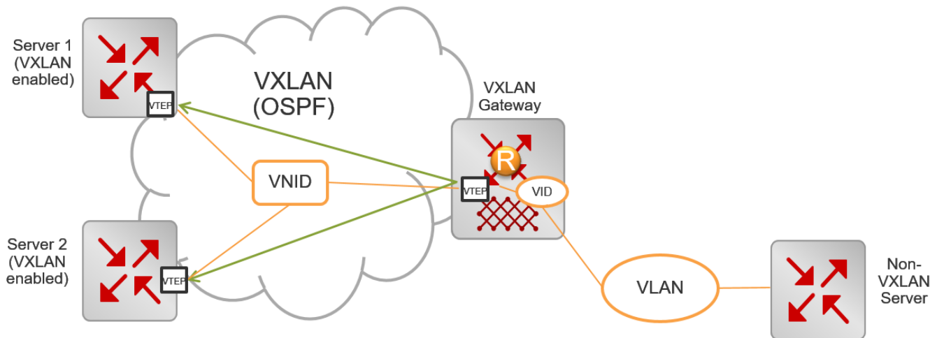
Figure 254: VXLAN-to-VLAN deployment
