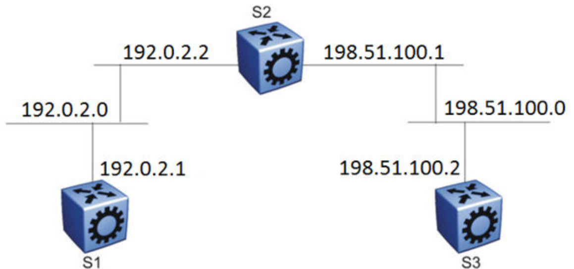
Figure 196: Example 2: OSPF on two subnets in one area
