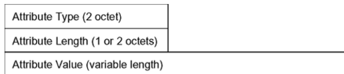
Figure 33: Path Attribute Encoding
