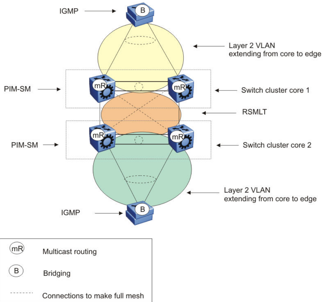
Figure 136: Multicast SMLT square 2
