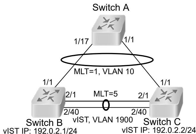
Figure 181: Network topology for traffic flow example
