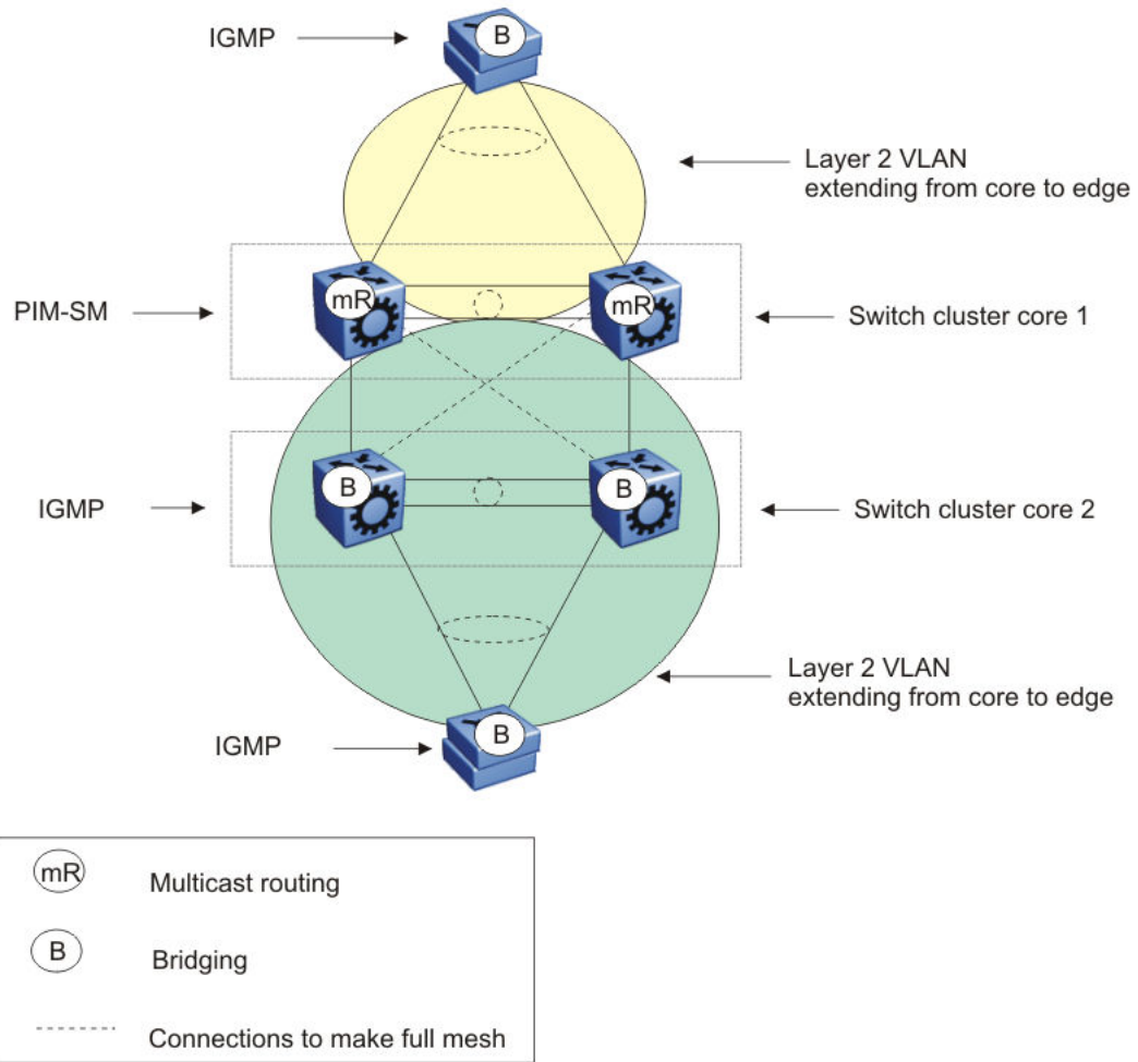
Figure 135: Multicast SMLT square 1
