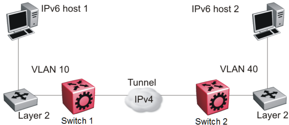
Figure 162: Tunnel configuration between router ports
