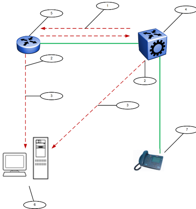
Figure 176: LLDP in a LAN
