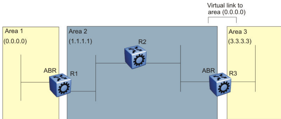
Figure 193: Virtual link between ABRs through a transit area
