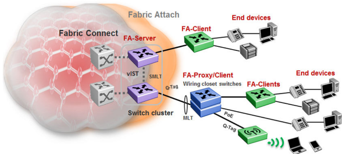
Figure 79: Fabric Attach in a single-homed SMLT deployment
