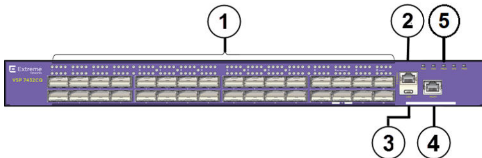
Figure 258: VSP 7432CQ
