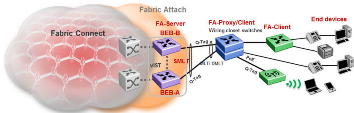
Figure 78: FA in a dual-homed SMLT deployment
