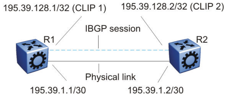
Figure 35: Routers with iBGP connections
