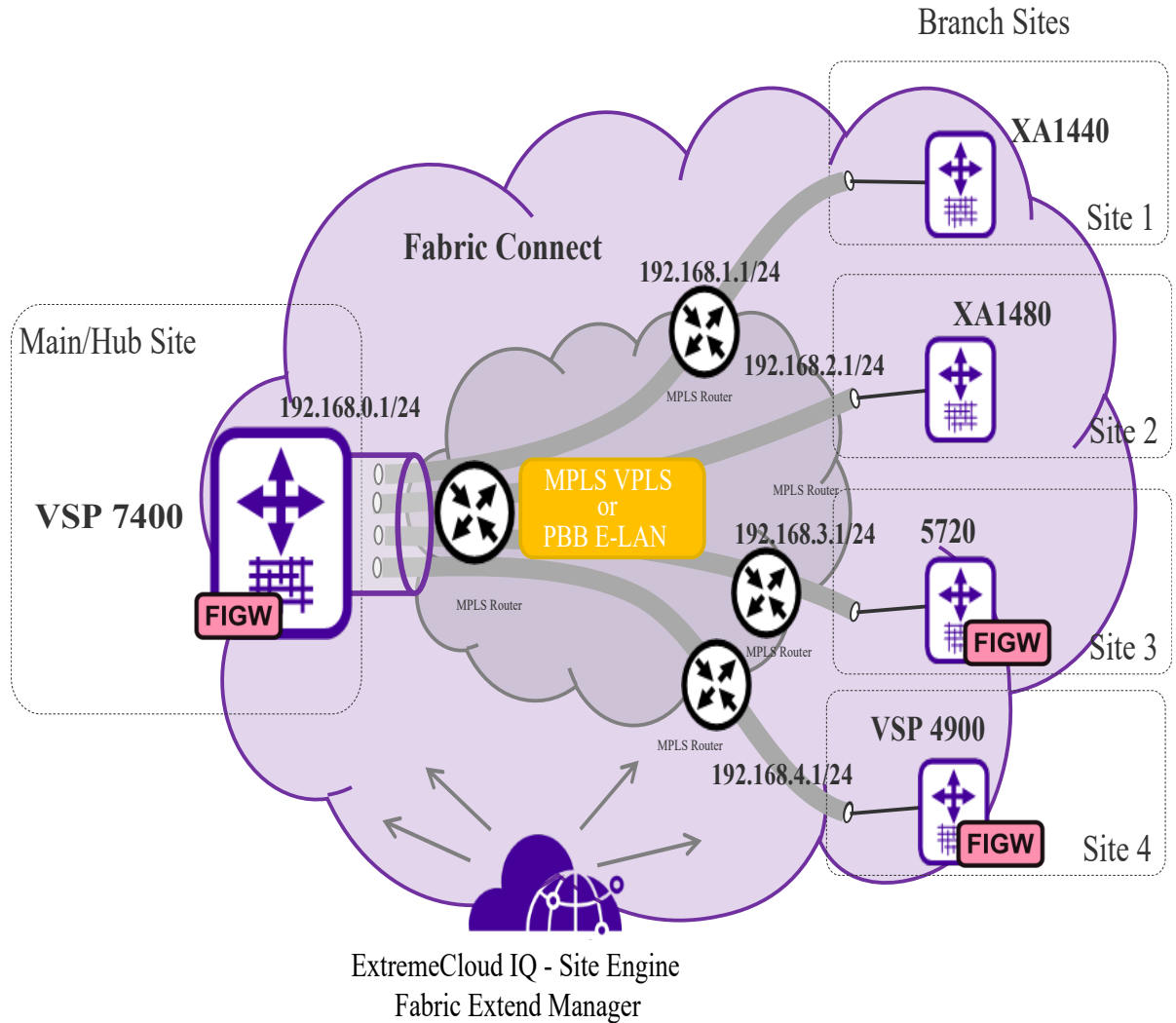
Figure 70: Fabric Extend VPLS Deployment Option
