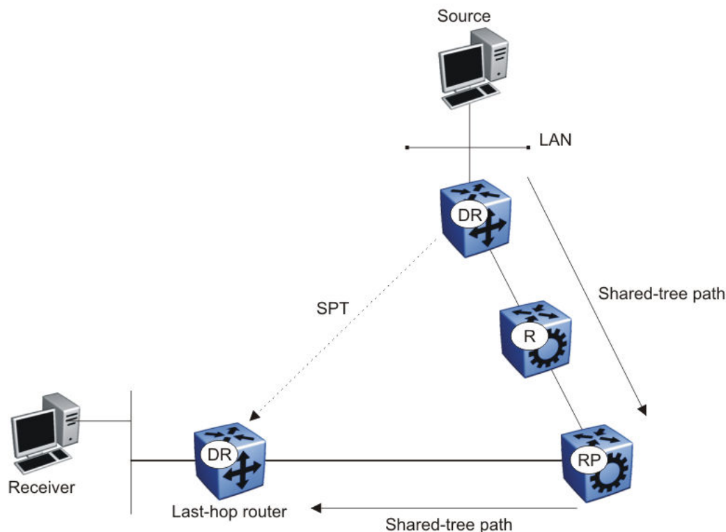
Figure 127: Shared tree and shortest-path tree
