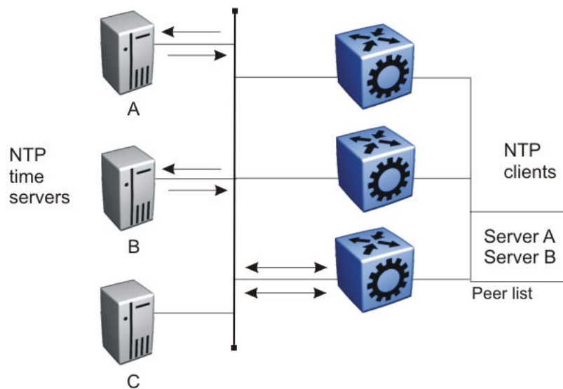
Figure 189: NTP Time Servers Operating in Unicast Client Mode
