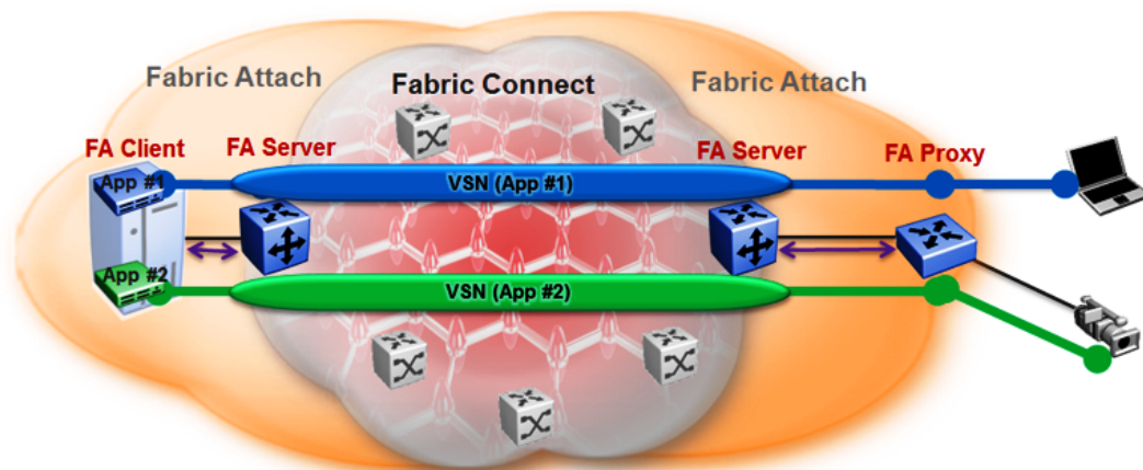
Figure 73: Fabric Attach Server connecting client or proxy devices to the Fabric network
