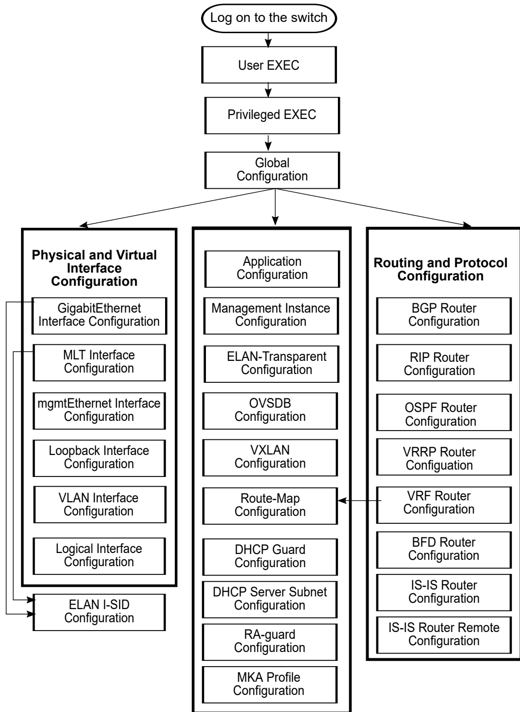
Figure 13: CLI Command Mode Navigation
