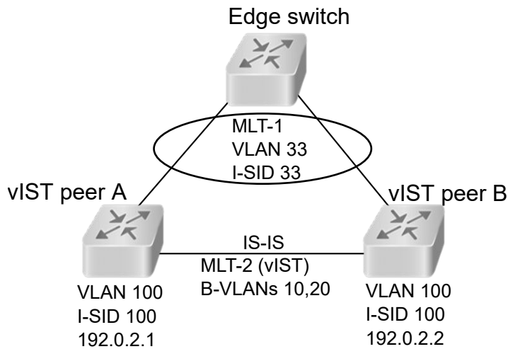
Figure 182: SMLT with vIST configuration example
