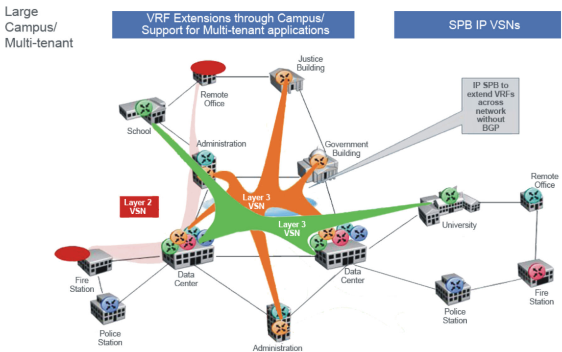
Figure 59: Multi-tenant SPBM metro network
