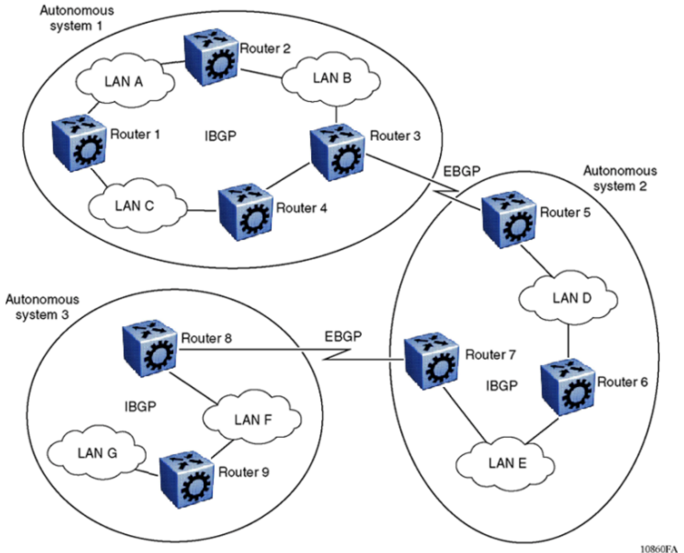
Figure 20: Internetwork segmented into three autonomous systems
