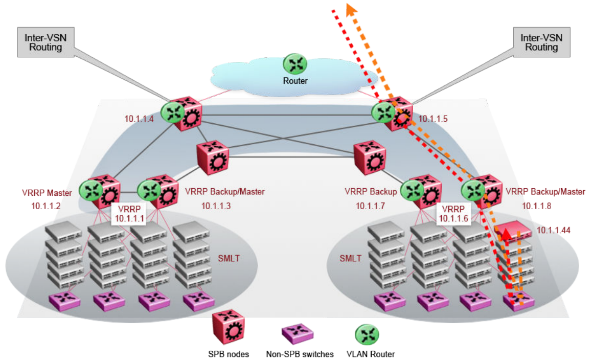
Figure 109: Optimized routing after moving VMs
