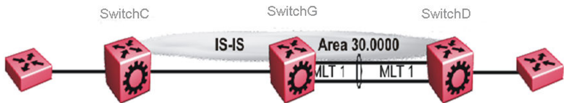
Figure 64: IS-IS SPBM global
