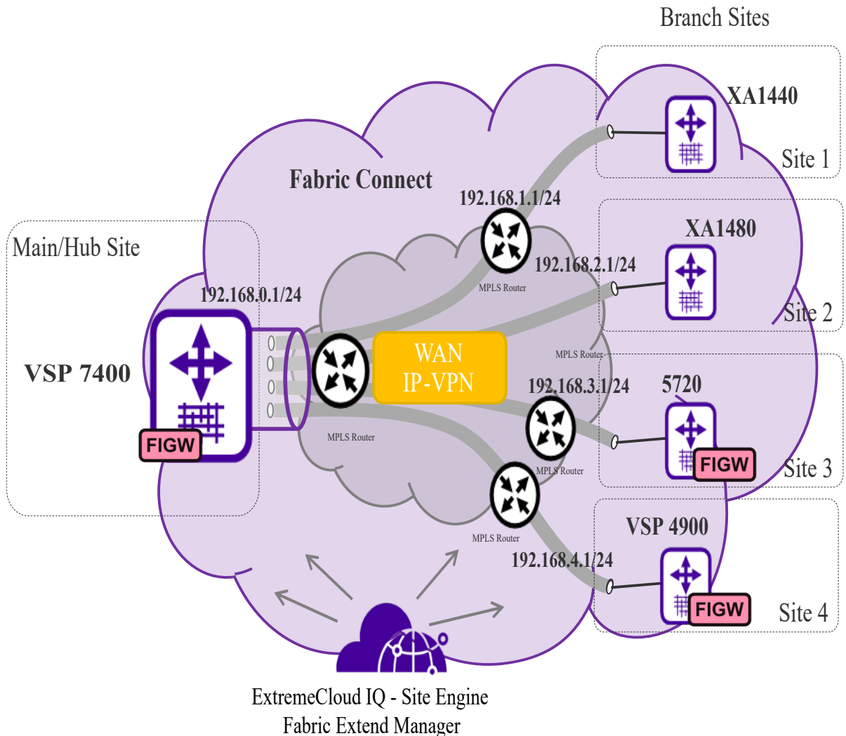
Figure 69: Fabric Extend IP VPN Deployment Option
