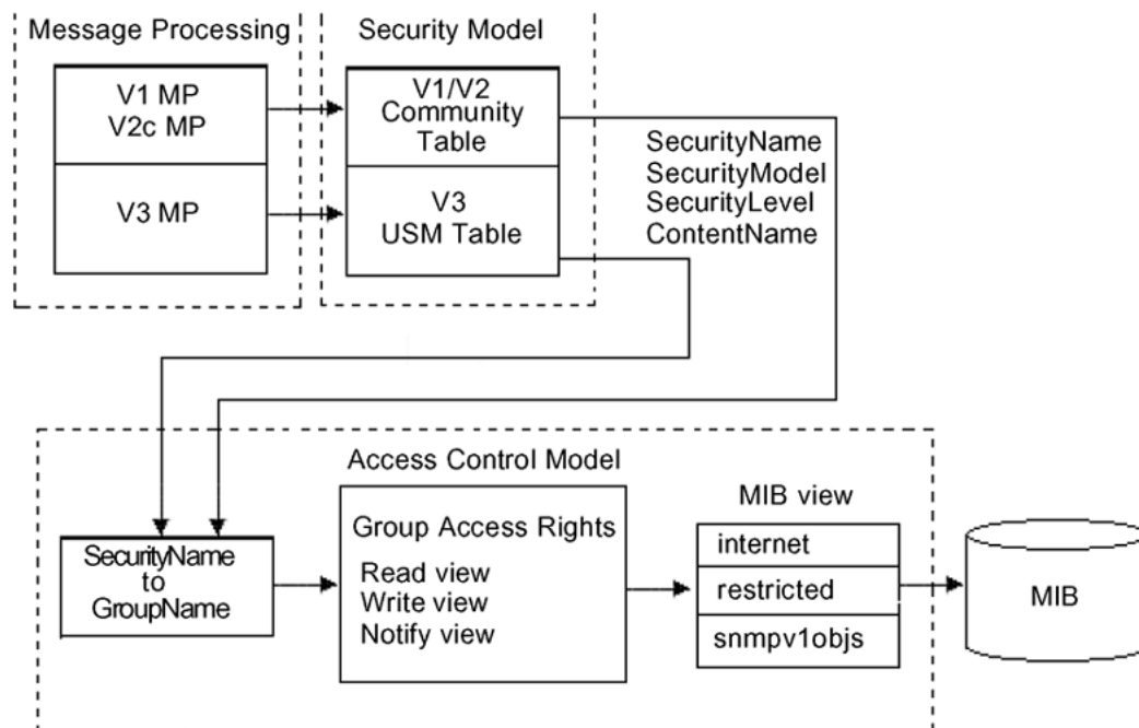
Figure 220: USM association with VACM
