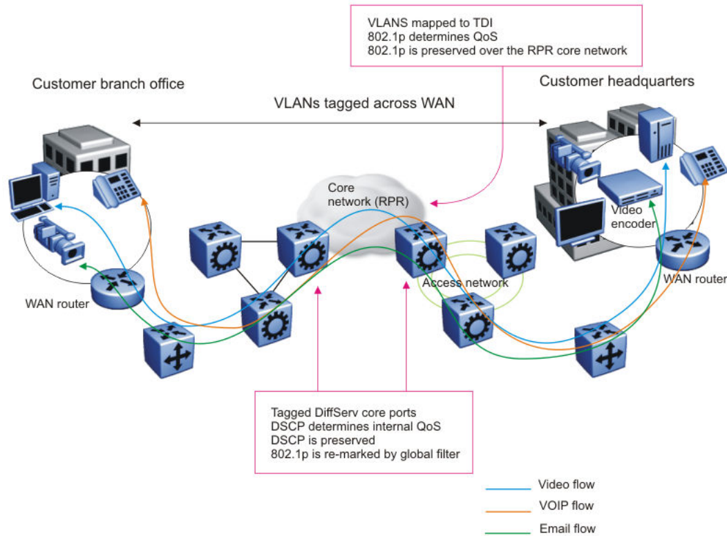
Figure 202: RPR QoS interworking
