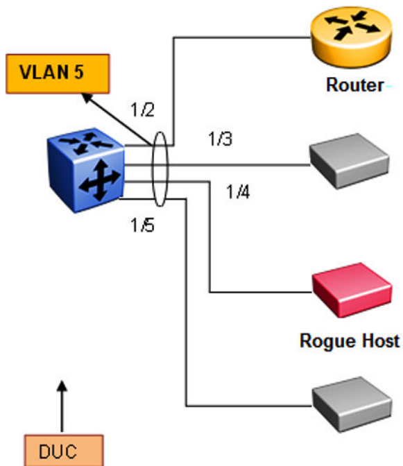
Figure 167: RA Guard Topology1
