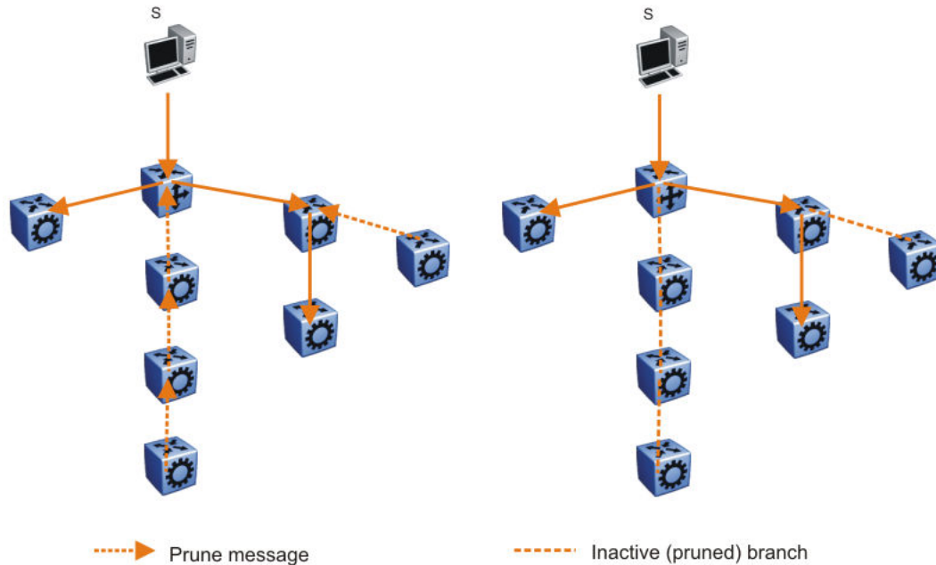
Figure 123: Pruning routers from a distribution tree
