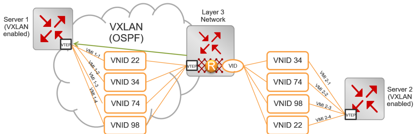
Figure 255: VXLAN-to-VXLAN deployment
