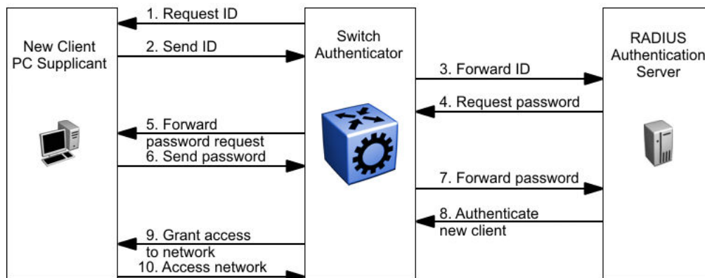
Figure 56: EAP configuration example
