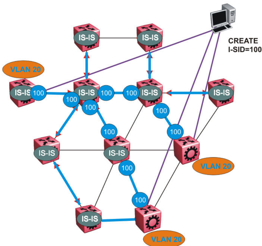
Figure 92: SPBM BMAC and I-SID population
