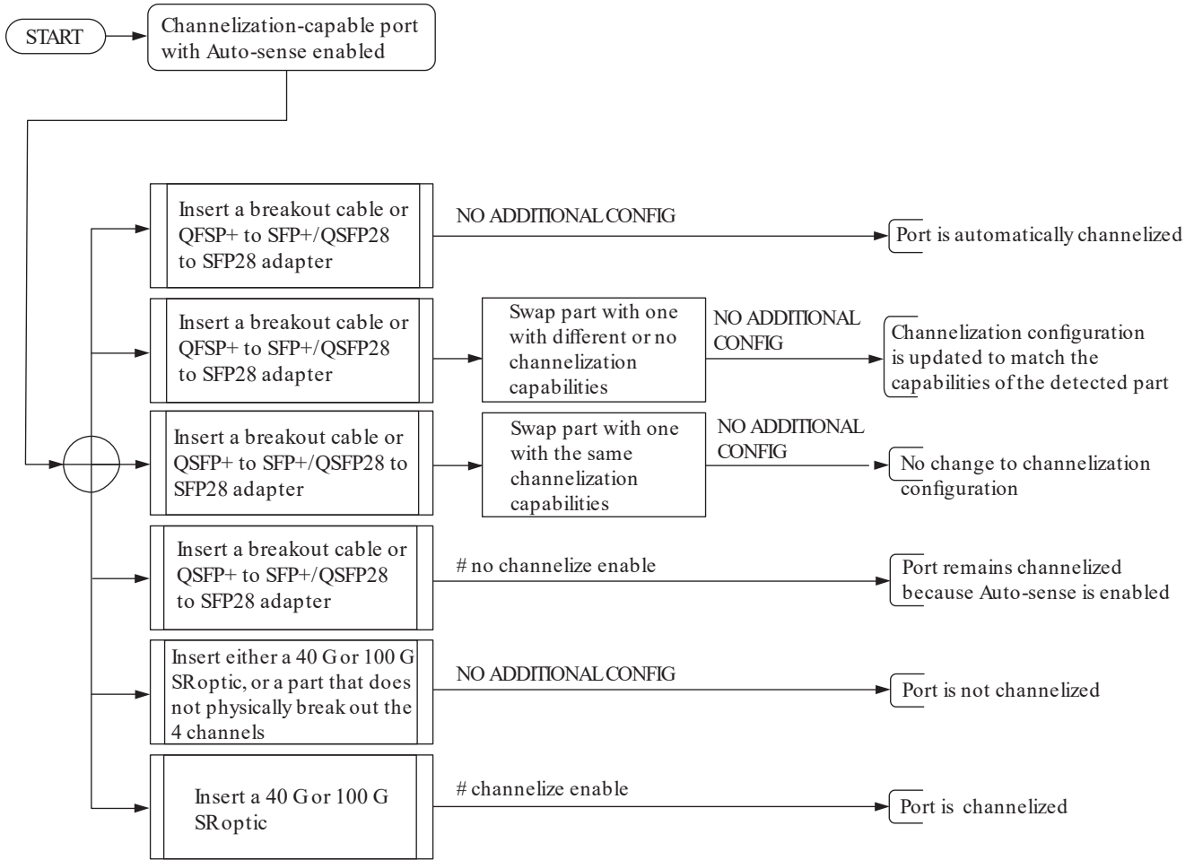
Figure 10: Automatic Channelization with Auto-sense enabled
