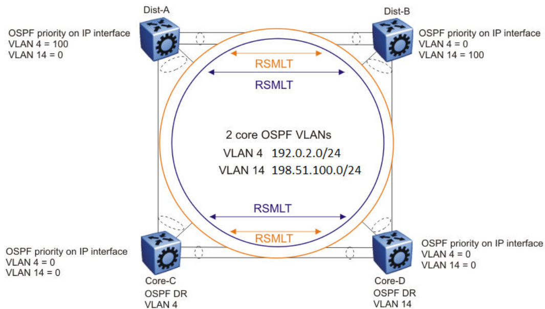
Figure 194: RSMLT with dual core VLANs
