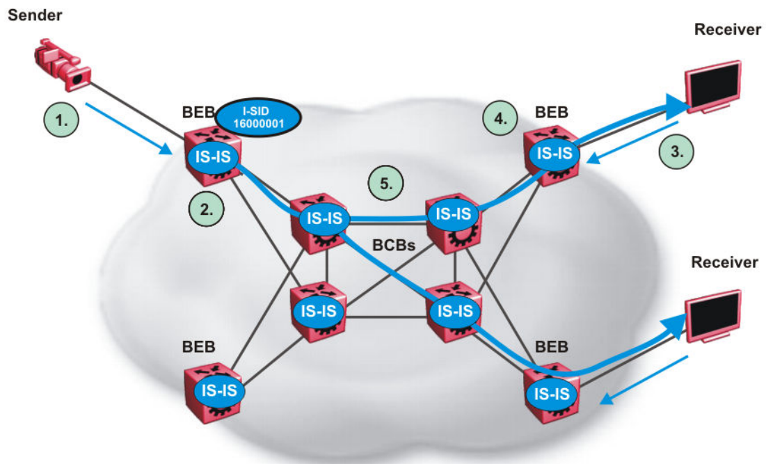
Figure 141: IP Multicast over Fabric Connect streams
