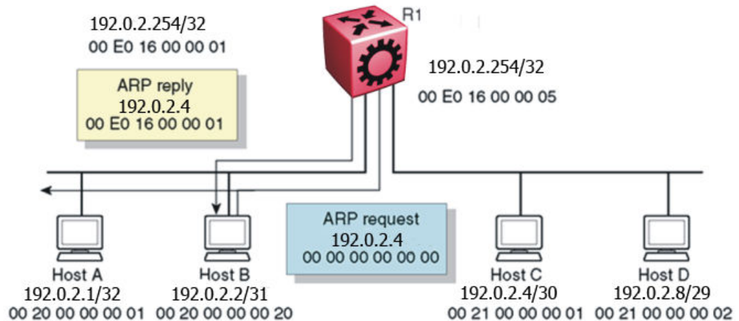
Figure 18: Proxy ARP operation
