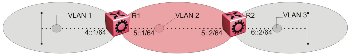
Figure 161: IPv6 routing between VLANs
