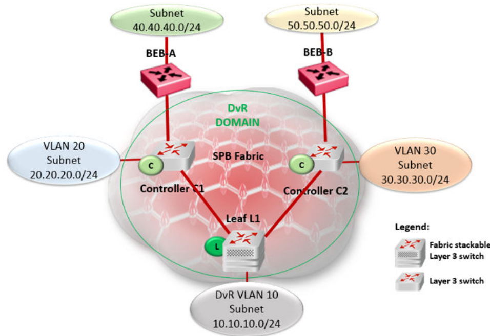
Figure 52: Redistribution of IPv4 local and static routes
