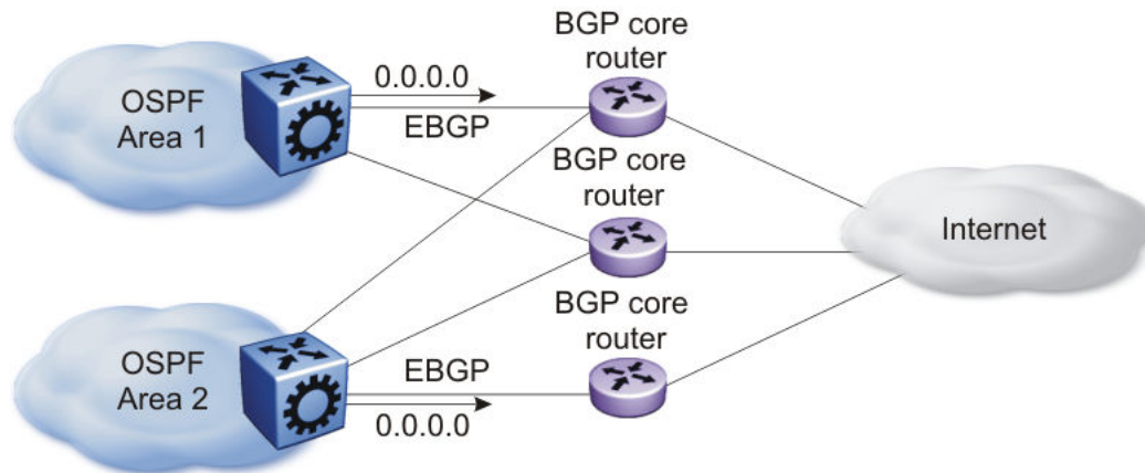
Figure 41: Multiple OSPF Regions Peering with the Internet
