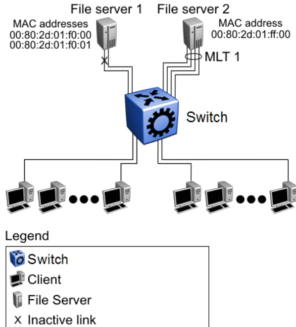
Figure 186: Switch-to-server multilink trunk configuration
