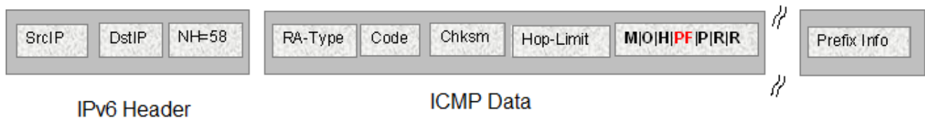
Figure 173: IPv6 ICMP RA data packet outline for router preference validation
