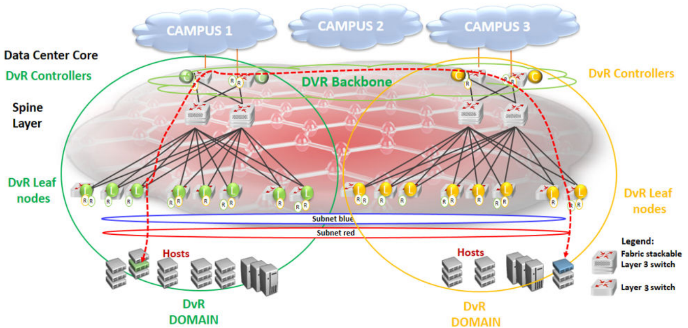
Figure 51: Shortest path routing between servers in different data centers
