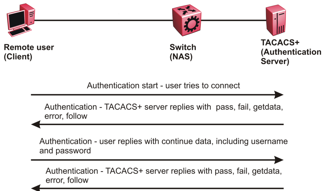
Figure 232: Authentication process
