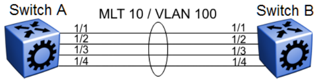
Figure 183: MLT within a VLAN
