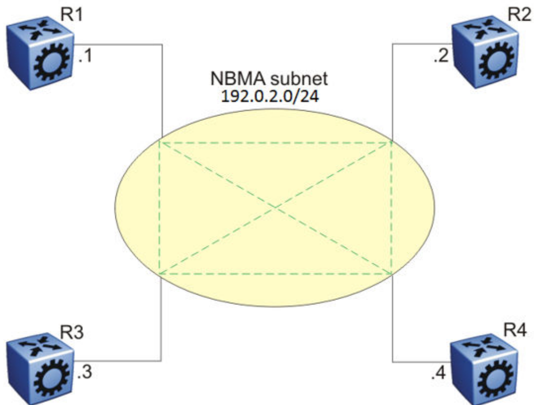
Figure 191: NBMA Subnet
