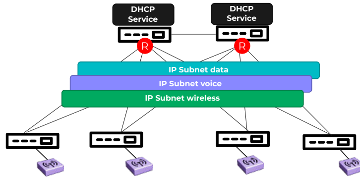
Figure 46: DHCP Server with a Single VRF - Small Campus Network
