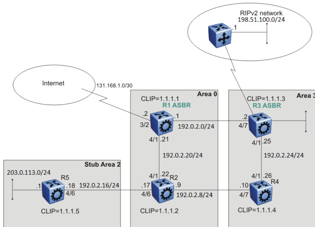
Figure 190: Multiarea configuration example
