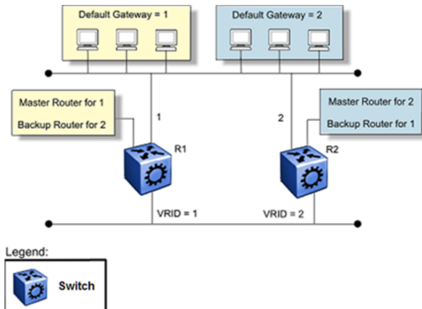
Figure 250: Virtual Router Redundancy Protocol configuration
