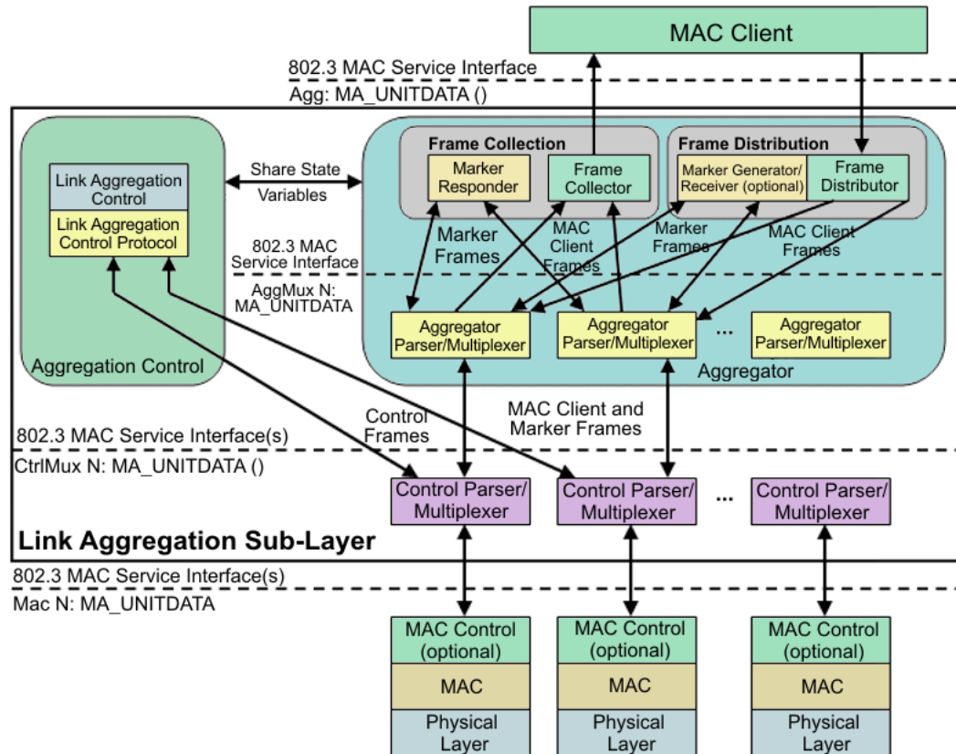
Figure 175: Link aggregation sublayer (according to IEEE 802.3ad)
