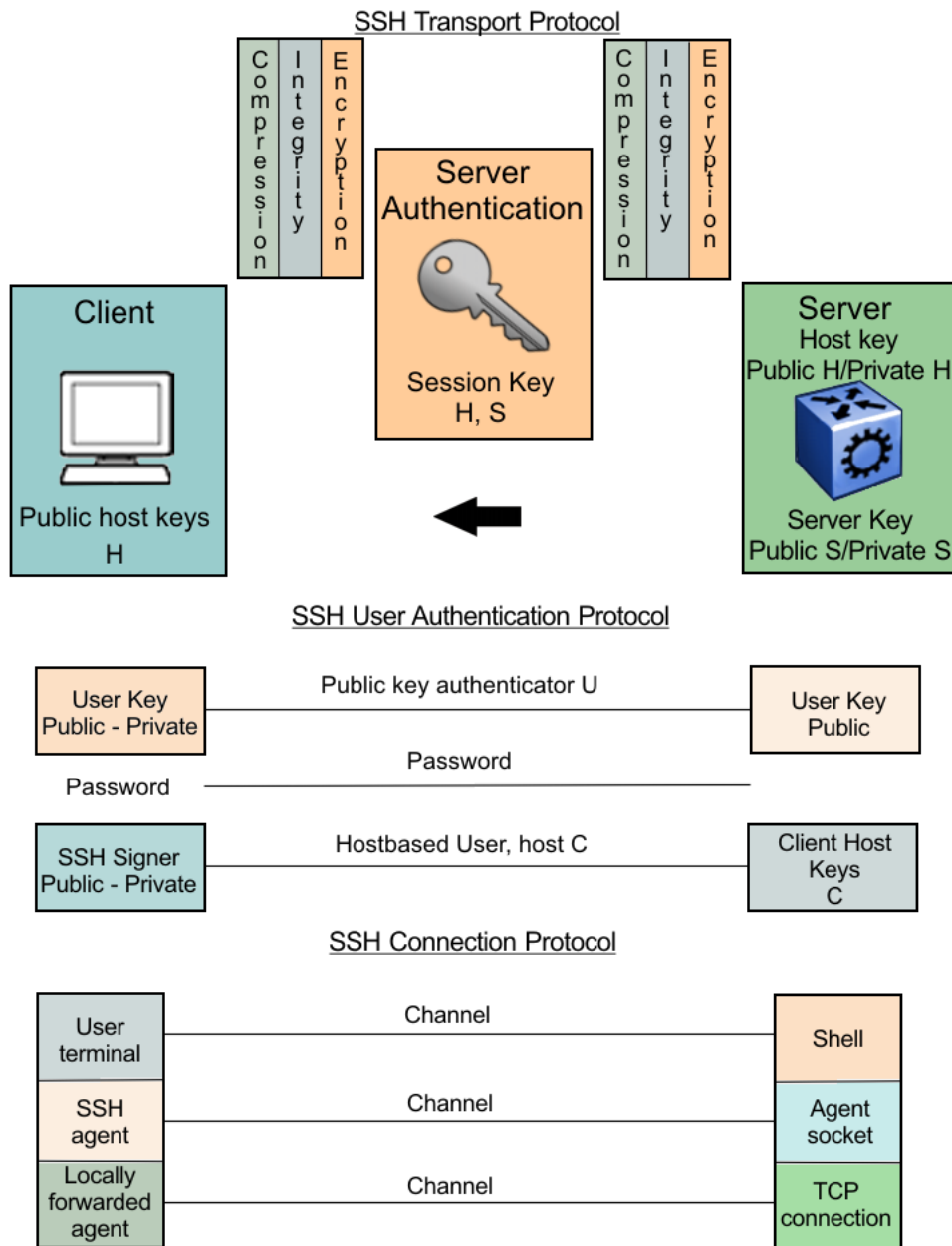
Figure 218: Separate SSH version 2 protocols
