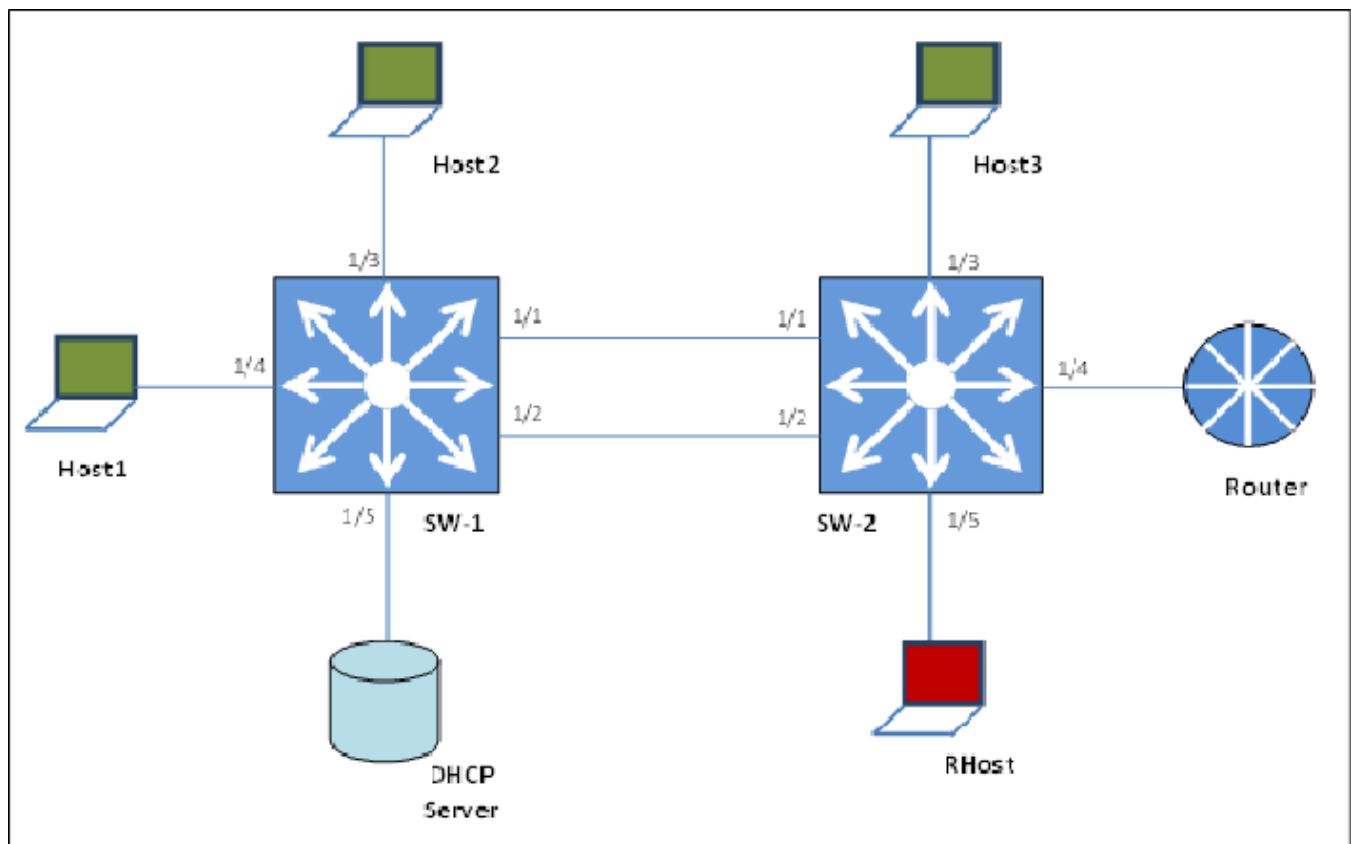
Figure 174: FHS deployment topology
