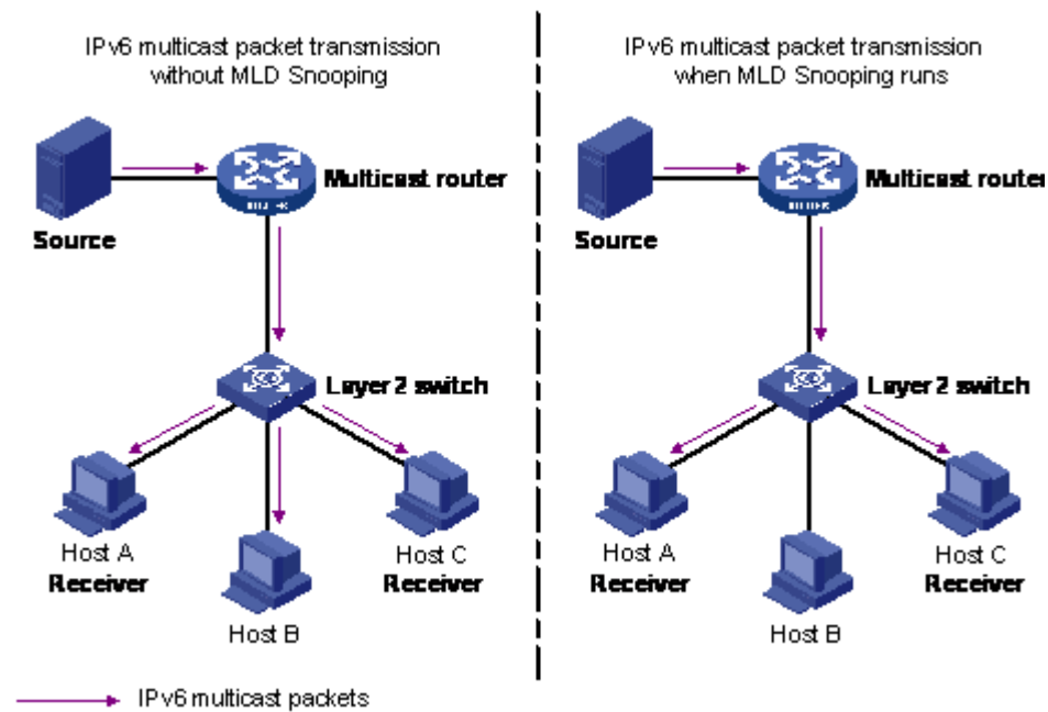
Figure 139: IPv6 multicast packet transmission when MLD snooping is enabled and not enabled
