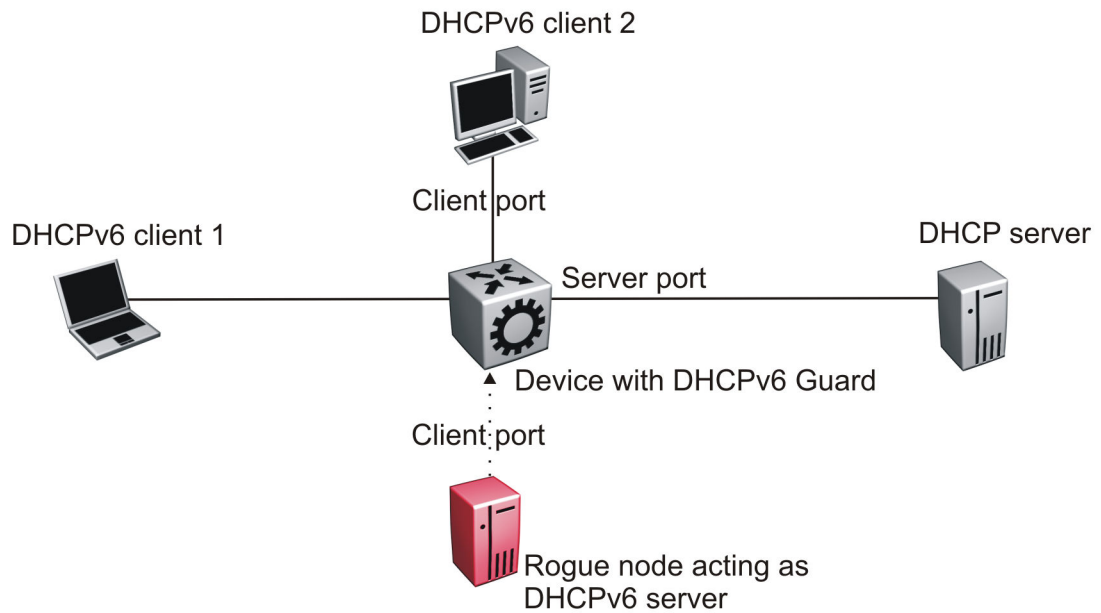
Figure 165: DHCPv6 Topology 1
