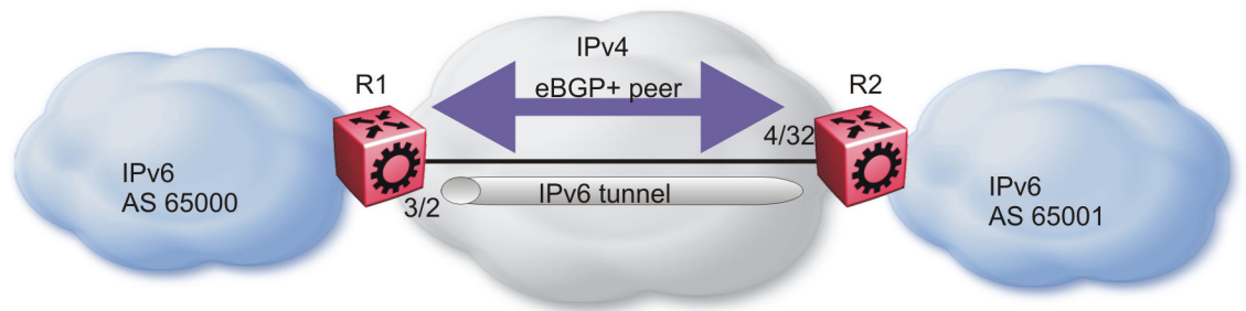
Figure 43: eBGP+ peers with IPv6 tunneling
