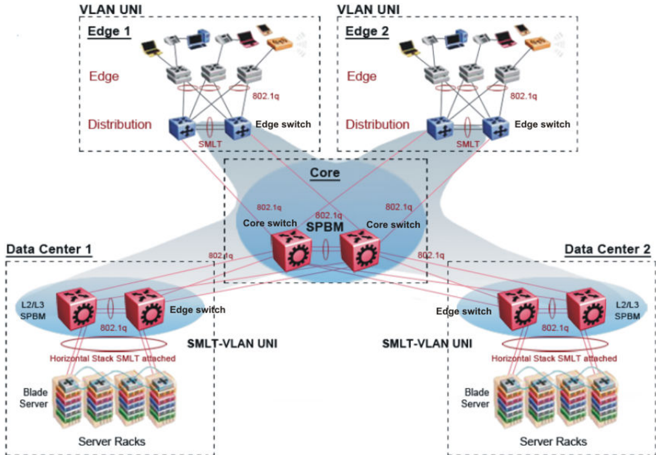
Figure 102: SPBM campus without SMLT
