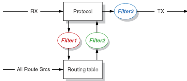
Figure 214: Route filtering stages
