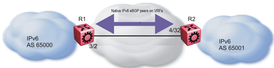
Figure 45: Native IPv6 eBGP peers on VRFs
