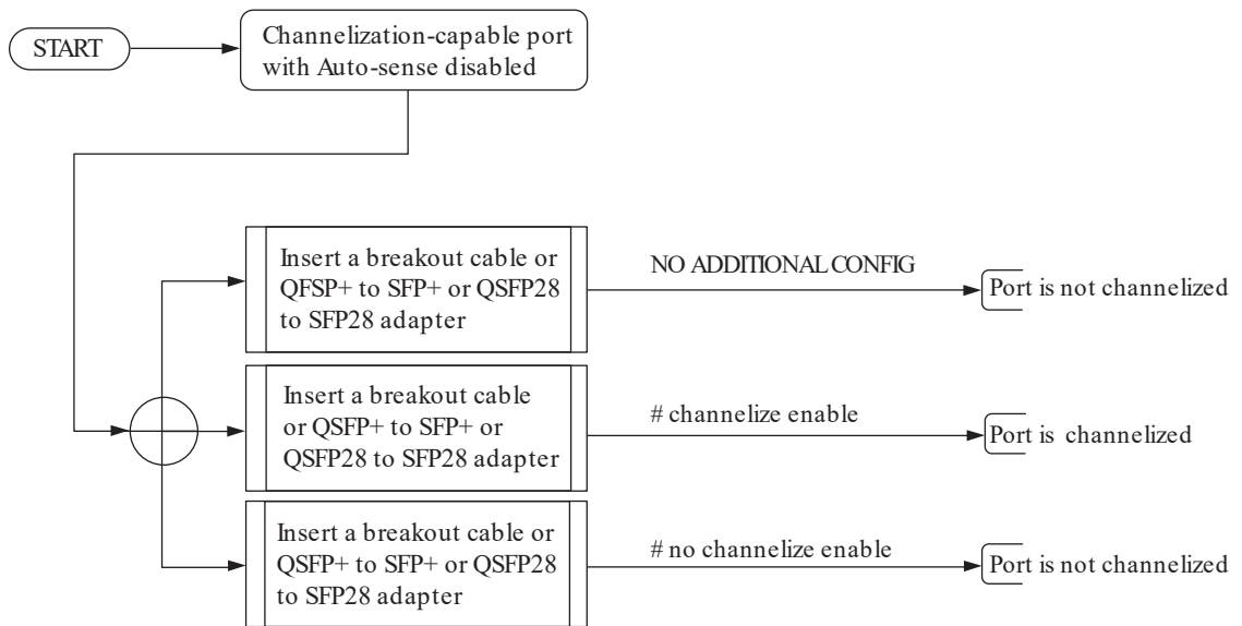
Figure 11: Automatic Channelization with Auto-sense disabled
