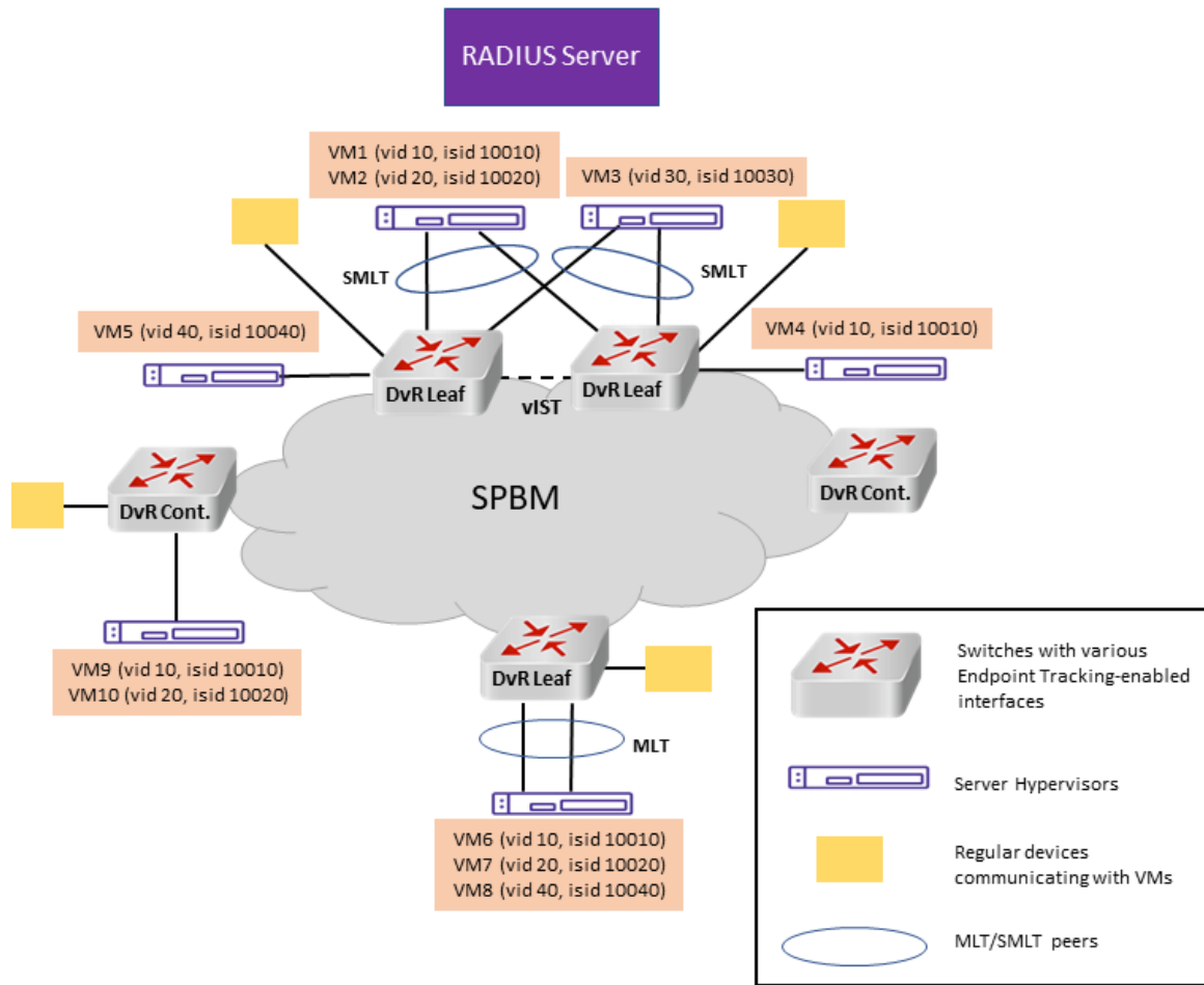
Figure 84: DvR Topology Example
