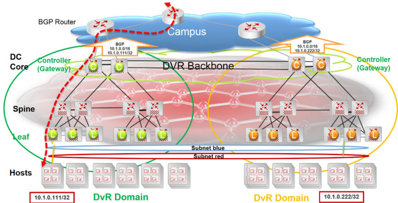
Figure 54: Traffic flow optimized with route redistribution
