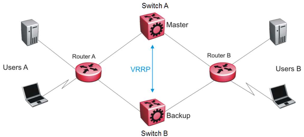
Figure 253: VRRP network topology
