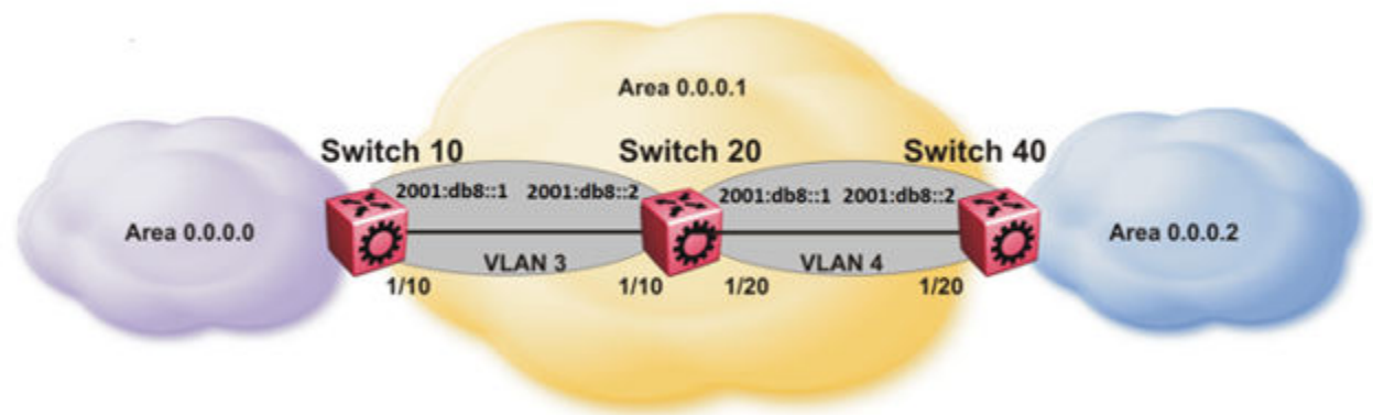
Figure 149: OSPFv3 virtual link with IPsec configuration
