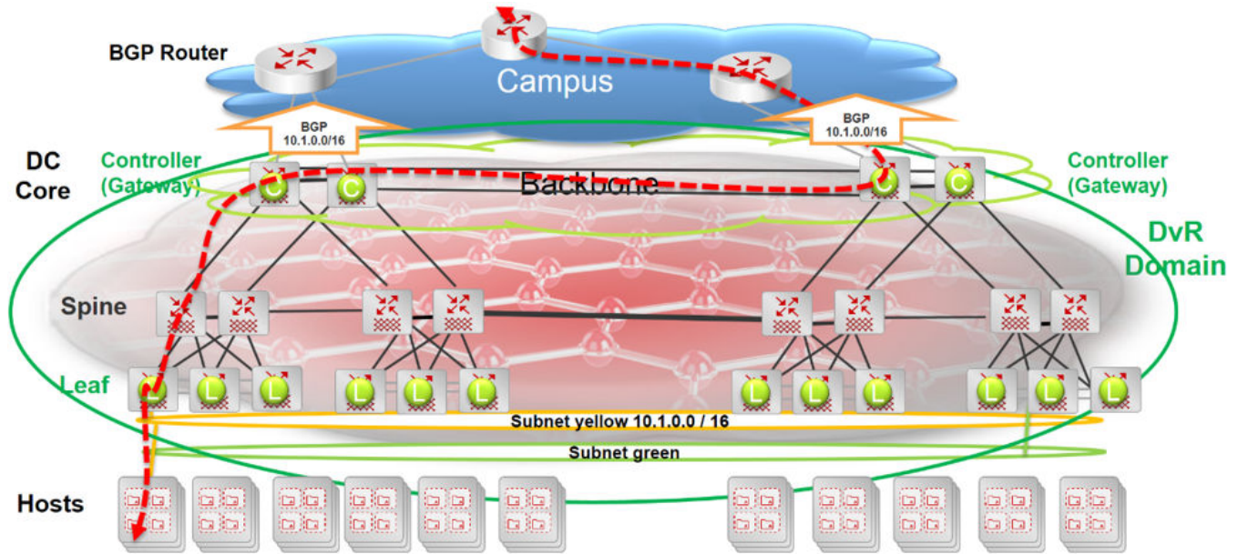
Figure 53: Inefficient traffic flow
