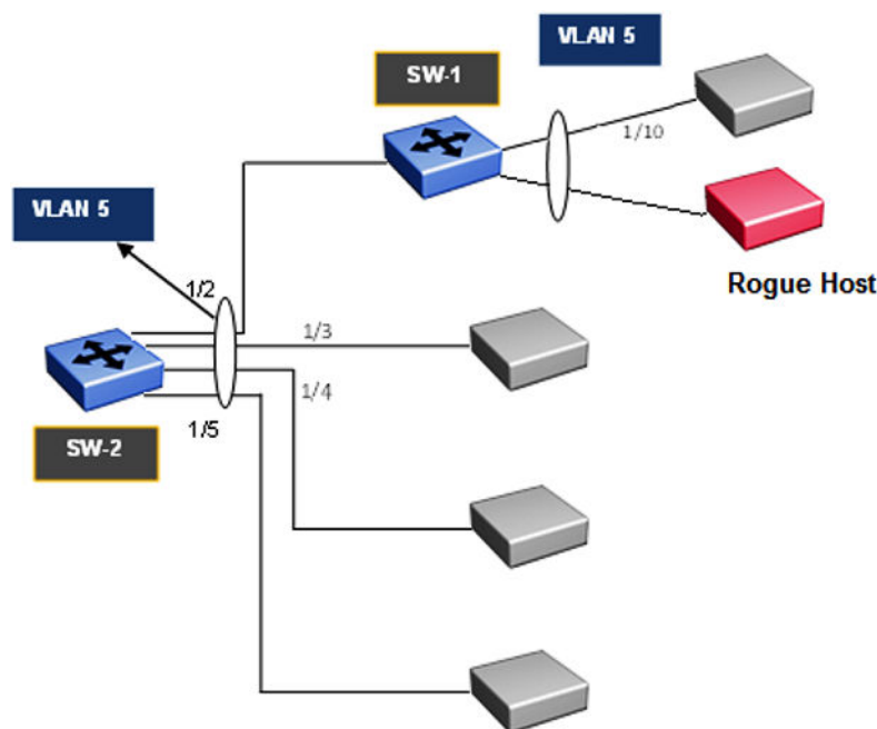
Figure 164: First Hop Security topology
