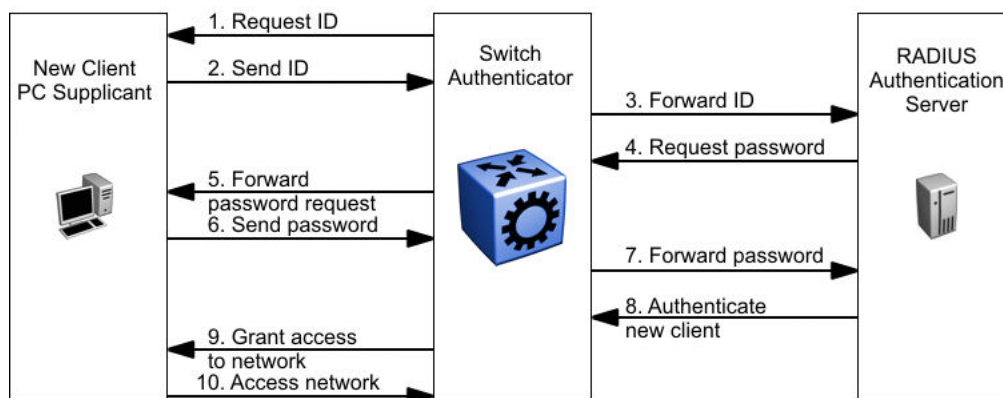
Figure 57: EAP configuration example
