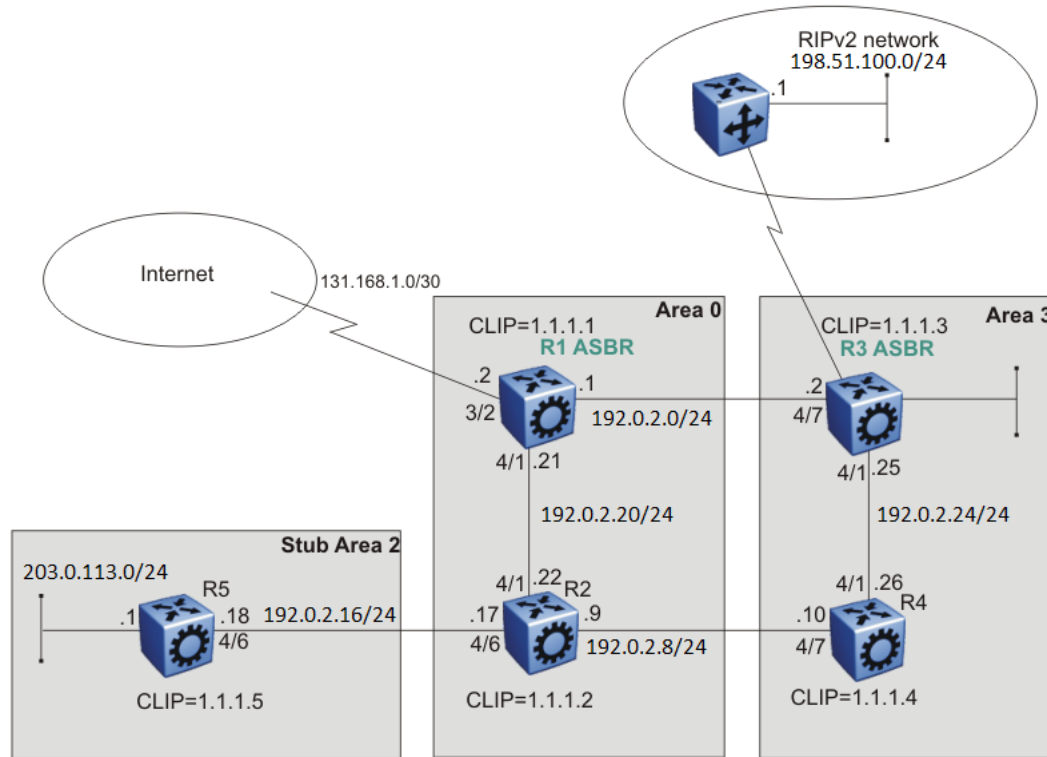
Figure 194: Multiarea configuration example
