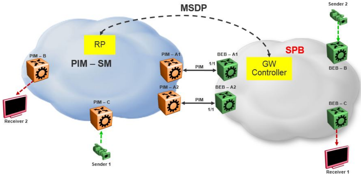
Figure 230: SPB-PIM Gateway base case configuration
