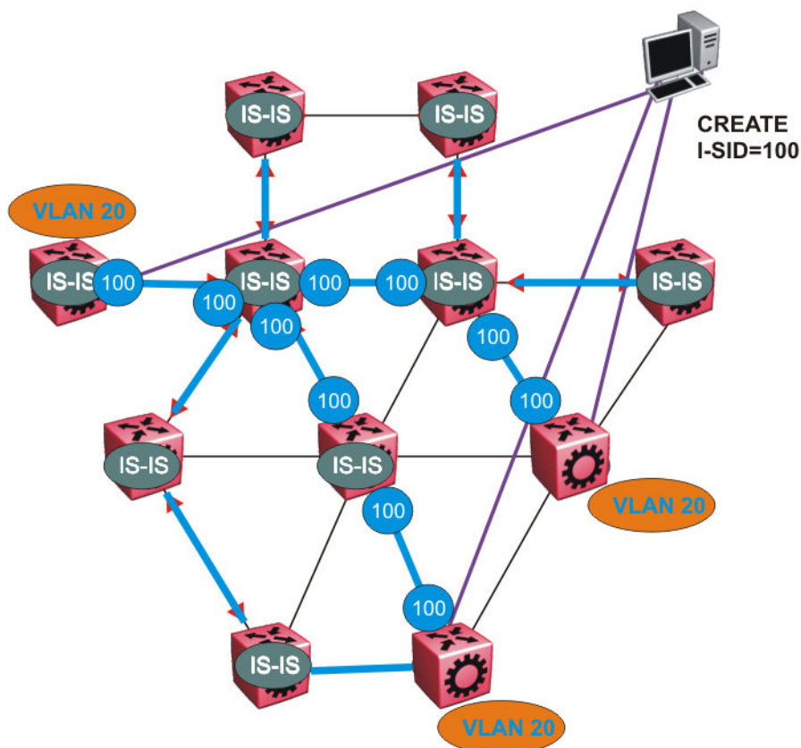
Figure 96: SPBM BMAC and I-SID population
