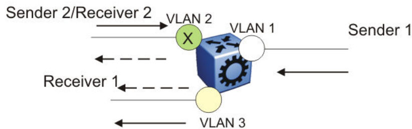
Figure 130: Data flow using deny-both policy
