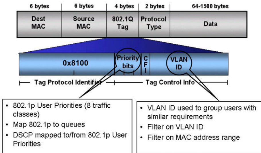
Figure 247: VLAN tag insertion
