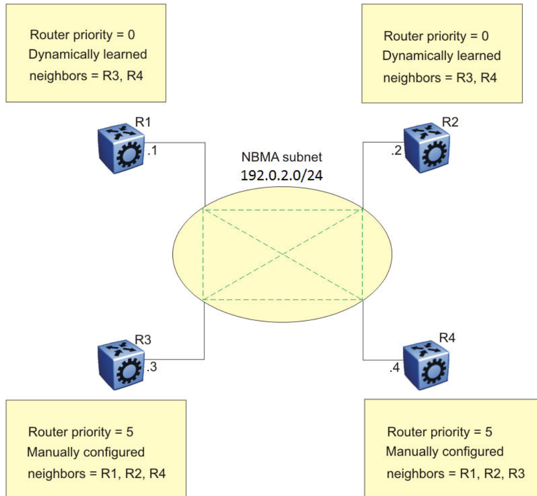
Figure 196: NBMA Subnet Configuration Example
