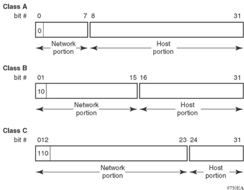
Figure 154: Network and host boundaries in IP address classes
