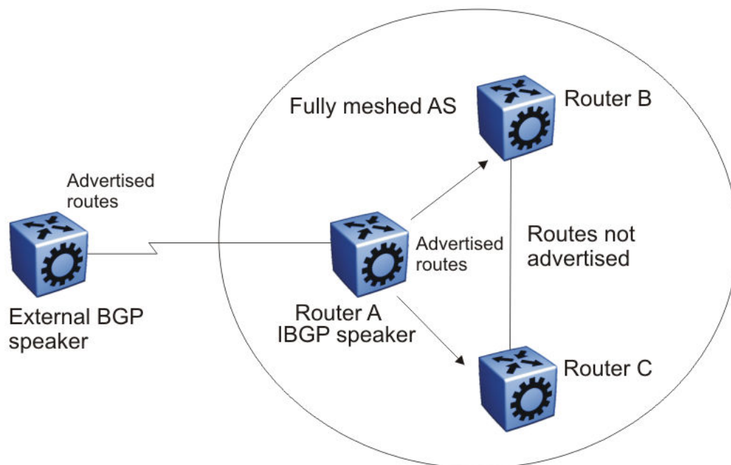
Figure 29: Fully meshed AS with iBGP speakers
