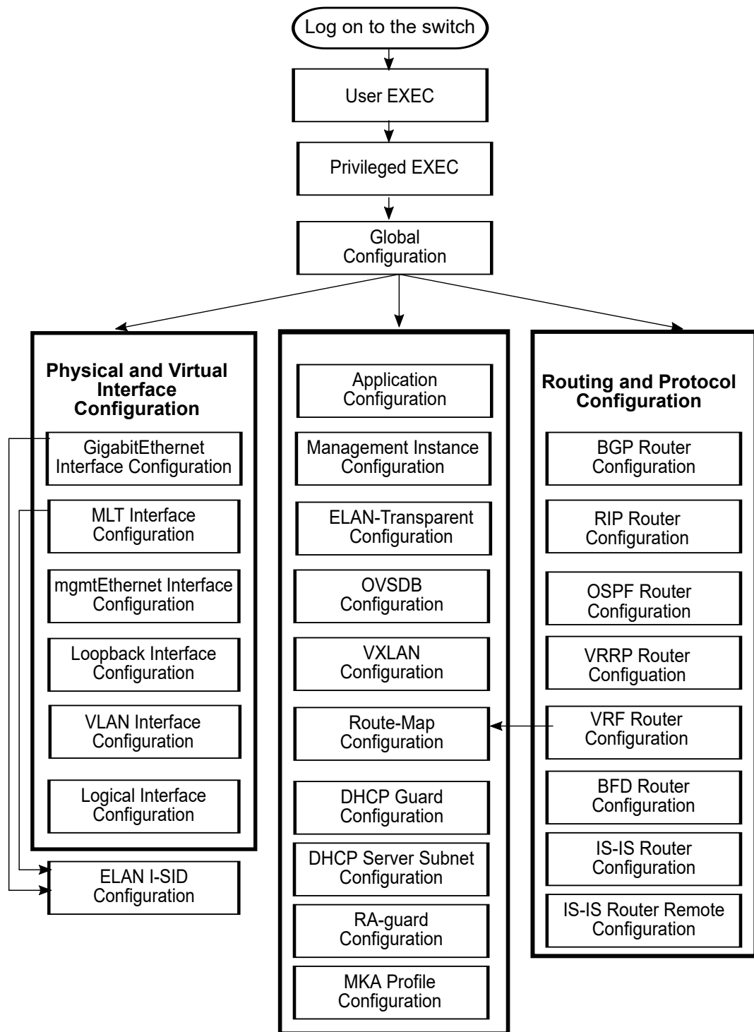
Figure 14: CLI Command Mode Navigation
