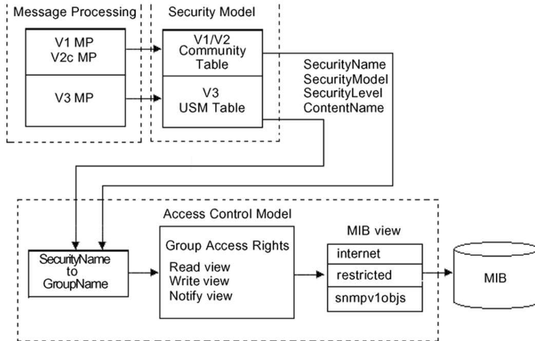
Figure 224: USM association with VACM
