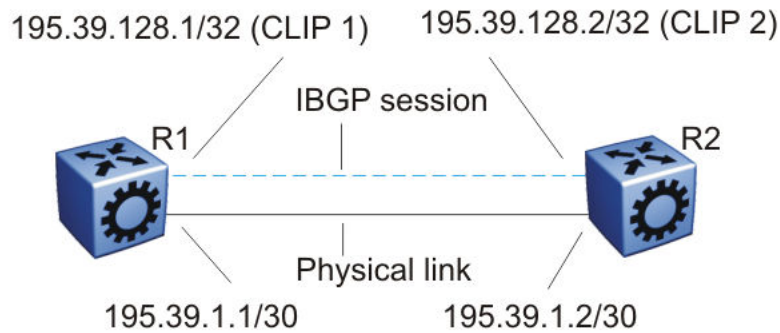
Figure 36: Routers with iBGP connections
