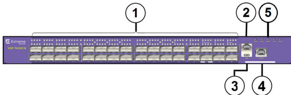
Figure 262: VSP 7432CQ
