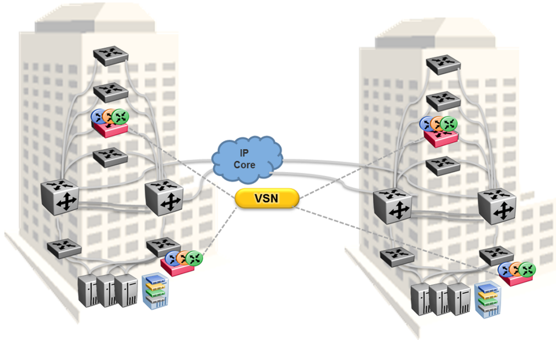
Figure 74: Fabric Extend Full Mesh Campus Deployment Option
