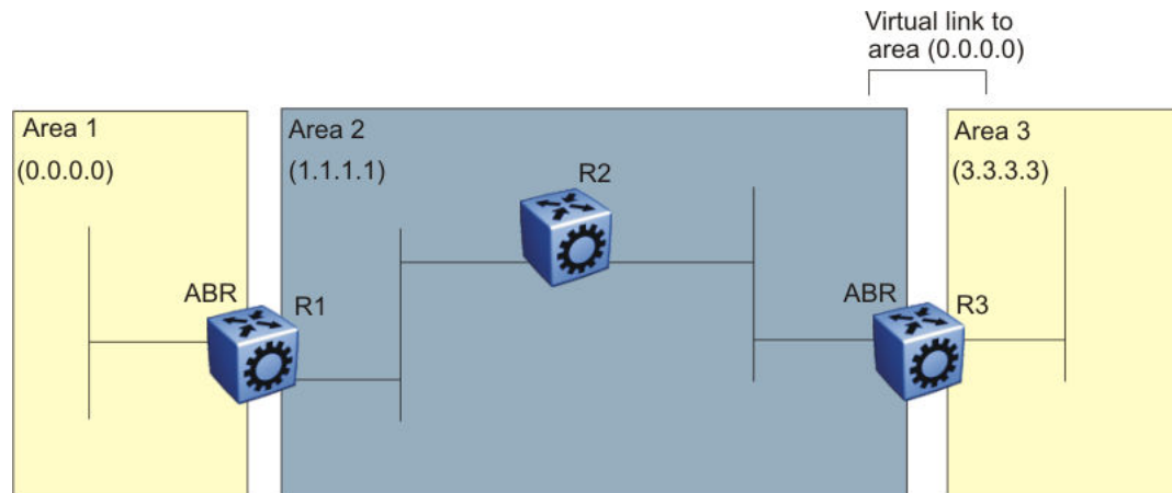
Figure 197: Virtual link between ABRs through a transit area
