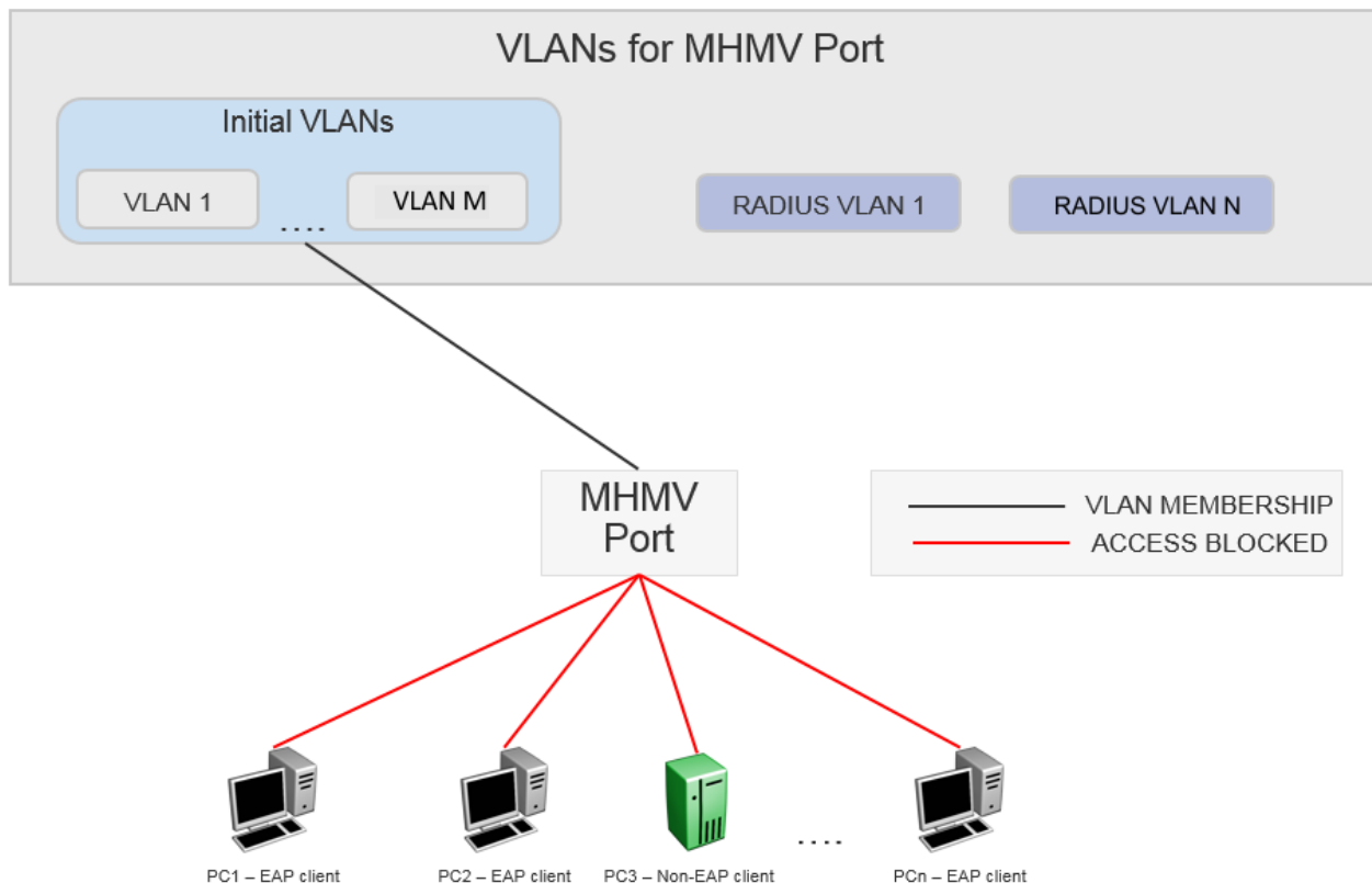
Figure 60: MHMV - clients not authenticated
