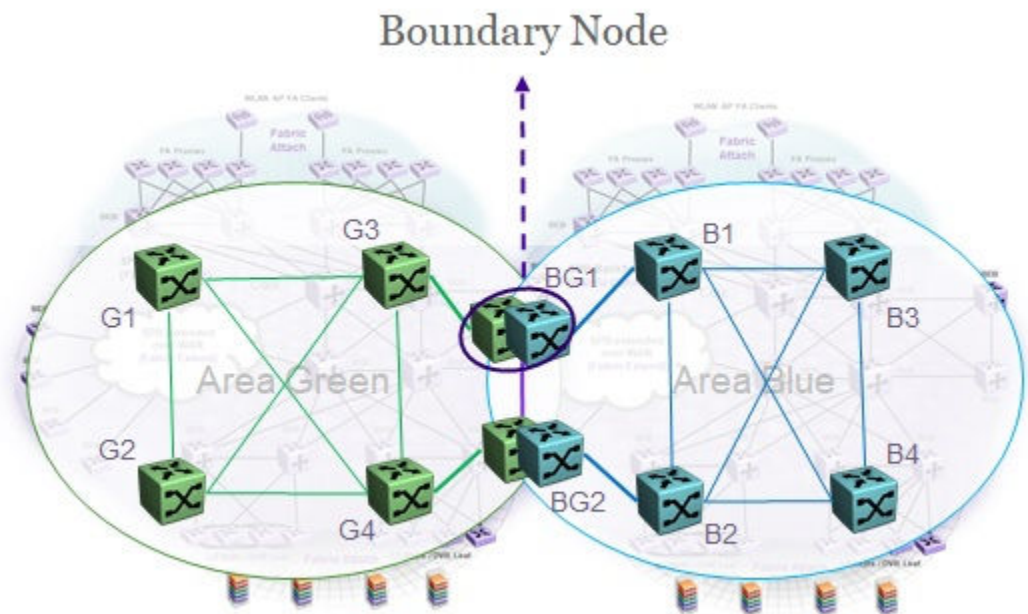
Figure 90: Boundary nodes in the Multi-area SPB network
