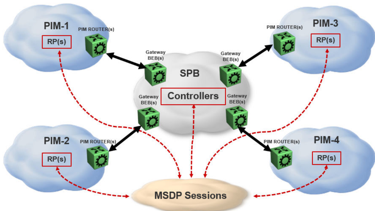
Figure 228: Multicast over Fabric Connect with SPB-PIM GW
