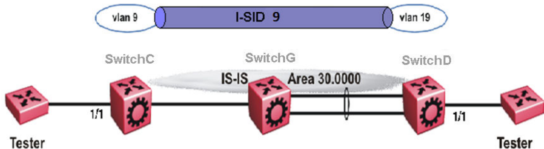
Figure 101: Layer 2 VSN with different VLAN IDs
