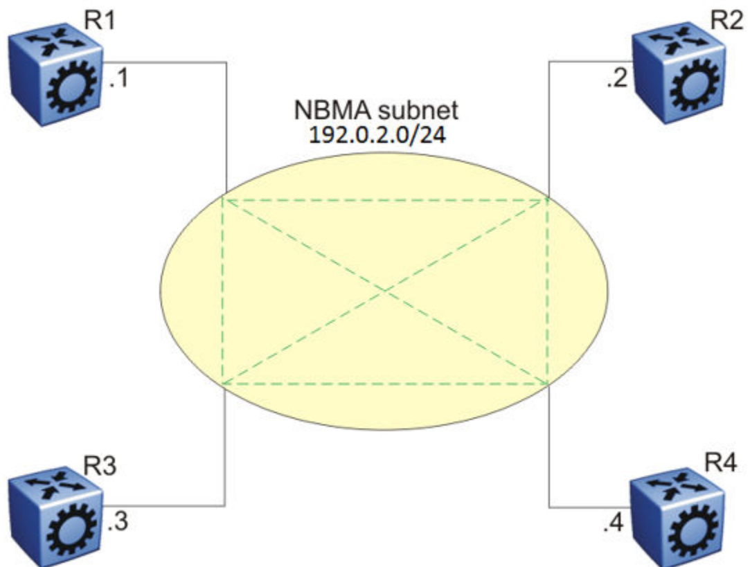
Figure 195: NBMA Subnet
