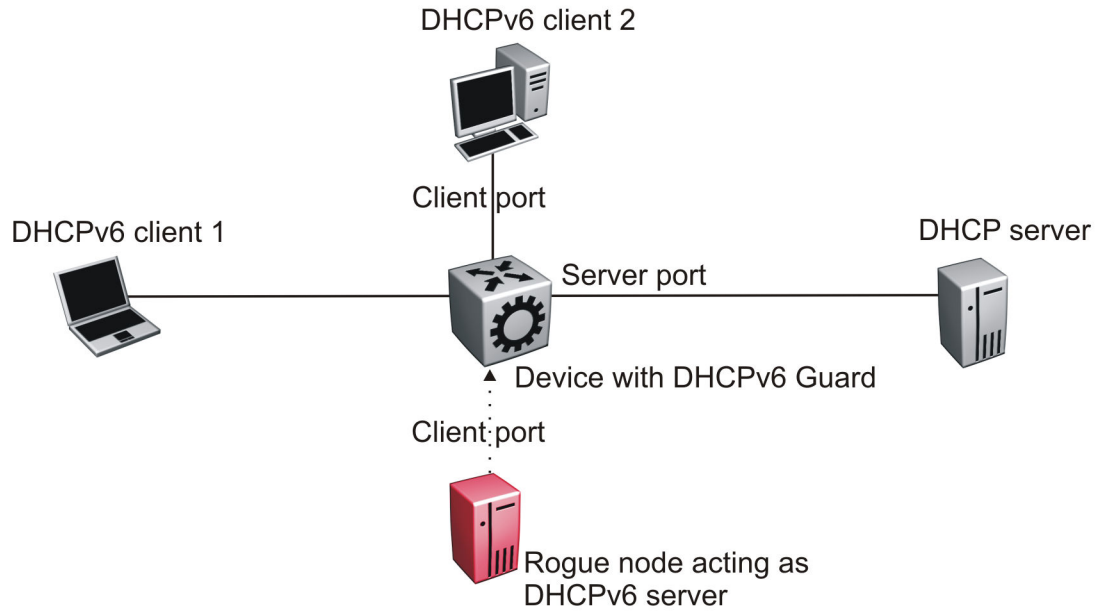
Figure 169: DHCPv6 Topology 1
