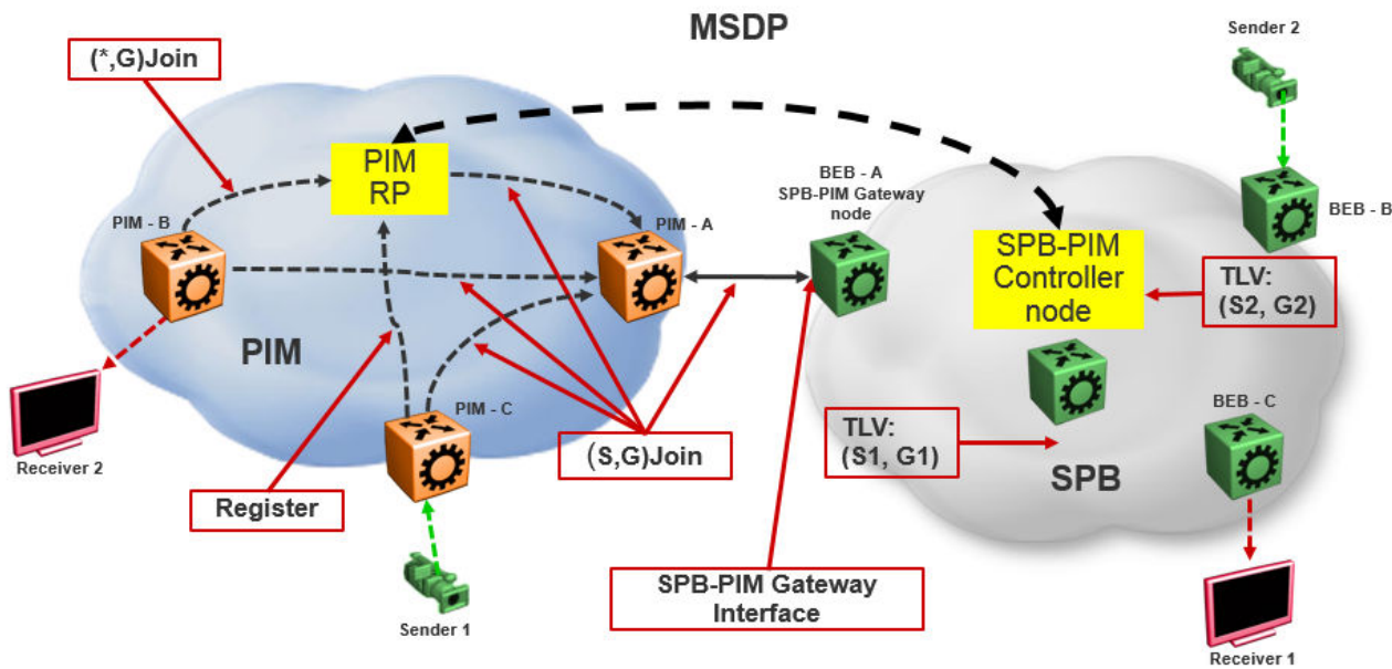
Figure 229: SPB-PIM GW components
