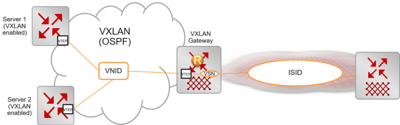
Figure 260: VXLAN-to-SPB deployment
