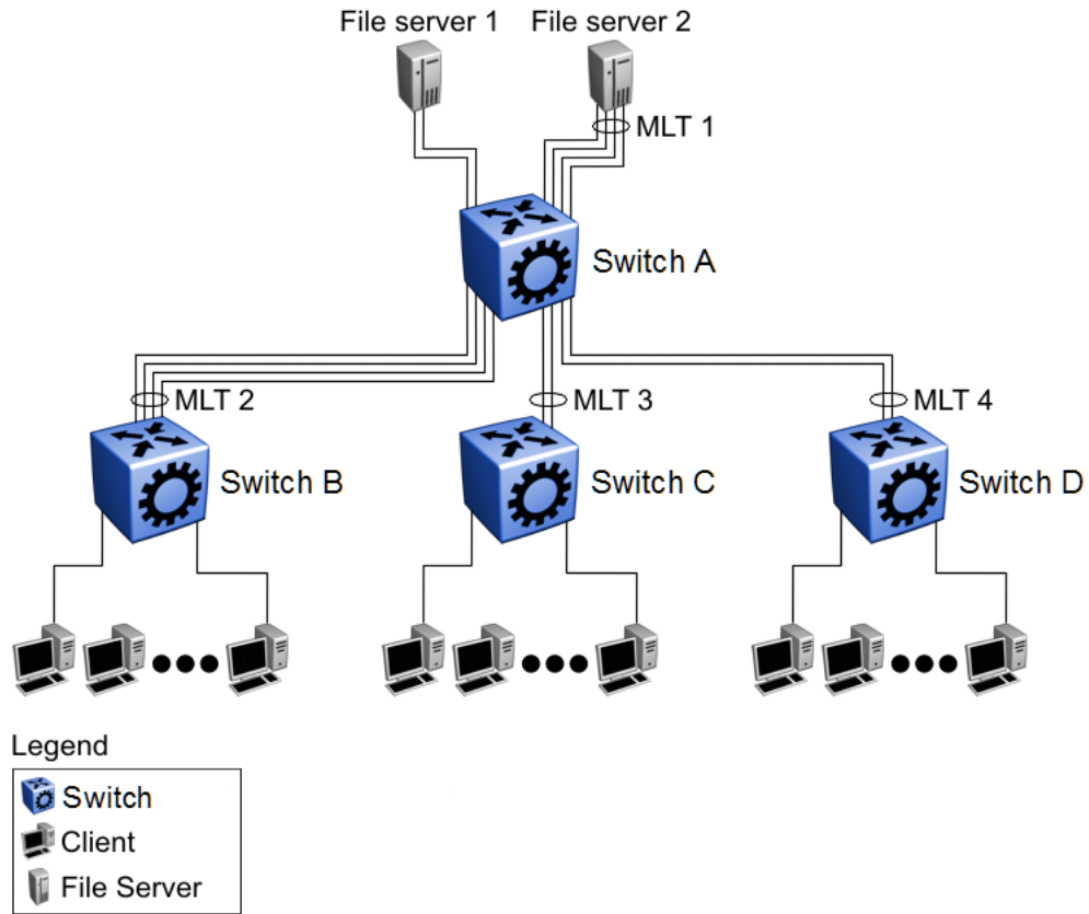
Figure 191: Client/server multilink trunk configuration
