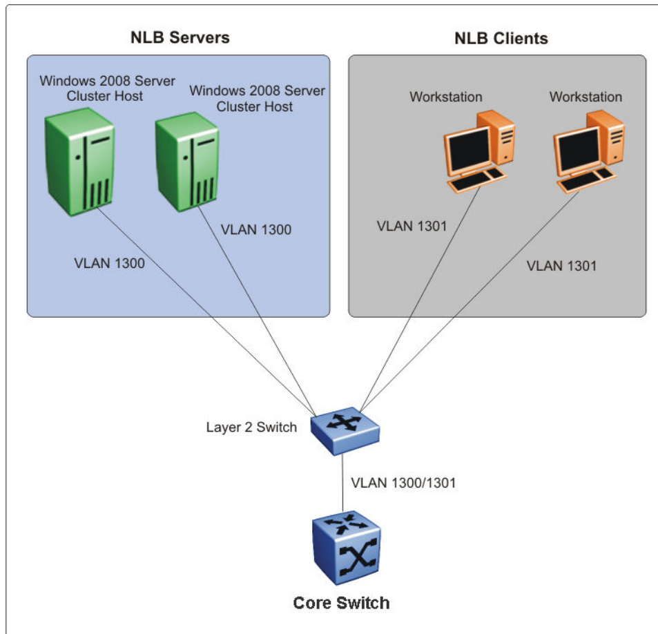
Figure 250: Supported NLB topology–example 2
