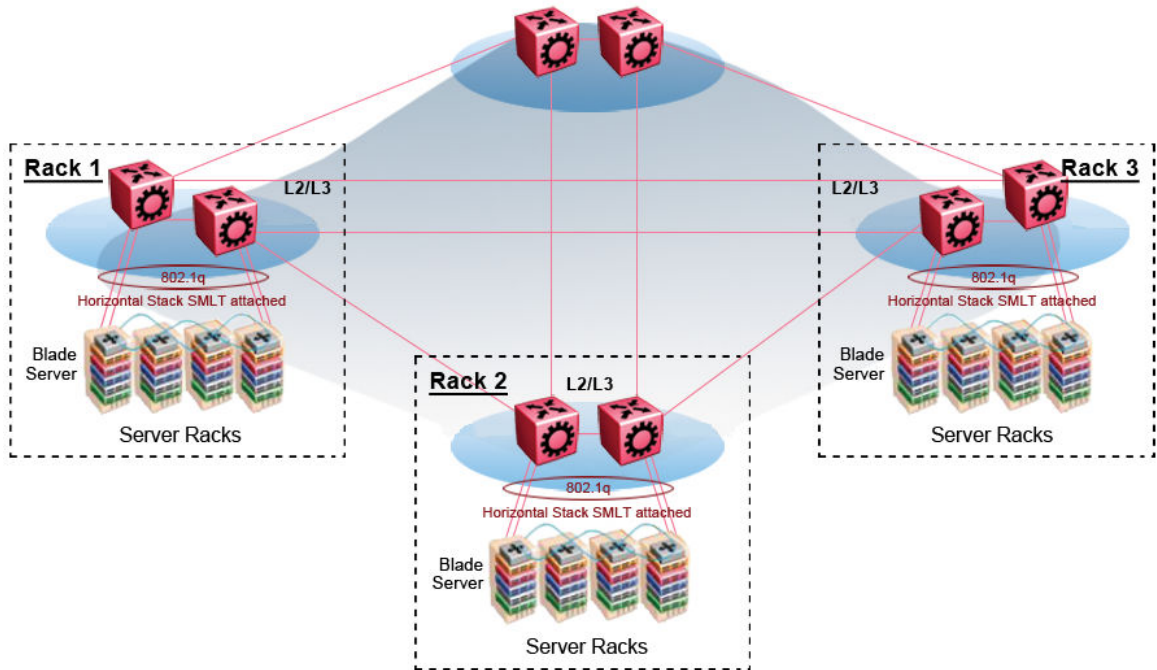
Figure 63: SPBM ring topology with shared data centers
