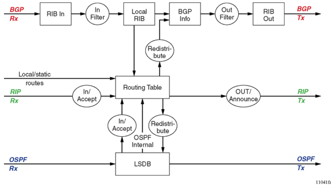
Figure 216: Route filtering for BGP, RIP, and OSPF routing protocols
