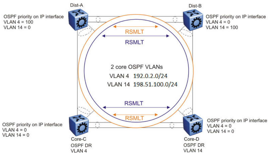
Figure 198: RSMLT with dual core VLANs
