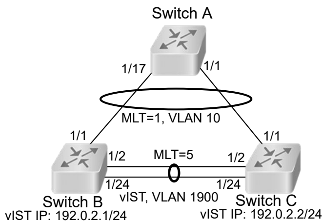
Figure 185: Network topology for traffic flow example
