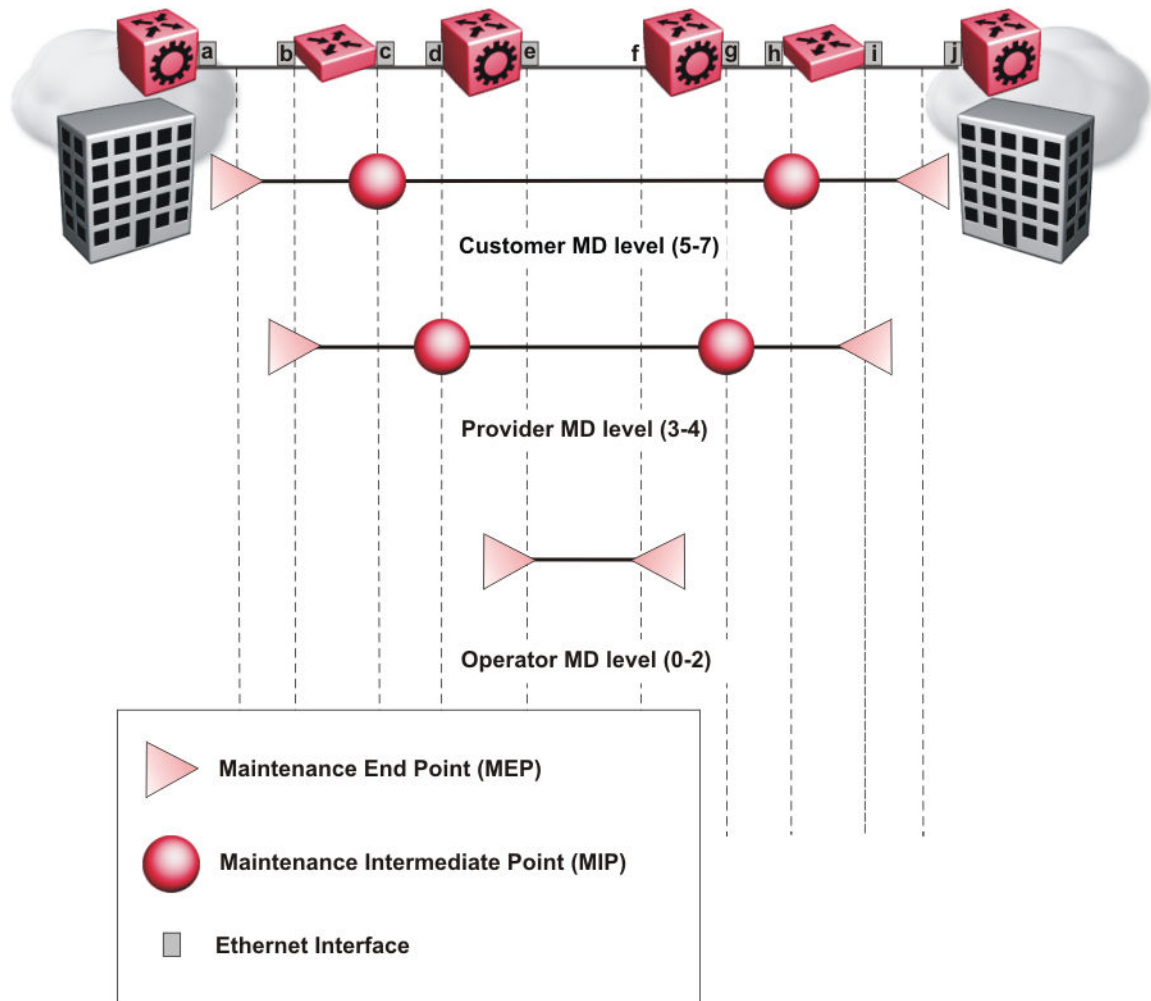
Figure 242: MD level assignment
