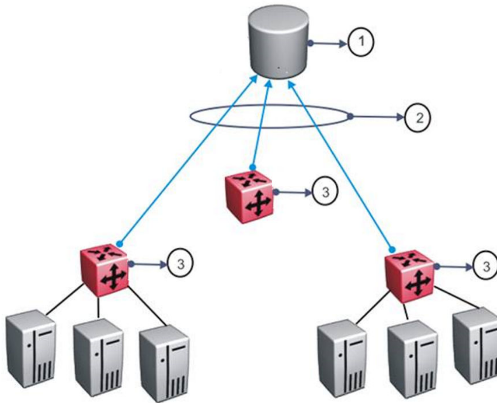
Figure 20: Application Telemetry Overview
