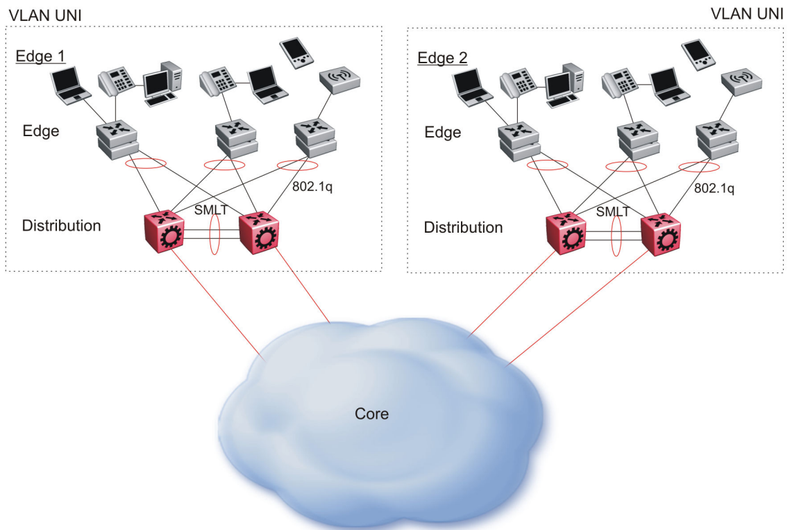
Figure 105: Access to the SPBM Core
