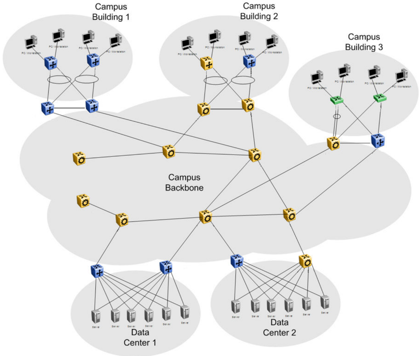
Figure 115: SPBM IP shortcuts in a campus
