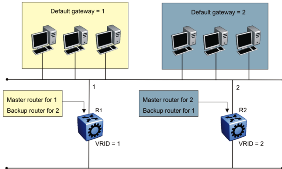
Figure 255: VRRP network configuration
