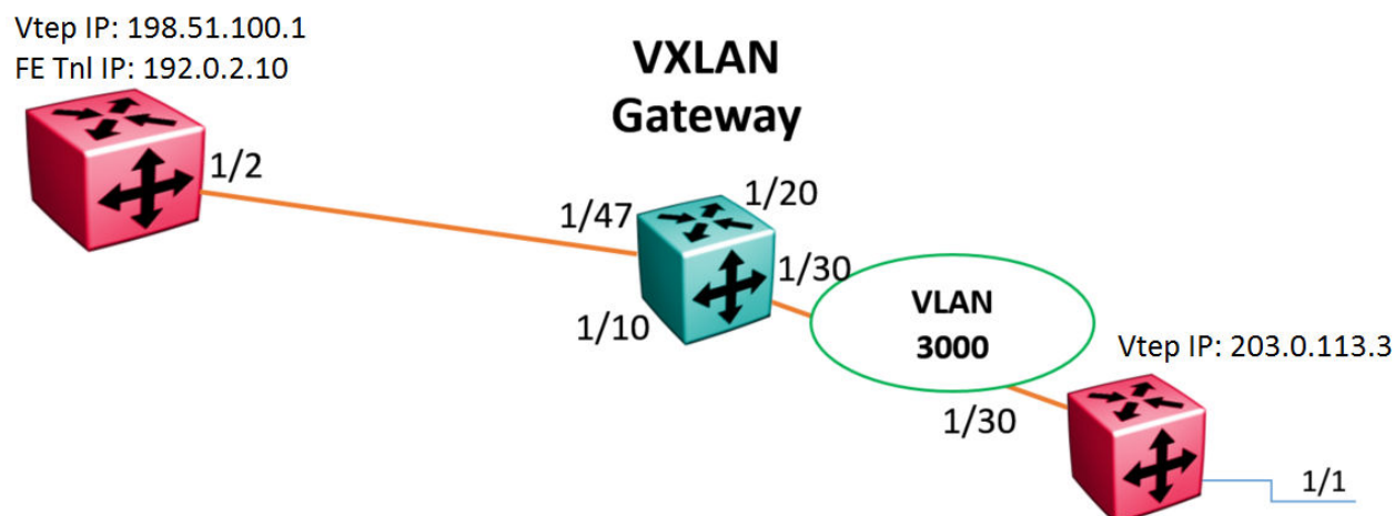
Figure 261: VXLAN Gateway configuration example
