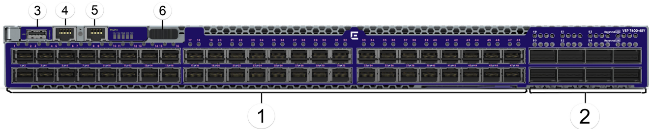
Figure 263: VSP 7400-48Y
