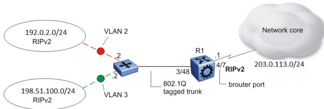
Figure 212: Configuration example-RIPv2 only
