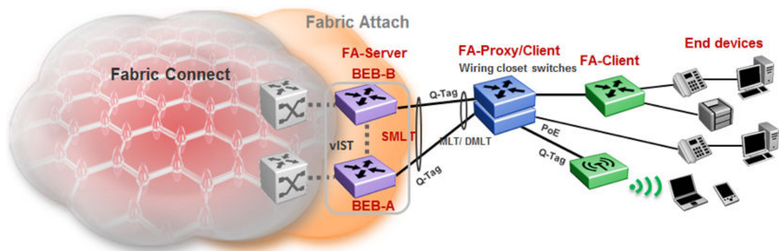
Figure 81: FA in a dual-homed SMLT deployment
