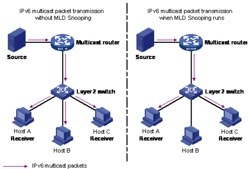
Figure 143: IPv6 multicast packet transmission when MLD snooping is enabled and not enabled
