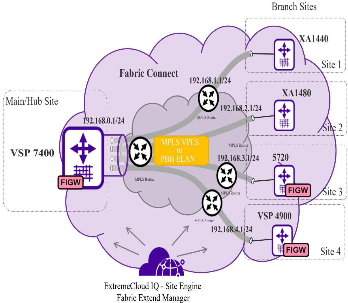
Figure 73: Fabric Extend VPLS Deployment Option
