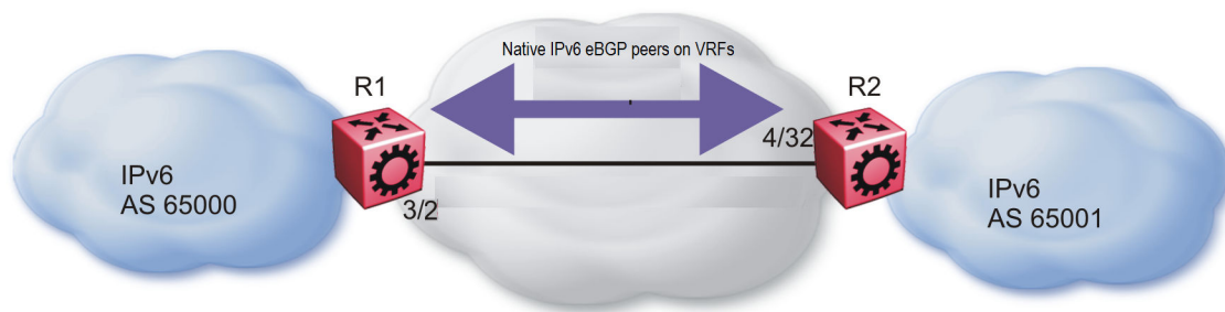
Figure 46: Native IPv6 eBGP peers on VRFs
