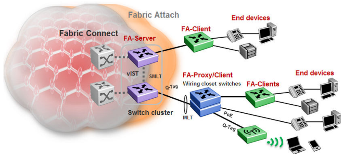
Figure 82: Fabric Attach in a single-homed SMLT deployment
