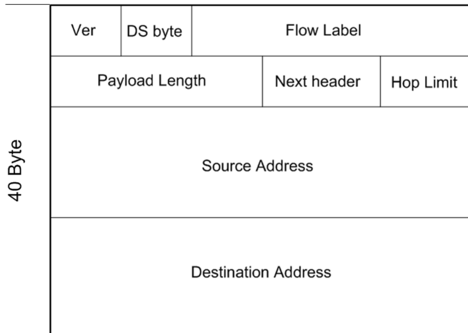
Figure 159: IPv6 header
