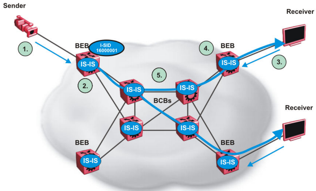
Figure 145: IP Multicast over Fabric Connect streams
