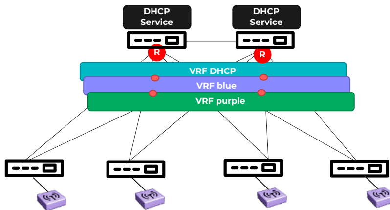
Figure 48: DHCP Server with Multiple VRF - Small Campus Network
