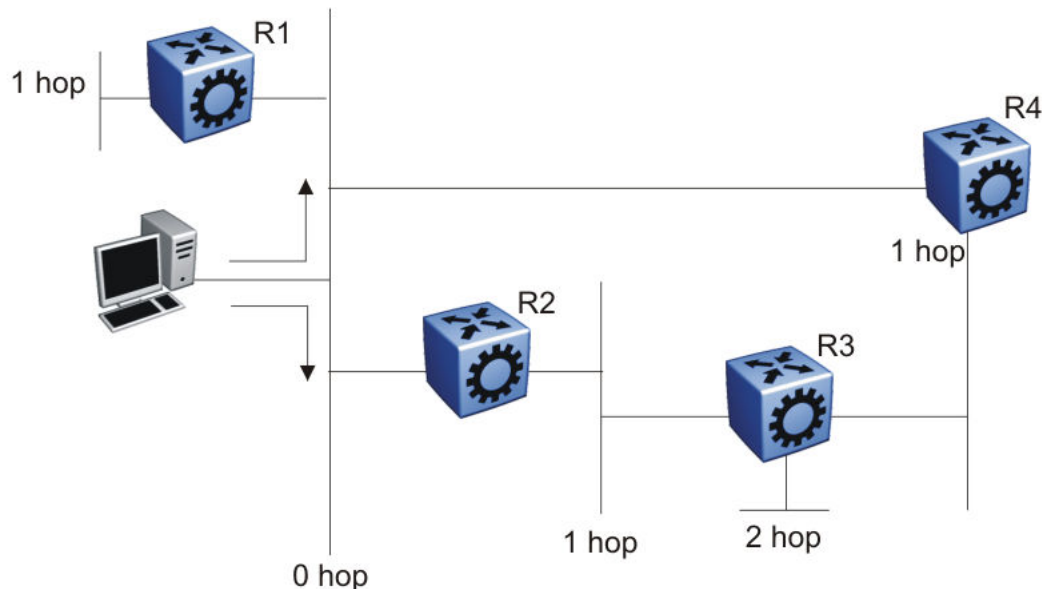
Figure 210: Hop count or metric in RIP
