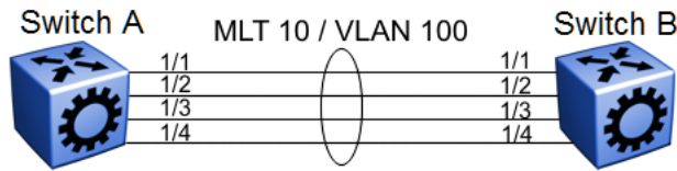
Figure 187: MLT within a VLAN
