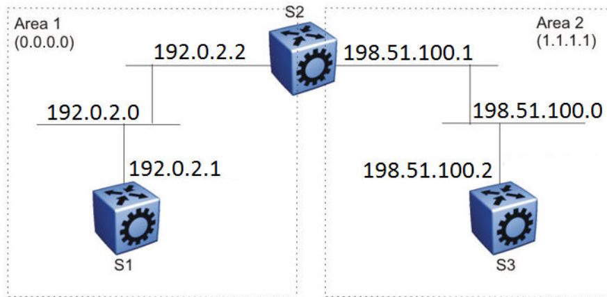
Figure 201: Example 3: OSPF on two subnets in two areas
