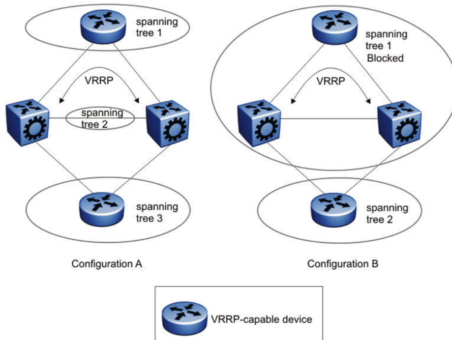
Figure 256: VRRP and STG configurations
