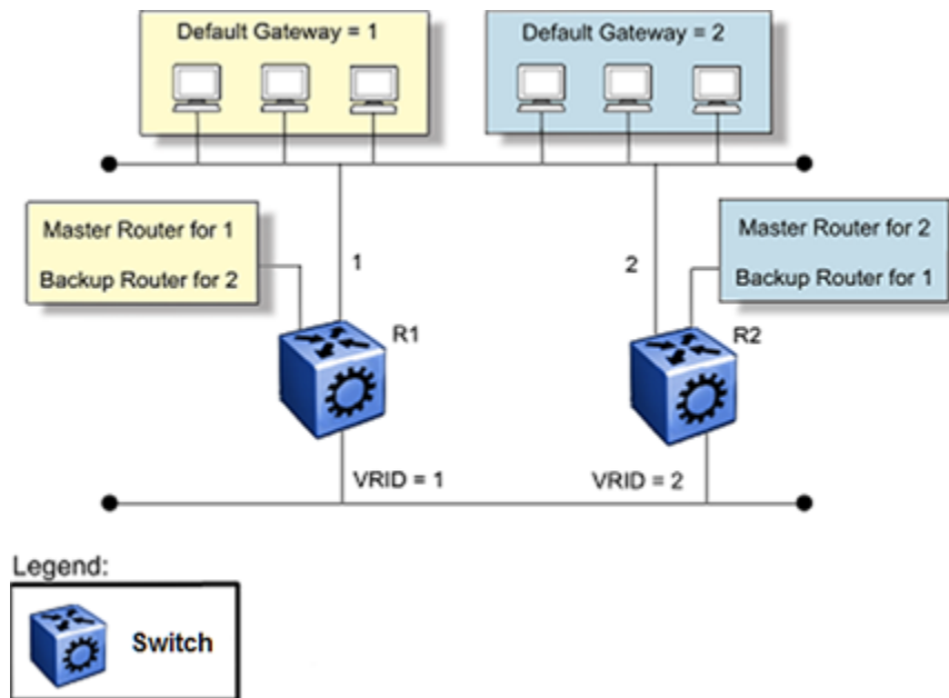
Figure 254: Virtual Router Redundancy Protocol configuration
