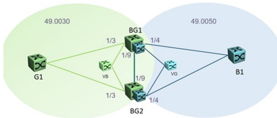
Figure 92: Multi-area SPB network example
