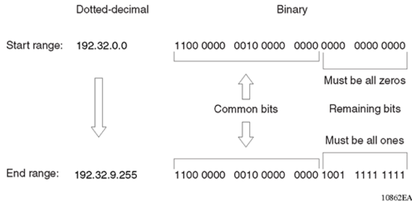
Figure 24: Binary notation conversion
