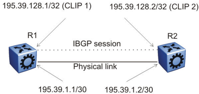
Figure 156: Routers with iBGP connections
