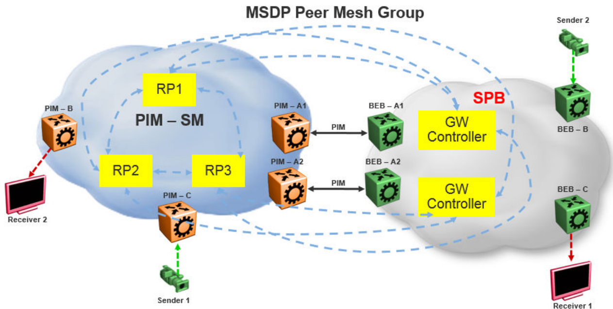
Figure 232: Peer Mesh Group
