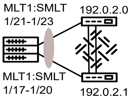
Figure 84: FA configuration in dual-homed SMLT
