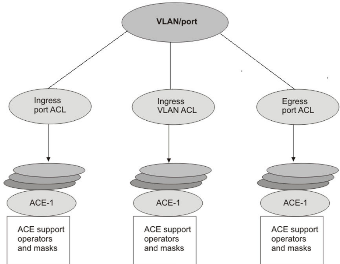
Figure 241: ACE and ACL relationships
