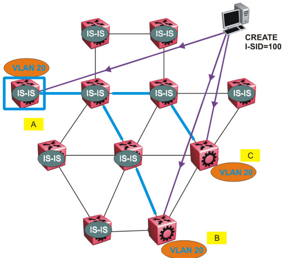
Figure 97: Shortest path tree for source node A
