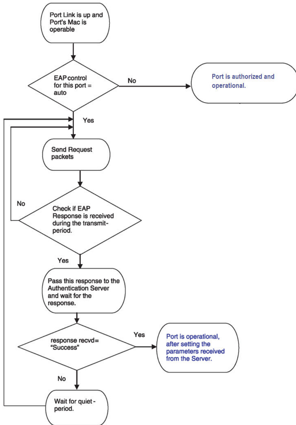
Figure 59: EAP flow diagram
