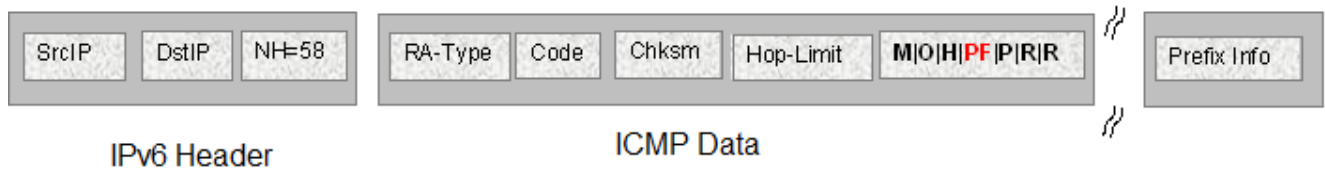
Figure 177: IPv6 ICMP RA data packet outline for router preference validation
