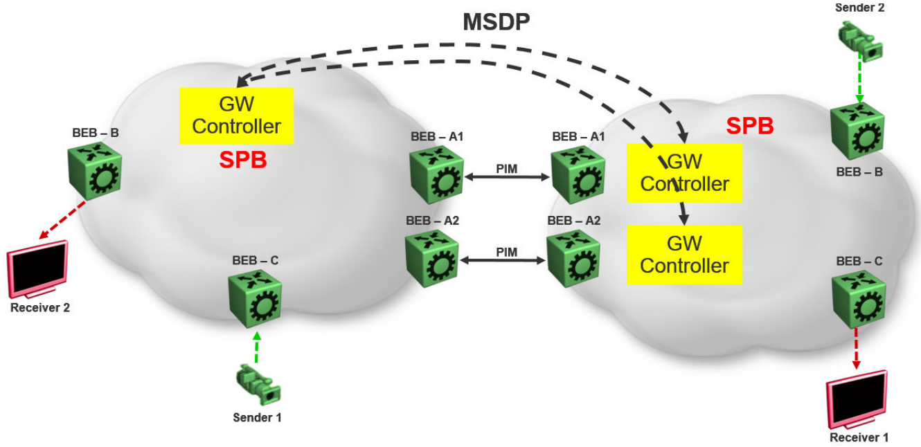
Figure 234: SPB domain interconnect
