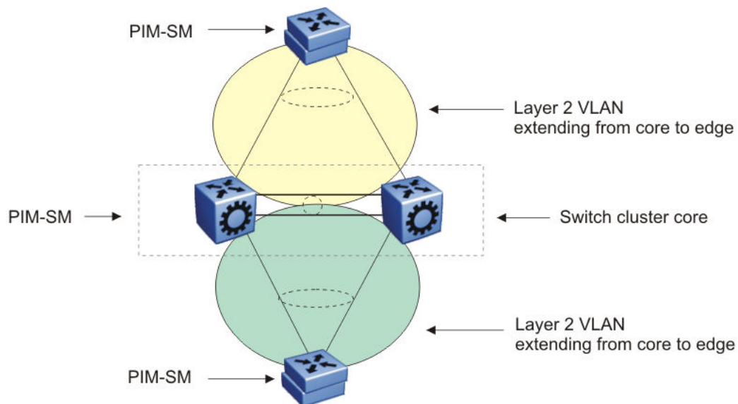
Figure 138: Multicast SMLT triangle
