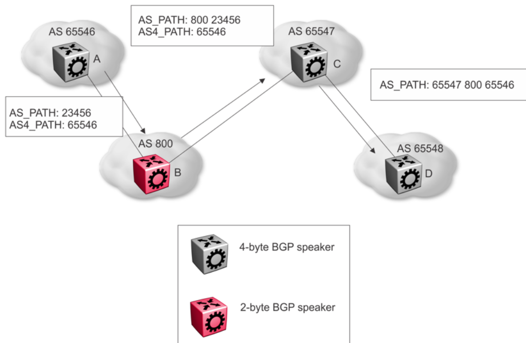
Figure 23: 2-byte and 4-byte Mixed Environment
