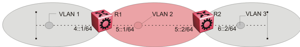
Figure 165: IPv6 routing between VLANs
