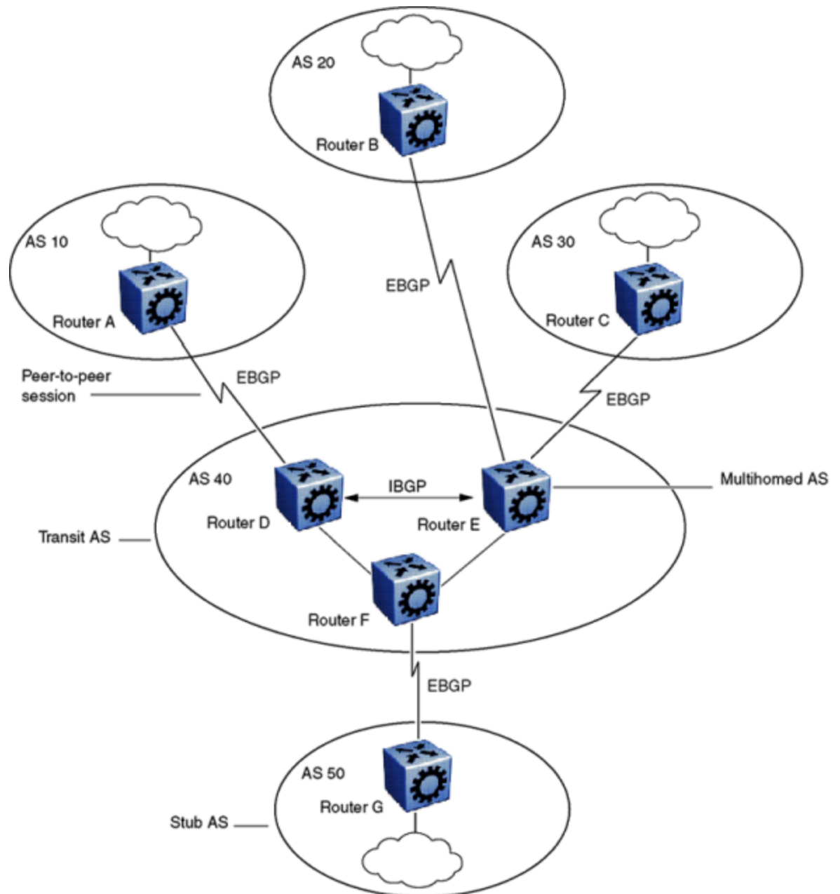
Figure 22: BGP networks
