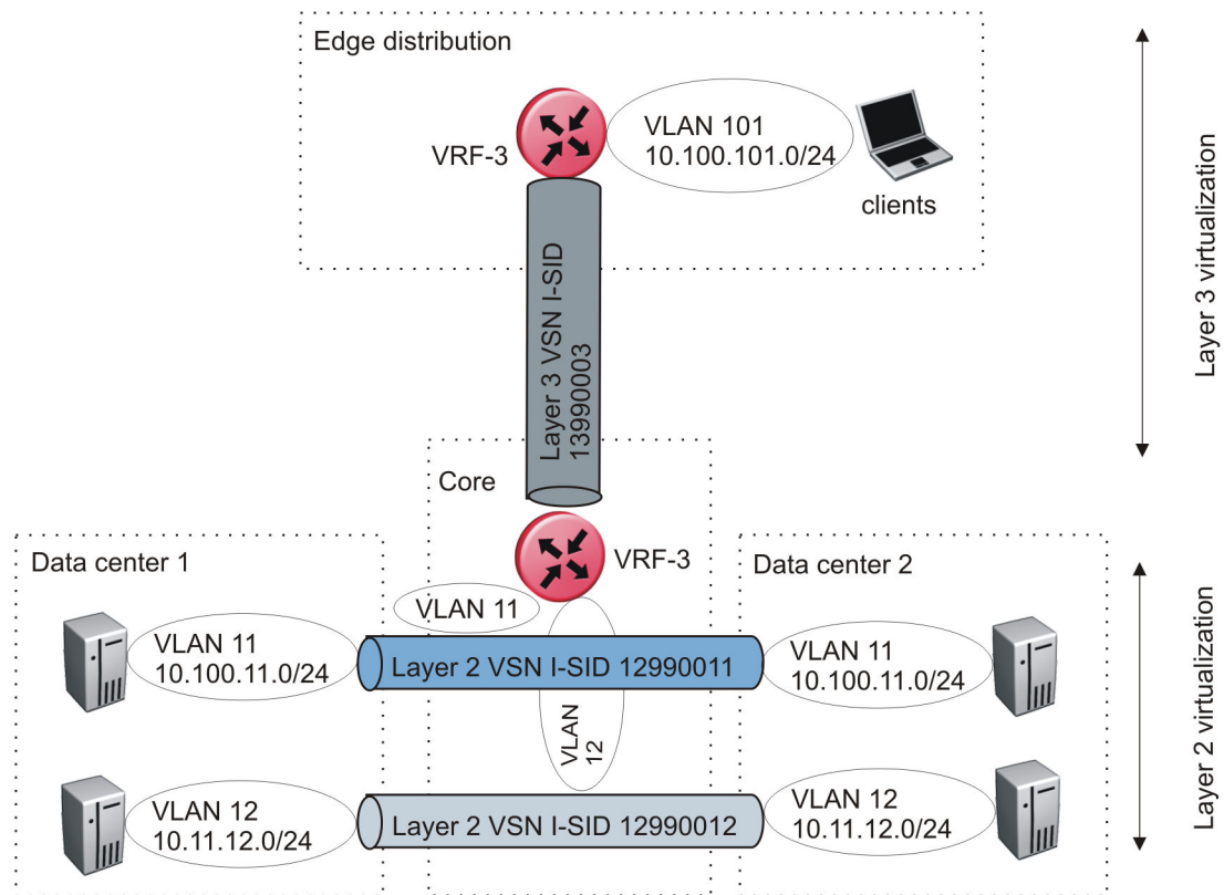
Figure 108: VRF scenario to move traffic between data centers
