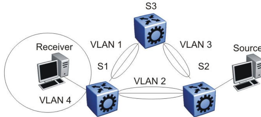
Figure 134: IP multicast sources and receivers on interconnected VLANs
