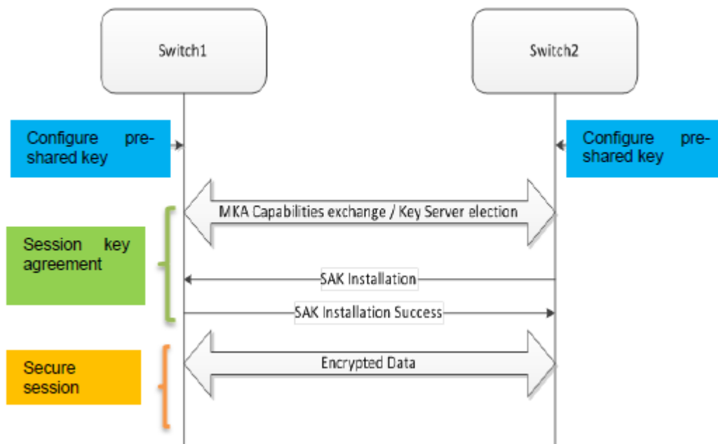
Figure 182: Switch to switch MACsec deployment scenario
