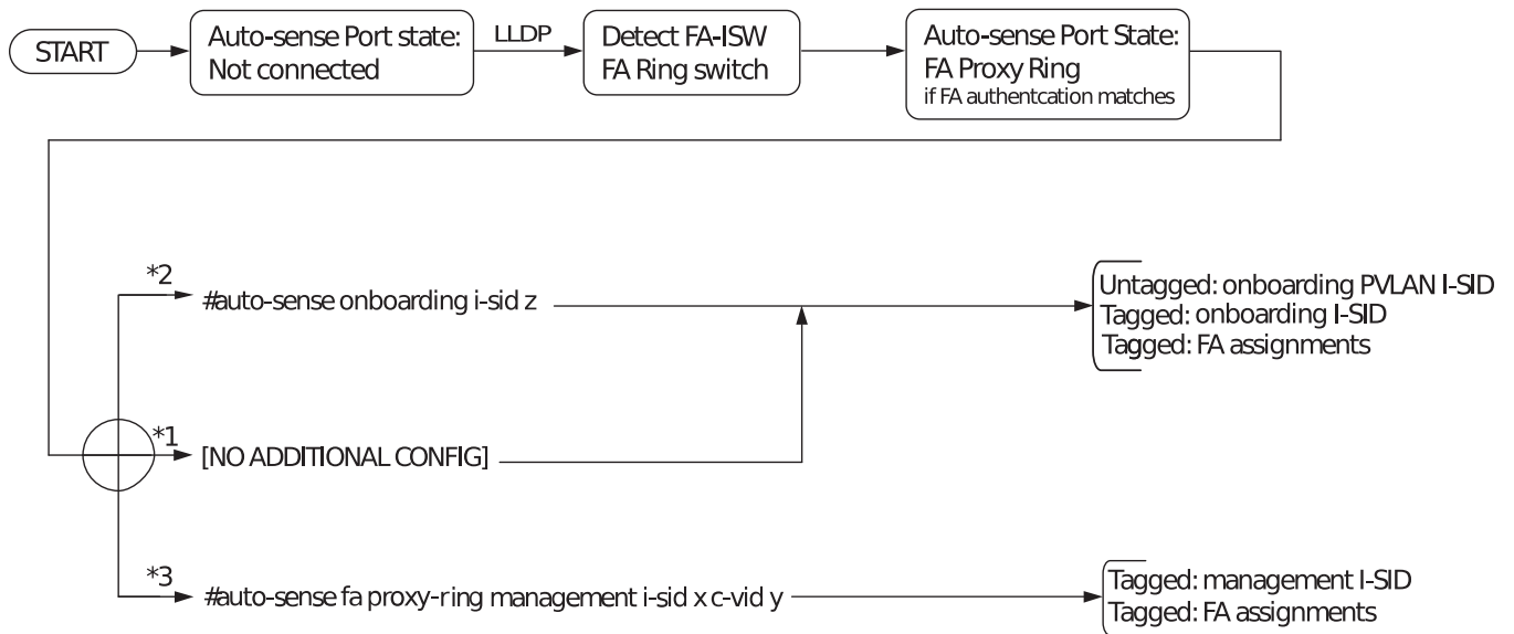
Figure 7: Auto-sense FA Proxy Ring Switch
