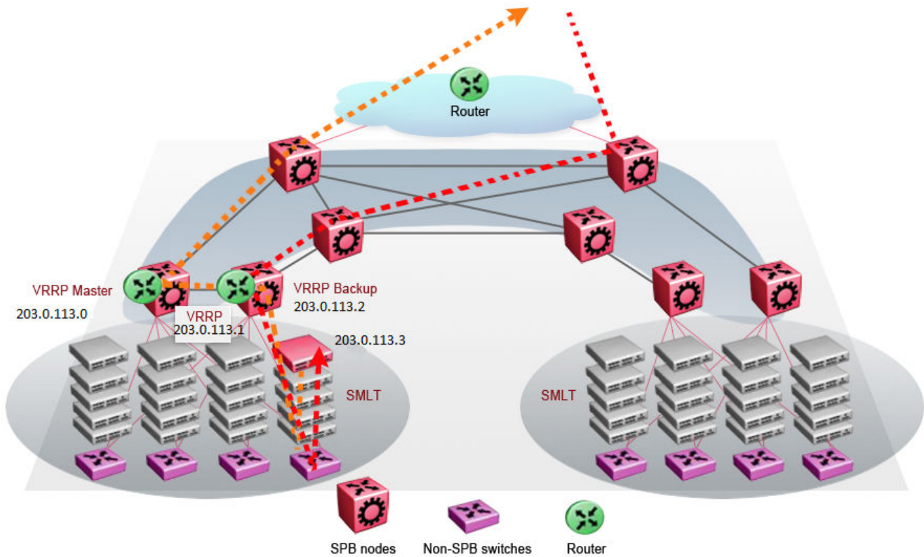
Figure 110: Traditional routing before moving VMs
