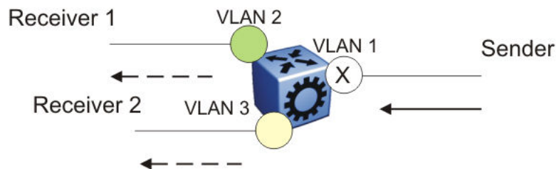
Figure 128: Data flow using deny-tx policy
