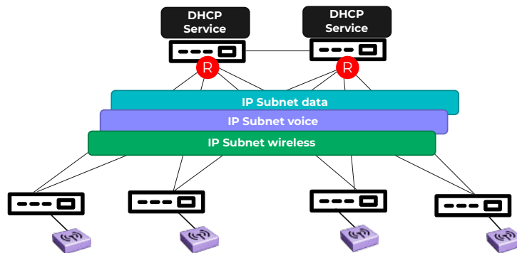
Figure 47: DHCP Server with a Single VRF - Small Campus Network
