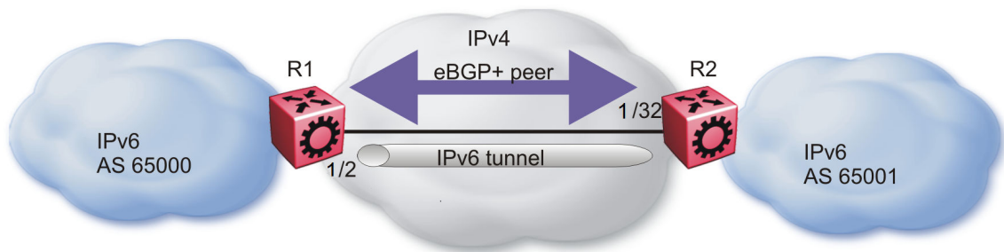
Figure 44: eBGP+ peers with IPv6 tunneling
