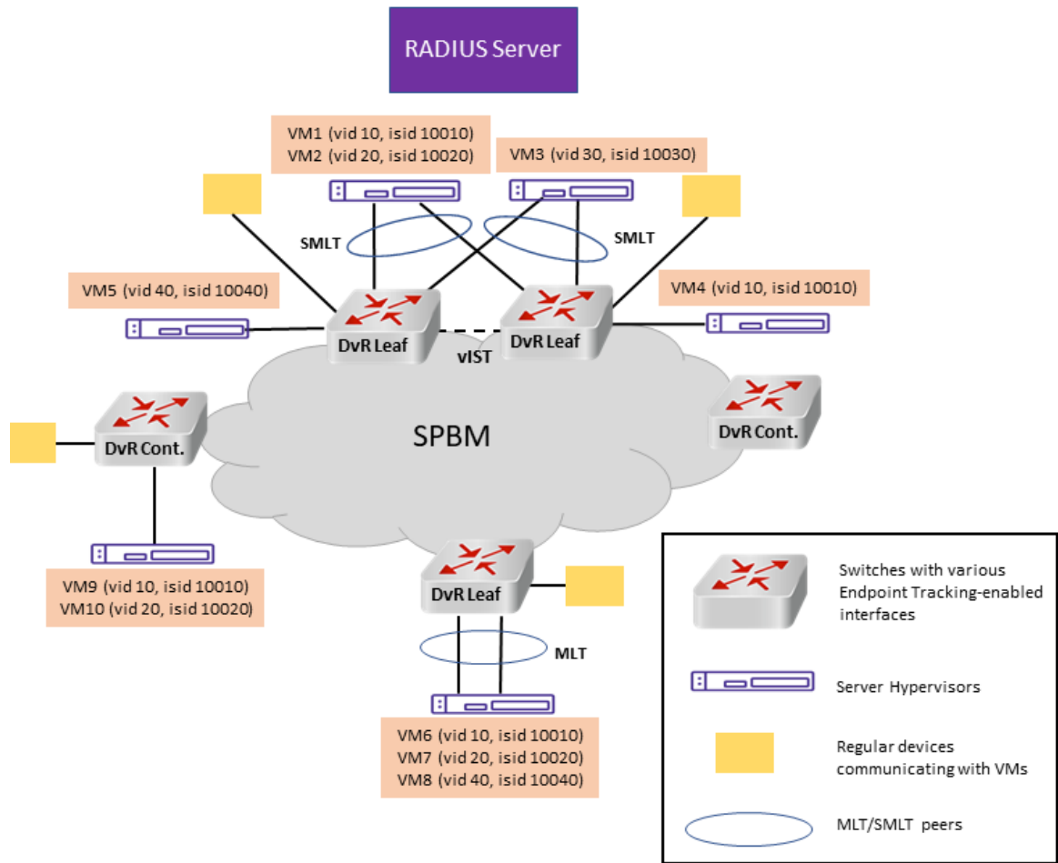
Figure 88: DvR Topology Example
