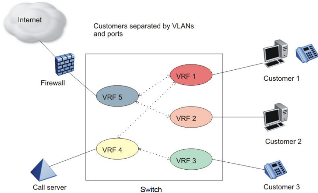
Figure 253: Inter-VRF forwarding
