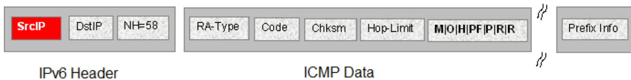
Figure 172: IPv6 ICMP RA Data Packet Outline
