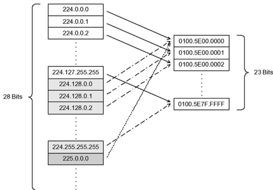
Figure 135: Multicast IP address to MAC address mapping
