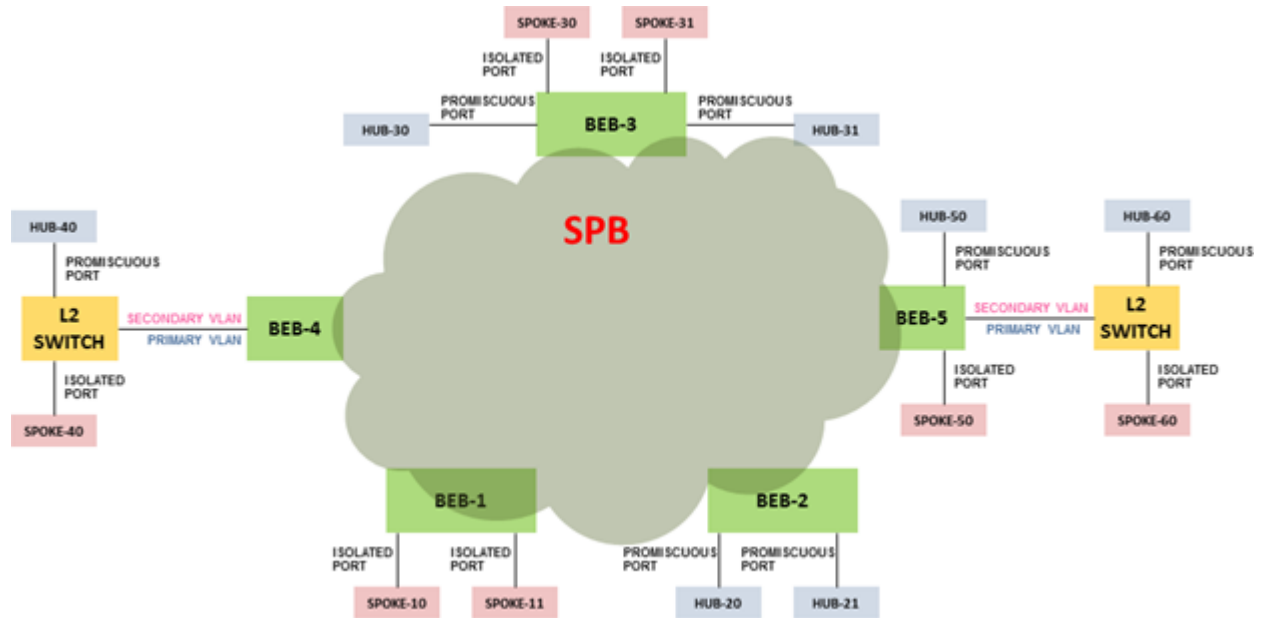
Figure 65: Sample E-Tree configuration
