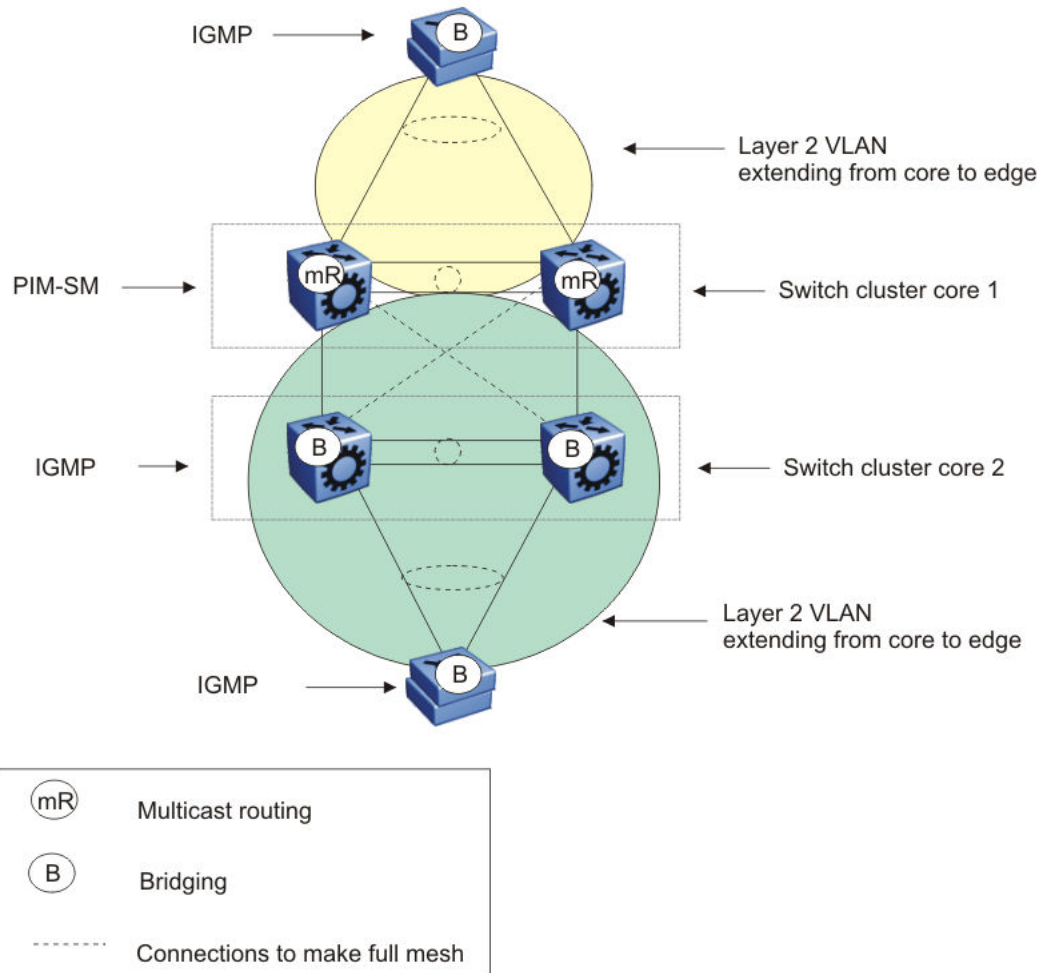
Figure 139: Multicast SMLT square 1
