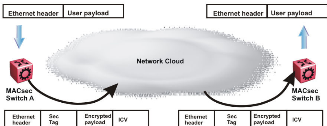
Figure 183: MACsec operation
