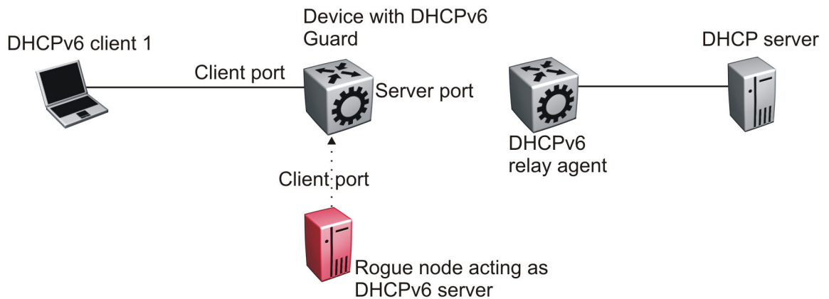
Figure 170: DHCPv6 Topology 2
