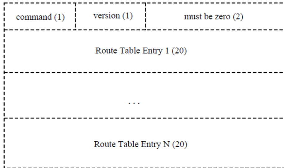
Figure 211: RIPng packet format
