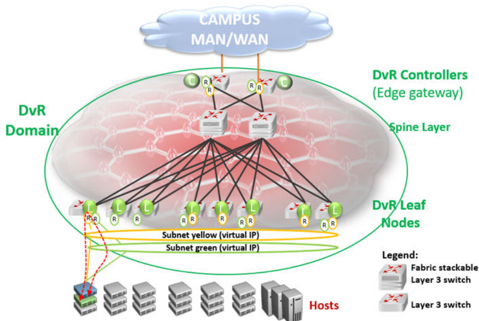
Figure 51: SPB Fabric network with central Layer 3 Controller and distributed Layer 3 datapath at the edges
