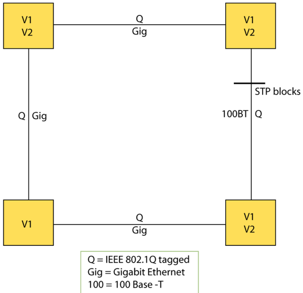
Figure 251: VLAN isolation
