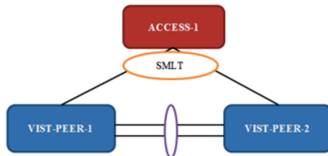
Figure 94: Example of Transparent Port UNI over vIST
