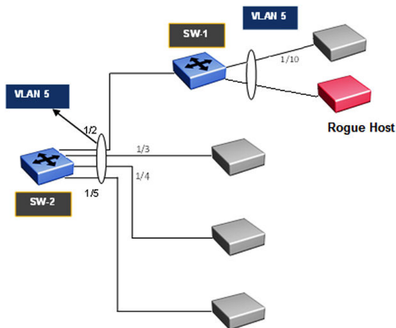
Figure 168: First Hop Security topology
