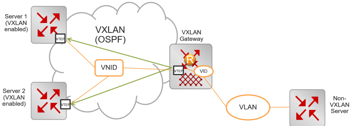
Figure 258: VXLAN-to-VLAN deployment
