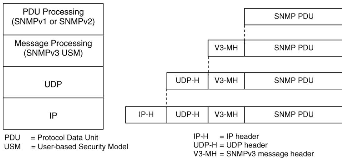
Figure 223: SNMPv3 USM
