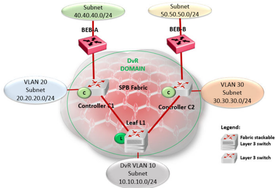
Figure 53: Redistribution of IPv4 local and static routes
