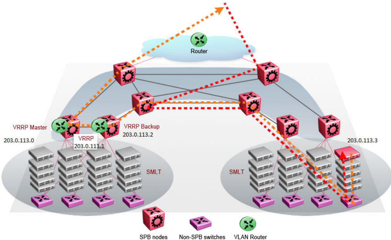
Figure 111: Traditional routing after moving VMs
