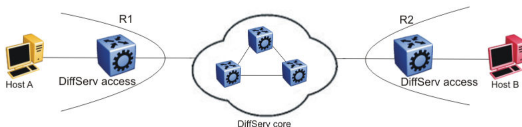
Figure 203: DiffServ network core and edge devices
