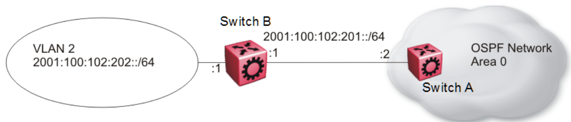
Figure 202: OSPFv3 configuration
