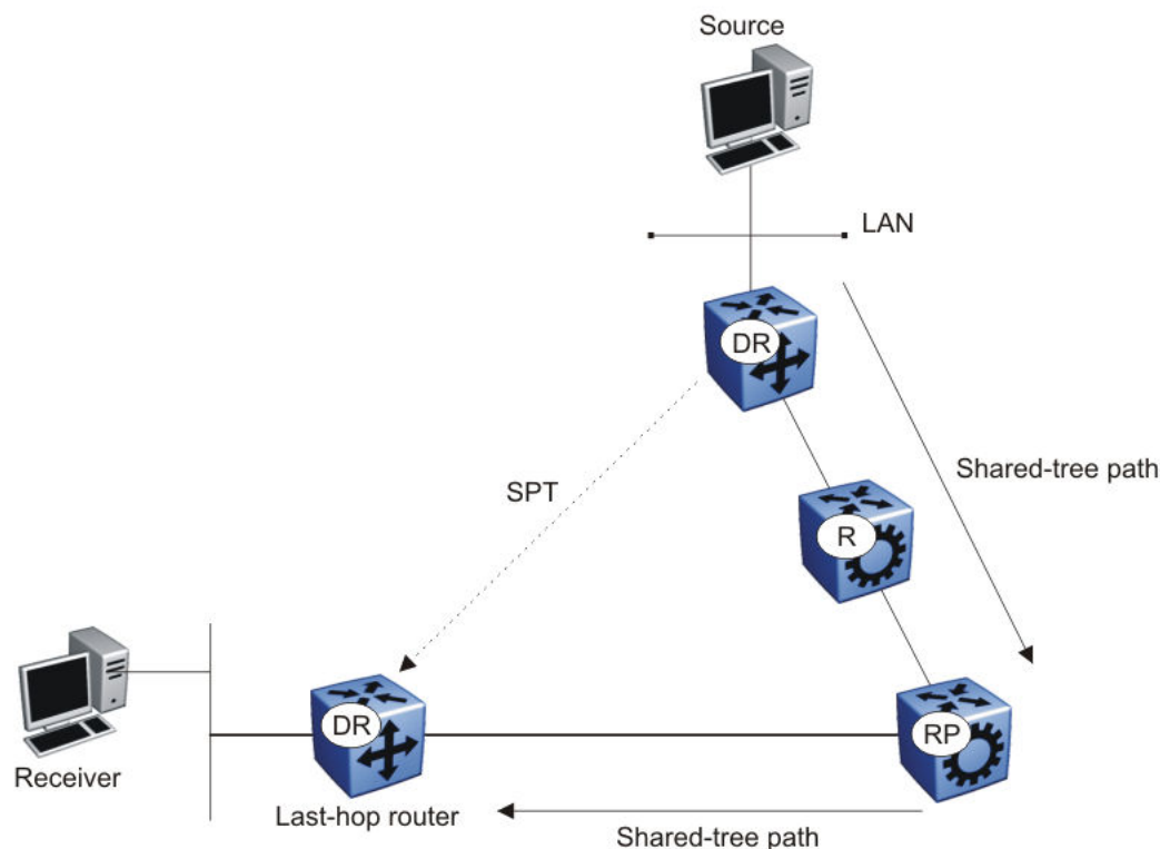
Figure 131: Shared tree and shortest-path tree
