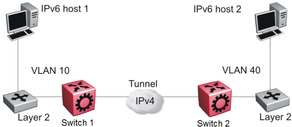
Figure 166: Tunnel configuration between router ports
