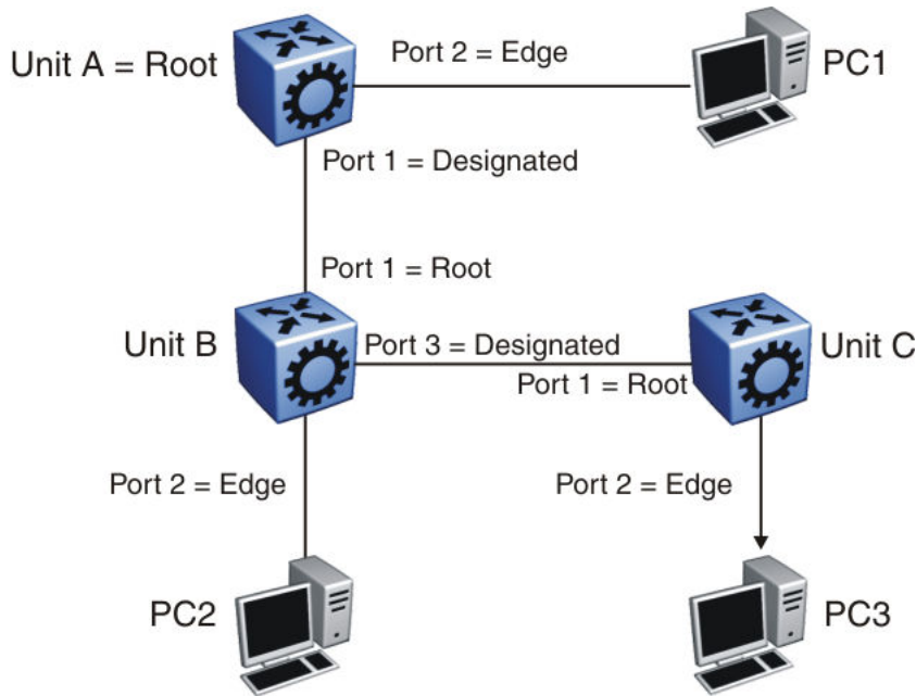
Figure 225: RSTP negotiation process
