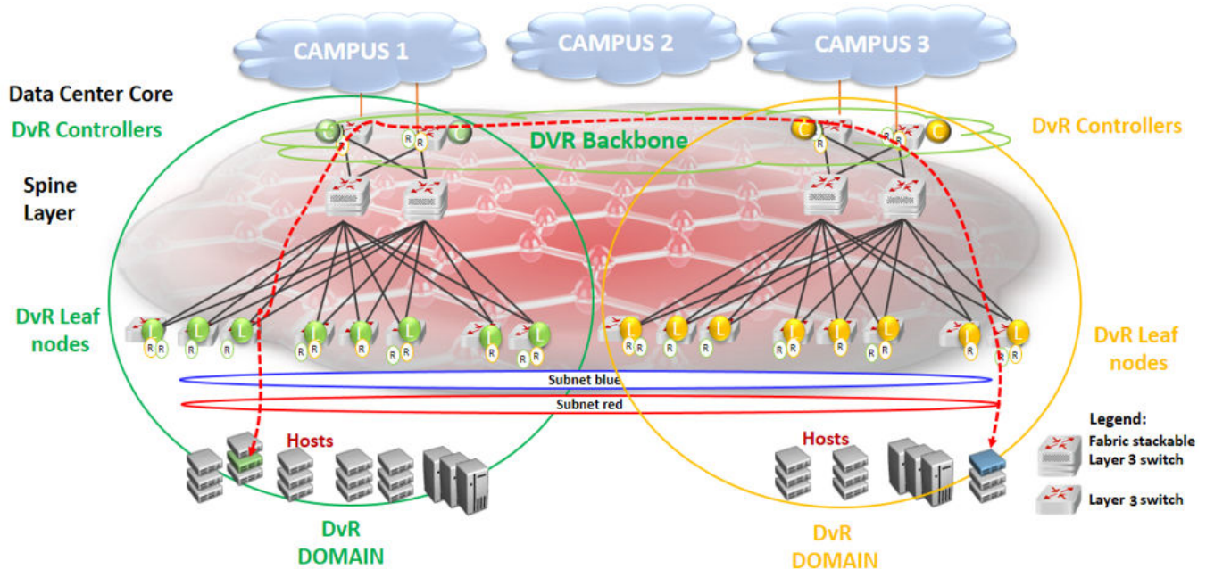
Figure 52: Shortest path routing between servers in different data centers
