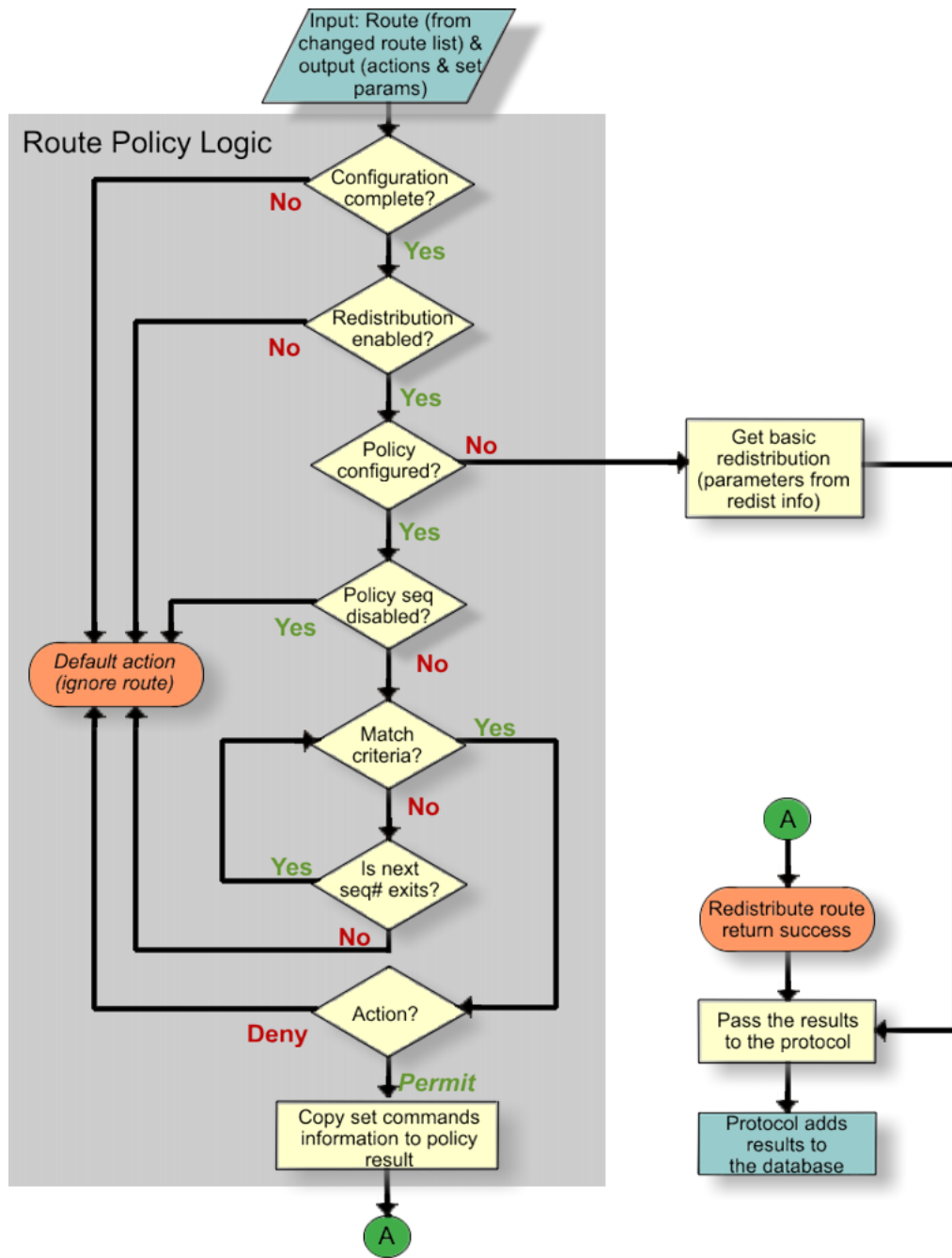
Figure 219: Route filtering logic
