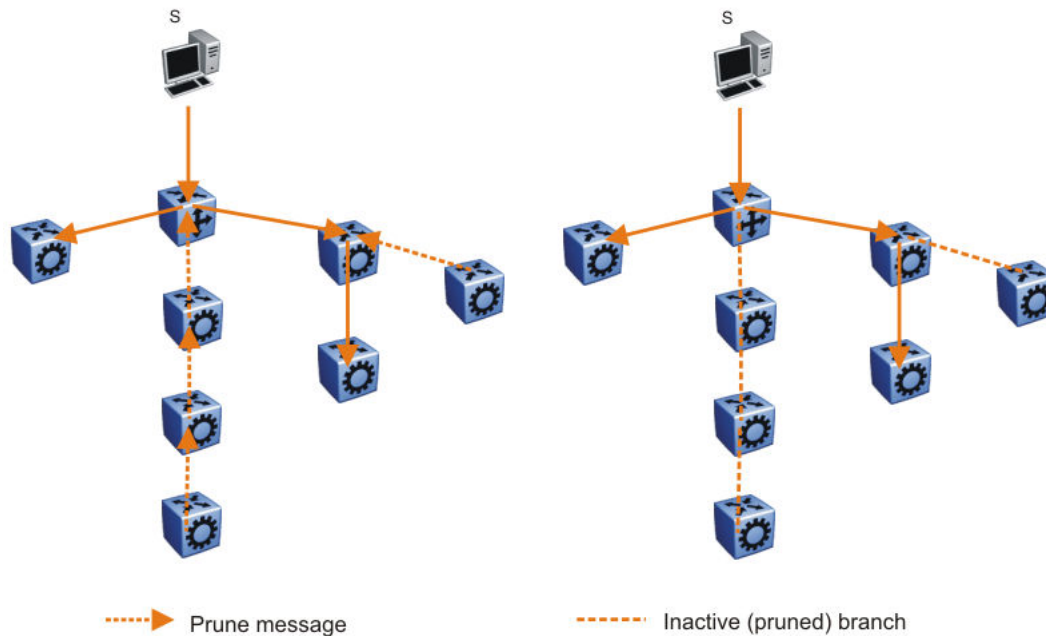
Figure 127: Pruning routers from a distribution tree
