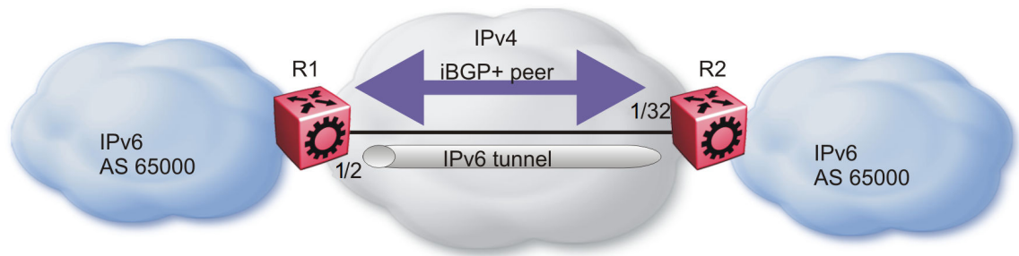
Figure 45: iBGP+ peers on CLIP interfaces with IPv6 tunneling
