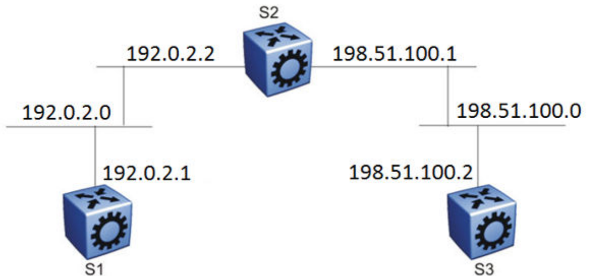
Figure 200: Example 2: OSPF on two subnets in one area
