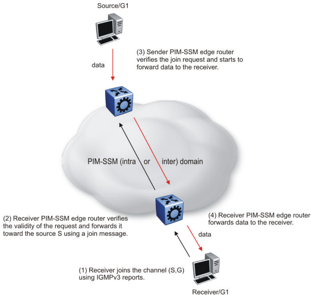
Figure 133: PIM-SSM architecture
