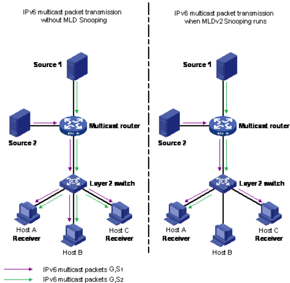
Figure 144: IPv6 multicast packet transmission when MLD v2 snooping is enabled and not enabled
