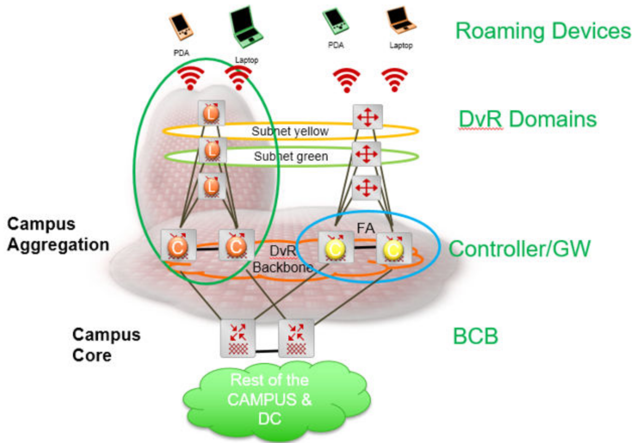
Figure 56: Wireless roaming in Campus
