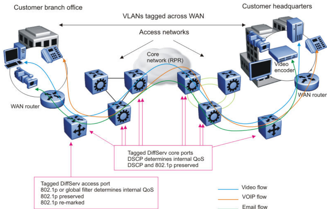
Figure 205: Trusted bridged traffic
