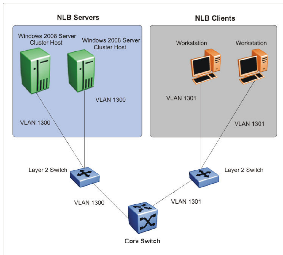
Figure 249: Supported NLB topology–example 1
