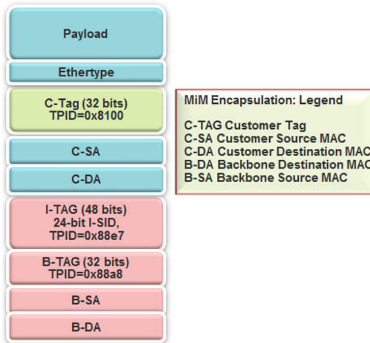
Figure 80: MiM encapsulation
