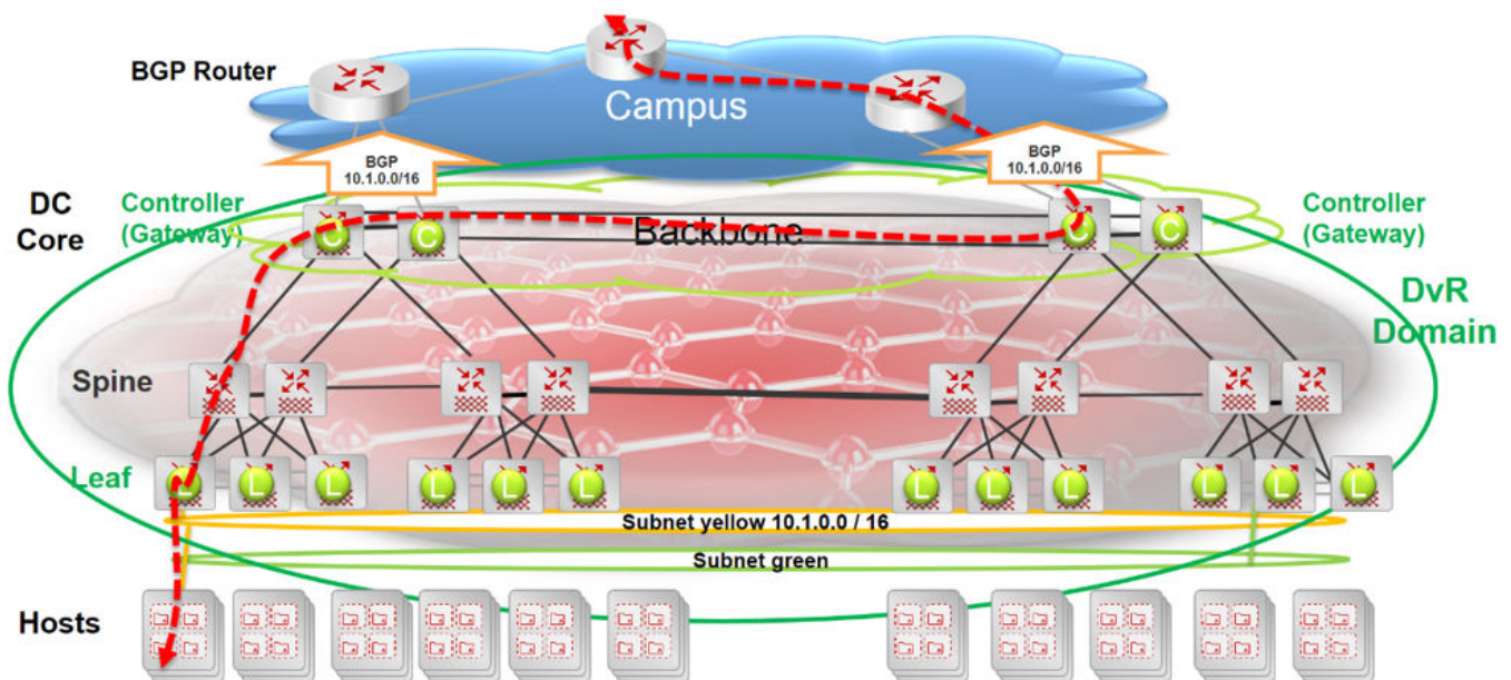
Figure 54: Inefficient traffic flow
