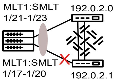
Figure 85: FA behavior in dual-homed SMLT during a link failure
