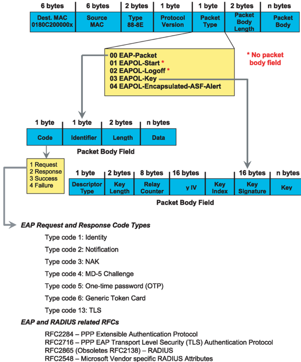
Figure 58: 802.1x Ethernet frame
