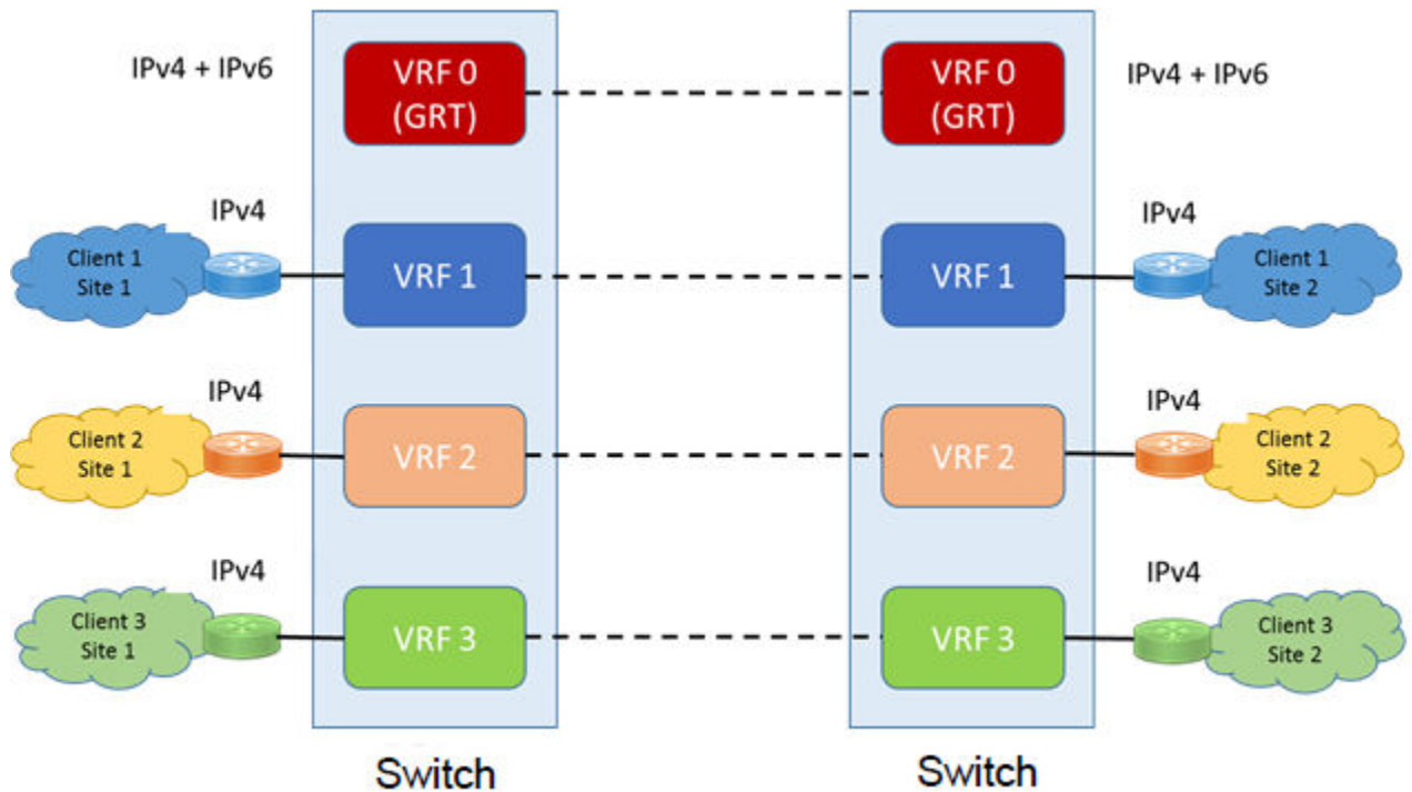
Figure 252: Multiple virtual routers in one system
