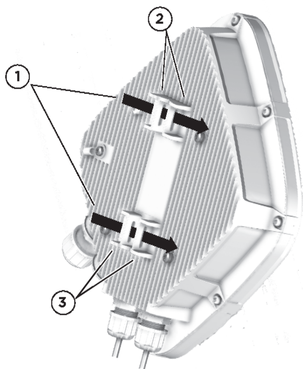
Figure 29: Pole mount strap slots on the back of the access point
