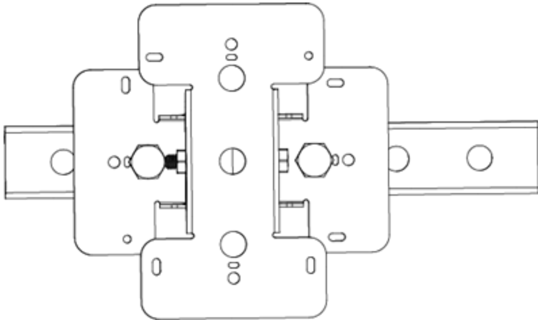
Figure 33: MBO-ART03 bracket attached to the Unistrut structure
