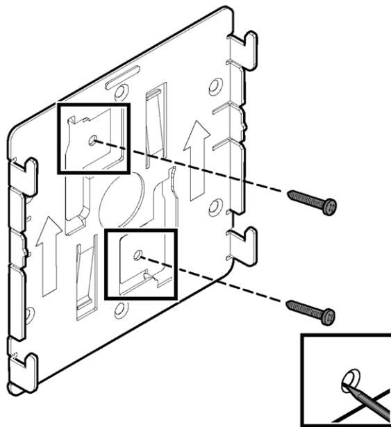
Figure 27: 37201 main mounting metal bracket
