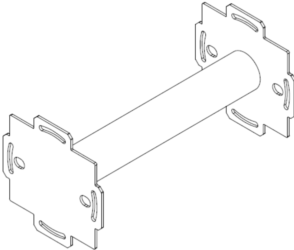
Figure 42: KT-150173-01 extension arm
