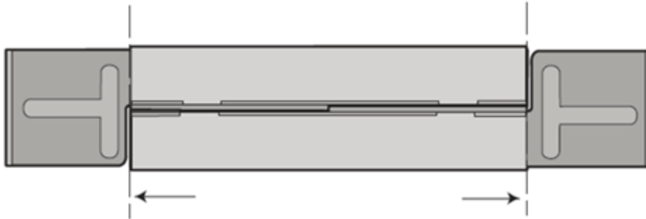
Figure 8: AH-ACC-BKT-AC-KIT protruded ceiling tile bracket parts attached together
