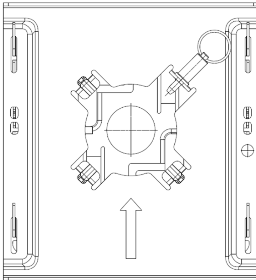
Figure 28: AX-BKT-WNGADAPT bracket
