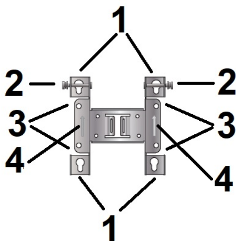
Figure 31: AH-ACC-BKT-ASM Accessory
