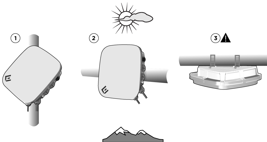
Figure 30: Access point pole mount positions
