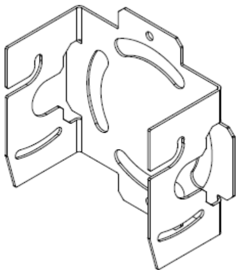
Figure 39: KT-147407-02 bracket 1-axis tilt part side view
