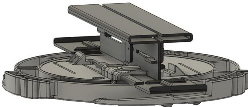
Figure 19: AH-ACC-BKT-TB-NF Adapter
