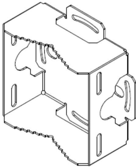
Figure 45: KT-147407-02 bracket pole part side view
