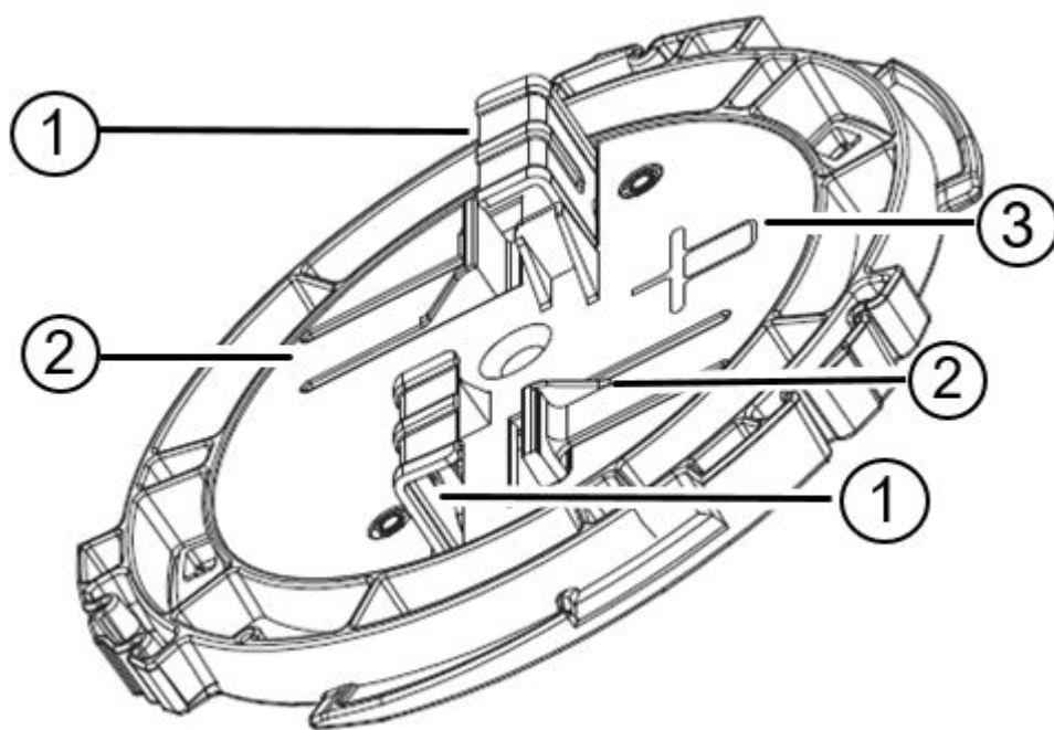
Figure 3: AH-ACC-BKT-AX-IL accessory bracket
