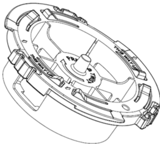
Figure 1: AH-ACC-BKT-AX-WL bracket
