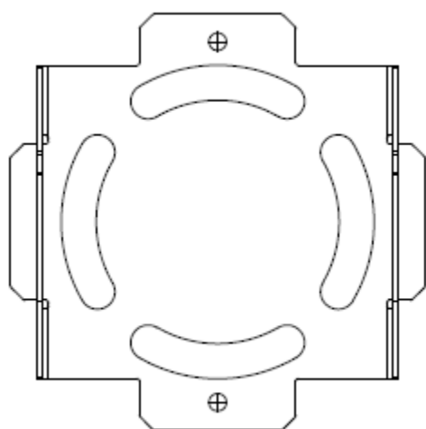
Figure 38: KT-147407-02 bracket 1-axis tilt part front view
