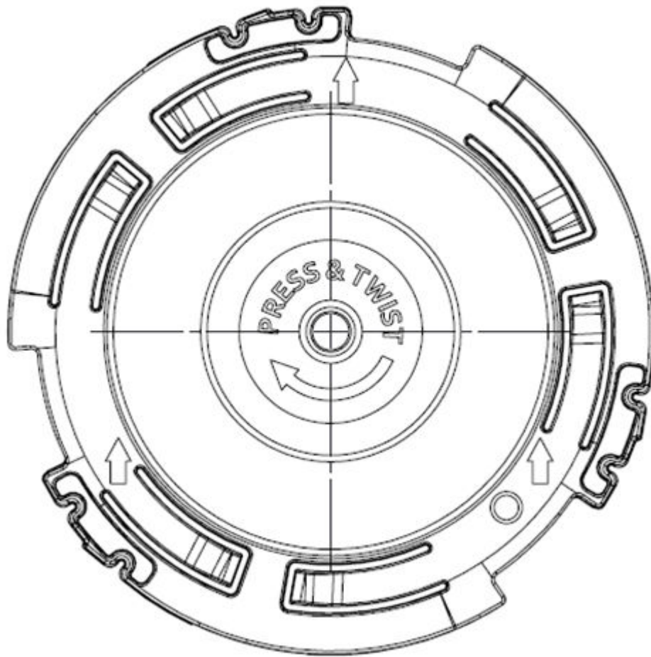
Figure 23: ACC-BKT-AX-JB Accessory Bracket Plastic Part
