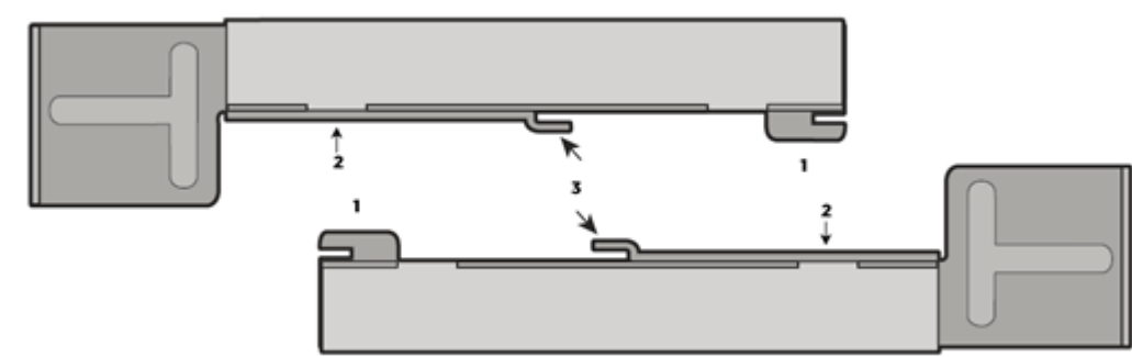
Figure 6: Locking tabs and bracket slots
