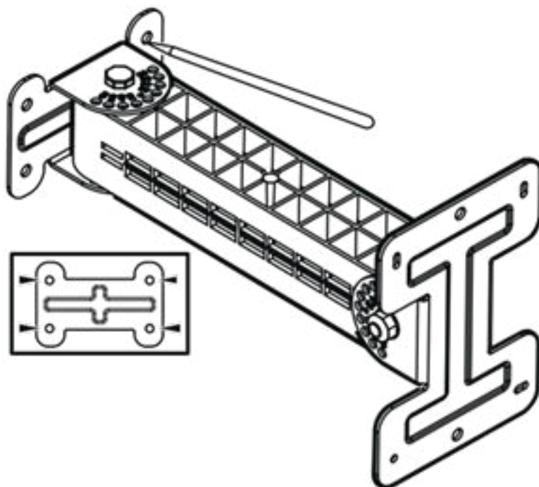
Figure 43: MBO-ART02 articulating mounting bracket wall holes template
