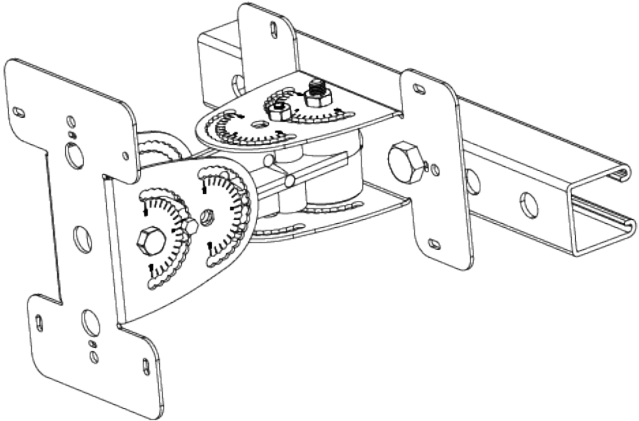
Figure 32: MBO-ART03 bracket angular adjustments
