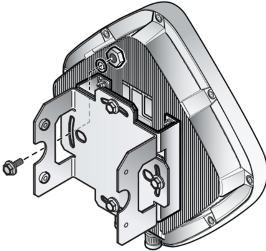
Figure 41: KT-147407-02 flat part attachment to -AX adapter bracket
