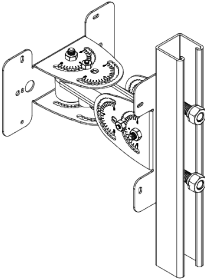
Figure 34: MBO-ART03 torque position on the Unistrut structure
