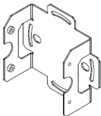
Figure 37: KT-147407-02 bracket flat part side view
