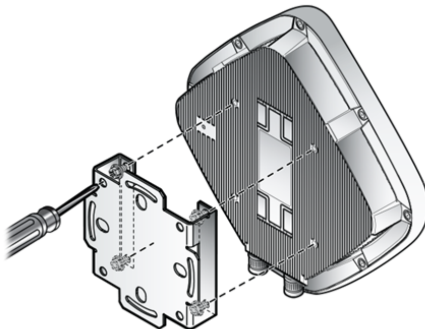
Figure 40: ACC-MBO-KT-AX adapter bracket attachment to an outdoor access point
