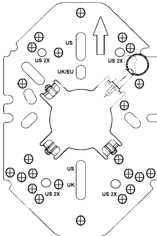
Figure 22: ACC-BKT-AX-JB Accessory Bracket Metal Part
