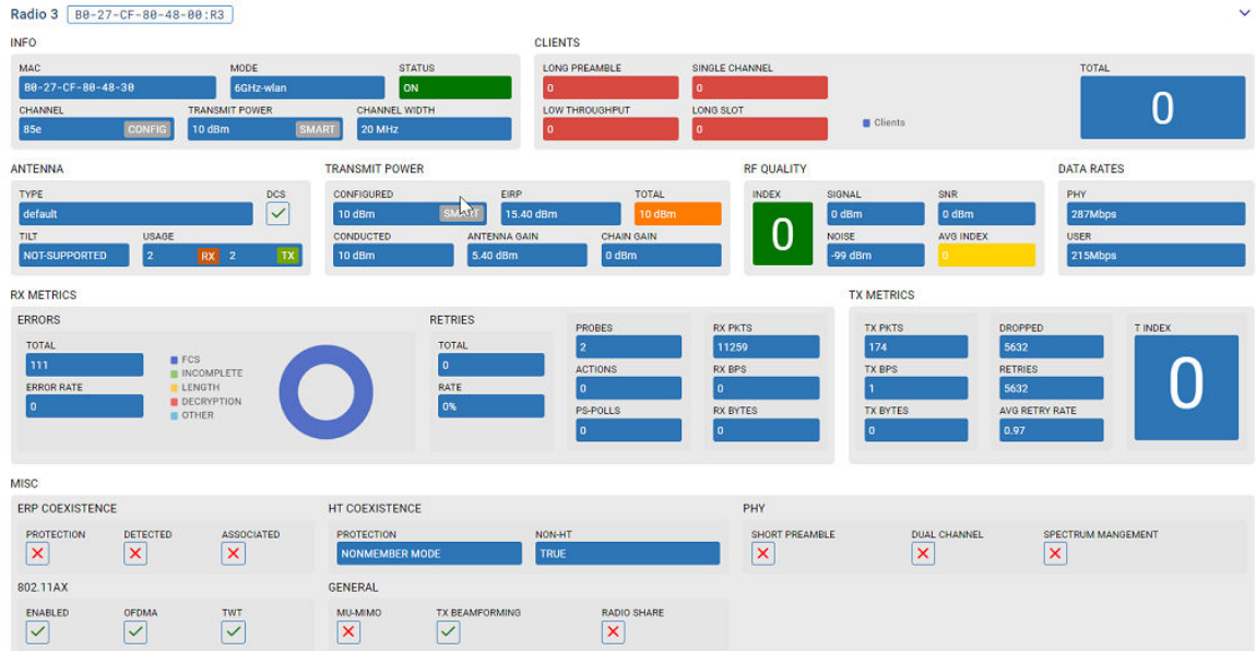
Figure 15: AP Statistics - Radios Detailed Display
