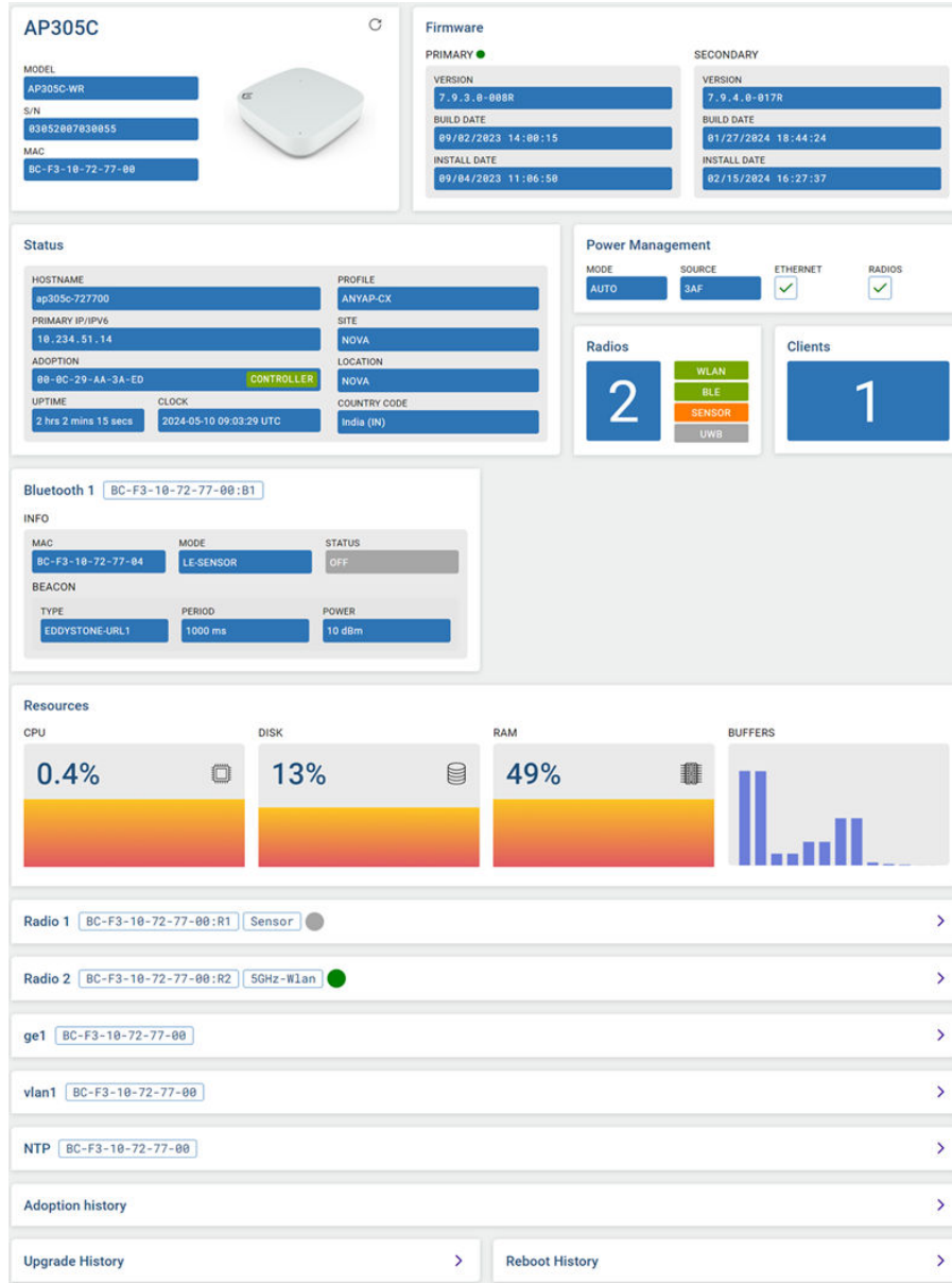
Figure 6: Example of Device Statistics Display for APs
