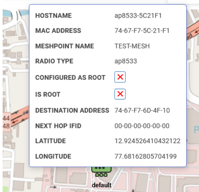
Figure 52: Mesh point geographical details
