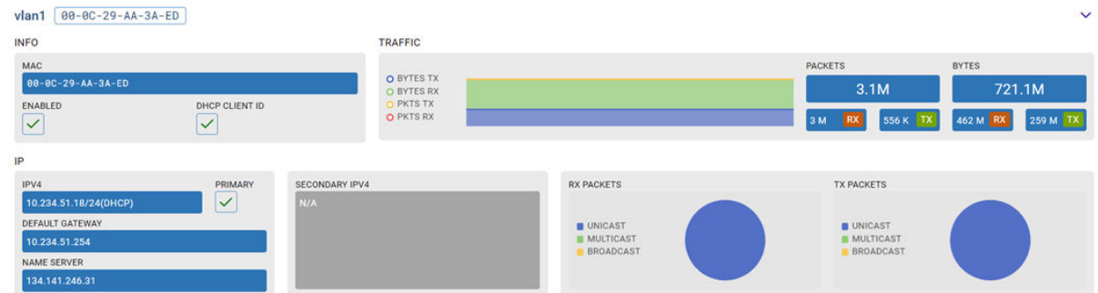
Figure 32: Controller Statistics – VLAN Details Display
