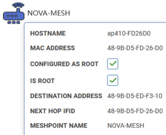
Figure 51: Mesh Point statistical logical view data
