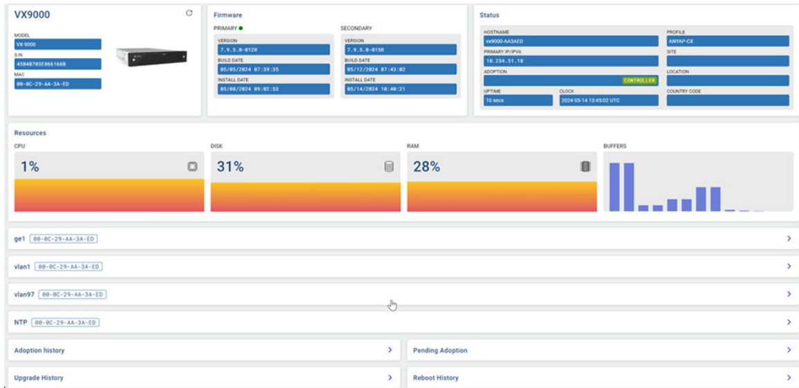
Figure 24: Controller Statistics
