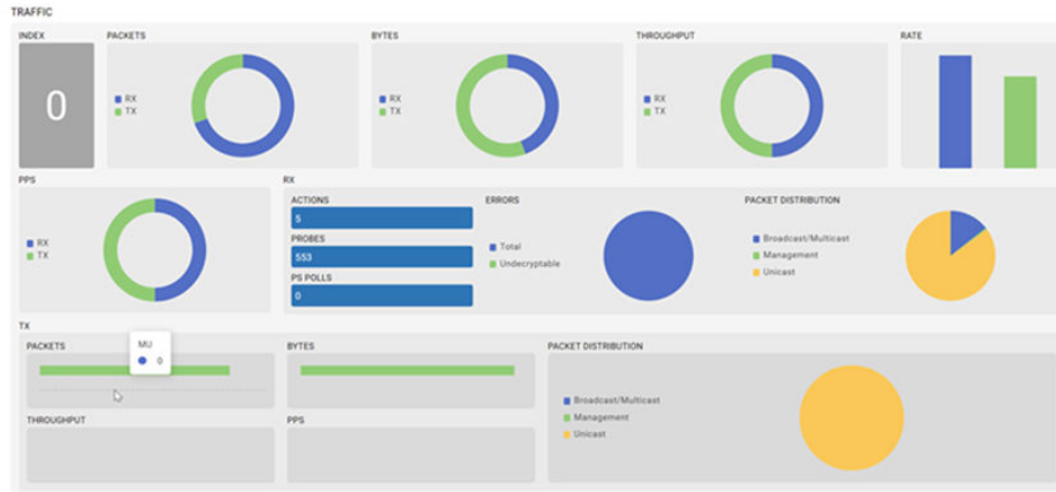
Figure 50: Client Performance Statistics – Example Traffic Display
