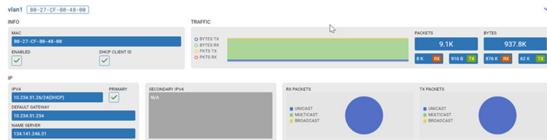
Figure 19: AP Statistics – VLAN Details Display
