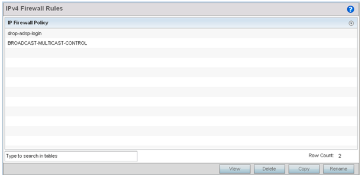
Figure 345: IP Firewall Policy Screen
