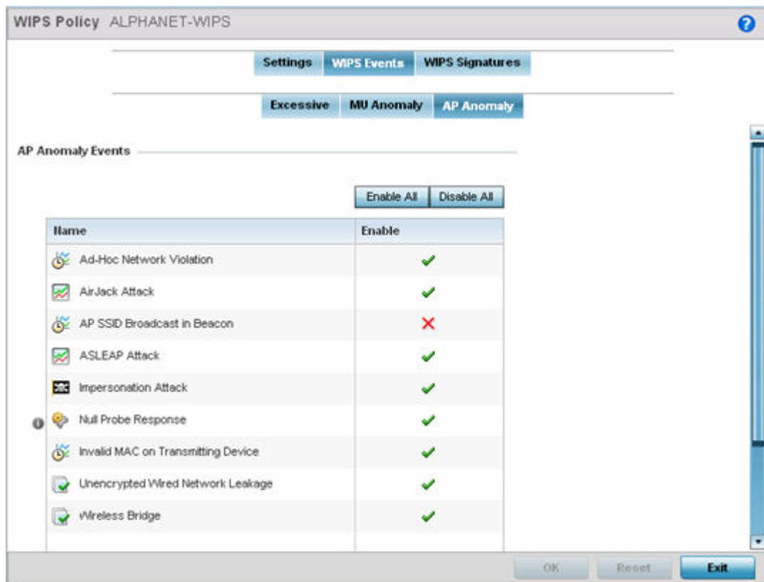
Figure 368: Wireless IPS Screen - WIPS Events - AP Anomaly Tab
