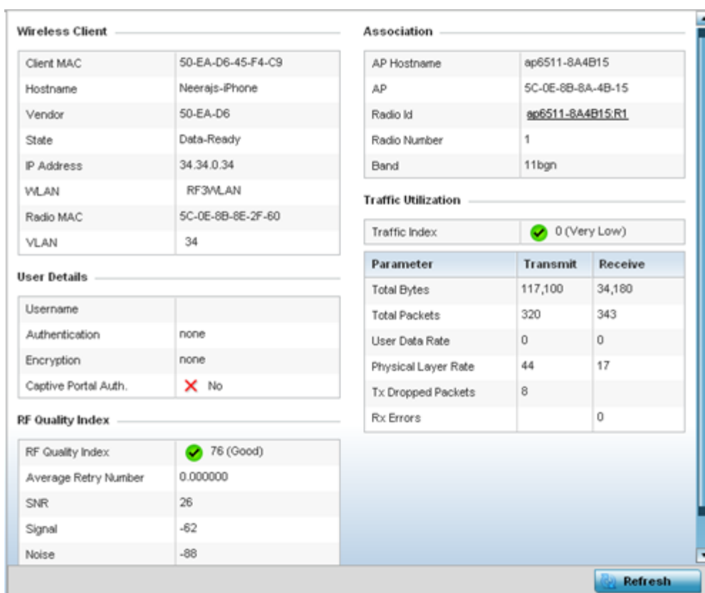
Figure 419: Wireless Client - Statistics - Health Screen
