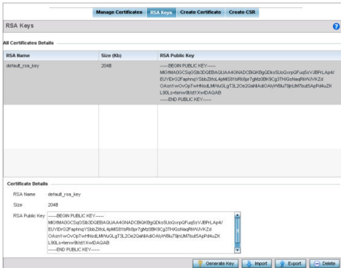
Figure 133: Certificate Management - RSA Keys Screen
