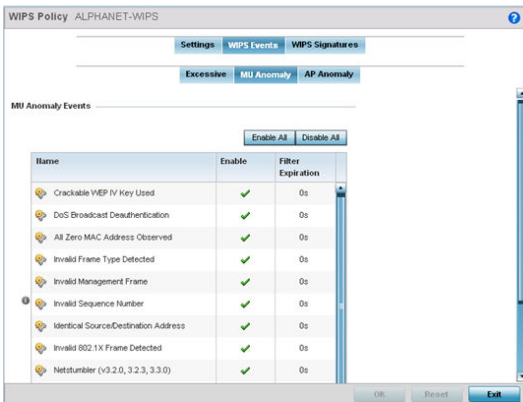
Figure 367: Wireless IPS Screen - WIPS Events - MU Anomaly Tab
