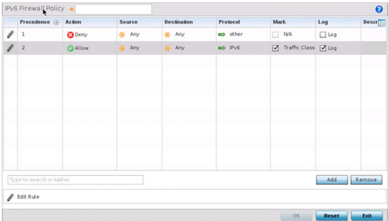
Figure 346: IP Firewall Rules Screen - Adding a New Rule
