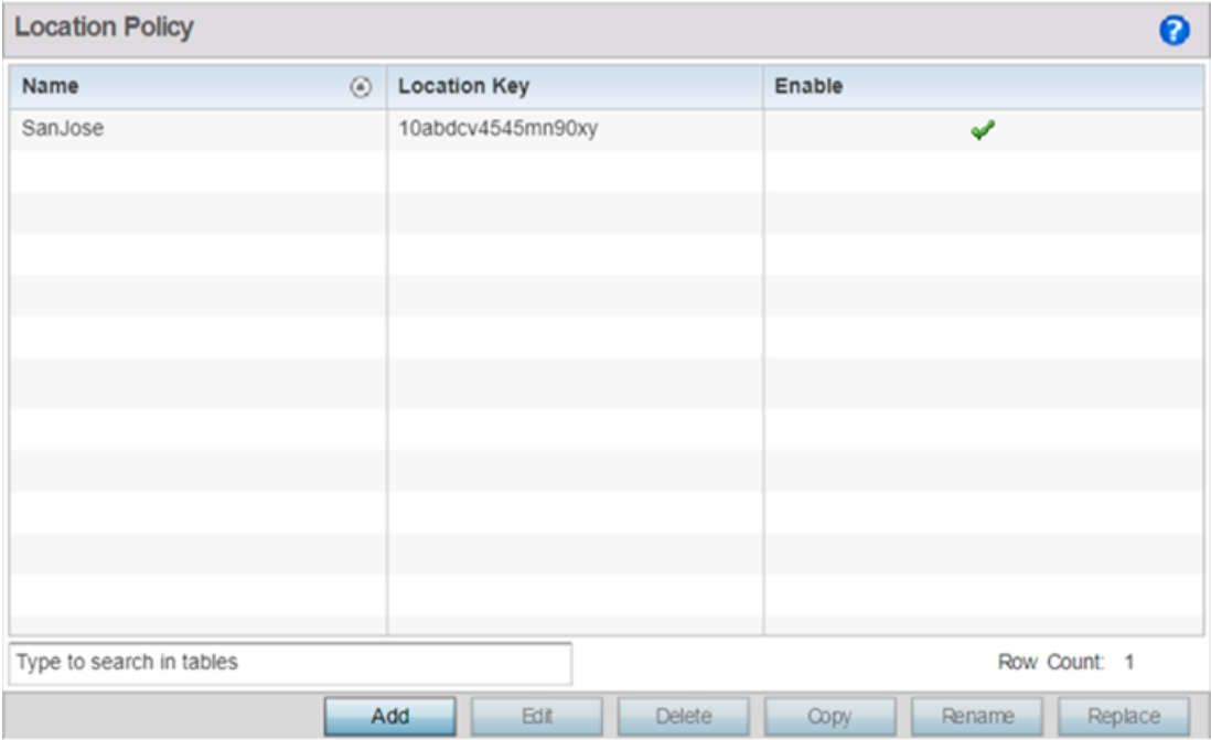
Figure 336: Configuration → Wireless → Location Policy
