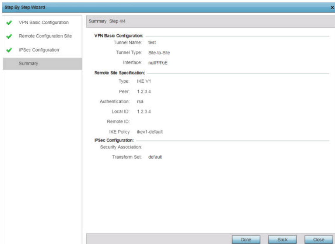
Figure 221: Summary Step 4/4 Screen
