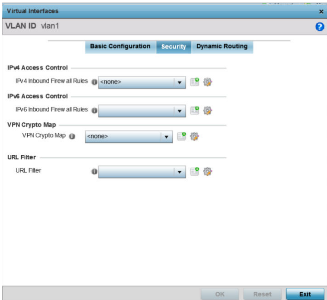
Figure 157: Profile Overrides - Interface - VLAN Interface - Security Screen
