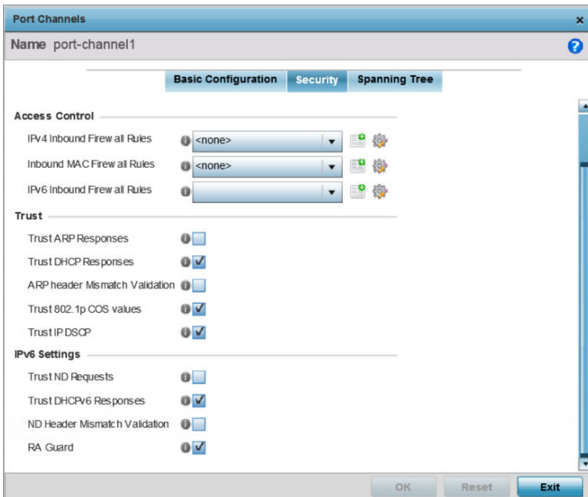
Figure 161: Port channel - Security Configuration Screen
