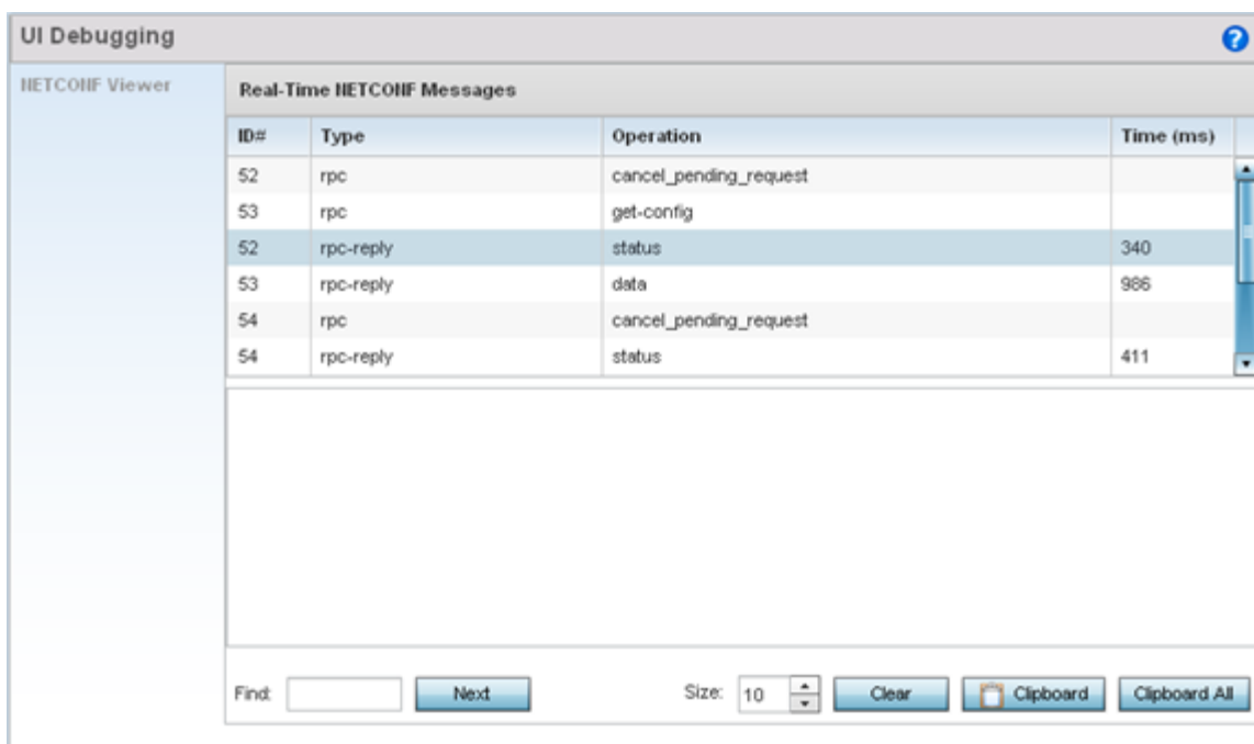
Figure 406: UI Debugging screen - NETCONF Viewer
