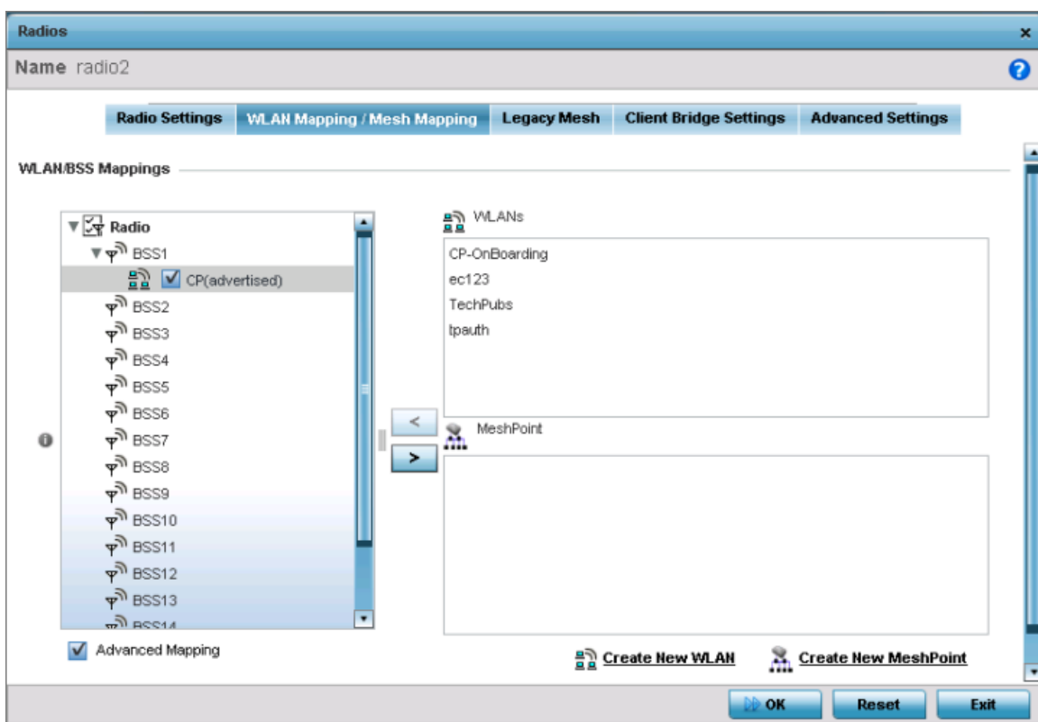
Figure 165: Profile Overrides - Radio Interface - WLAN Mapping / Mesh Mapping Screen
