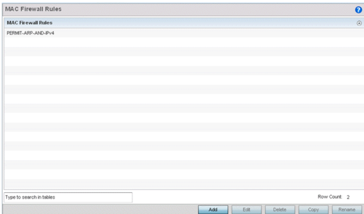
Figure 363: MAC Firewall Rules Screen
