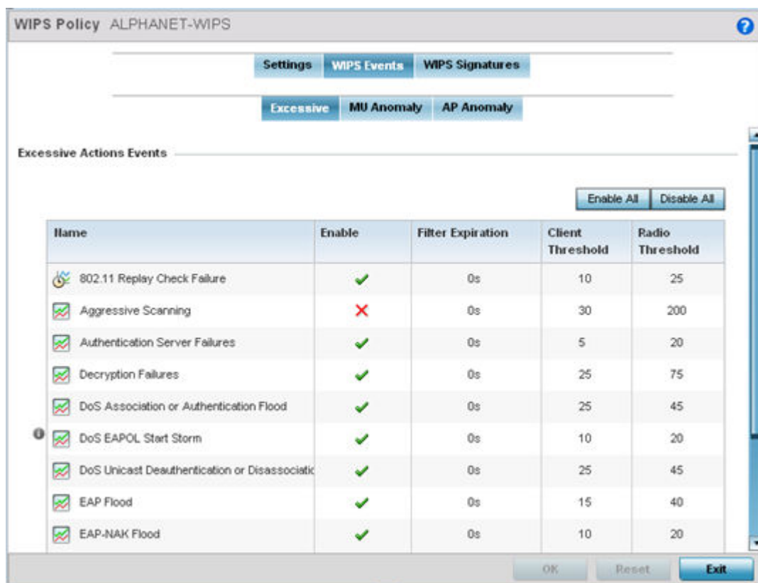
Figure 366: Wireless IPS Screen - WIPS Events - Excessive Tab
