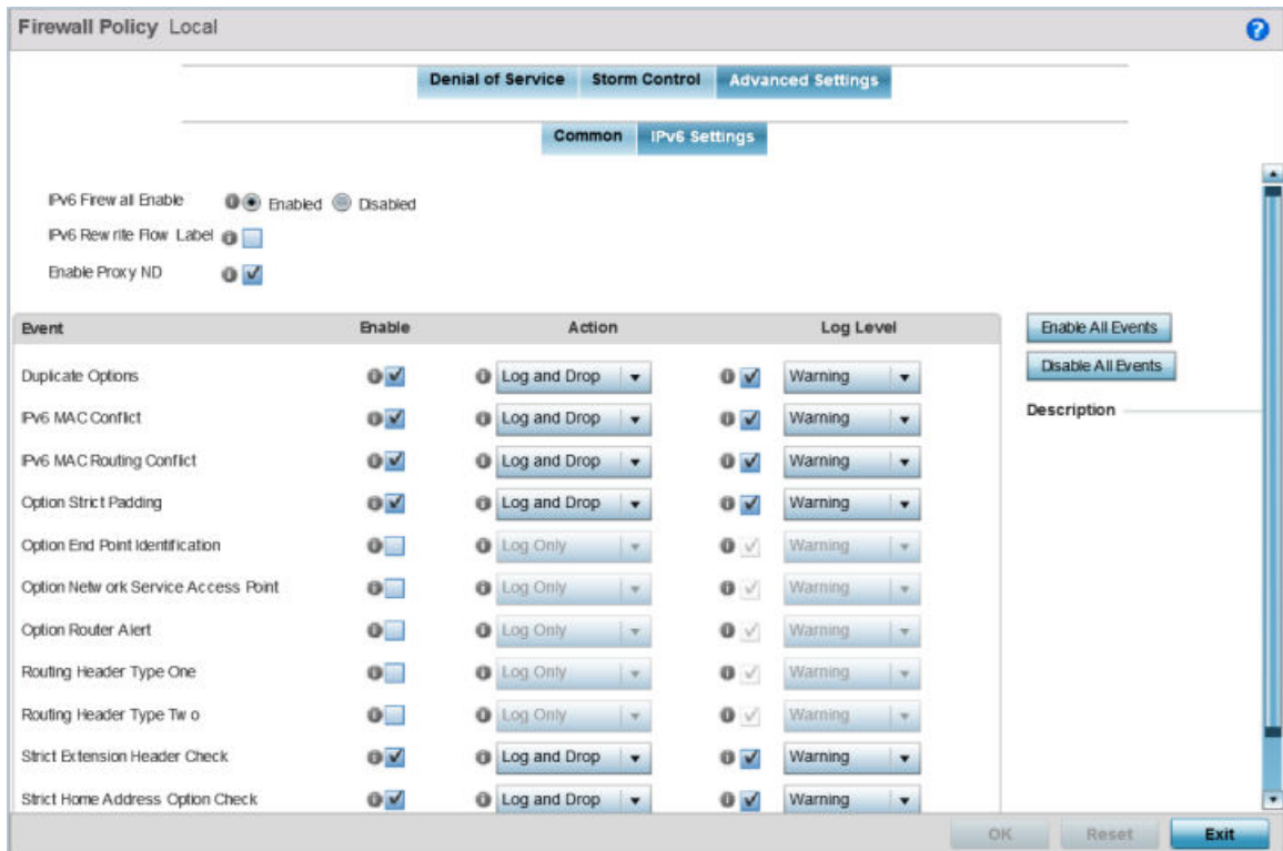
Figure 345: Wireless Firewall - Add/Edit - Advanced Settings - IPv6 Settings Tab
