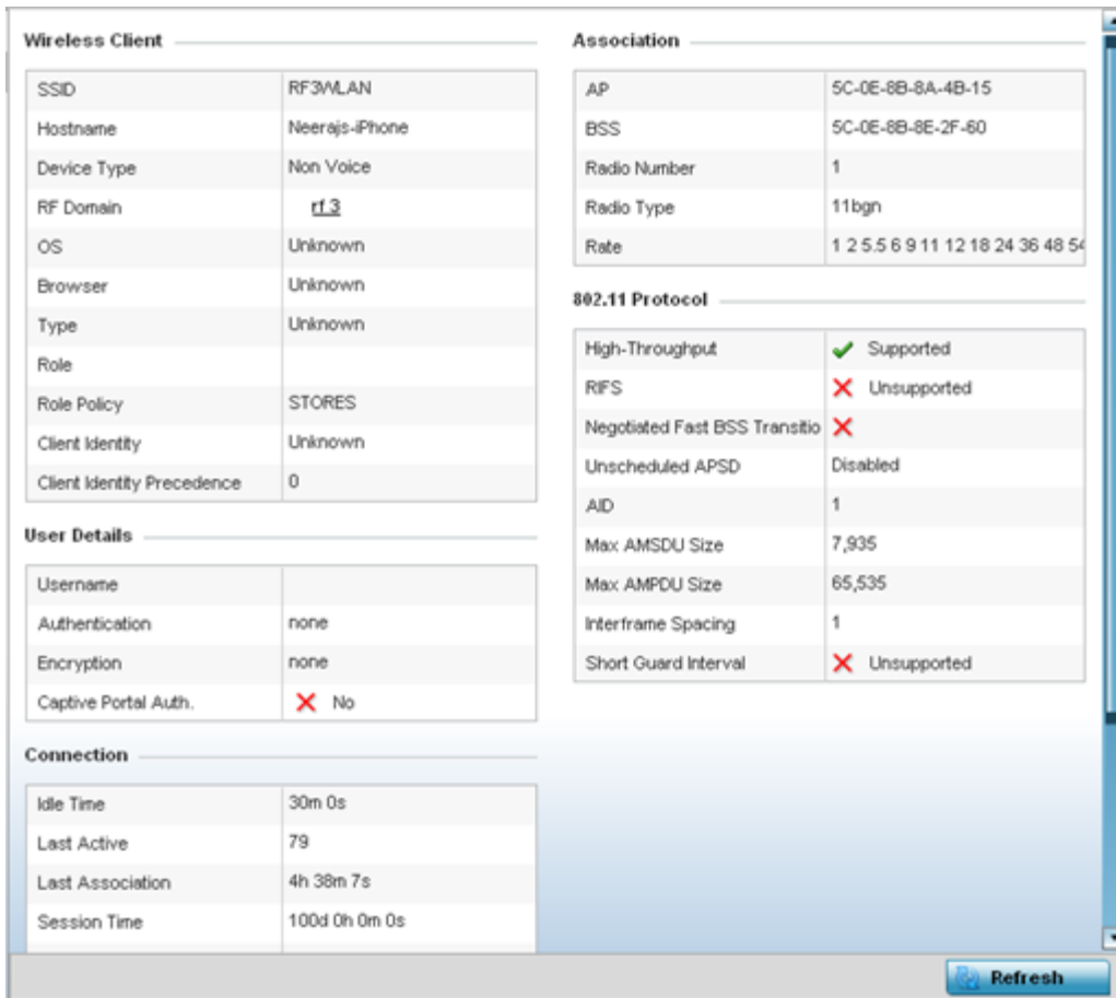
Figure 435: Wireless Client Detailed Statistics Screen
