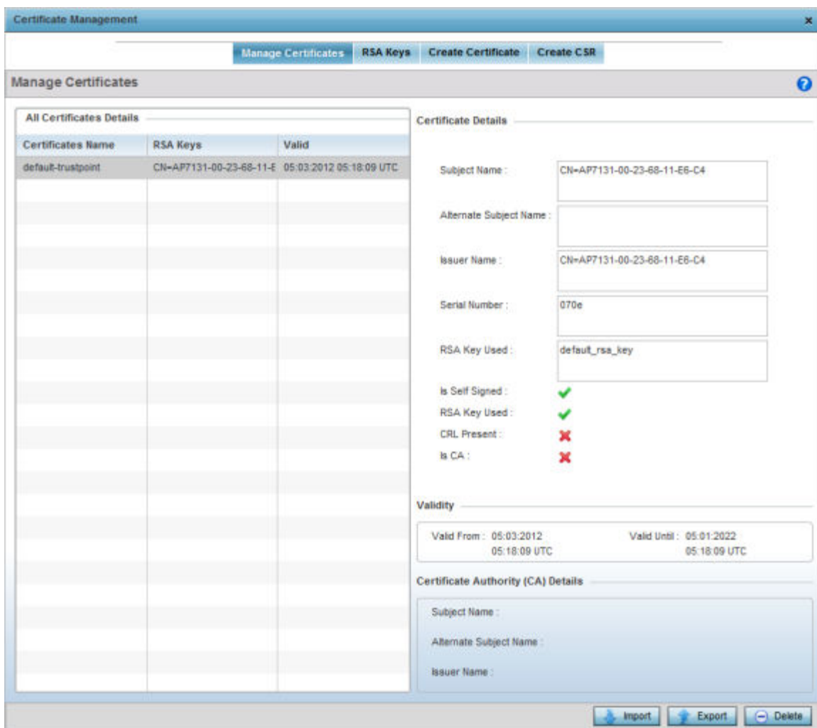
Figure 132: Certificate Management - Manage Certificates Screen
