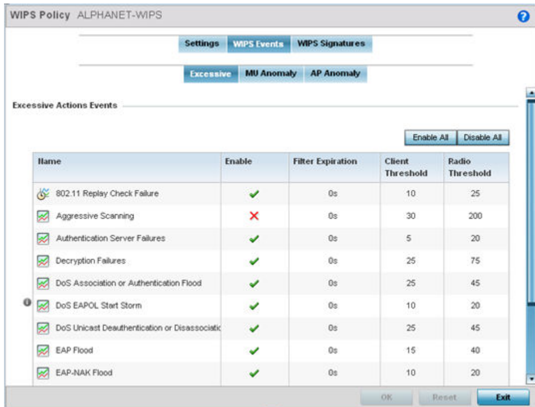
Figure 373: Wireless IPS Screen - WIPS Events - Excessive Tab
