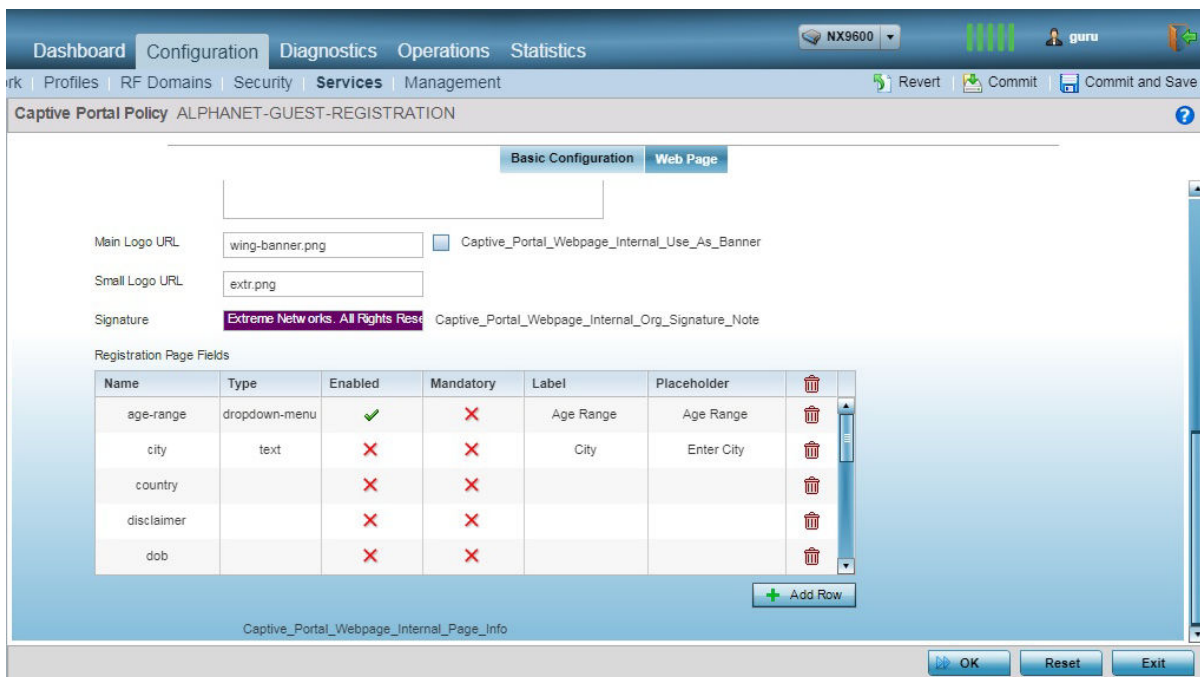
Figure 384: Captive Portal Policy - Web Page - Internal - Registration - Registration Page Fields Table
