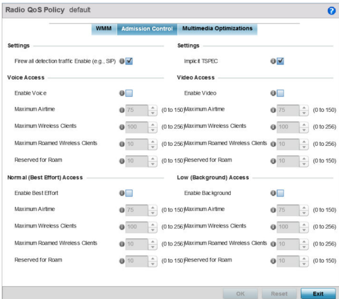
Figure 310: Radio QoS Policy Admission Control Screen
