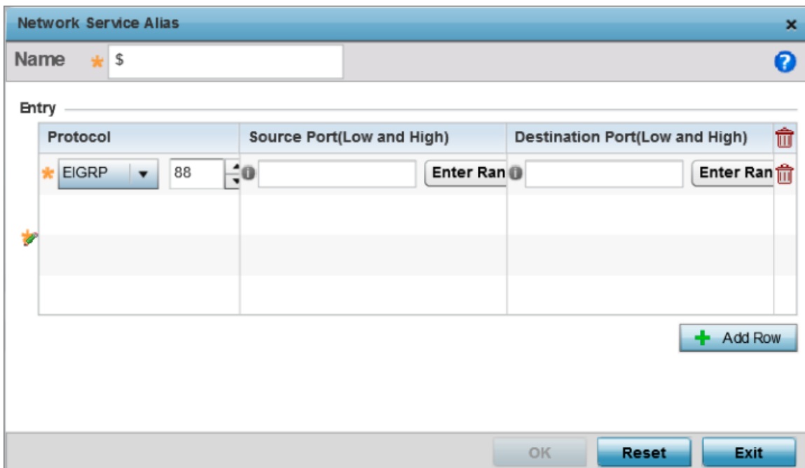
Figure 215: Network Alias - Network Service Alias Add screen
