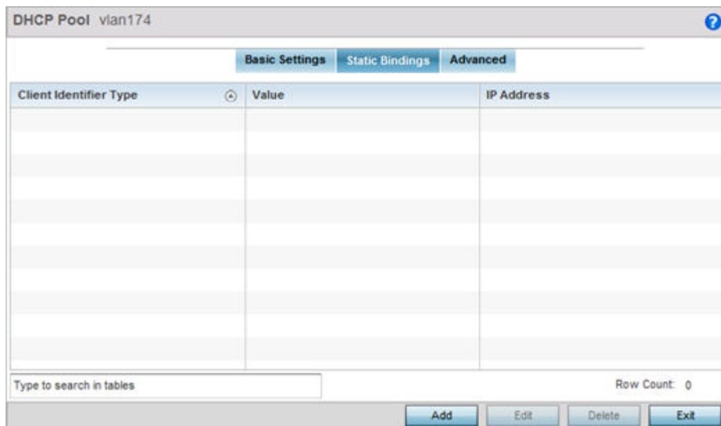
Figure 391: DHCP Pools - Add/Edit - Static Bindings Tab
