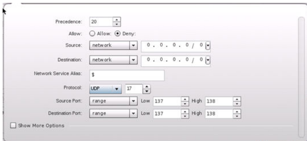
Figure 350: WLAN Security - IP Firewall Rules - Edit Rule Screen
