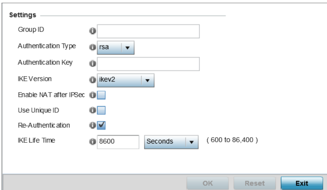
Figure 224: Profile Overrides - Security - Auto IPsec Tunnel Configuration Screen
