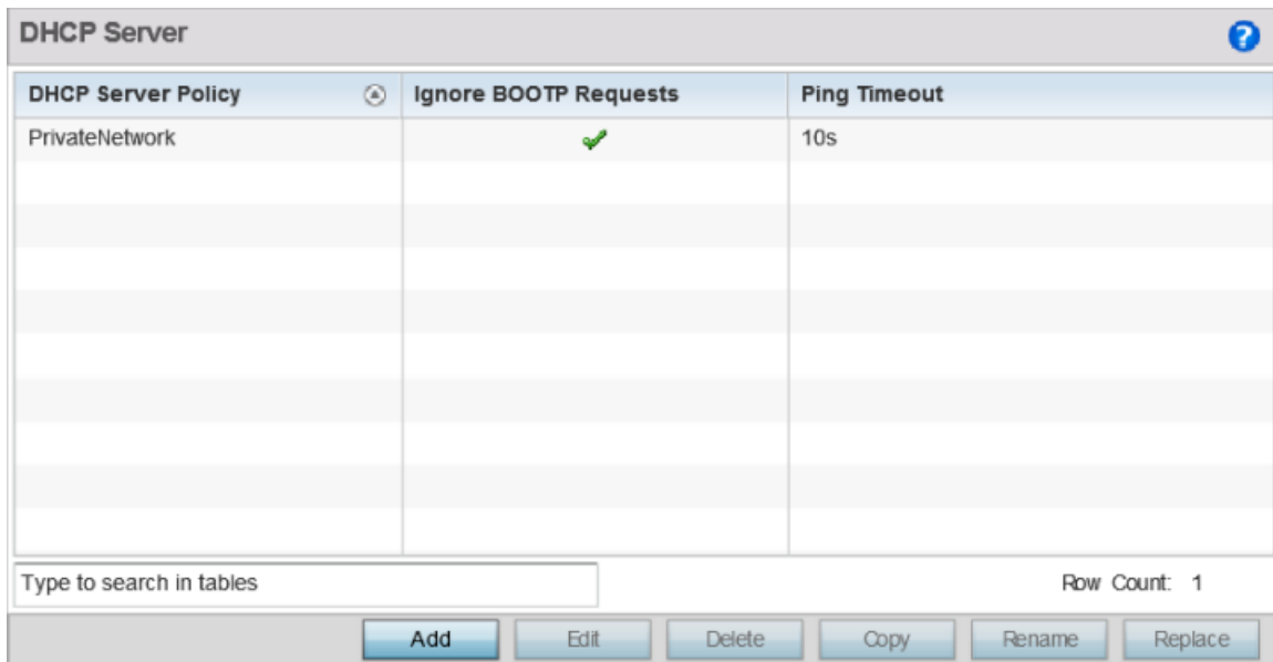
Figure 388: DHCP Server Policy Screen
