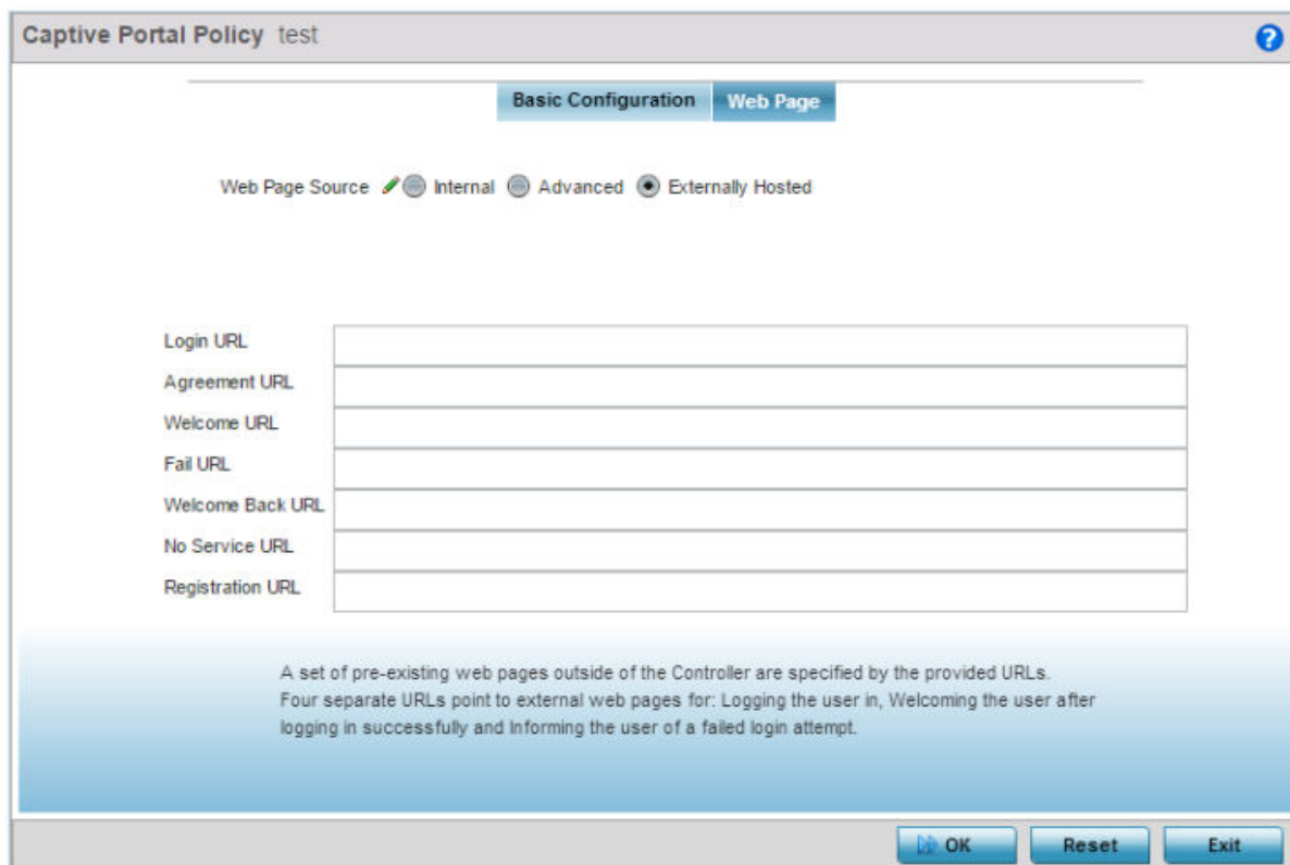
Figure 385: Captive Portal Policy Screen - Web Page Tab - Externally Hosted Web Page Screen
