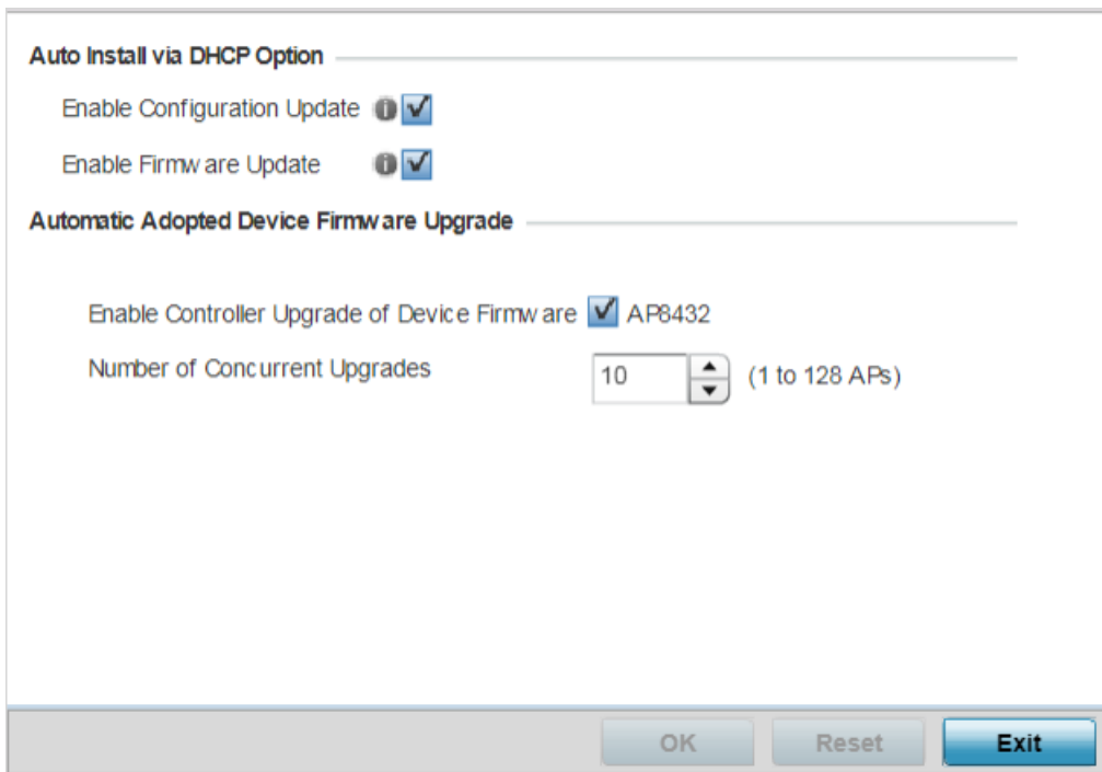
Figure 248: Management - Firmware Upgrade Configuration Screen
