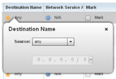
Figure 352: IWLAN Security - IP Firewall Rules - Add/Edit Specific Criteria Pop-up
