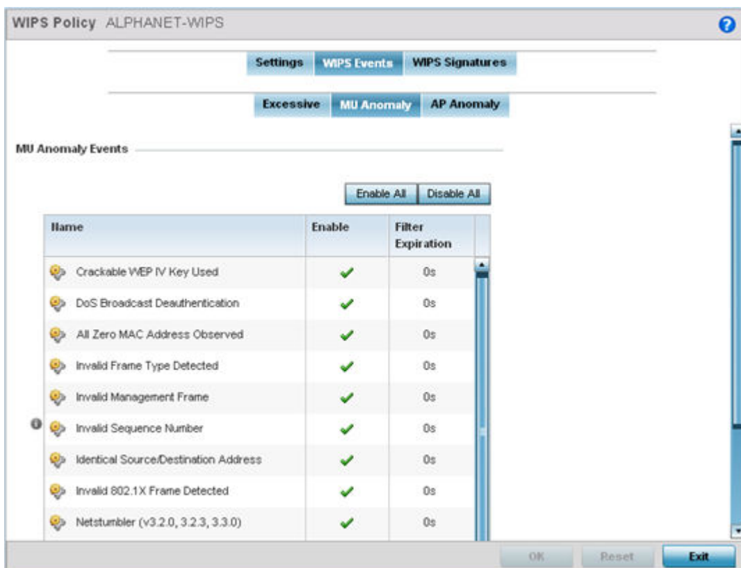
Figure 374: Wireless IPS Screen - WIPS Events - MU Anomaly Tab
