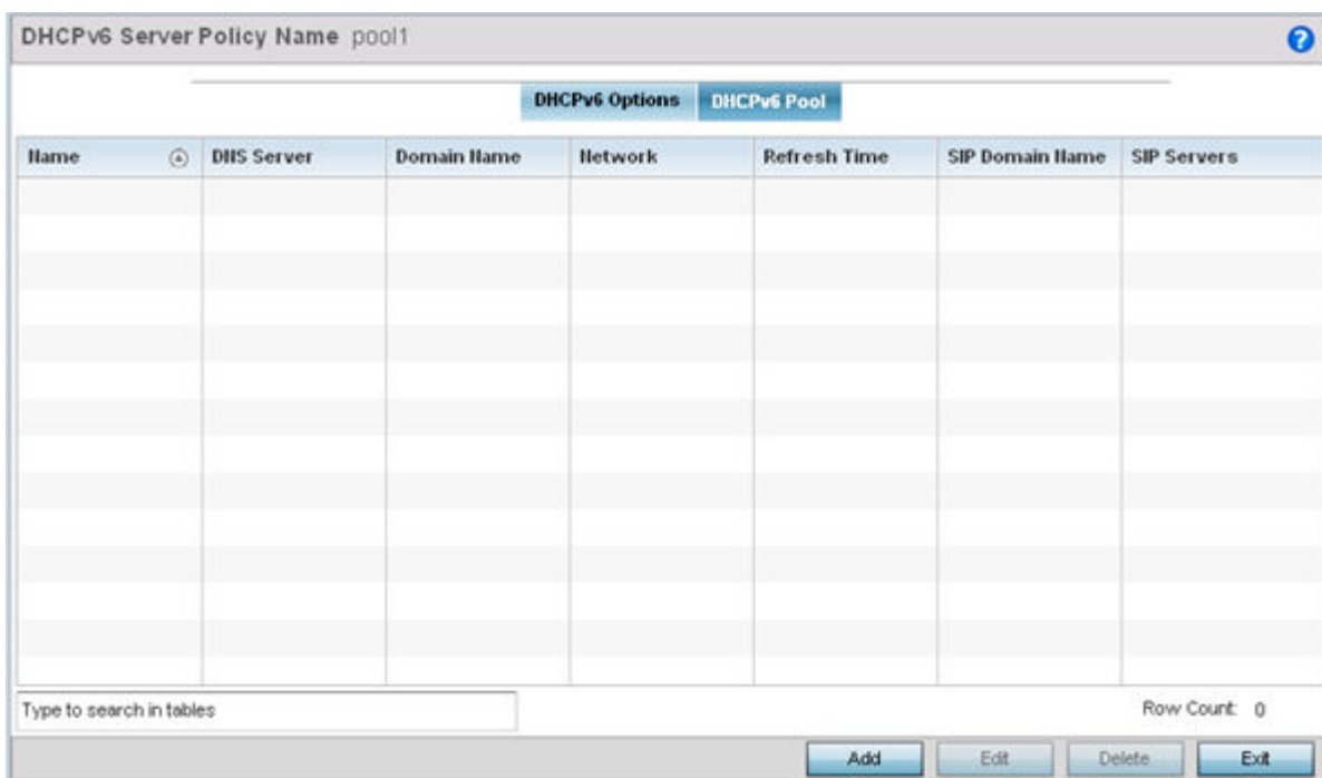
Figure 403: DHCP Server Policy - DHCPv6 Pool Tab
