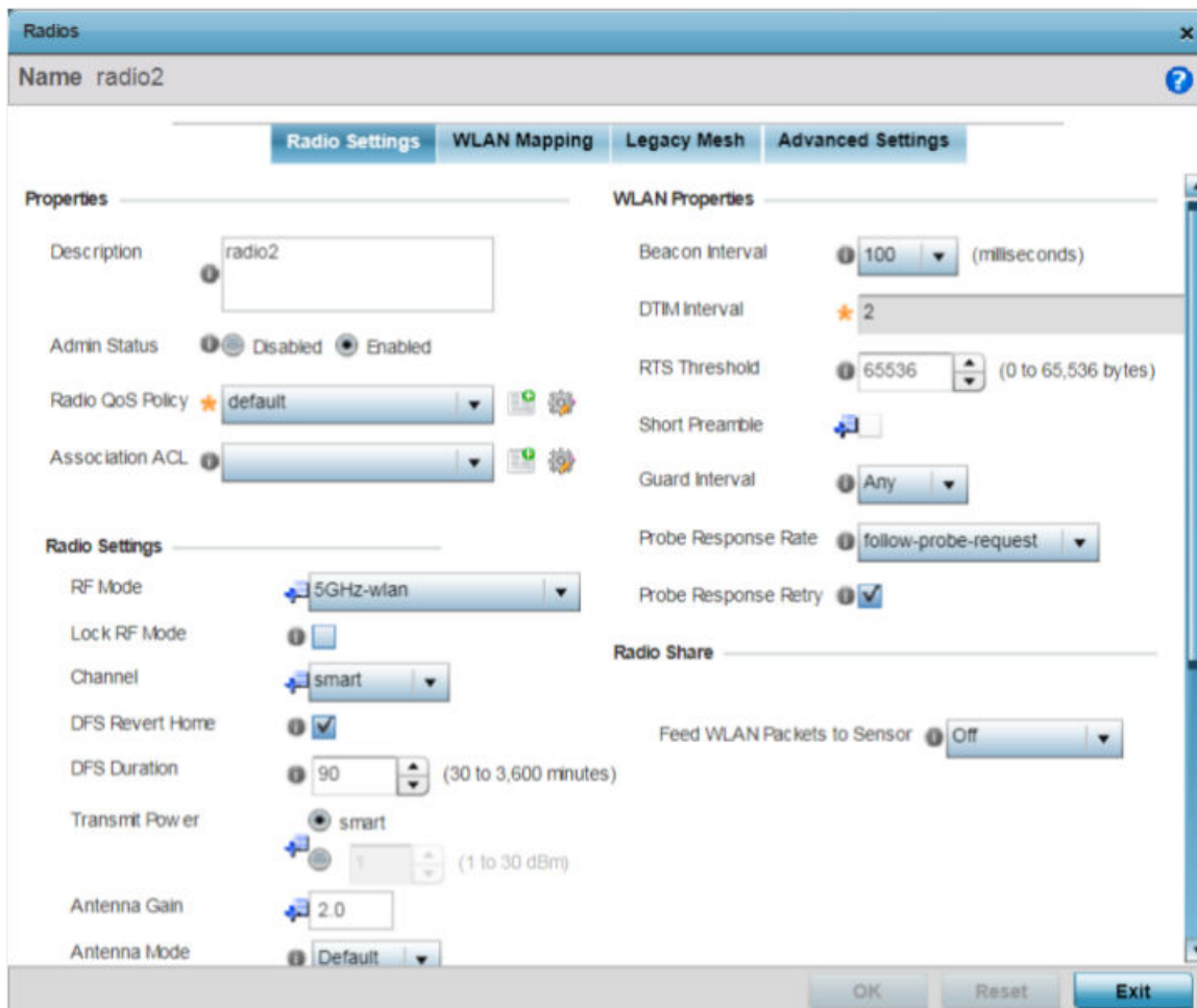
Figure 166: Radio Interface - Radio Settings Screen
