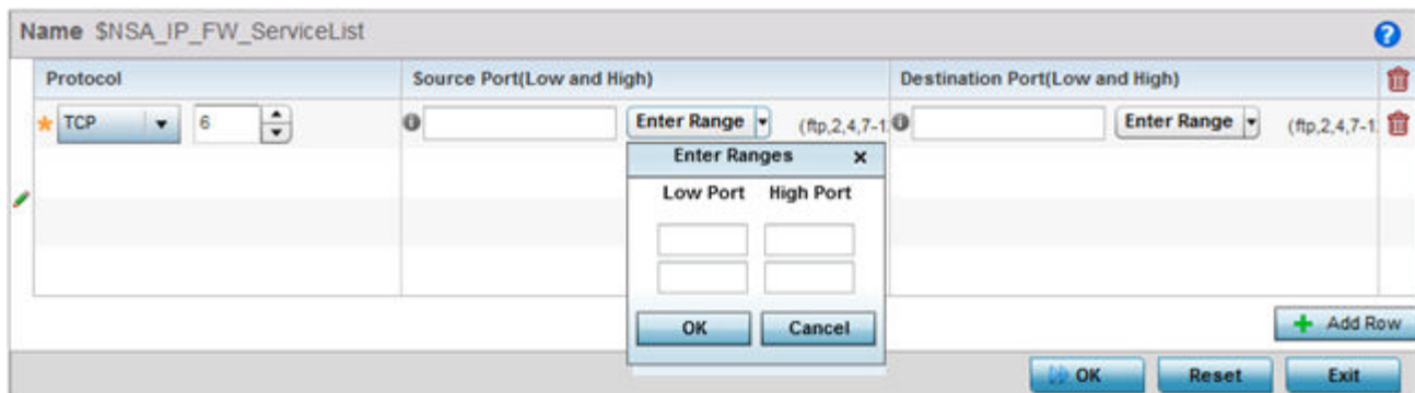
Figure 357: IP Firewall Network Service Alias - Add/Edit Screen
