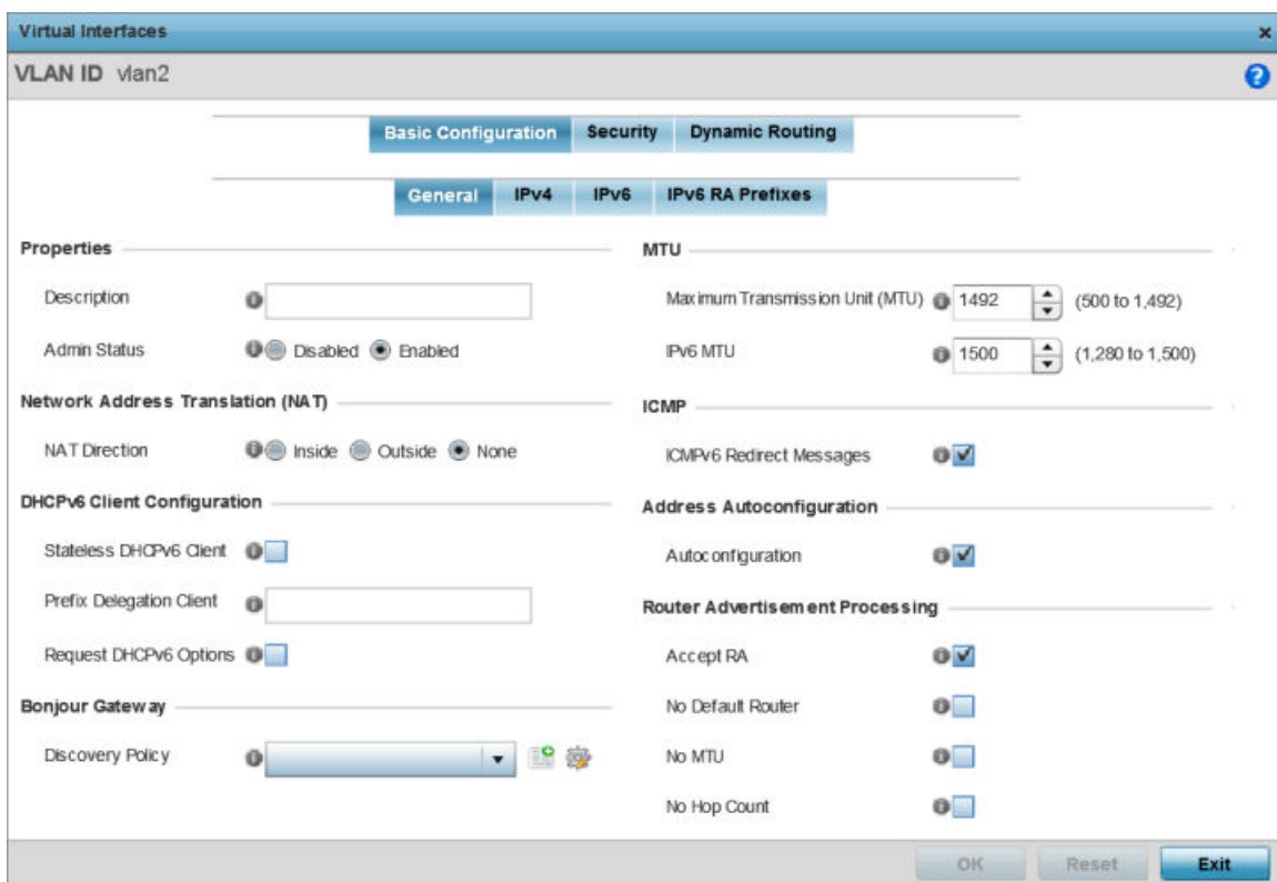
Figure 196: OSPF - VLAN Interface Configuration Screen
