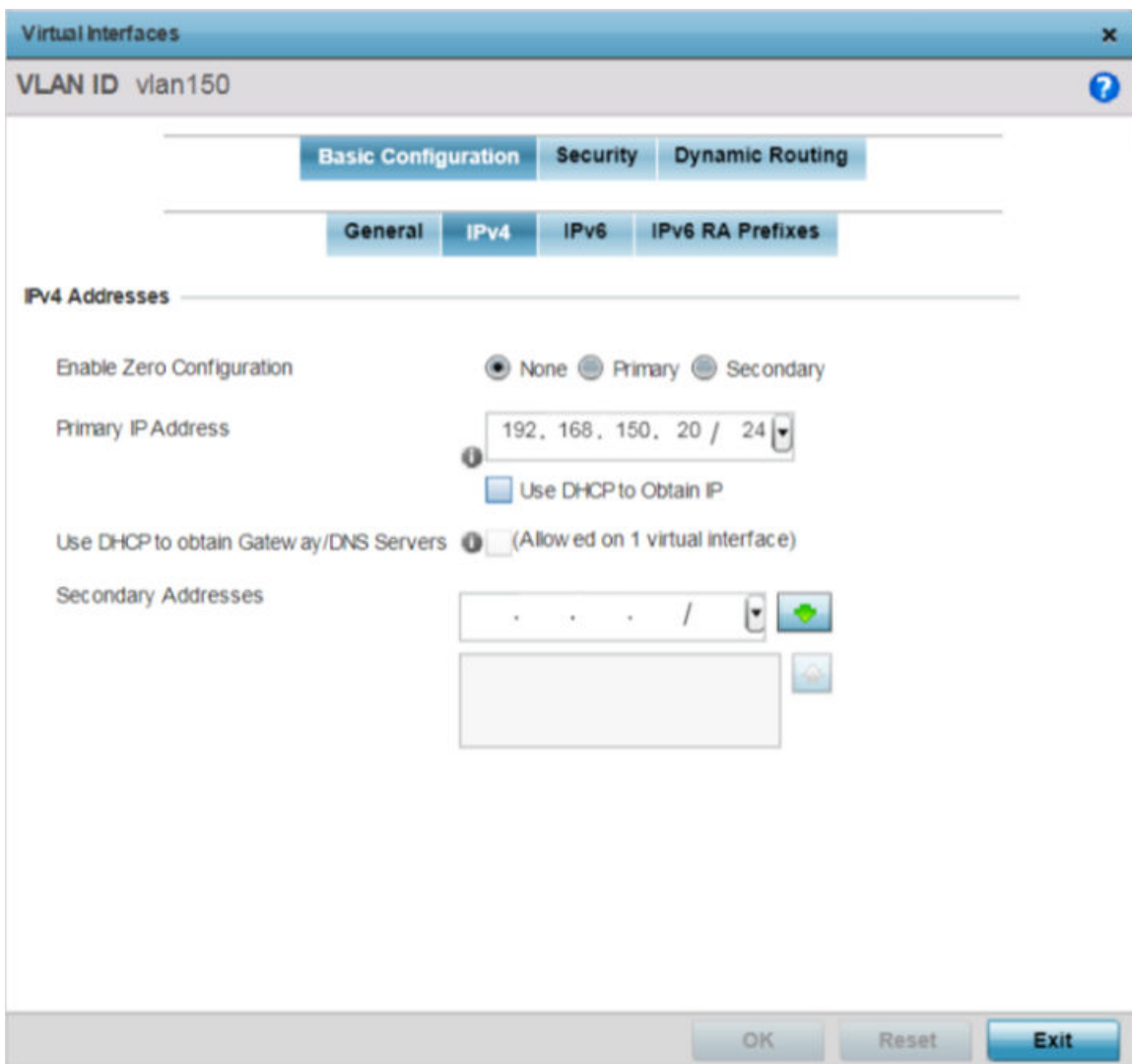
Figure 30: Profile Overrides - Virtual Interfaces Basic Configuration Screen - IPv4 Tab
