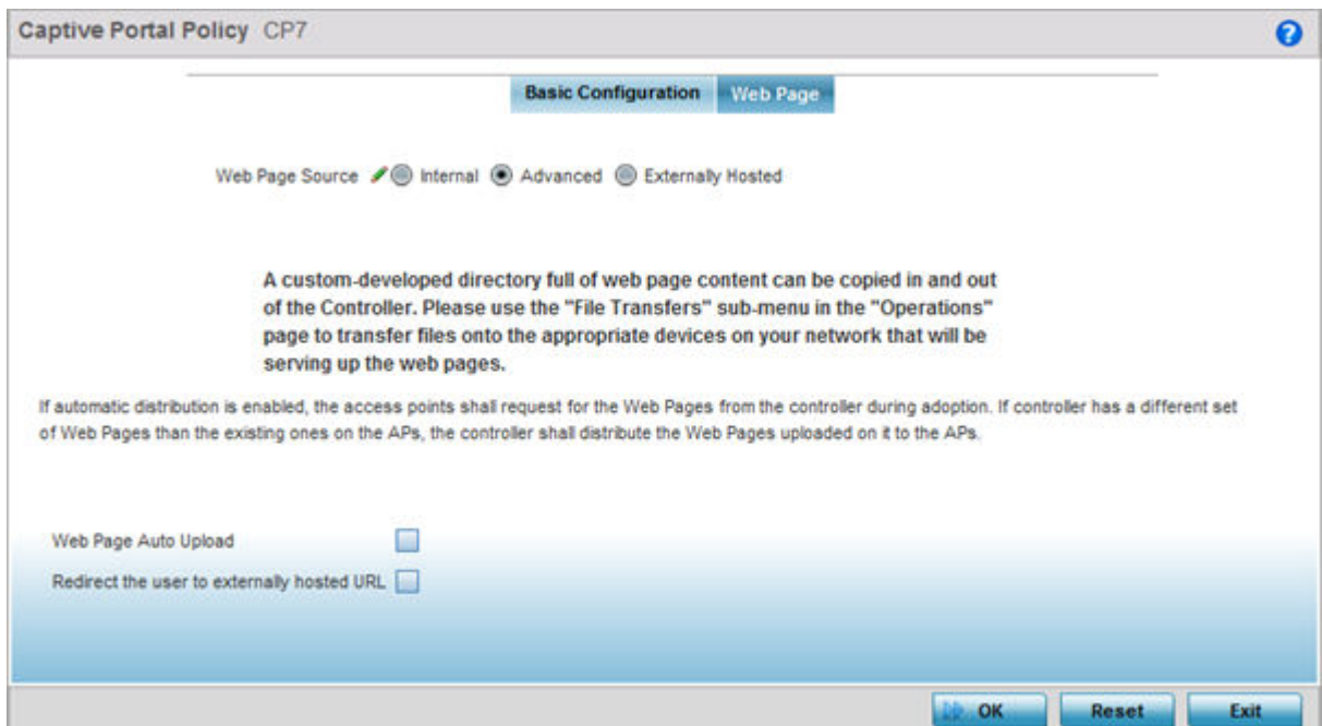
Figure 386: Captive Portal Policy - Web Page Screen - Advanced Option
