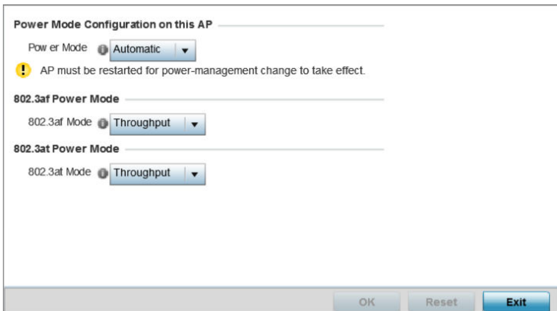
Figure 144: Device Configuration - System Profile - Power Screen
