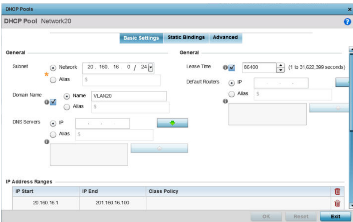
Figure 390: DHCP Pools - Add/Edit - Basic Settings Tab
