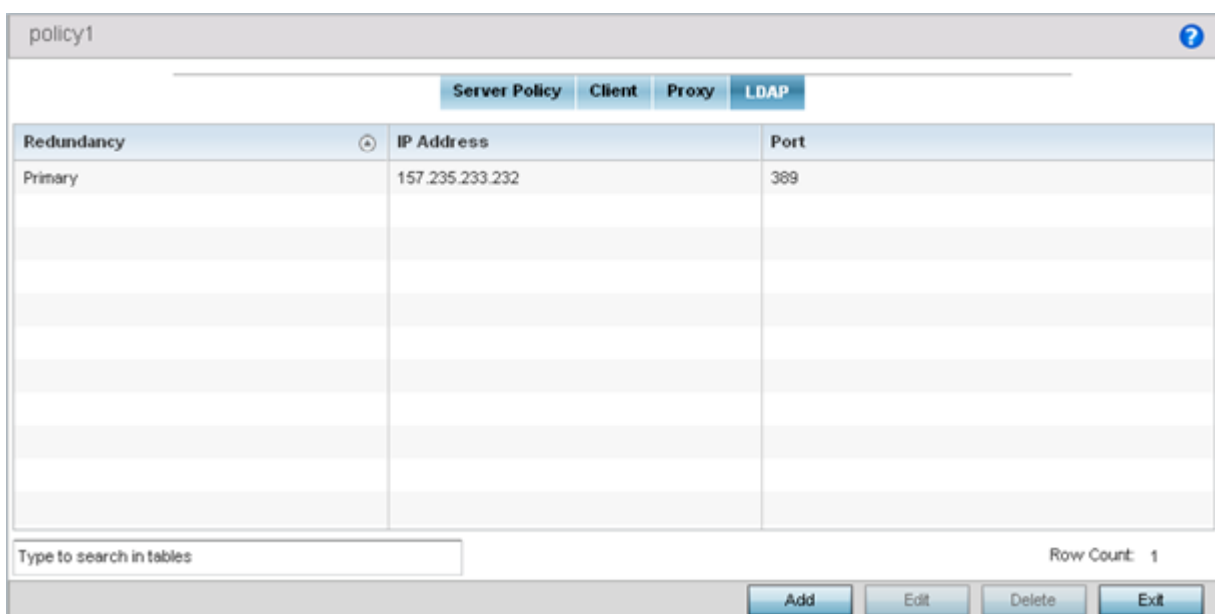
Figure 413: RADIUS Server Policy Screen - LDAP Tab
