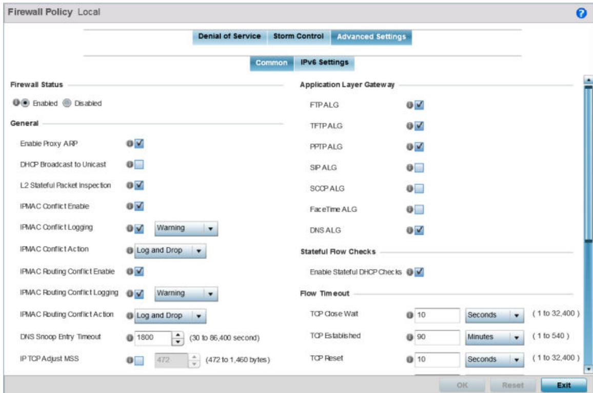
Figure 346: Wireless Firewall - Add/Edit - Advanced Settings - Common Tab
