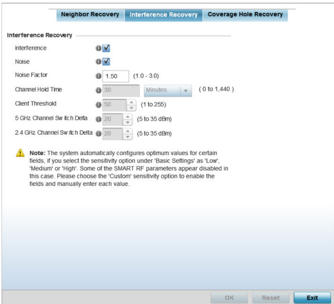
Figure 318: SMART RF - Advanced Configuration Screen - Interference Recovery Tab
