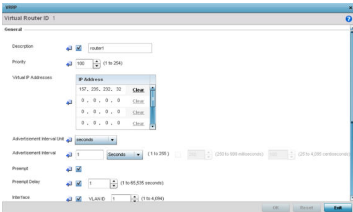
Figure 241: Device Overrides - VRRP - Virtual Router Screen
