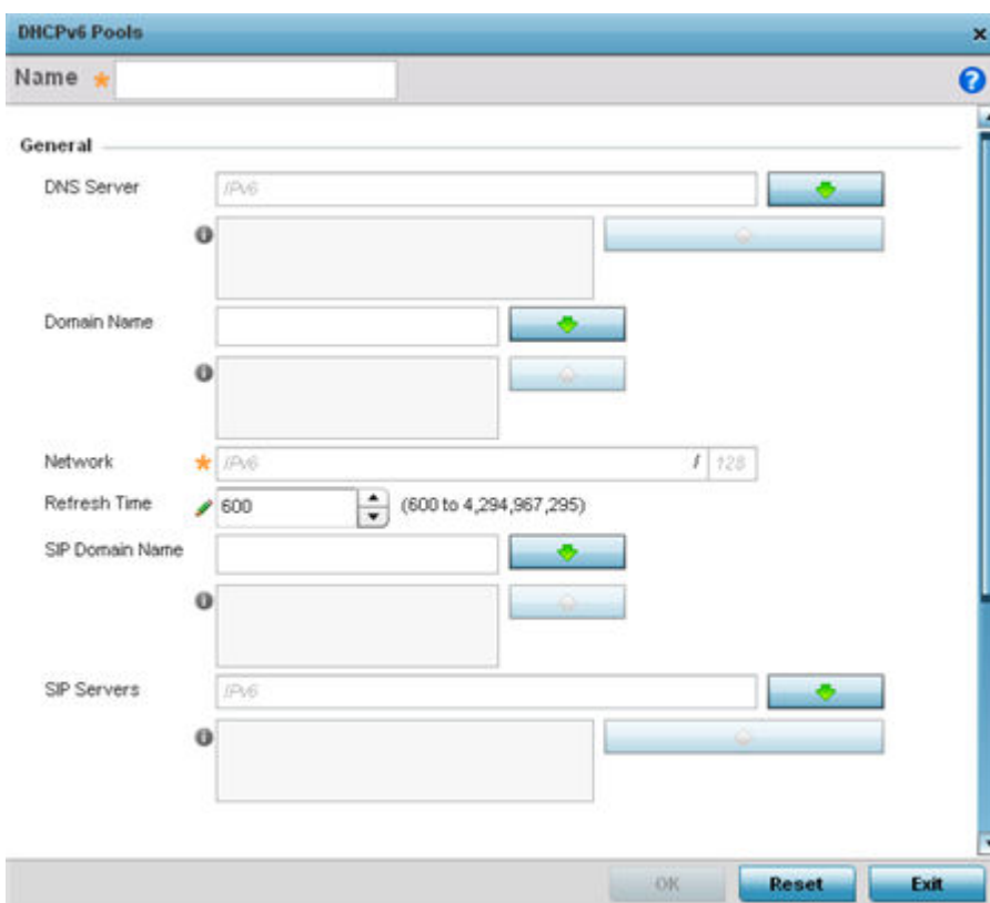
Figure 404: DHCP Server Policy - DHCPv6 Pool - Add/Edit Screen
