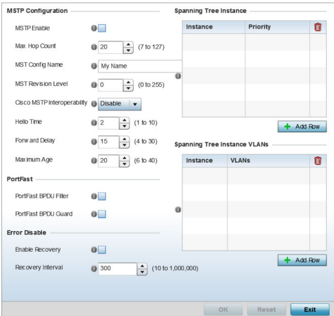
Figure 188: Spanning Tree Configuration Screen
