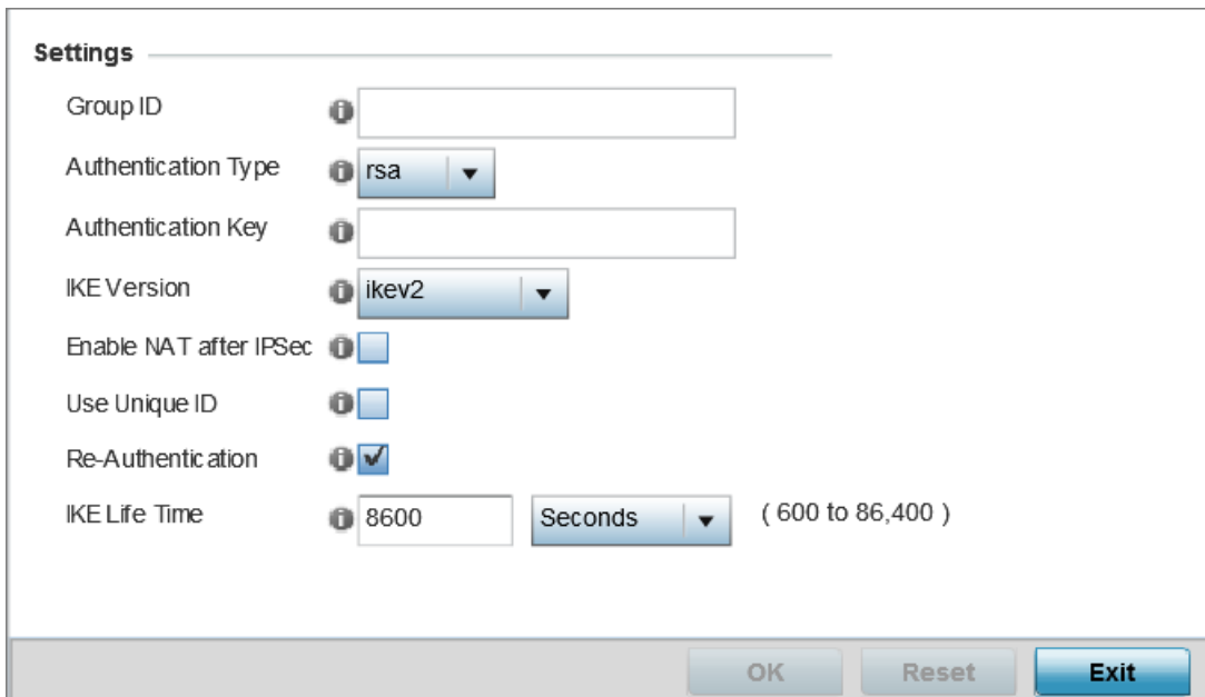
Figure 223: Profile Overrides - Security - Auto IPsec Tunnel Configuration Screen
