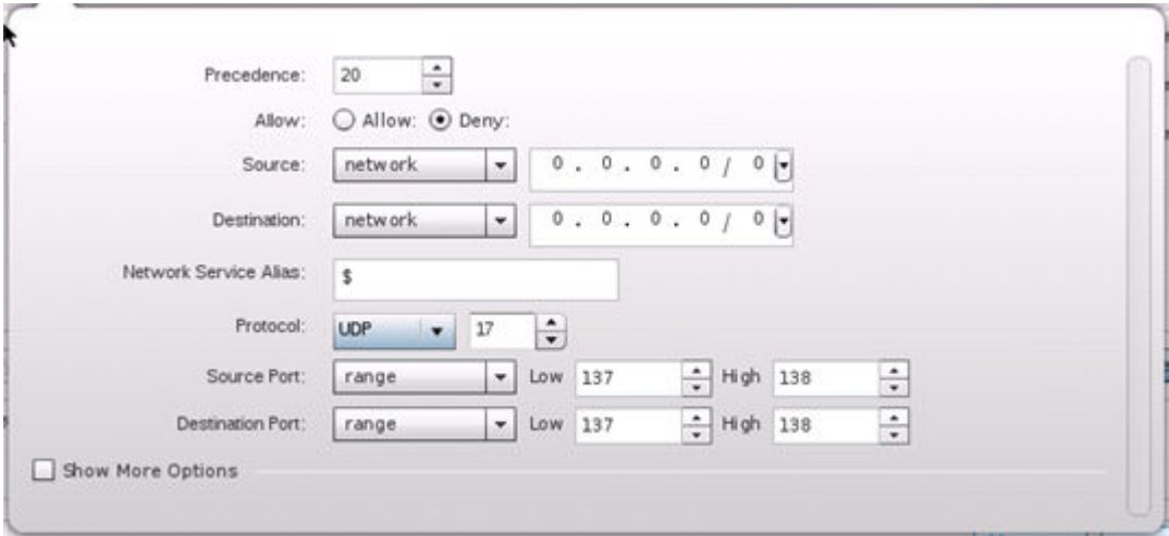
Figure 349: WLAN Security - IP Firewall Rules - Edit Rule Screen
