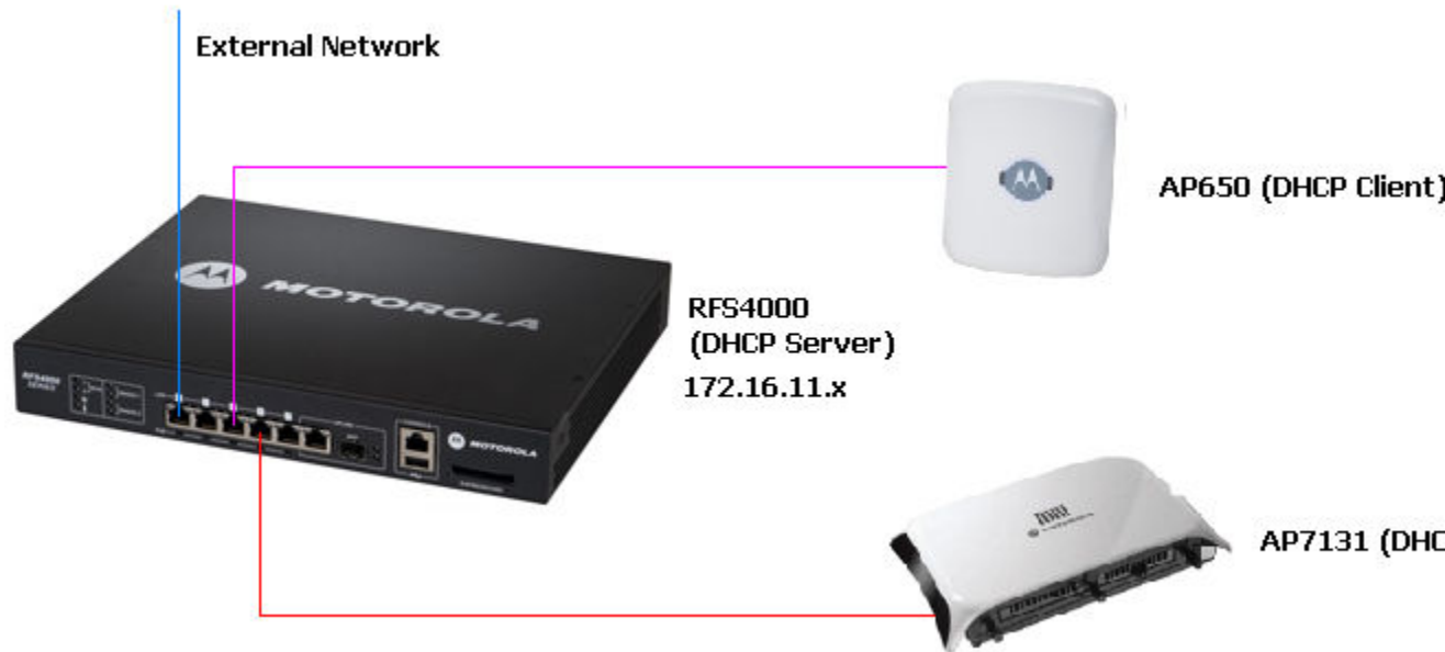
Figure 2: Network Design
