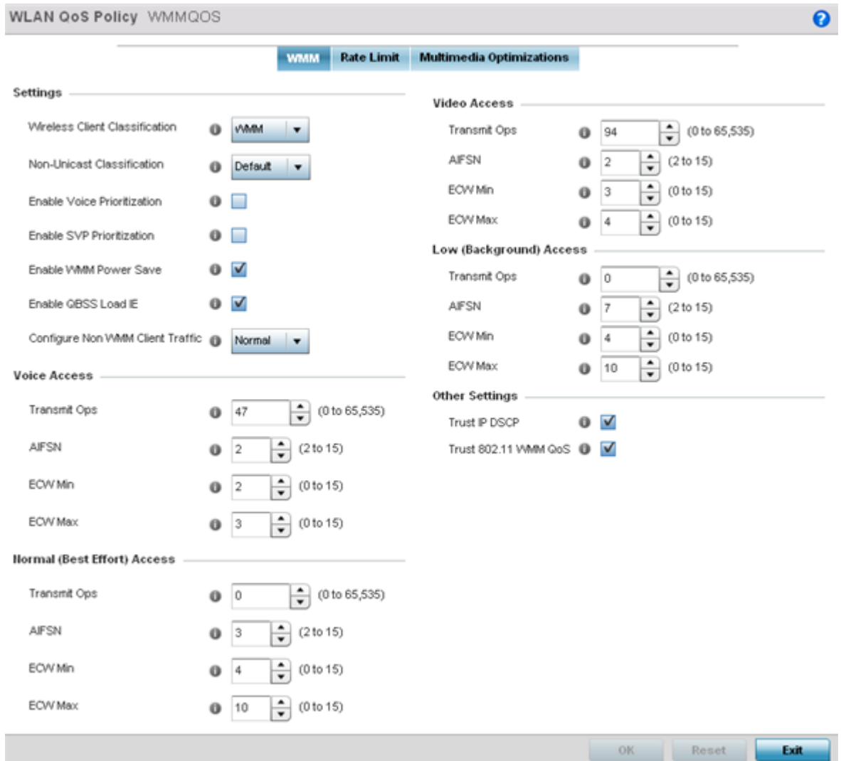
Figure 304: WLAN QoS Policy Screen - WMM Tab
