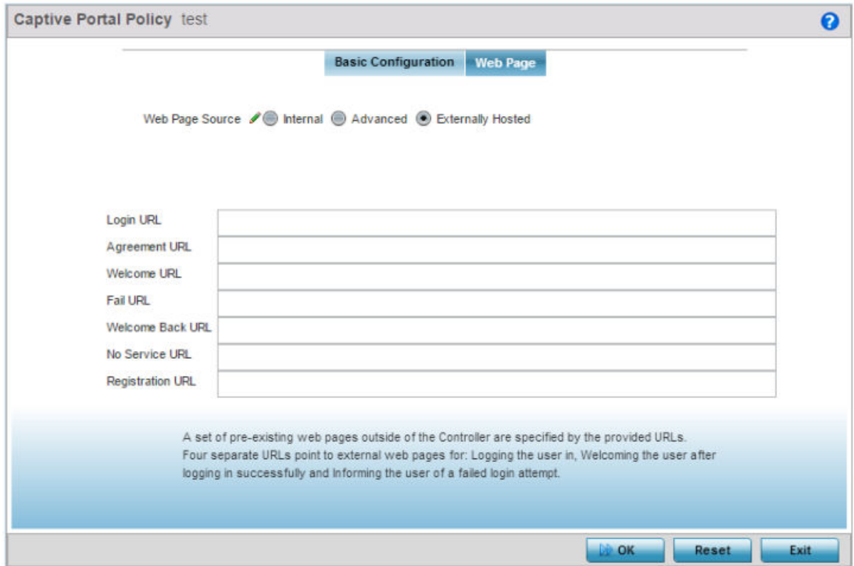
Figure 387: Captive Portal Policy Screen - Web Page Tab - Externally Hosted Web Page Screen
