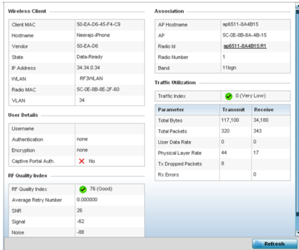
Figure 438: Wireless Client - Statistics - Health Screen
