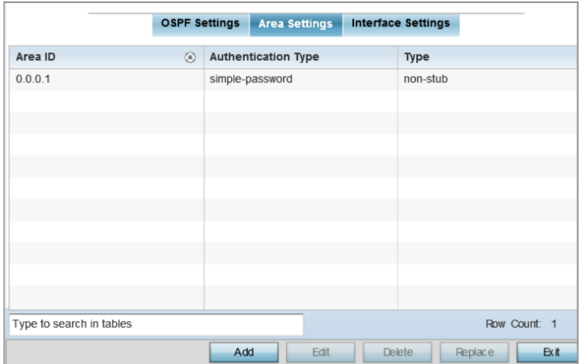
Figure 193: OSPF - Area Setting Configuration Screen
