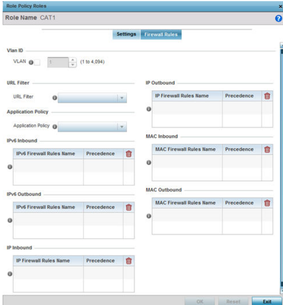
Figure 361: Wireless Client Roles - Add/Edit - Roles - Firewall Rules Tab
