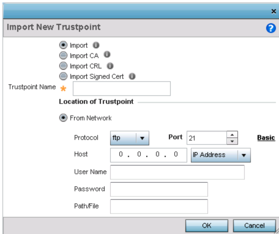
Figure 133: Import New Trustpoint Window
