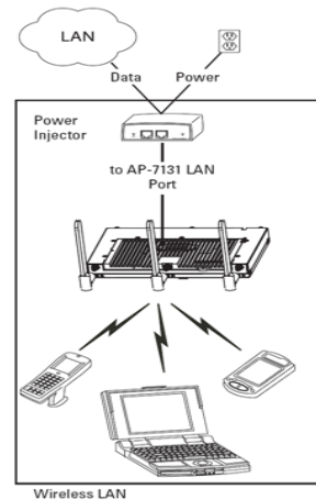
Figure 1 AP-PSBIAS-1P3-AFR Power Injector
