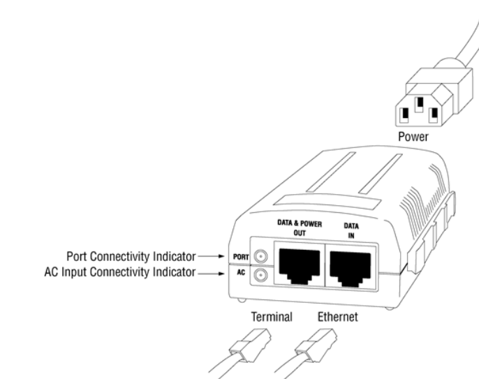
Figure 3 Cabling the Power Injector
