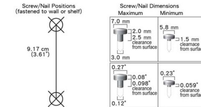
Figure 2 Screw and nail positions
