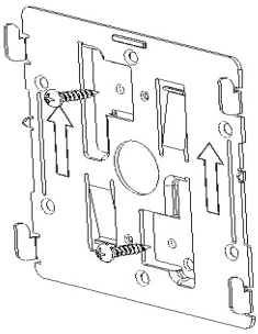
Figure 1 Attaching Mounting Bracket to the Wall
