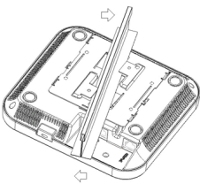
Figure 3 Rotating the AP-7532/AP-7532I (internal antenna) chassis 45 degrees counter-clockwise
