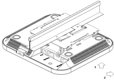
Figure 2 Installing AP-7532/AP-7532I (internal antenna) on the T-bar
