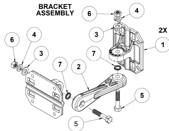
Figure 3 Mast Mount Configuration
