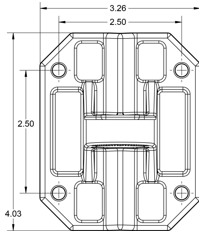
Figure 1 HDMNT Bracket
