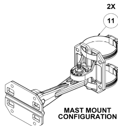
Figure 3 Mast Mount Configuration
