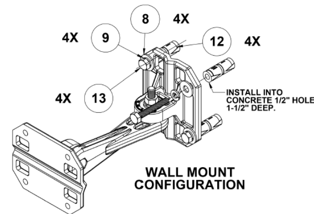
Figure 5 Wall Mount Configuration
