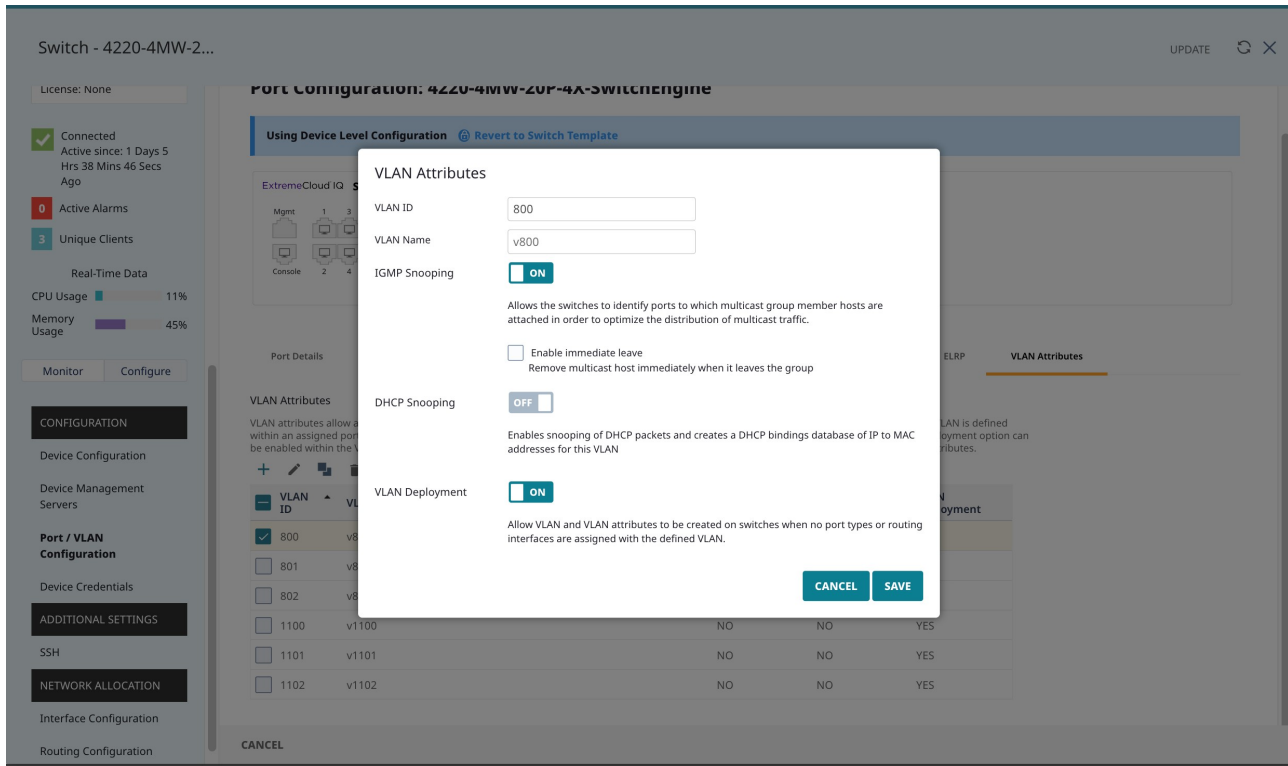
Figure 16: VLAN Attributes
