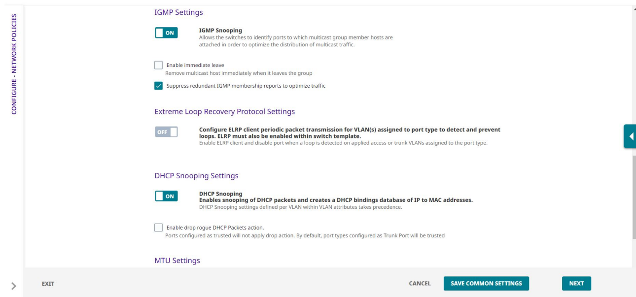
Figure 10: DHCP Snooping Network Policy
