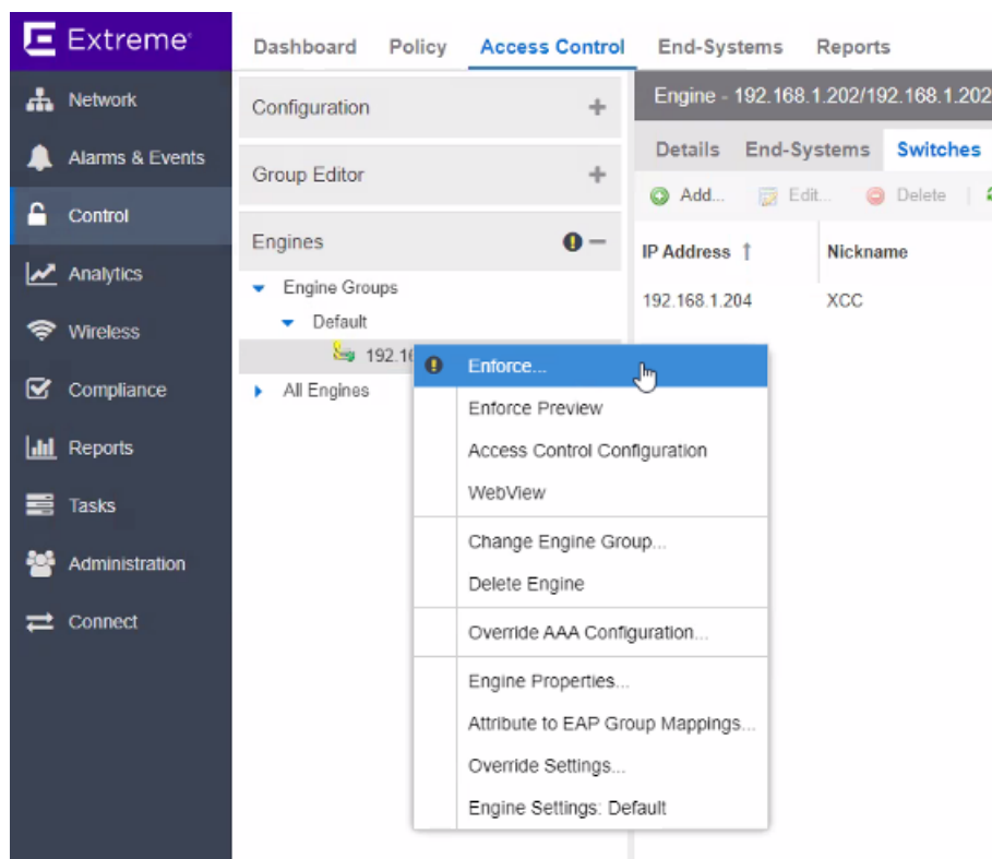
Figure 73: Enforce Changes
