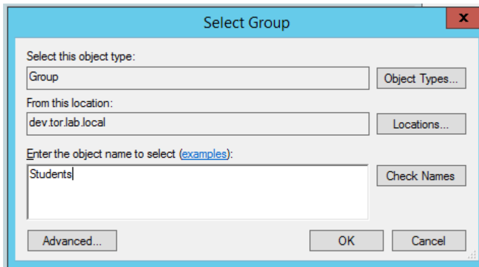
Figure 21: Select Group
