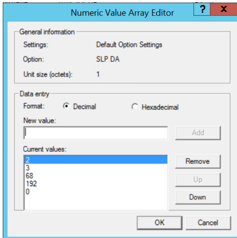
Figure 6: DHCP Option 78 Array Decimal Values
