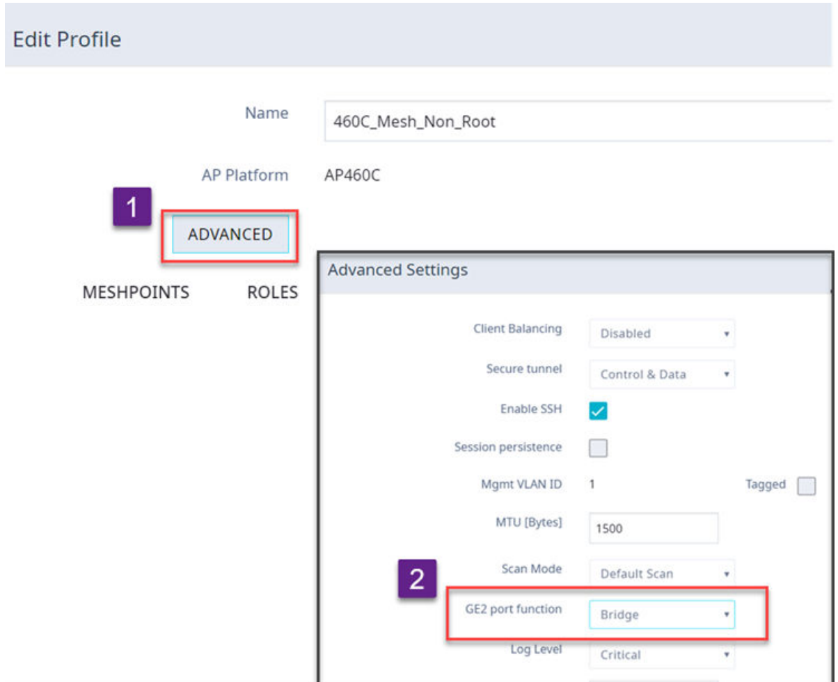
Figure 32: Configure Transparent Bridge from Device Group Configuration Profile
