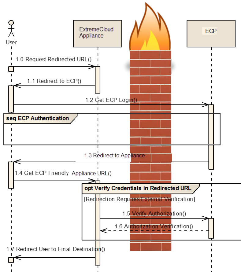
Figure 34: Firewall Friendly ECP Event Flow with ExtremeCloud IQ Controller
