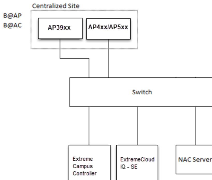
Figure 33: External NAC Server / ExtremeCloud IQ Controller Setup
