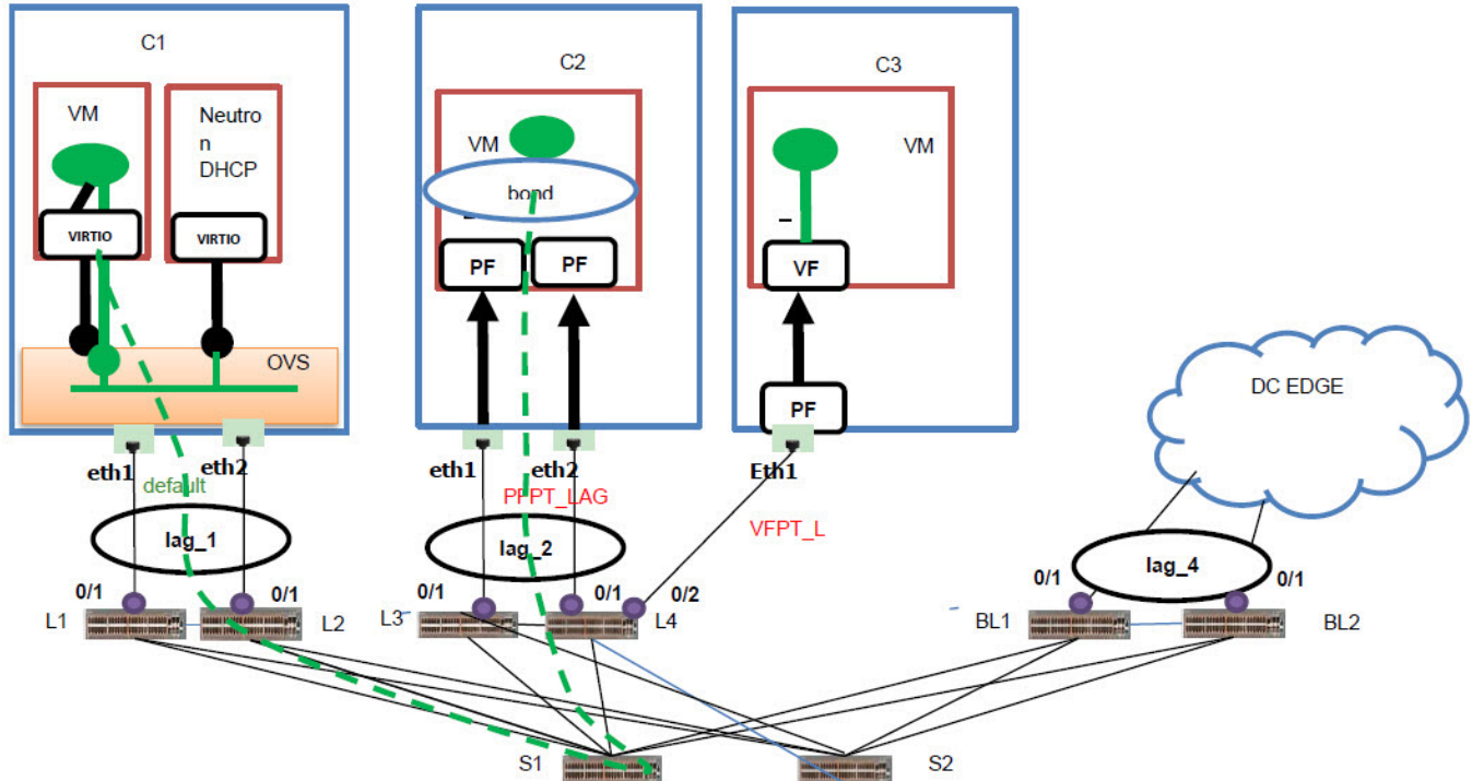
Figure 12: Overview of Virtio VM, PFPT, and VFPT segment network with DC Edge
