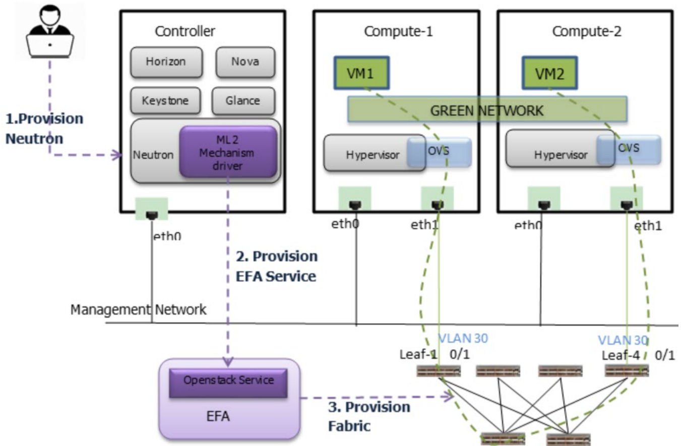
Figure 8: Overview of ML2 Mechanism Driver within Neutron
