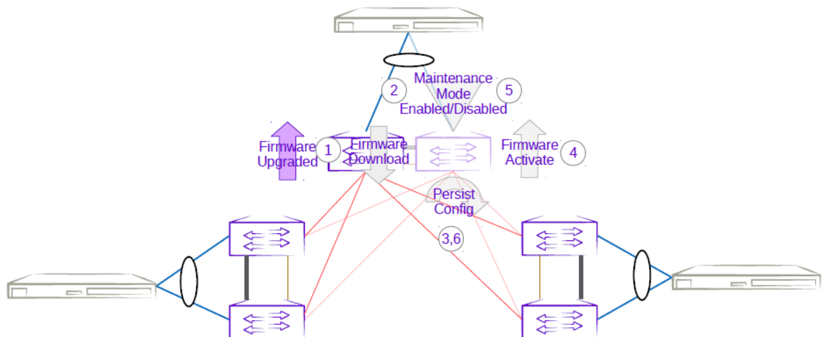
Figure 35: Three-rack centralized second MCT leaf firmware upgrade with maintenance mode
