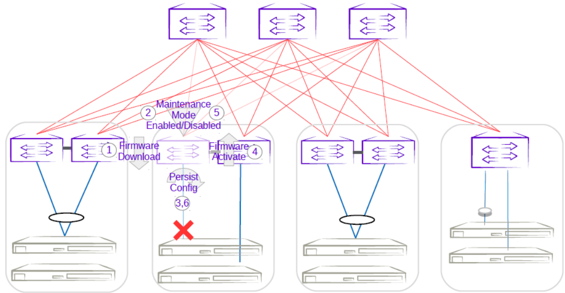
Figure 46: Single-homed server traffic loss
