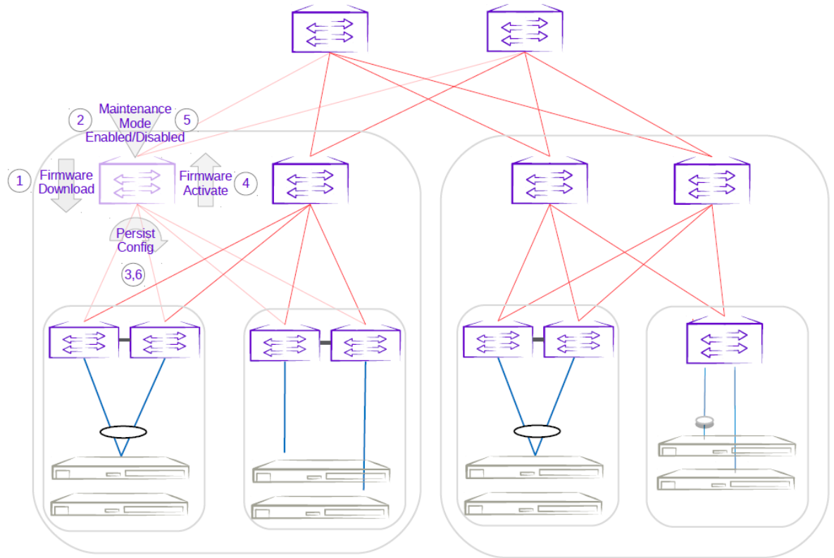
Figure 30: First spine firmware upgrade with maintenance mode
