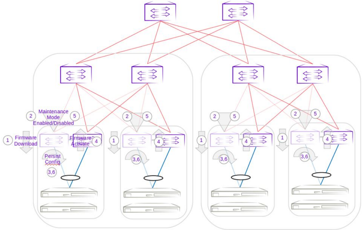
Figure 39: Group 1 - Firmware download execution of lower IP address MCT Peer leaf devices
