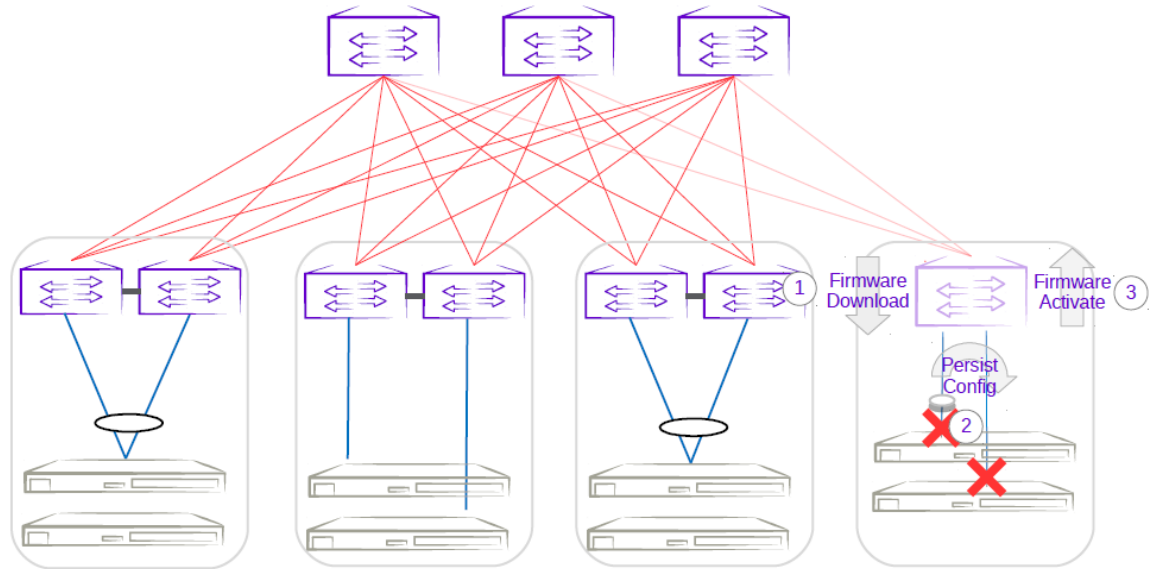
Figure 45: Single-leaf traffic loss
