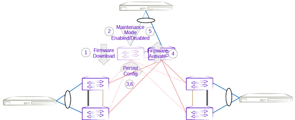
Figure 34: Three-rack centralized first MCT leaf firmware upgrade with maintenance mode
