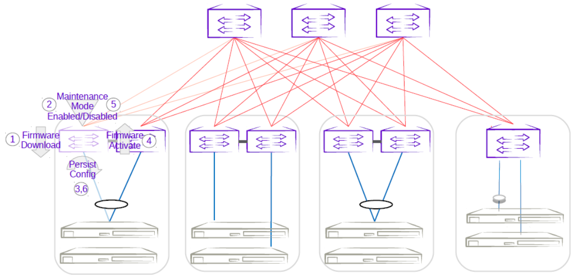
Figure 32: First MCT leaf firmware upgrade with maintenance mode
