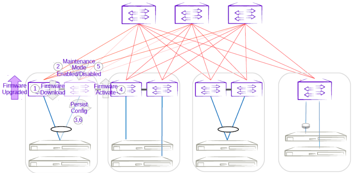
Figure 33: Second MCT leaf firmware upgrade with maintenance mode
