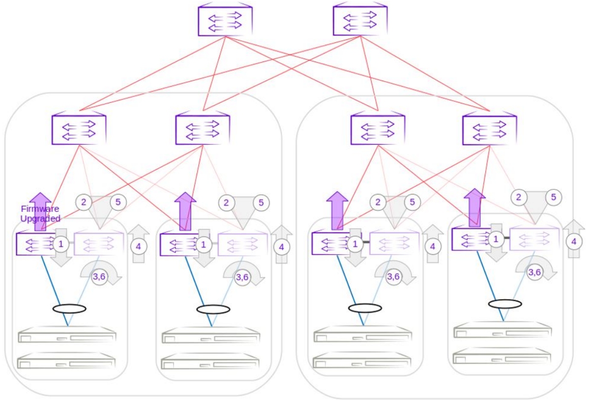
Figure 40: Group 2 - Firmware download execution of higher IP address MCT Peer leaf devices
