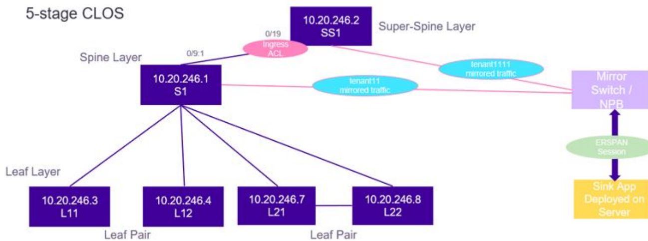
Figure 27: 5-stage Clos topology
