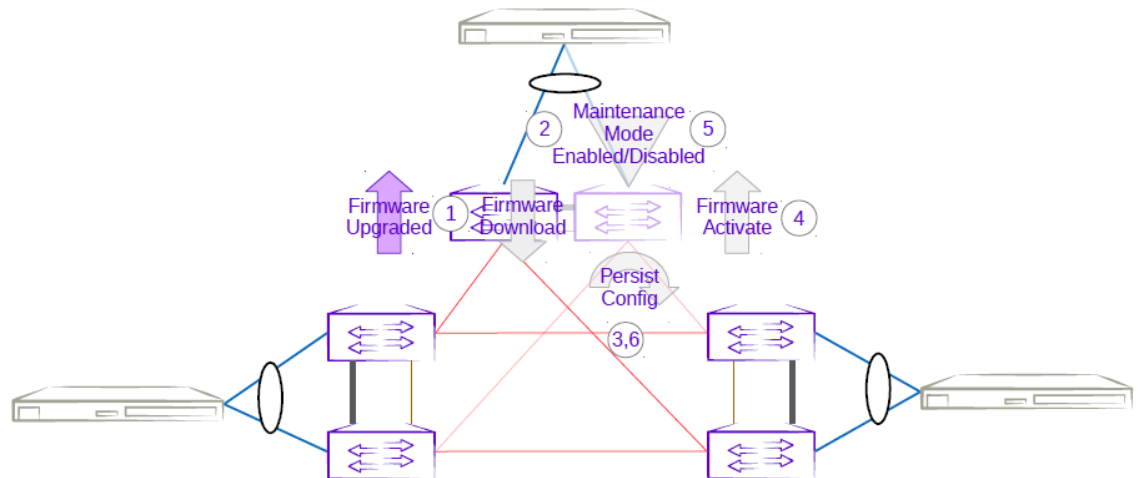
Figure 40: Three-rack ring second MCT leaf firmware upgrade with maintenance mode
