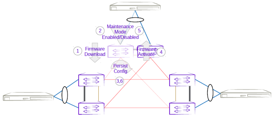
Figure 39: Three-rack ring first MCT leaf firmware upgrade with maintenance mode
