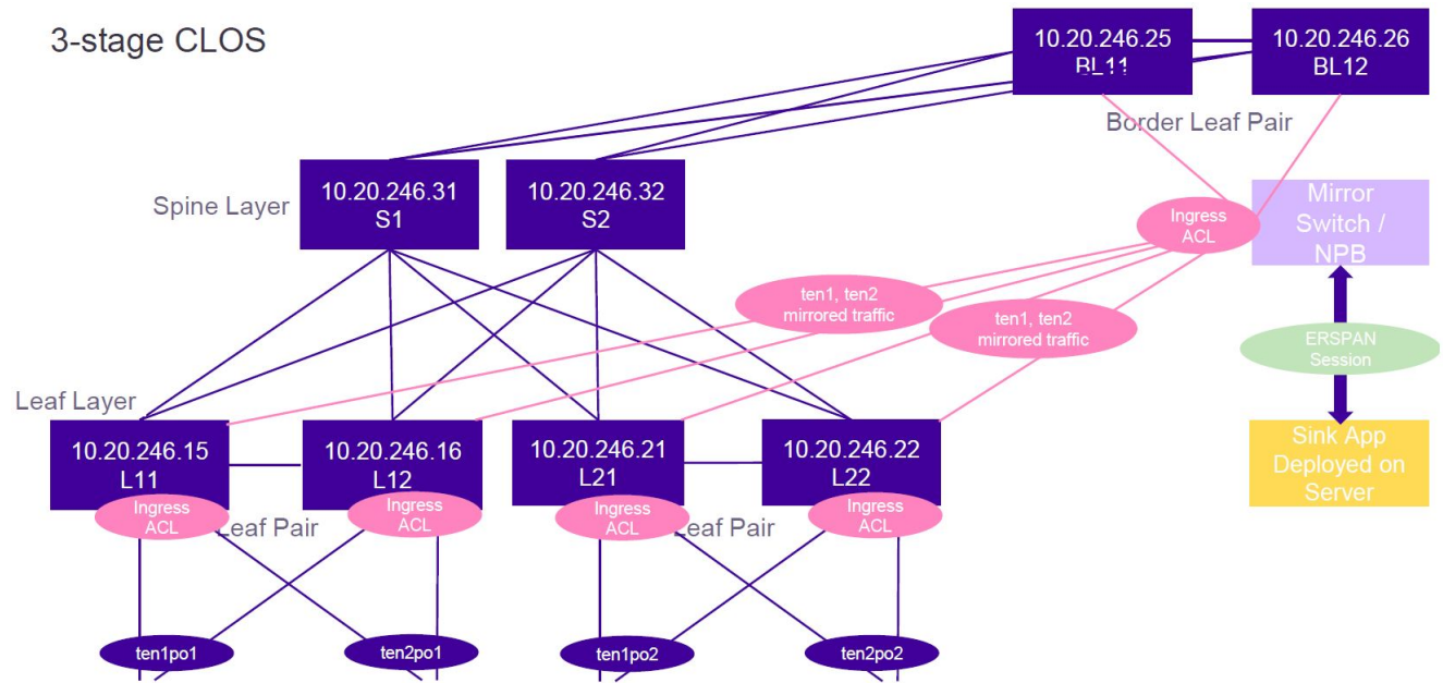
Figure 28: VLAN-based traffic mirroring topology
