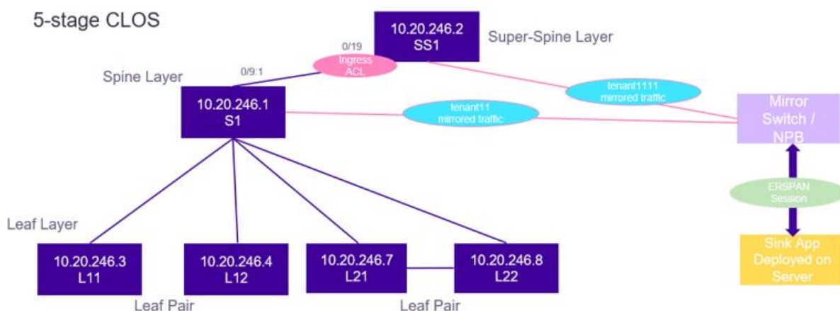
Figure 30: 5-stage Clos topology
