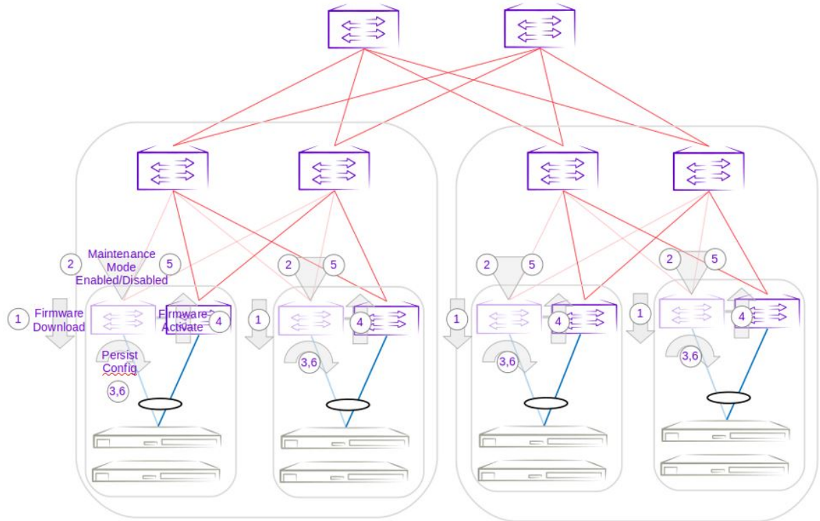
Figure 42: Group 1 - Firmware download execution of lower IP address MCT Peer leaf devices
