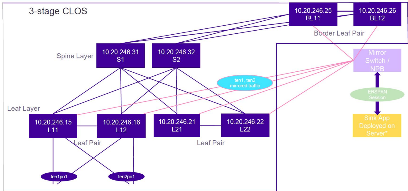
Figure 26: Port-based traffic mirroring topology
