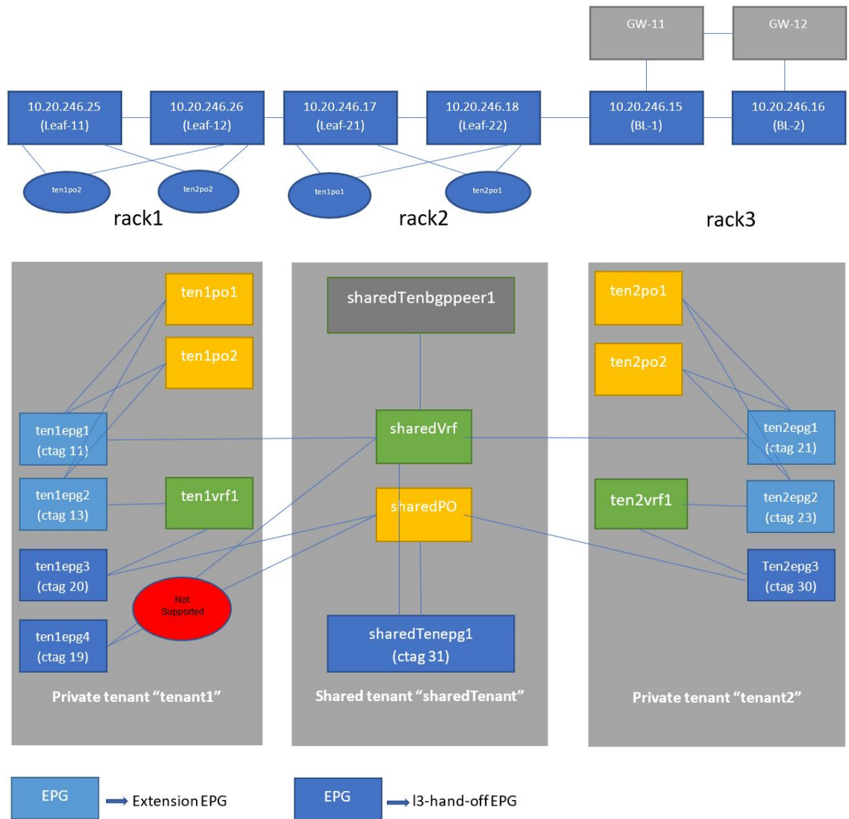
Figure 23: Shared VRF Configuration Overview
