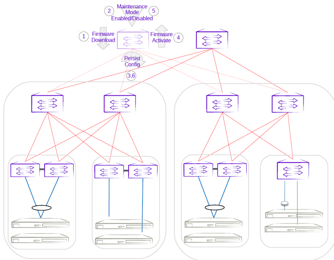
Figure 31: First super-spine firmware upgrade with maintenance mode
