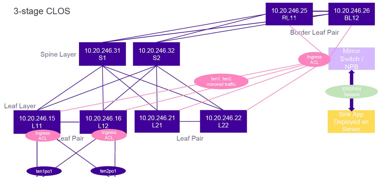
Figure 27: Flow-based traffic mirroring topology
