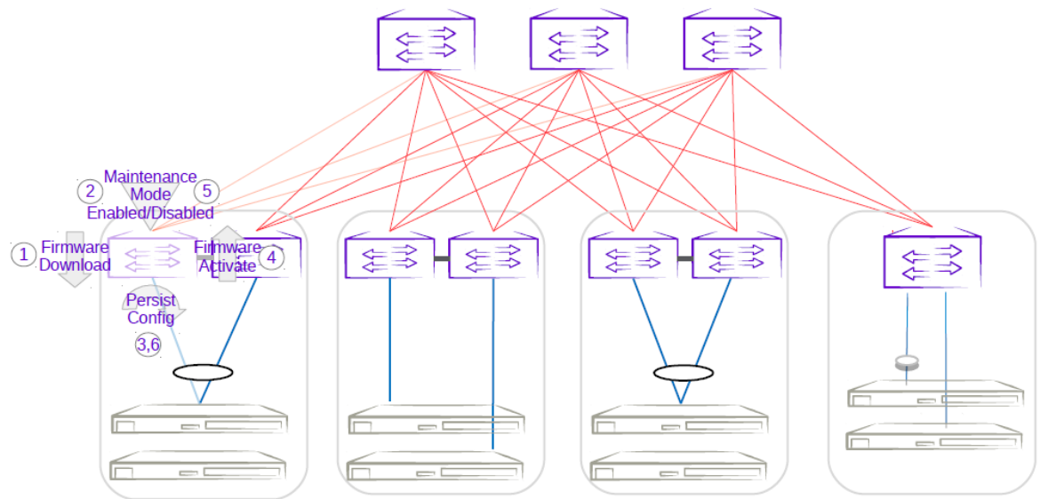
Figure 35: First MCT leaf firmware upgrade with maintenance mode
