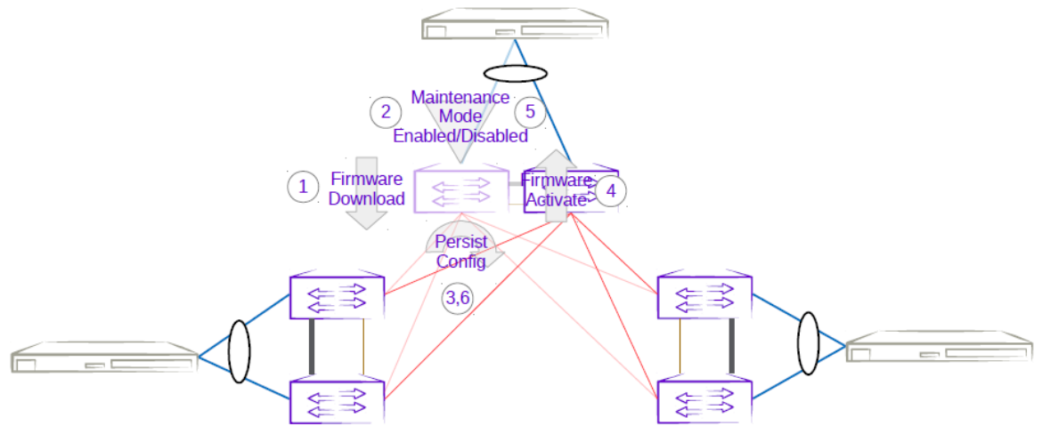
Figure 37: Three-rack centralized first MCT leaf firmware upgrade with maintenance mode
