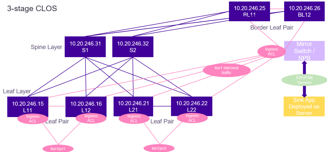
Figure 29: ICL port traffic mirroring topology
