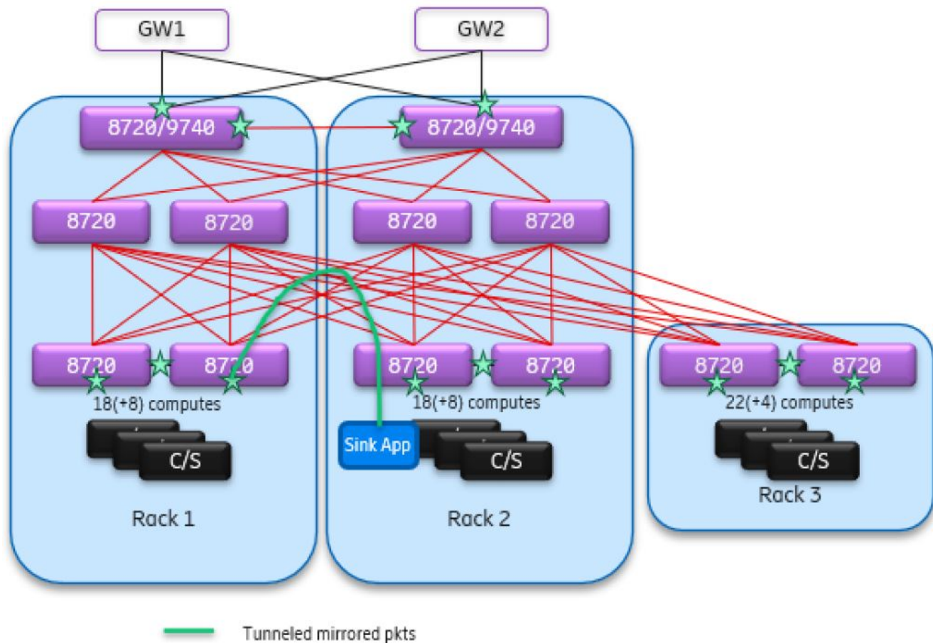
Figure 24: In-band traffic mirroring topology
