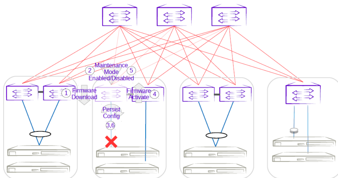
Figure 49: Single-homed server traffic loss
