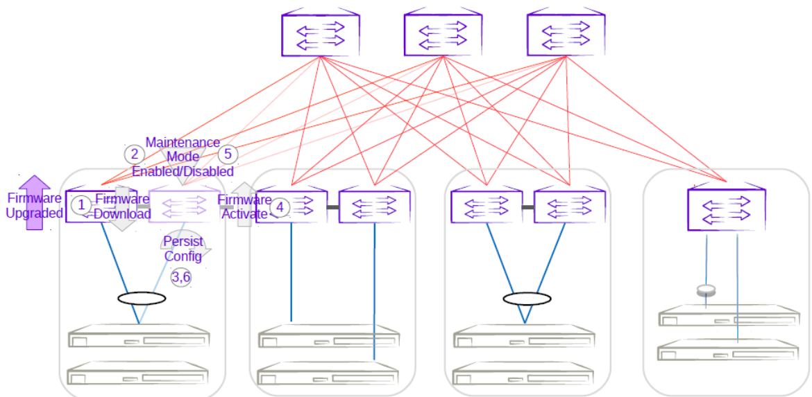
Figure 36: Second MCT leaf firmware upgrade with maintenance mode
