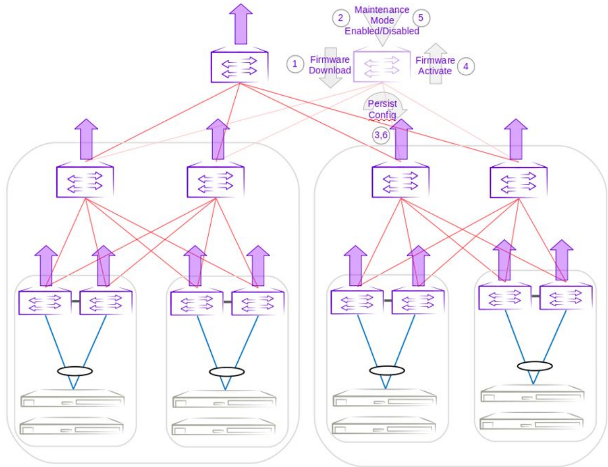
Figure 47: Group 6 - Firmware download execution of highest IP address super-spine device
