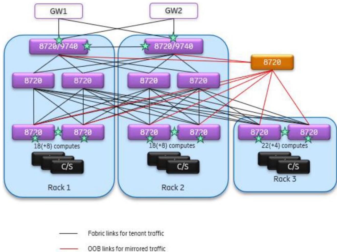
Figure 25: Out-of-band traffic mirroring topology
