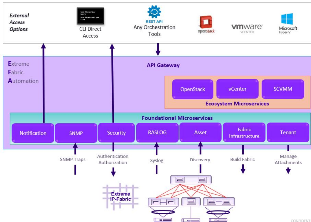
Figure 1: EFA orchestration
