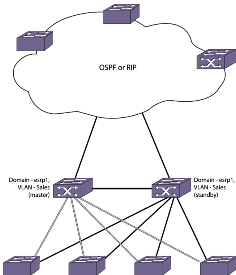
Figure 176: Single ESRP Domain Using Layer 2 and Layer 3 Redundancy
