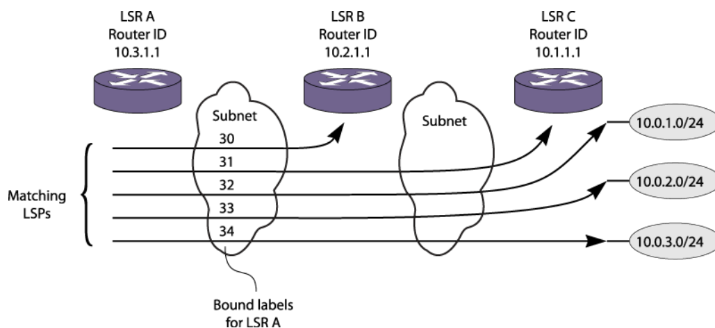
Figure 192: Matching and Calculated LSP Next Hops
