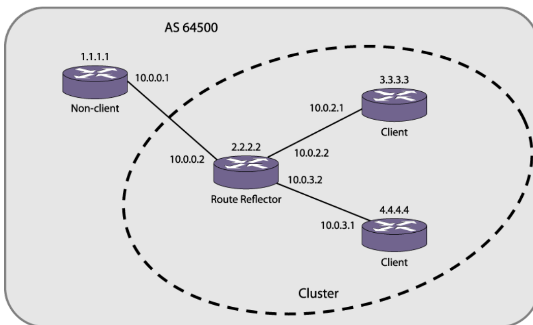
Figure 238: Route Reflectors
