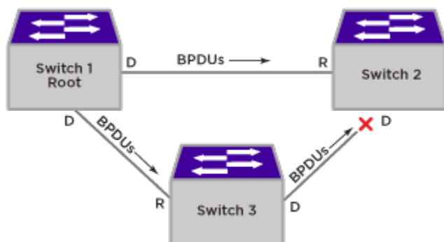
Figure 143: STP Disabled on Switch 2
