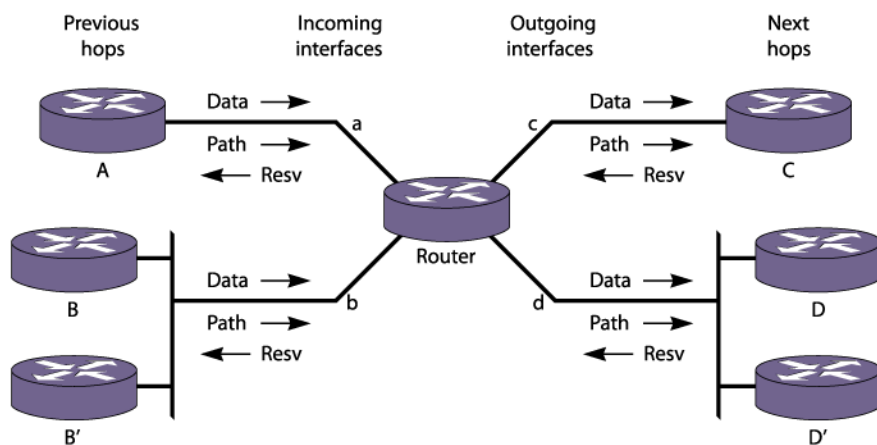
Figure 201: RSVP Messages
