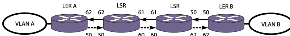
Figure 203: Static LSP Example
