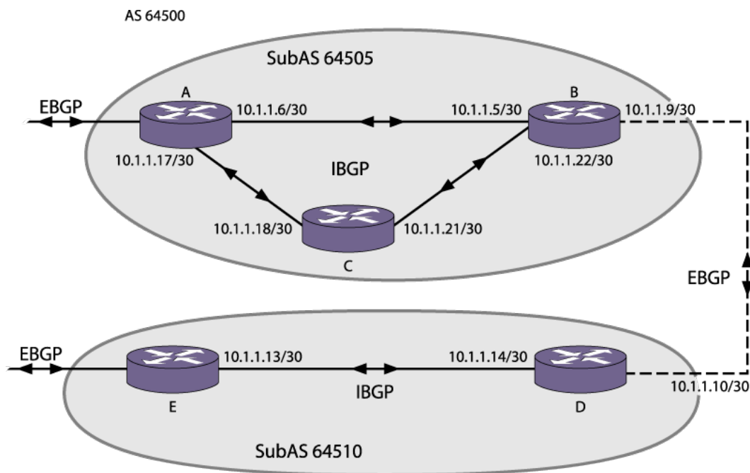
Figure 239: Routing Confederation
