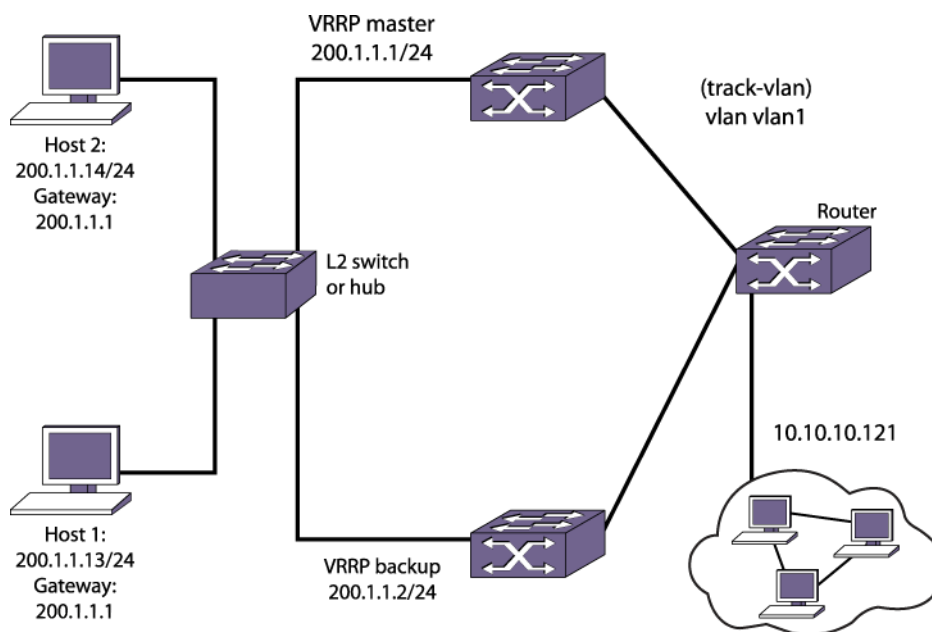
Figure 185: VRRP Tracking
