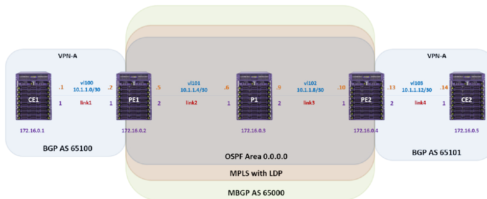
Figure 247: Layer 3 Virtual Private Network
