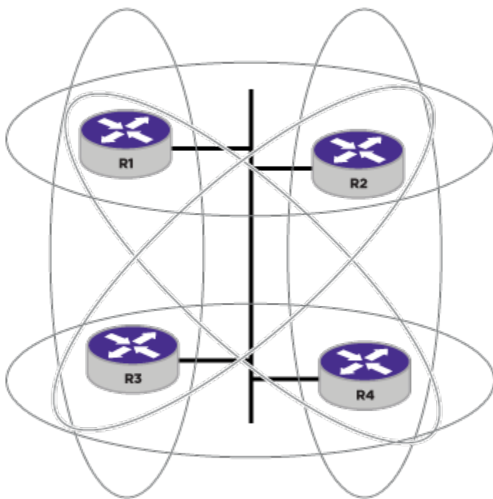
Figure 234: Point-to-Point Adjacencies in a Four-Router Network
