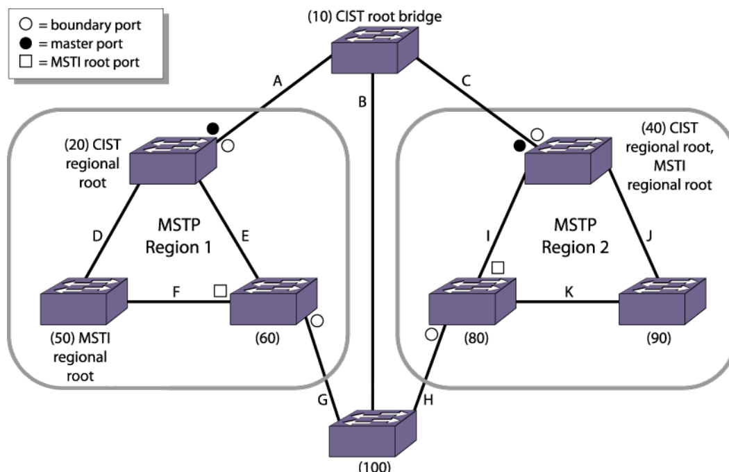
Figure 162: Sample MSTP Topology with Two MSTP Regions
