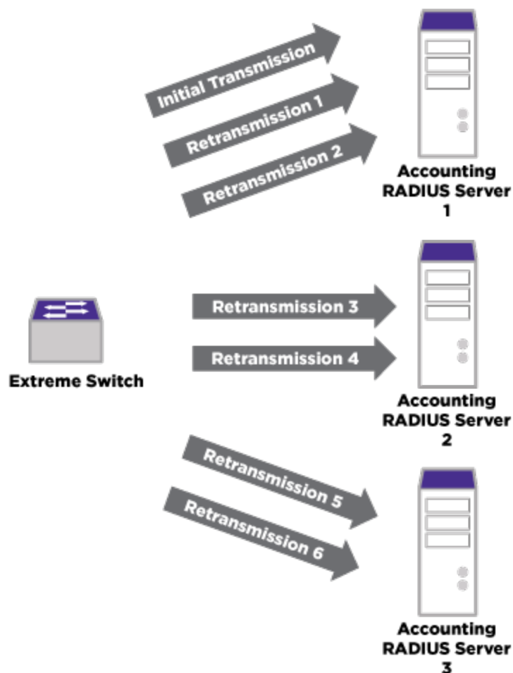
Figure 112: Accounting Retransmission Algorithm (No Servers Responding)
