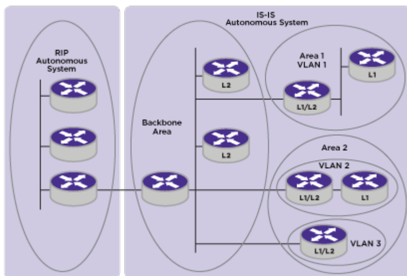
Figure 237: AS External Route Redistribution
