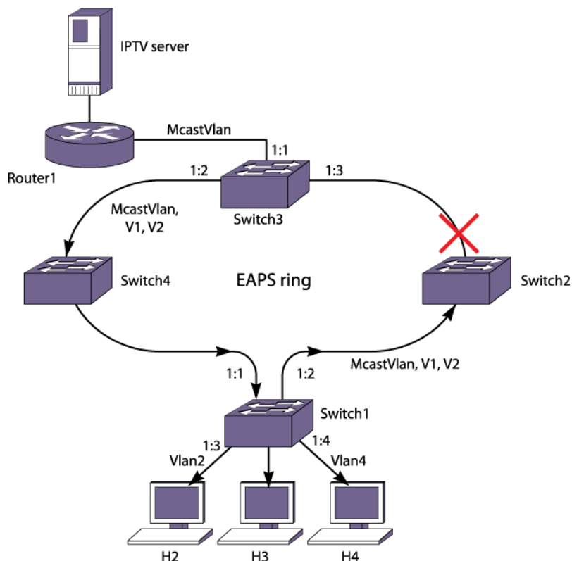
Figure 258: MVR on an EAPS Ring
