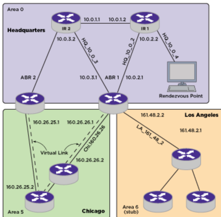
Figure 252: IP Multicast Routing Using PIM-SM Configuration Example
