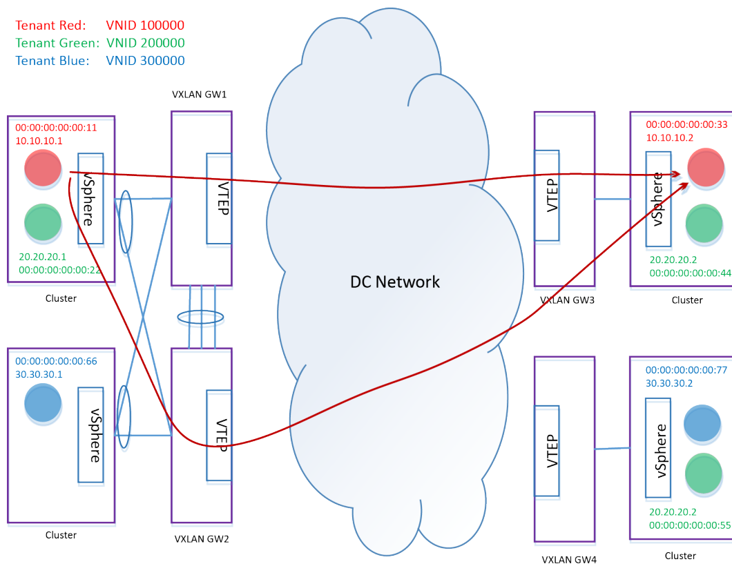
Figure 101: VXLAN Gateways with Three Tenants
