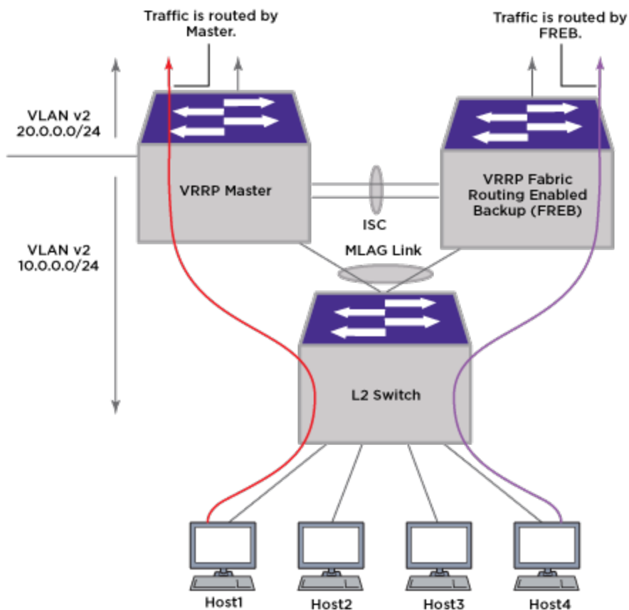
Figure 181: VRRP Fabric Routing
