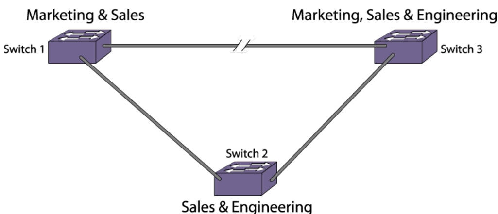
Figure 148: Incorrect Tag-Based STPD Configuration
