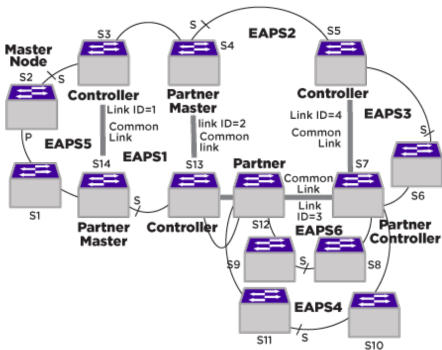
Figure 128: Advanced Basic Core and Right Angle Topology
