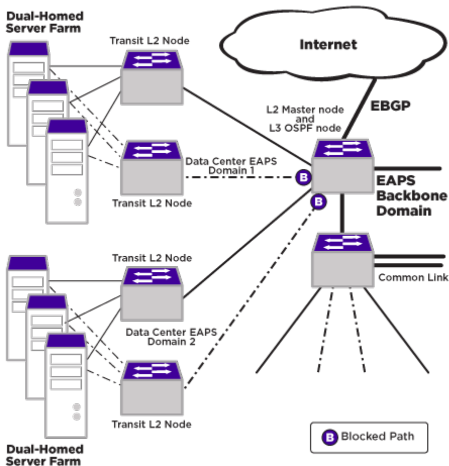
Figure 136: Data Center EAPS and OSPF Network Layer
