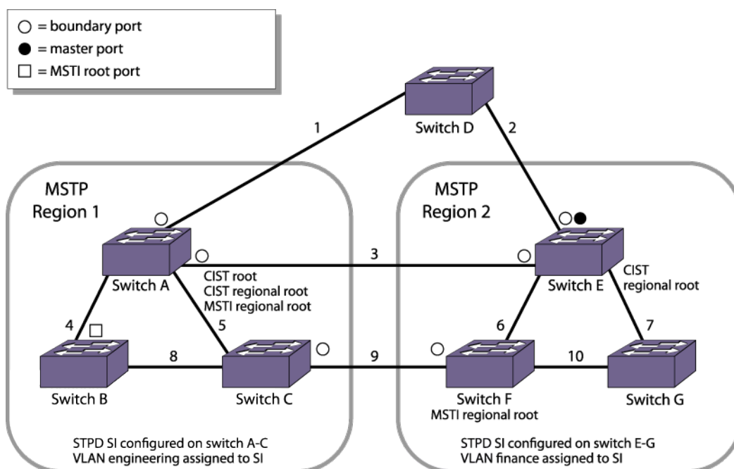
Figure 165: MSTP Topology with the CIST Root Bridge Contained within a Region
