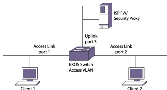
Figure 83: Upstream Forwarding or Disabling Egress Flooding Example
