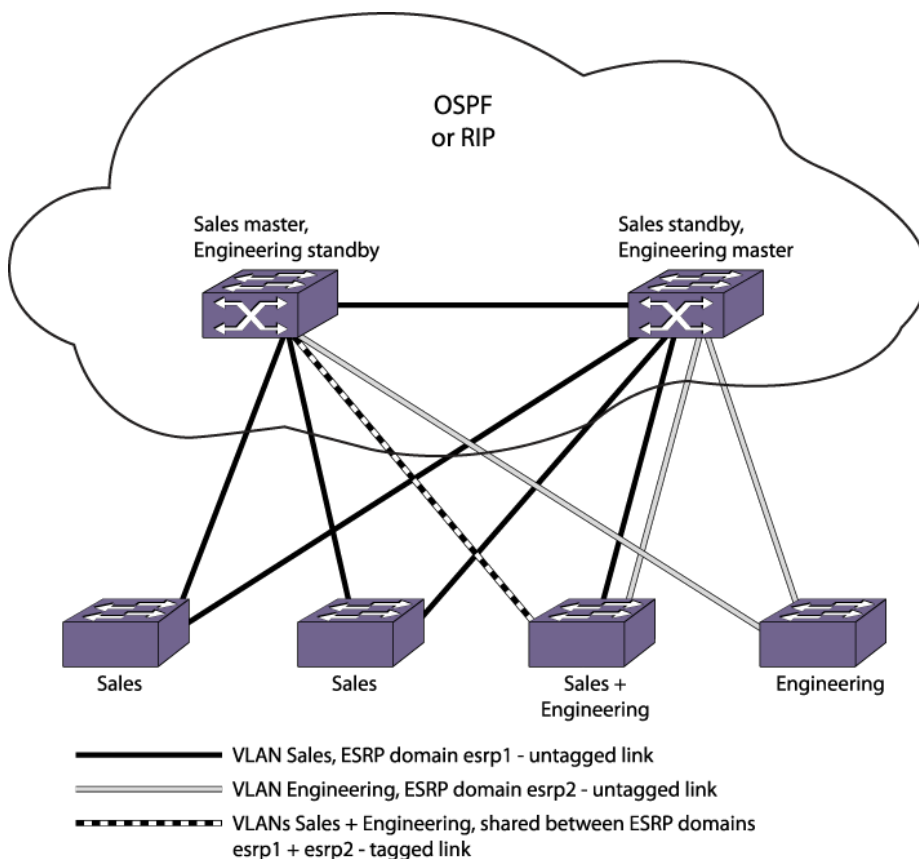
Figure 177: Multiple ESRP Domains Using Layer 2 and Layer 3 Redundancy
