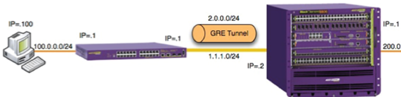
Figure 210: GRE Tunnel Configuration
