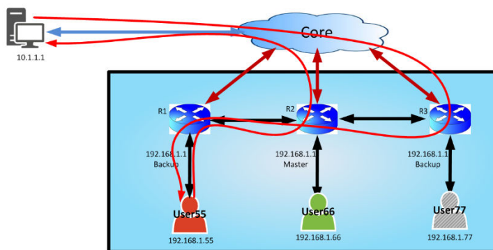
Figure 183: Asymmetric Routing and VRRP (2)
