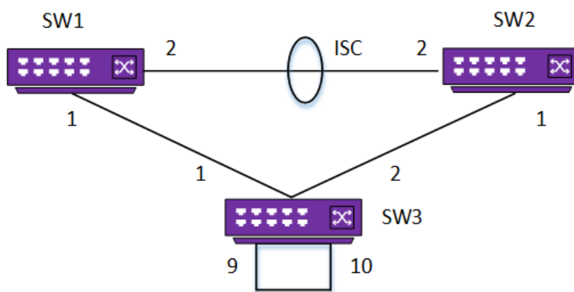
Figure 262: ELRP Egress Port Disable (2)
