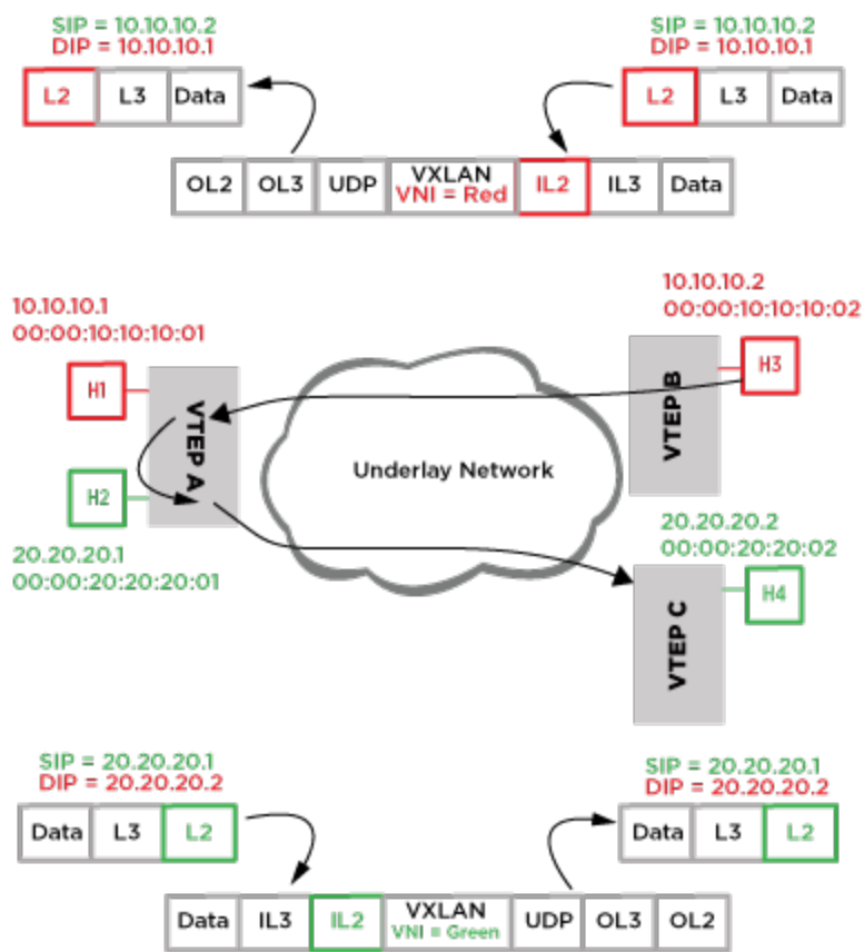
Figure 98: Routing in and out of a Tunnel
