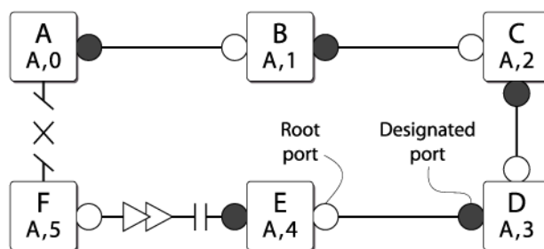
Figure 160: Completing the Topology Change
