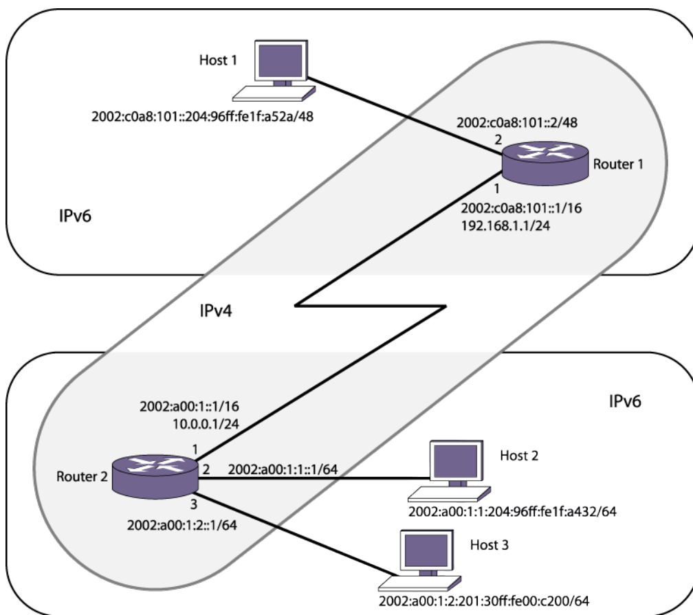
Figure 219: 6to4 Tunnel Configuration Example
