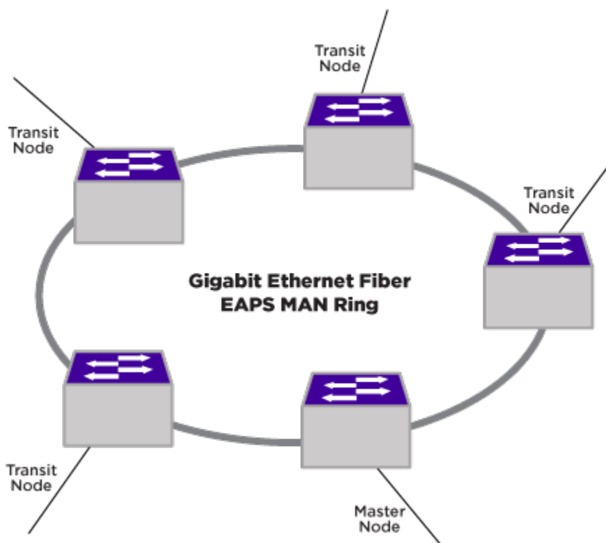
Figure 115: Gigabit Ethernet Fiber EAPS MAN Ring
