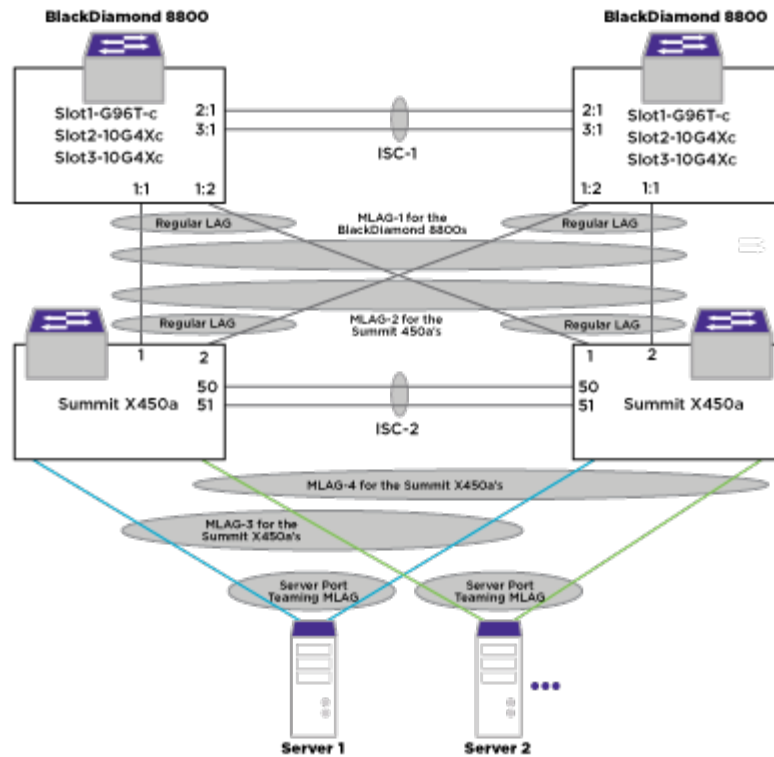
Figure 29: Two-tier MLAG Network
