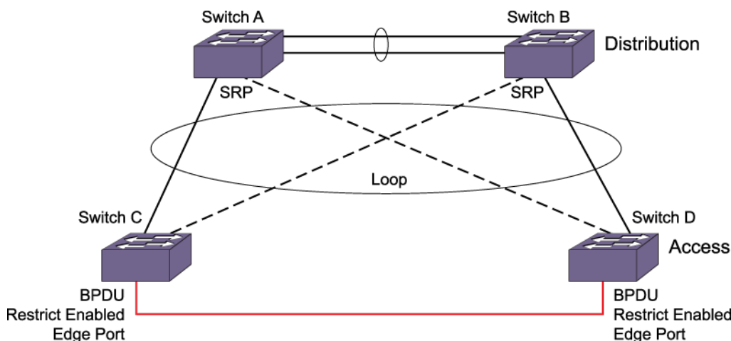
Figure 146: BPDU Restrict
