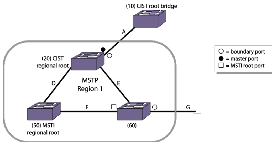
Figure 163: Closeup of MSTP Region 1
