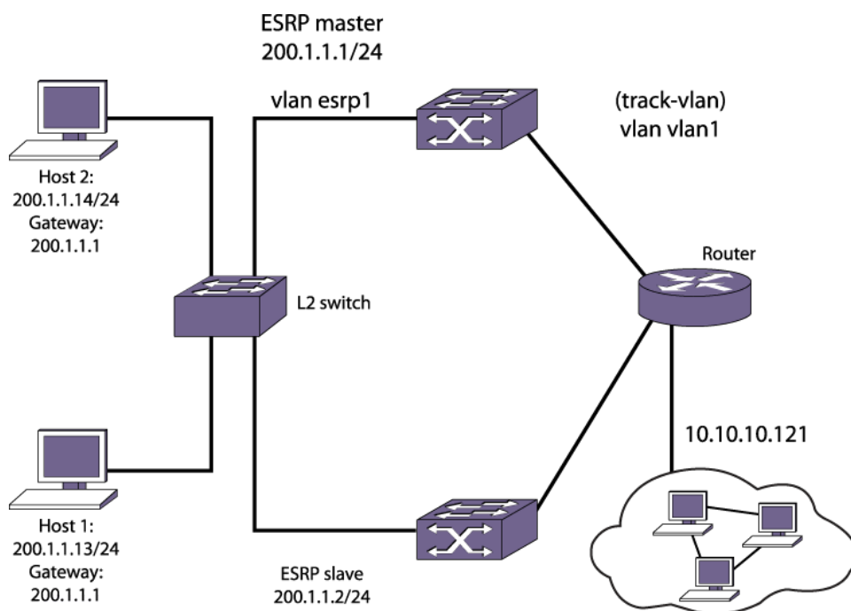
Figure 174: ESRP Tracking
