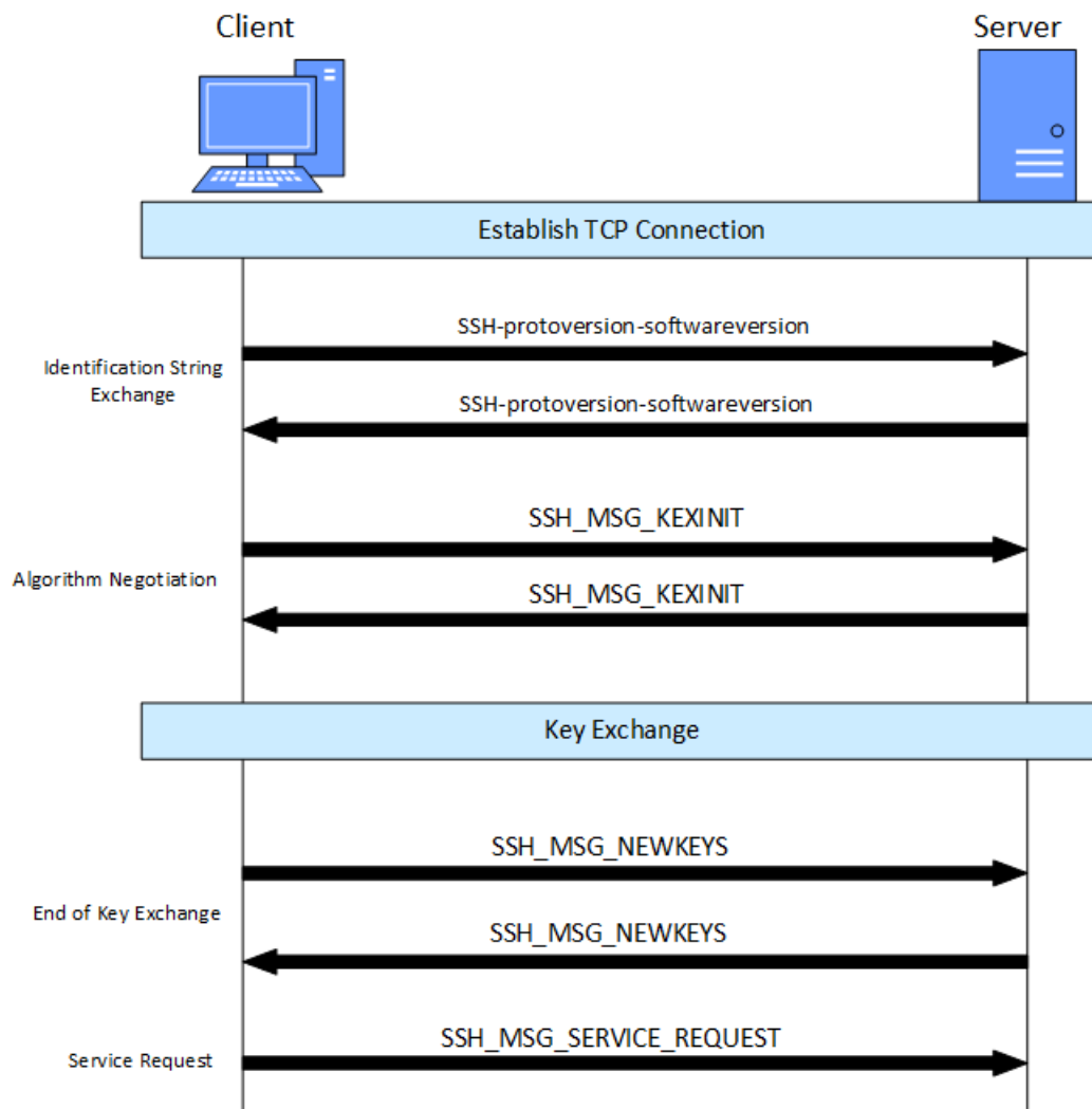
Figure 113: SSH Client /Server Connection Steps
