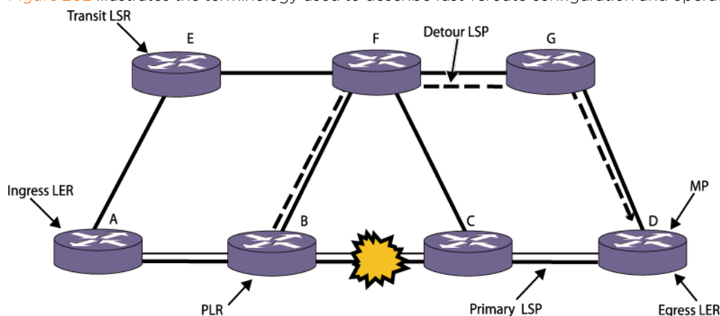
Figure 202: Fast-Reroute Terminology
