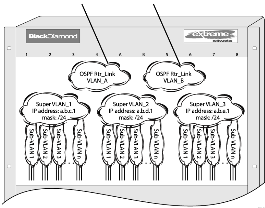
Figure 214: VLAN Aggregation
