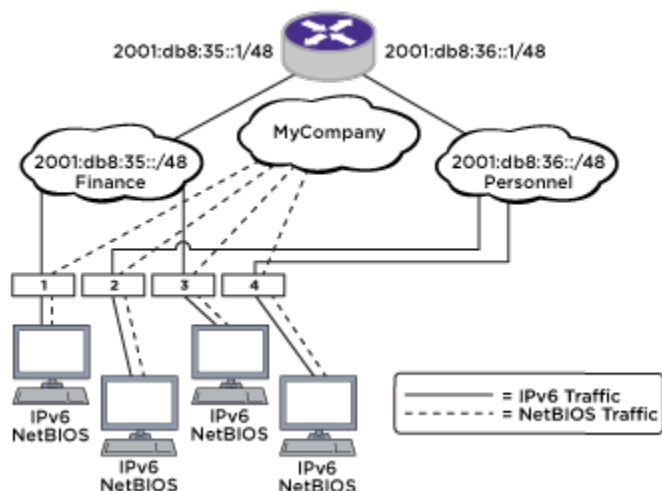
Figure 217: IPv6 Unicast Routing Configuration Example
