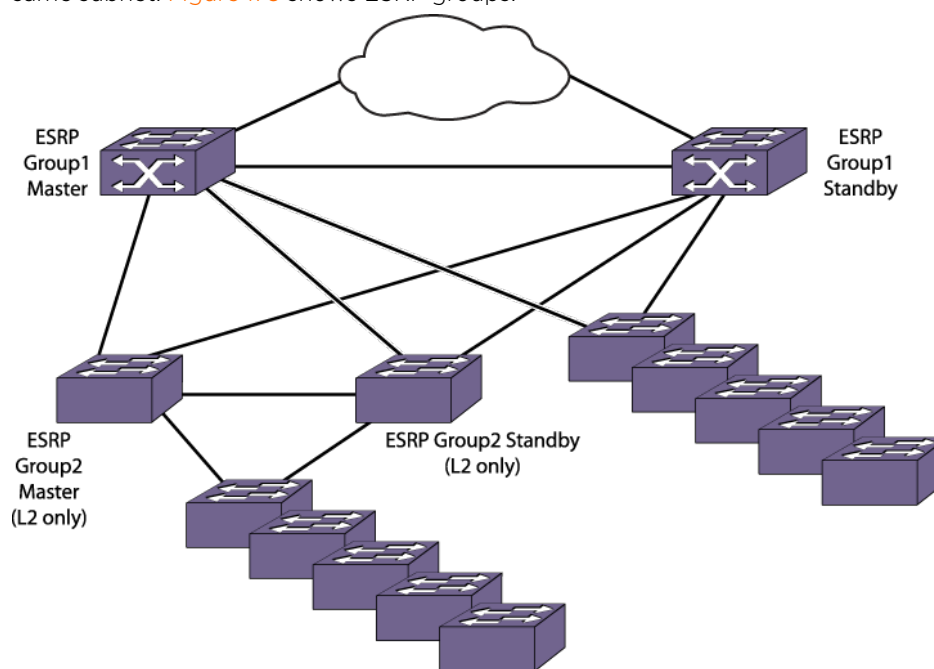
Figure 173: ESRP Groups
