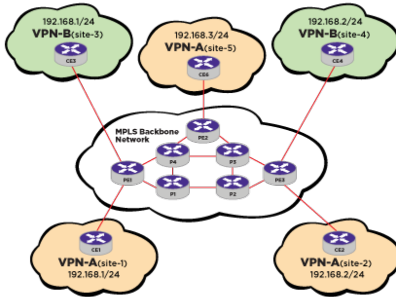
Figure 245: Different Router Roles in L3 VPN
