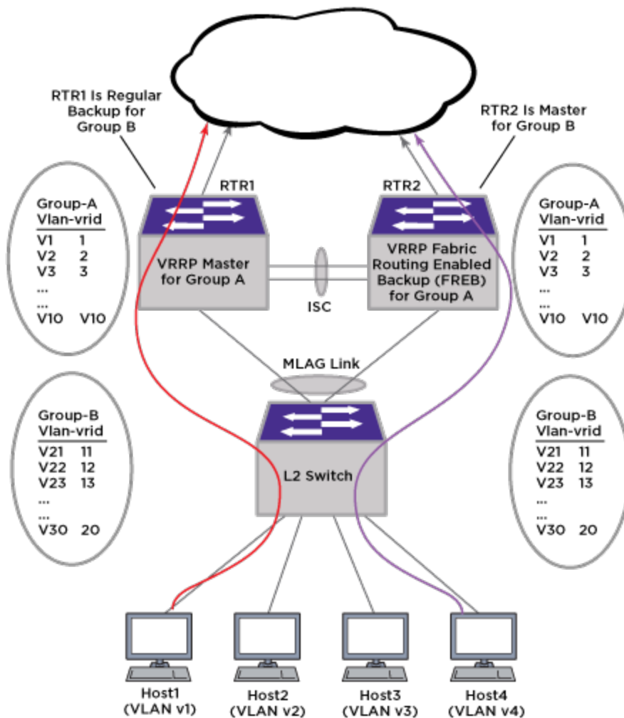
Figure 184: Example VRRP Group Configuration
