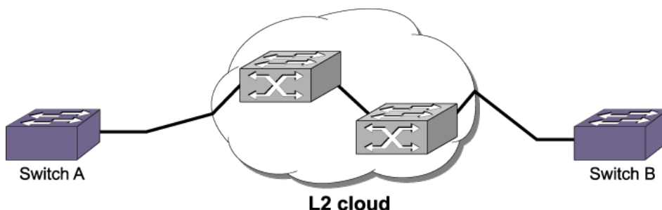
Figure 58: ELSM Through a Layer 2 Cloud
