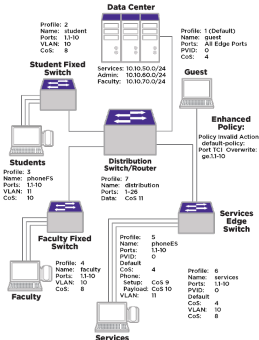
Figure 95: College-Based Policy Configuration
