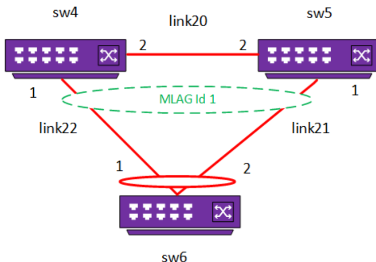
Figure 261: ELRP Egress Port Disable (1)
