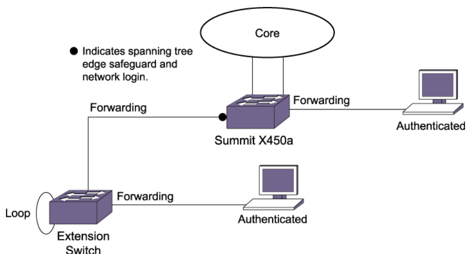
Figure 167: Traffic Monitoring on the Edge Side
