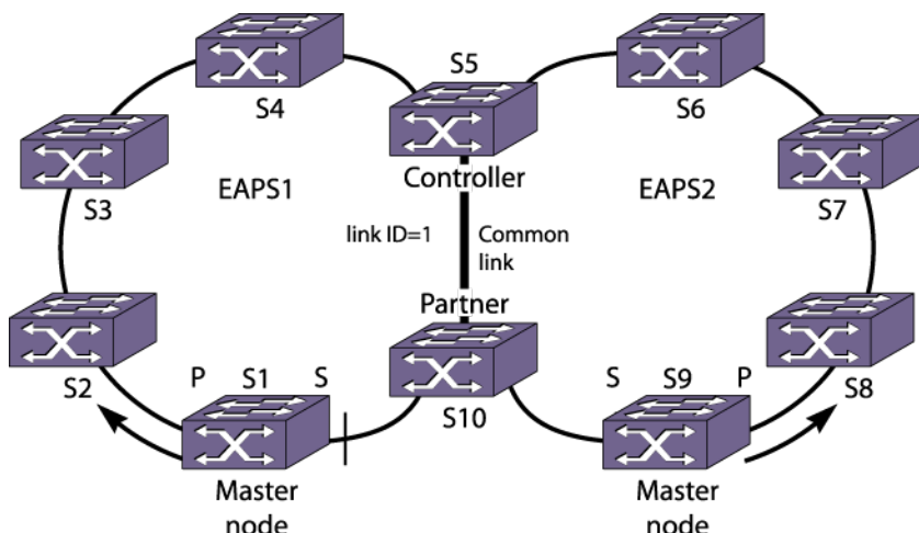
Figure 118: Multiple Rings Sharing a Common Link
