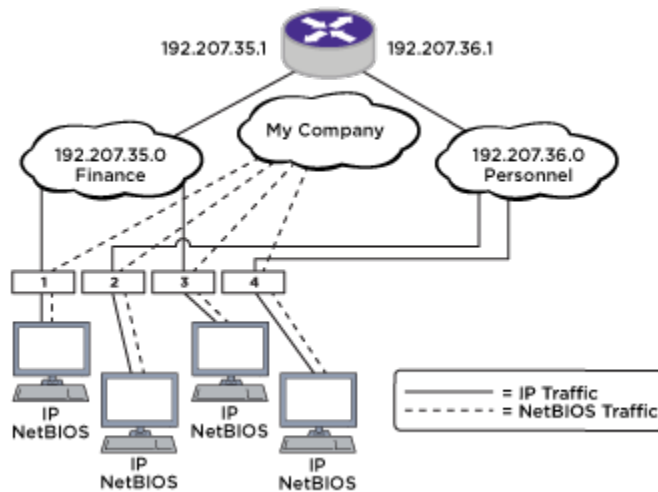
Figure 221: RIP Configuration Example
