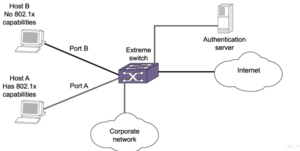
Figure 93: Guest VLAN for Network Login
