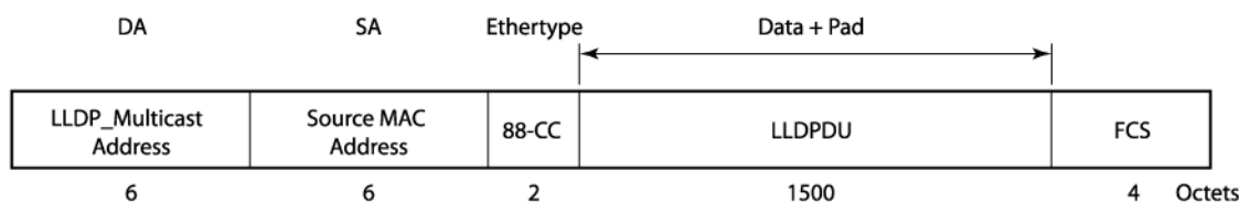
Figure 46: LLDP Packet Format
