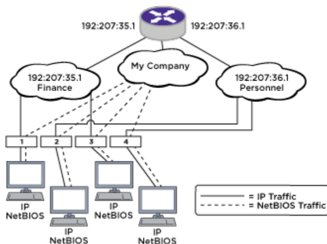
Figure 212: Unicast Routing Configuration Example
