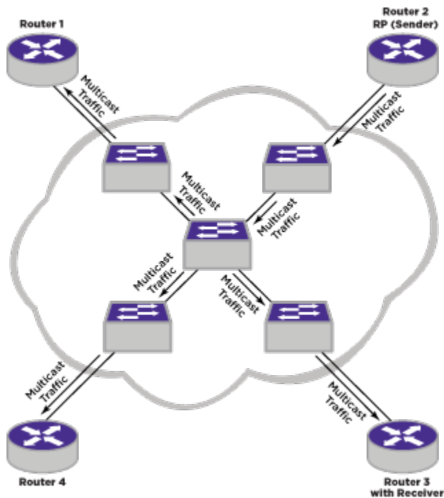
Figure 249: Multicast Without PIM Snooping
