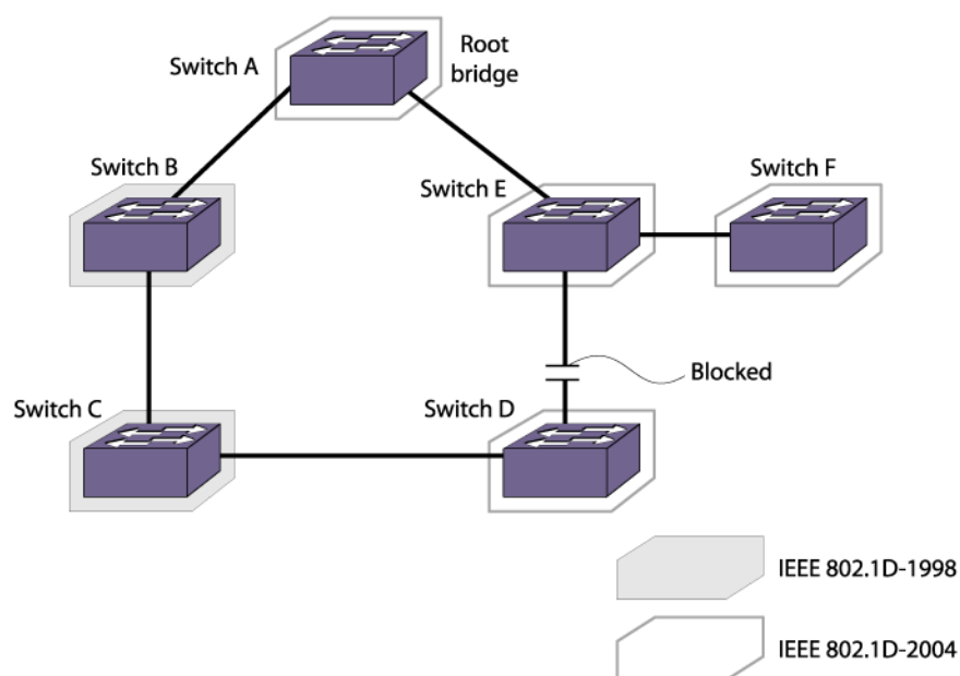
Figure 140: 802.1D-1998 and 802.1D-2004 Mixed Bridge Topology
