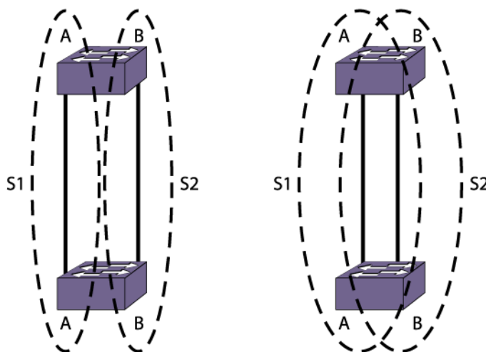
Figure 149: Limitations of Traditional STPD
