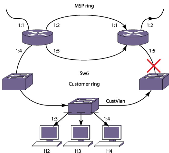
Figure 257: Inter-Multicast VLAN Forwarding
