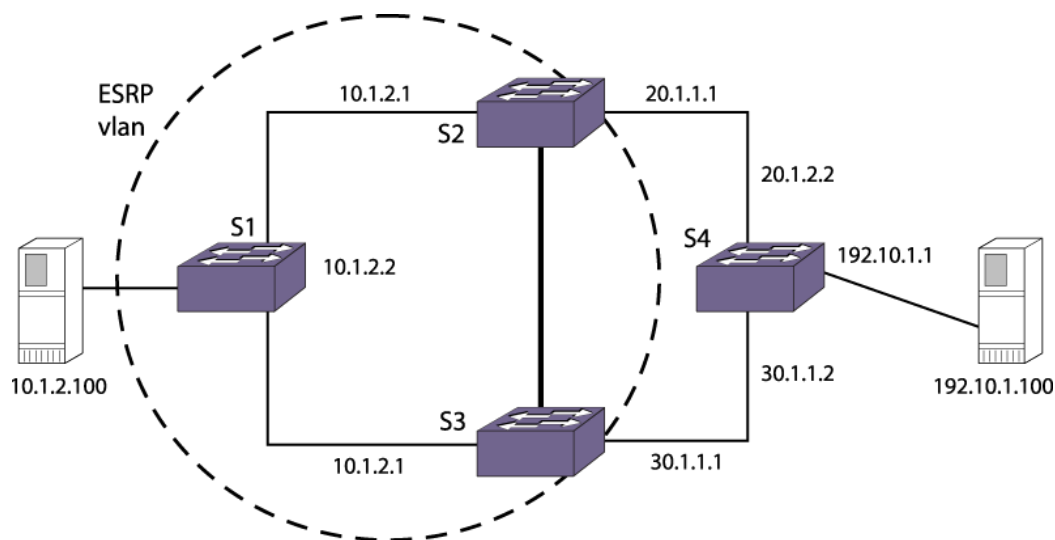
Figure 105: MAC Address Limits and VLANs Participating in ESRP
