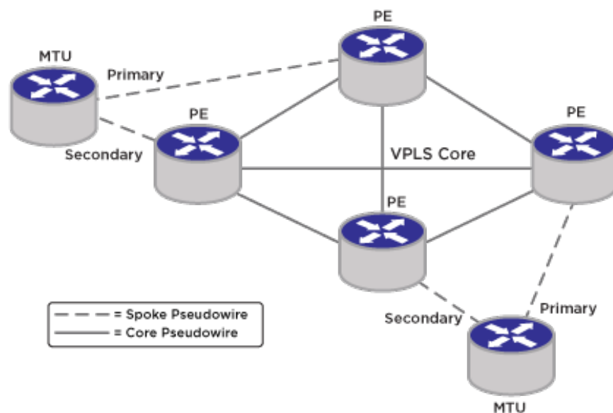
Figure 194: Example H-VPLS Network with Redundant Spokes
