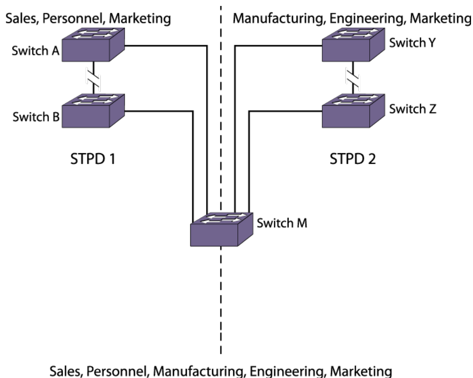
Figure 147: Multiple STPDs
