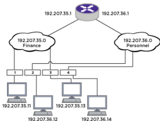
Figure 209: Routing Between VLANs
