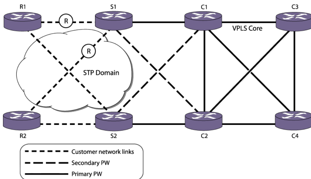
Figure 198: Redundant Edge H-VPLS Network with STP Example
