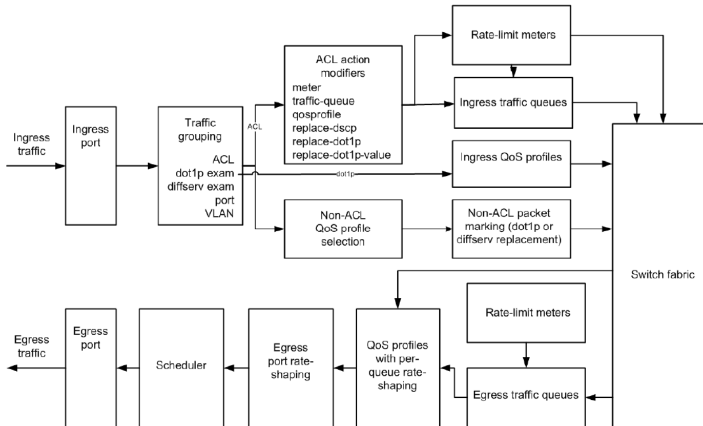
Figure 88: QoS on Extreme Networks Switches
