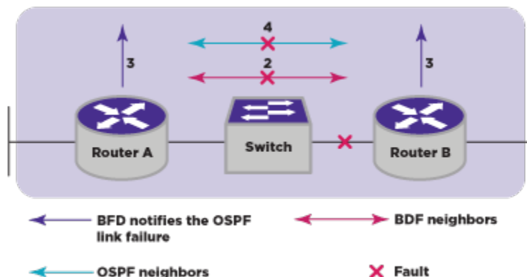
Figure 229: OSPFv3 Neighbor Relationship Eliminated by BFD Fault Detection
