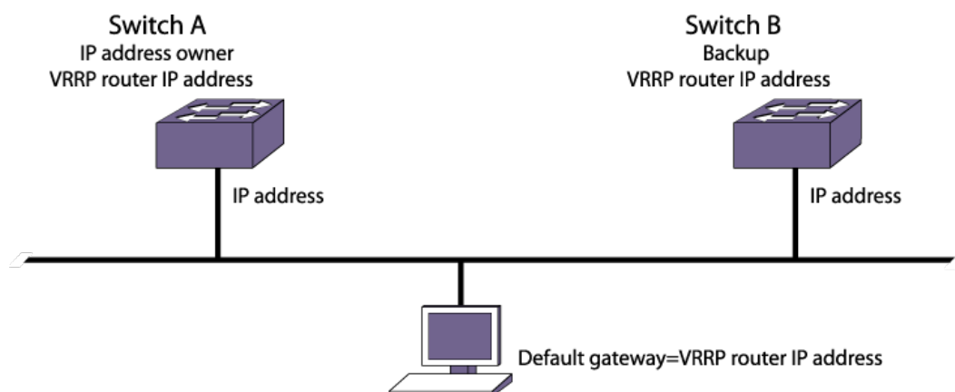
Figure 178: Simple VRRP Network
