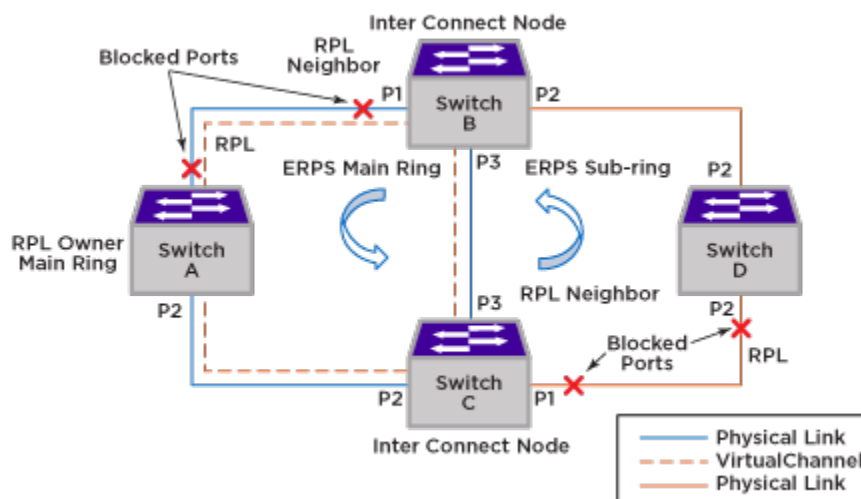
Figure 139: Sample ERPS Configuration
