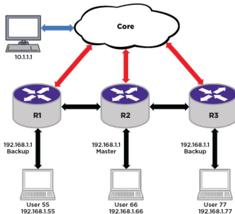
Figure 182: Asymmetric Routing and VRRP (1)
