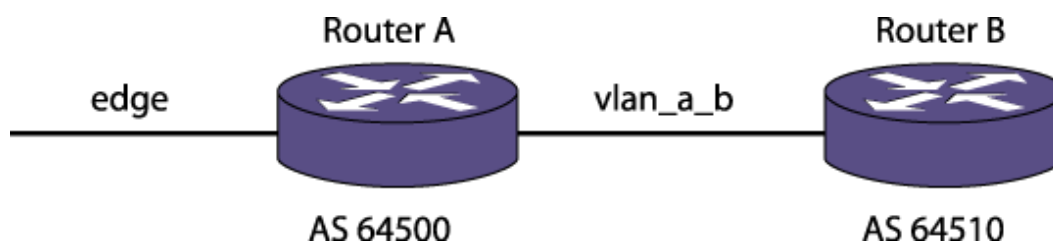
Figure 243: BGP IPv4 Route Filtering Example
