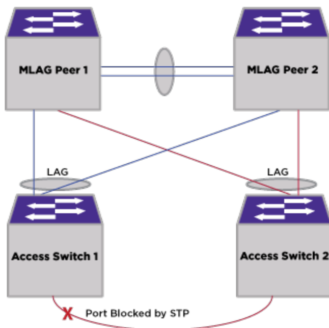
Figure 168: MLAG and MSTP/RSTP
