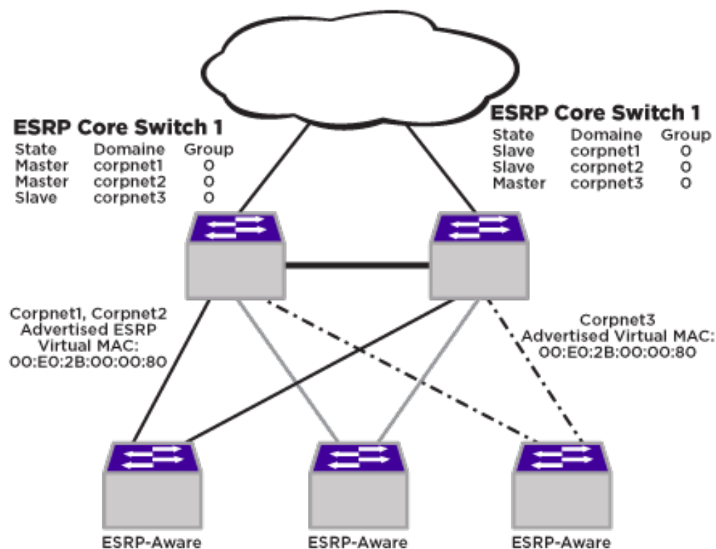
Figure 172: Example of a Basic ESRP Topology
