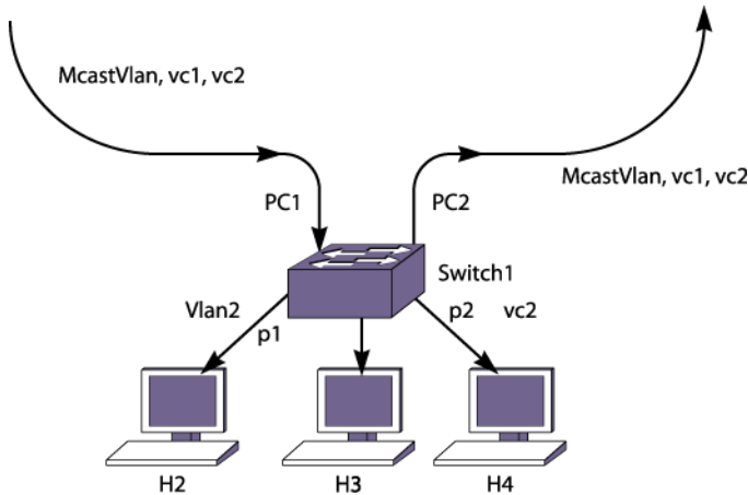
Figure 256: Multiple VLANs in the Core Network
