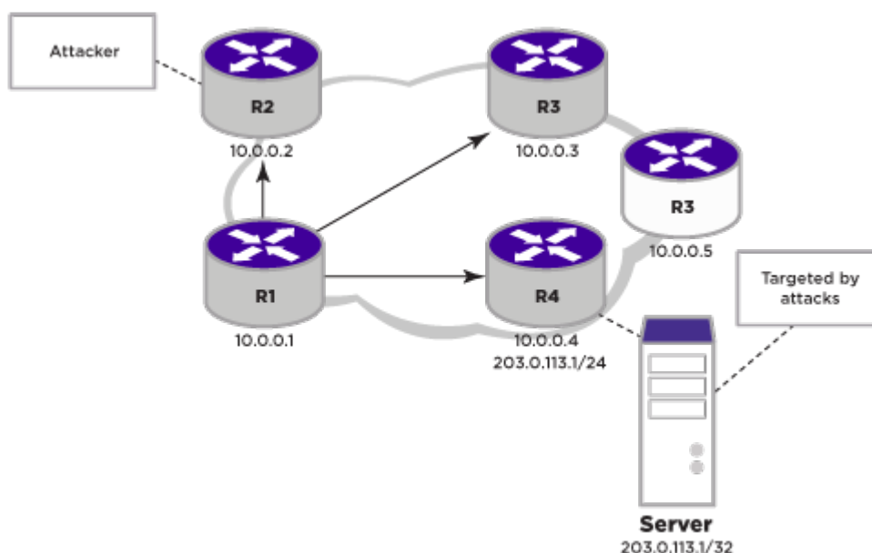
Figure 242: Black Hole Routing Using BGP
