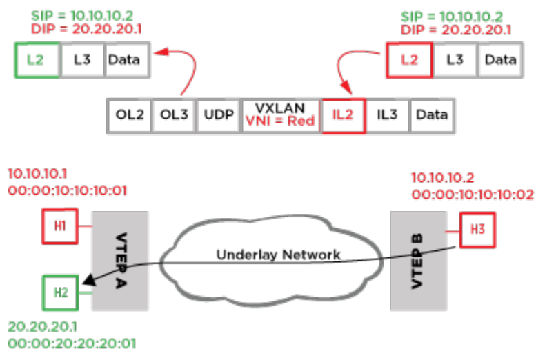
Figure 97: Routing from a Tunnel
