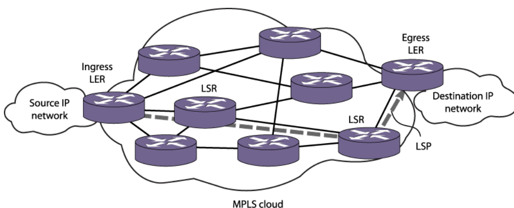
Figure 186: MPLS Network
