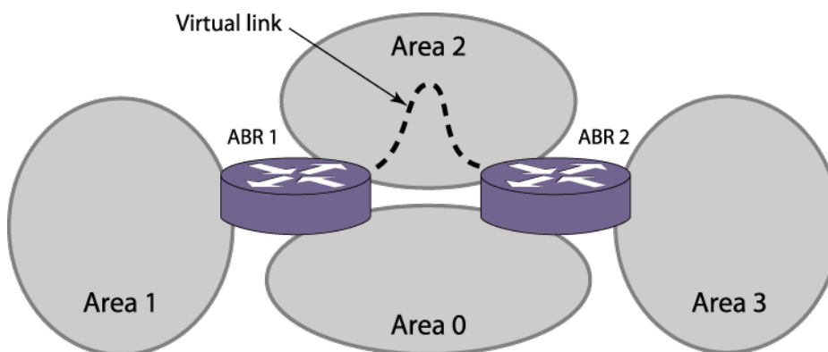
Figure 225: Virtual Link Providing Redundancy
