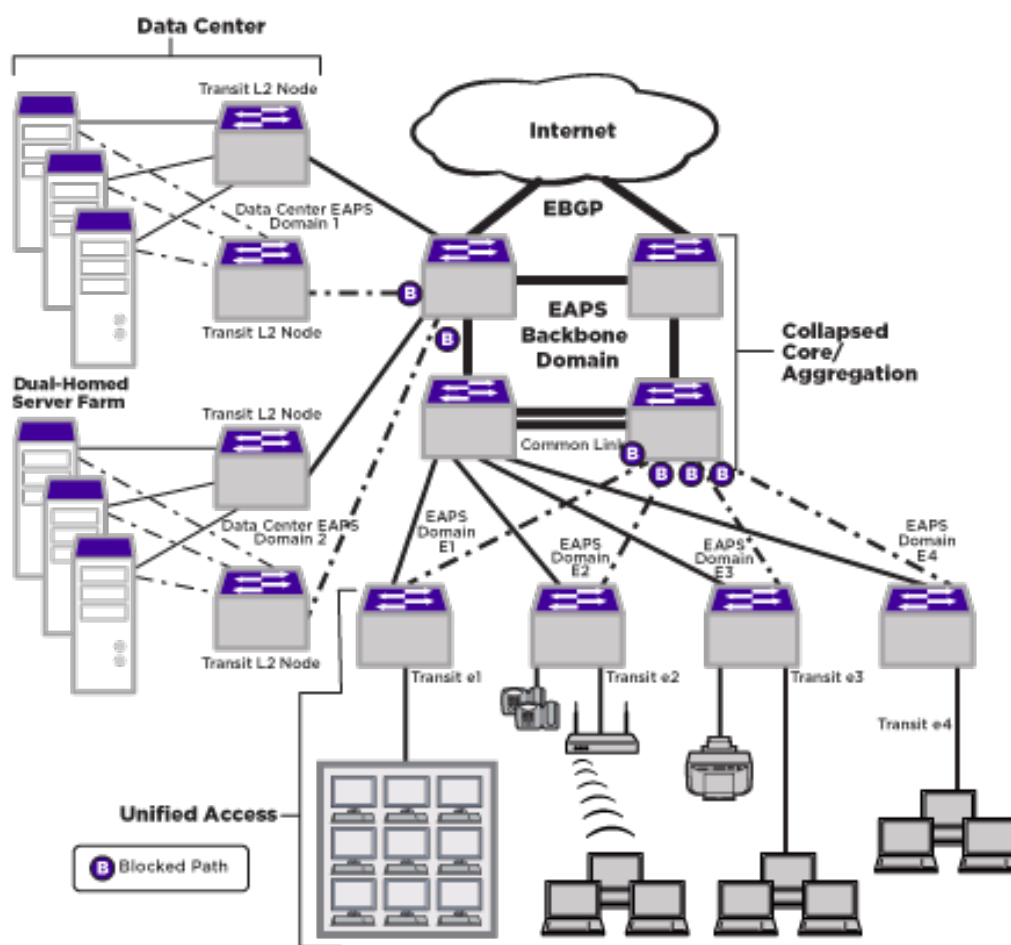
Figure 131: Extreme Networks EAPS Everywhere
