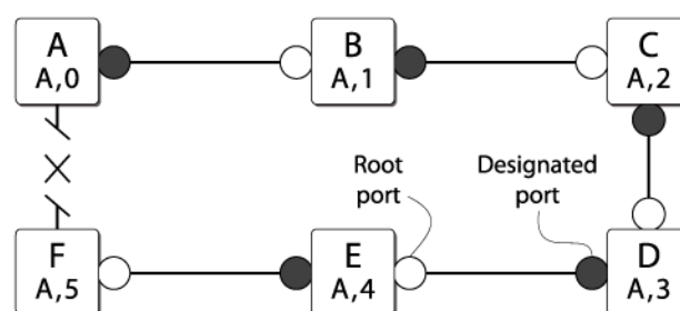
Figure 161: Final Network Configuration
