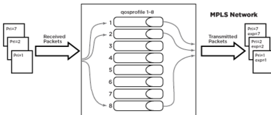
Figure 204: Mapping Dot1p to EXP Bits
