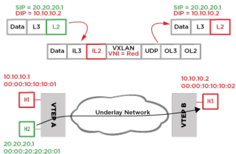
Figure 96: Routing into a Tunnel
