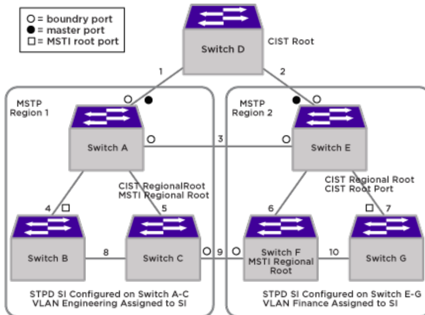
Figure 171: MSTP Configuration Example
