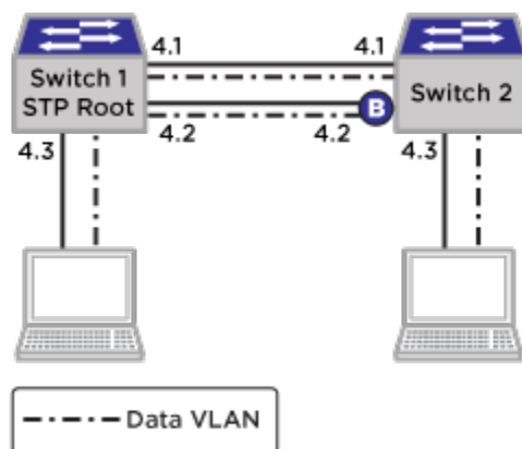
Figure 130: Sample STP Network for Migration to EAPS
