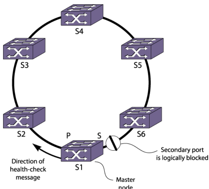
Figure 116: EAPS Operation
