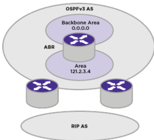
Figure 232: OSPFv3 Route Redistribution
