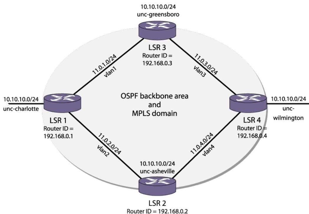
Figure 207: Full Mesh Configuration Example
