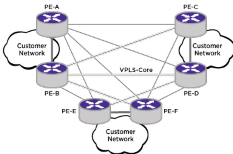
Figure 195: Example Protected Access VPLS Network
