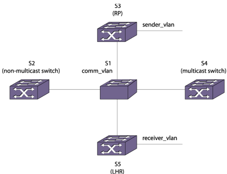
Figure 253: PIM Snooping Configuration Example
