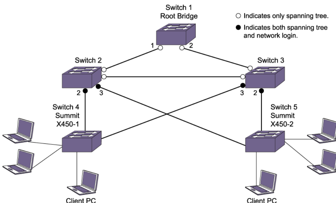
Figure 166: STP and Network Login Enabled
