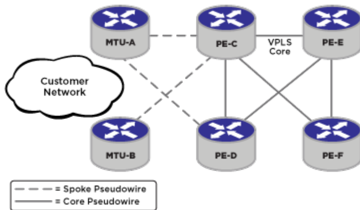
Figure 197: Example Redundant Edge H-VPLS Network
