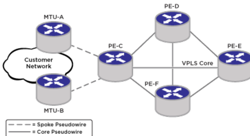
Figure 196: Example Protected Access H-VPLS Network
