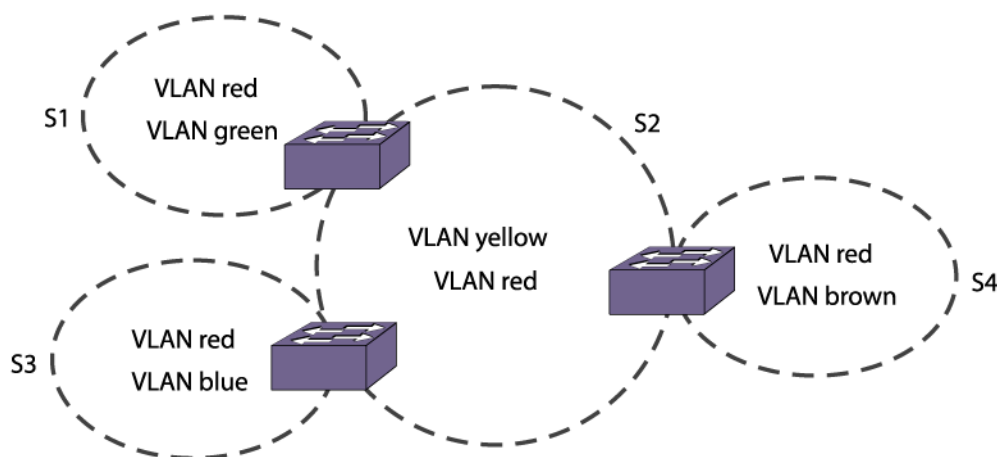
Figure 169: EMISTP Configuration Example
