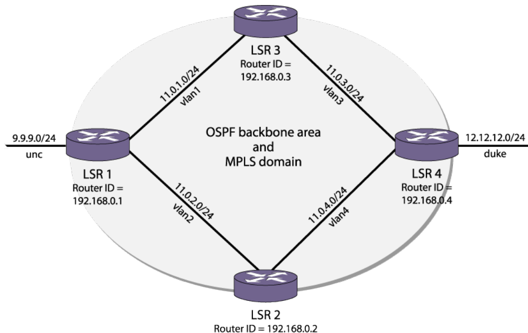
Figure 205: MPLS Configuration Example
