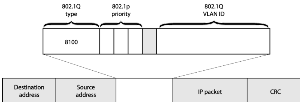
Figure 89: 802.1p Priority Bits
