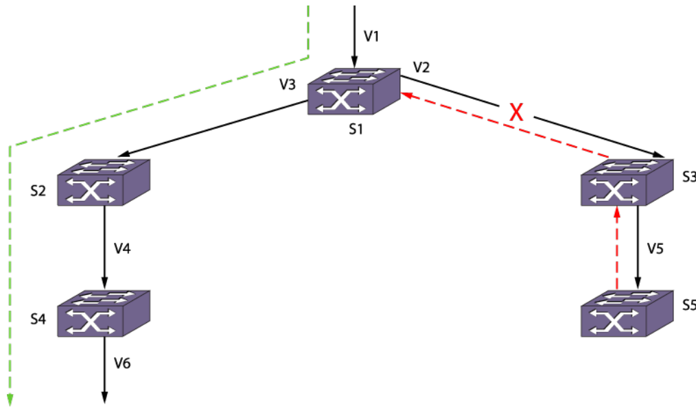
Figure 248: PIM-DM Operation
