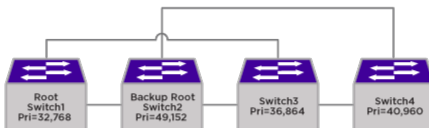
Figure 141: STP Root Bridge Loss Example
