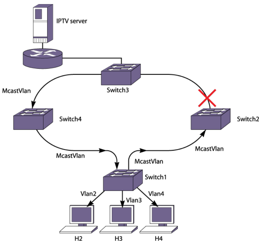
Figure 255: Basic MVR Deployment
