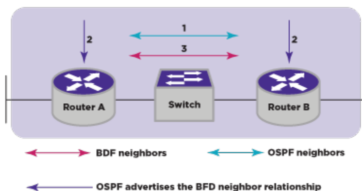
Figure 228: Basic Operational Flow of OSPFv3 BFD
