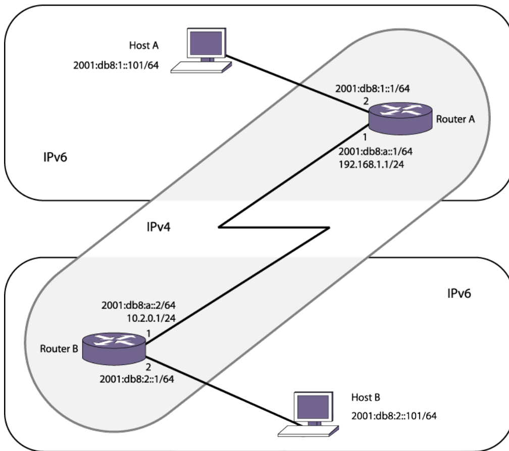
Figure 218: 6in4 Tunnel Example
