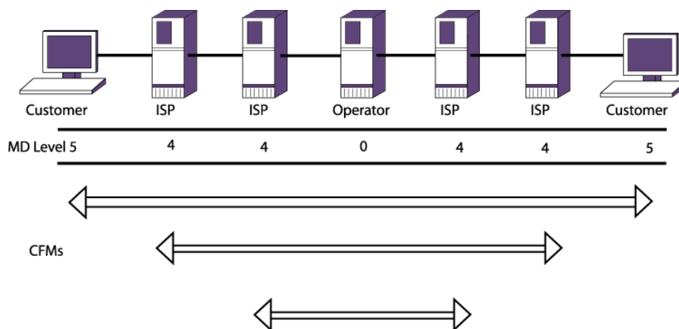
Figure 48: CFM Hierarchical Domains Example
