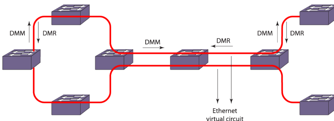
Figure 51: Two-Way Frame Delay and Frame Delay Variance Measurement
