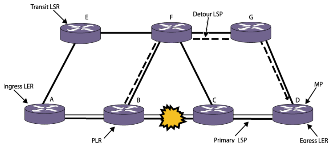
Figure 204: Fast-Reroute Terminology
