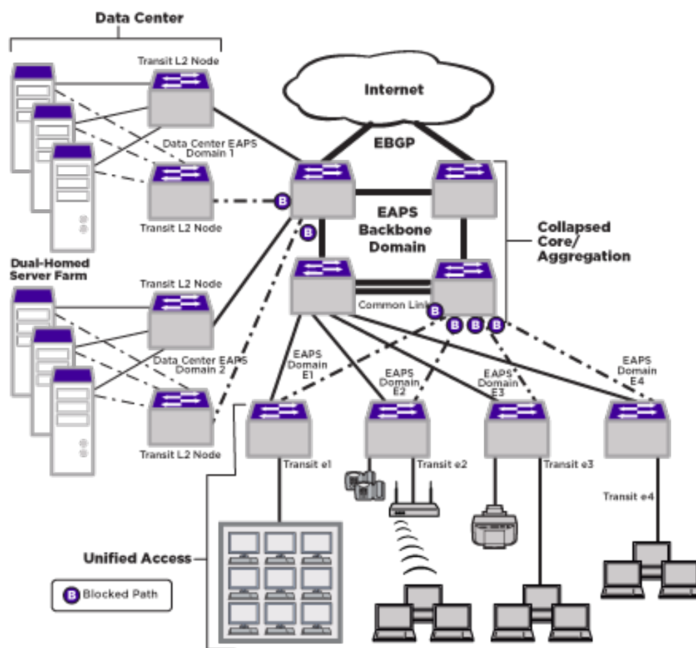
Figure 133: Extreme Networks EAPS Everywhere
