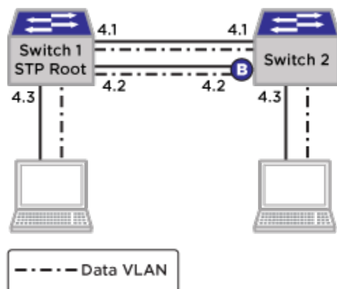
Figure 132: Sample STP Network for Migration to EAPS
