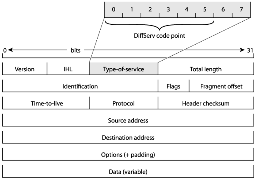
Figure 92: DiffServe Code Point
