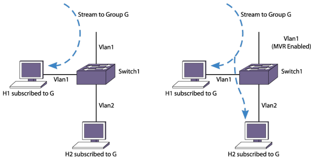
Figure 256: Standard VLAN Compared to an MVR VLAN
