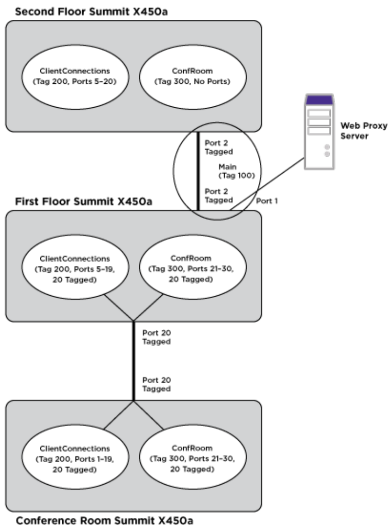
Figure 73: PVLAN Configuration Example 2
