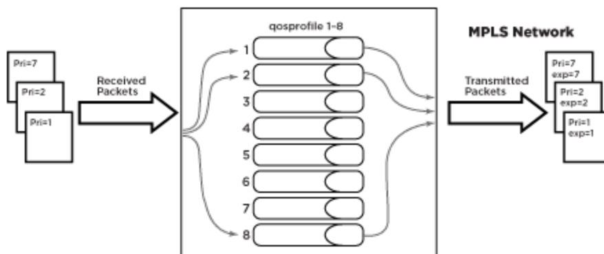
Figure 206: Mapping Dot1p to EXP Bits
