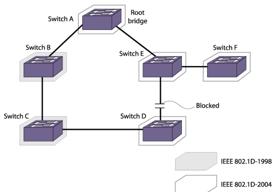
Figure 142: 802.1D-1998 and 802.1D-2004 Mixed Bridge Topology
