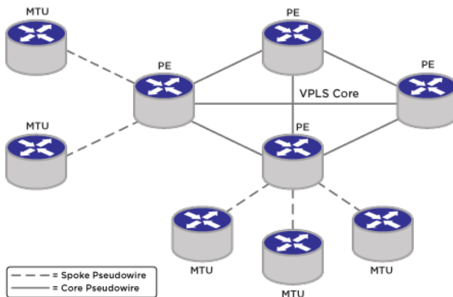
Figure 195: Example H-VPLS Network
