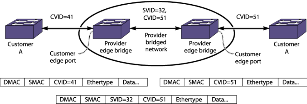
Figure 81: CVID Translation
