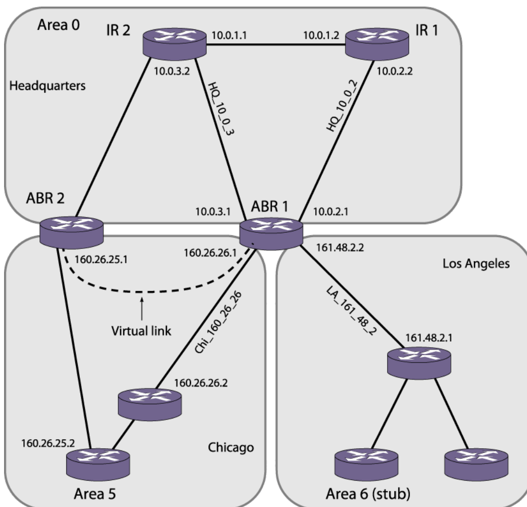
Figure 229: OSPF Configuration Example
