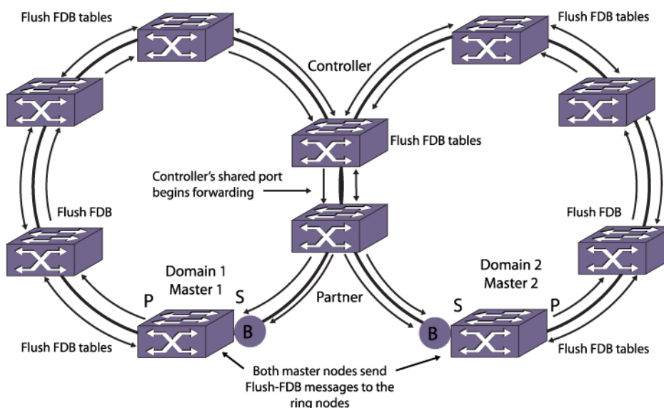
Figure 125: Common-Link Restored
