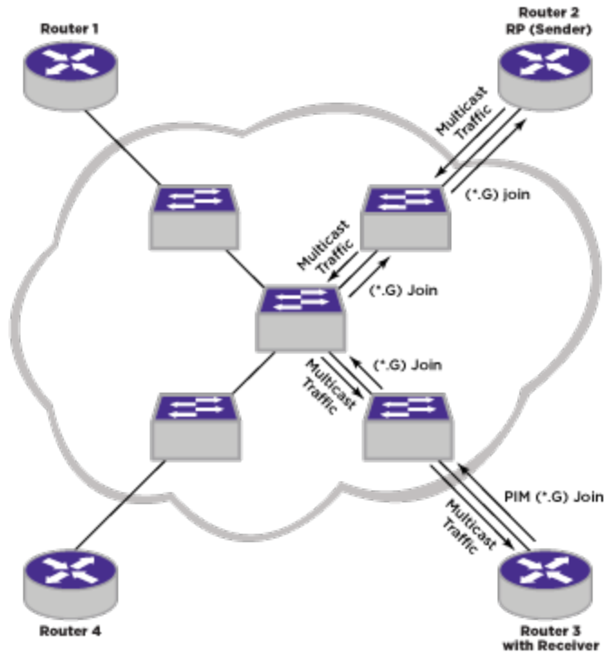
Figure 252: Multicast With PIM Snooping
