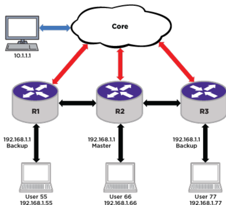
Figure 184: Asymmetric Routing and VRRP (1)
