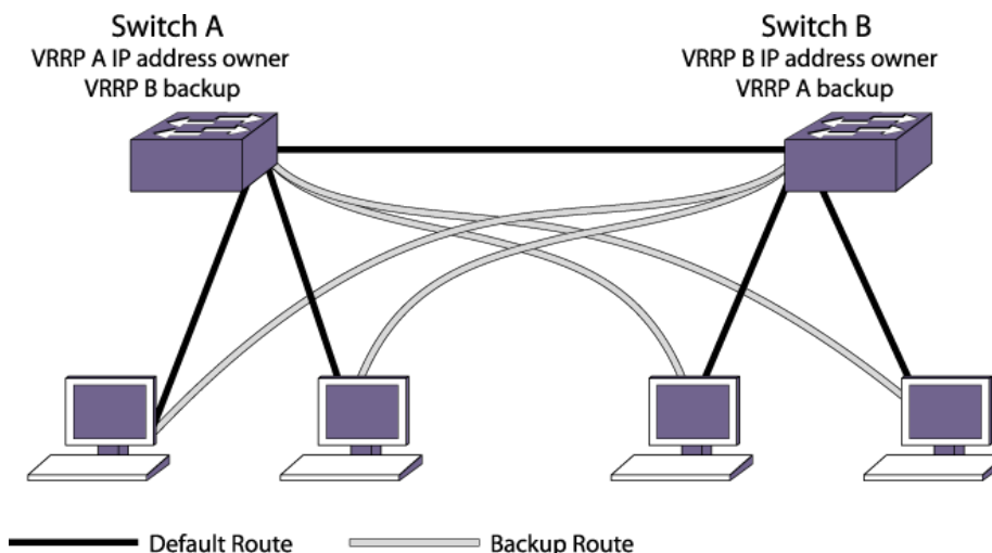
Figure 181: VRRP Load-sharing Configuration
