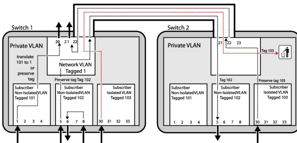
Figure 70: Private VLAN Support on Multiple Switches
