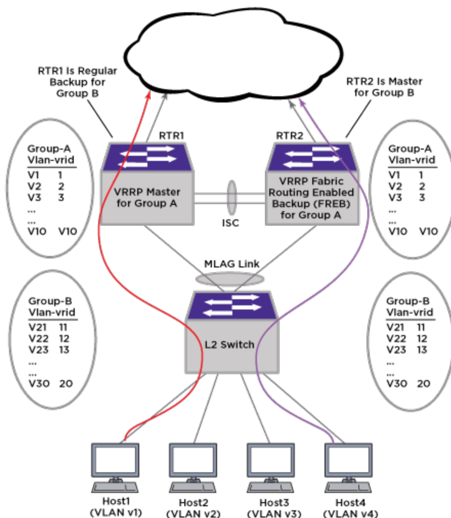
Figure 186: Example VRRP Group Configuration
