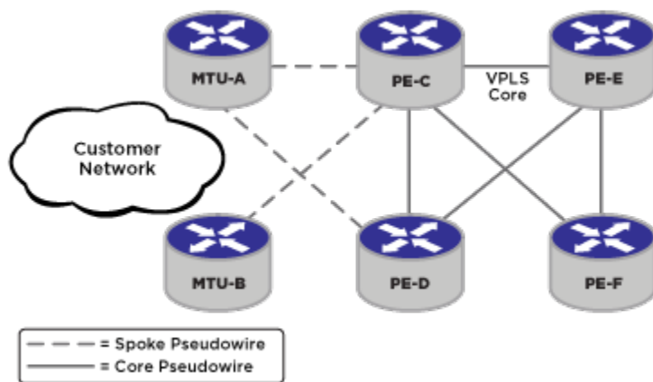
Figure 199: Example Redundant Edge H-VPLS Network
