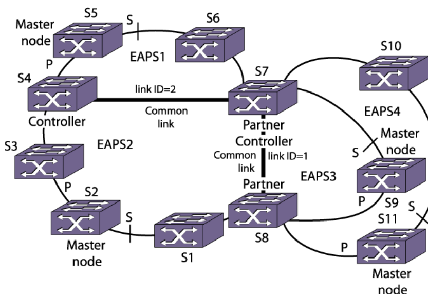
Figure 128: Right-Angle Topology
