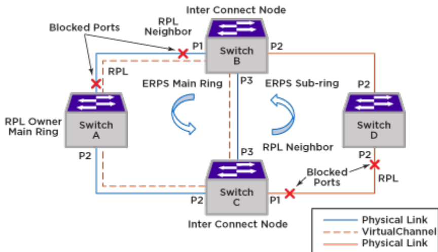
Figure 141: Sample ERPS Configuration
