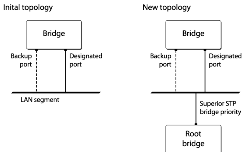
Figure 155: Example of Root Port Rapid Behavior
