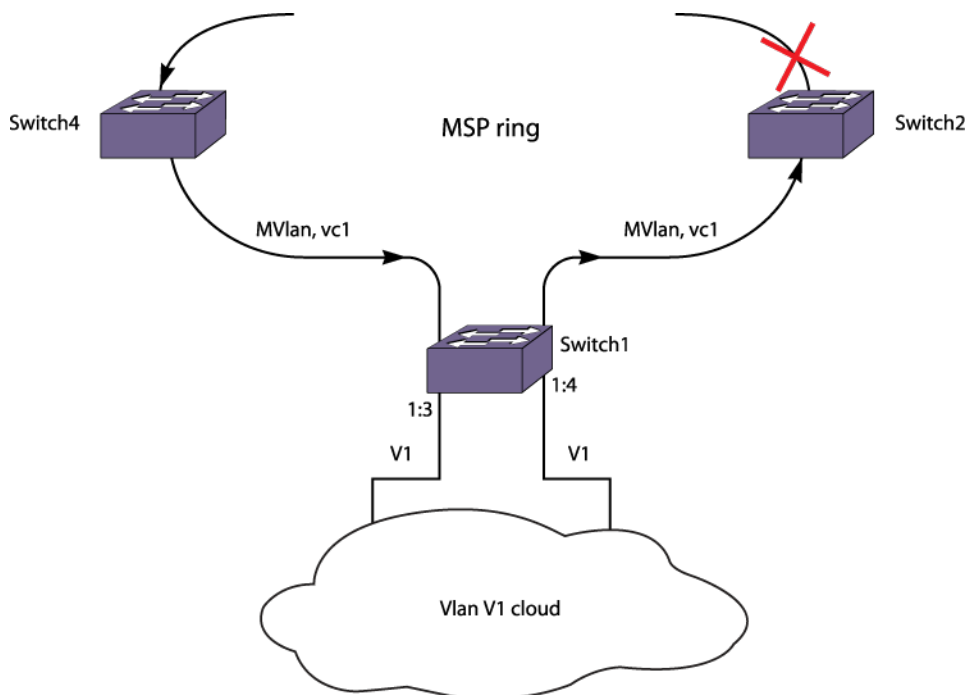
Figure 261: MVR with STP
