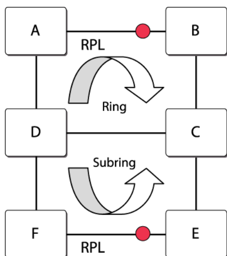
Figure 140: Ring and Sub-ring Network
