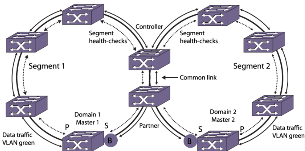
Figure 122: Segment Health-Check Messages
