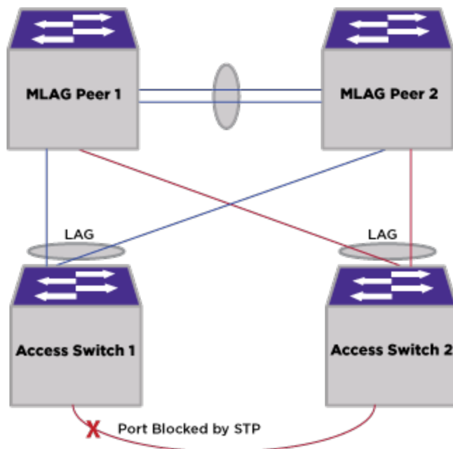
Figure 170: MLAG and MSTP/RSTP
