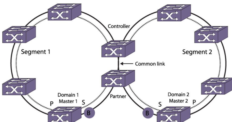
Figure 121: Master Node Operation in a Multiple Ring Topology
