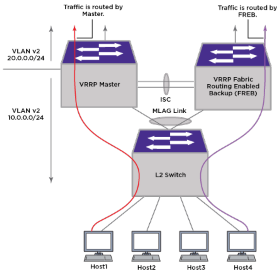
Figure 183: VRRP Fabric Routing
