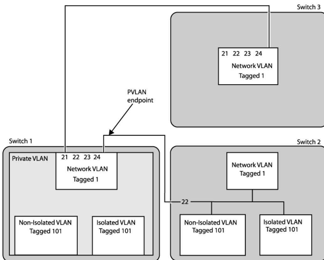
Figure 71: Private VLAN Connections to Switches Outside the PVLAN
