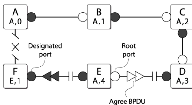
Figure 161: Communicating Port Status to Neighbors
