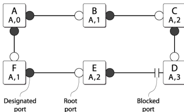
Figure 156: Initial Network Configuration
