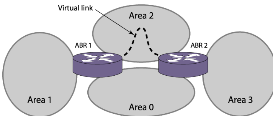
Figure 227: Virtual Link Providing Redundancy
