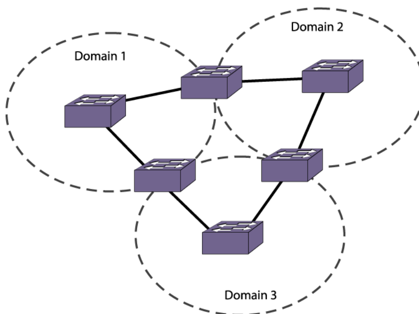
Figure 154: Looped VLAN Topology
