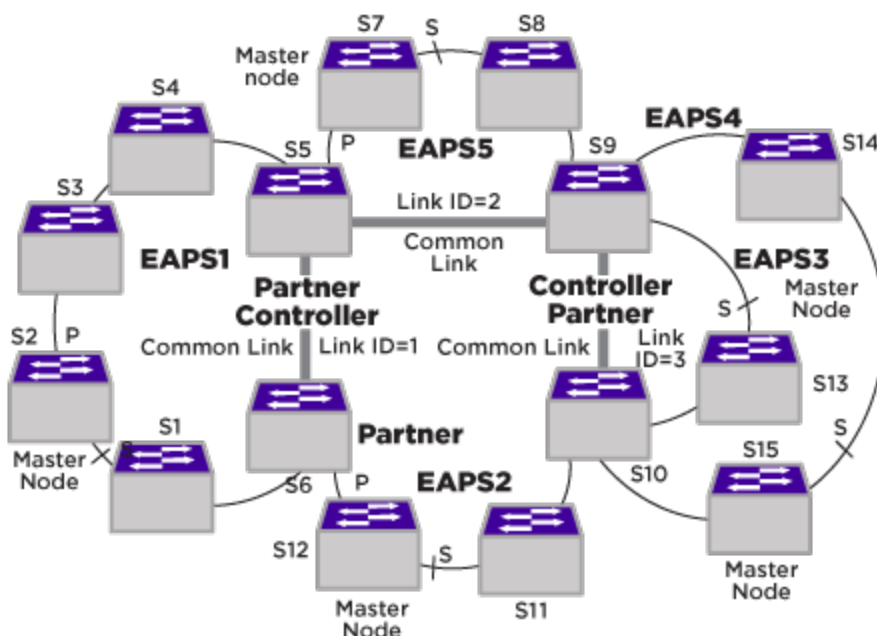
Figure 129: Basic Core and Right Angle Topology
