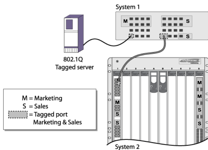
Figure 64: Physical Diagram of Tagged and Untagged Traffic
