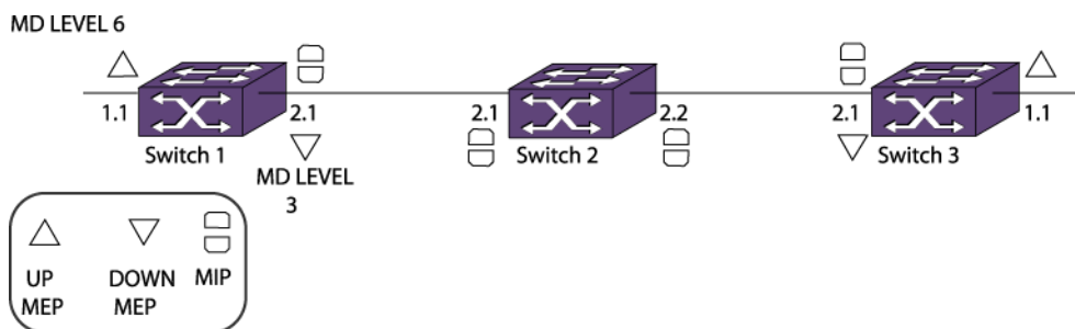
Figure 50: CFM Configuration Example
