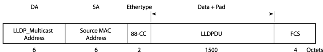
Figure 47: LLDP Packet Format
