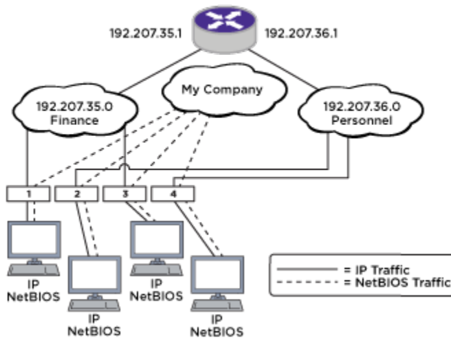
Figure 223: RIP Configuration Example
