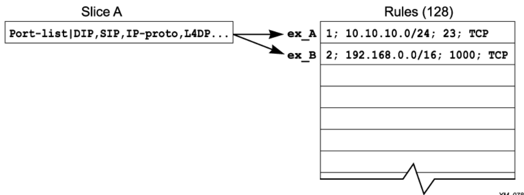
Figure 88: ACL Entry ex_A and ex_B
