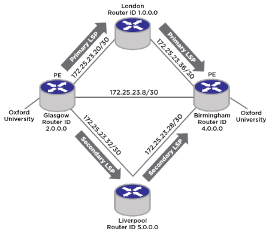
Figure 210: RSVP-TE Configuration Example
