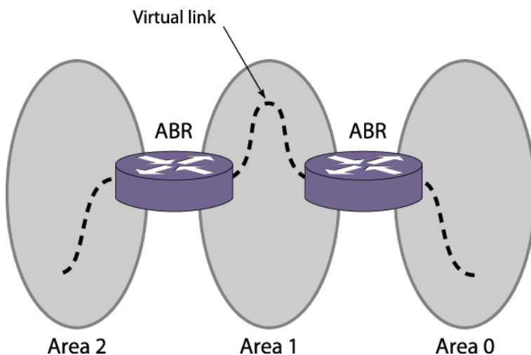
Figure 226: Virtual Link Using Area 1 as a Transit Area
