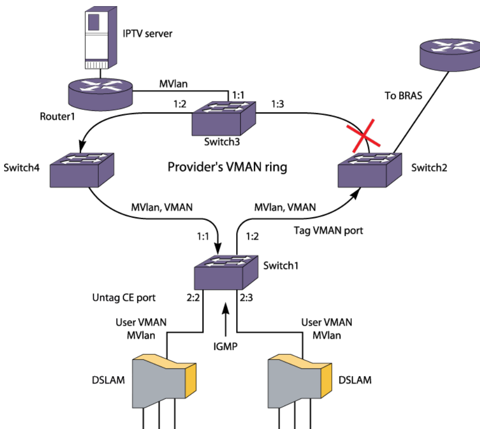
Figure 262: MVR in a VMAN Environment
