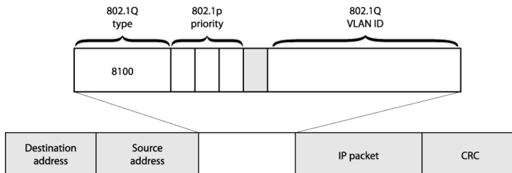
Figure 91: 802.1p Priority Bits
