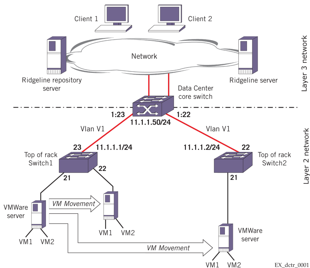
Figure 85: Sample XNV Topology
