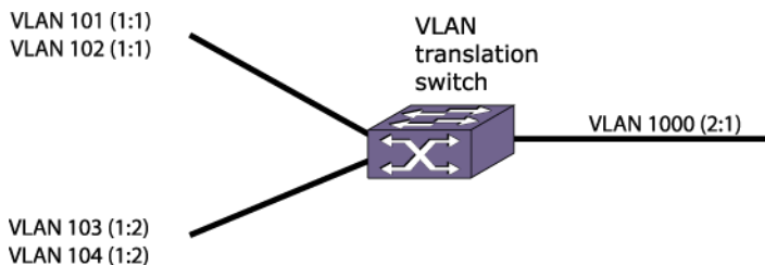
Figure 75: VLAN Translation Configuration Example
