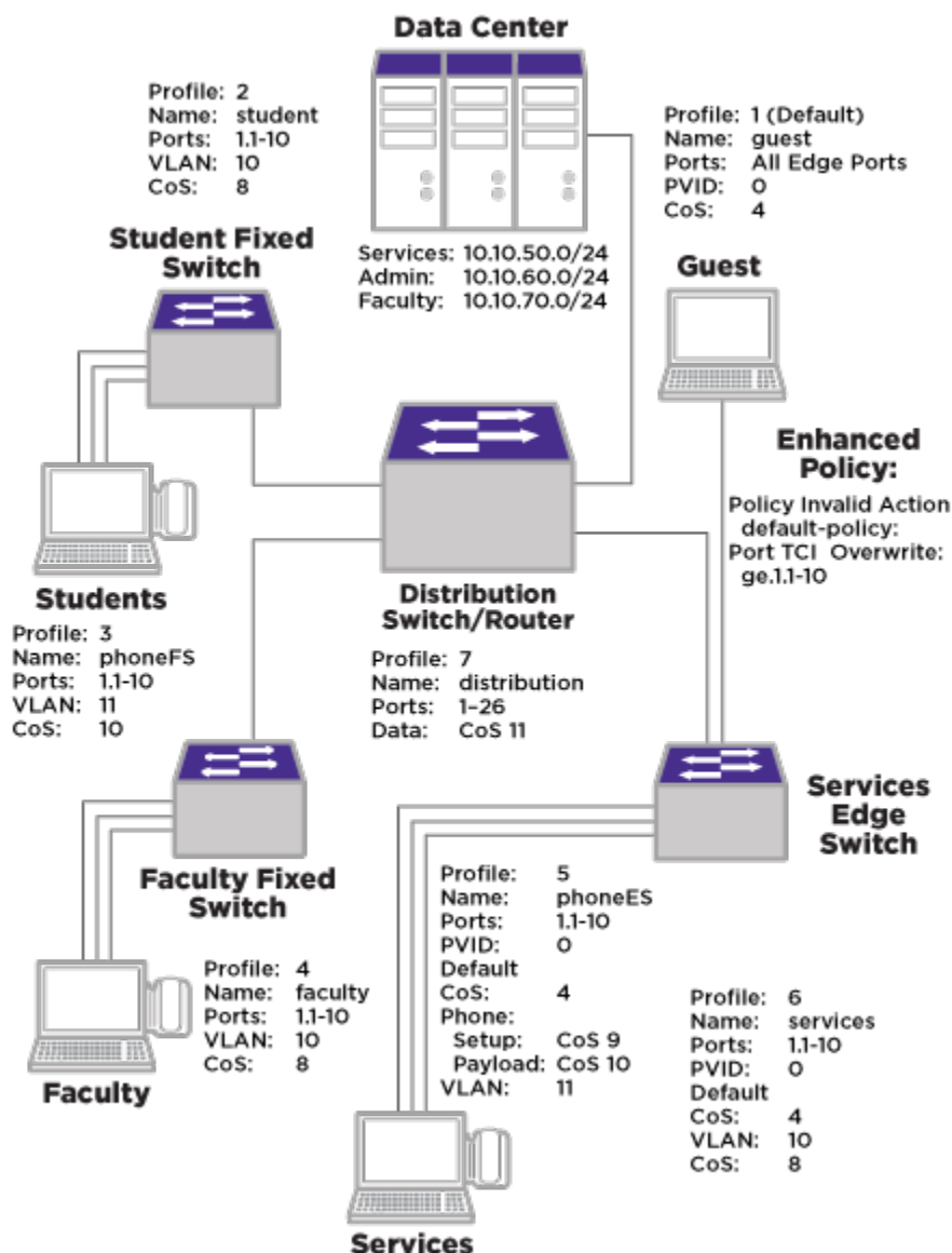
Figure 97: College-Based Policy Configuration
