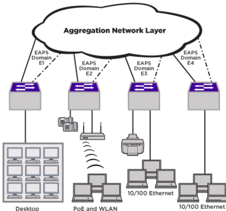
Figure 134: Converged Network Edge (Unified Access Layer)
