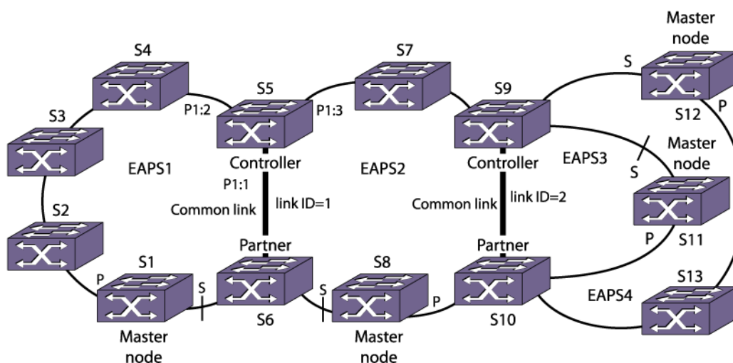
Figure 127: Basic Core Topology
