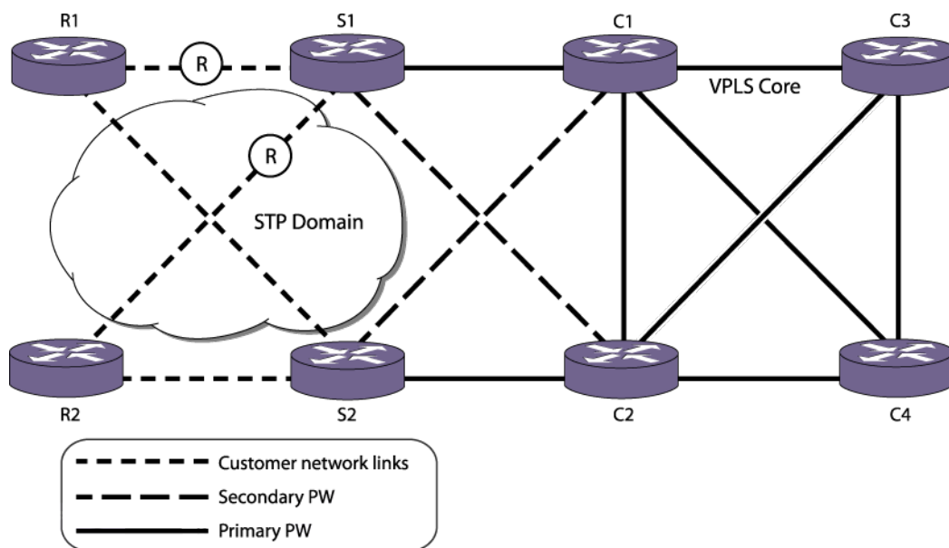
Figure 200: Redundant Edge H-VPLS Network with STP Example
