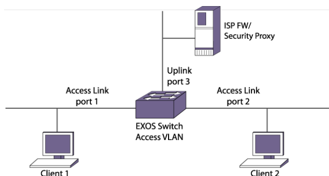
Figure 84: Upstream Forwarding or Disabling Egress Flooding Example
