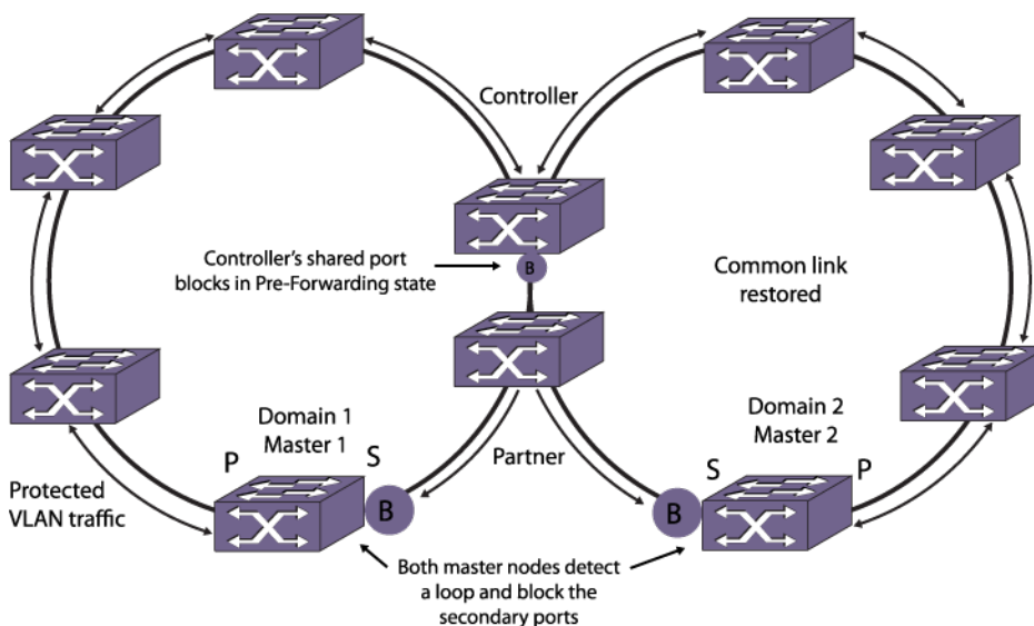
Figure 124: Common Link in Pre-Forwarding State
