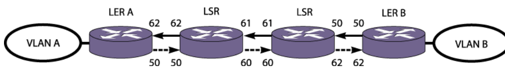
Figure 205: Static LSP Example
