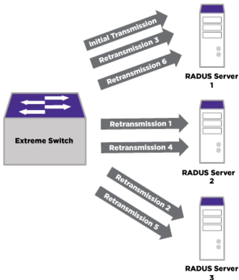
Figure 112: Authentication Retransmission Algorithm for a Single RADIUS Transaction (No Servers Responding 1)
