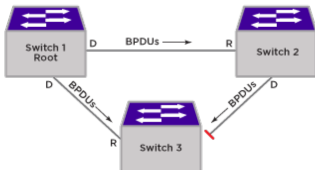
Figure 144: Switch 1 Elected as Root
