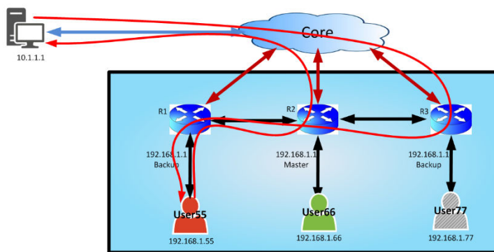
Figure 185: Asymmetric Routing and VRRP (2)
