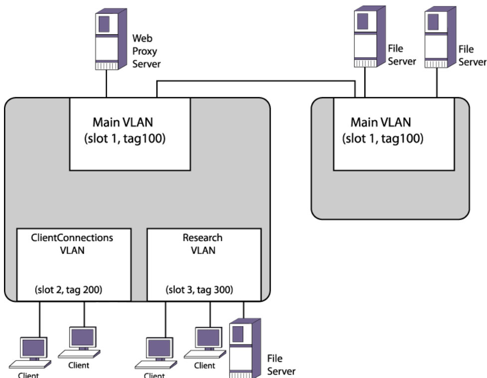
Figure 72: PVLAN Configuration Example 1
