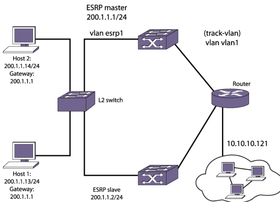
Figure 176: ESRP Tracking
