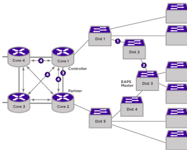
Figure 201: VPLS with Redundant EAPS Configuration Example
