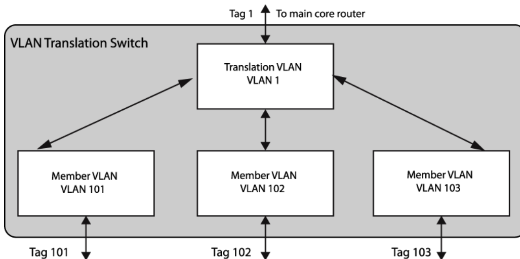
Figure 74: VLAN Translation Switch Configuration
