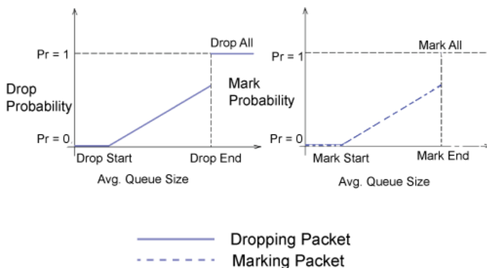
Figure 93: WRED Behavior with and without ECN
