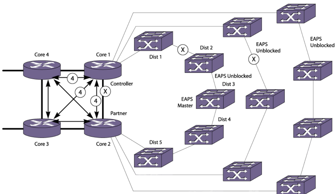
Figure 202: VPLS with Parallel Redundant EAPS Rings Configuration Example
