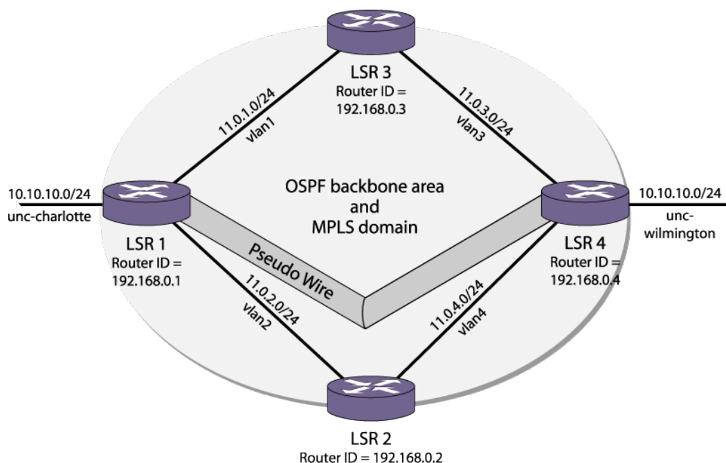
Figure 208: MPLS VPLS Configuration Example
