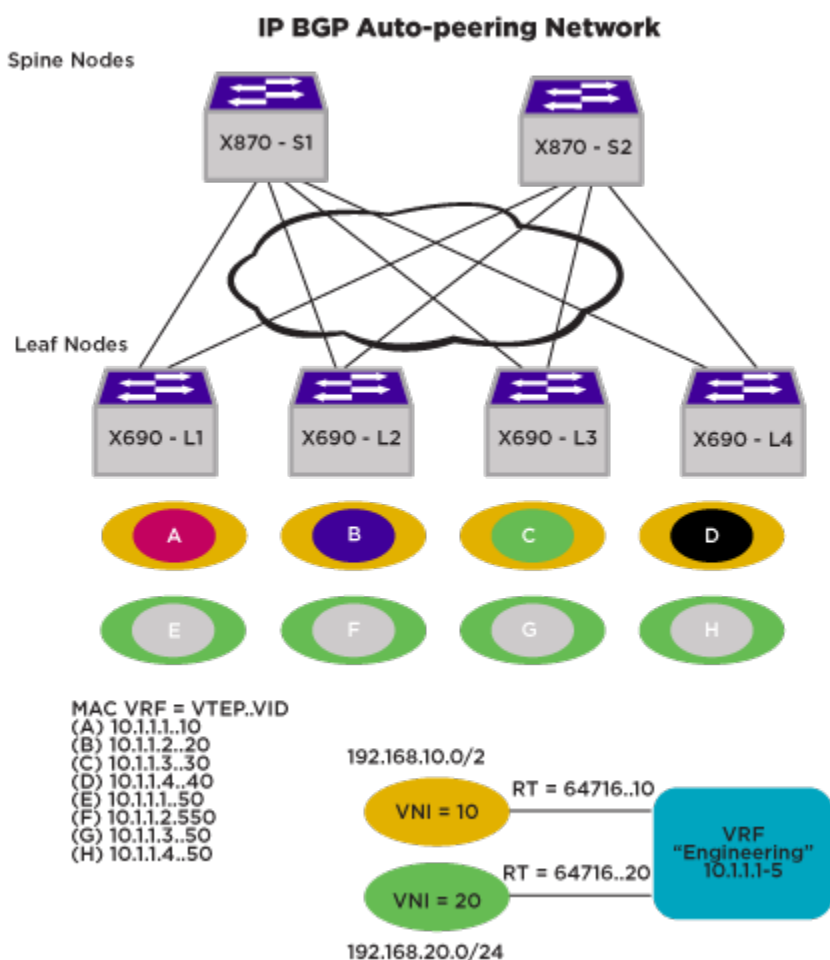
Figure 45: EVPN and Asymmetric VRF Routing in BGP Auto-peering
