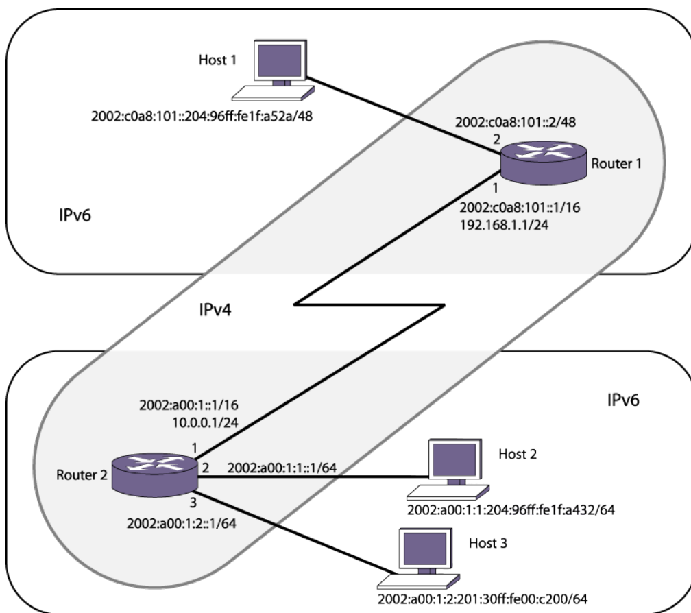
Figure 221: 6to4 Tunnel Configuration Example
