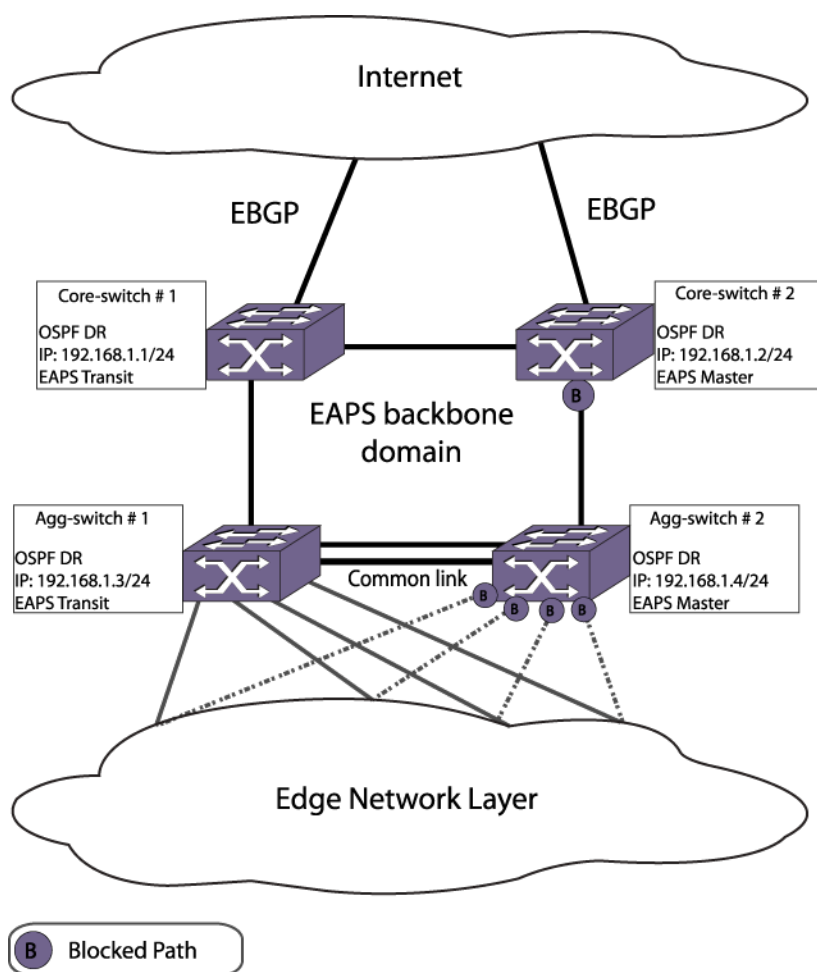
Figure 137: Core EAPS and OSPF Network Layer
