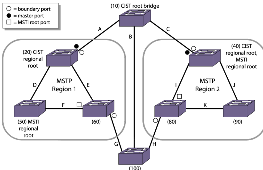
Figure 164: Sample MSTP Topology with Two MSTP Regions
