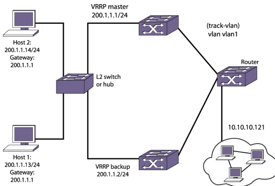
Figure 187: VRRP Tracking
