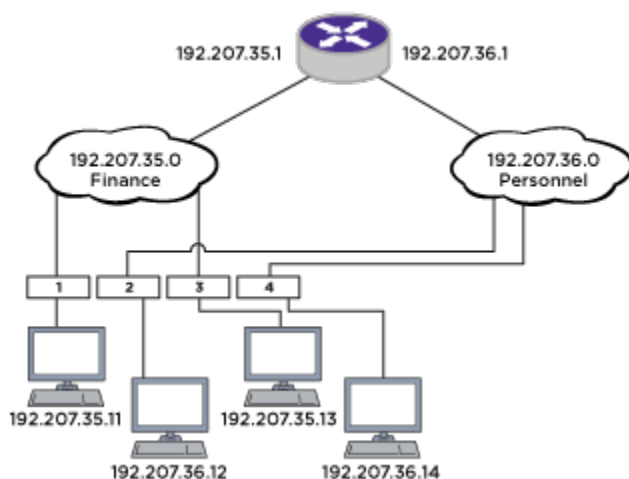
Figure 211: Routing Between VLANs
