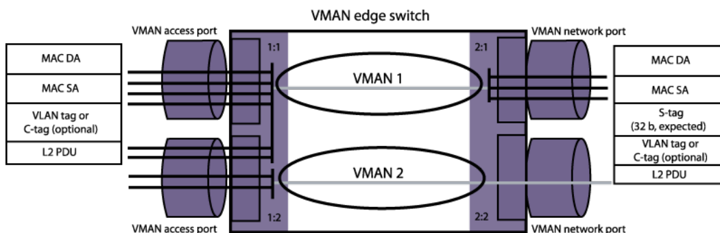
Figure 79: Tag Usage at the VMAN Access Switch
