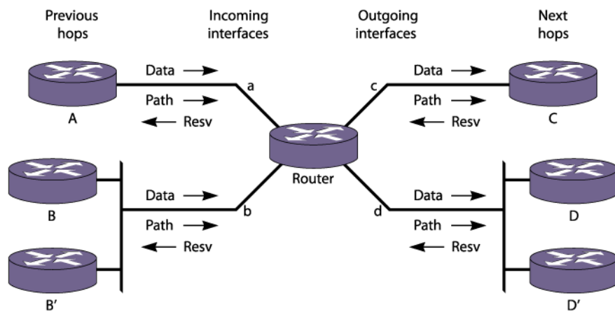
Figure 203: RSVP Messages
