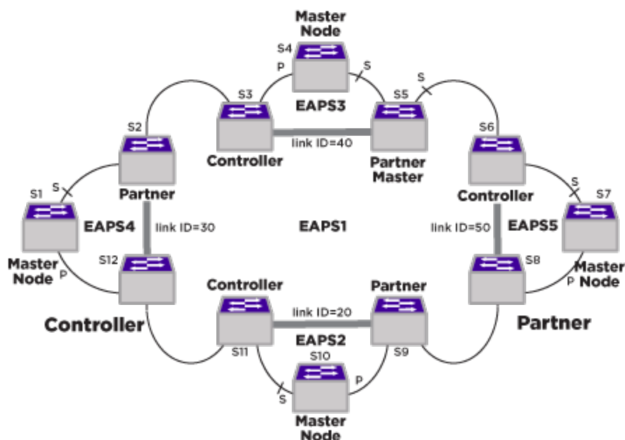
Figure 131: Large Core and Access Ring Topology
