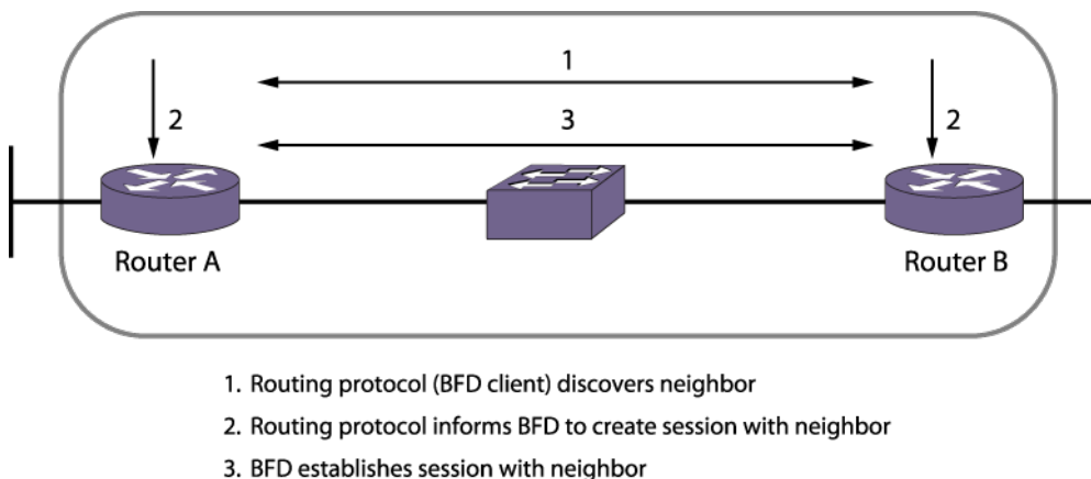
Figure 56: BFD Topology
