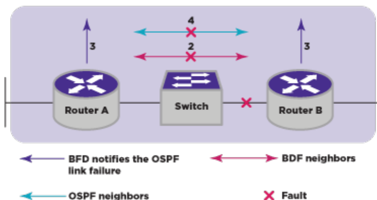
Figure 225: OSPF Neighbor Relationship Eliminated by BFD Fault Detection
