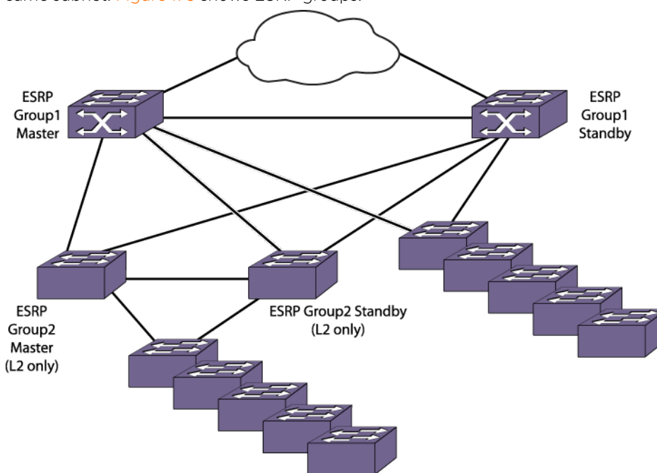
Figure 175: ESRP Groups
