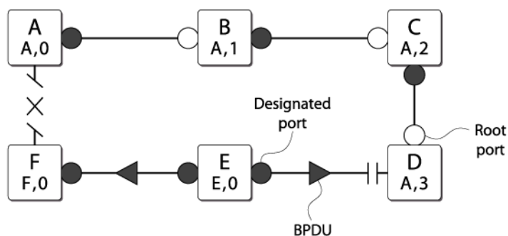
Figure 158: New Root Bridge Selected
