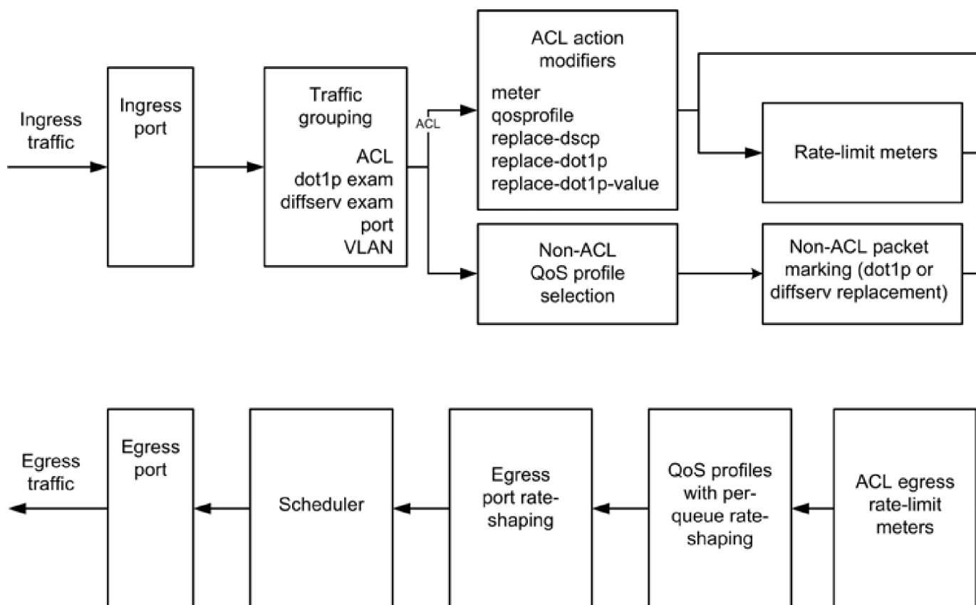
Figure 94: QoS on SummitStack and Summit Family Switches
