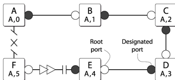
Figure 162: Completing the Topology Change
