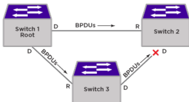
Figure 145: STP Disabled on Switch 2
