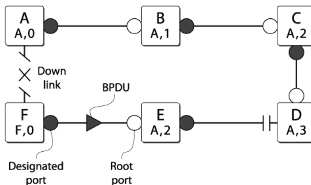
Figure 157: Down Link Detected
