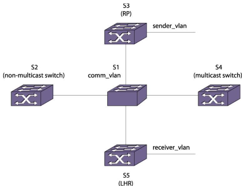
Figure 255: PIM Snooping Configuration Example
