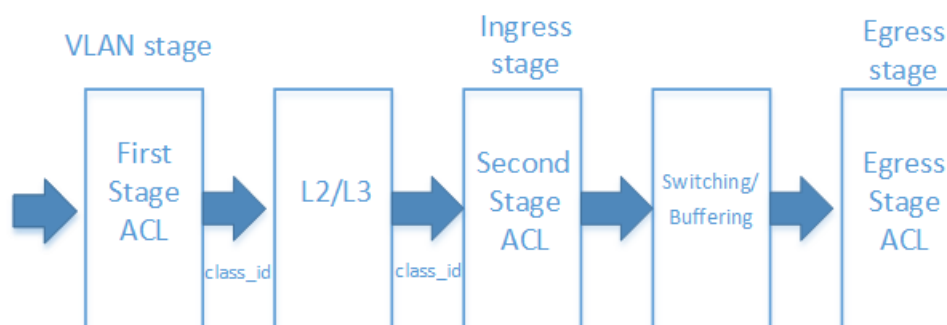
Figure 87: ACL Stages
