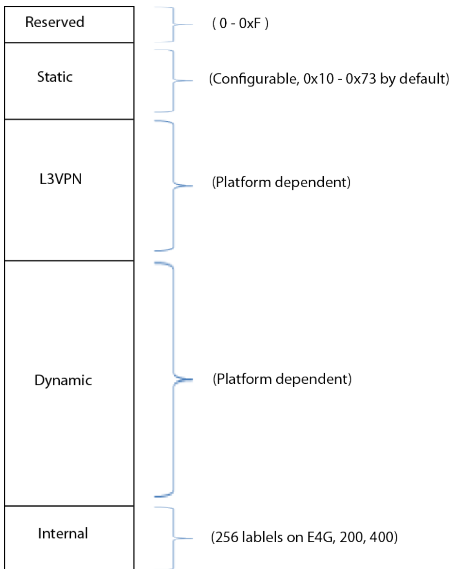
Figure 193: MPLS Label Space Partitions
