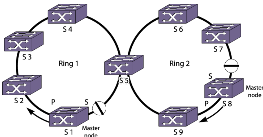
Figure 119: Two Rings Interconnected by One Switch
