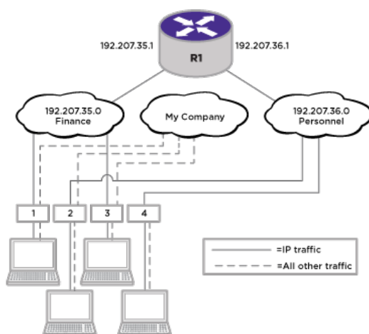
Figure 66: Protocol-Based VLANs
