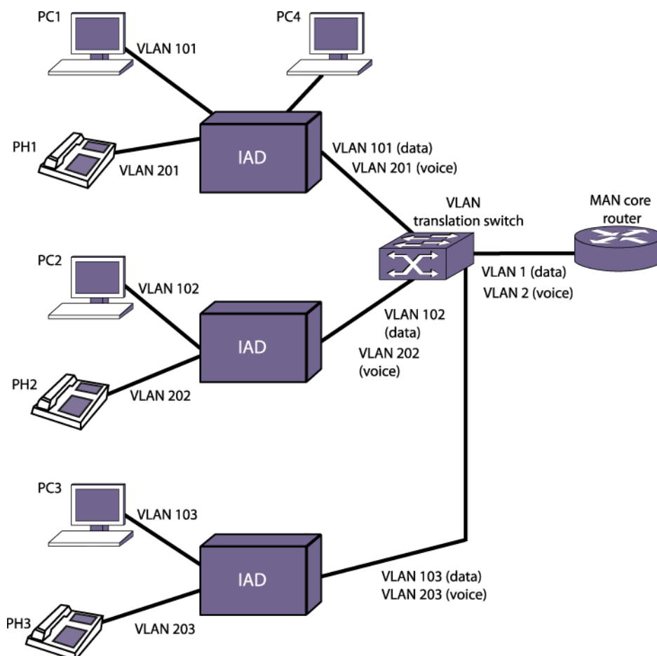
Figure 67: VLAN Translation Application
