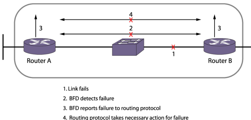
Figure 57: BFD Failure Detection
