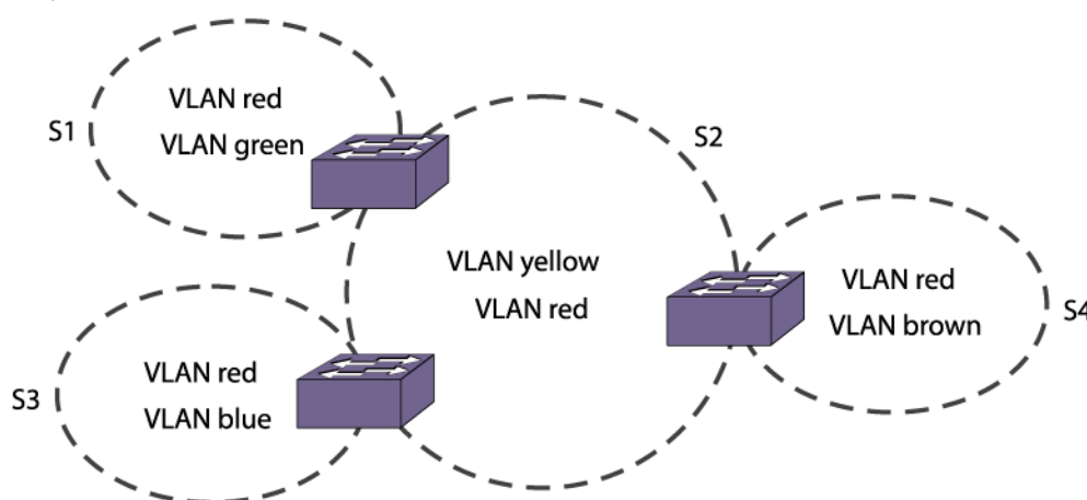
Figure 152: VLANs Spanning Multiple STPDs
