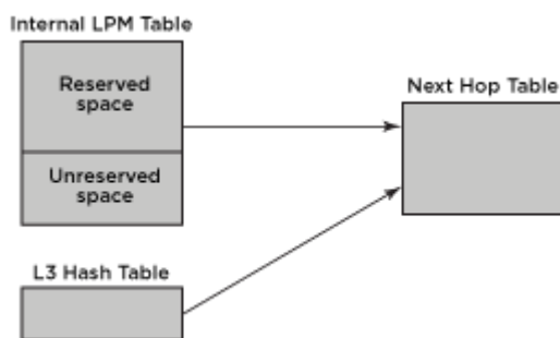
Figure 213: Hardware Forwarding Tables
