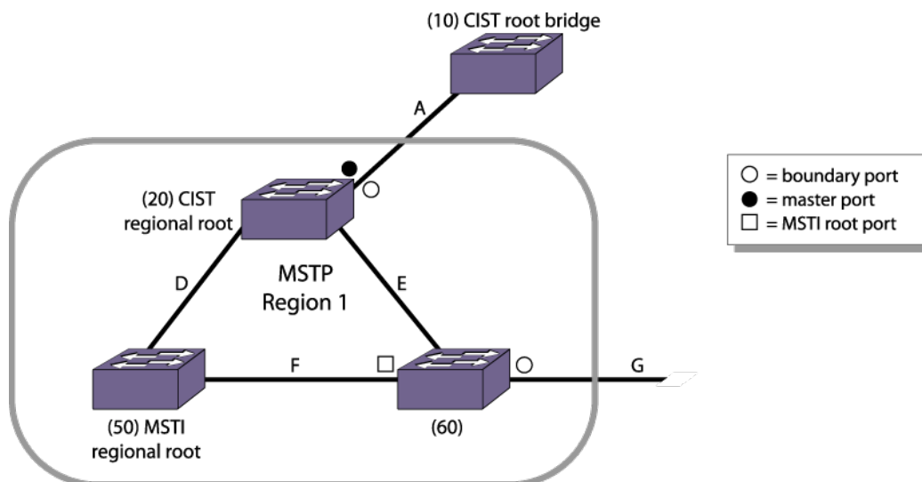
Figure 165: Closeup of MSTP Region 1
