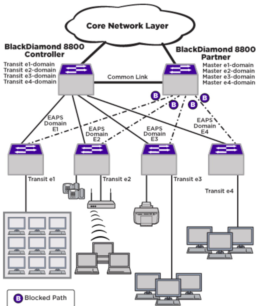
Figure 135: L2 Aggregation Network Layer
