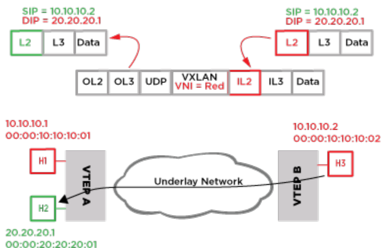
Figure 99: Routing from a Tunnel
