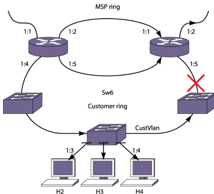
Figure 259: Inter-Multicast VLAN Forwarding
