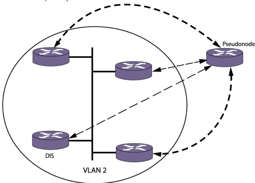
Figure 237: Broadcast Adjacencies in a Four-Router Network
