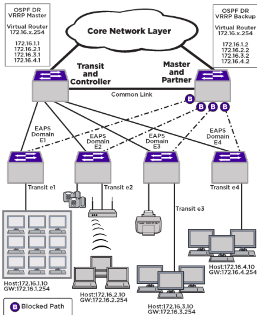
Figure 136: L2 and L3 Aggregation Network Layer
