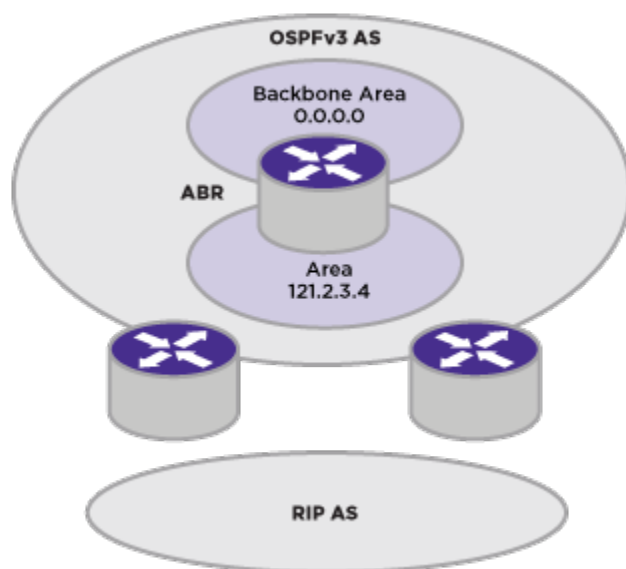
Figure 234: OSPFv3 Route Redistribution
