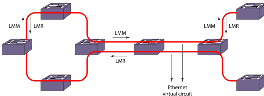
Figure 53: Two-Way Frame-Loss Measurement
