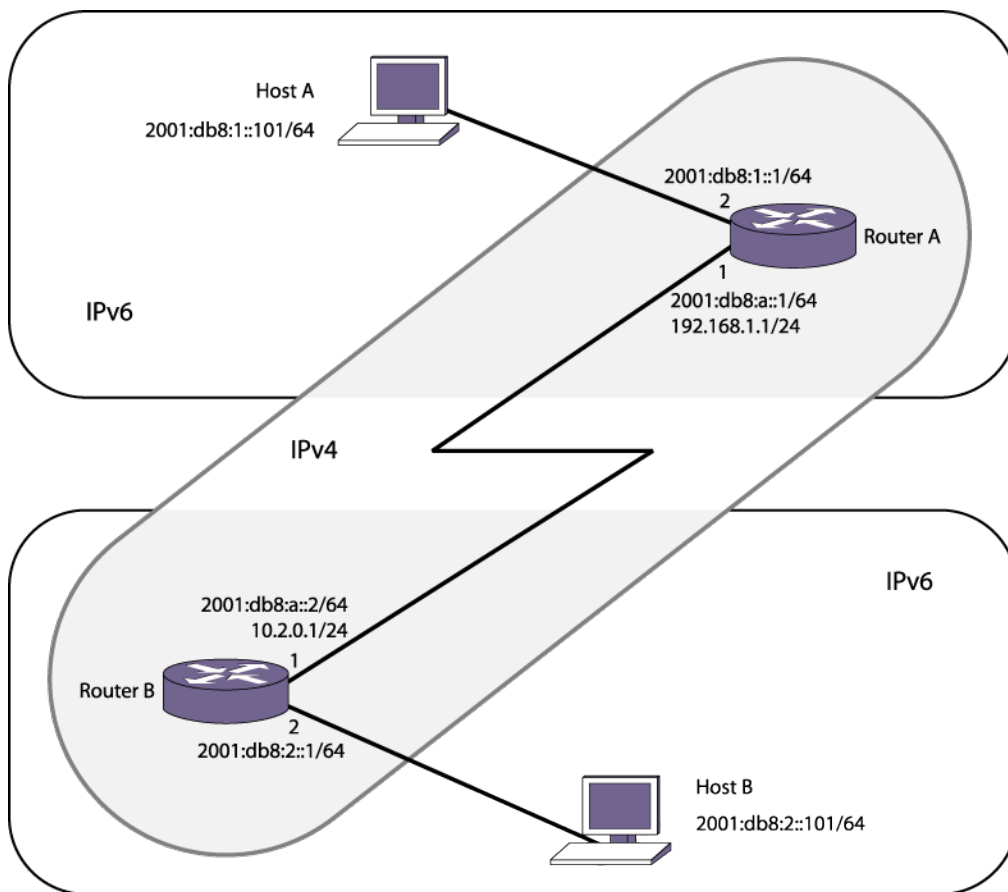
Figure 220: 6in4 Tunnel Example
