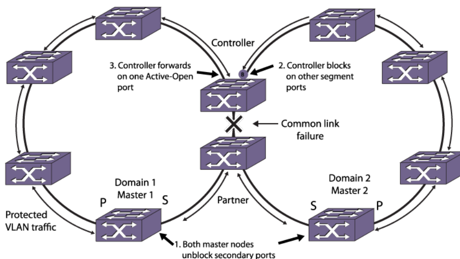
Figure 123: Common Link Failure
