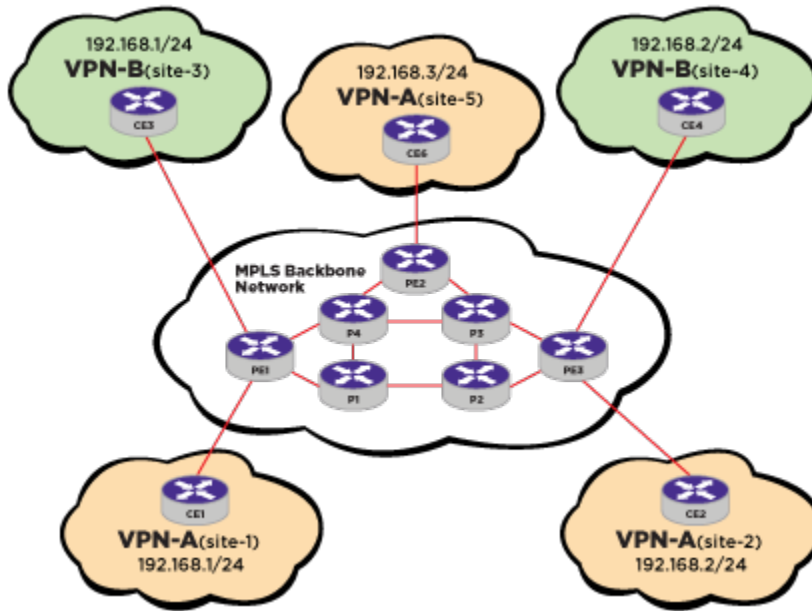
Figure 248: BGP/MPLS VPN Example
