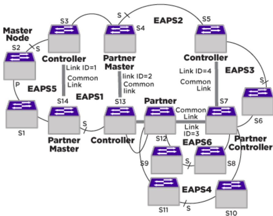
Figure 130: Advanced Basic Core and Right Angle Topology
