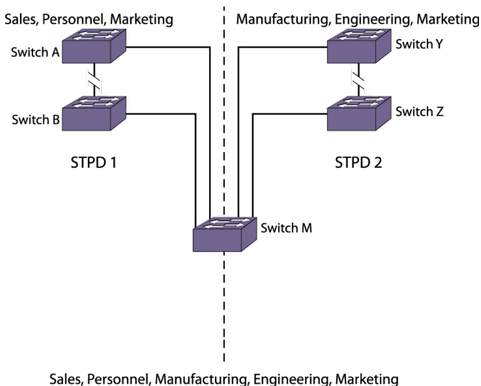
Figure 172: RSTP Example
