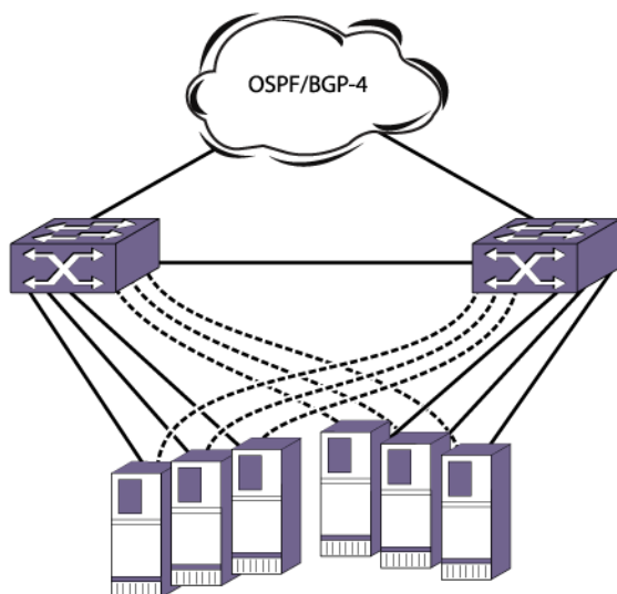
Figure 177: ESRP Host Attach
