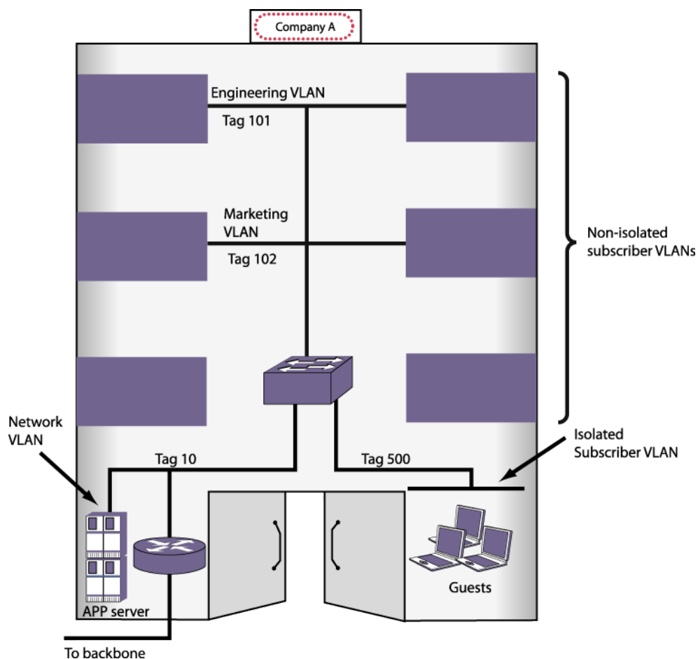
Figure 68: VLAN Isolation Application
