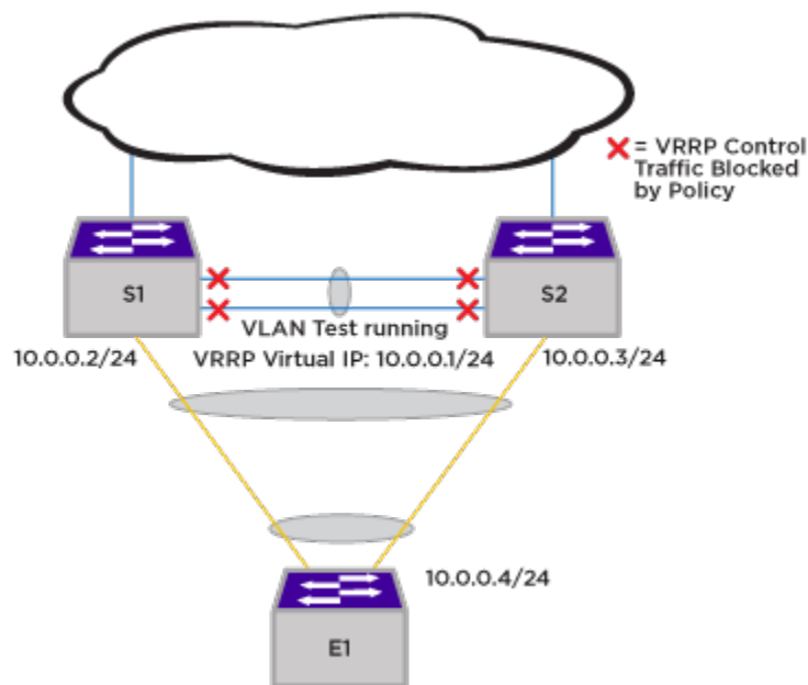
Figure 182: VRRP Active-Active
