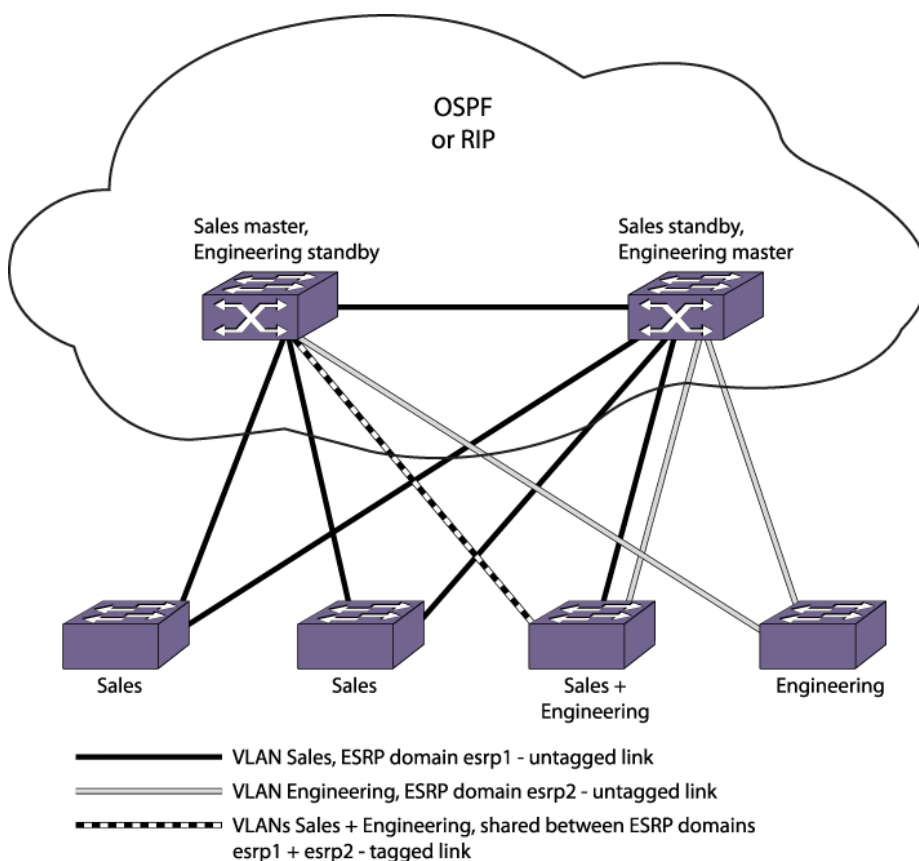
Figure 179: Multiple ESRP Domains Using Layer 2 and Layer 3 Redundancy
