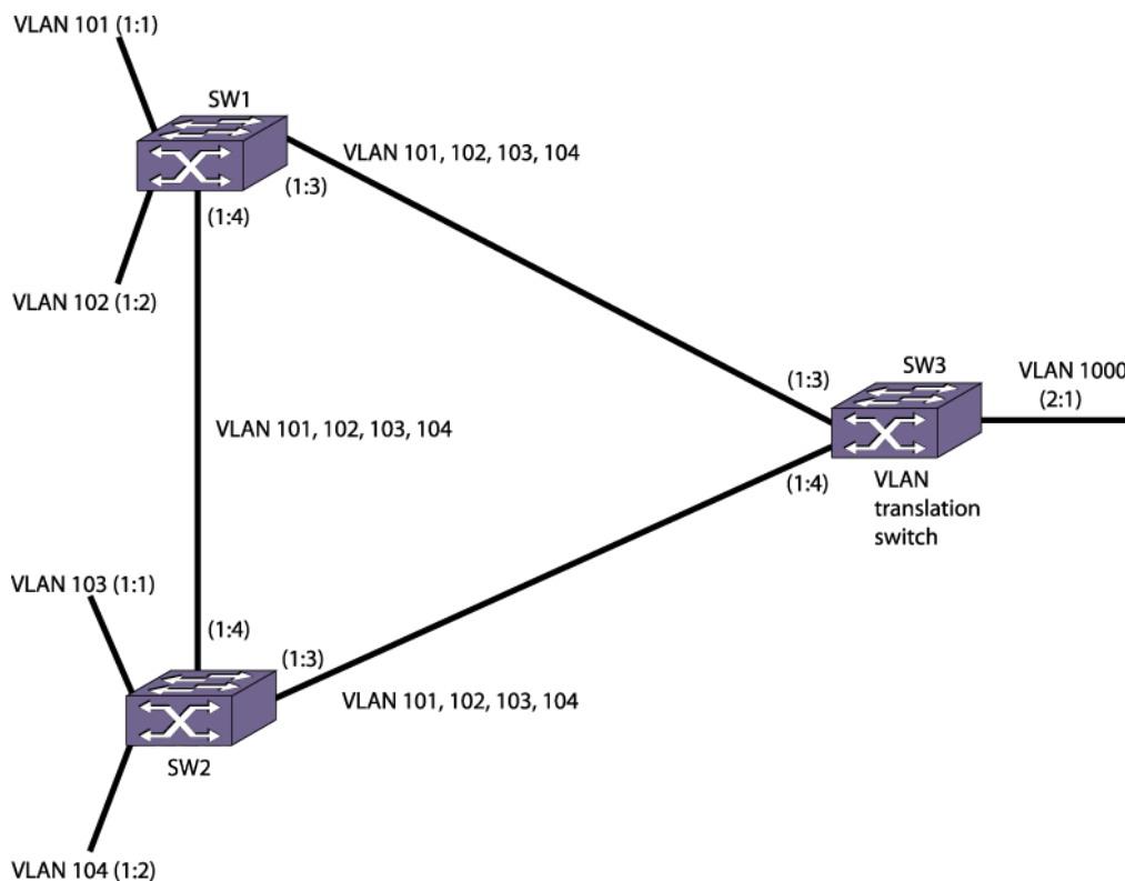
Figure 77: STP Redundancy Configuration Example
