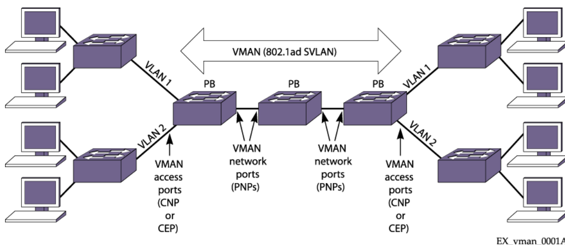
Figure 78: VMAN in PBN
