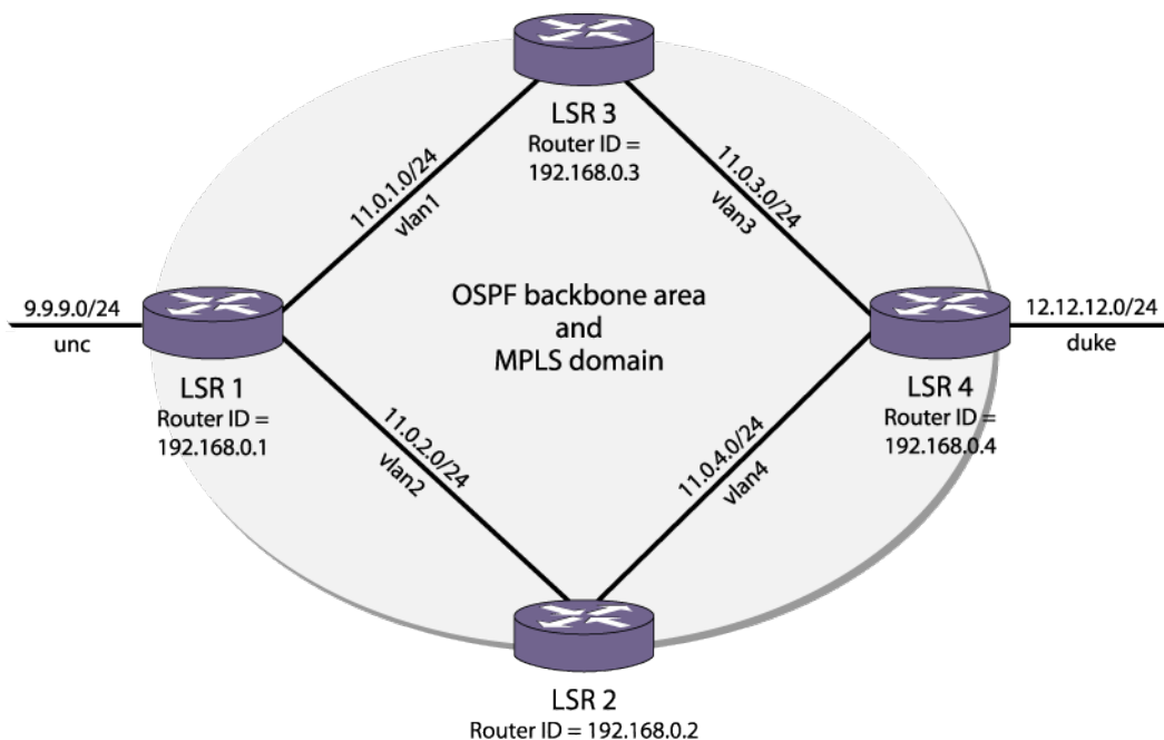
Figure 207: MPLS Configuration Example
