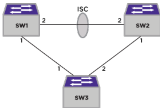
Figure 264: ELRP Egress Port Disable (2)
