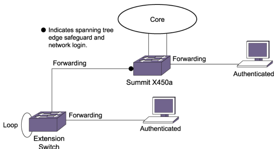
Figure 169: Traffic Monitoring on the Edge Side
