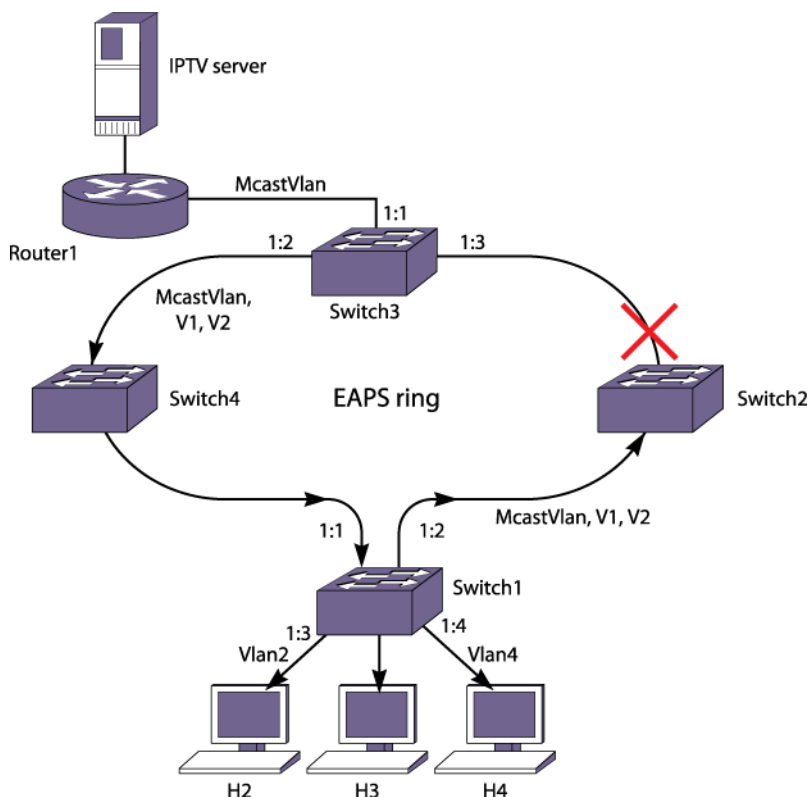
Figure 260: MVR on an EAPS Ring
