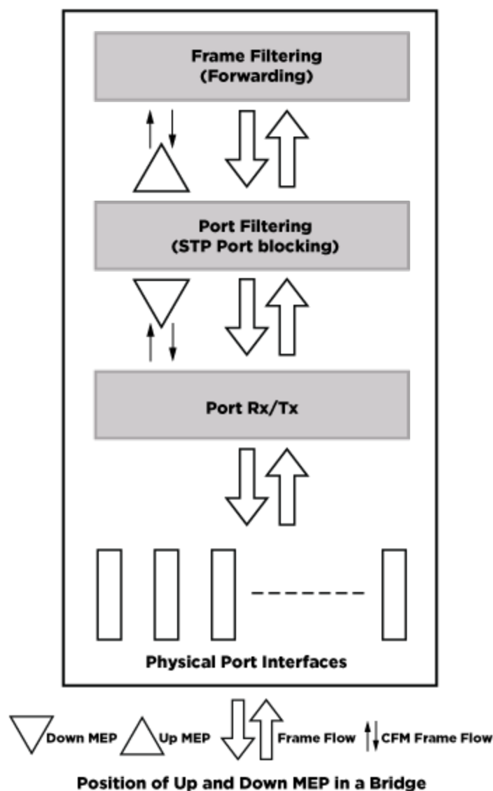
Figure 49: CFM UP and DOWN MEP at the Logical Level
