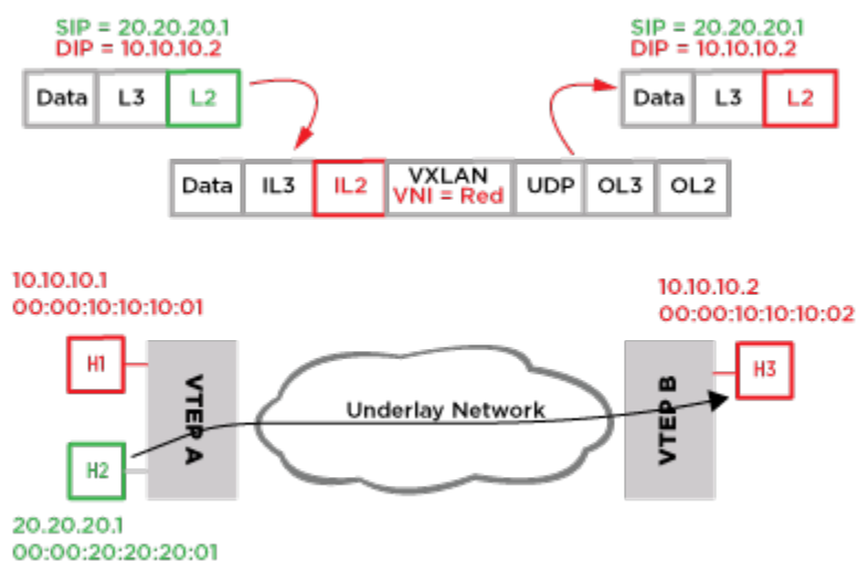
Figure 98: Routing into a Tunnel
