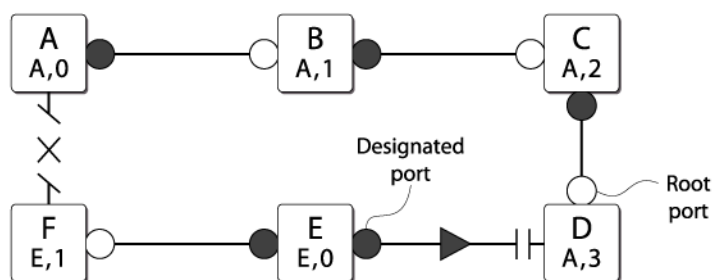
Figure 159: Communicating New Root Bridge Status to Neighbors
