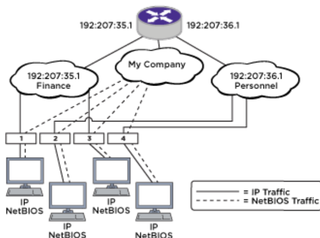
Figure 214: Unicast Routing Configuration Example
