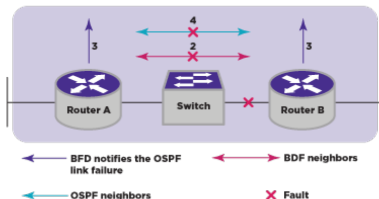
Figure 231: OSPFv3 Neighbor Relationship Eliminated by BFD Fault Detection
