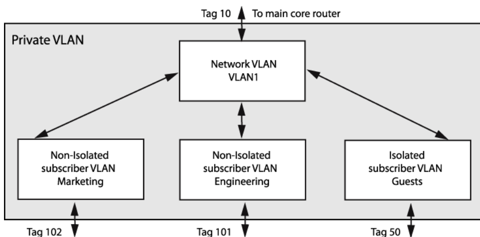
Figure 69: Private VLAN Switch Components
