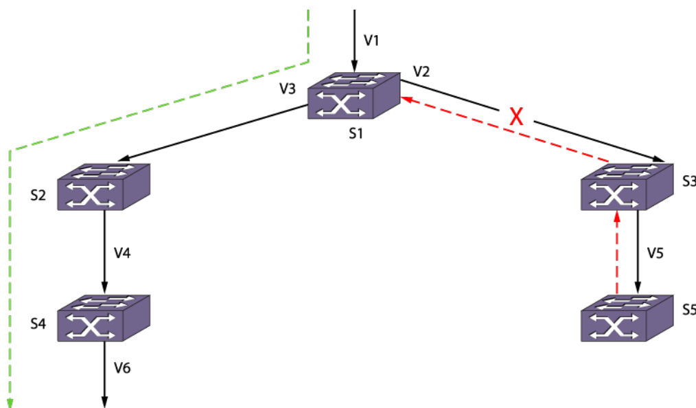
Figure 250: PIM-DM Operation
