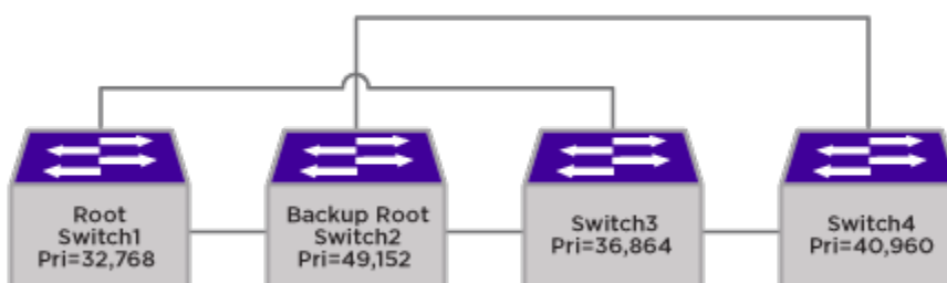
Figure 143: STP Root Bridge Loss Example
