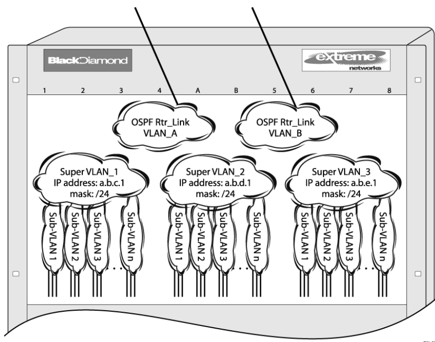
Figure 216: VLAN Aggregation
