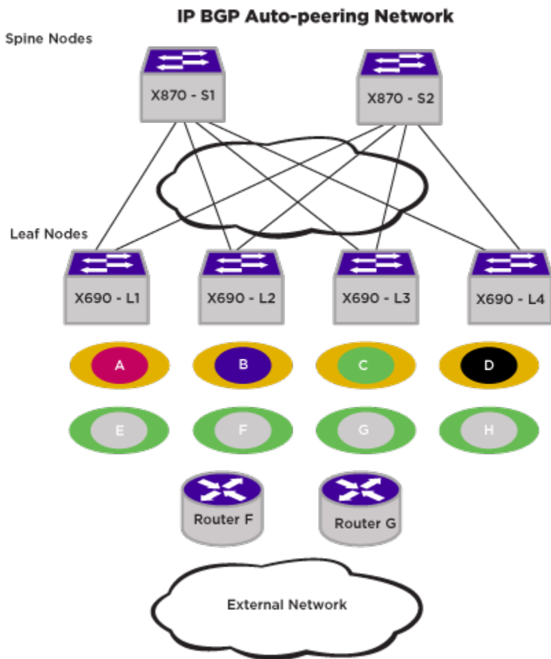
Figure 46: EVPN and Asymmetric VRF Routing in BGP Auto-peering with Routers
