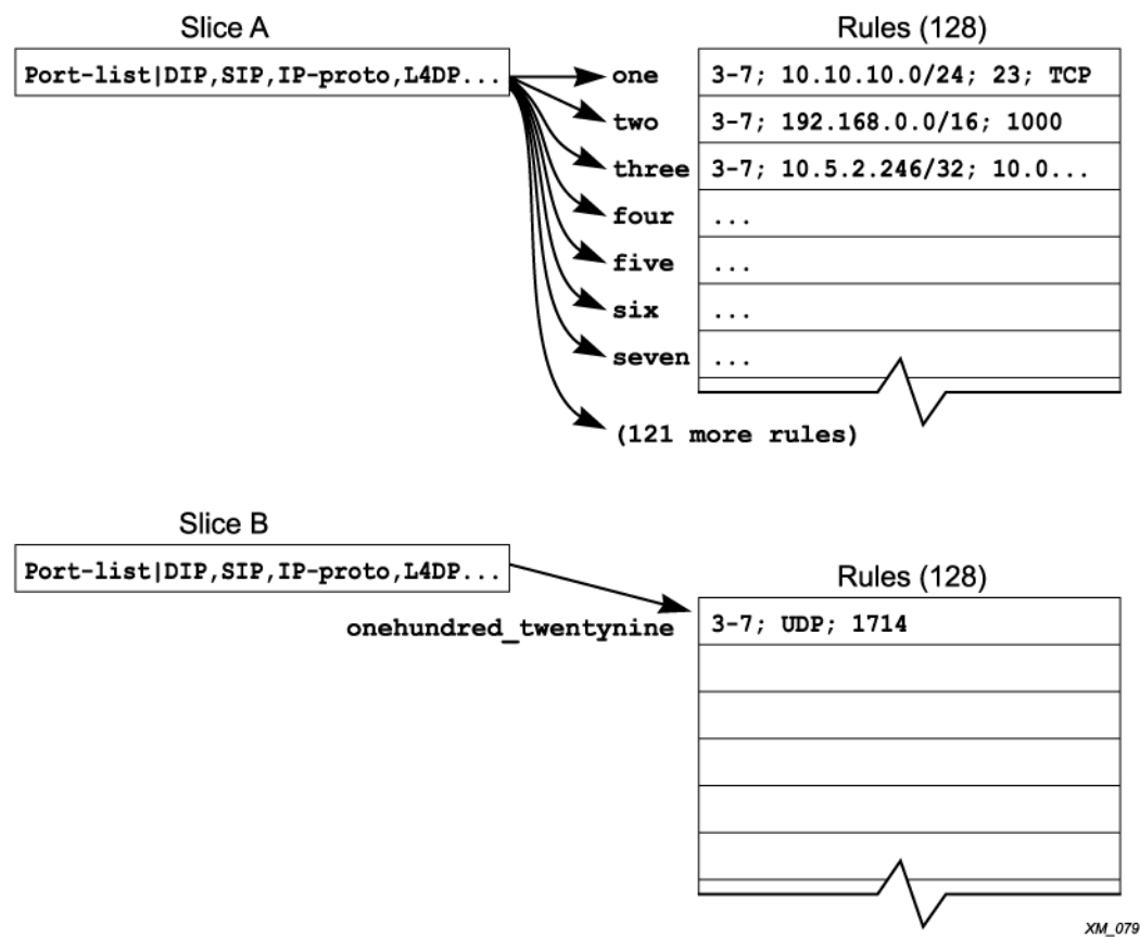
Figure 89: ACL Entry one Through onehundred_twentynine
