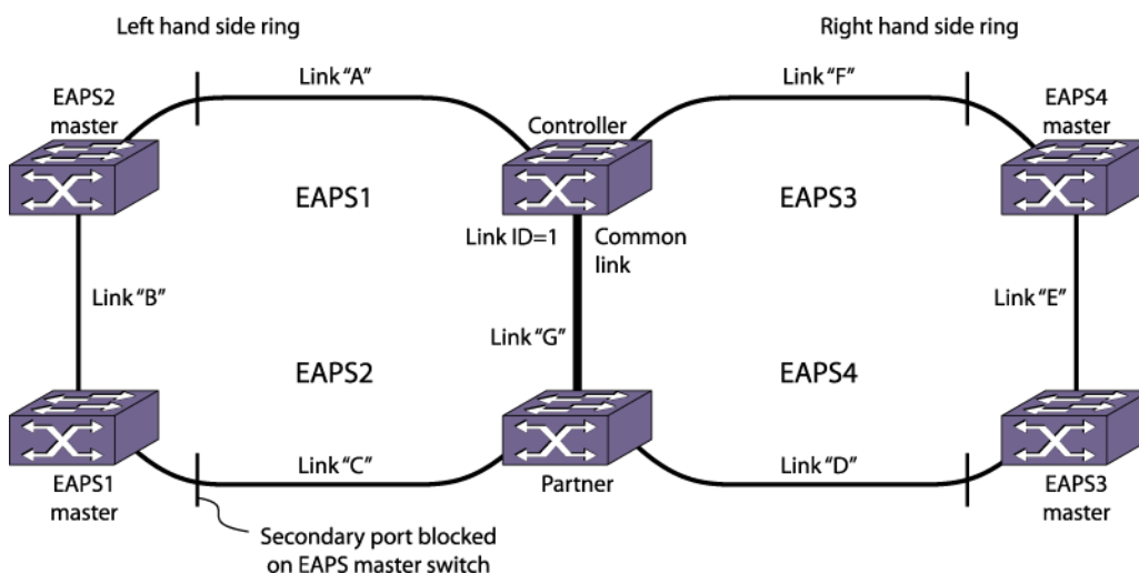
Figure 126: EAPS Common Link Topology with Spatial Reuse
