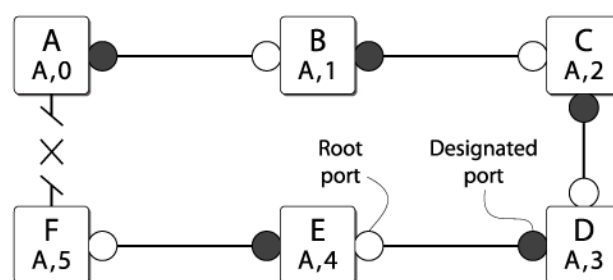
Figure 163: Final Network Configuration
