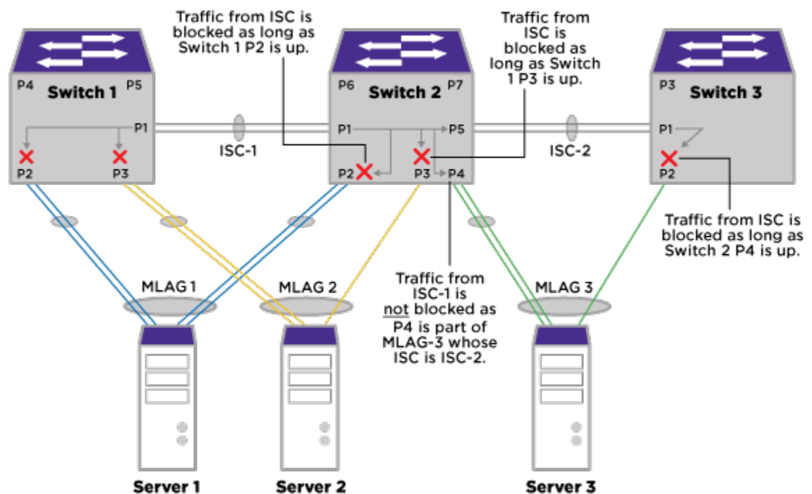
Figure 20: Traffic Flow
