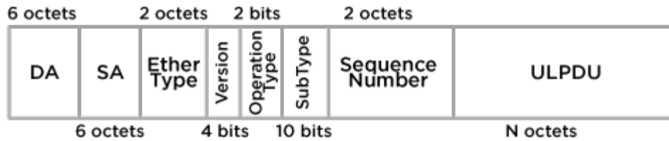
Figure 36: ECPDU Structure
