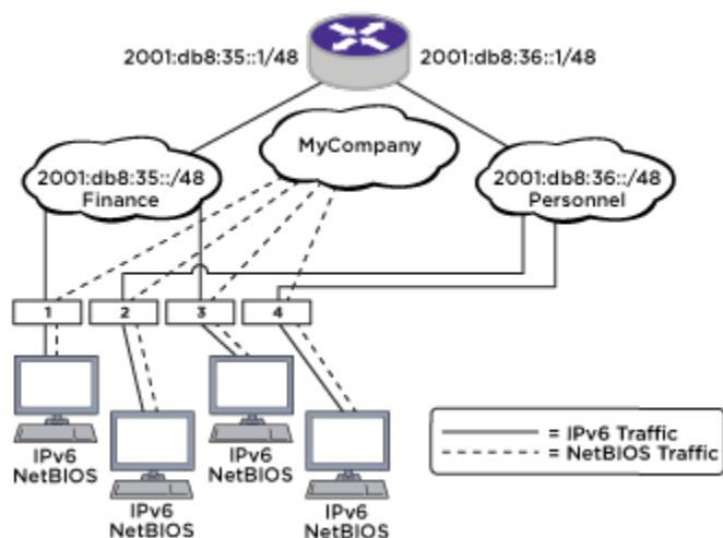
Figure 219: IPv6 Unicast Routing Configuration Example
