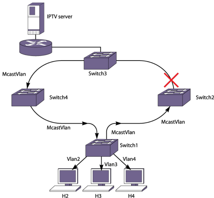
Figure 257: Basic MVR Deployment
