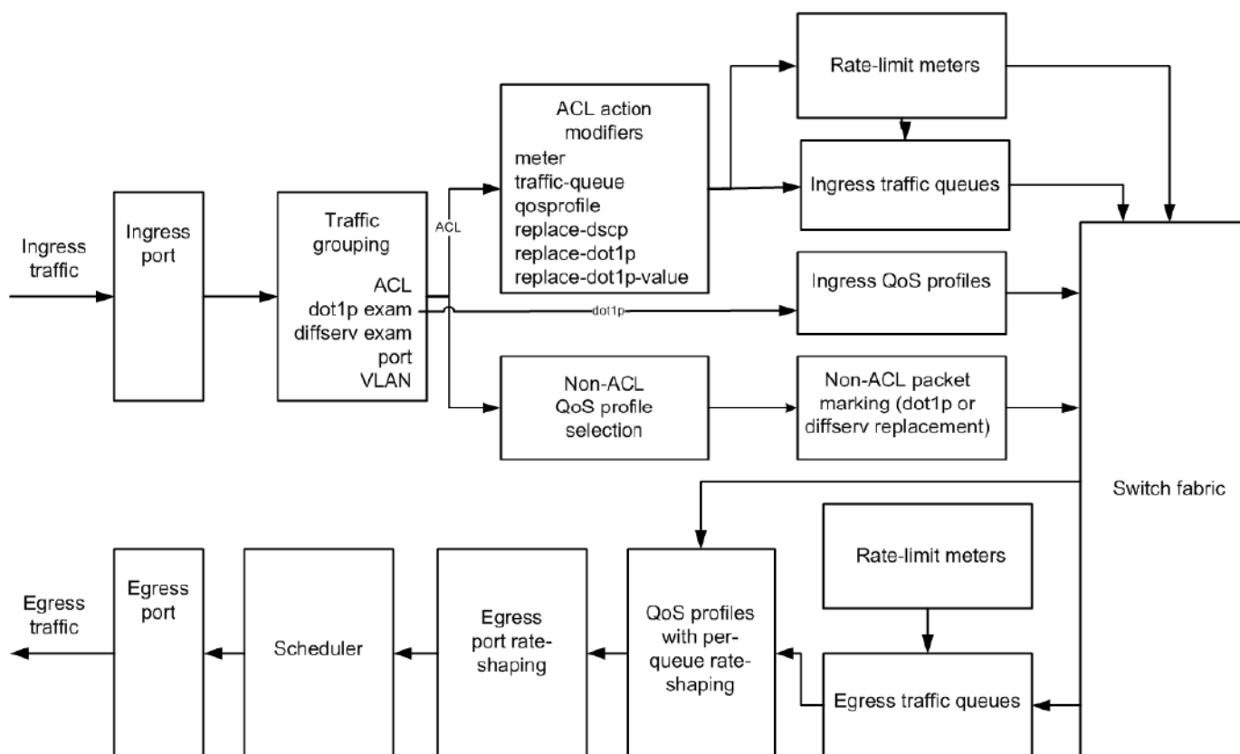
Figure 90: QoS on Extreme Networks Switches
