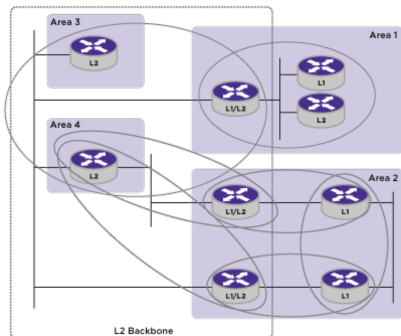
Figure 238: Basic Autonomous System
