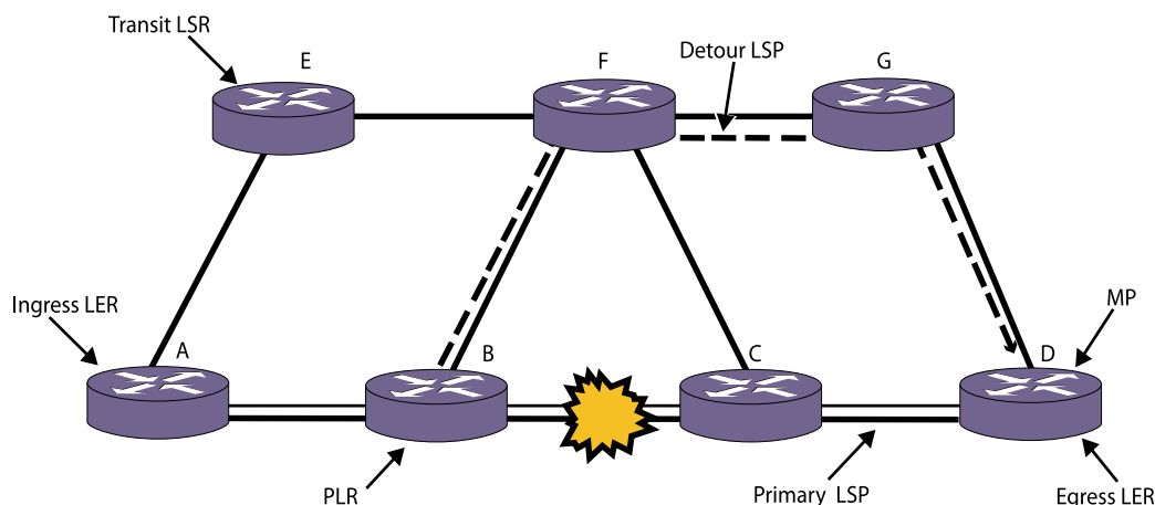
Figure 213: Fast-Reroute Terminology
