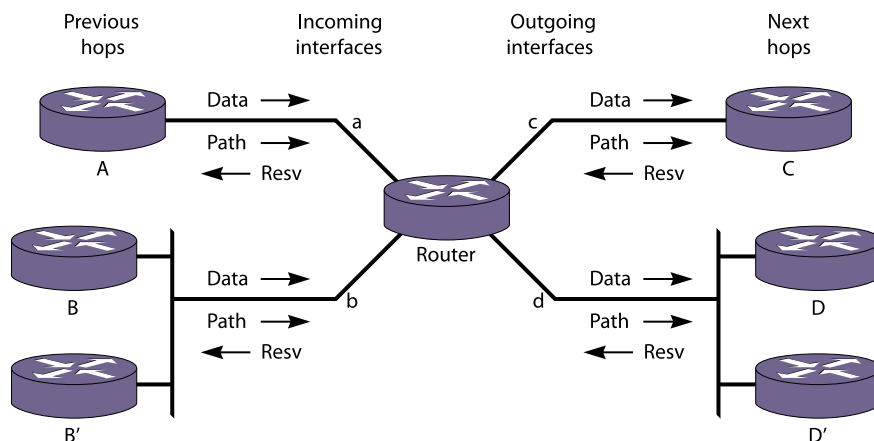
Figure 212: RSVP Messages
