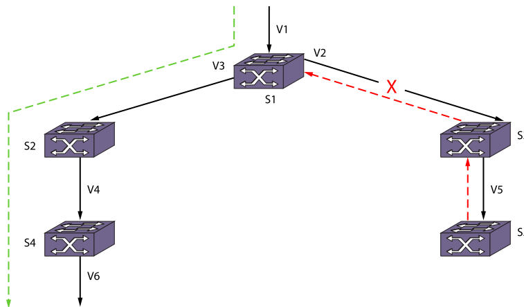
Figure 259: PIM-DM Operation
