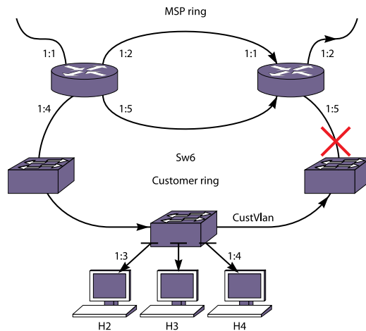
Figure 268: Inter-Multicast VLAN Forwarding
