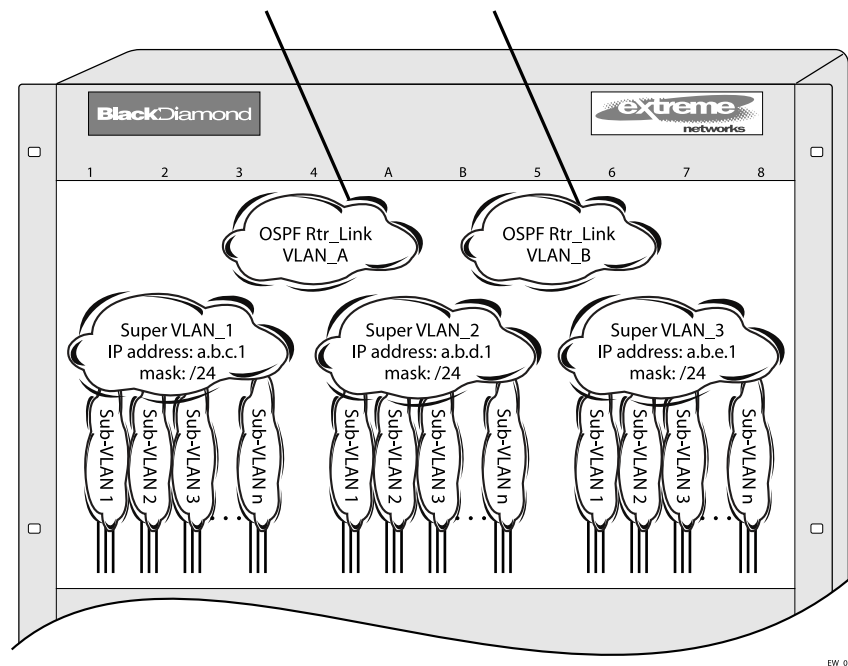
Figure 225: VLAN Aggregation
