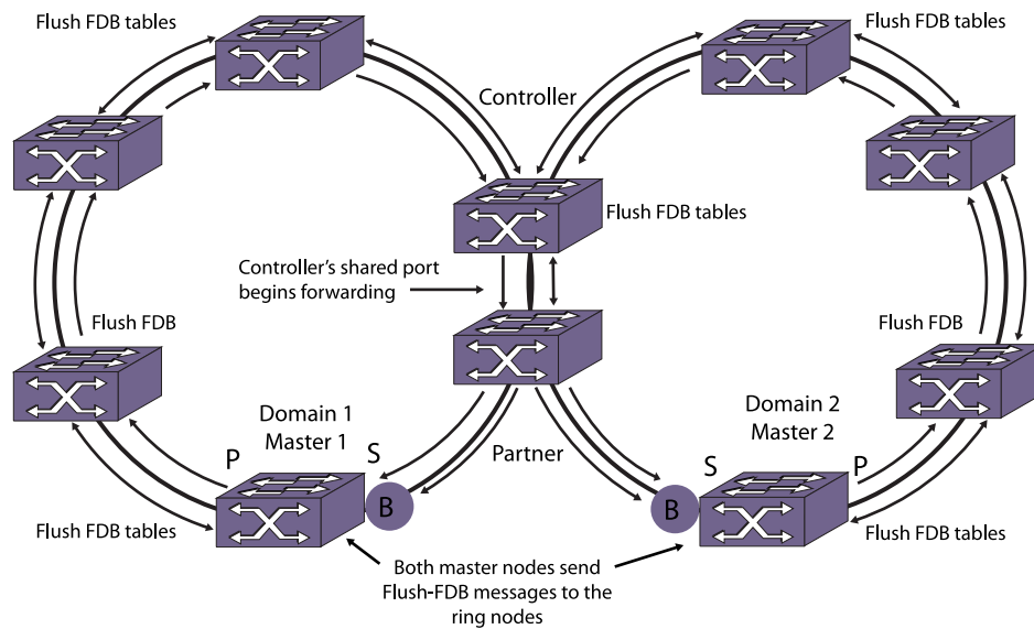
Figure 134: Common-Link Restored
