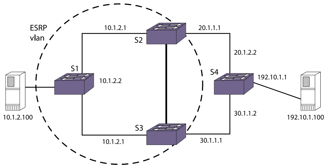
Figure 116: MAC Address Limits and VLANs Participating in ESRP
