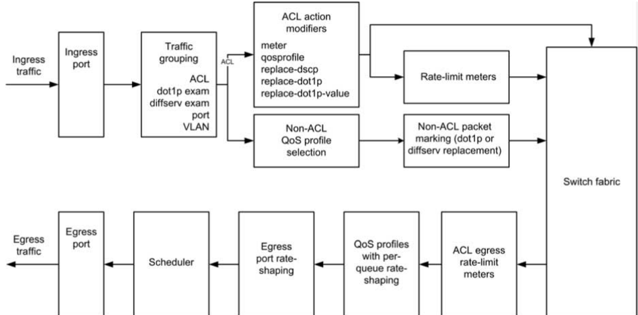
Figure 103: QoS on SummitStack and ExtremeSwitching Switches
