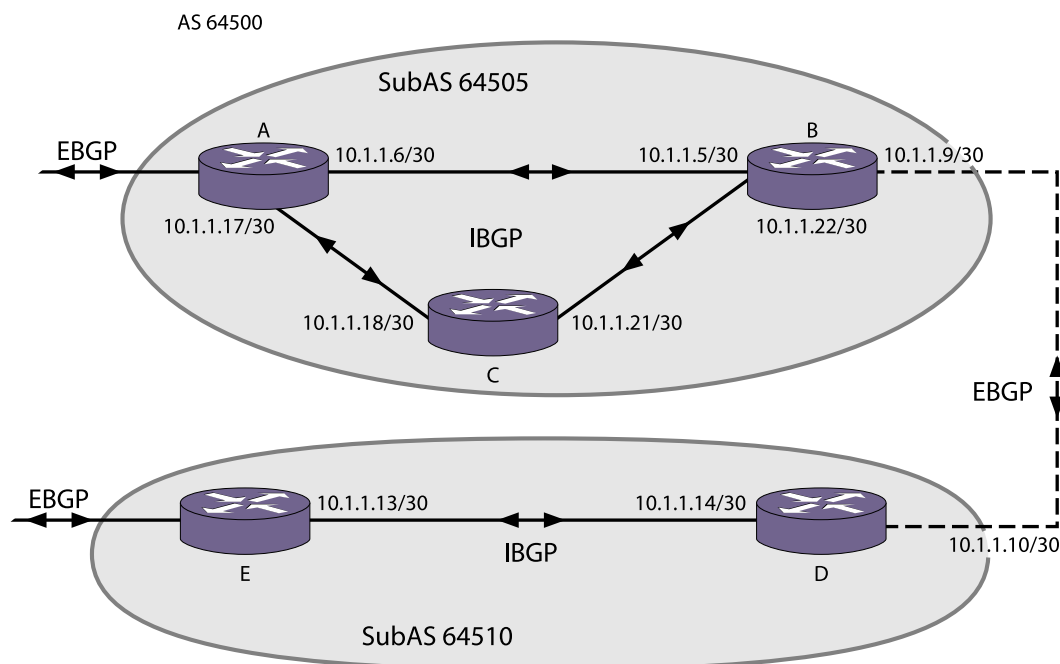
Figure 250: Routing Confederation
