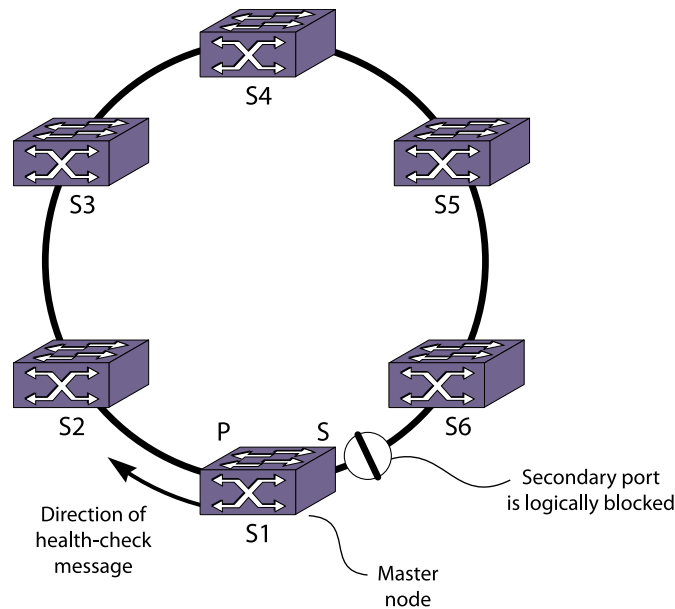
Figure 127: EAPS Operation
