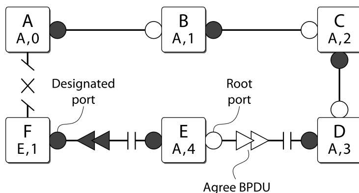
Figure 170: Communicating Port Status to Neighbors
