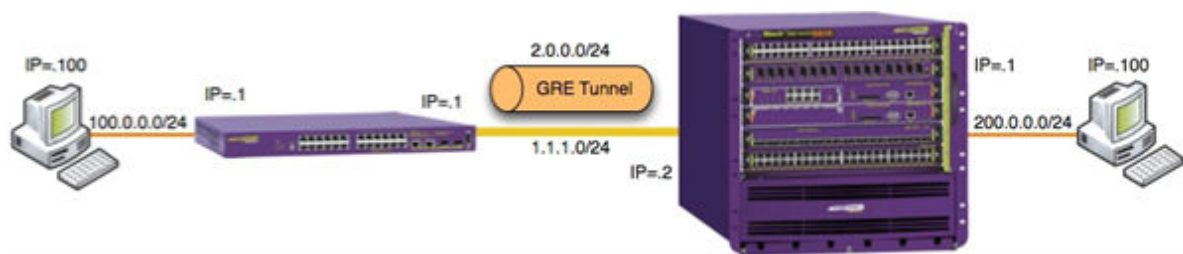
Figure 221: GRE Tunnel Configuration
