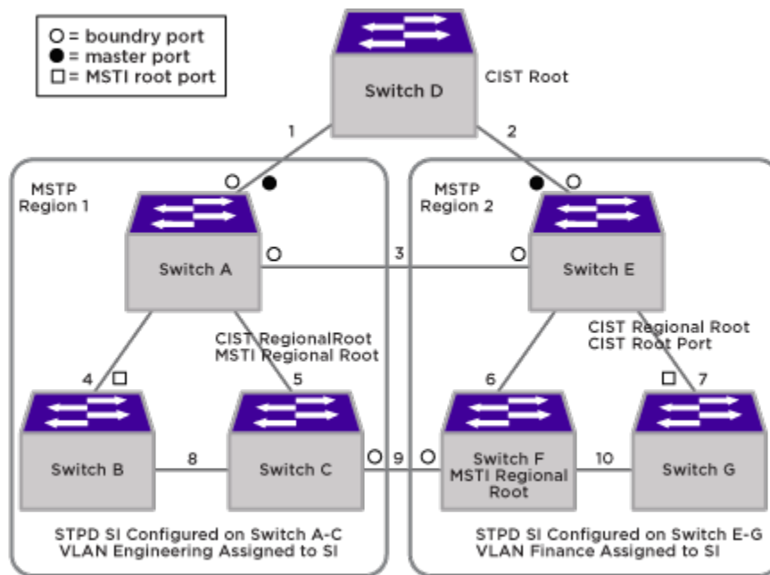
Figure 182: MSTP Configuration Example
