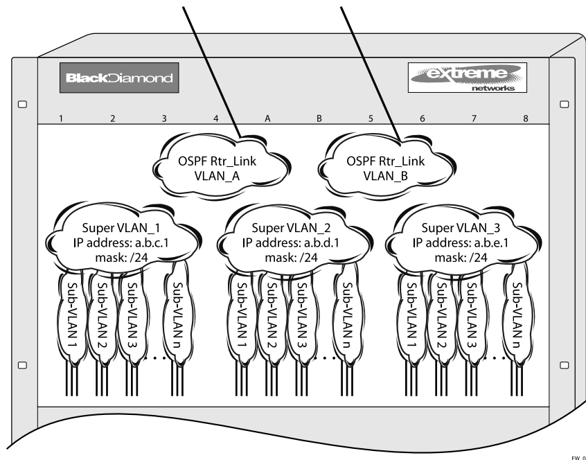
Figure 225: VLAN Aggregation
