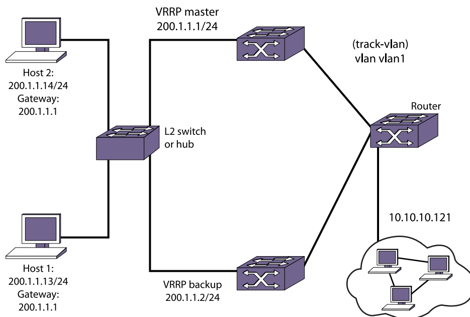
Figure 196: VRRP Tracking
