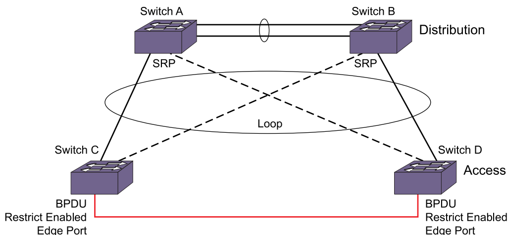
Figure 157: BPDU Restrict
