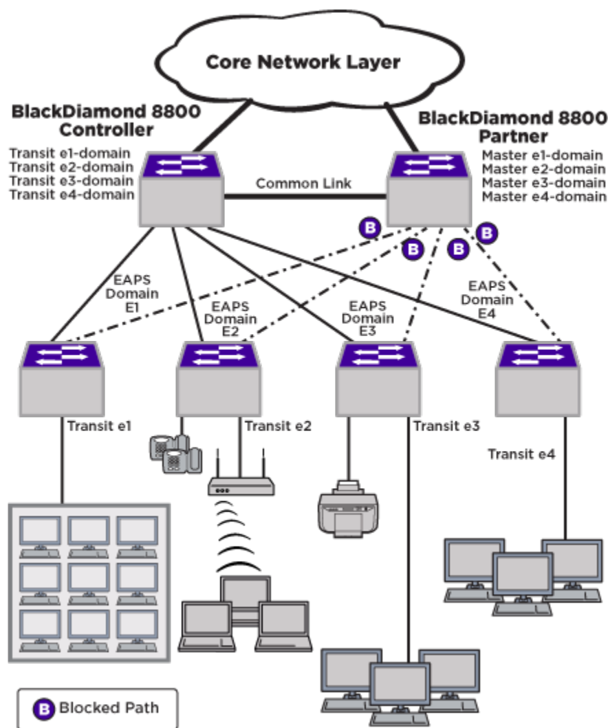
Figure 144: L2 Aggregation Network Layer
