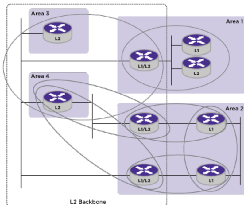
Figure 247: Basic Autonomous System
