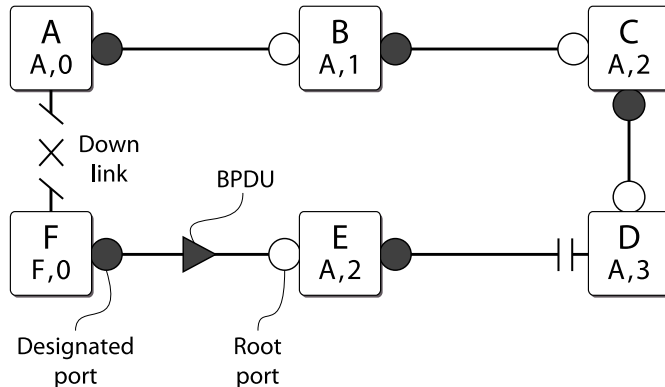
Figure 166: Down Link Detected
