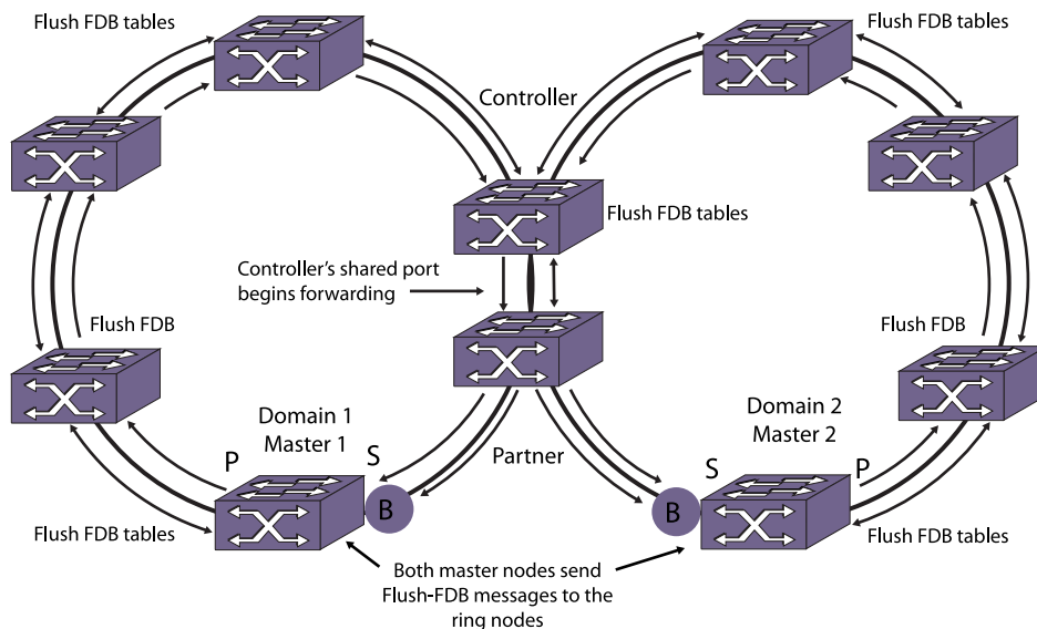
Figure 134: Common-Link Restored
