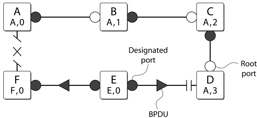
Figure 167: New Root Bridge Selected
