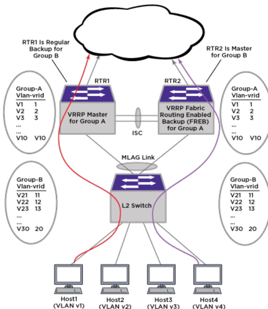
Figure 195: Example VRRP Group Configuration
