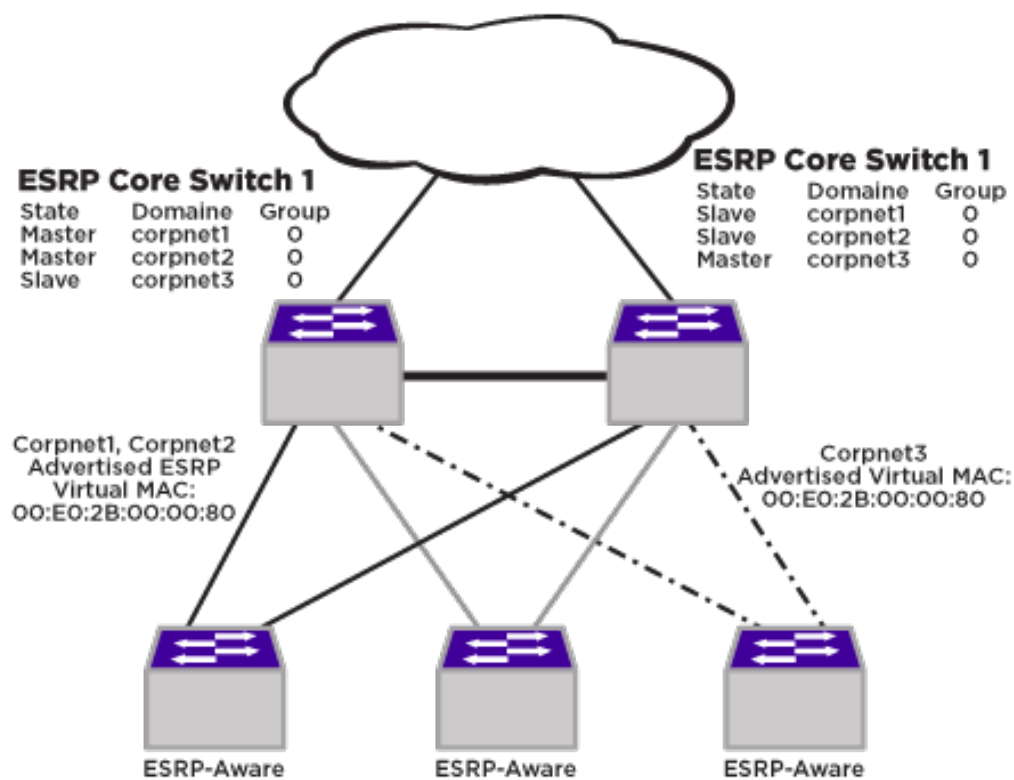
Figure 183: Example of a Basic ESRP Topology
