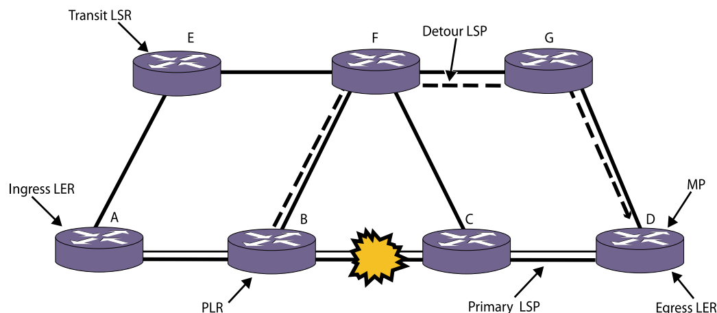
Figure 213: Fast-Reroute Terminology
