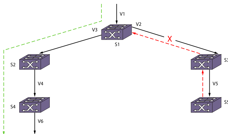
Figure 259: PIM-DM Operation
