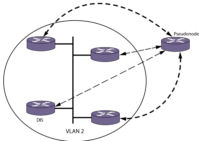
Figure 246: Broadcast Adjacencies in a Four-Router Network
