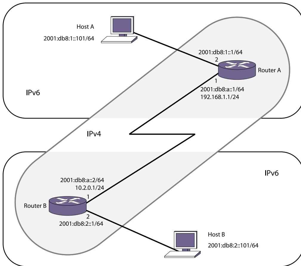
Figure 235: 6in4 Tunnel Example
