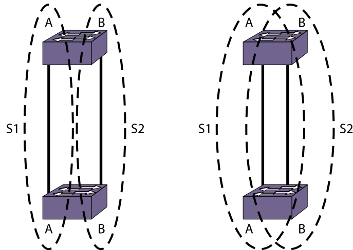
Figure 166: Limitations of Traditional STPD
