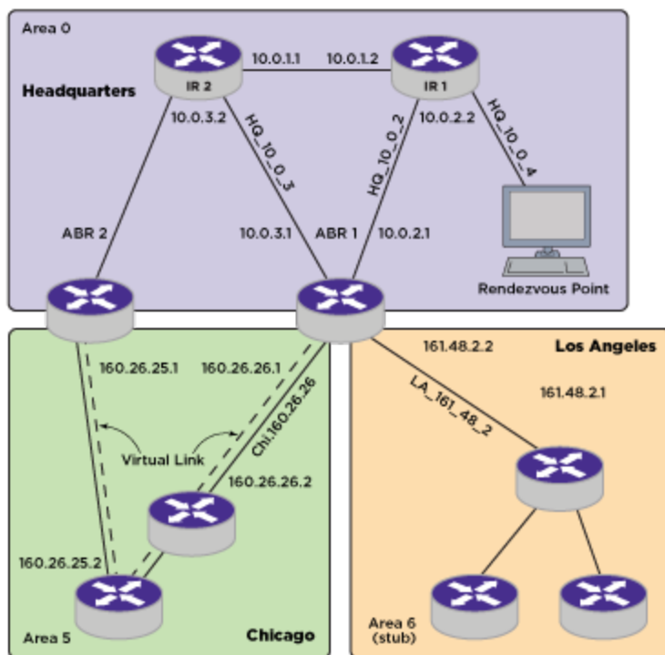
Figure 270: IP Multicast Routing Using PIM-SM Configuration Example
