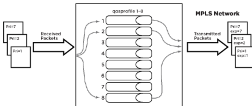
Figure 221: Mapping Dot1p to EXP Bits
