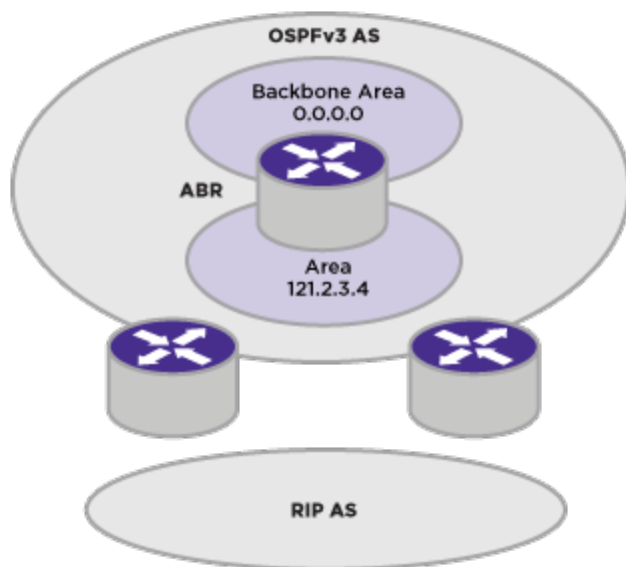
Figure 249: OSPFv3 Route Redistribution
