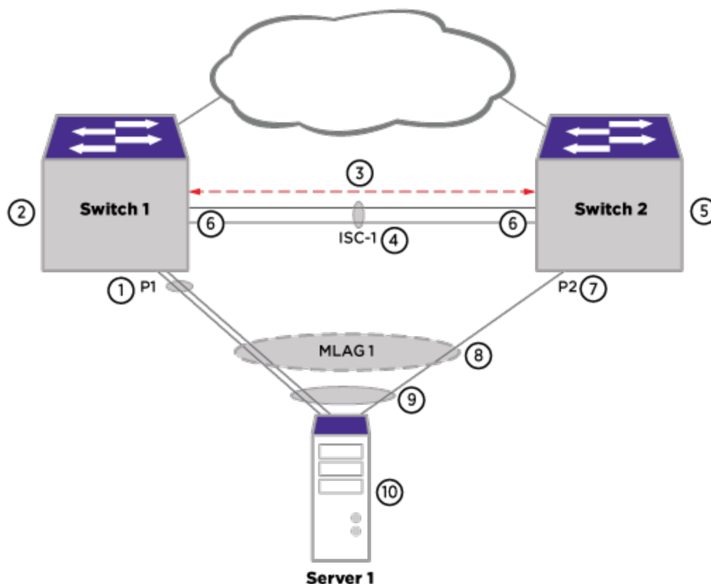
Figure 17: MLAG Elements
