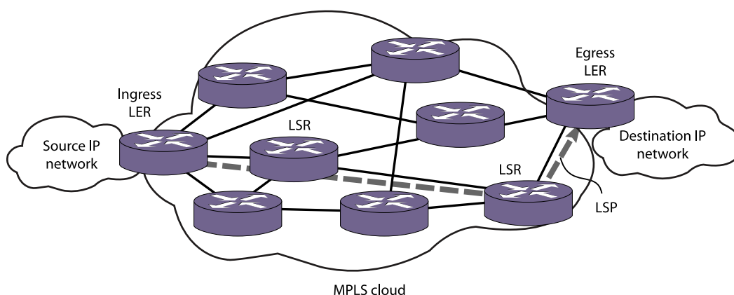
Figure 203: MPLS Network
