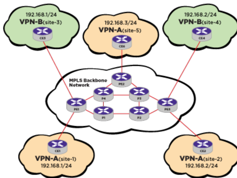
Figure 262: Different Router Roles in L3 VPN
