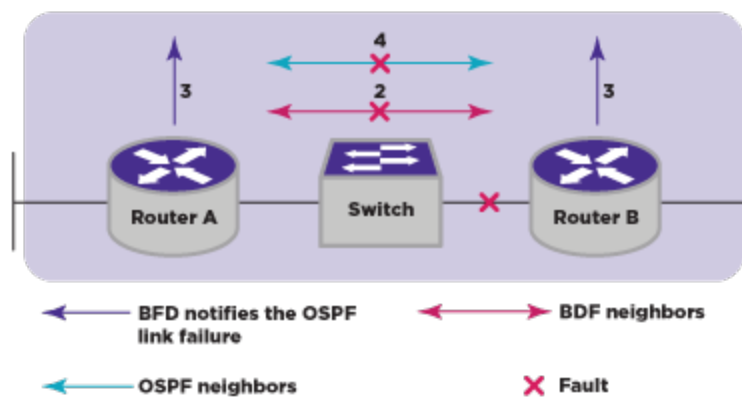
Figure 240: OSPF Neighbor Relationship Eliminated by BFD Fault Detection
