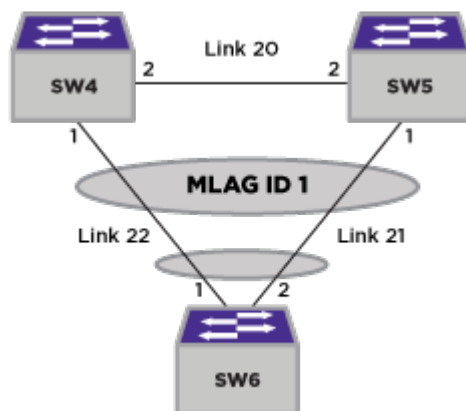
Figure 279: ELRP Egress Port Disable (1)
