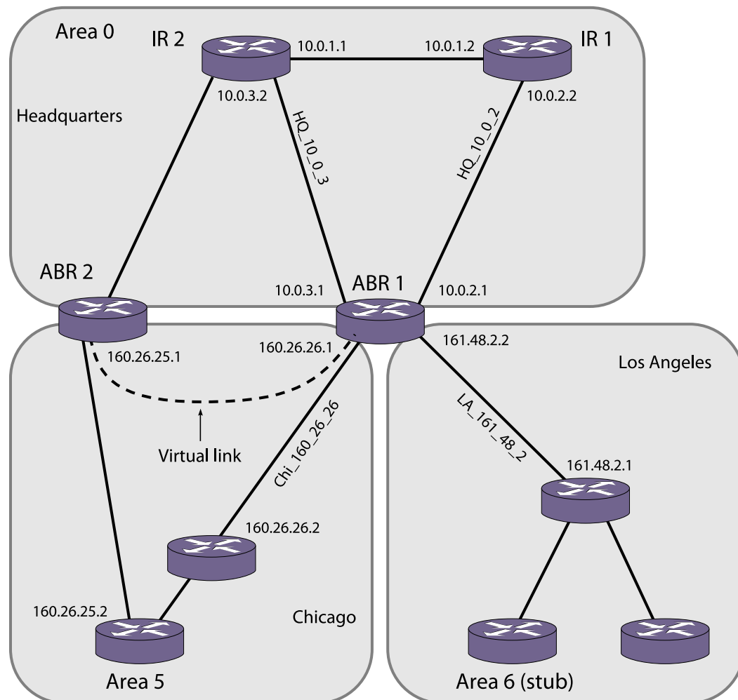
Figure 244: OSPF Configuration Example
