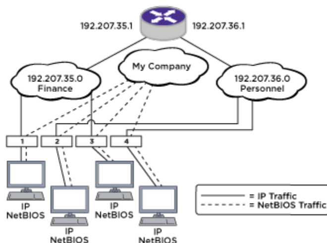
Figure 238: RIP Configuration Example
