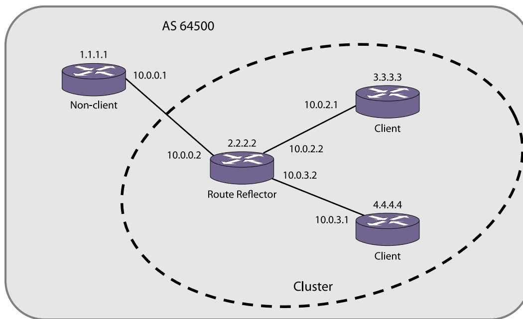
Figure 255: Route Reflectors
