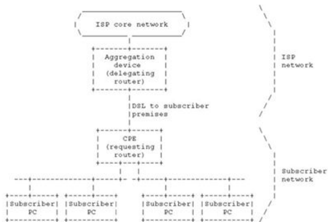
Figure 233: Prefix Delgation Example
