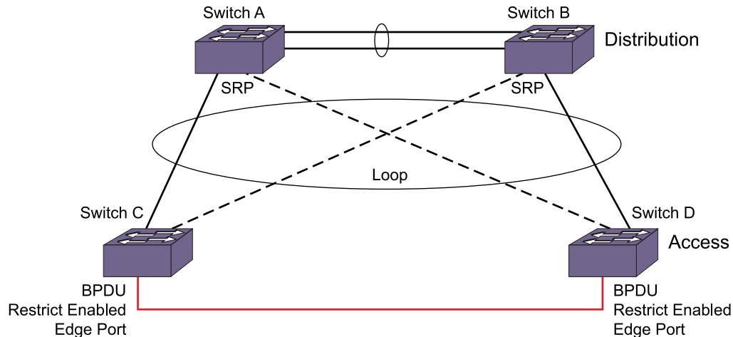
Figure 163: BPDU Restrict
