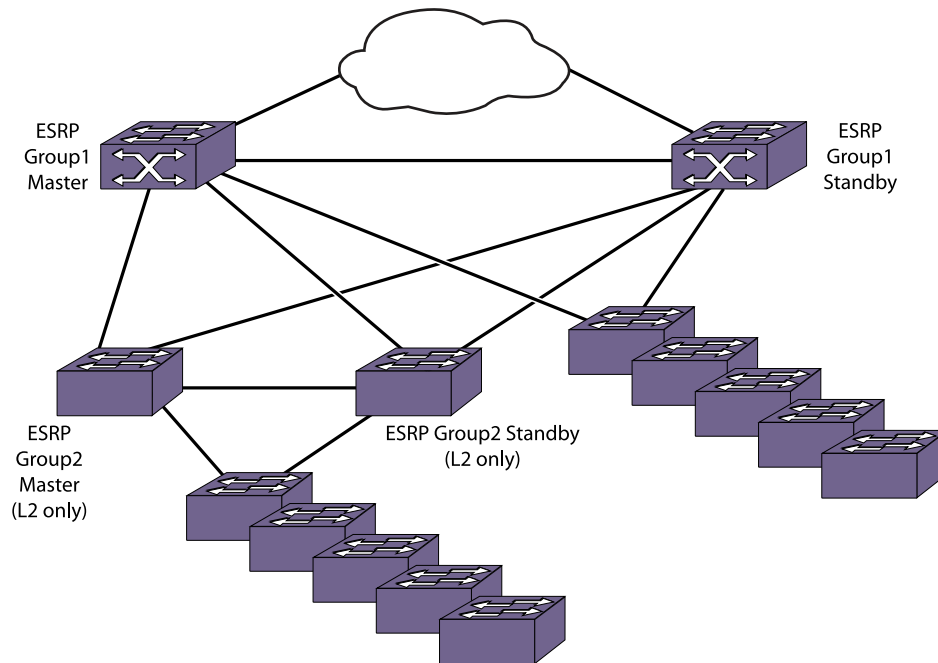
Figure 190: ESRP Groups
