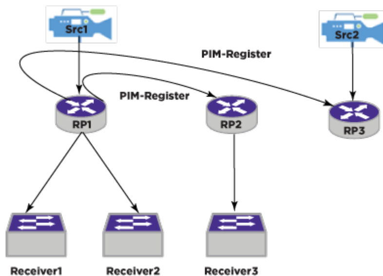
Figure 268: Anycast RP Operation
