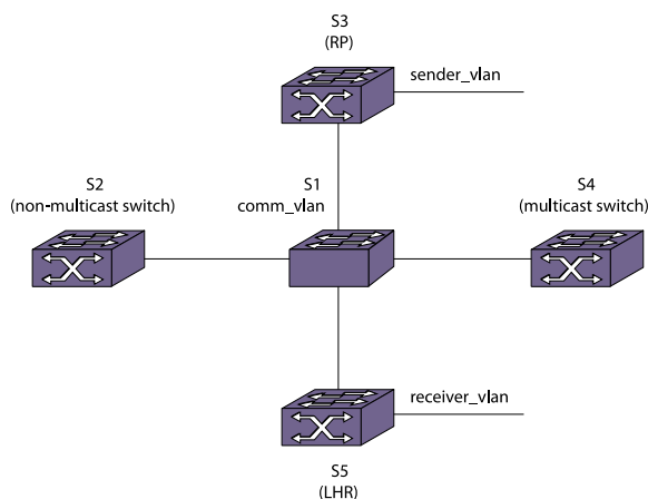
Figure 271: PIM Snooping Configuration Example
