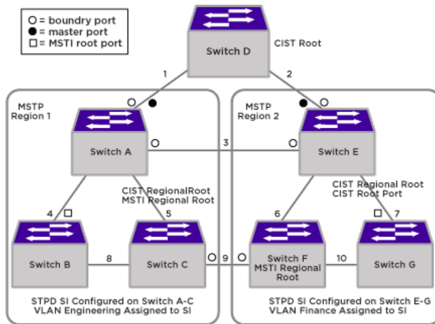
Figure 188: MSTP Configuration Example
