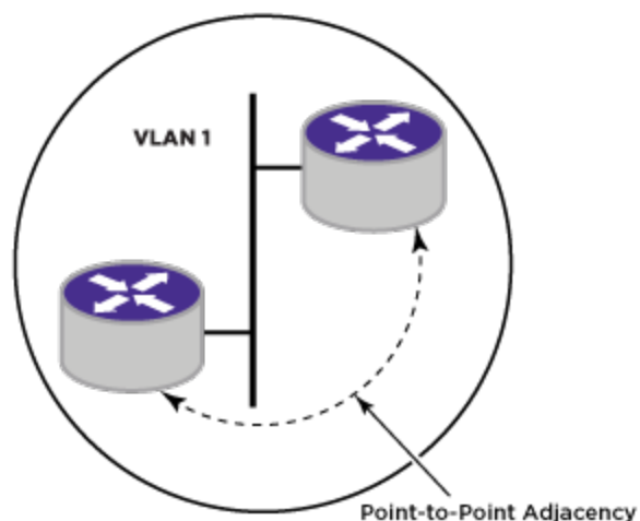
Figure 250: Point-to-Point Adjacency
