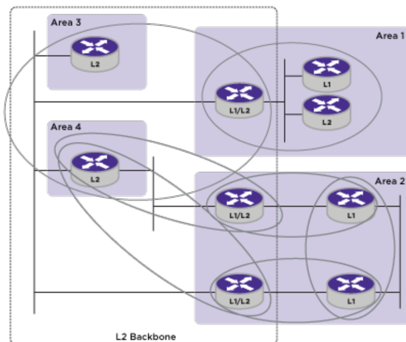
Figure 253: Basic Autonomous System
