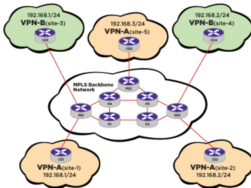
Figure 263: BGP/MPLS VPN Example
