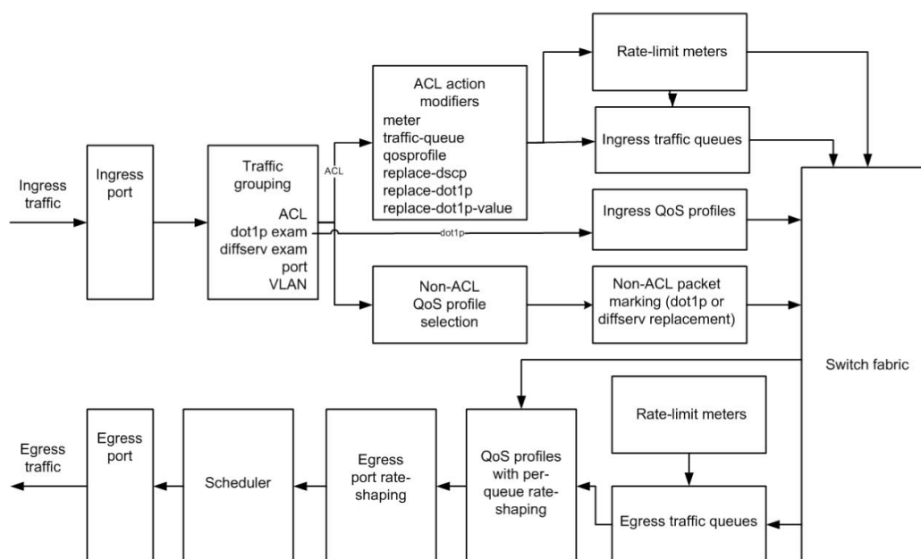
Figure 102: QoS on Extreme Networks Switches
