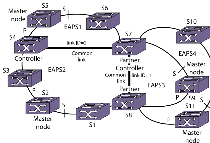
Figure 143: Right-Angle Topology
