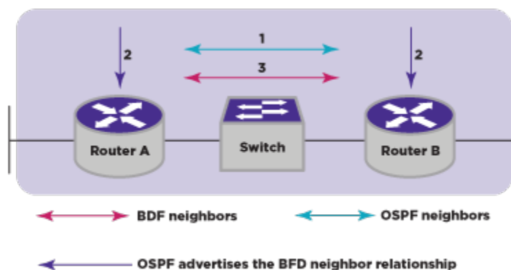
Figure 239: Basic Operational Flow of OSPF BFD
