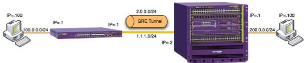
Figure 227: GRE Tunnel Configuration
