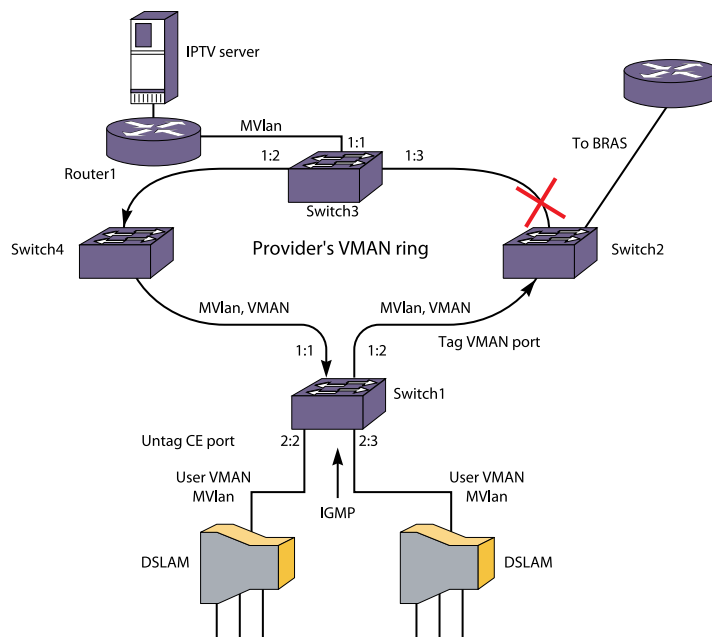
Figure 278: MVR in a VMAN Environment
