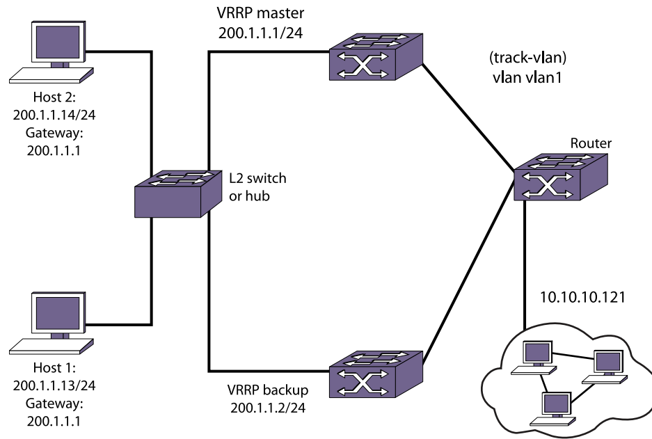
Figure 202: VRRP Tracking
