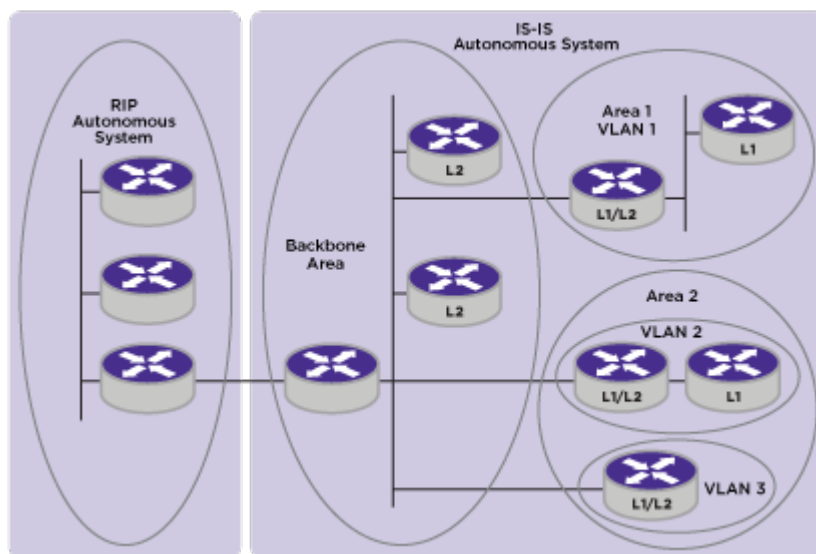
Figure 254: AS External Route Redistribution
