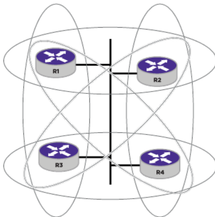
Figure 251: Point-to-Point Adjacencies in a Four-Router Network
