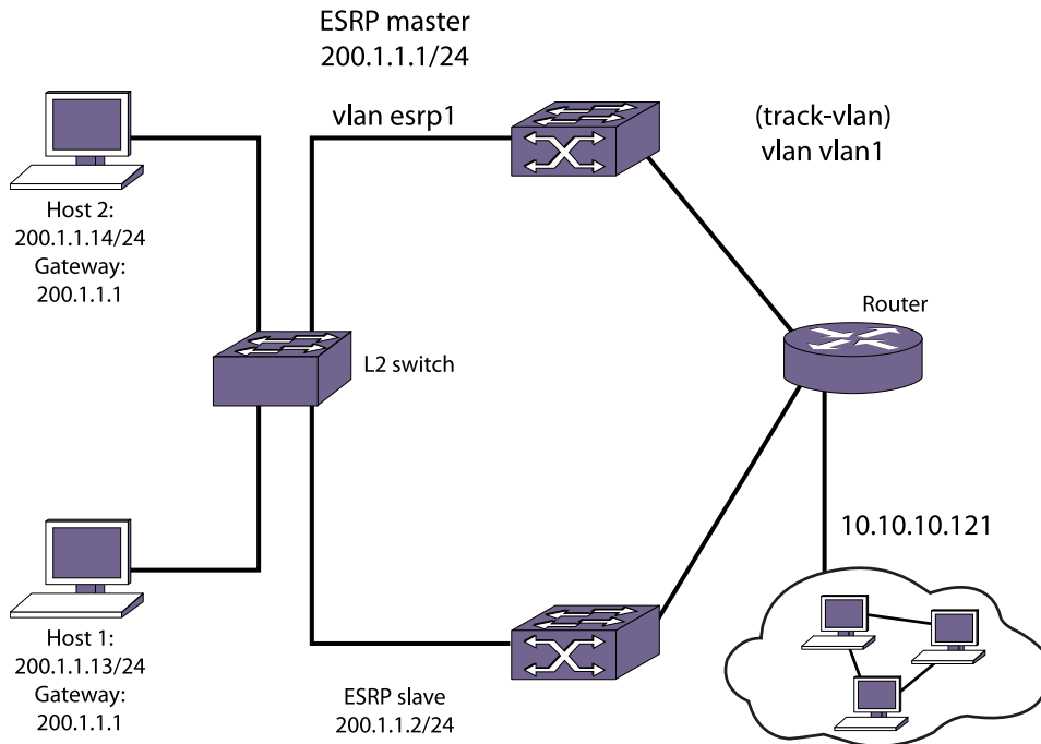
Figure 191: ESRP Tracking
