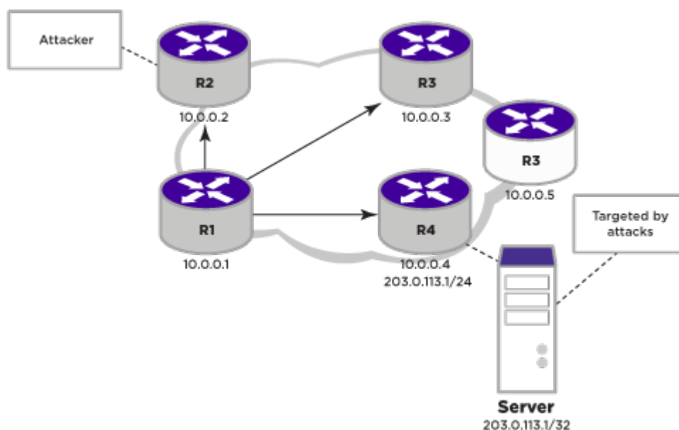
Figure 259: Black Hole Routing Using BGP
