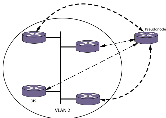
Figure 252: Broadcast Adjacencies in a Four-Router Network
