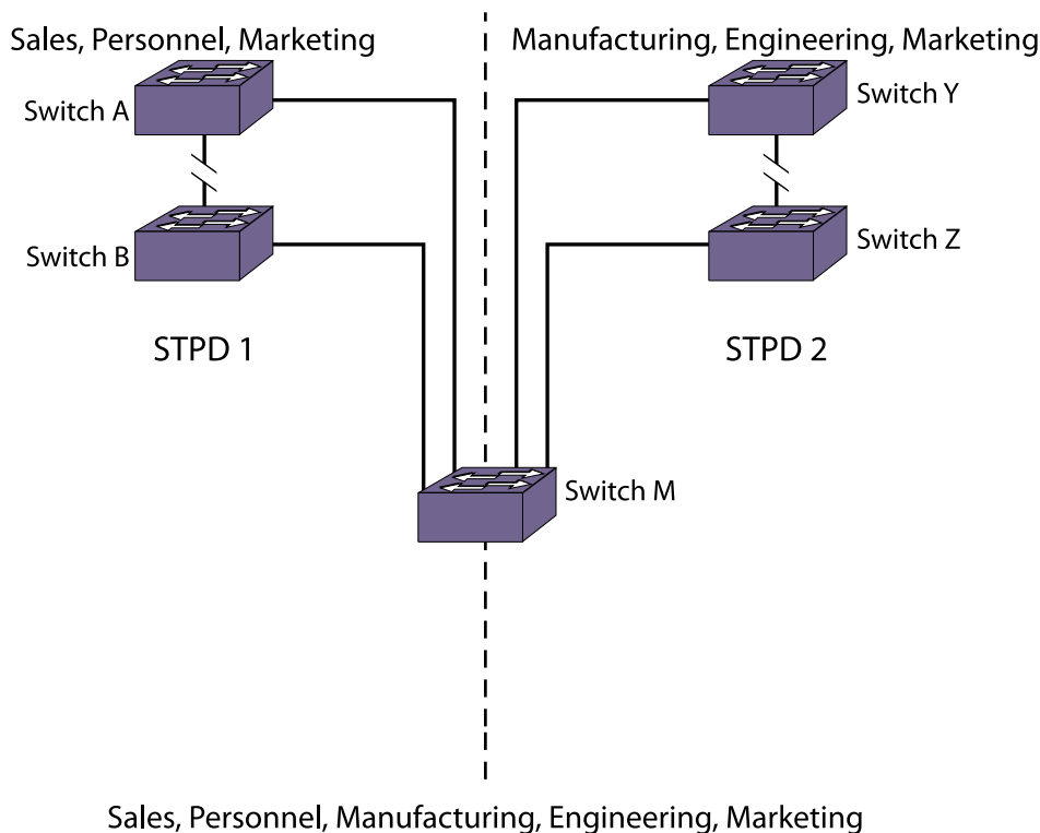
Figure 187: RSTP Example
