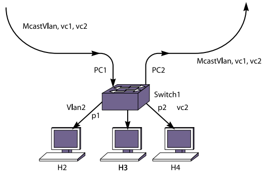
Figure 274: Multiple VLANs in the Core Network
