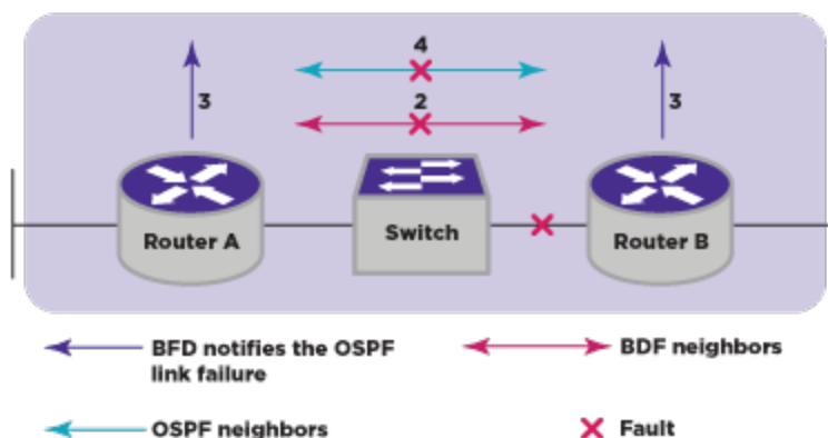
Figure 246: OSPFv3 Neighbor Relationship Eliminated by BFD Fault Detection
