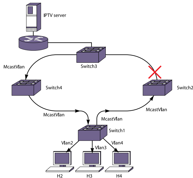
Figure 273: Basic MVR Deployment
