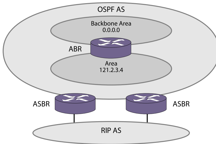
Figure 243: OSPF Route Redistribution
