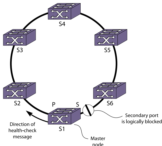
Figure 133: EAPS Operation
