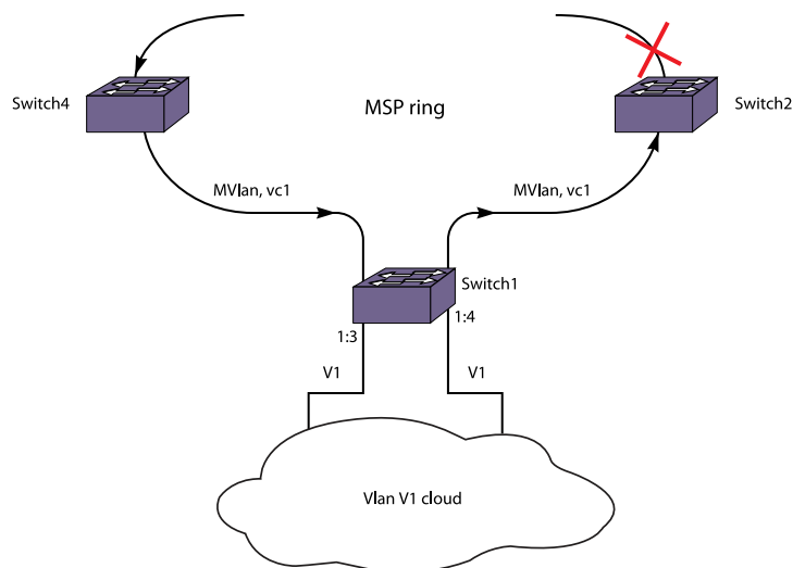
Figure 277: MVR with STP
