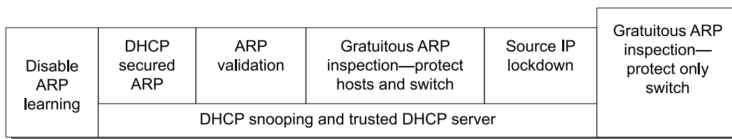
Figure 126: IP Security Dependencies
