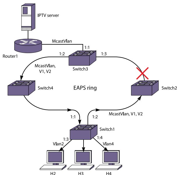
Figure 276: MVR on an EAPS Ring
