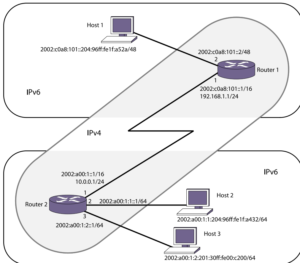
Figure 236: 6to4 Tunnel Configuration Example
