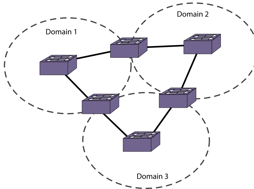
Figure 169: Looped VLAN Topology
