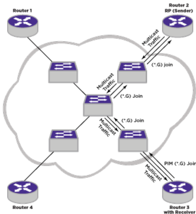
Figure 267: Multicast With PIM Snooping
