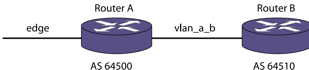
Figure 260: BGP IPv4 Route Filtering Example
