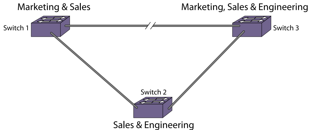
Figure 165: Incorrect Tag-Based STPD Configuration
