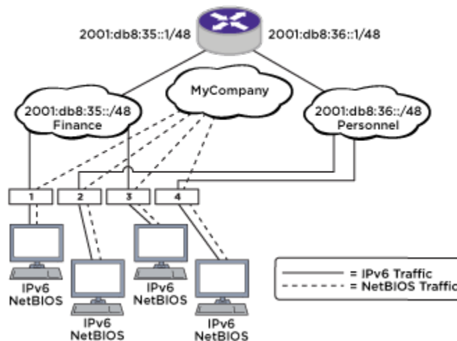
Figure 234: IPv6 Unicast Routing Configuration Example
