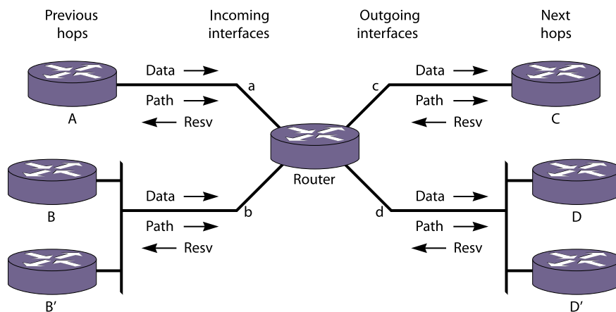
Figure 218: RSVP Messages
