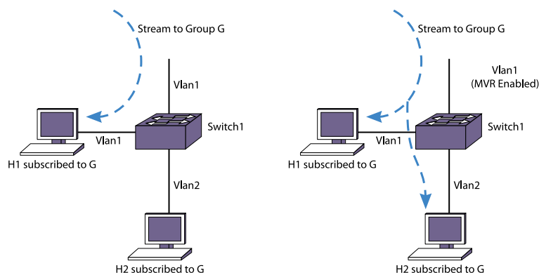
Figure 272: Standard VLAN Compared to an MVR VLAN
