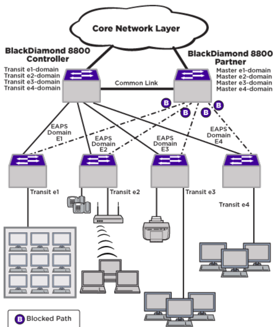
Figure 150: L2 Aggregation Network Layer
