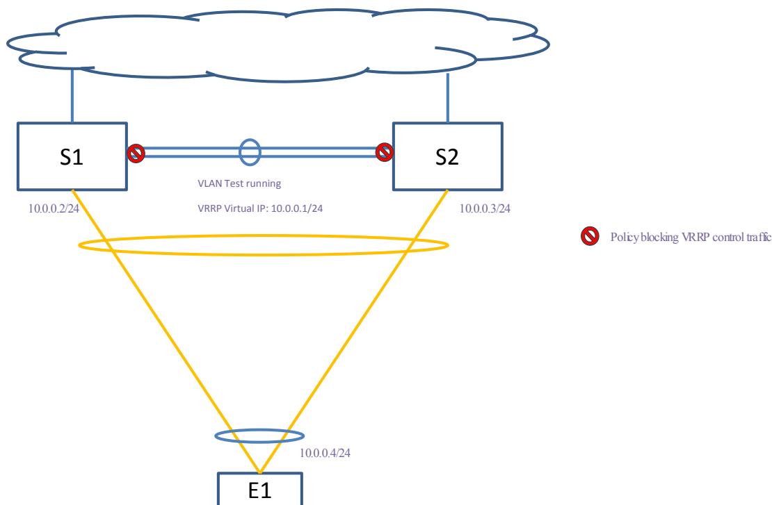
Figure 197: VRRP Active-Active
