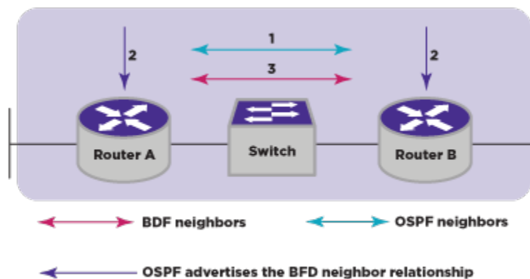
Figure 245: Basic Operational Flow of OSPFv3 BFD
