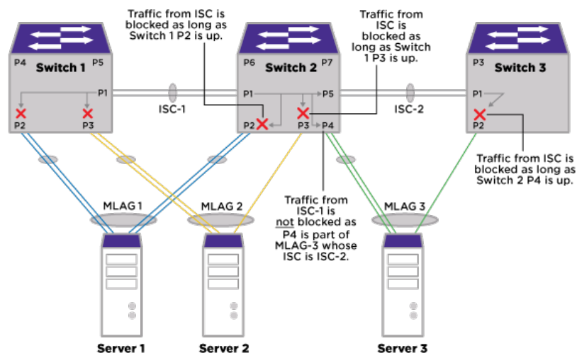
Figure 20: Traffic Flow
