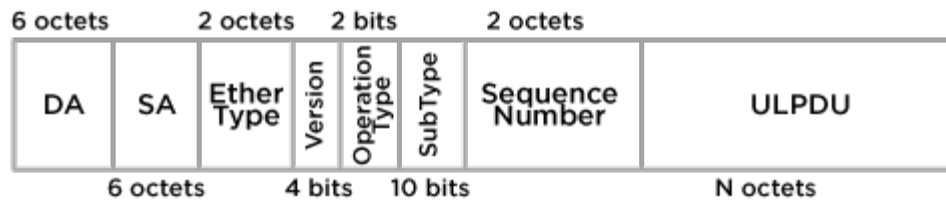
Figure 36: ECPDU Structure
