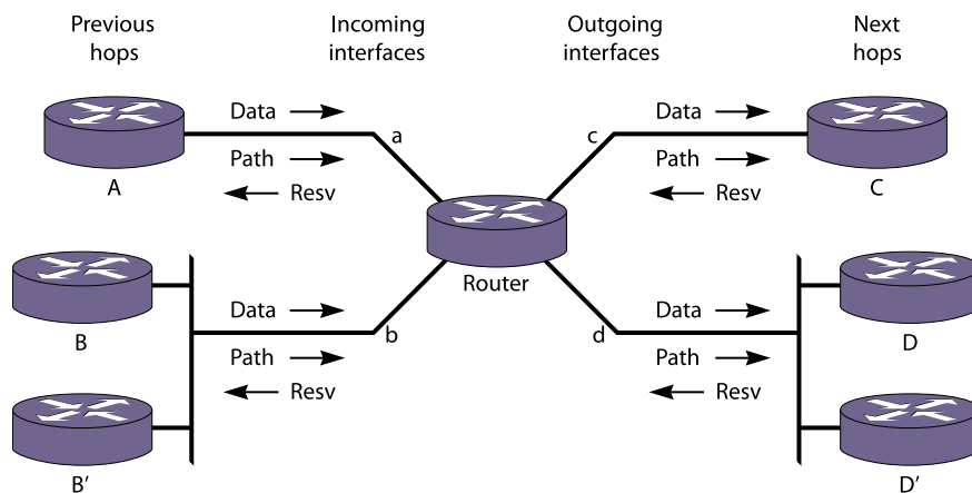
Figure 222: RSVP Messages
