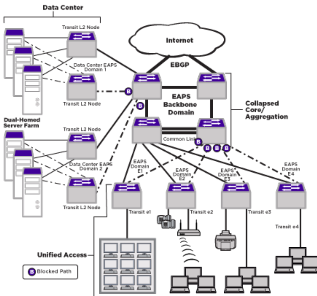
Figure 152: Extreme Networks EAPS Everywhere
