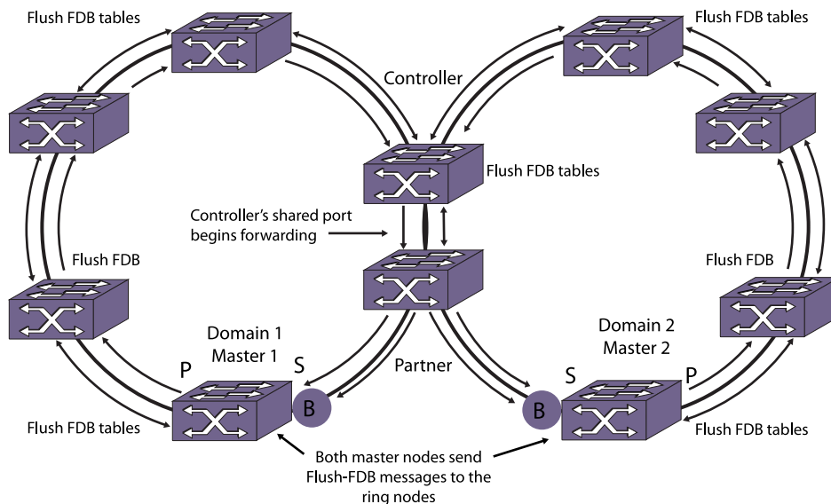
Figure 144: Common-Link Restored
