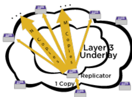
Figure 117: Example Assisted Replication Topology
