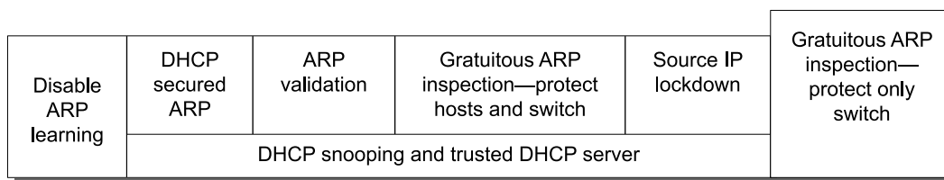
Figure 129: IP Security Dependencies
