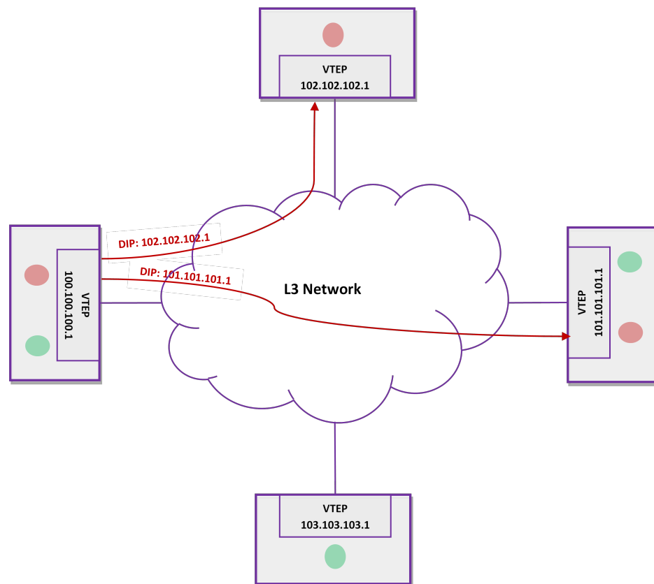
Figure 114: Head-end Replication
