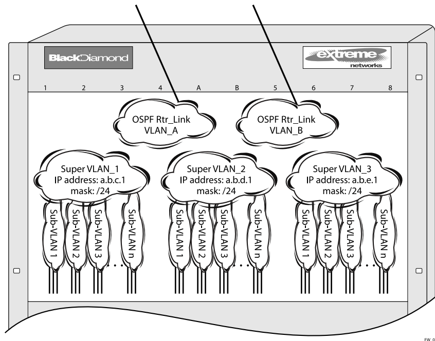
Figure 235: VLAN Aggregation
