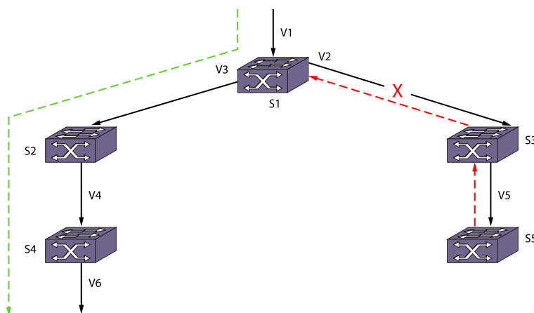
Figure 273: PIM-DM Operation
