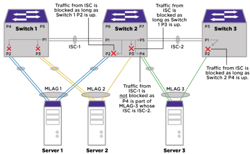
Figure 20: Traffic Flow
