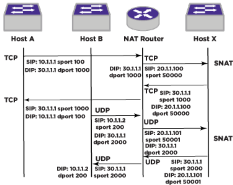
Figure 238: NAPT Example
