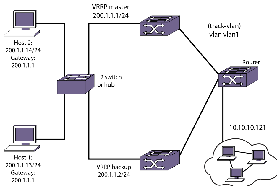
Figure 206: VRRP Tracking
