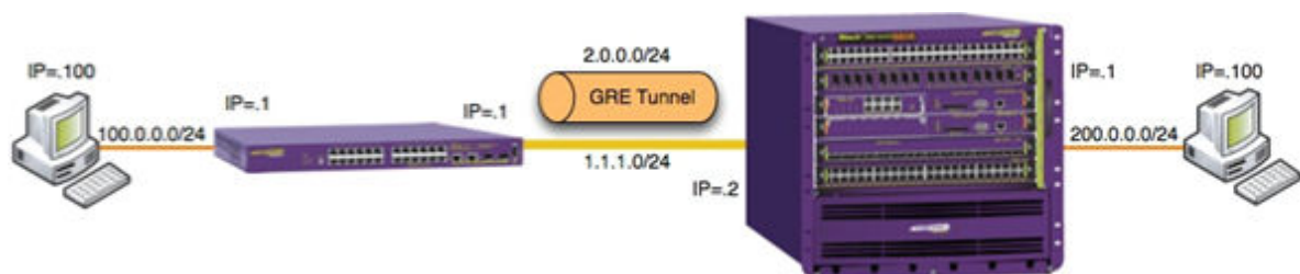
Figure 231: GRE Tunnel Configuration
