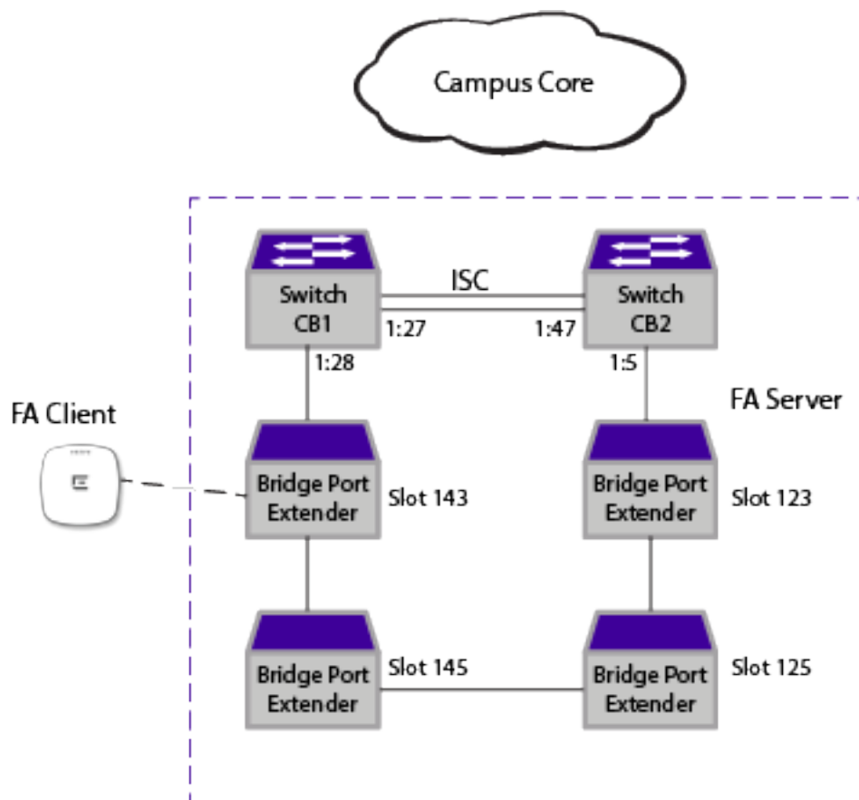
Figure 96: FA Clients Connect to BPE with Ring MLAG-Connected FA Server Peers
