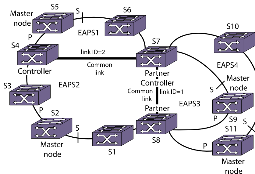
Figure 147: Right-Angle Topology
