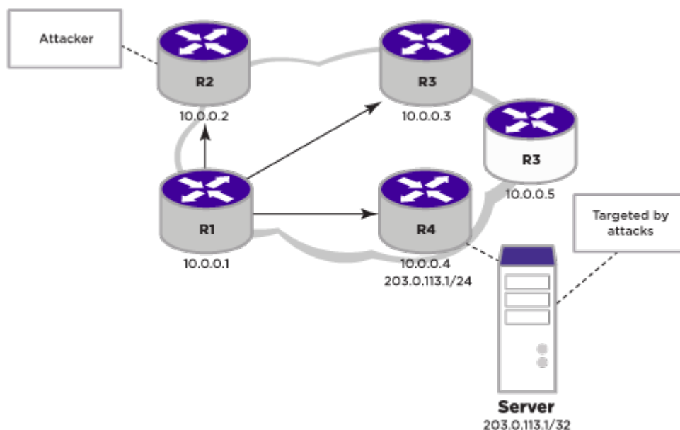
Figure 267: Black Hole Routing Using BGP
