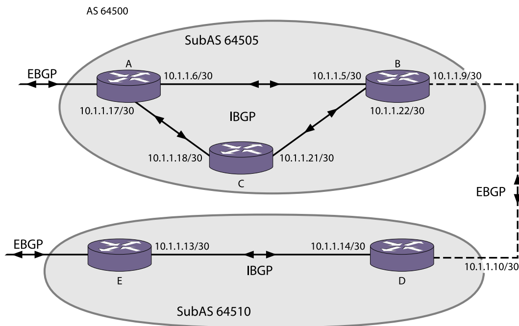
Figure 264: Routing Confederation
