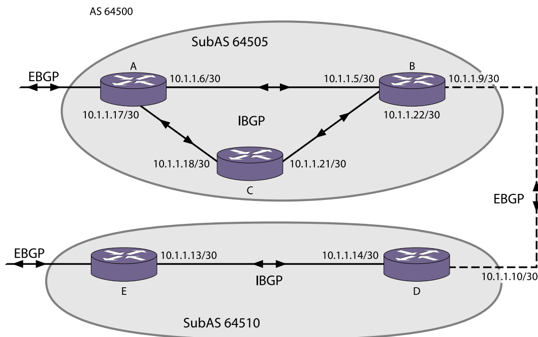
Figure 264: Routing Confederation
