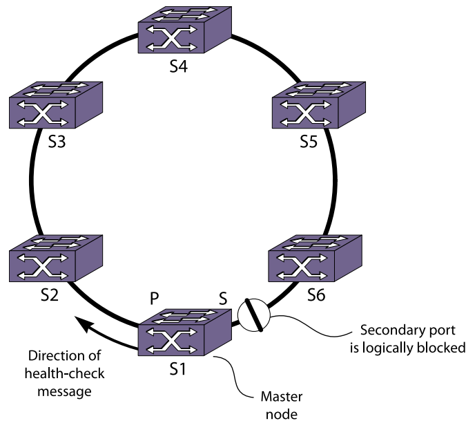
Figure 137: EAPS Operation
