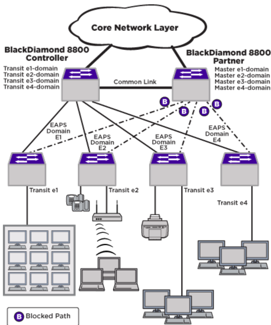
Figure 154: L2 Aggregation Network Layer
