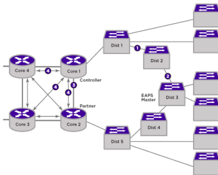
Figure 220: VPLS with Redundant EAPS Configuration Example
