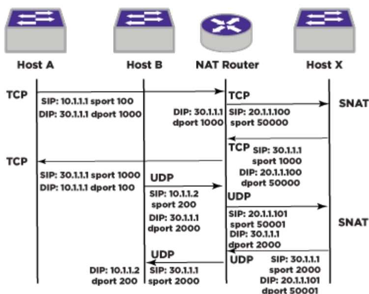
Figure 238: NATP Example
