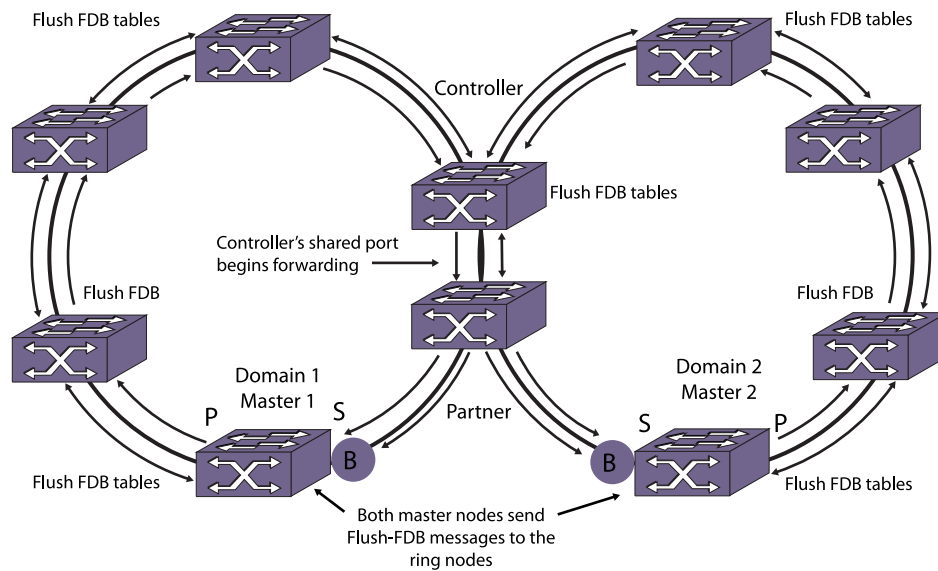
Figure 144: Common-Link Restored
