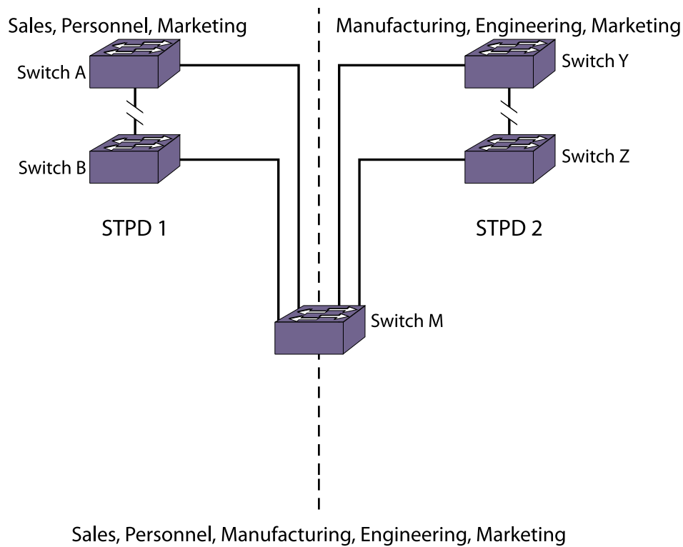
Figure 168: Multiple STPDs
