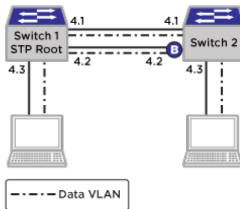
Figure 151: Sample STP Network for Migration to EAPS
