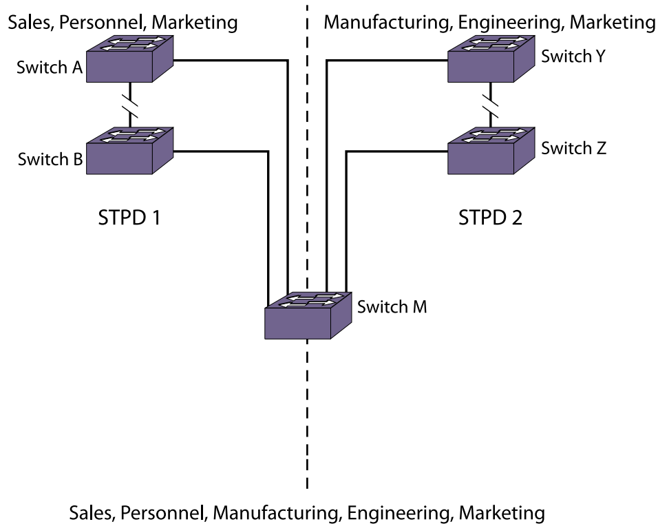
Figure 191: RSTP Example
