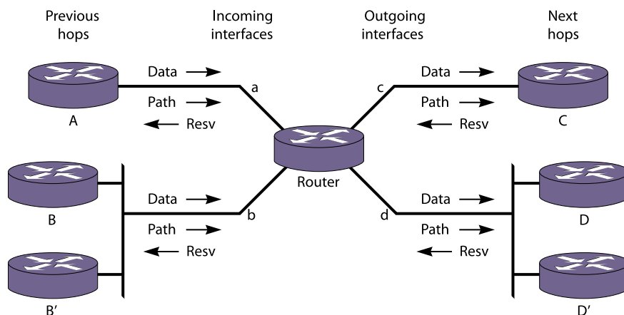
Figure 221: RSVP Messages
