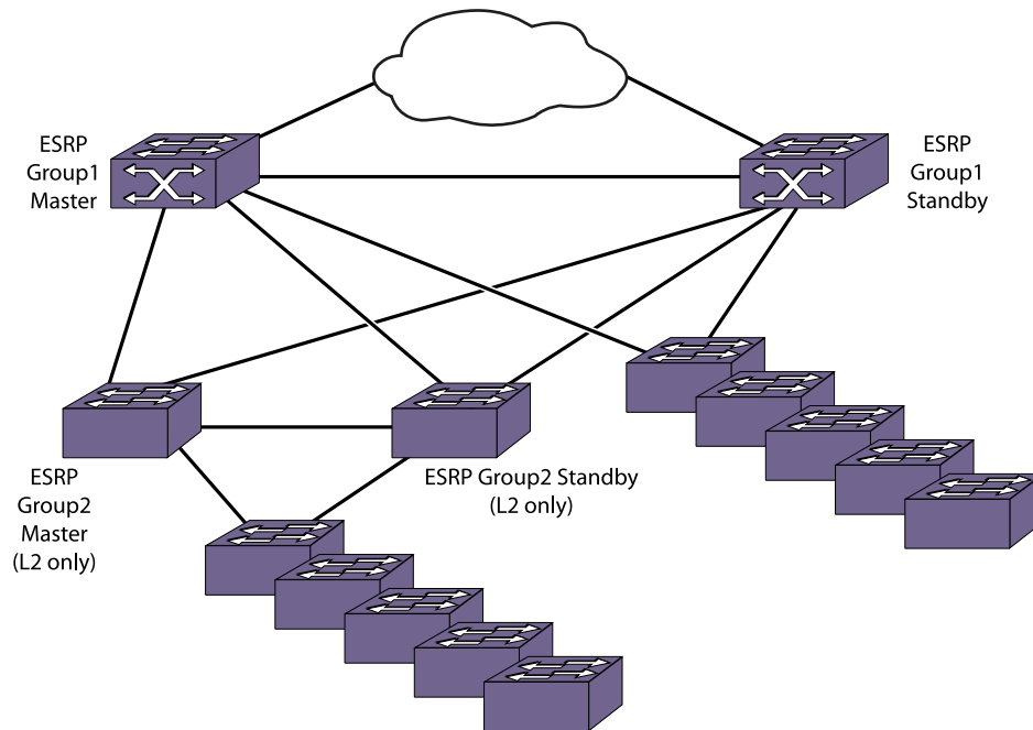
Figure 193: ESRP Groups
