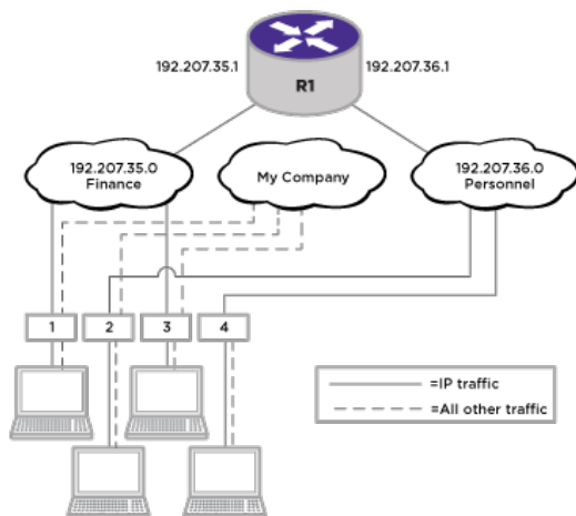
Figure 70: Protocol-Based VLANs
