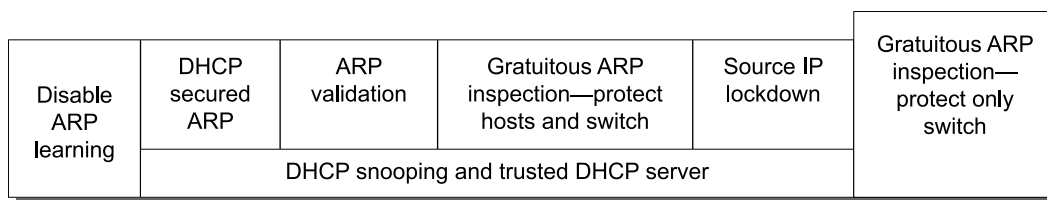
Figure 128: IP Security Dependencies
