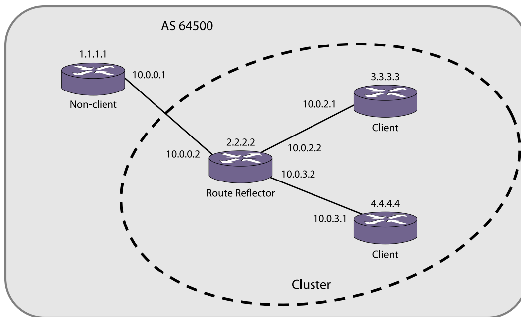
Figure 262: Route Reflectors
