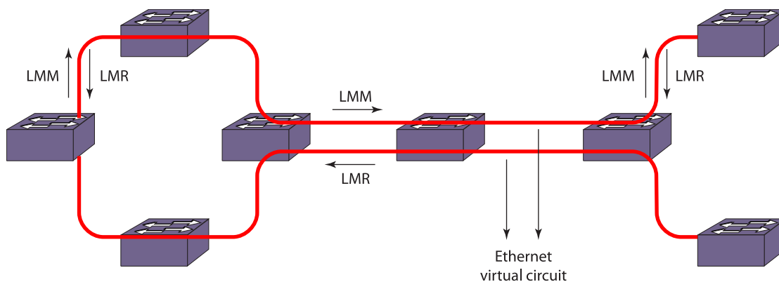
Figure 57: Two-Way Frame-Loss Measurement
