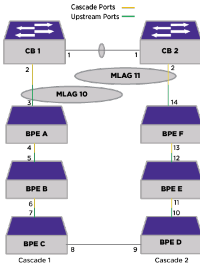
Figure 41: One-Arm MLAG
