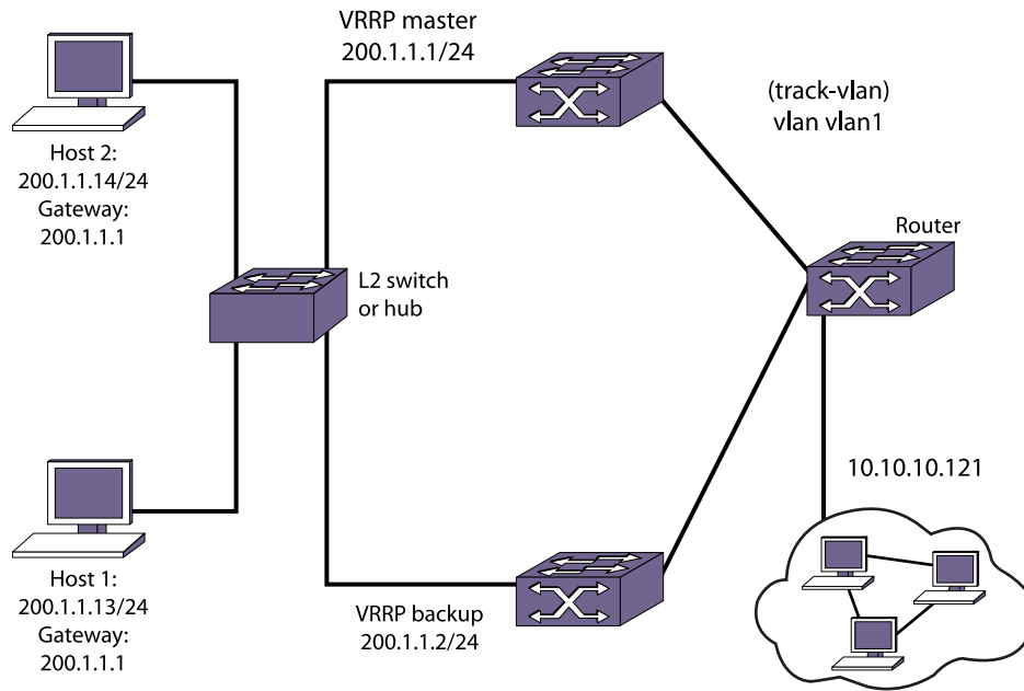
Figure 205: VRRP Tracking
