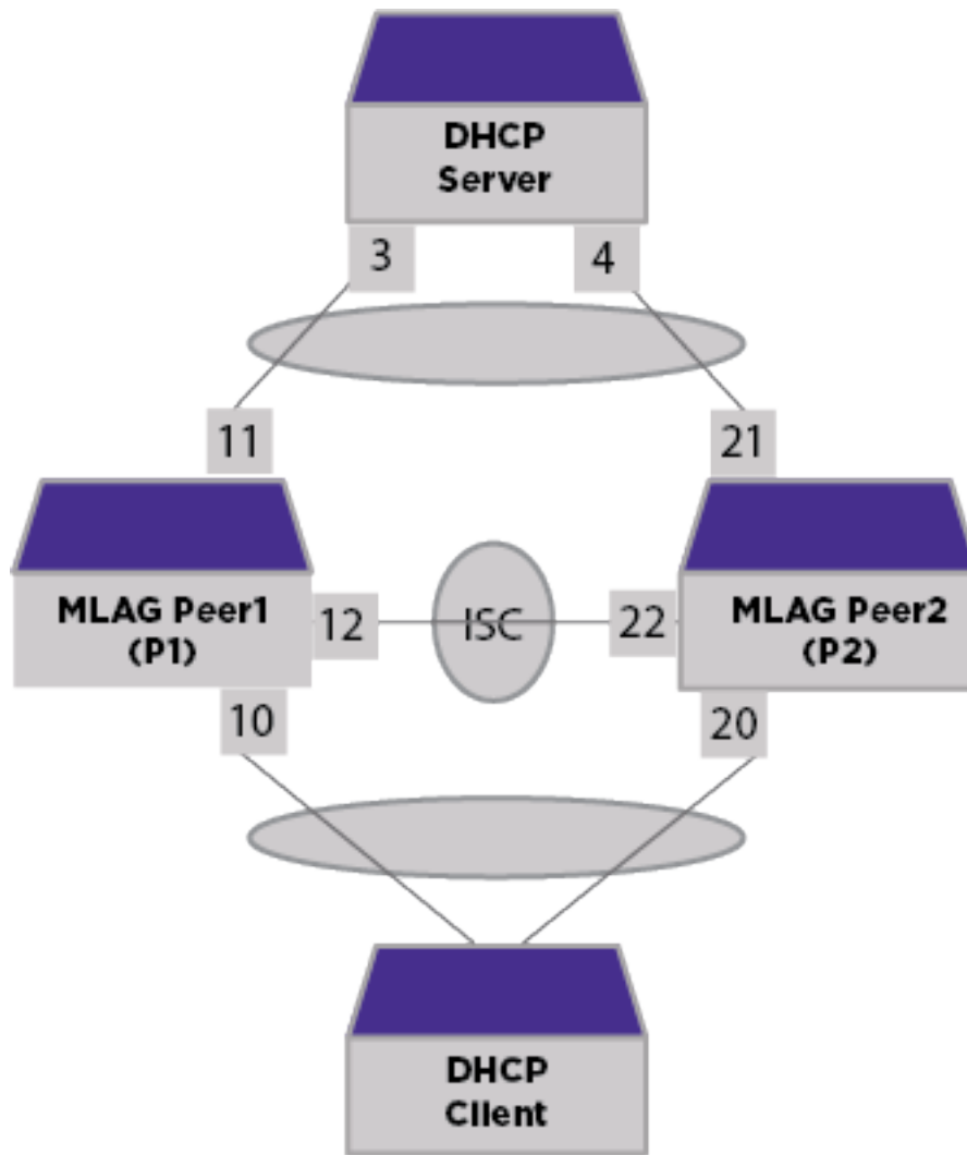
Figure 129: MLAG Topology
