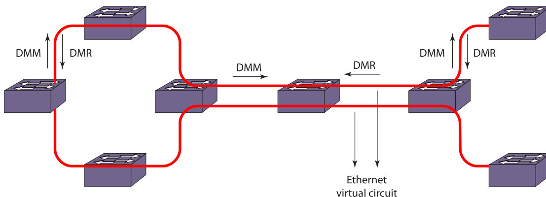
Figure 55: Two-Way Frame Delay and Frame Delay Variance Measurement
