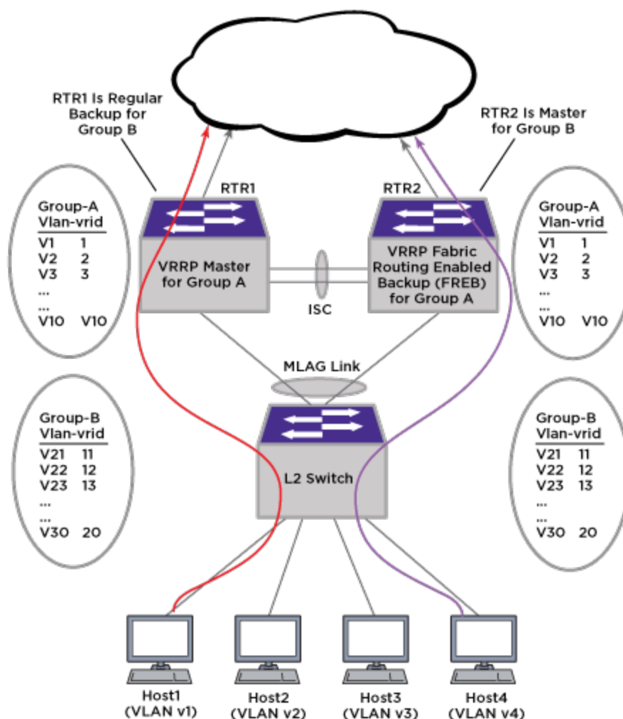
Figure 204: Example VRRP Group Configuration
