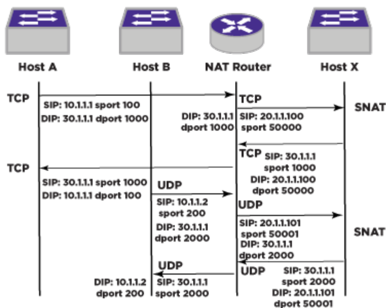
Figure 237: NATP Example
