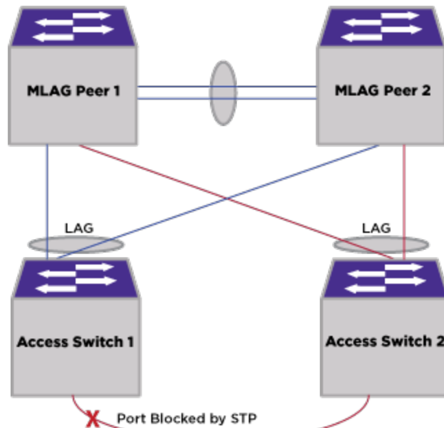
Figure 188: MLAG and MSTP/RSTP
