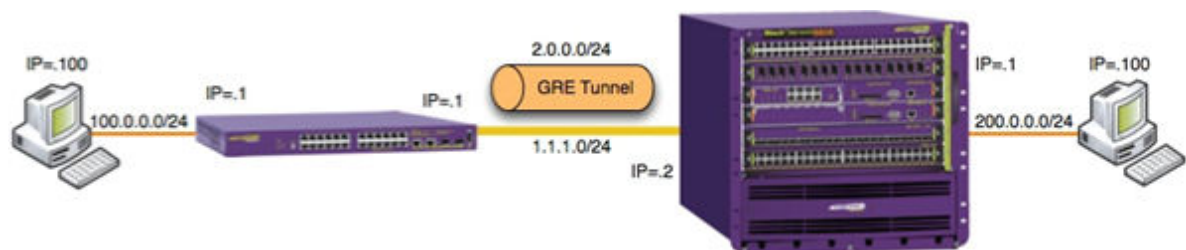
Figure 230: GRE Tunnel Configuration
