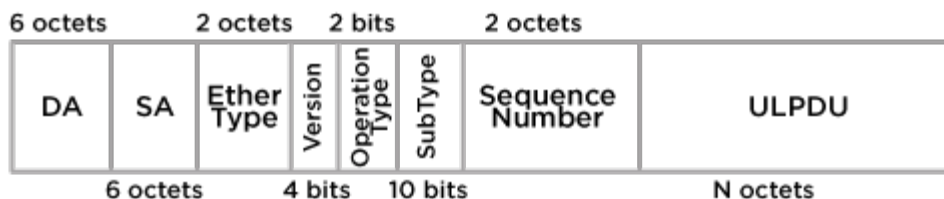
Figure 35: ECPDU Structure
