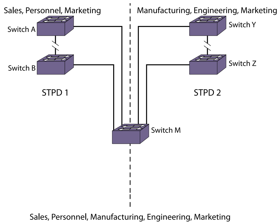
Figure 167: Multiple STPDs
