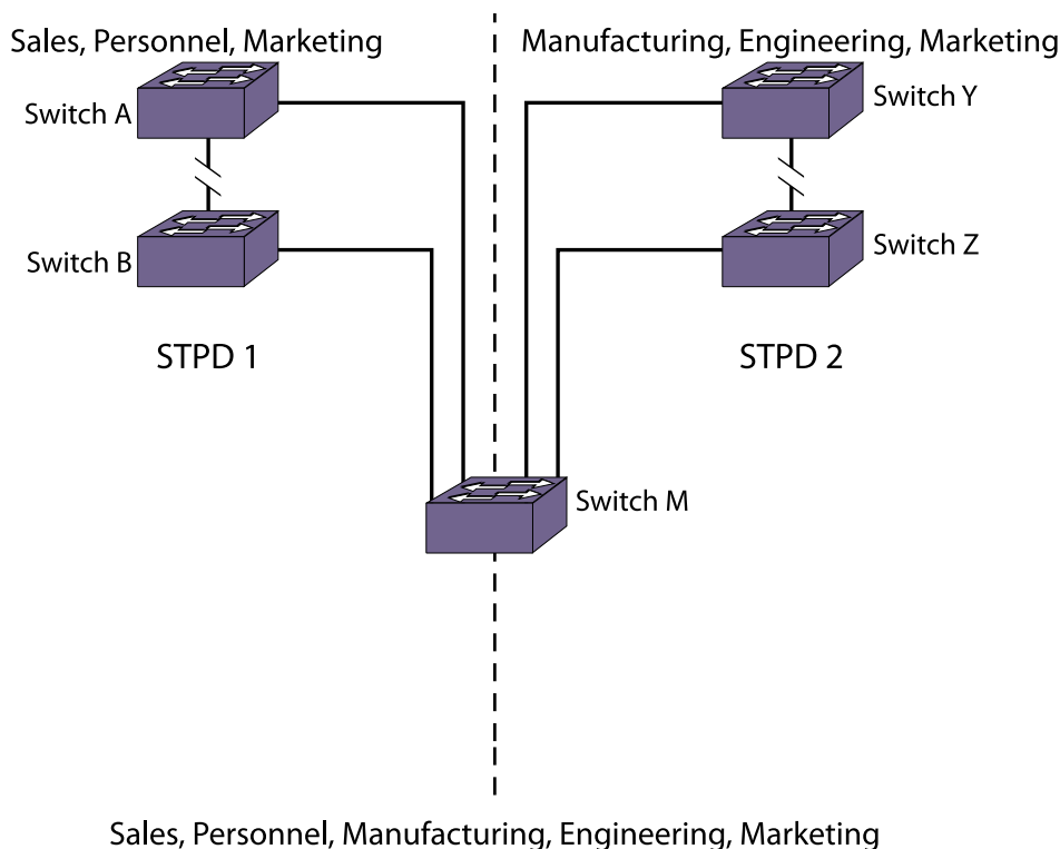
Figure 190: RSTP Example
