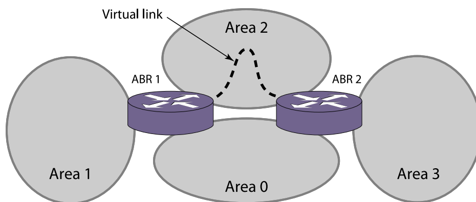
Figure 255: Virtual Link Providing Redundancy
