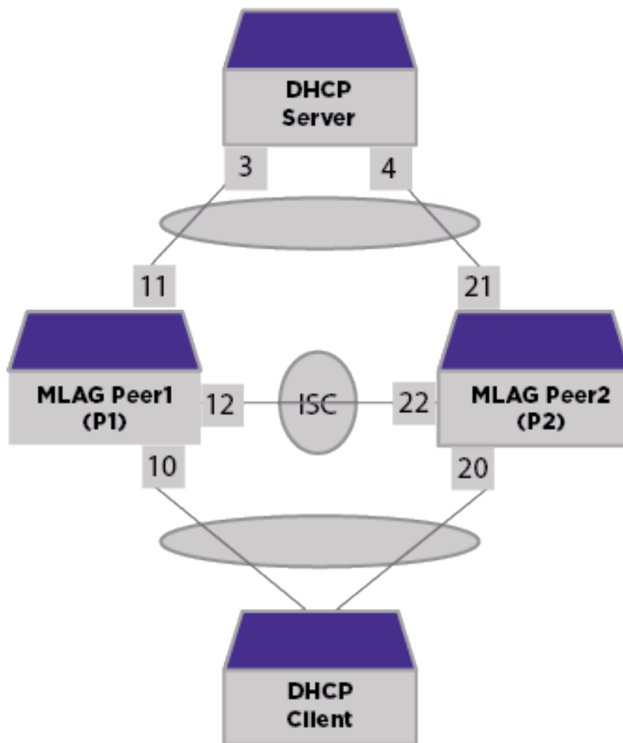
Figure 127: MLAG Topology
