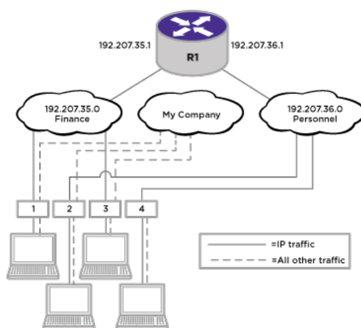
Figure 68: Protocol-Based VLANs
