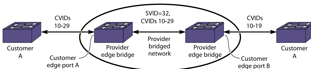
Figure 84: CVID Egress Filtering
