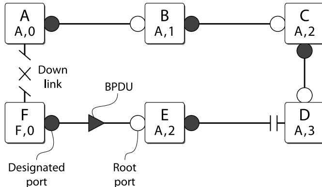
Figure 173: Down Link Detected
