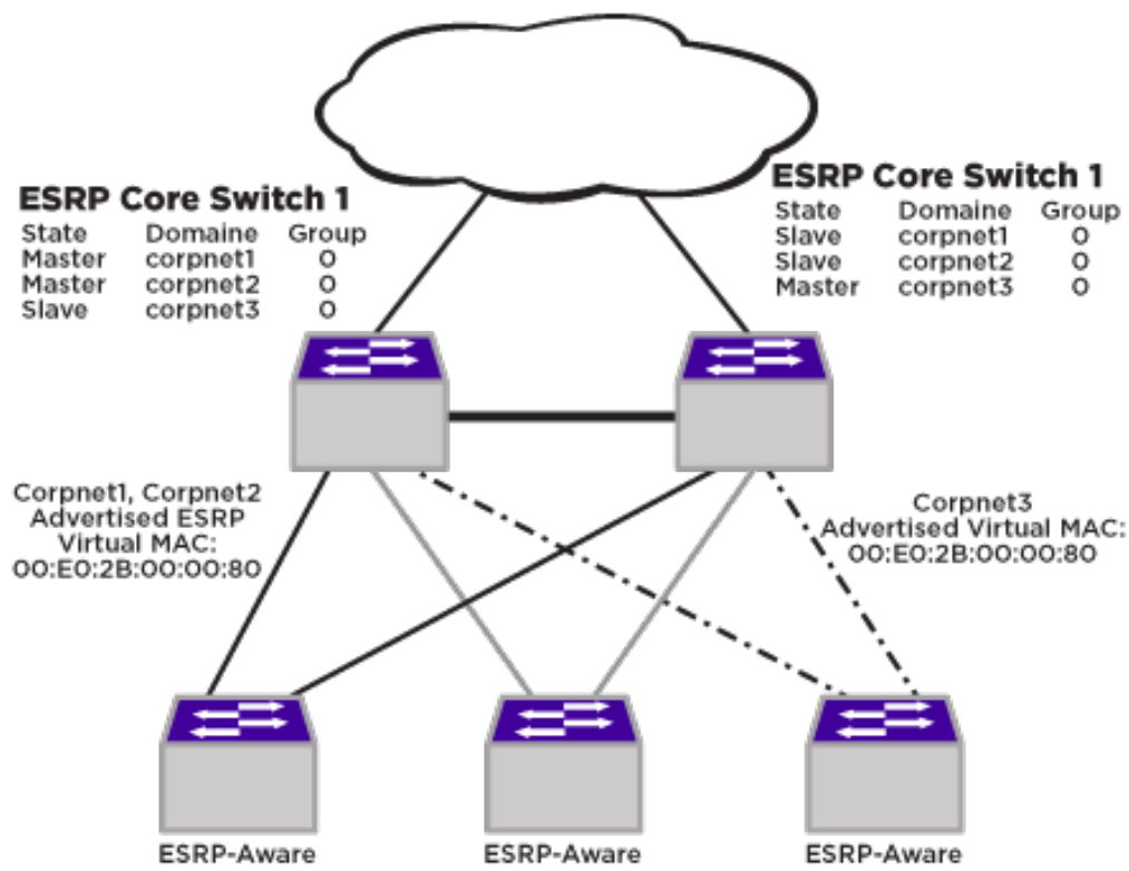
Figure 190: Example of a Basic ESRP Topology
