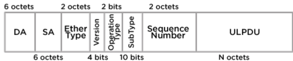
Figure 33: ECPDU Structure
