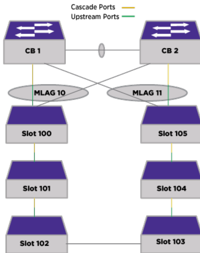
Figure 38: Cross-Connect MLAG
