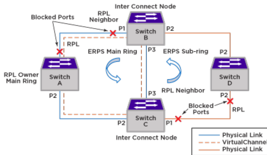
Figure 157: Sample ERPS Configuration
