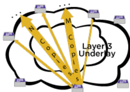
Figure 113: Example Head-End Replication Topology
