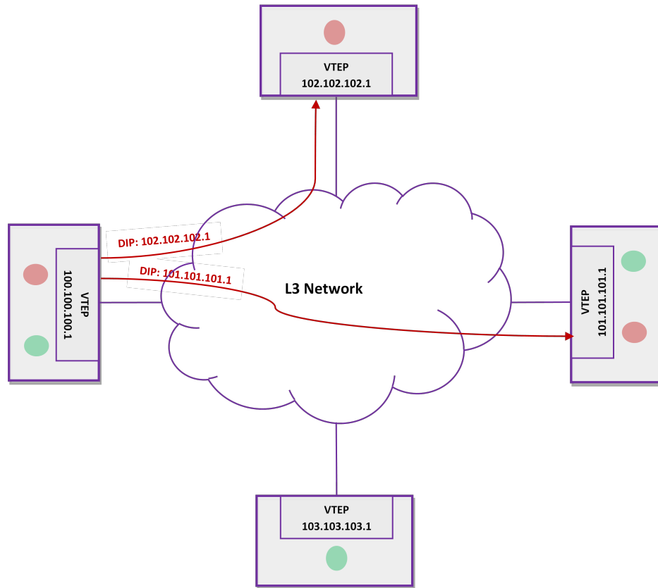
Figure 111: Head-end Replication
