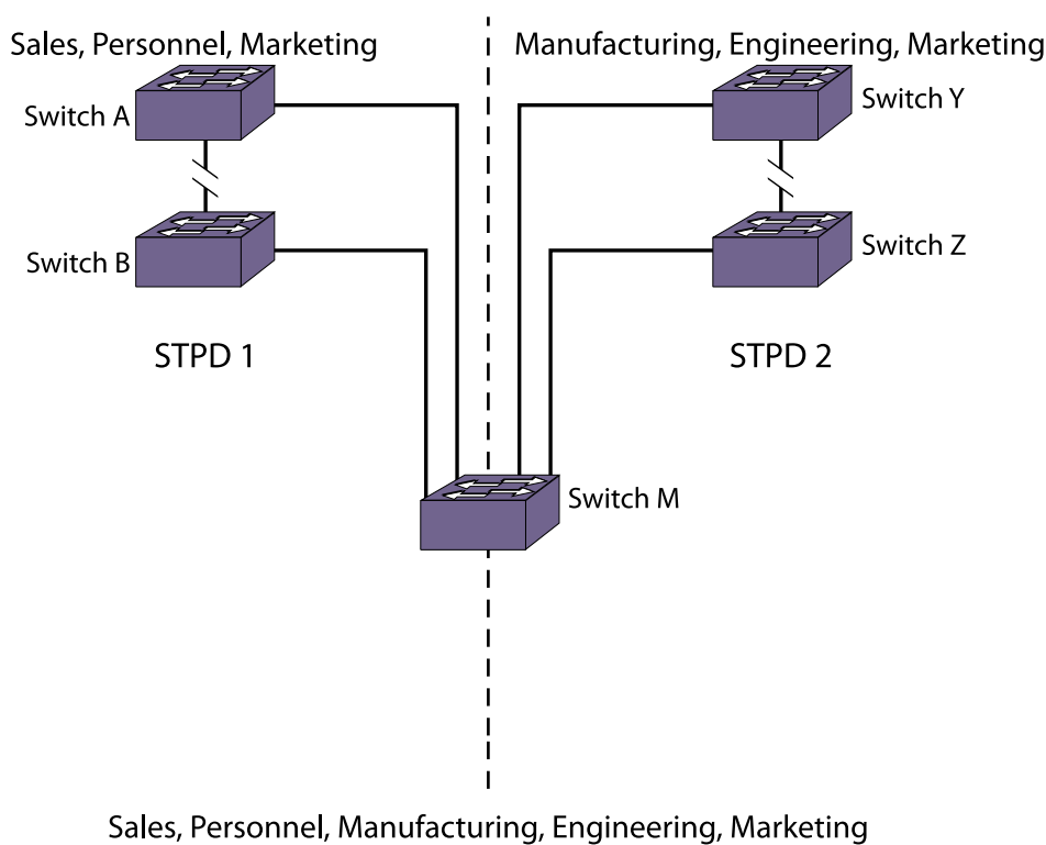
Figure 188: RSTP Example
