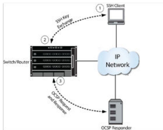
Figure 132: Public-Key Infrastructure Login Flow Overview
