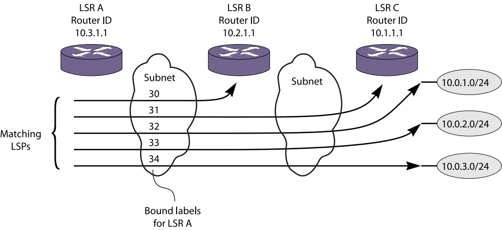
Figure 210: Matching and Calculated LSP Next Hops
