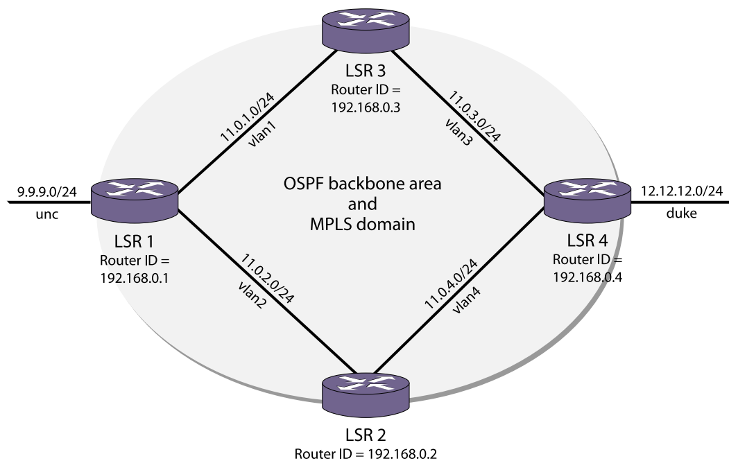
Figure 223: MPLS Configuration Example
