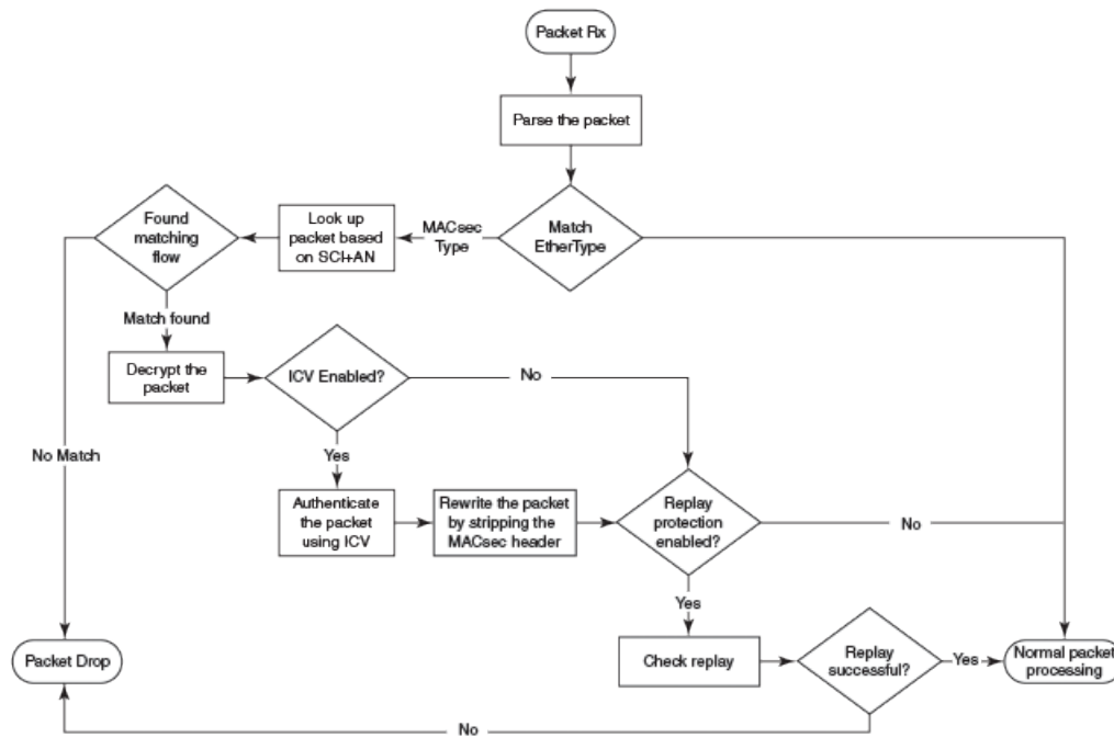
FIGURE 13 MACsec incoming frames
