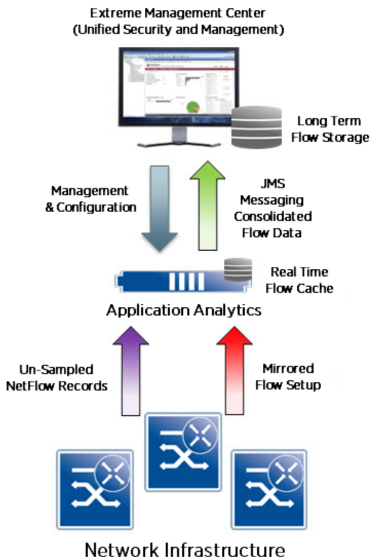
ExtremeAnalytics Deployment
