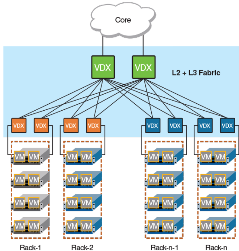
FIGURE 10 VDX 6740 and VDX 6940-based fabric
