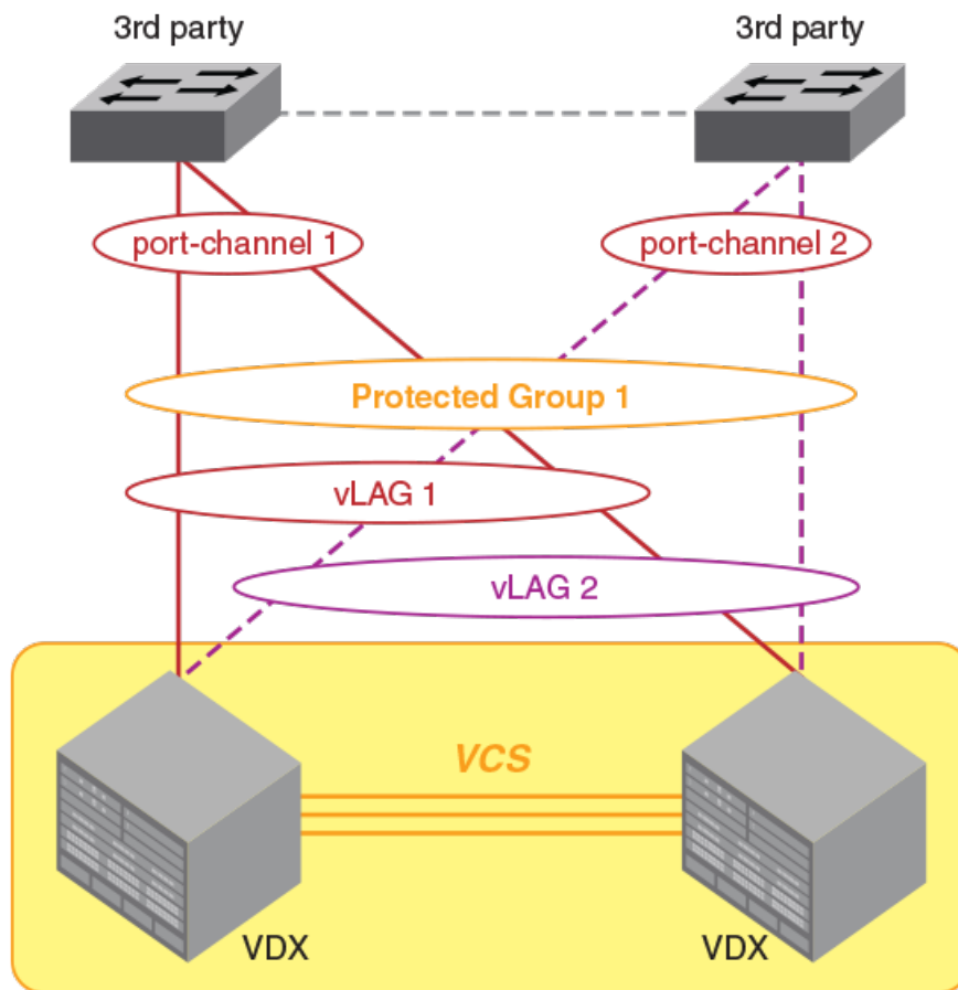
FIGURE 15 Port-channel redundancy group configuration
