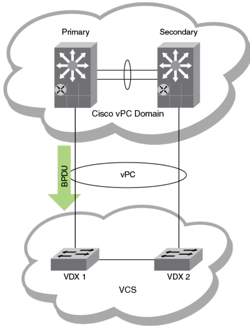
FIGURE 11 STP BPDUs processing without Peer-Switch
