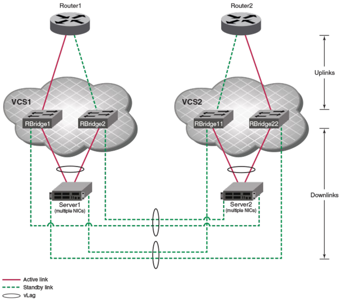
FIGURE 21 Redundant-link topology for VCS fabrics
