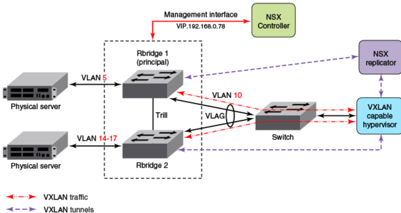
FIGURE 5 High-level communication for VXLAN overlay gateway with NSX Controller
