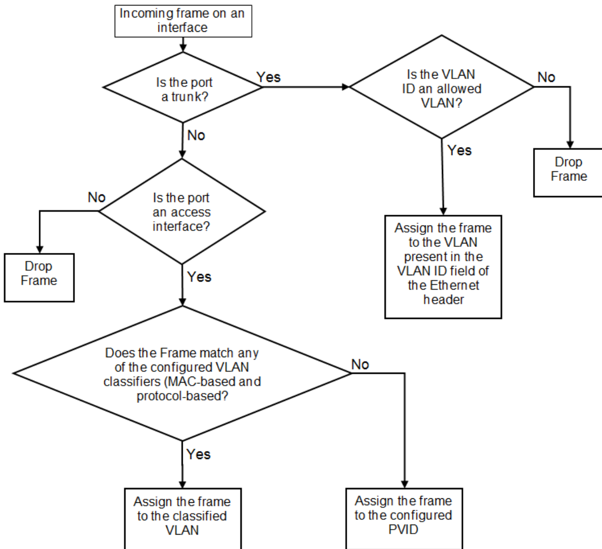
FIGURE 1 Ingress VLAN filtering
