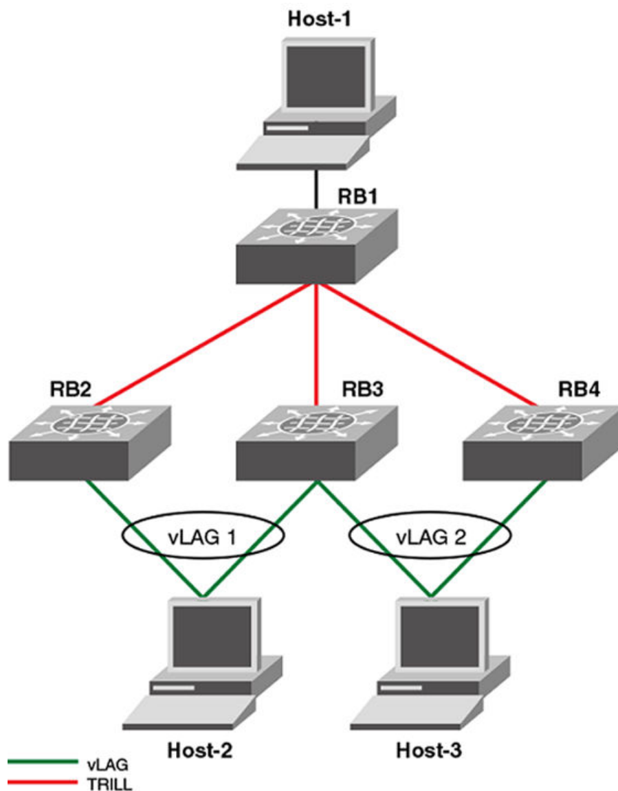
FIGURE 14 vLAG configuration of the ignore-split feature
