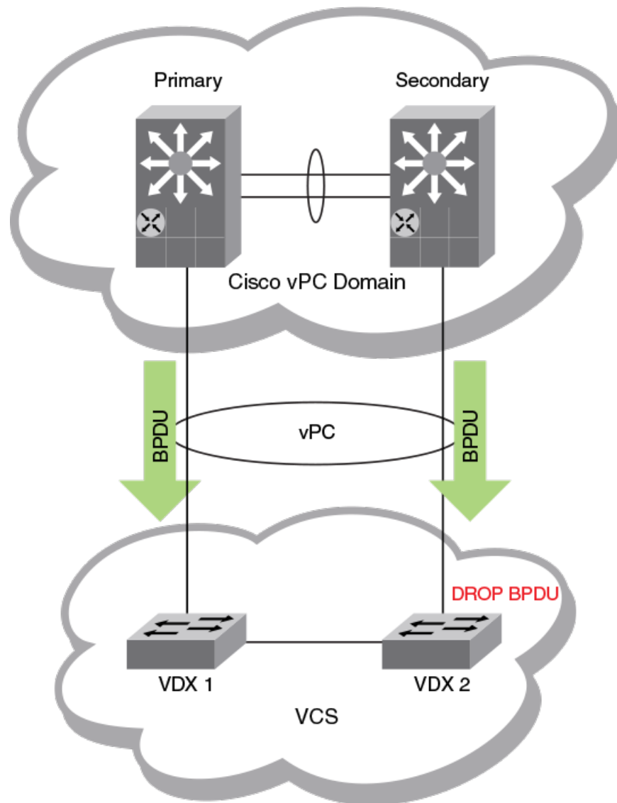
FIGURE 12 STP BPDUs Processing with Peer-Switch
