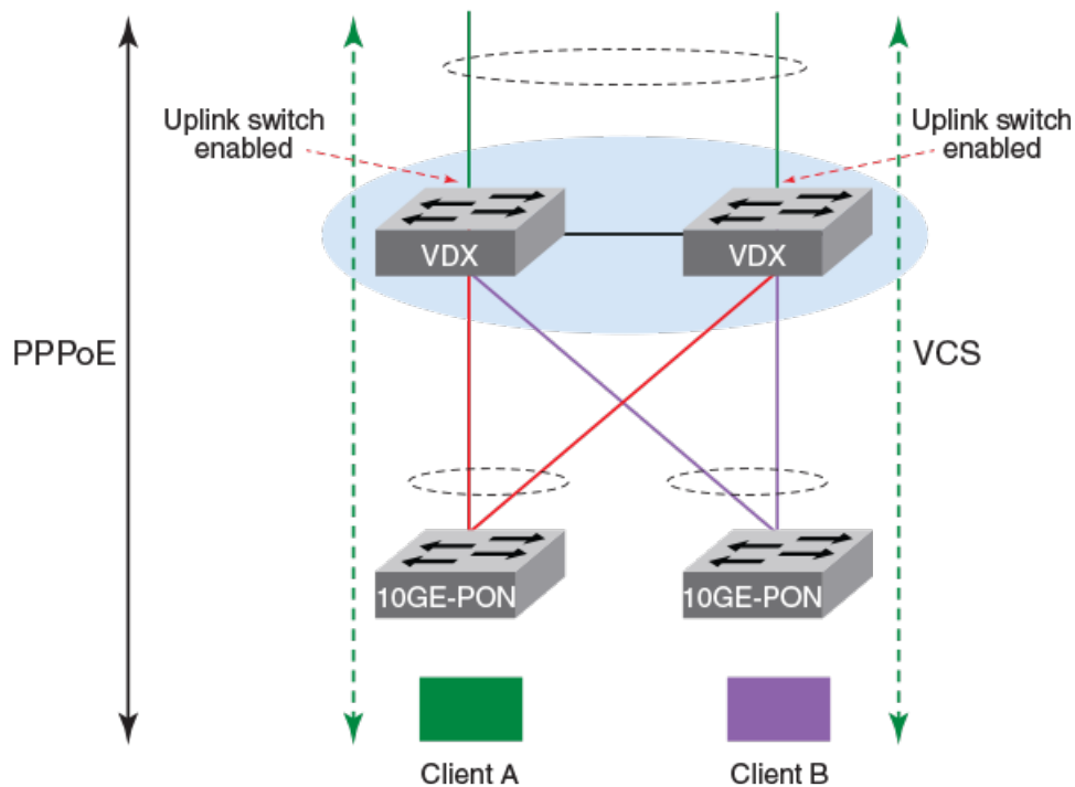
FIGURE 2 Layer 2 traffic between multiple clients and an uplink port
