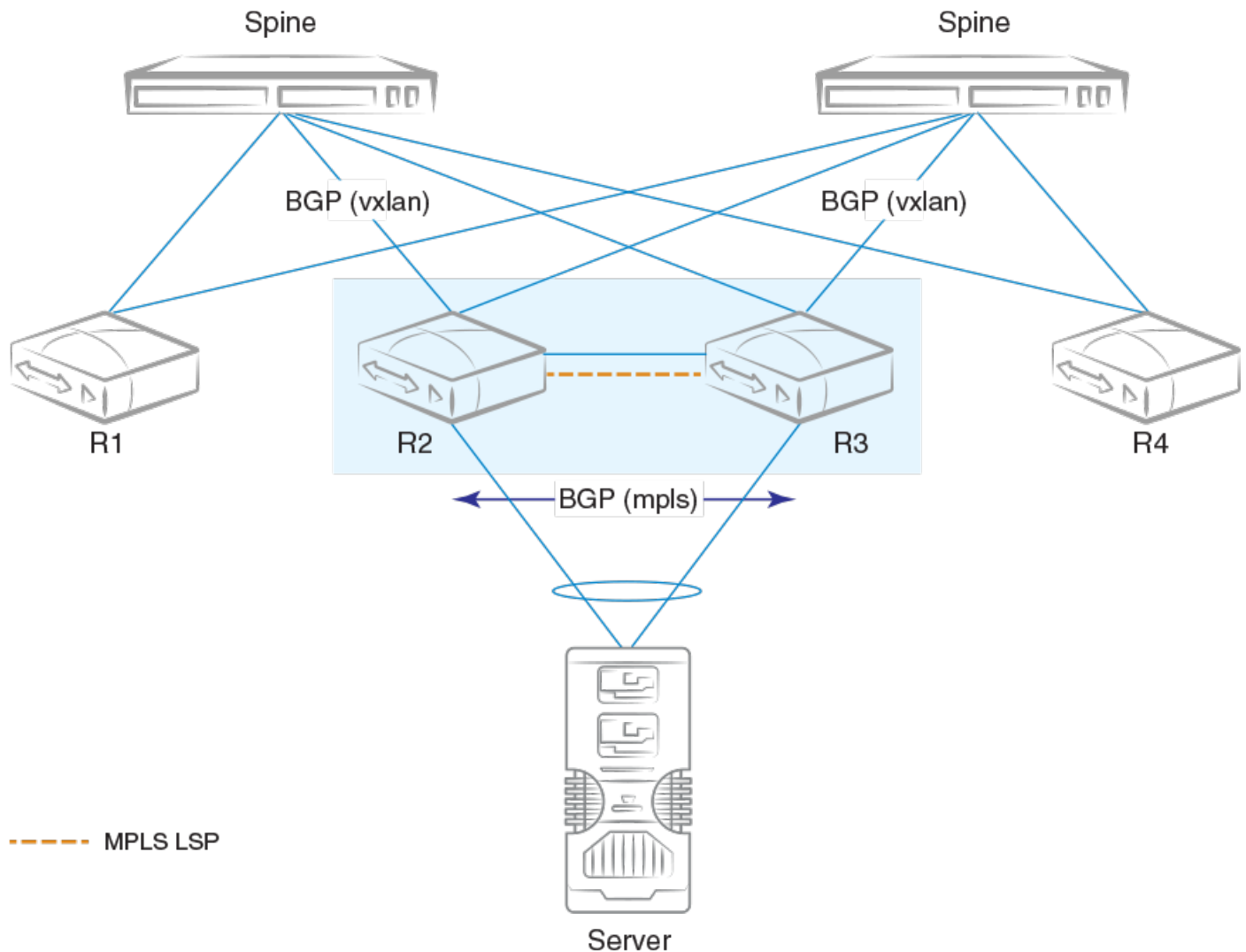
FIGURE 25 MCT with LVTEP and direct BGP peering
