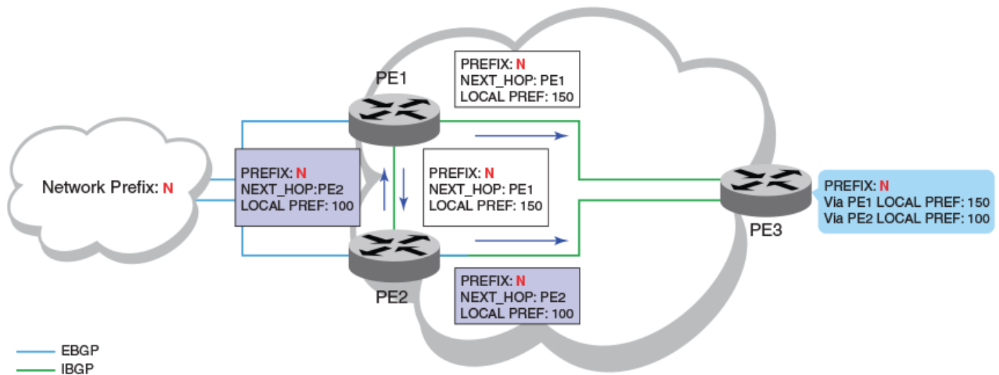
FIGURE 17 BGP best-external configuration
