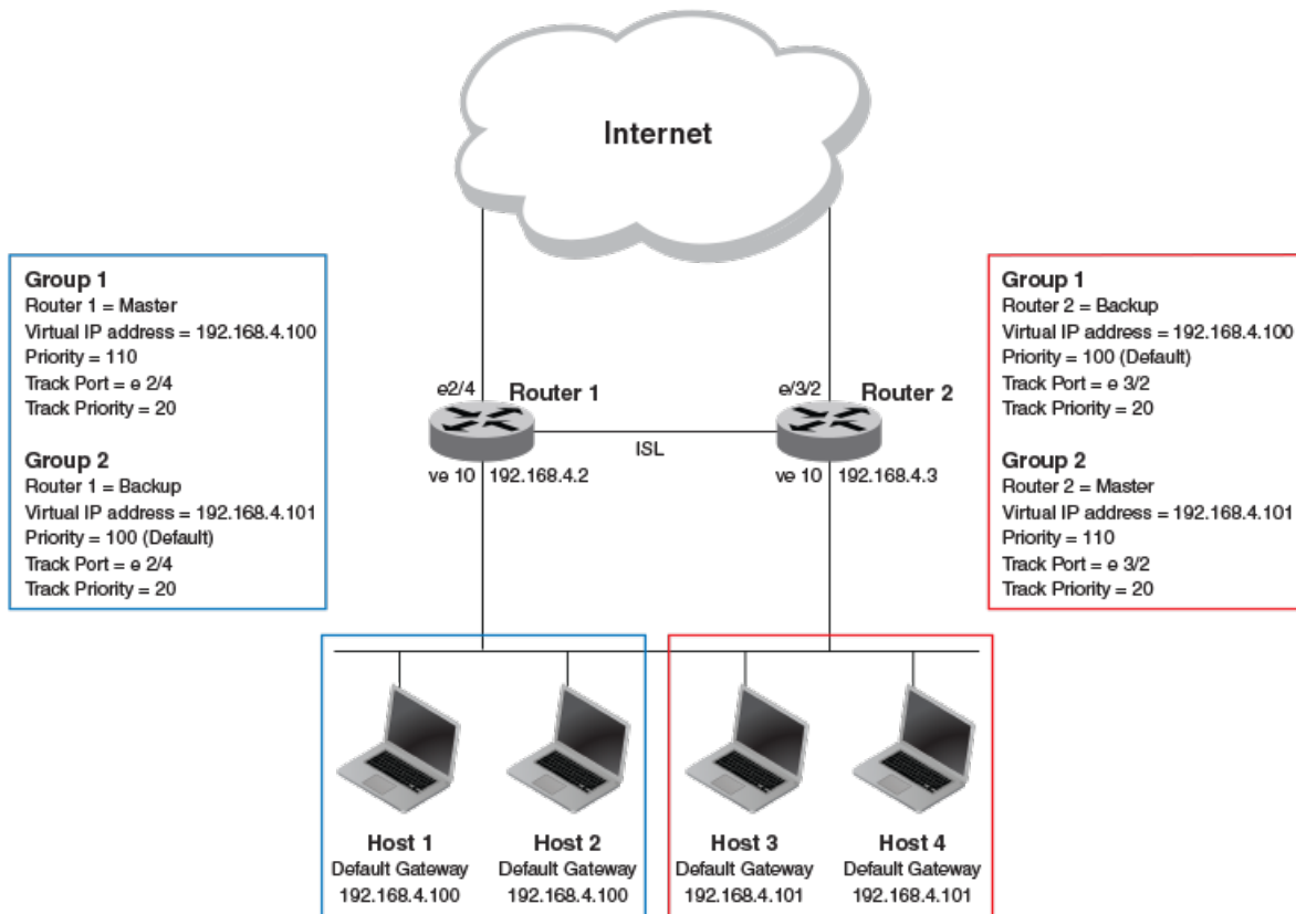
FIGURE 57 Multigroup VRRP routing topology
