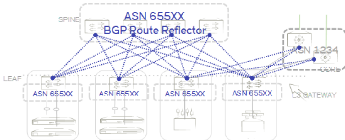
FIGURE 22 iBGP spine and leaf
