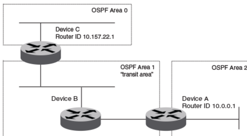
FIGURE 45 Defining OSPF virtual links within a network
