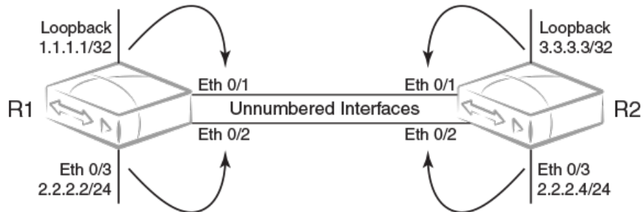
FIGURE 32 IP unnumbered and donor interfaces
