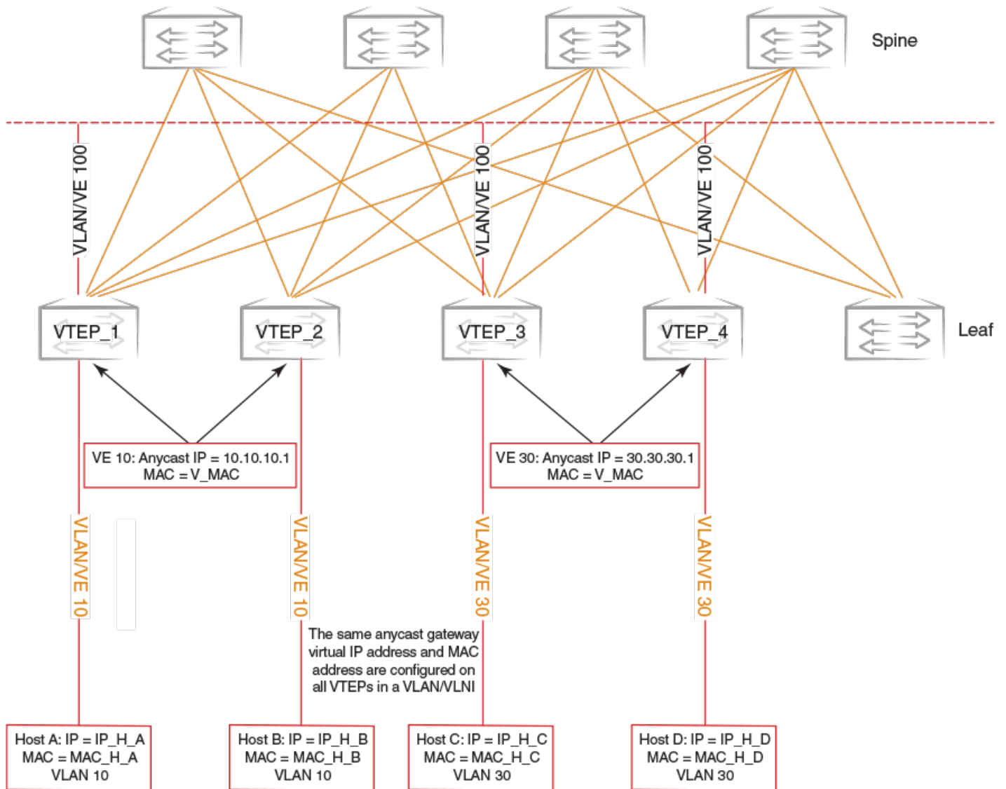
FIGURE 31 Static anycast gateway
