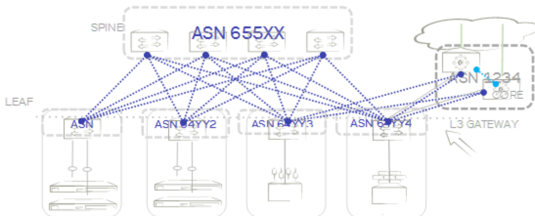
FIGURE 23 eBGP spine and leaf
