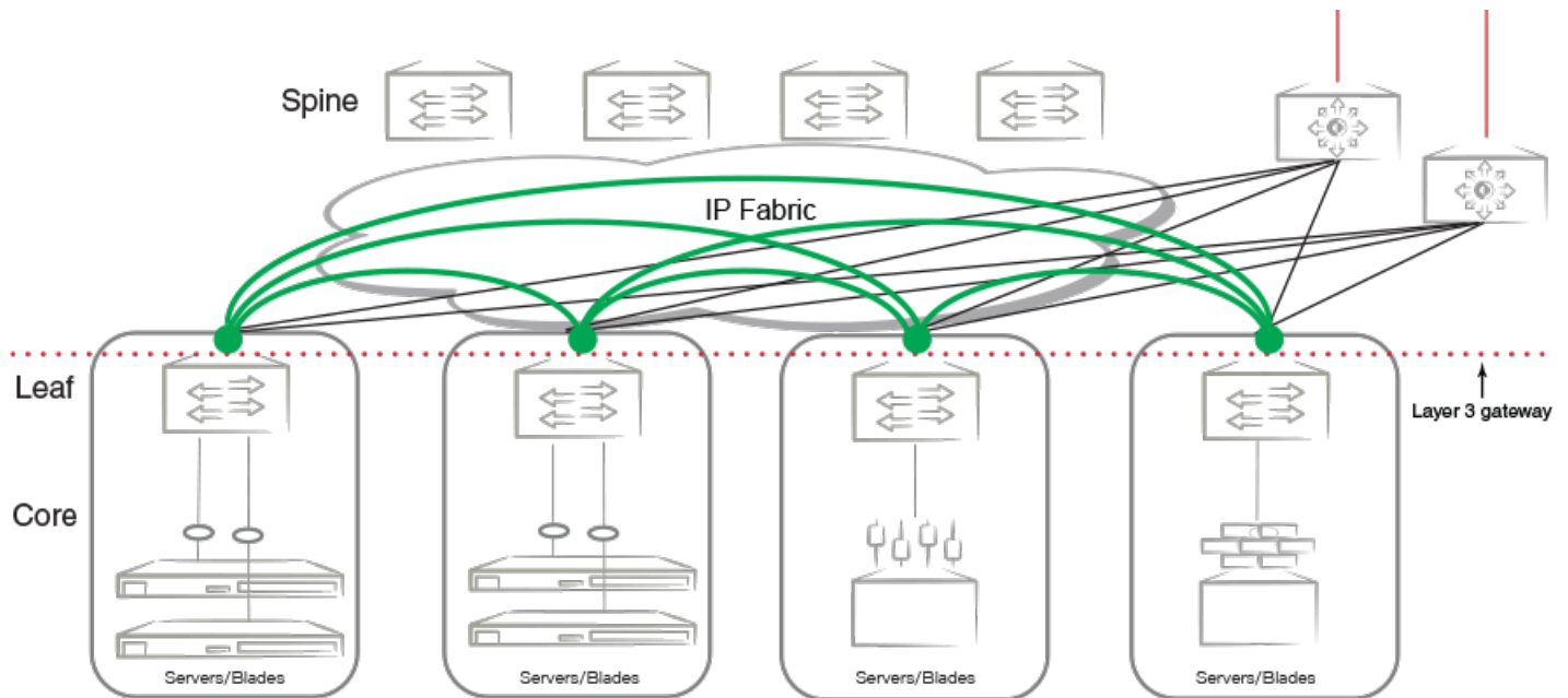
FIGURE 19 VXLAN connectivity in an IP Fabric
