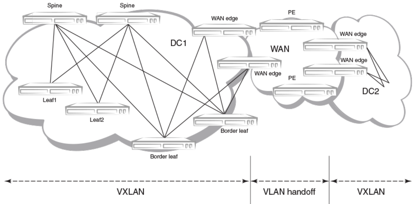
FIGURE 18 Supported BGP EVPN spine topology
