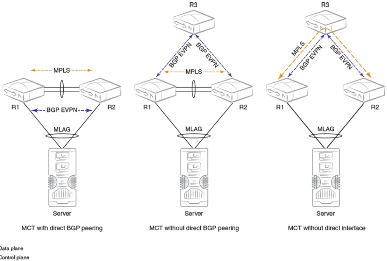
FIGURE 21 MCT use cases
