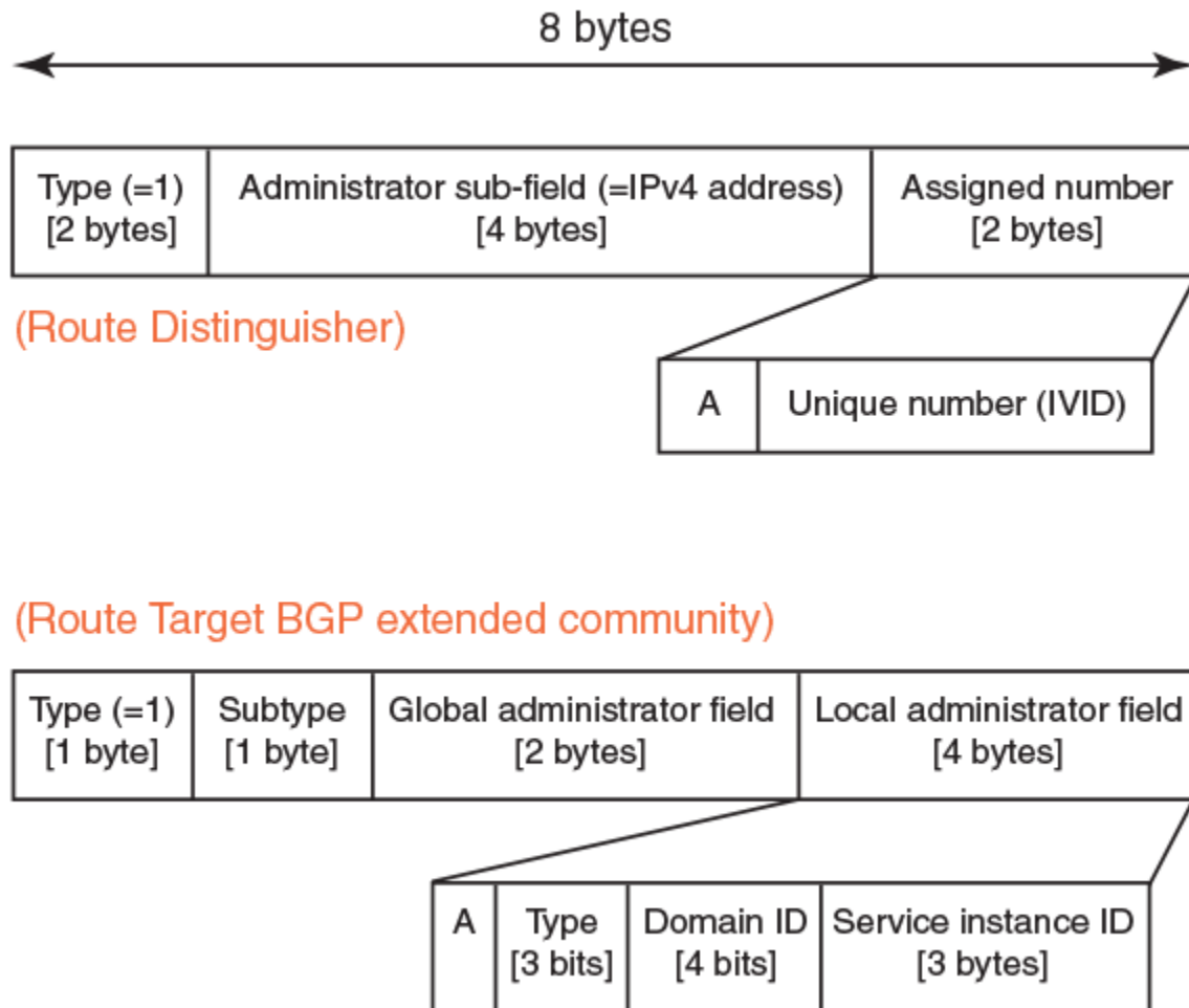
FIGURE 20 RD and RT formats
