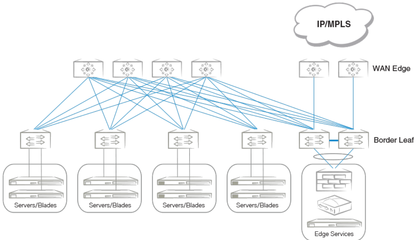
FIGURE 24 Border and service leaf
