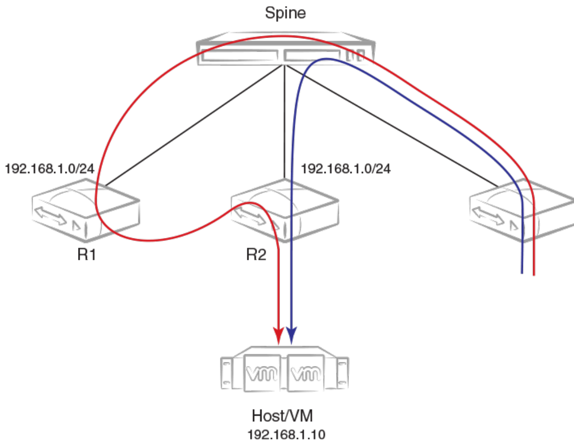
FIGURE 27 Avoiding suboptimal paths by converting MACIP routes to host routes
