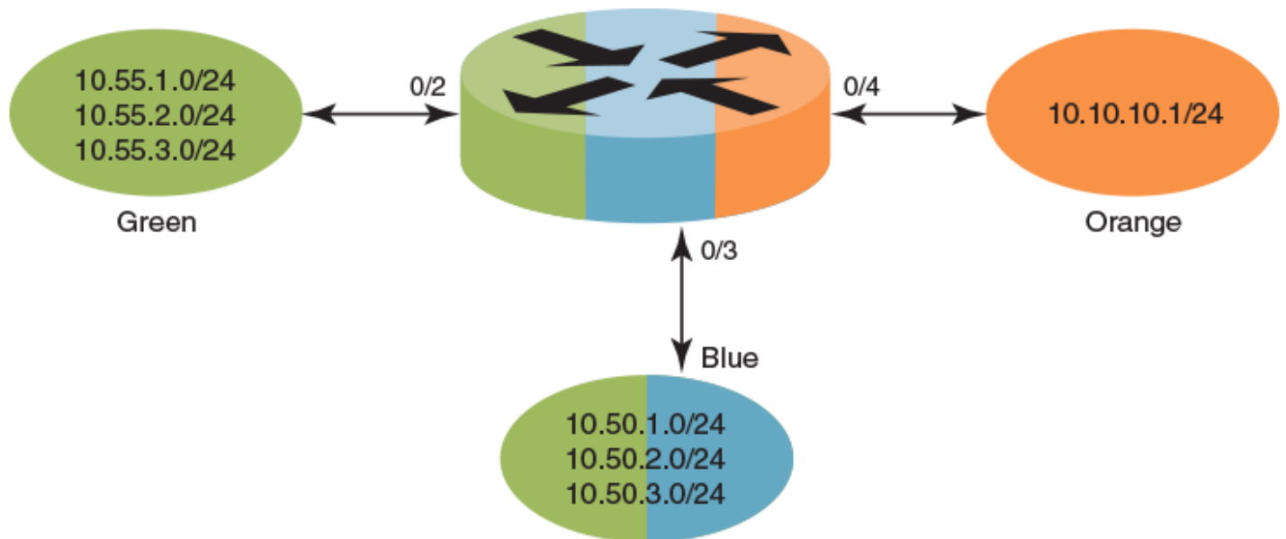
FIGURE 50 Static inter-VRF route leaking
