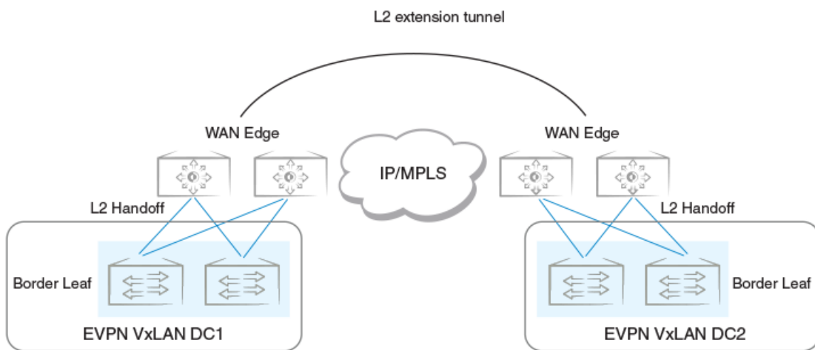
FIGURE 29 Layer 2 handoff-based DCI
