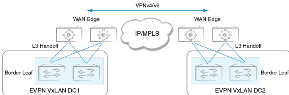
FIGURE 30 Layer 3 handoff-based DCI
