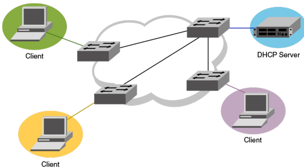
FIGURE 51 Inter-VRF route leaking example for connecting clients to a DHCP server in a different VRF.
