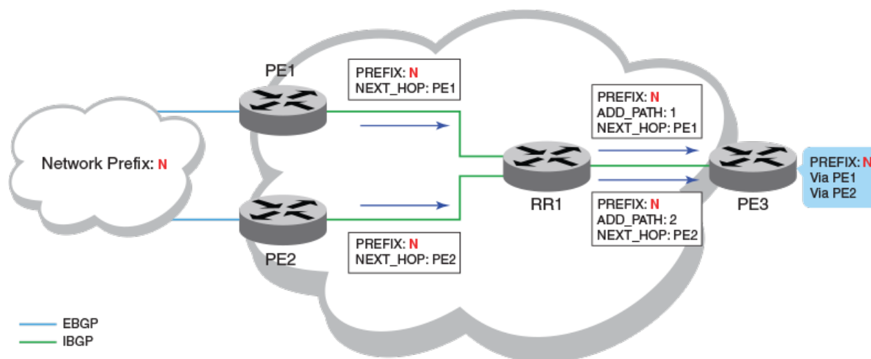
FIGURE 16 BGP additional-paths
