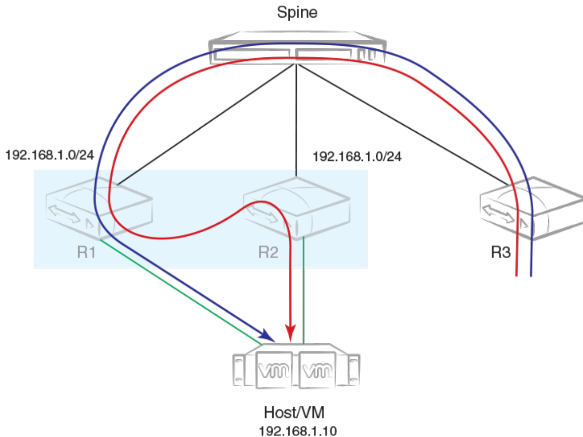
FIGURE 28 Avoiding traffic tromboning for EVPN Layer 3 traffic in an MCT cluster
