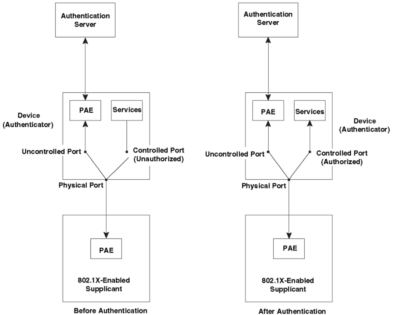
FIGURE 5 Controlled and uncontrolled ports before and after client authentication
