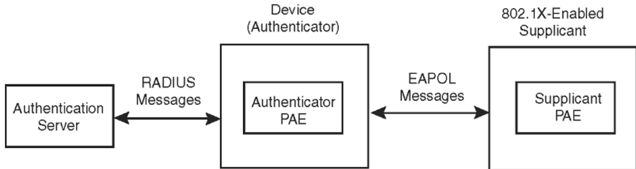
FIGURE 4 Authenticator PAE and supplicant PAE
