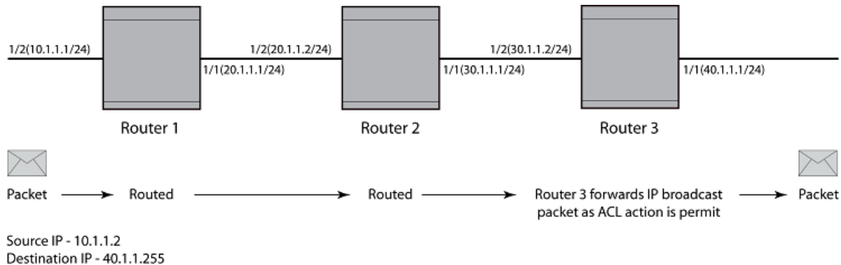
FIGURE 2 Filtering of IP directed broadcast traffic on the Router 3 interface
