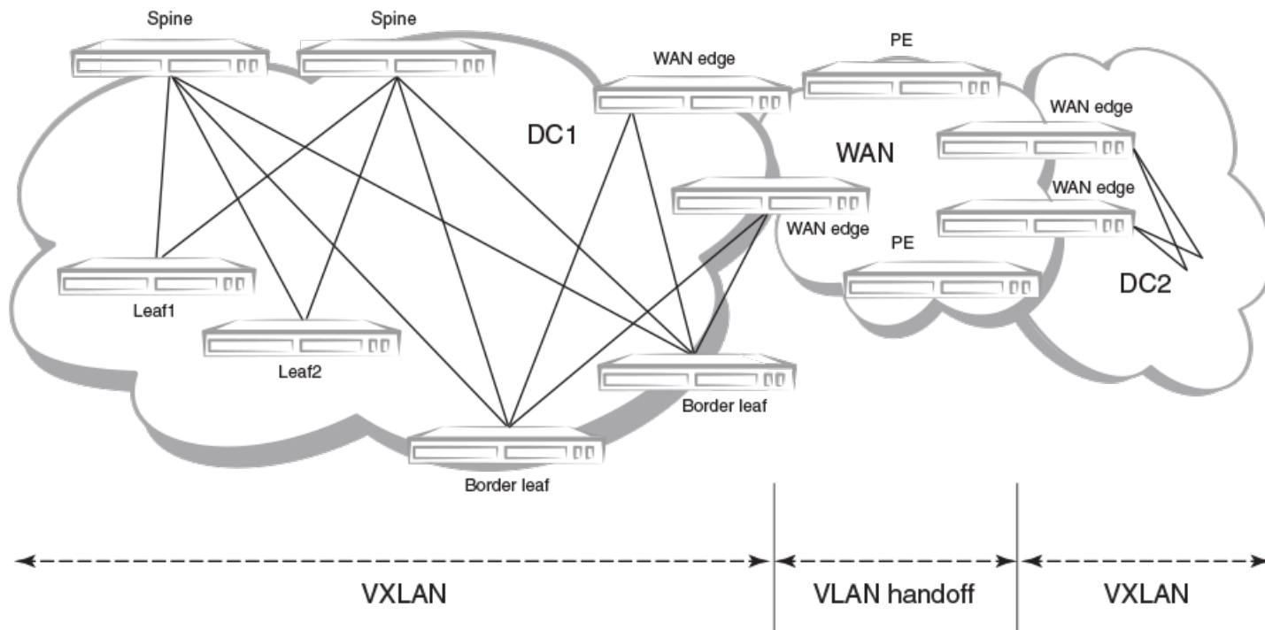
FIGURE 18 Supported BGP EVPN spine topology
