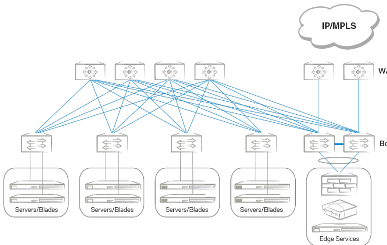
Figure 29: Border and service leaf
