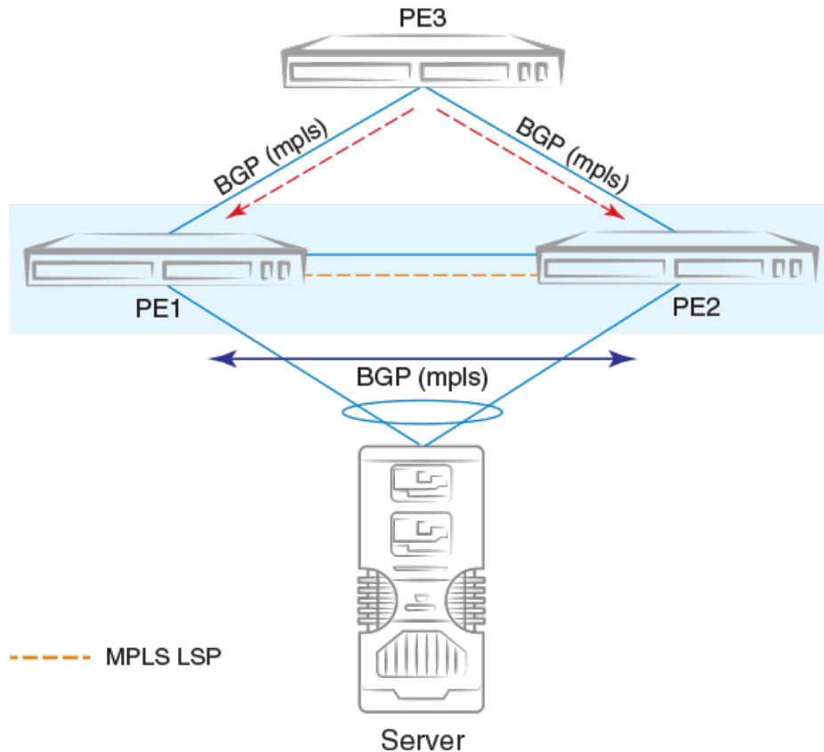
Figure 30: Aliasing in MPLS
