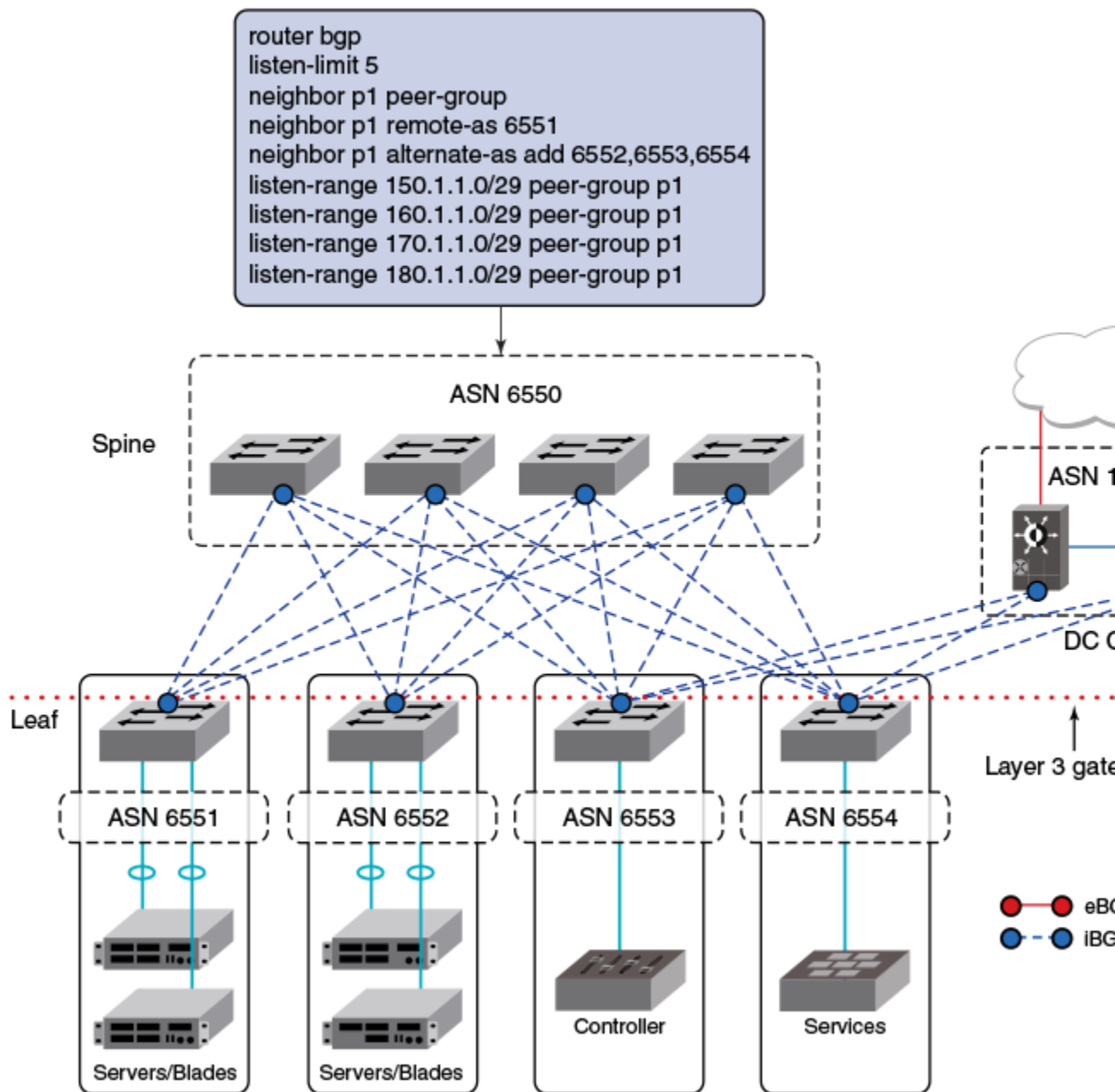
Figure 26: Minimum configuration at the spine level for BGP dynamic neighbors
