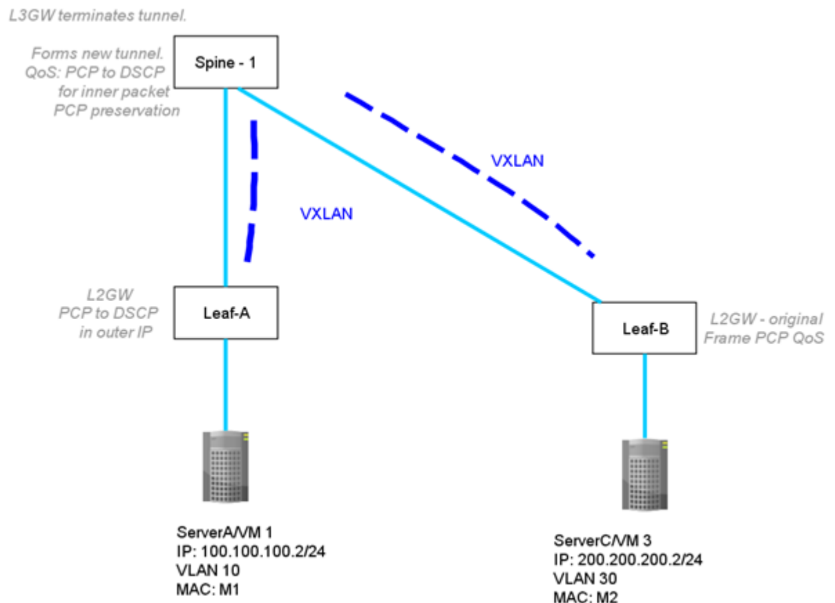
Figure 69: QoS for VXLAN Layer 2 and Layer 3 gateway interconnections
