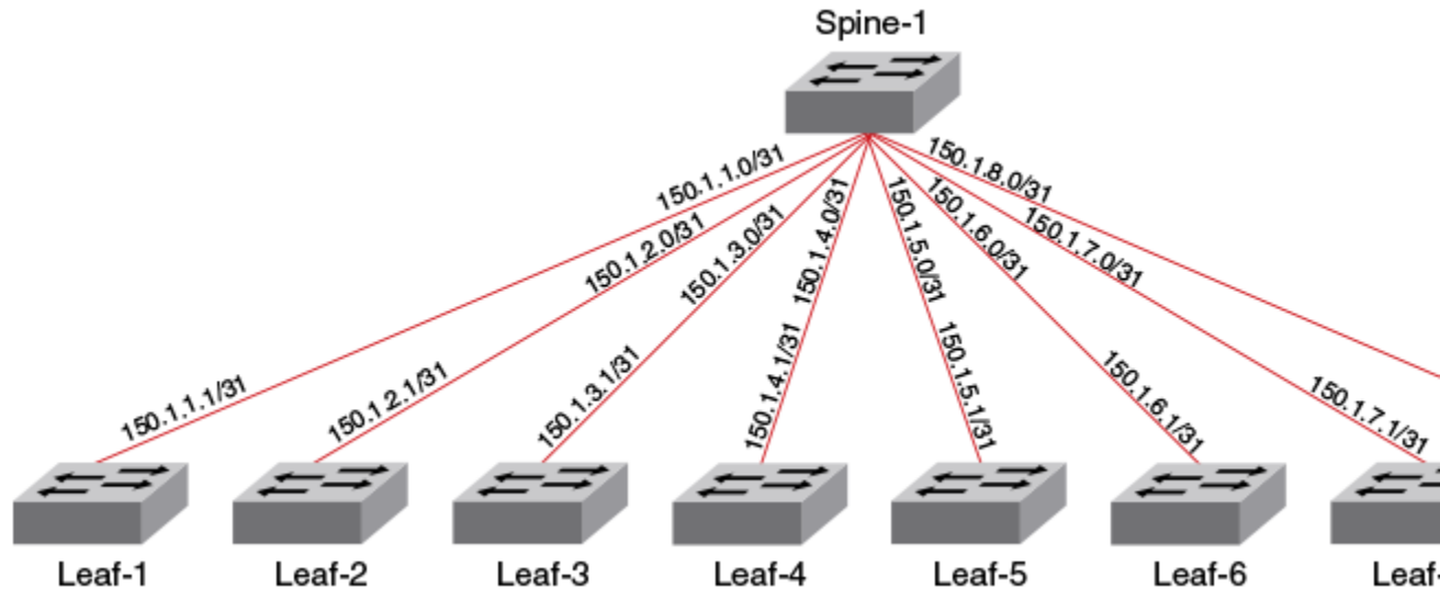
Figure 25: BGP session between spine and leaf nodes
