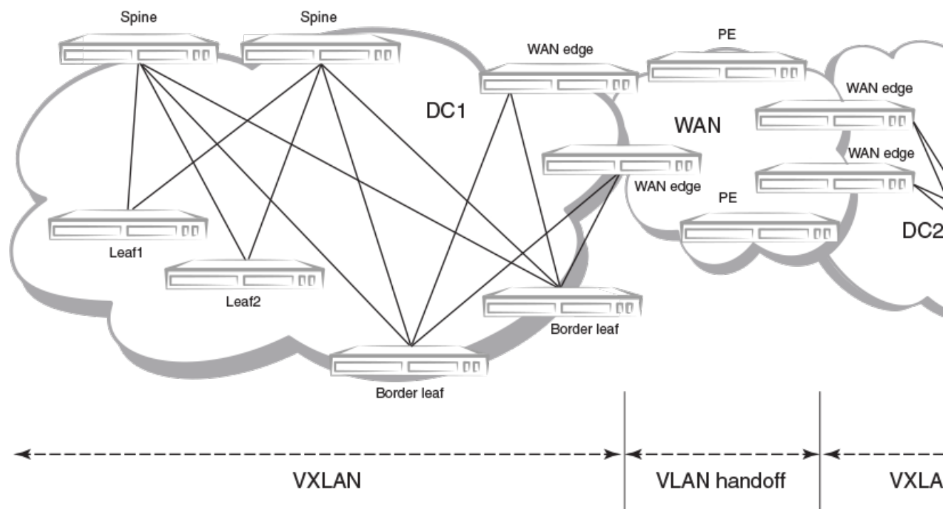
Figure 22: Supported BGP EVPN spine topology
