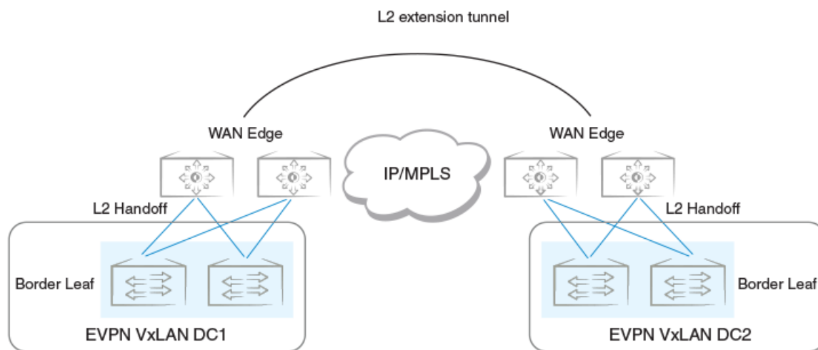
Figure 33: Layer 2 handoff-based DCI
