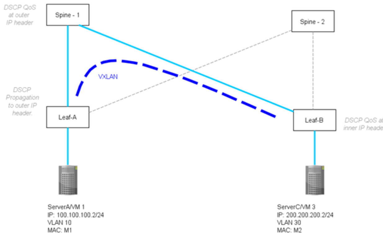
Figure 70: VXLAN L3 gateway support of intersubnet communication
