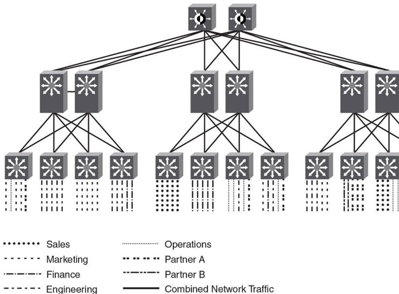
Figure 48: Example high-level Multi-VRF topology
