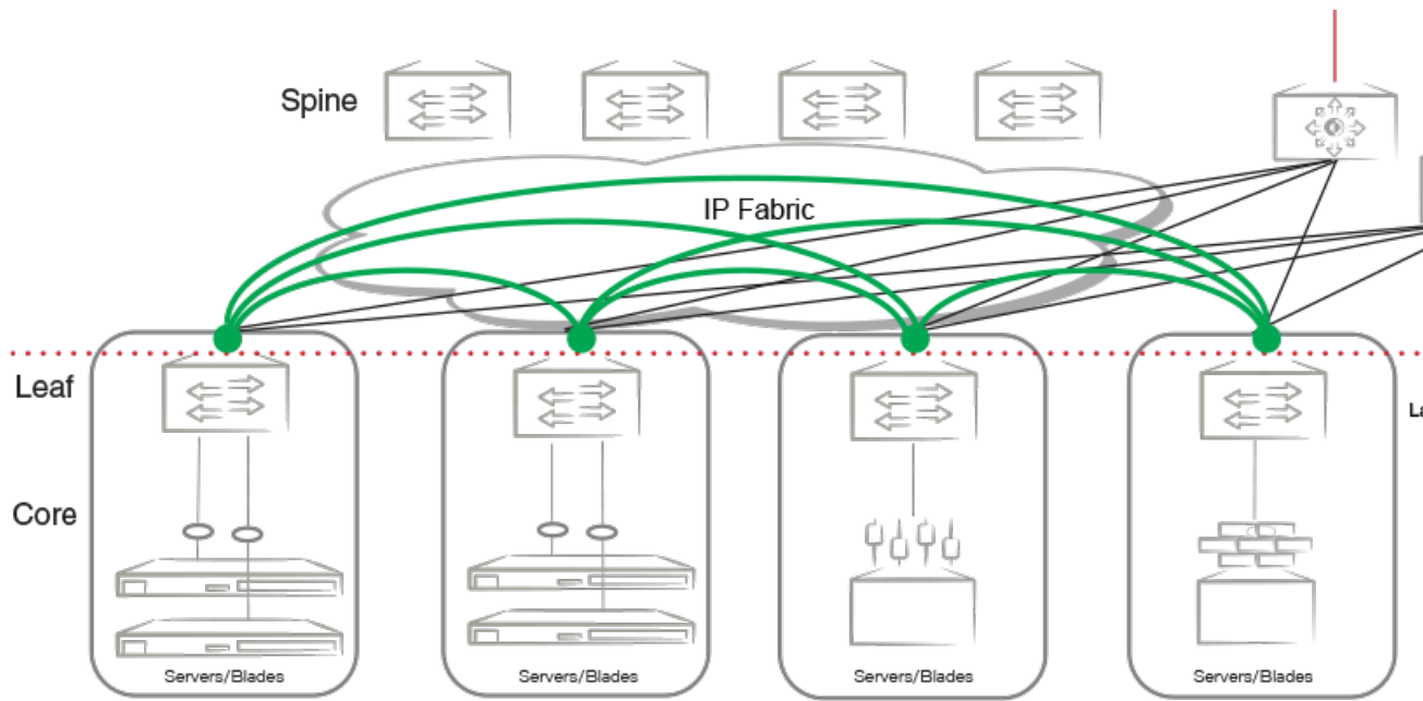
Figure 23: VXLAN connectivity in an IP Fabric
