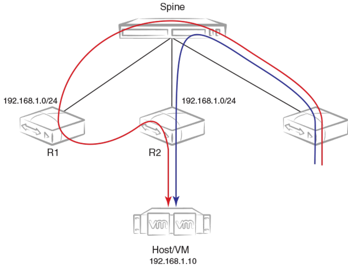
Figure 31: Avoiding suboptimal paths by converting MACIP routes to host routes
