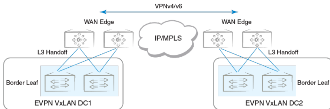
Figure 34: Layer 3 handoff-based DCI
