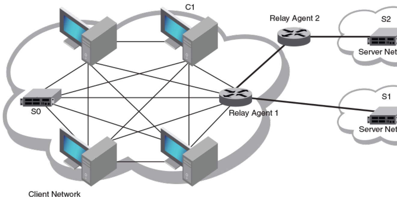
Figure 38: DHCP relay agent user scenarios
