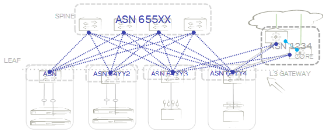
Figure 28: eBGP spine and leaf
