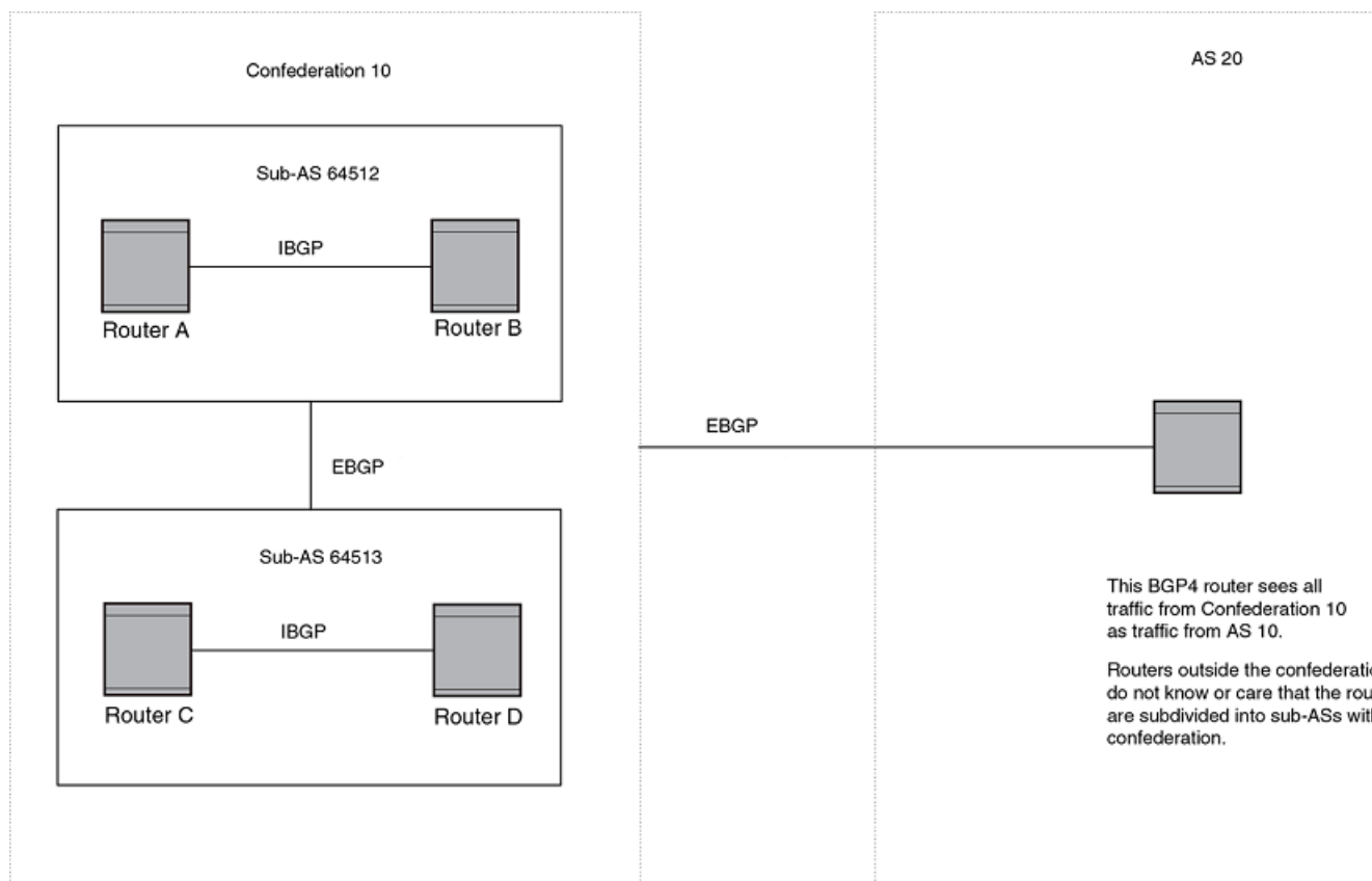
Figure 12: Example BGP4 confederation
