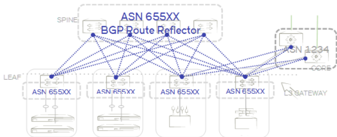
Figure 27: iBGP spine and leaf
